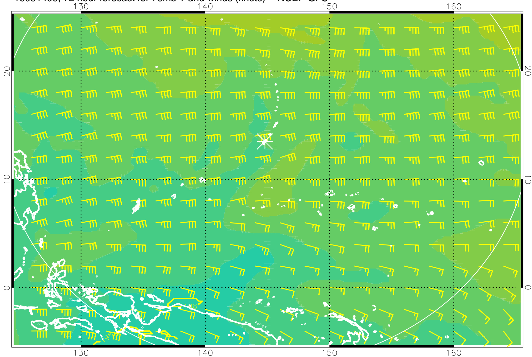
16081400, 72 hour forecast for 70mb T and winds (knots) -- NCEP GFS
