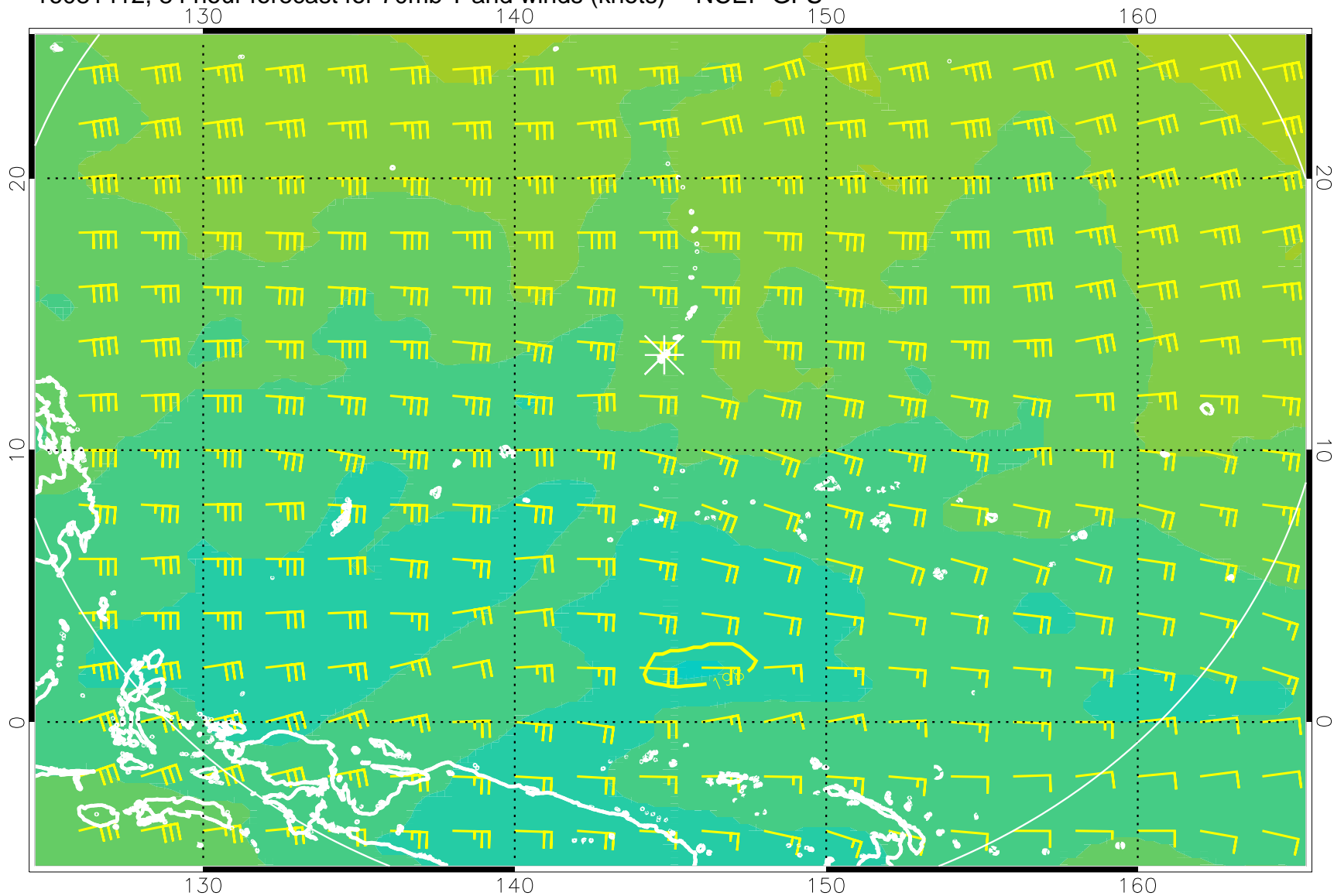
16081412, 84 hour forecast for 70mb T and winds (knots) -- NCEP GFS
