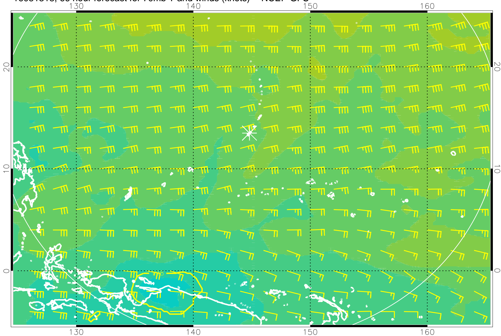
16081318, 66 hour forecast for 70mb T and winds (knots) -- NCEP GFS
