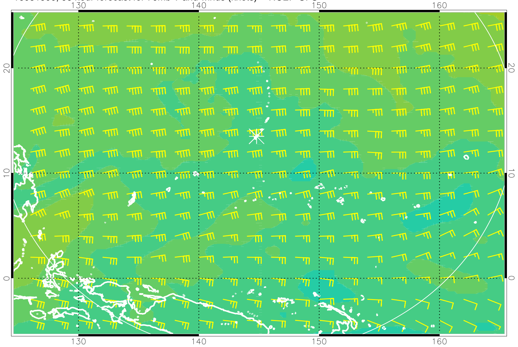
16081500, 96 hour forecast for 70mb T and winds (knots) -- NCEP GFS
