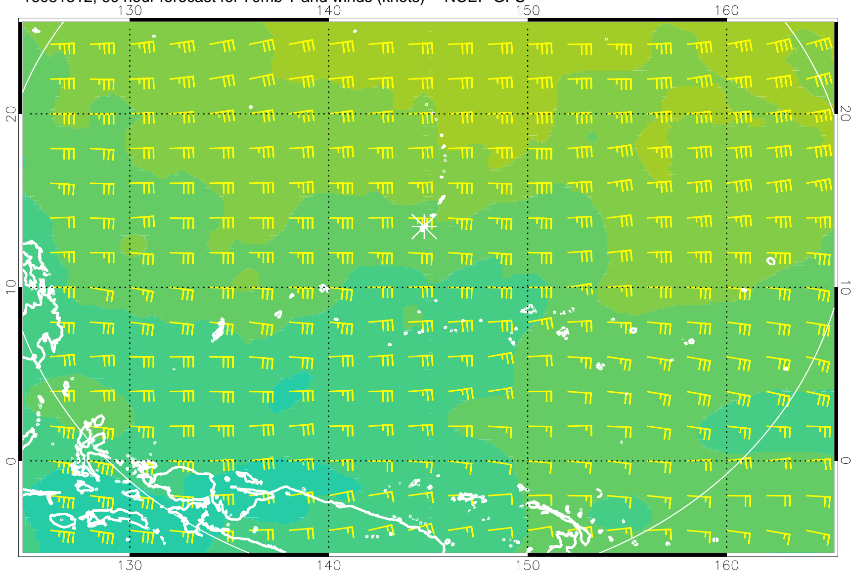
16081312, 60 hour forecast for 70mb T and winds (knots) -- NCEP GFS
