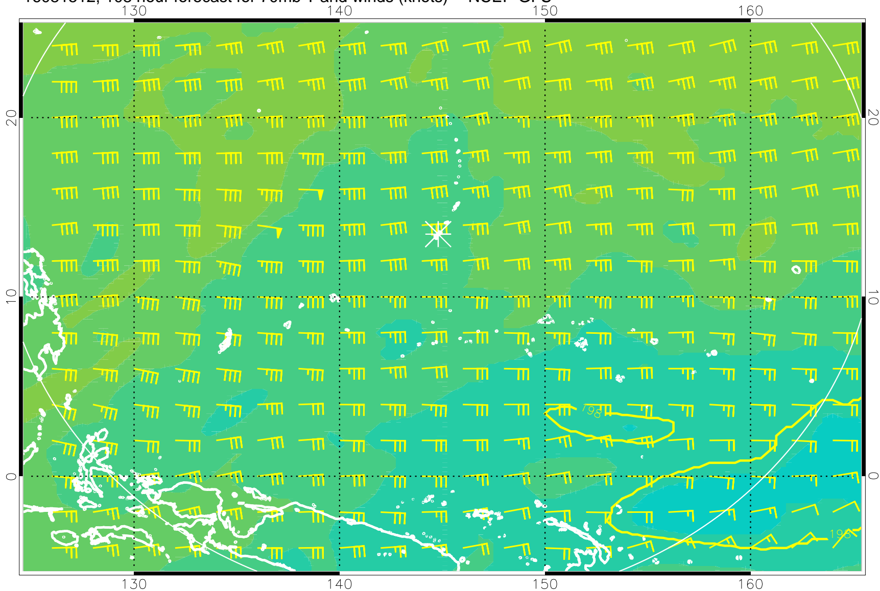
16081512, 108 hour forecast for 70mb T and winds (knots) -- NCEP GFS
