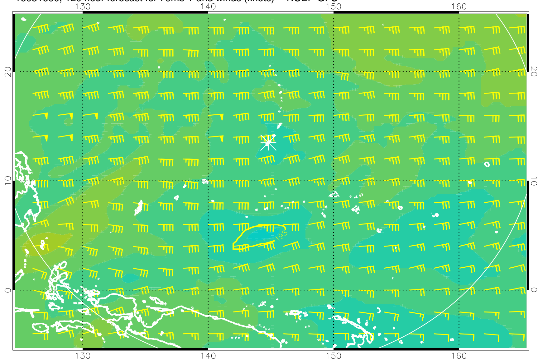
16081600, 120 hour forecast for 70mb T and winds (knots) -- NCEP GFS
