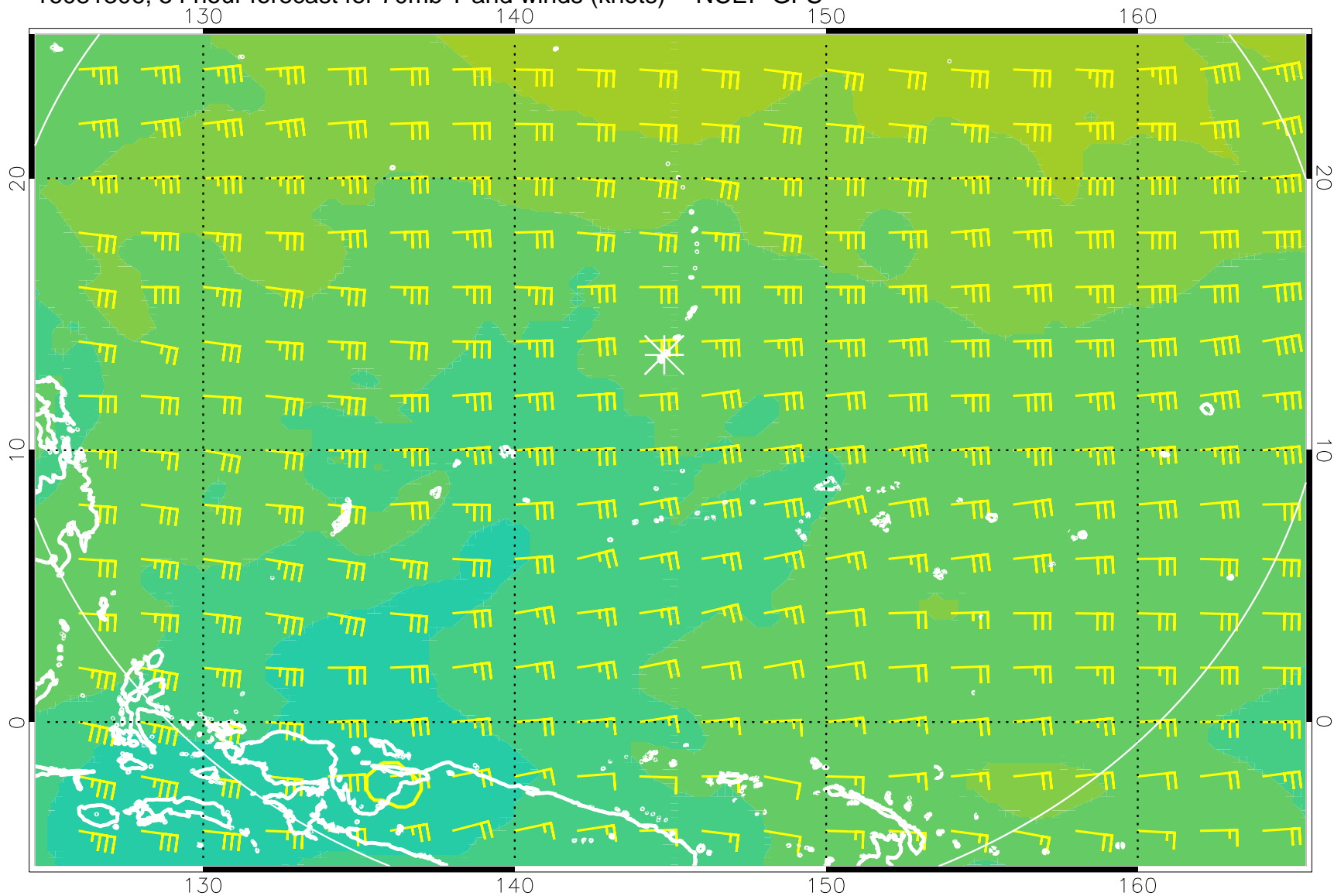
16081306, 54 hour forecast for 70mb T and winds (knots) -- NCEP GFS
