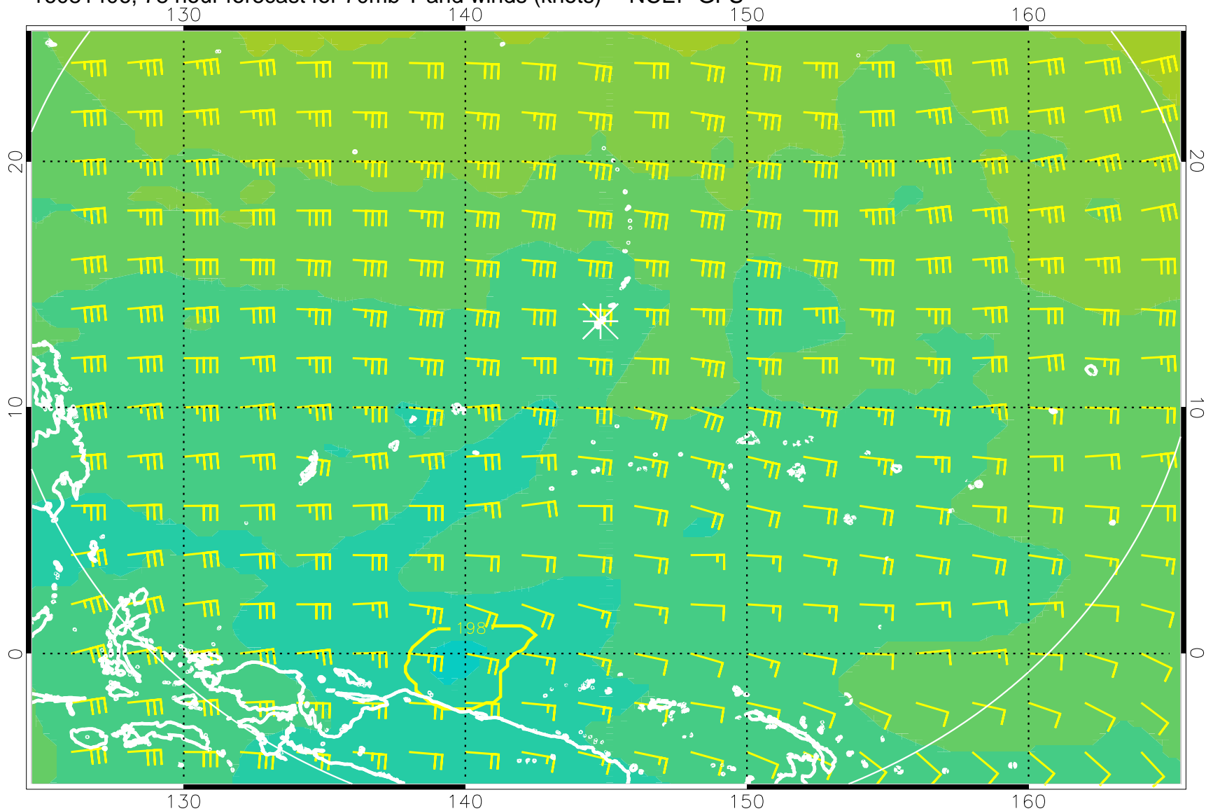
16081406, 78 hour forecast for 70mb T and winds (knots) -- NCEP GFS
