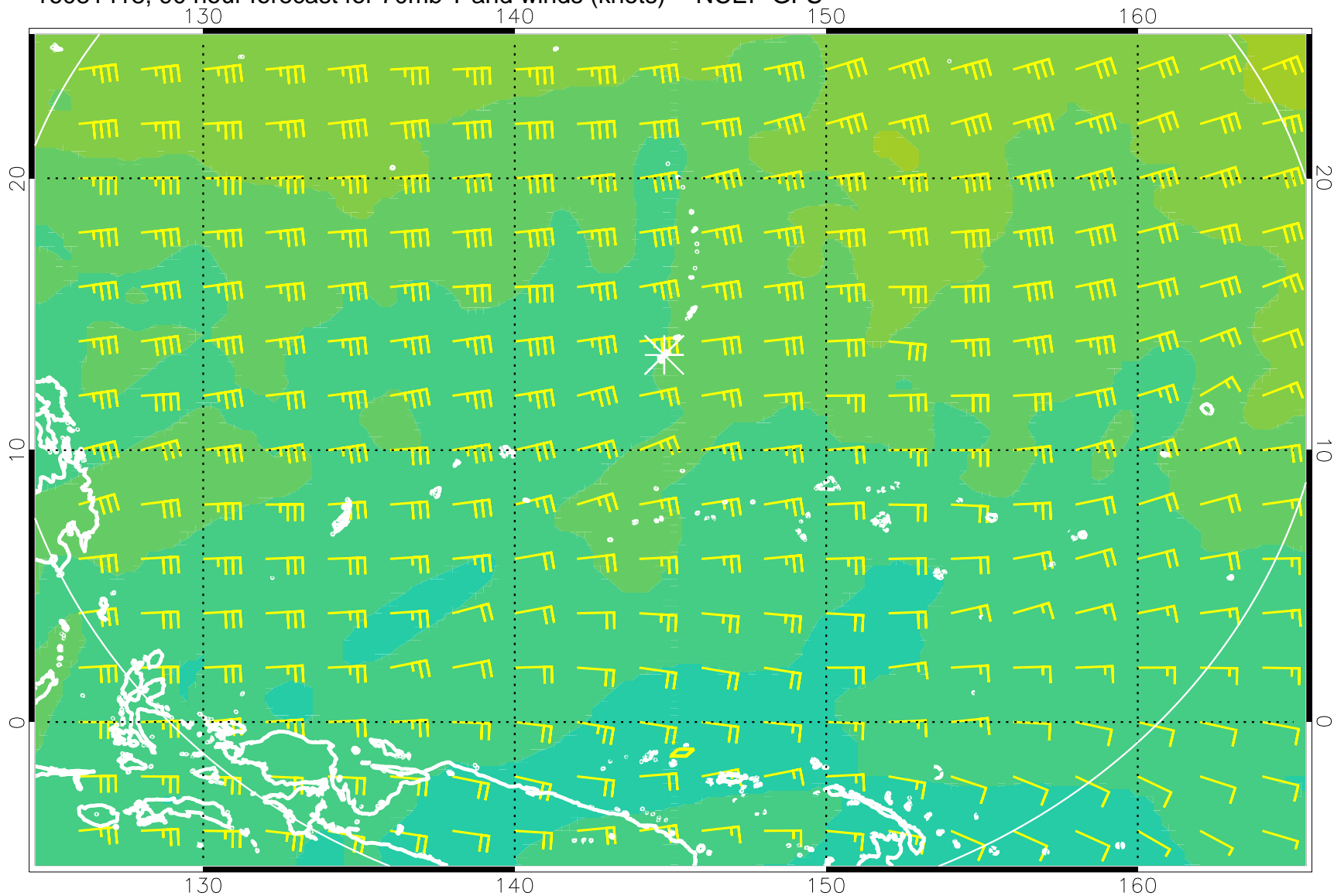
16081418, 90 hour forecast for 70mb T and winds (knots) -- NCEP GFS
