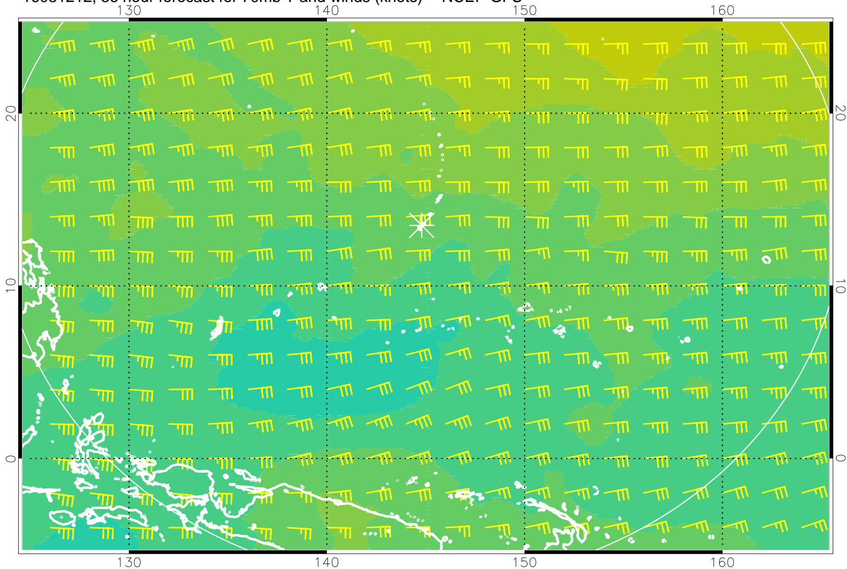
16081212, 36 hour forecast for 70mb T and winds (knots) -- NCEP GFS
