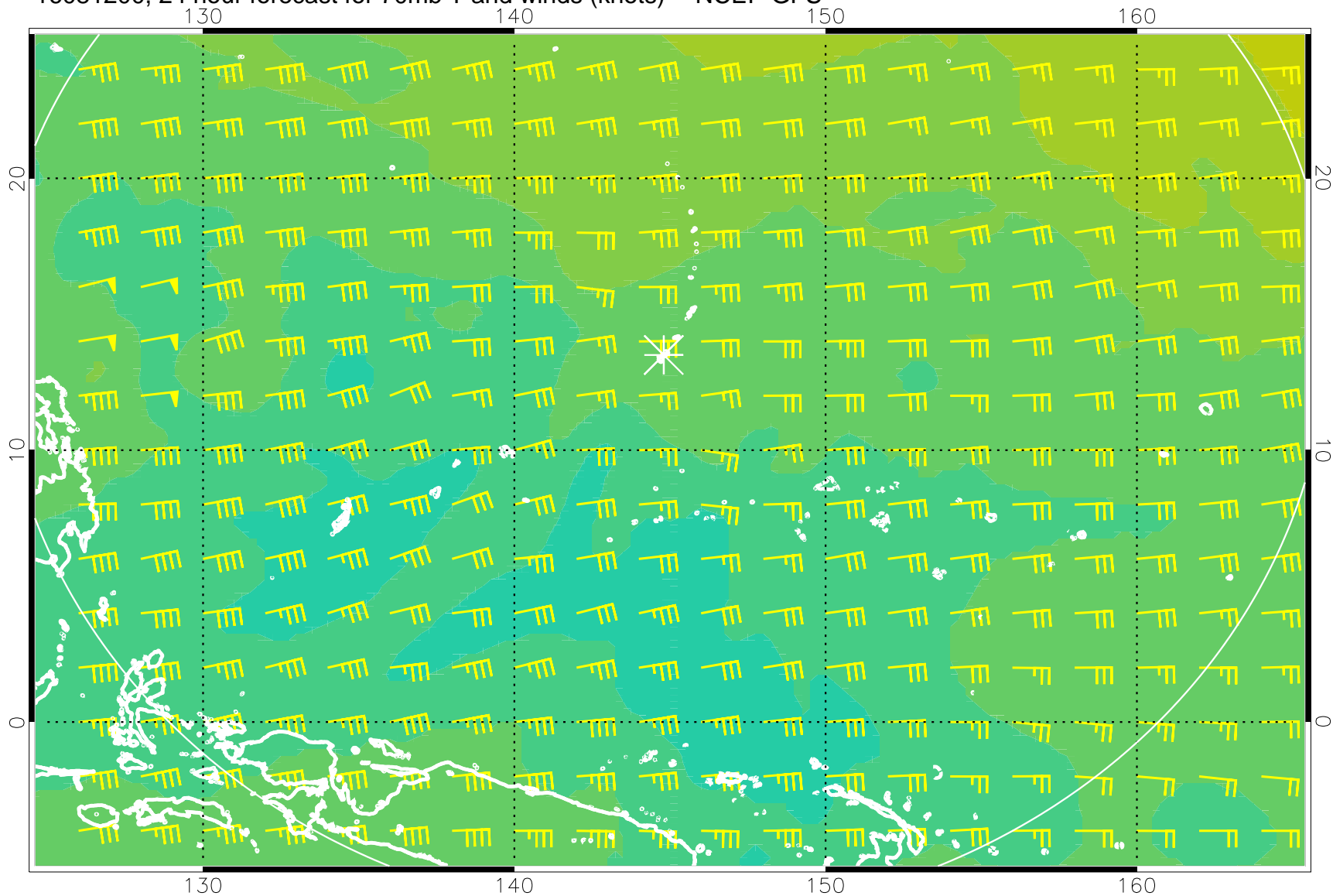
16081200, 24 hour forecast for 70mb T and winds (knots) -- NCEP GFS
