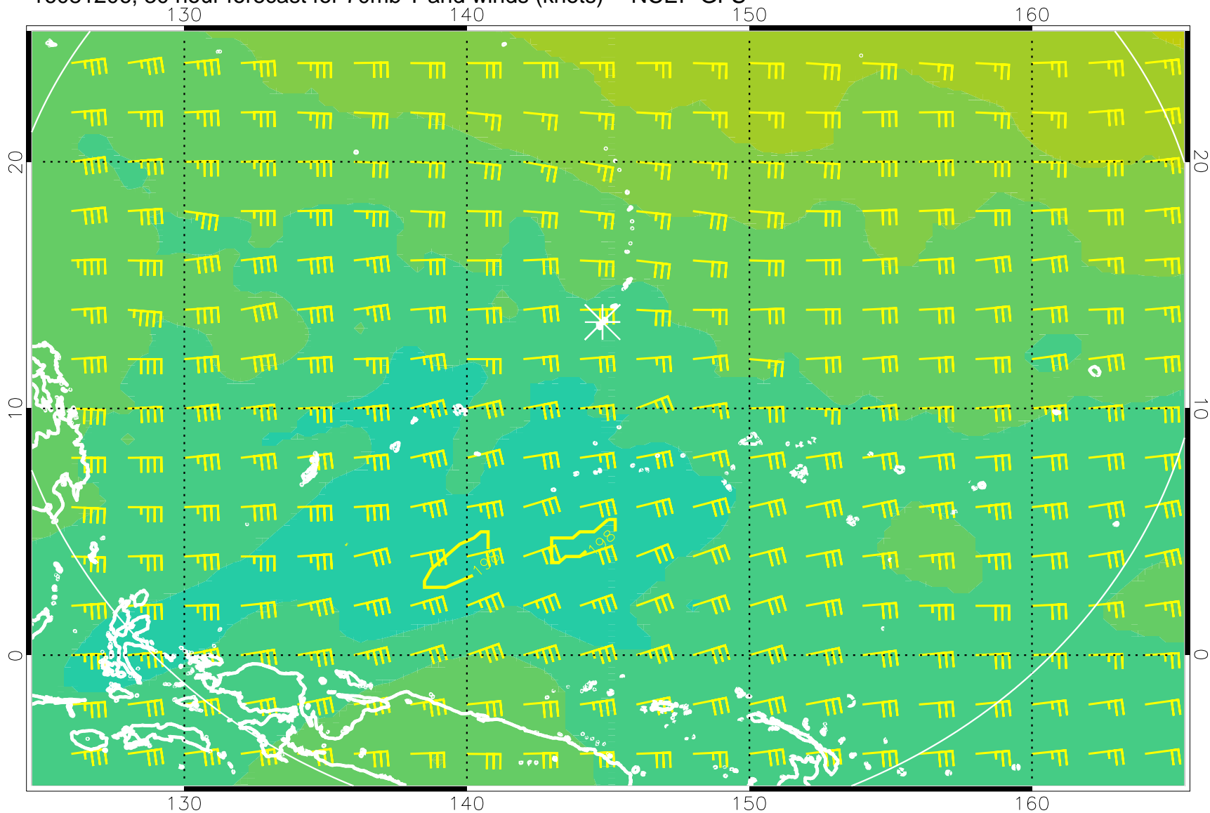
16081206, 30 hour forecast for 70mb T and winds (knots) -- NCEP GFS
