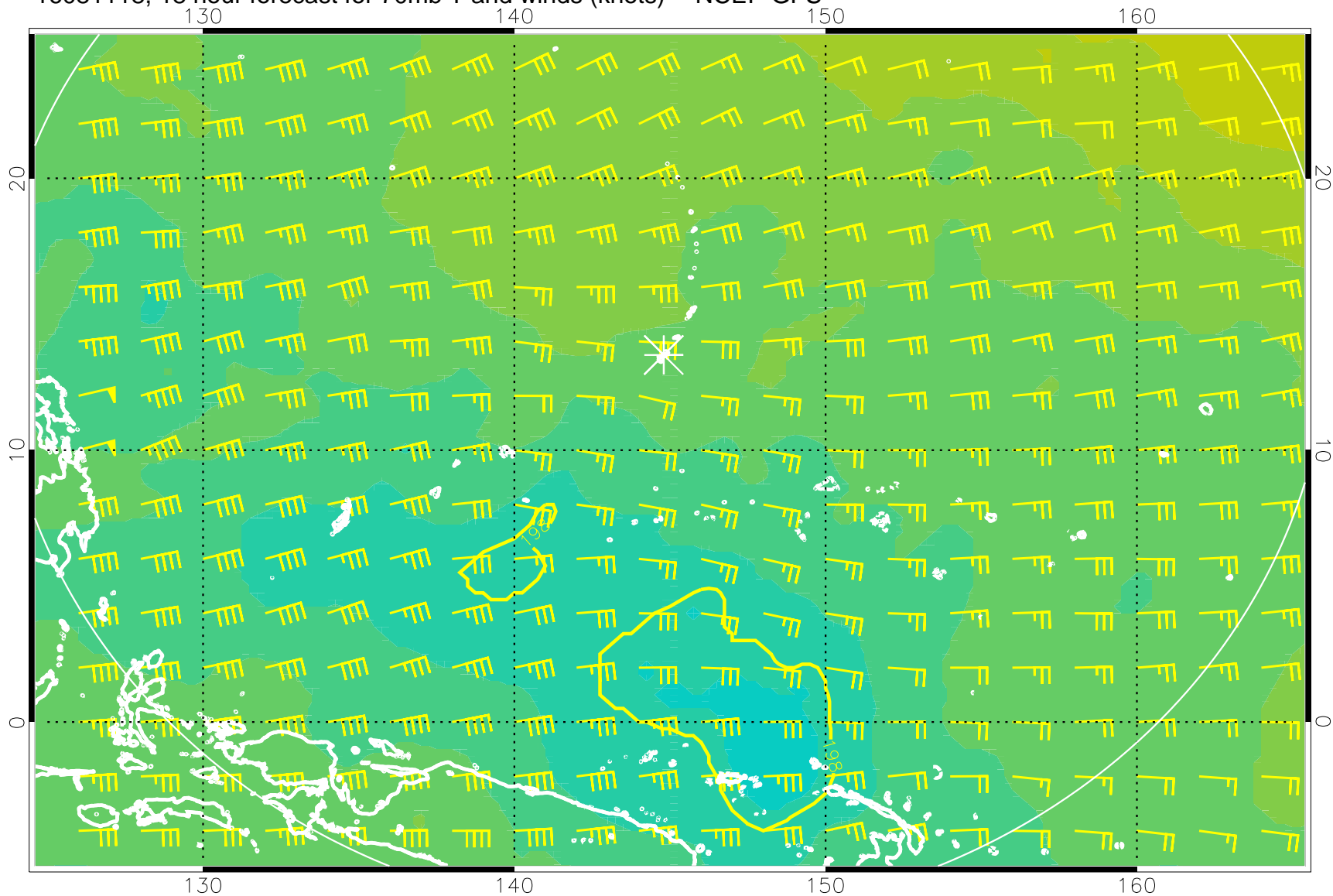
16081118, 18 hour forecast for 70mb T and winds (knots) -- NCEP GFS
