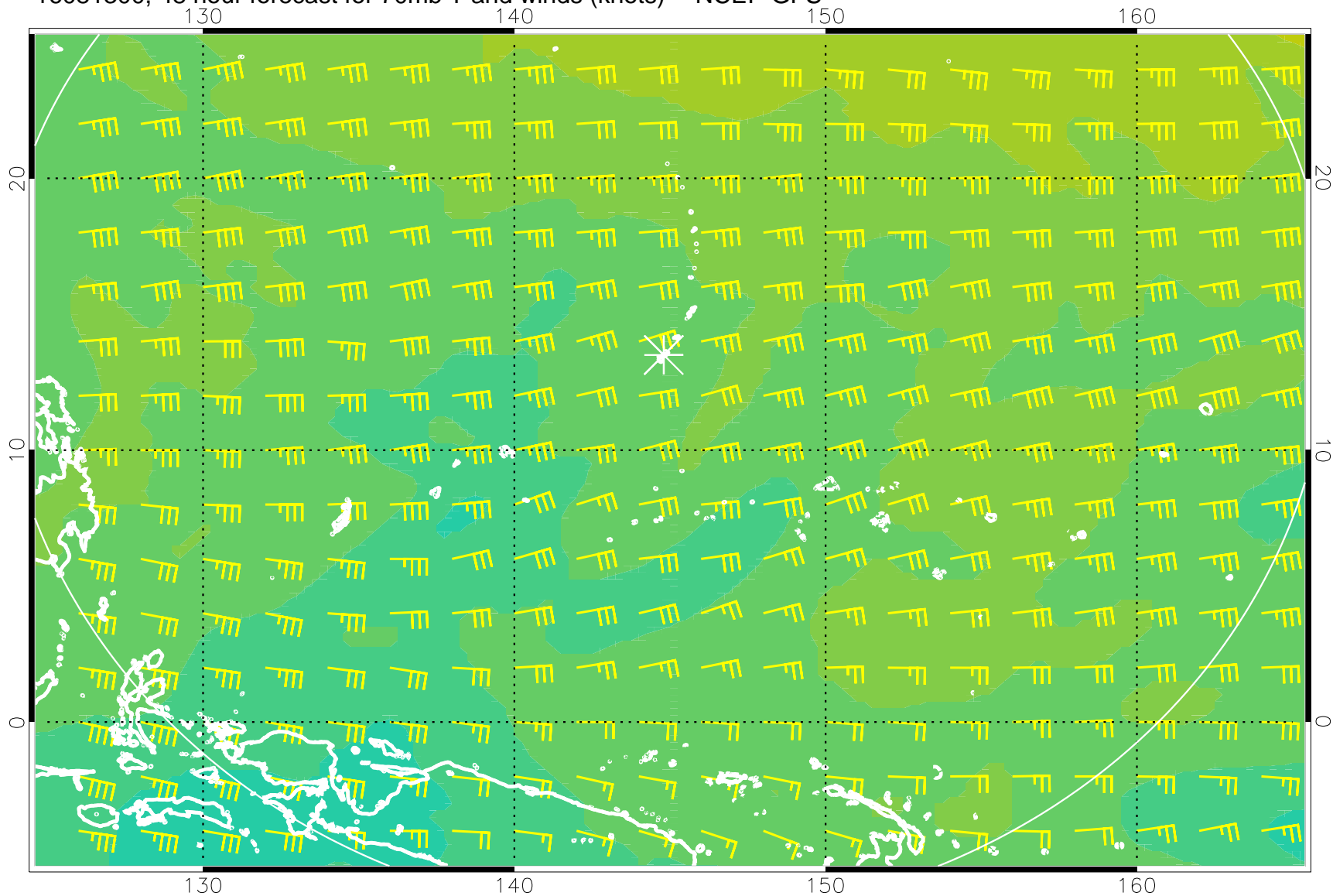
16081300, 48 hour forecast for 70mb T and winds (knots) -- NCEP GFS
