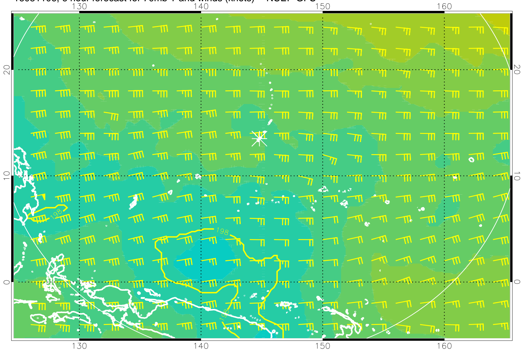
16081106, 6 hour forecast for 70mb T and winds (knots) -- NCEP GFS
