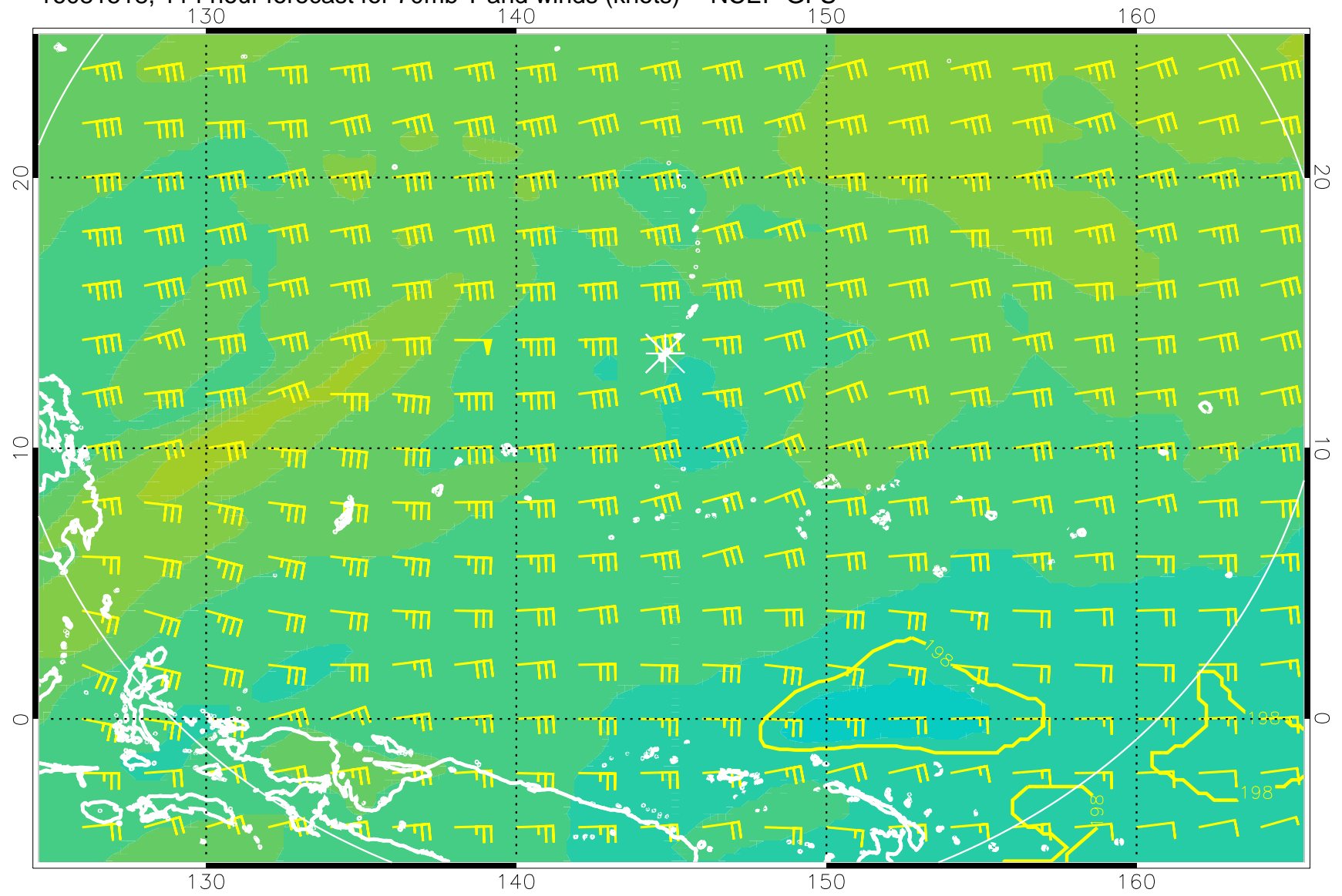
16081518, 114 hour forecast for 70mb T and winds (knots) -- NCEP GFS
