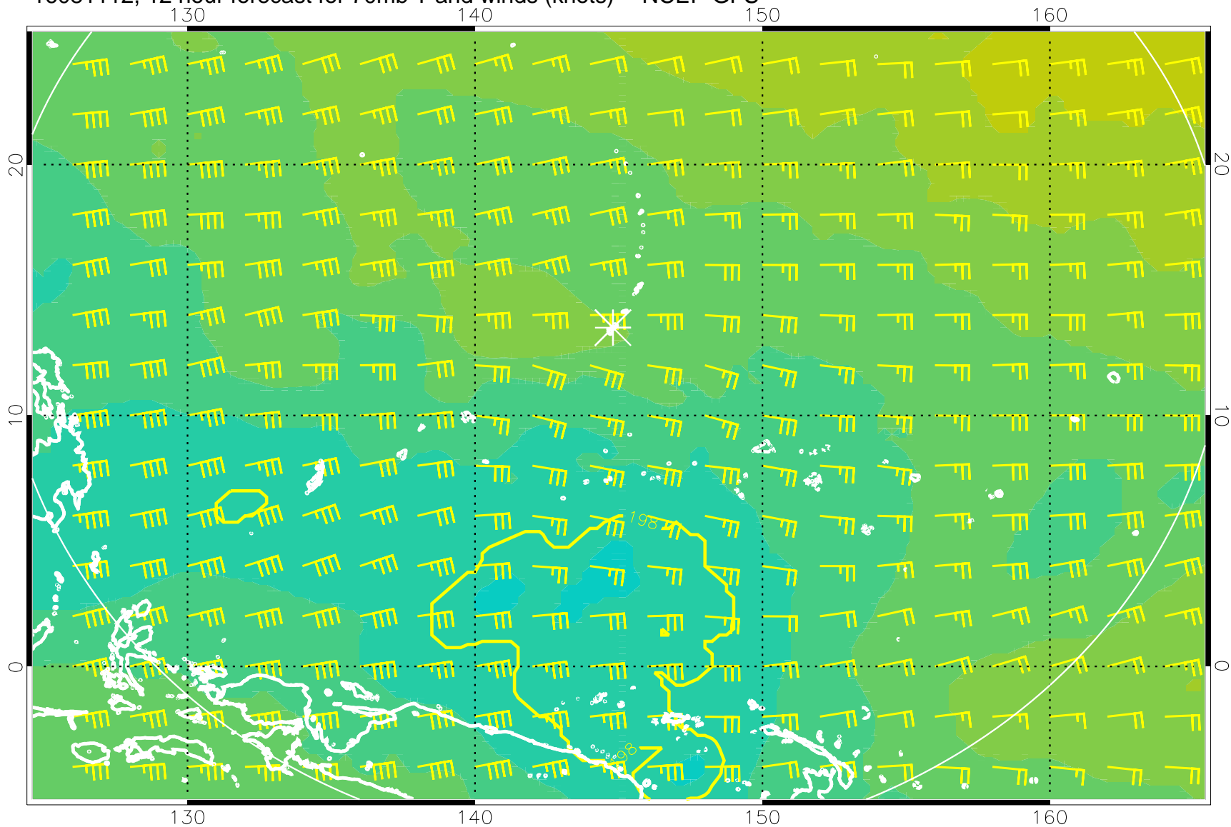
16081112, 12 hour forecast for 70mb T and winds (knots) -- NCEP GFS
