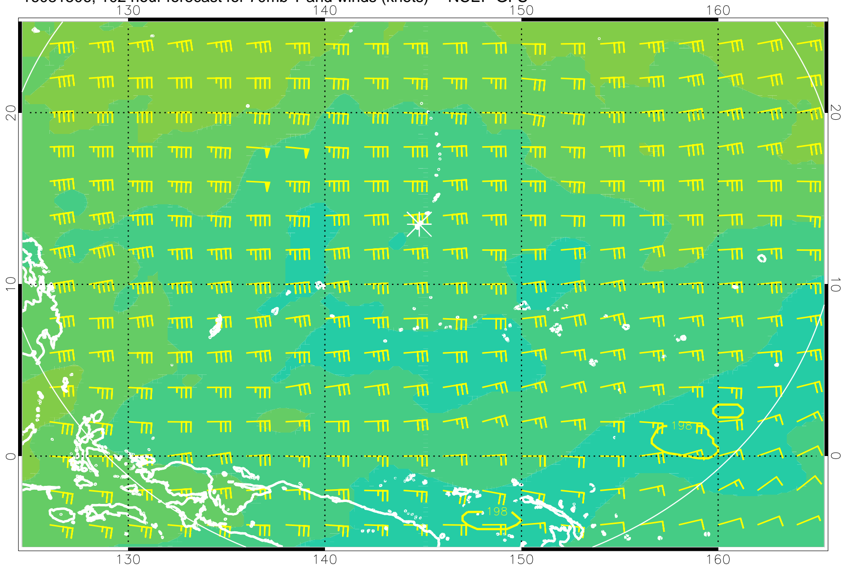
16081506, 102 hour forecast for 70mb T and winds (knots) -- NCEP GFS
