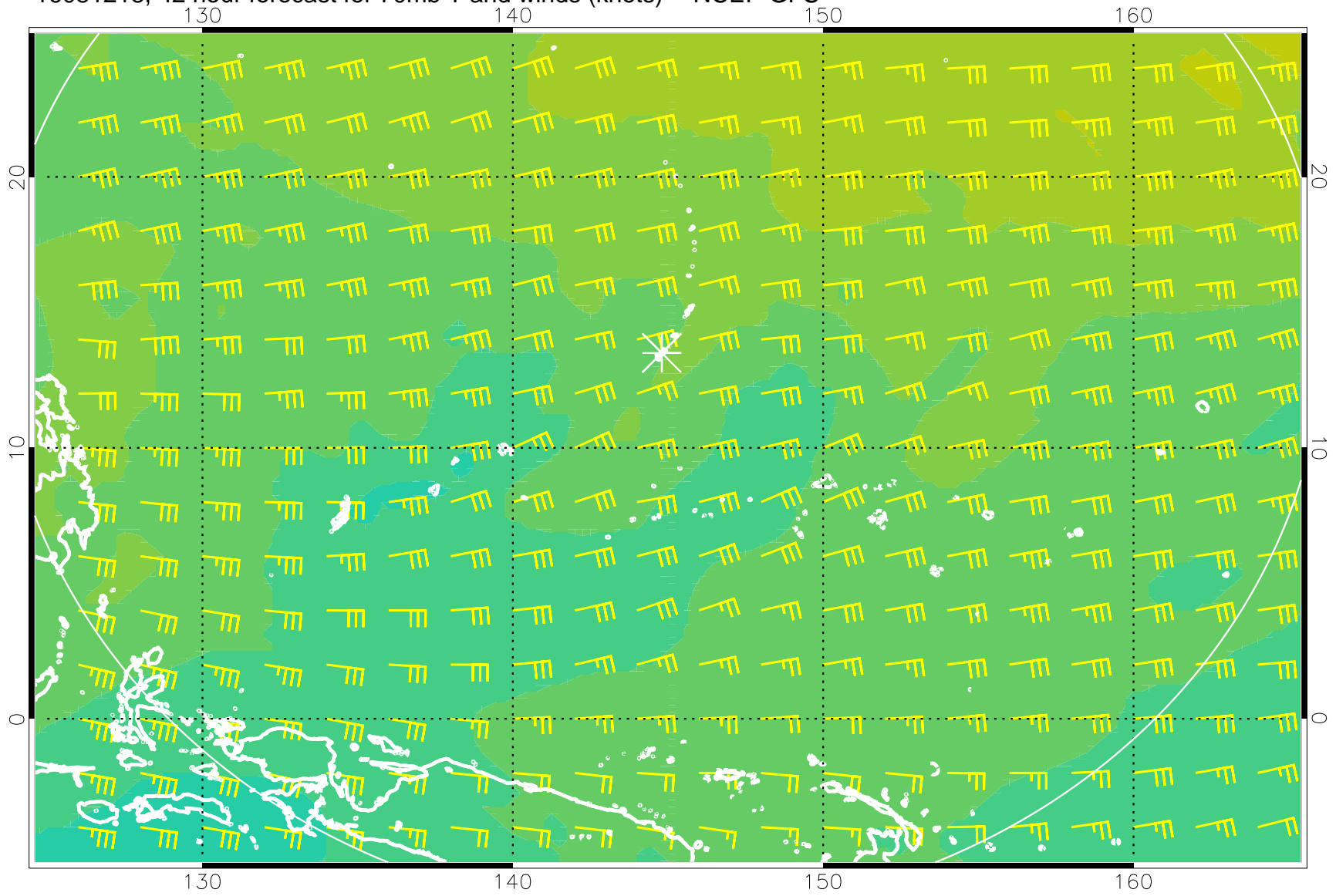
16081218, 42 hour forecast for 70mb T and winds (knots) -- NCEP GFS
