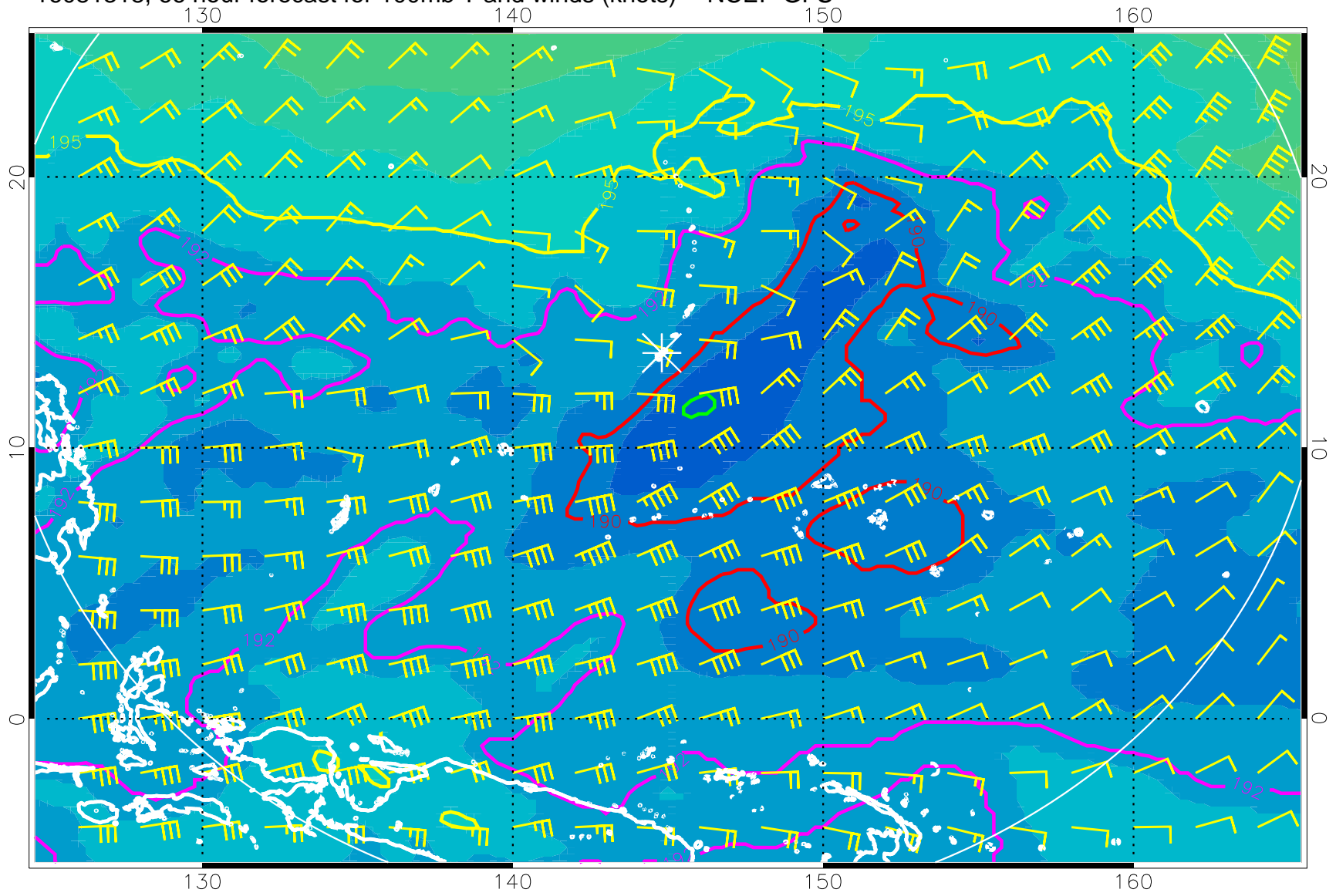
16081318, 66 hour forecast for 100mb T and winds (knots) -- NCEP GFS
