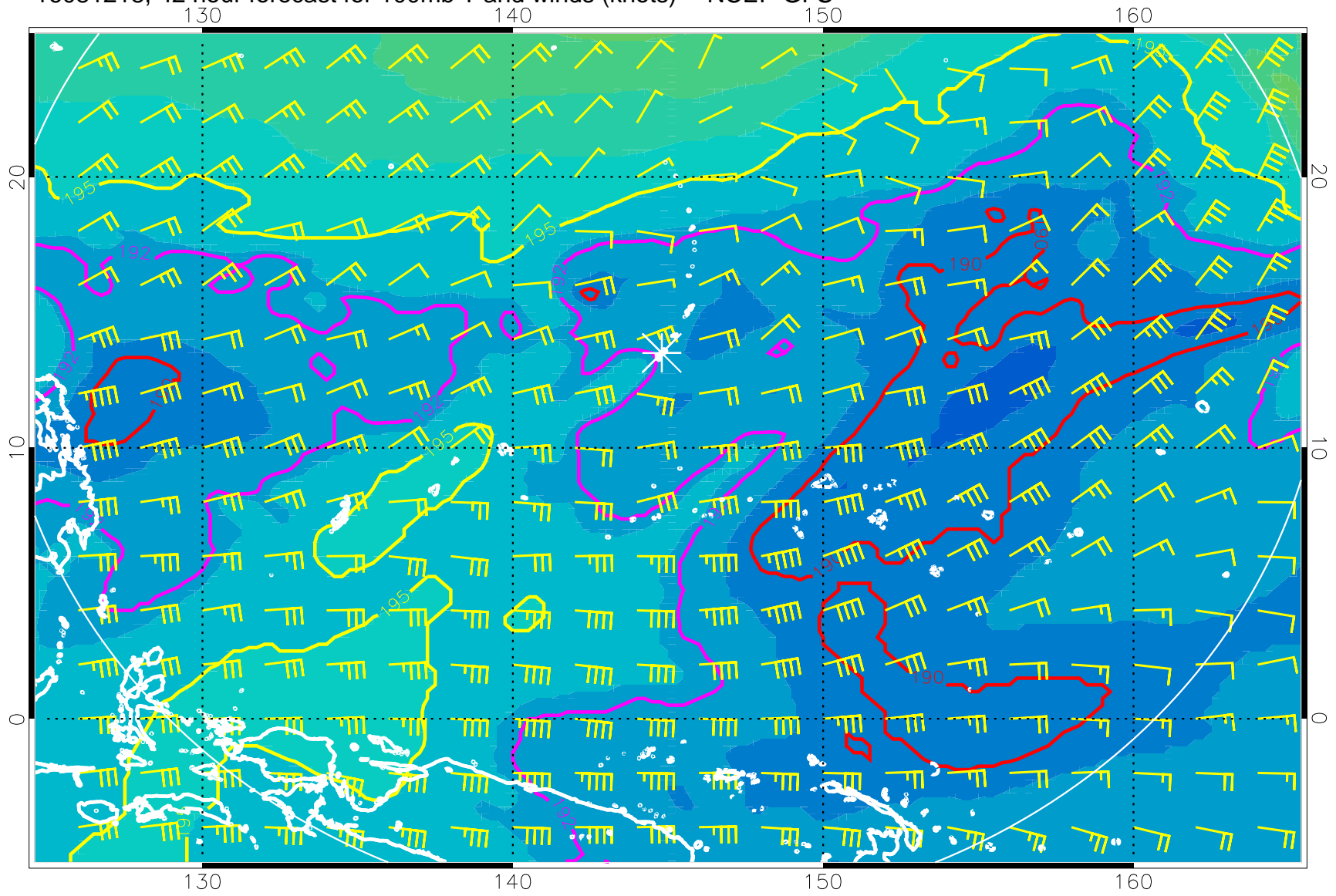
16081218, 42 hour forecast for 100mb T and winds (knots) -- NCEP GFS
