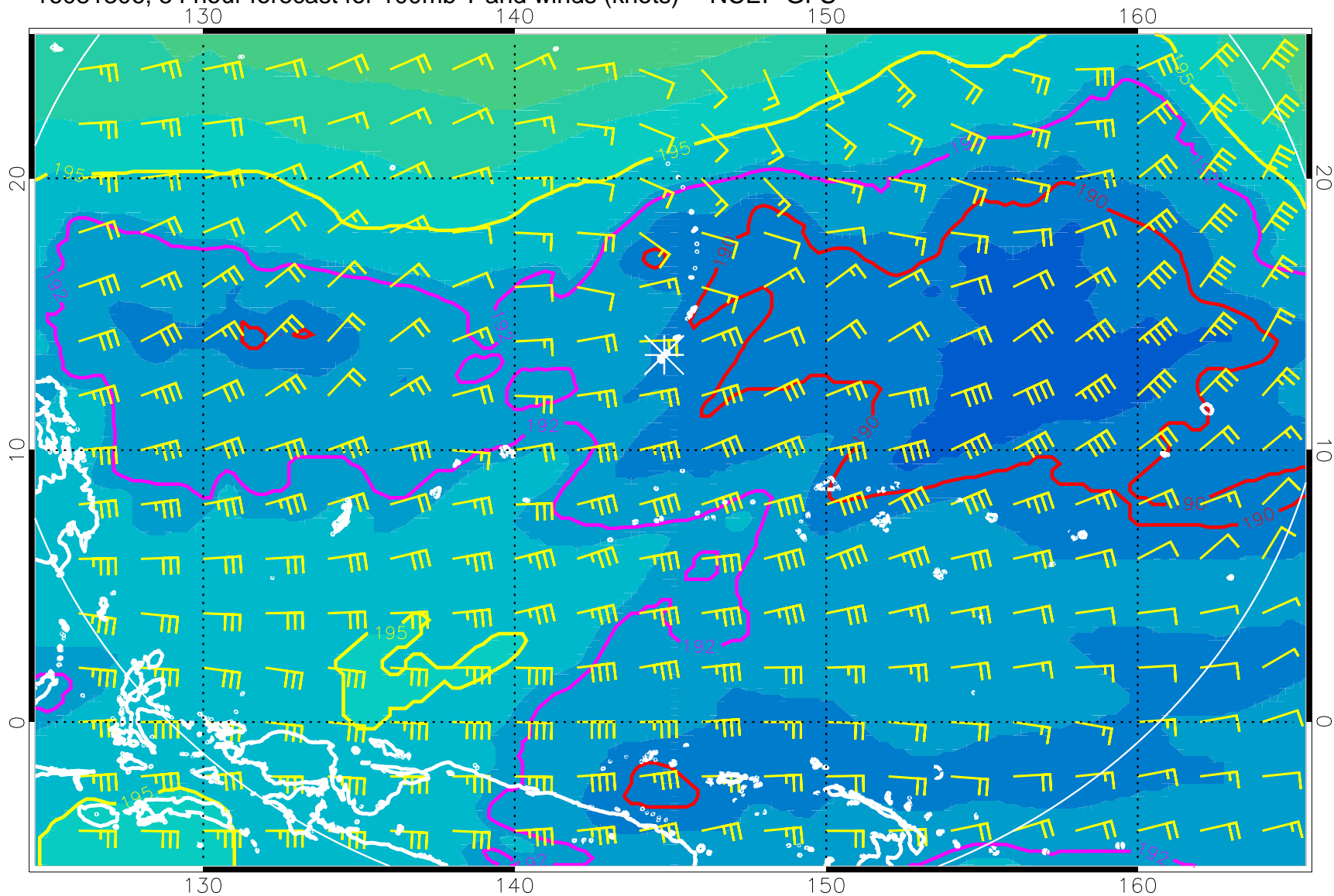
16081306, 54 hour forecast for 100mb T and winds (knots) -- NCEP GFS
