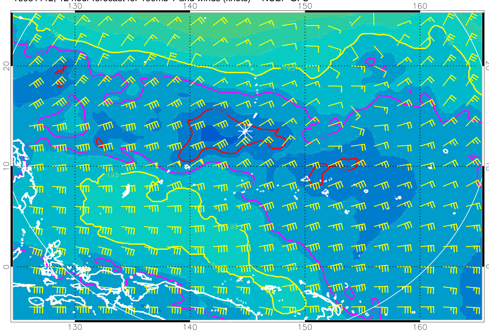
16081112, 12 hour forecast for 100mb T and winds (knots) -- NCEP GFS
