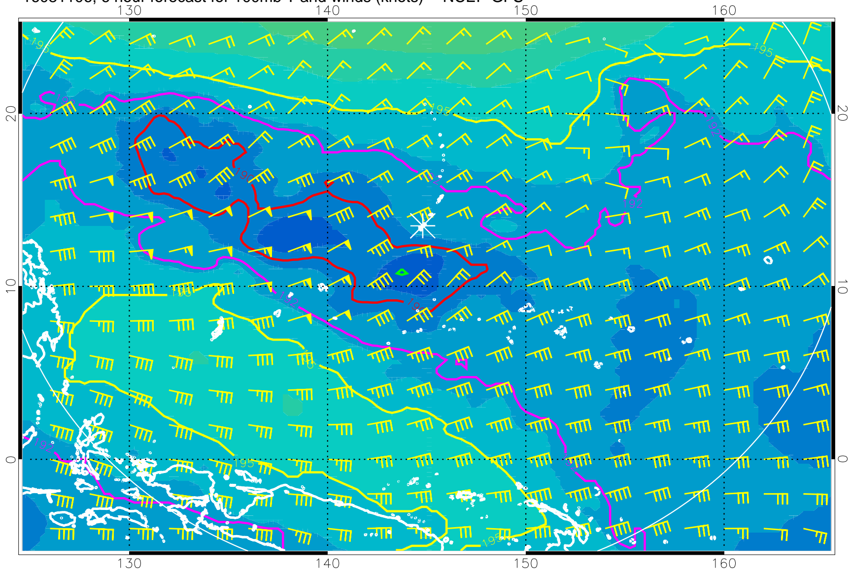
16081106, 6 hour forecast for 100mb T and winds (knots) -- NCEP GFS
