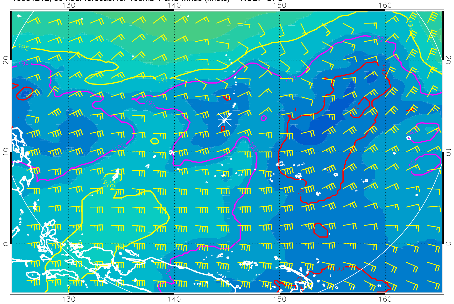
16081212, 36 hour forecast for 100mb T and winds (knots) -- NCEP GFS
