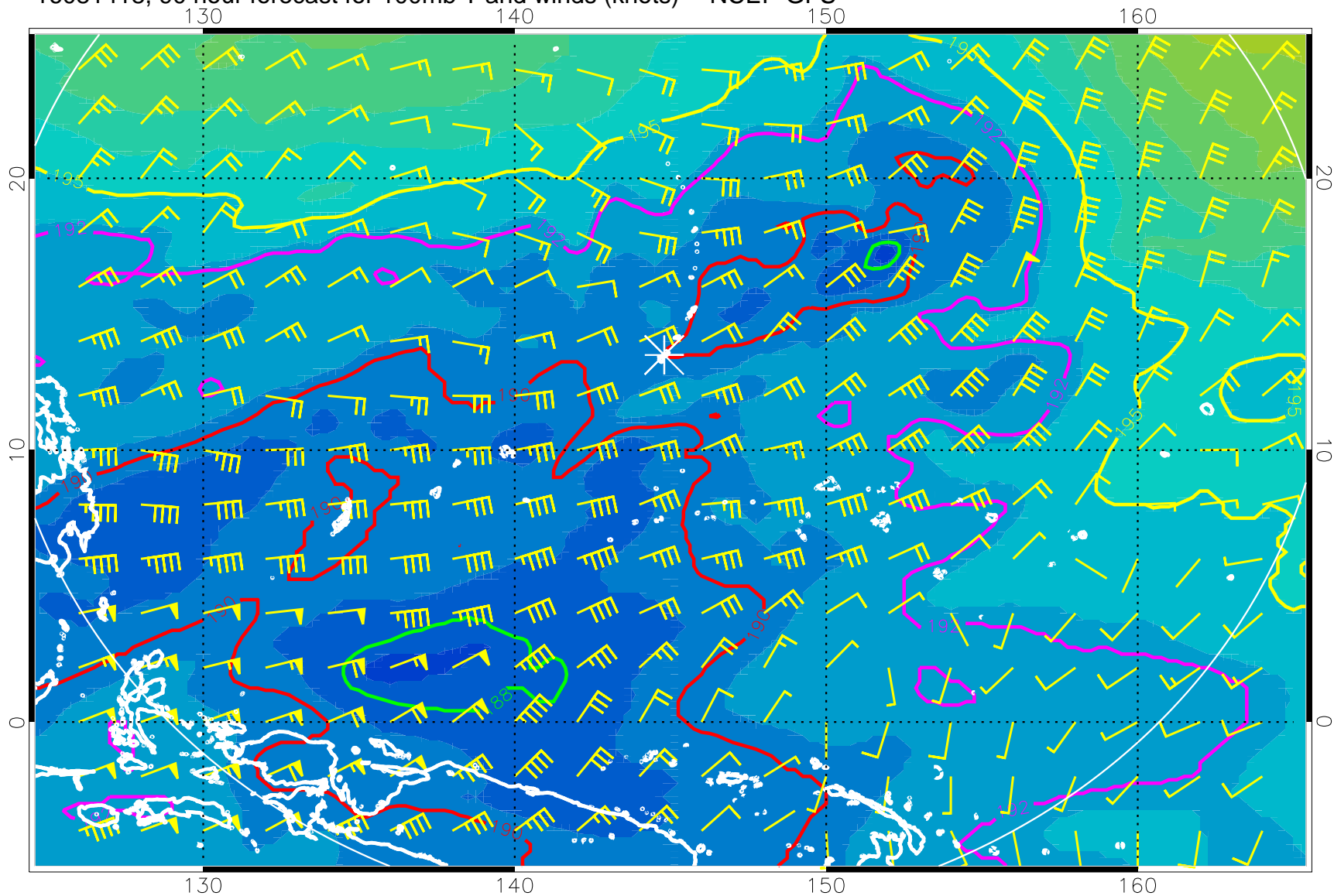
16081418, 90 hour forecast for 100mb T and winds (knots) -- NCEP GFS
