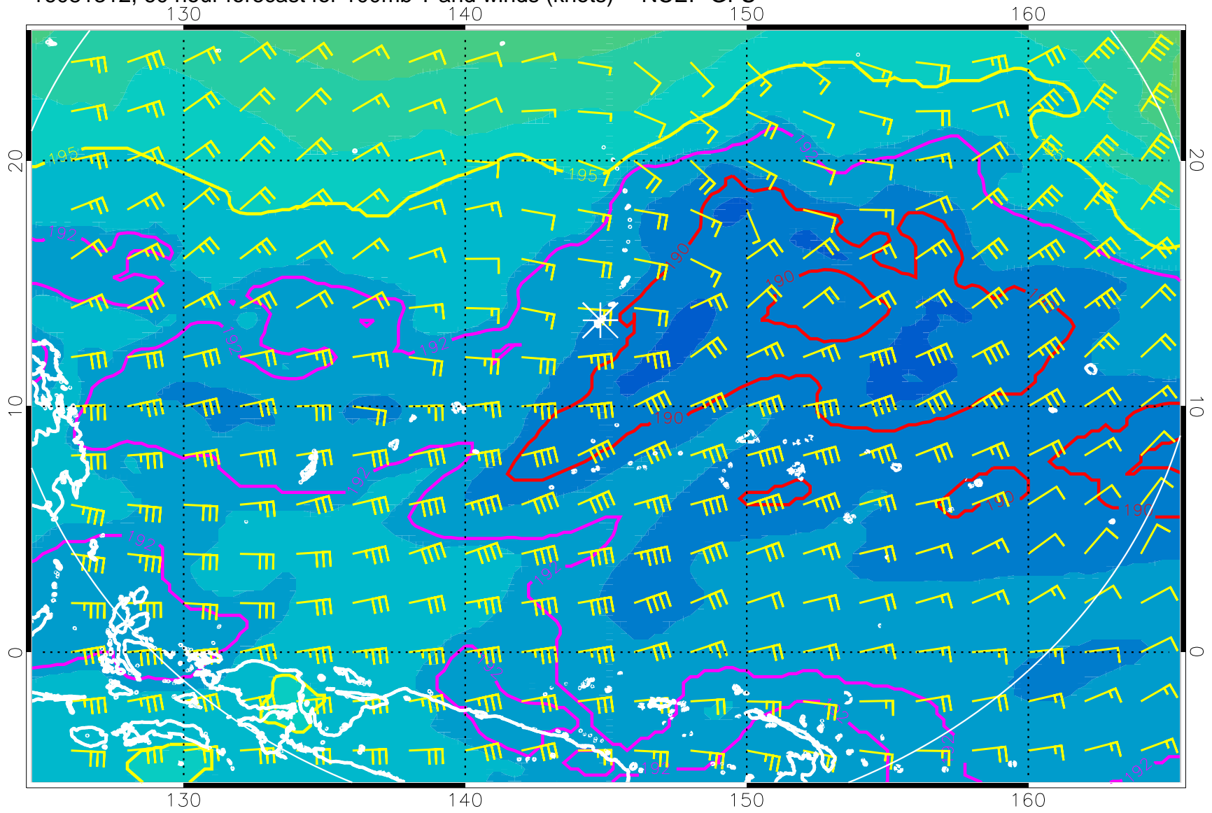
16081312, 60 hour forecast for 100mb T and winds (knots) -- NCEP GFS
