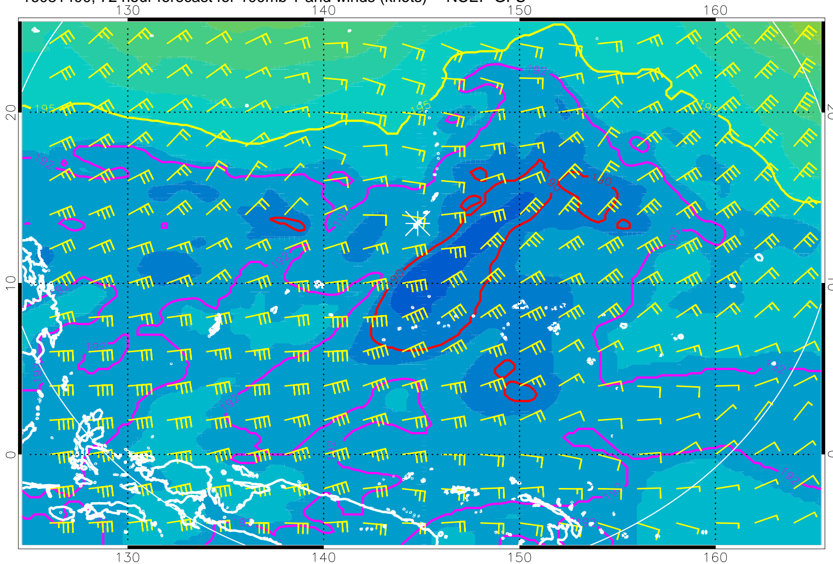
16081400, 72 hour forecast for 100mb T and winds (knots) -- NCEP GFS
