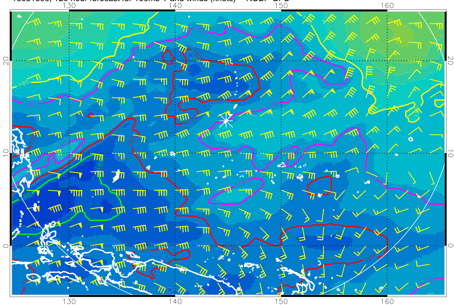
16081600, 120 hour forecast for 100mb T and winds (knots) -- NCEP GFS
