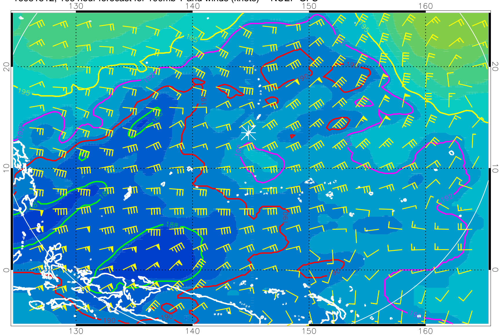
16081512, 108 hour forecast for 100mb T and winds (knots) -- NCEP GFS
