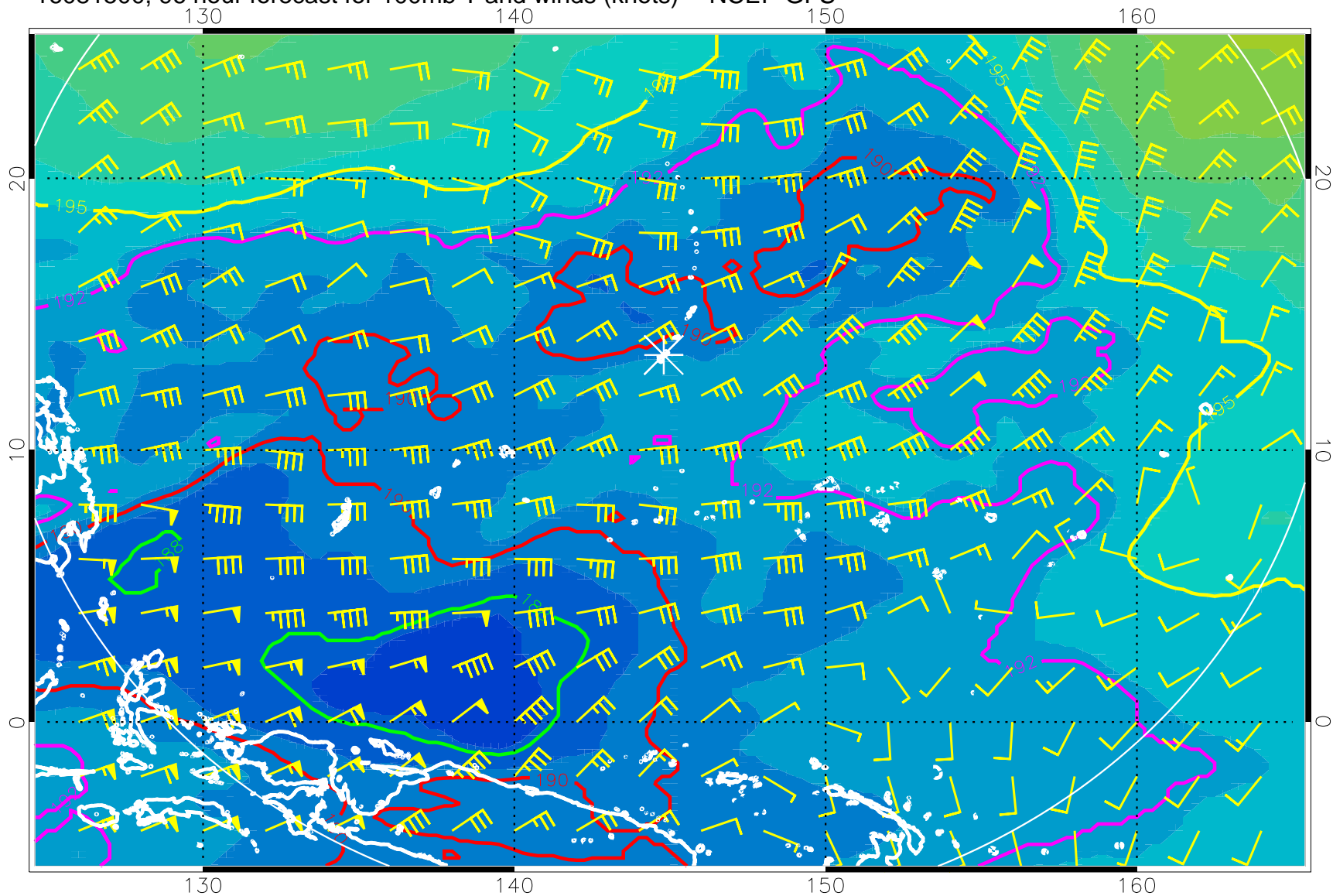
16081500, 96 hour forecast for 100mb T and winds (knots) -- NCEP GFS
