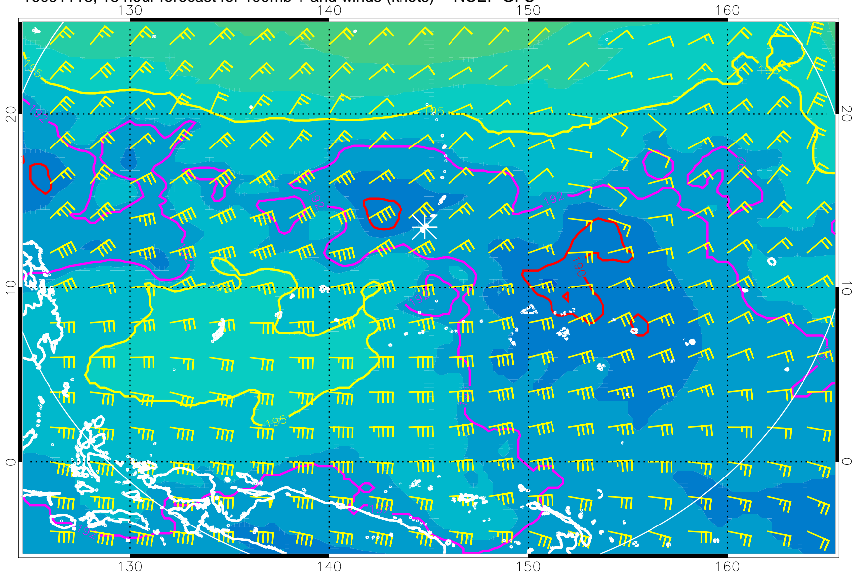
16081118, 18 hour forecast for 100mb T and winds (knots) -- NCEP GFS
