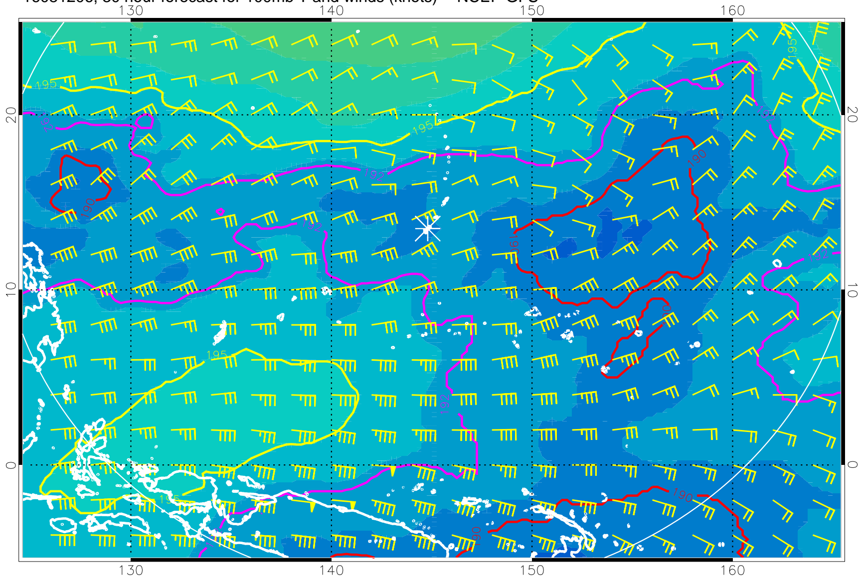
16081206, 30 hour forecast for 100mb T and winds (knots) -- NCEP GFS
