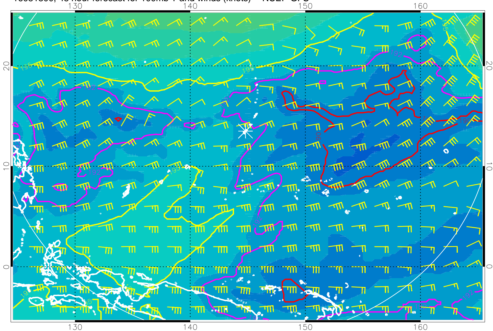
16081300, 48 hour forecast for 100mb T and winds (knots) -- NCEP GFS
