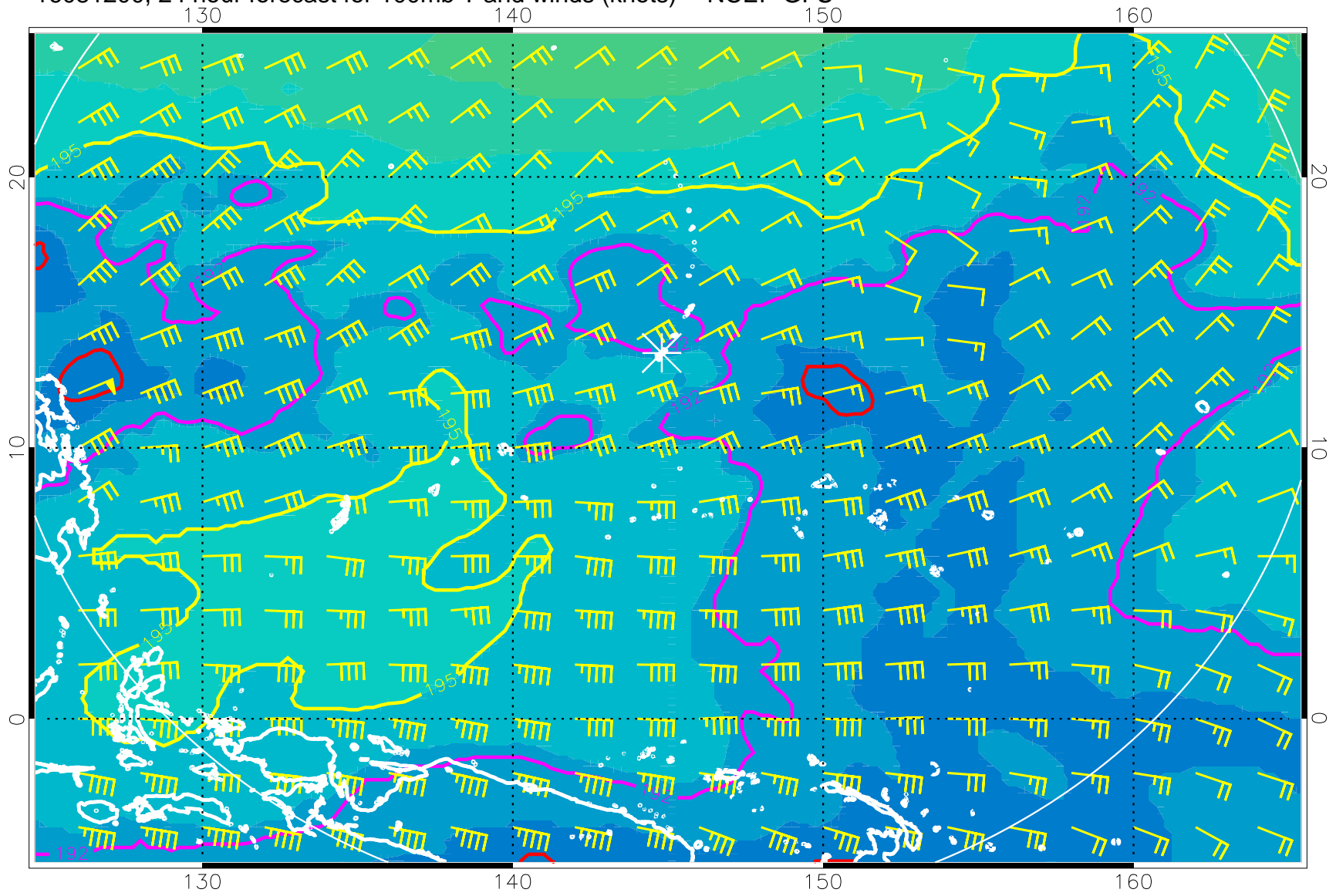
16081200, 24 hour forecast for 100mb T and winds (knots) -- NCEP GFS
