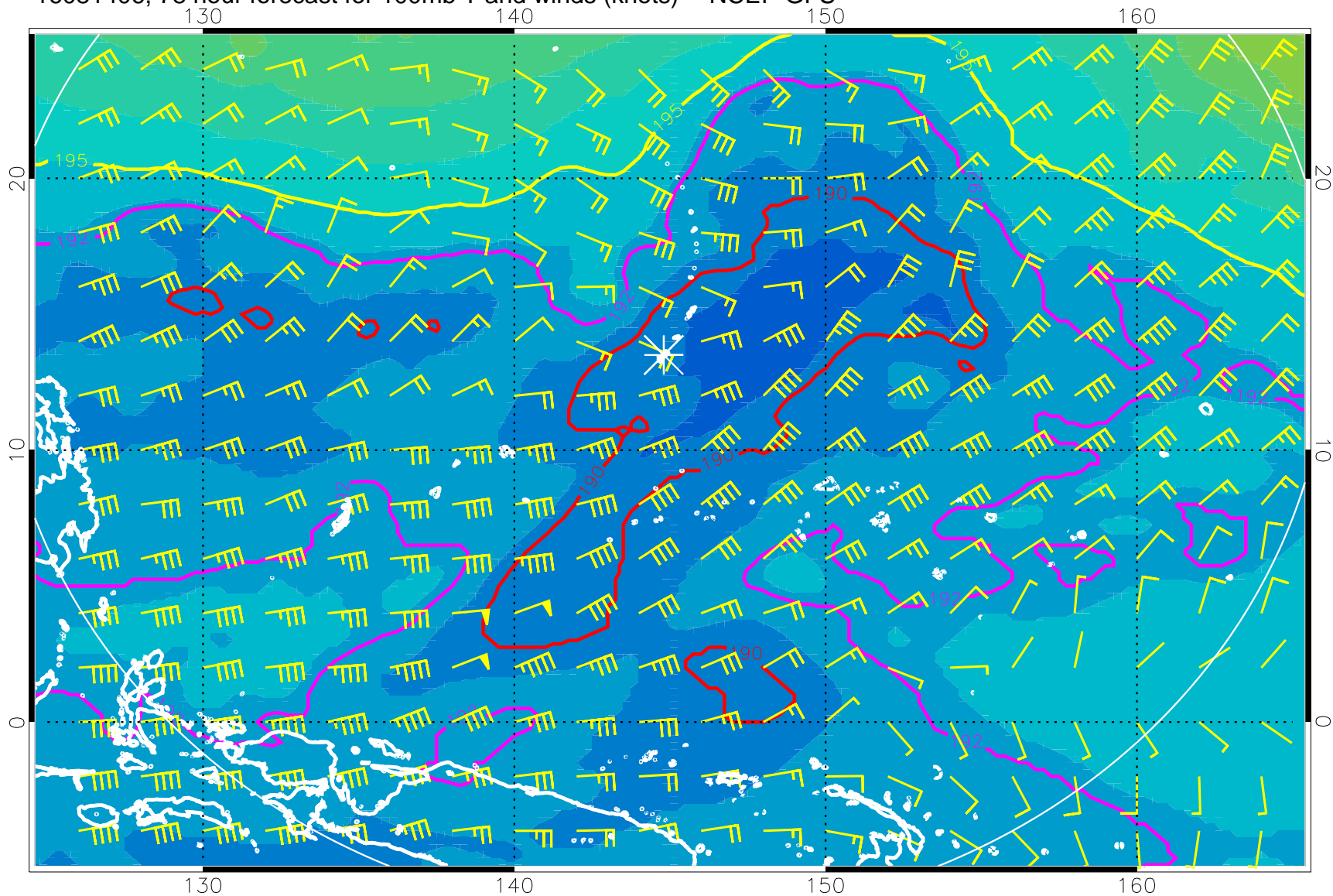
16081406, 78 hour forecast for 100mb T and winds (knots) -- NCEP GFS
