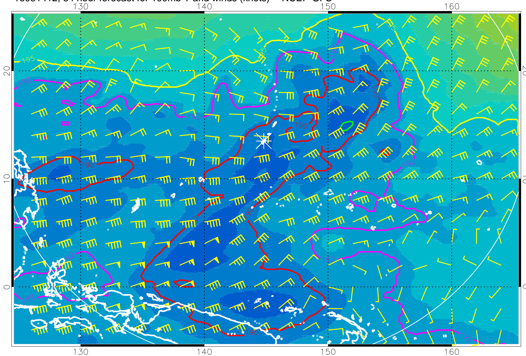
16081412, 84 hour forecast for 100mb T and winds (knots) -- NCEP GFS
