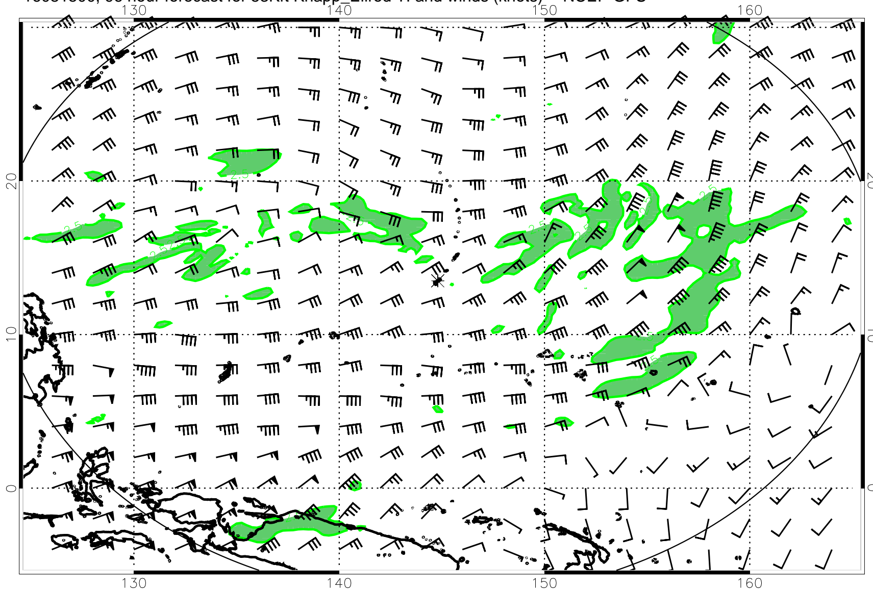
16081500, 96 hour forecast for 53Kft Knapp_Ellrod TI and winds (knots) -- NCEP GFS
