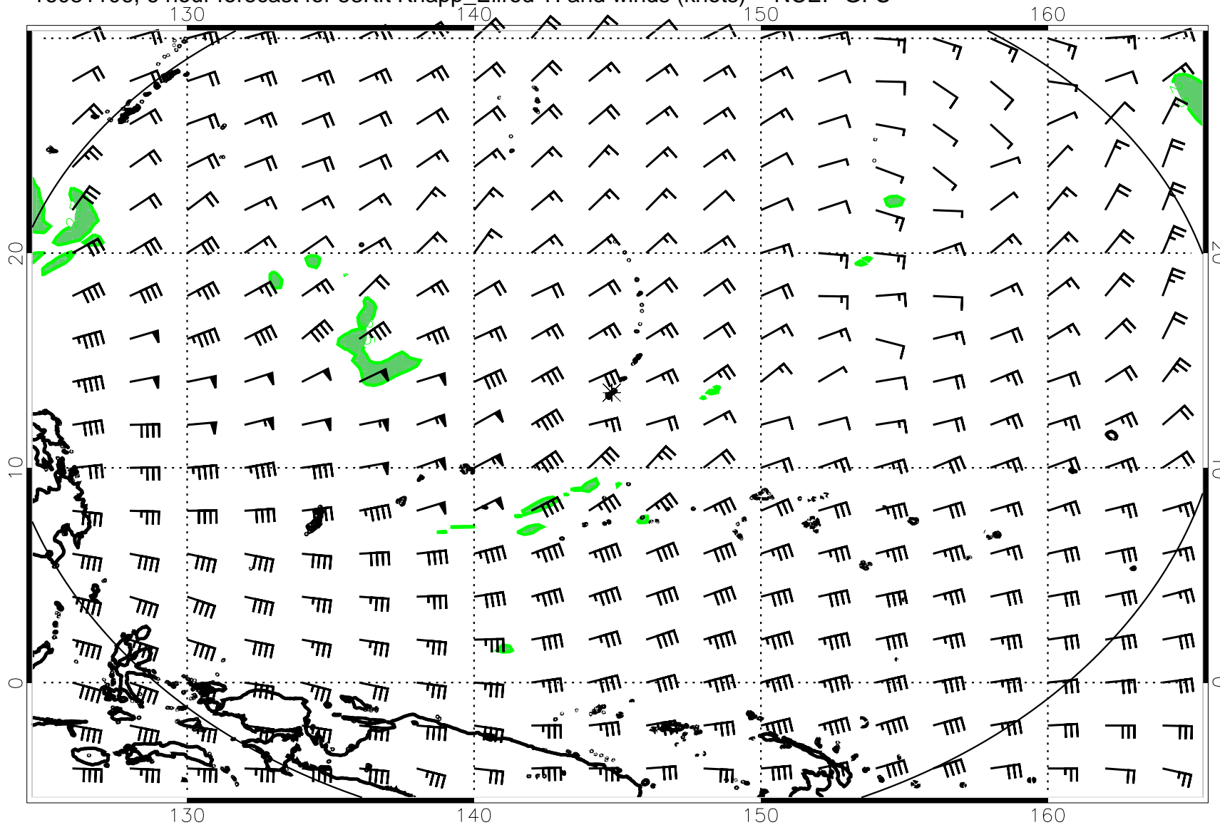
16081106, 6 hour forecast for 53Kft Knapp_Ellrod TI and winds (knots) -- NCEP GFS
