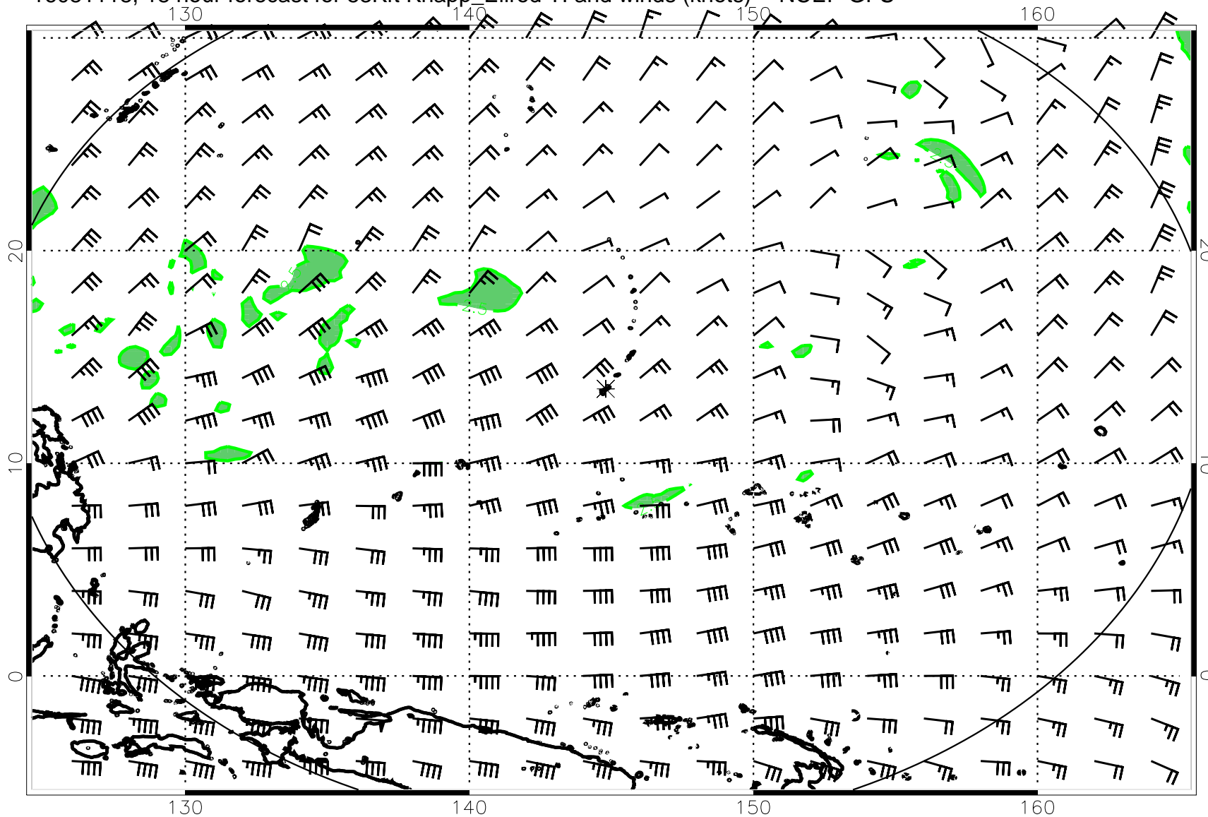
16081118, 18 hour forecast for 53Kft Knapp_Ellrod TI and winds (knots) -- NCEP GFS
