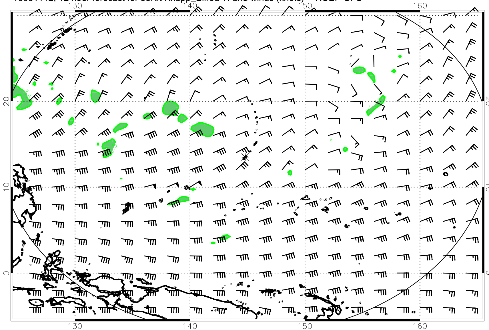
16081112, 12 hour forecast for 53Kft Knapp_Ellrod TI and winds (knots) -- NCEP GFS
