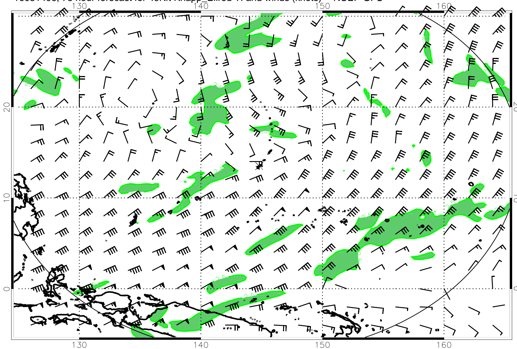
16081406, 78 hour forecast for 49Kft Knapp_Ellrod TI and winds (knots) -- NCEP GFS
