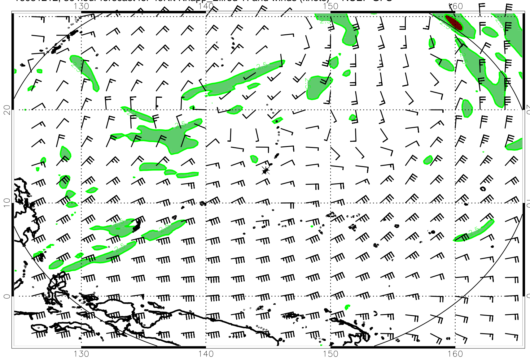
16081212, 36 hour forecast for 49Kft Knapp_Ellrod TI and winds (knots) -- NCEP GFS
