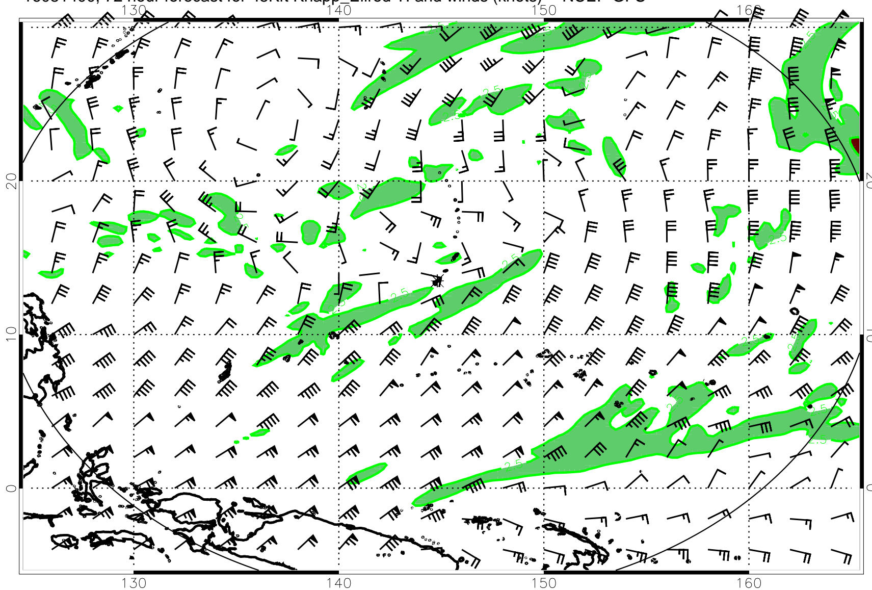
16081400, 72 hour forecast for 45Kft Knapp_Ellrod TI and winds (knots) -- NCEP GFS
