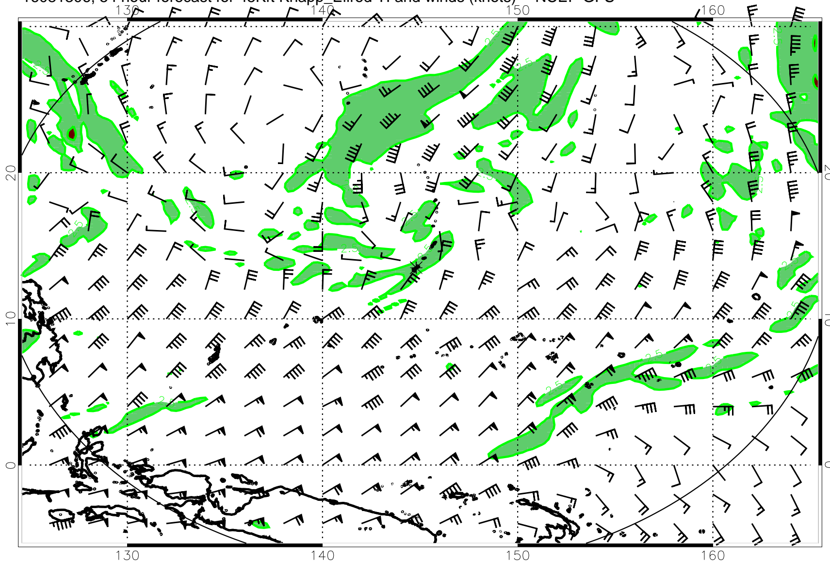
16081306, 54 hour forecast for 45Kft Knapp_Ellrod TI and winds (knots) -- NCEP GFS
