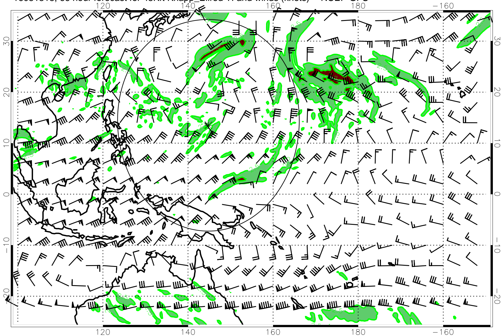
16081318, 66 hour forecast for 45Kft Knapp_Ellrod TI and winds (knots) -- NCEP GFS
