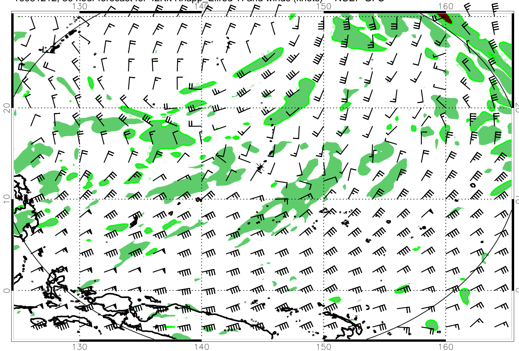
16081212, 36 hour forecast for 42Kft Knapp_Ellrod TI and winds (knots) -- NCEP GFS
