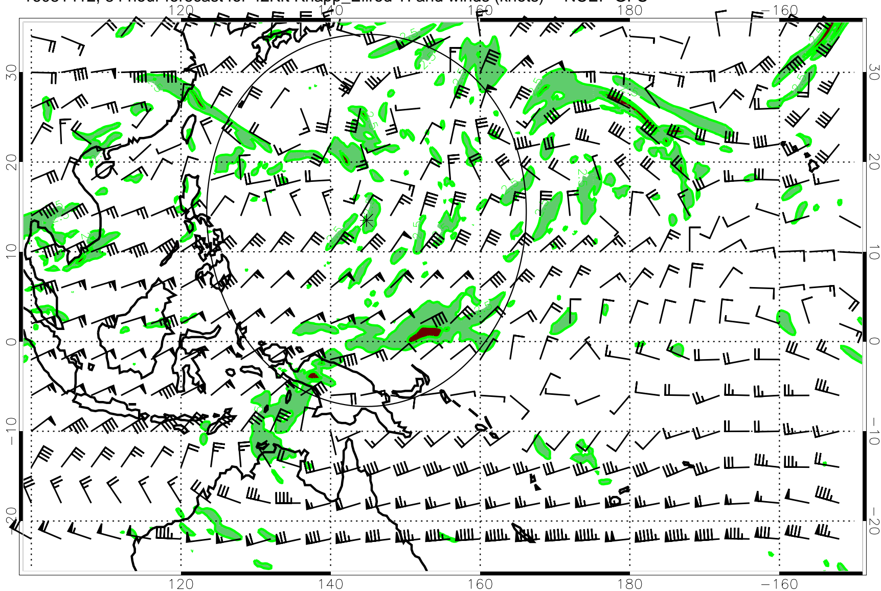
16081412, 84 hour forecast for 42Kft Knapp_Ellrod TI and winds (knots) -- NCEP GFS
