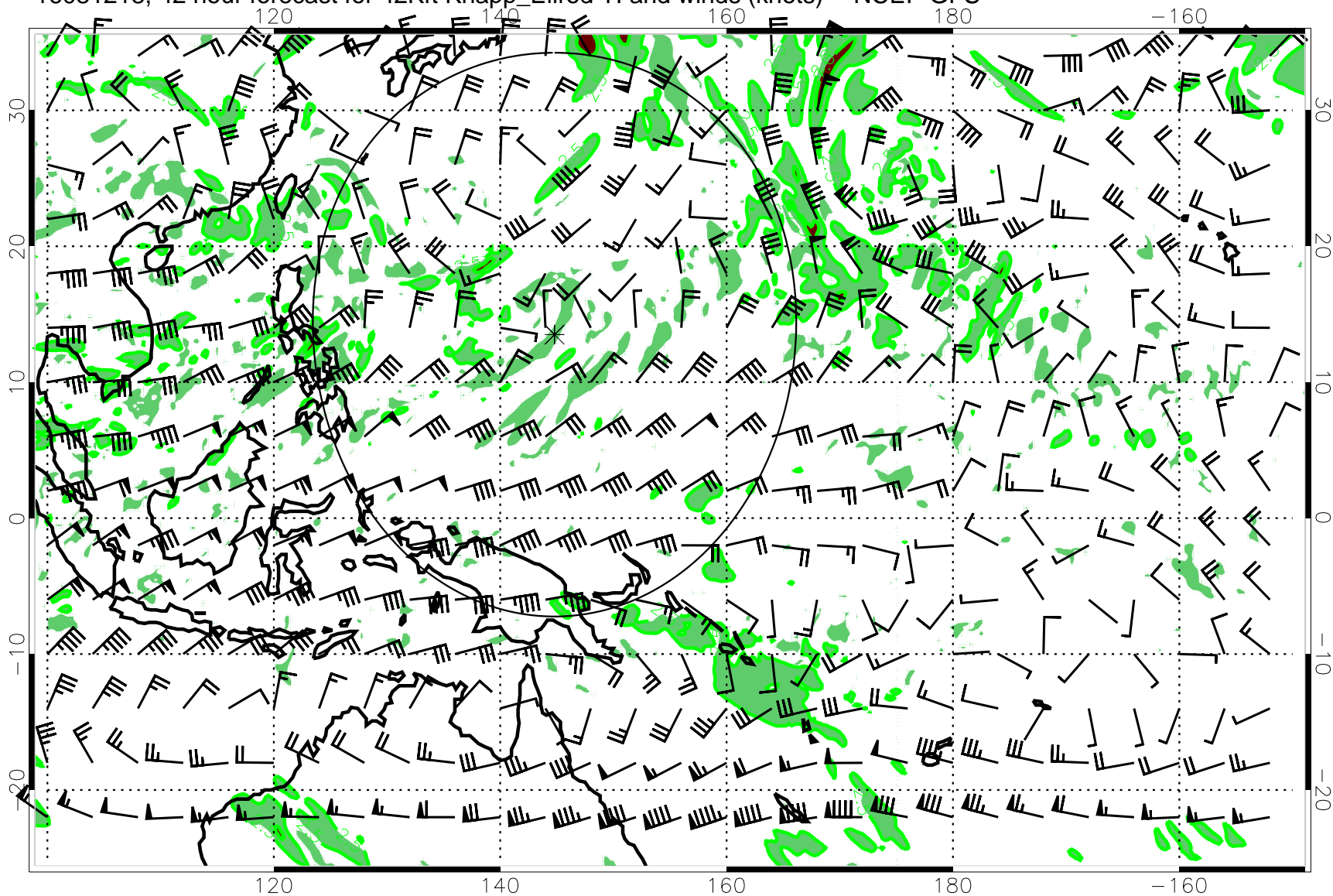
16081218, 42 hour forecast for 42Kft Knapp_Ellrod TI and winds (knots) -- NCEP GFS
