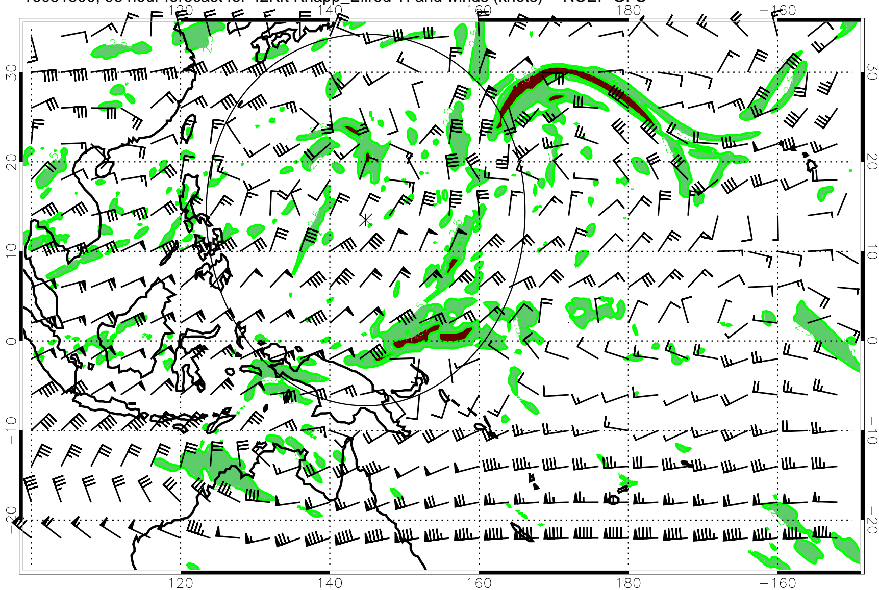
16081500, 96 hour forecast for 42Kft Knapp_Ellrod TI and winds (knots) -- NCEP GFS
