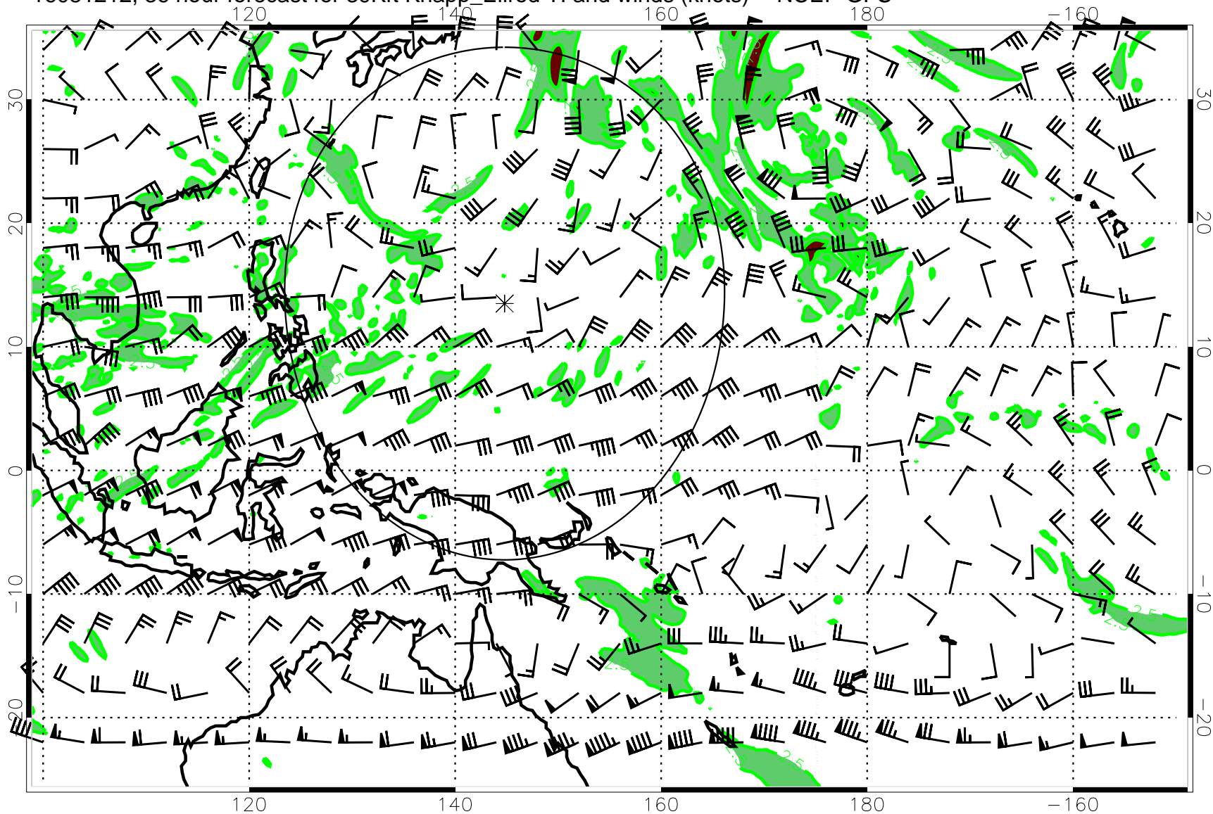
16081212, 36 hour forecast for 39Kft Knapp_Ellrod TI and winds (knots) -- NCEP GFS
