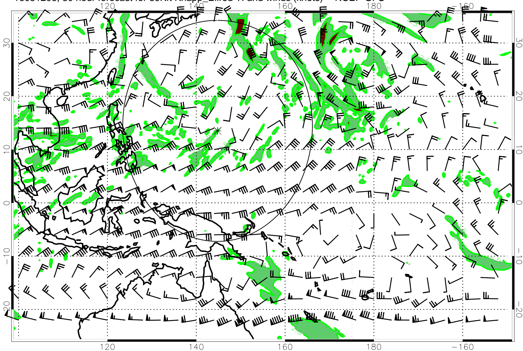
16081206, 30 hour forecast for 39Kft Knapp_Ellrod TI and winds (knots) -- NCEP GFS
