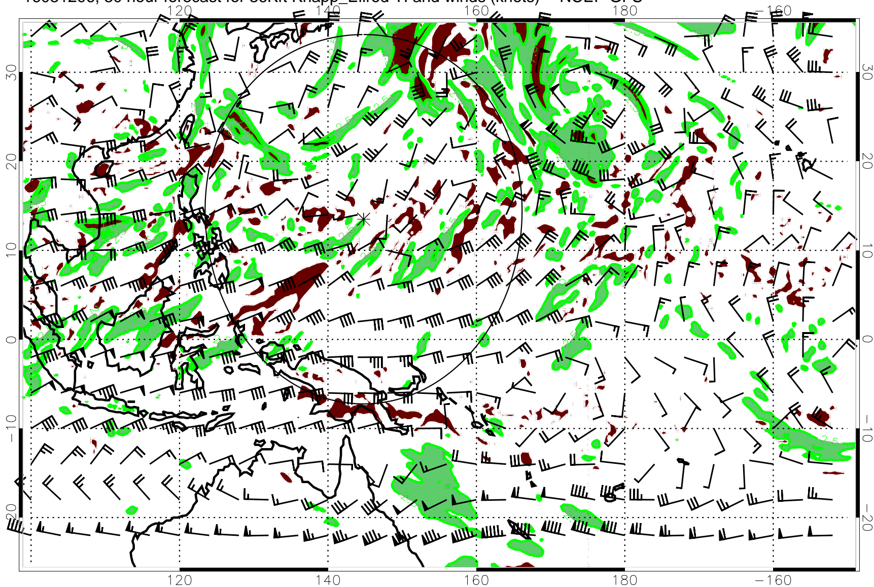
16081206, 30 hour forecast for 36Kft Knapp_Ellrod TI and winds (knots) -- NCEP GFS
