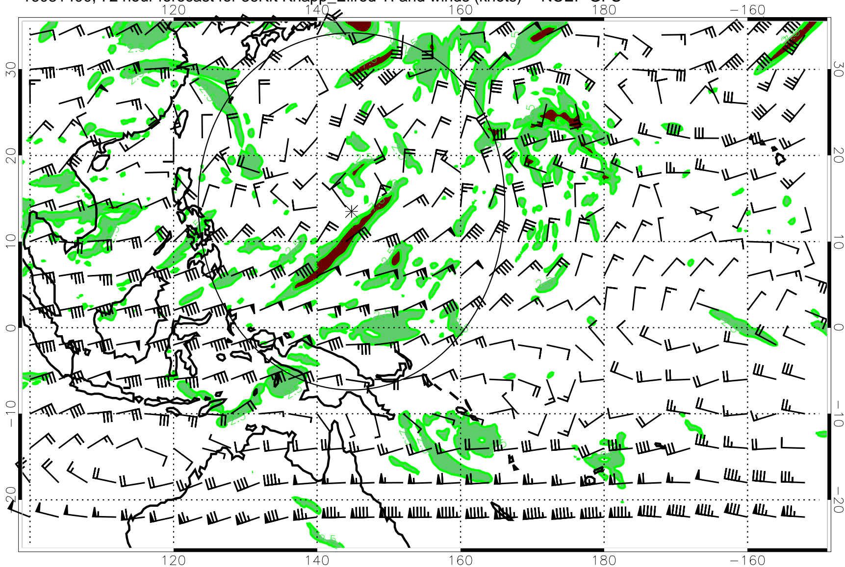
16081400, 72 hour forecast for 36Kft Knapp_Ellrod TI and winds (knots) -- NCEP GFS
