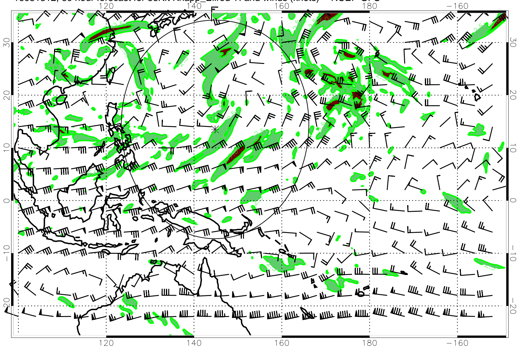
16081312, 60 hour forecast for 36Kft Knapp_Ellrod TI and winds (knots) -- NCEP GFS
