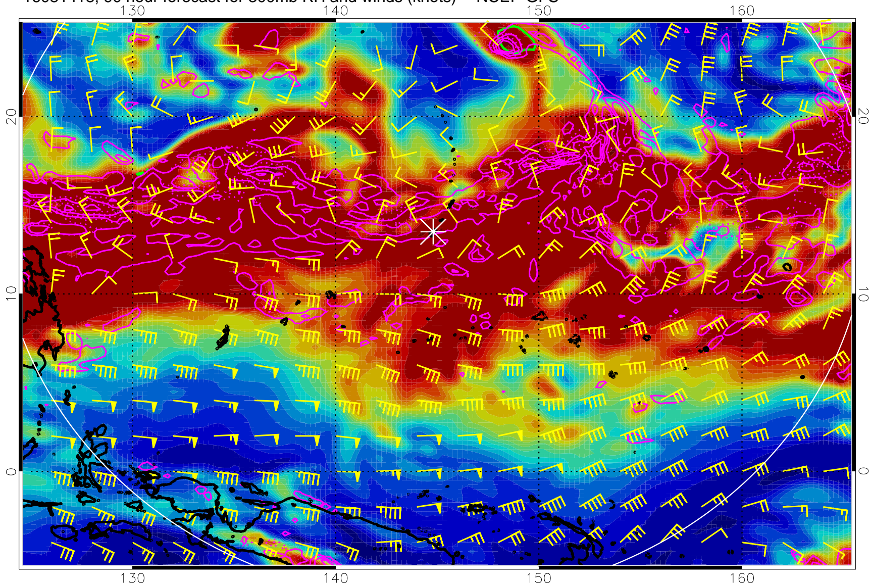
16081418, 90 hour forecast for 300mb RH and winds (knots) -- NCEP GFS
