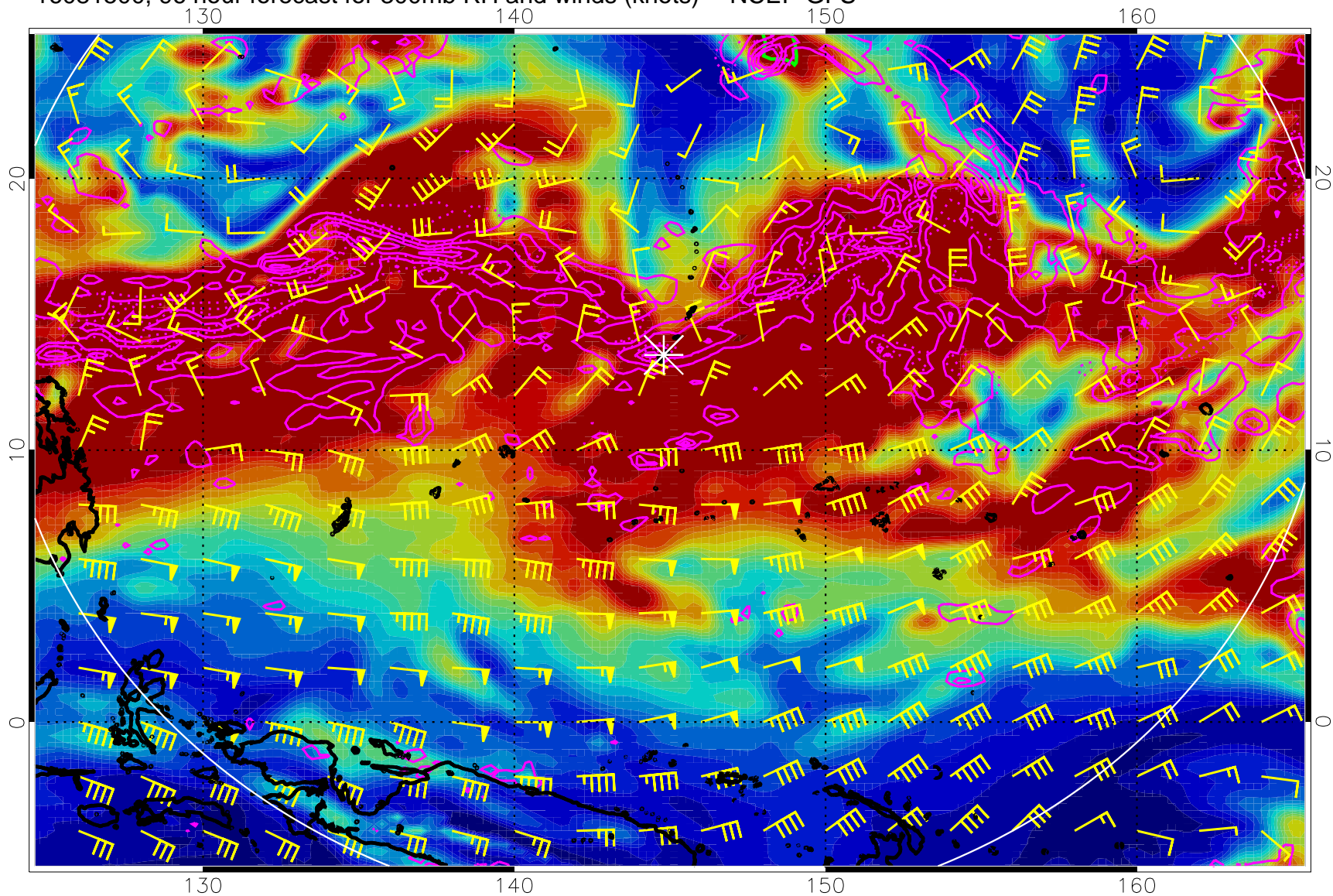
16081500, 96 hour forecast for 300mb RH and winds (knots) -- NCEP GFS
