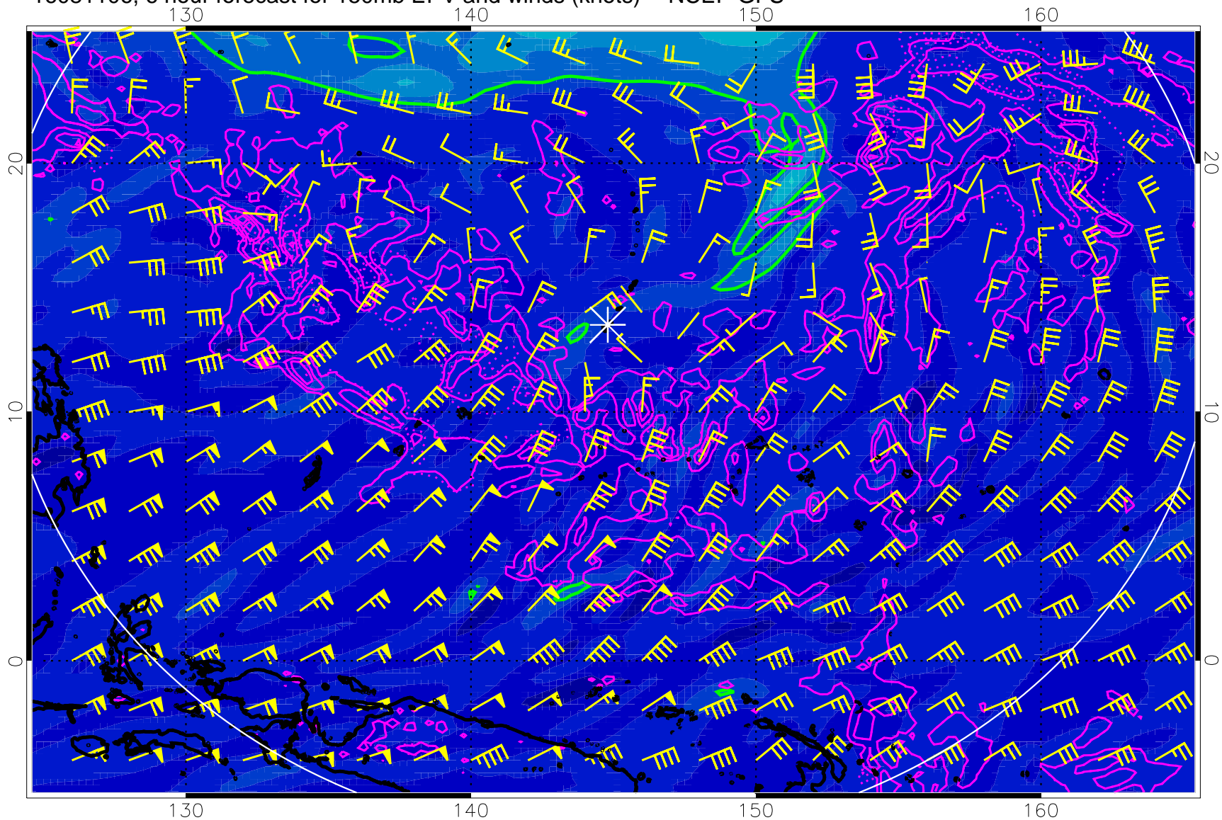
16081106, 6 hour forecast for 150mb EPV and winds (knots) -- NCEP GFS
