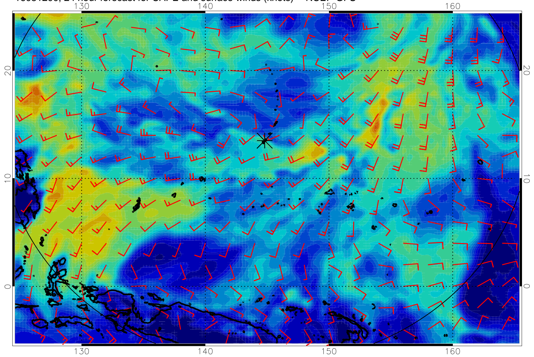
16081200, 24 hour forecast for CAPE and surface winds (knots) -- NCEP GFS
