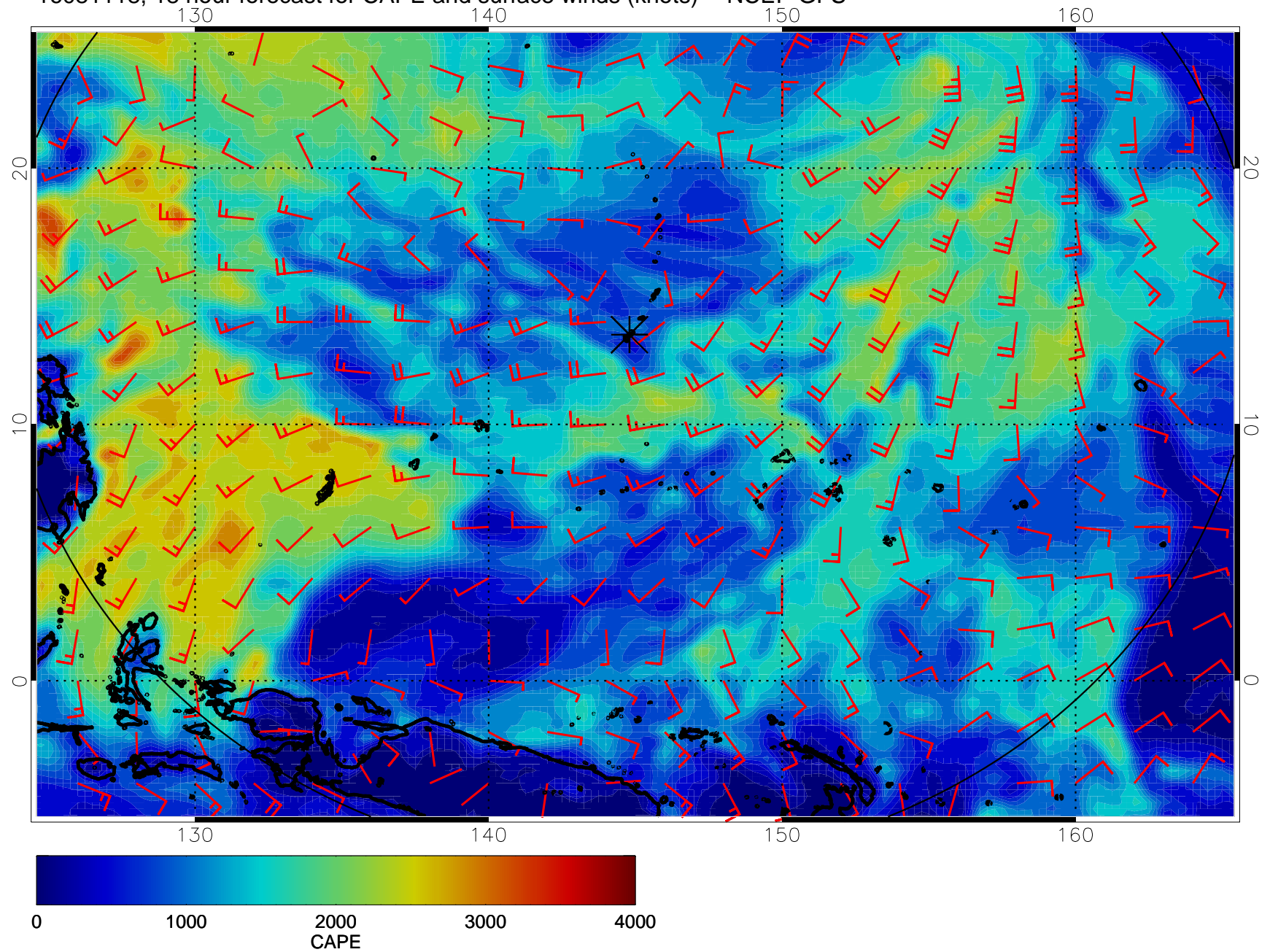
16081118, 18 hour forecast for CAPE and surface winds (knots) -- NCEP GFS
