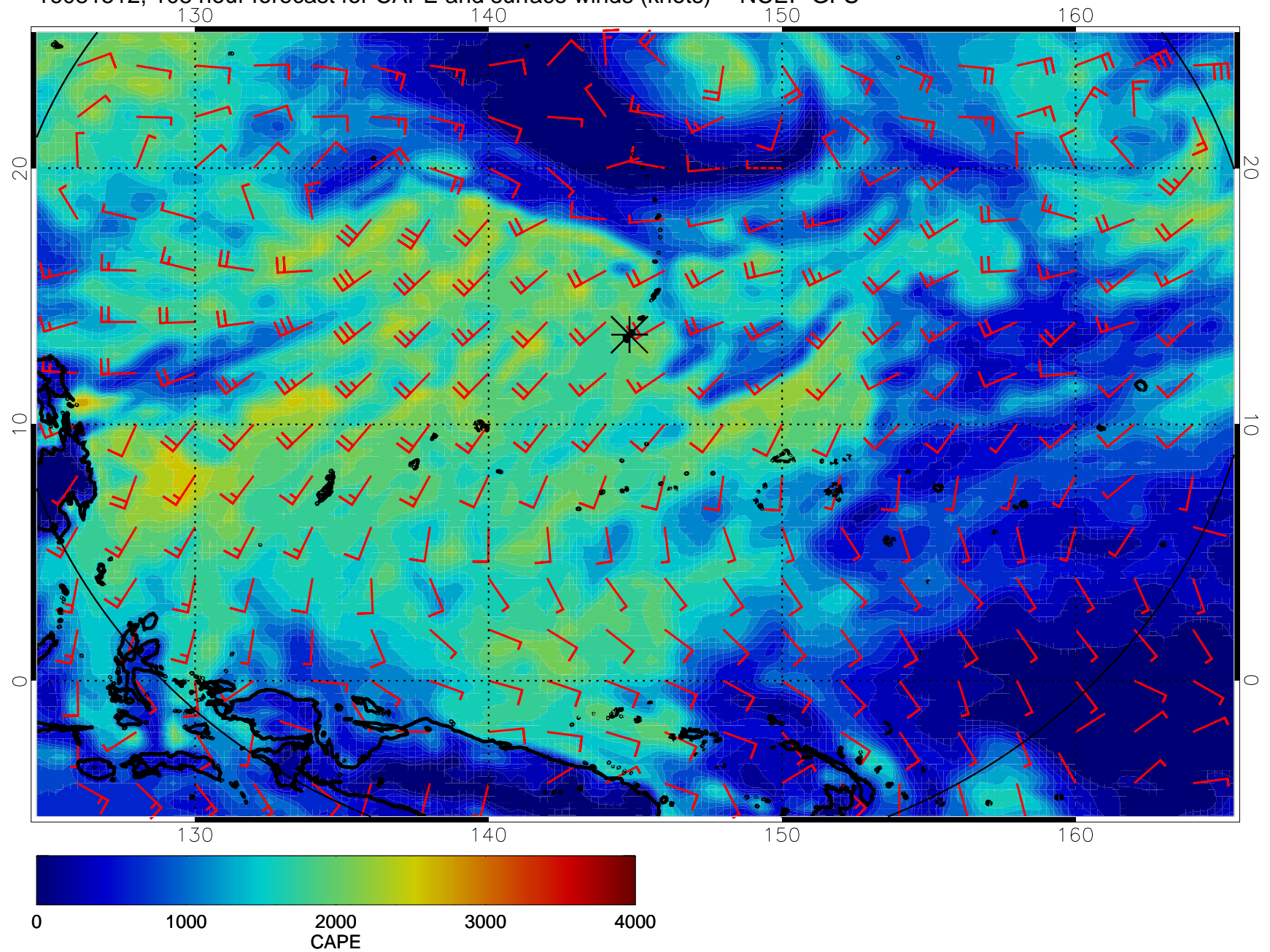
16081512, 108 hour forecast for CAPE and surface winds (knots) -- NCEP GFS
