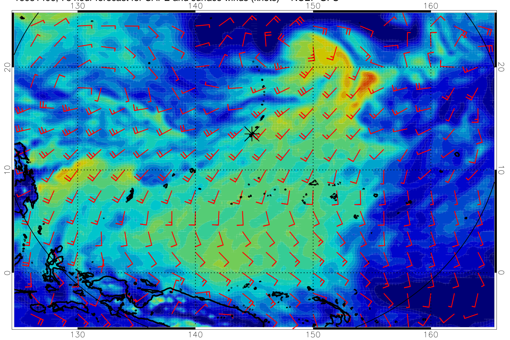
16081406, 78 hour forecast for CAPE and surface winds (knots) -- NCEP GFS
