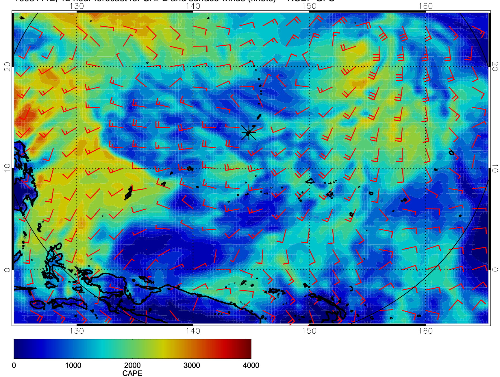
16081112, 12 hour forecast for CAPE and surface winds (knots) -- NCEP GFS
