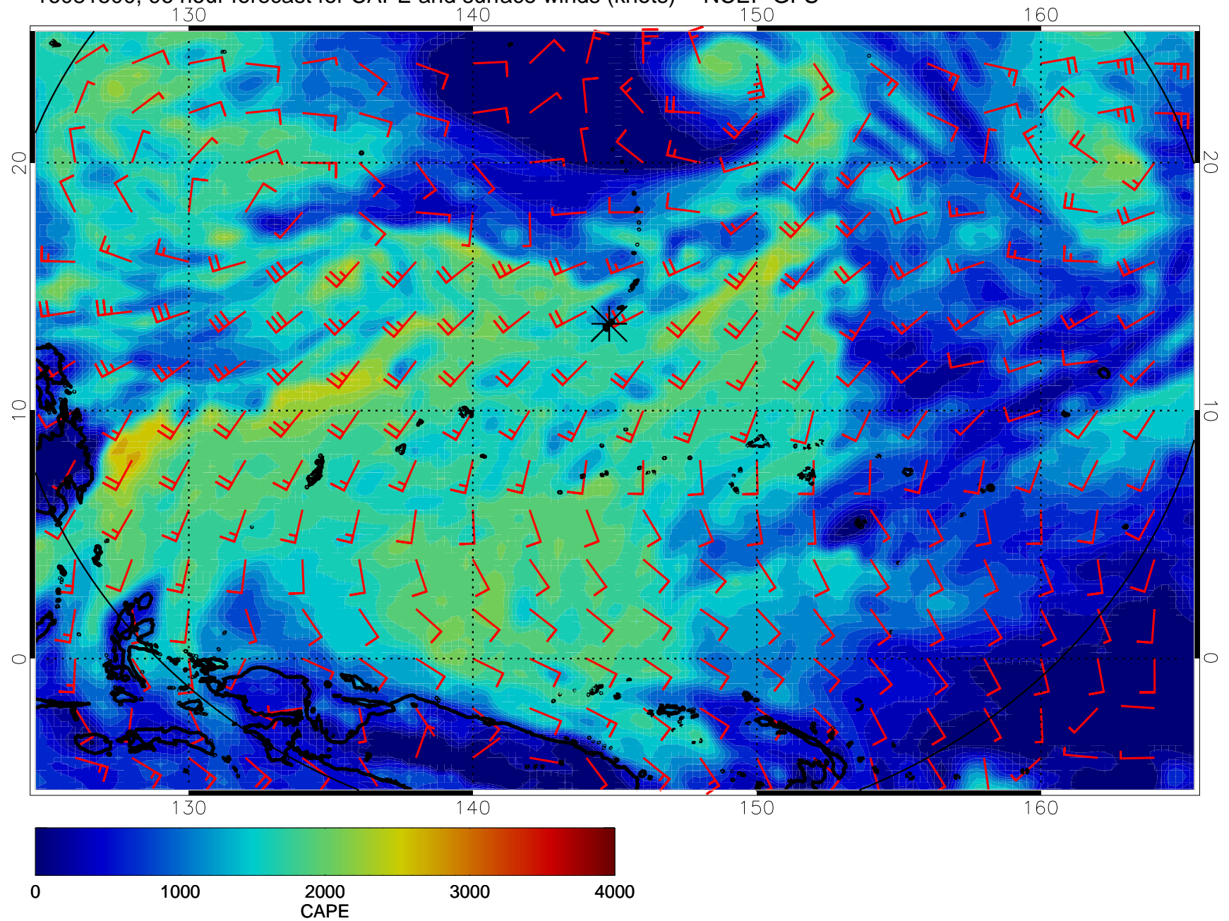
16081500, 96 hour forecast for CAPE and surface winds (knots) -- NCEP GFS
