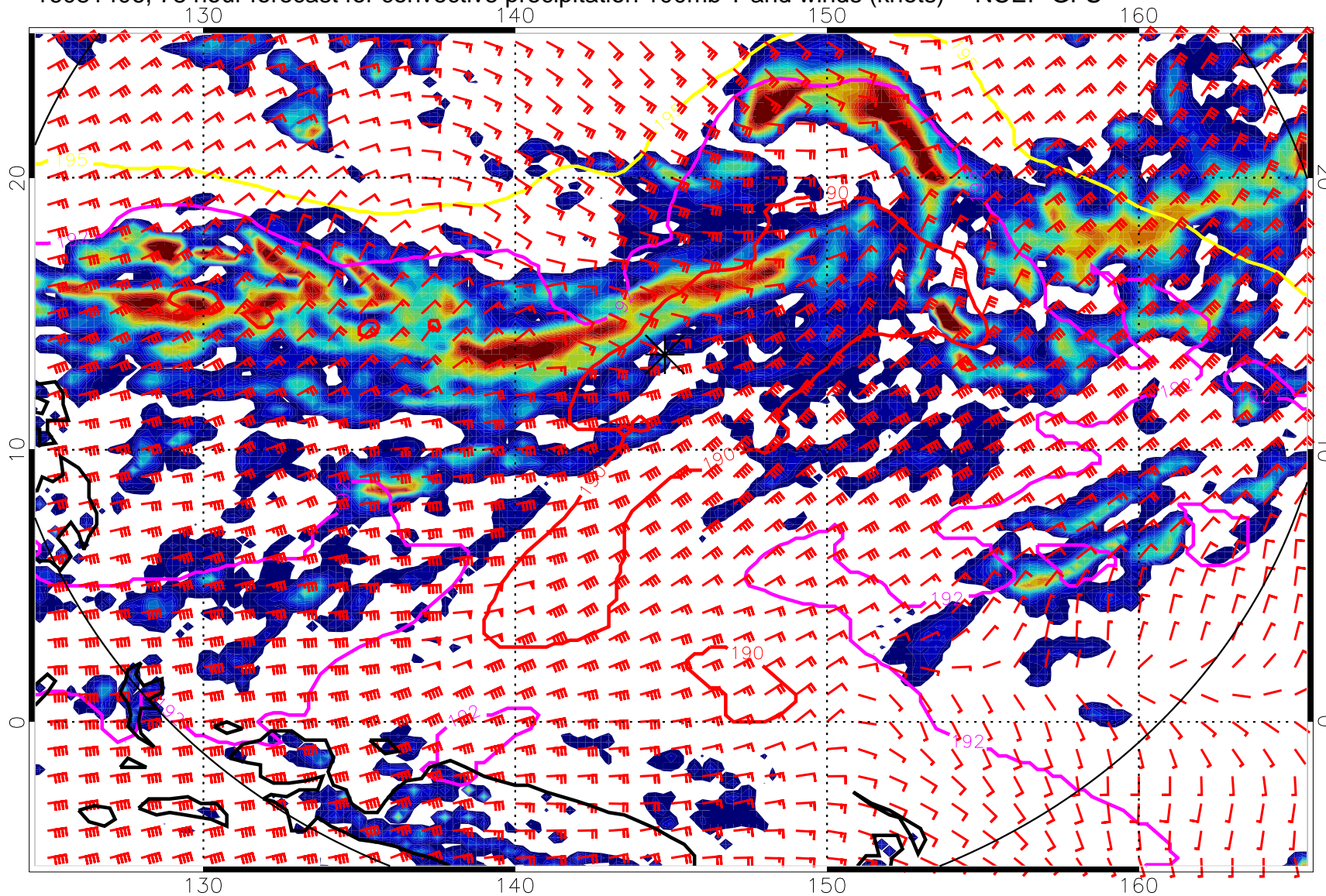
16081406, 78 hour forecast for convective precipitation 100mb T and winds (knots) -- NCEP GFS
