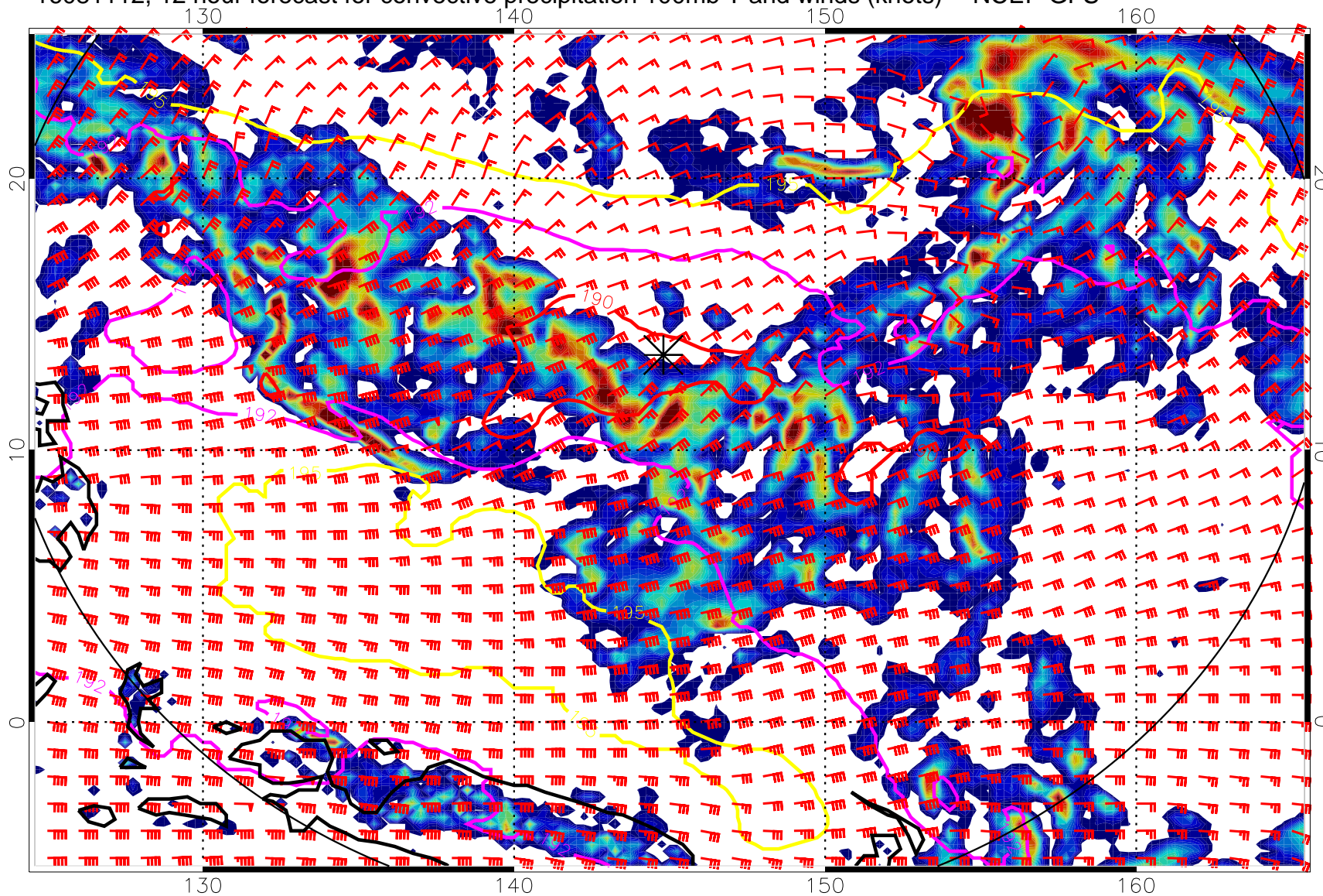
16081112, 12 hour forecast for convective precipitation 100mb T and winds (knots) -- NCEP GFS
