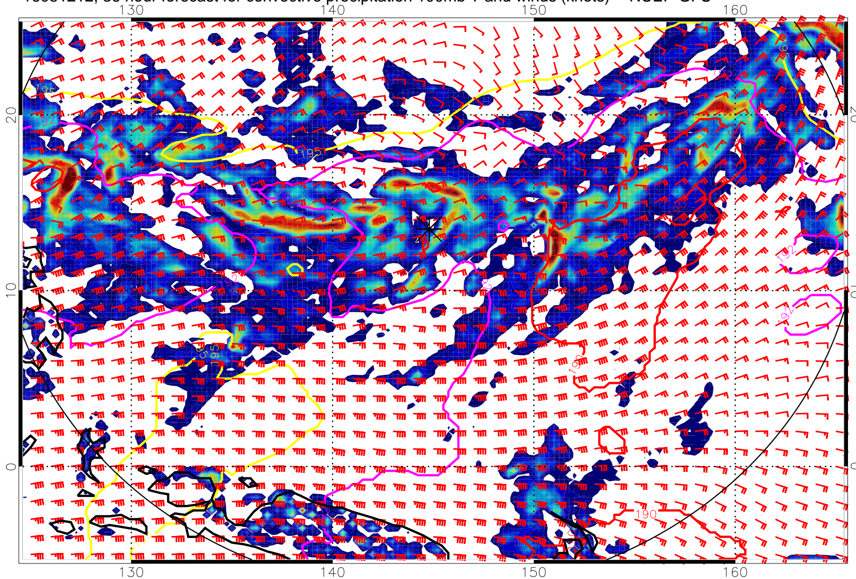
16081212, 36 hour forecast for convective precipitation 100mb T and winds (knots) -- NCEP GFS
