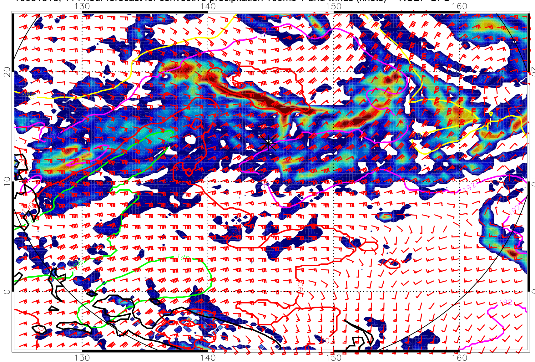
16081518, 114 hour forecast for convective precipitation 100mb T and winds (knots) -- NCEP GFS
