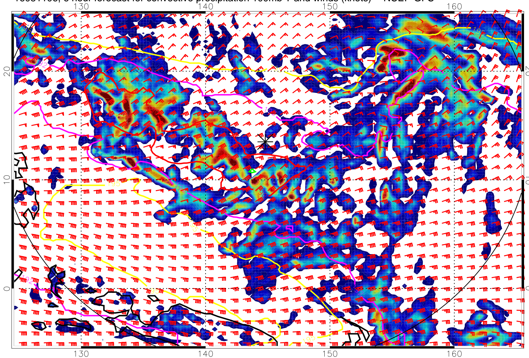
16081106, 6 hour forecast for convective precipitation 100mb T and winds (knots) -- NCEP GFS
