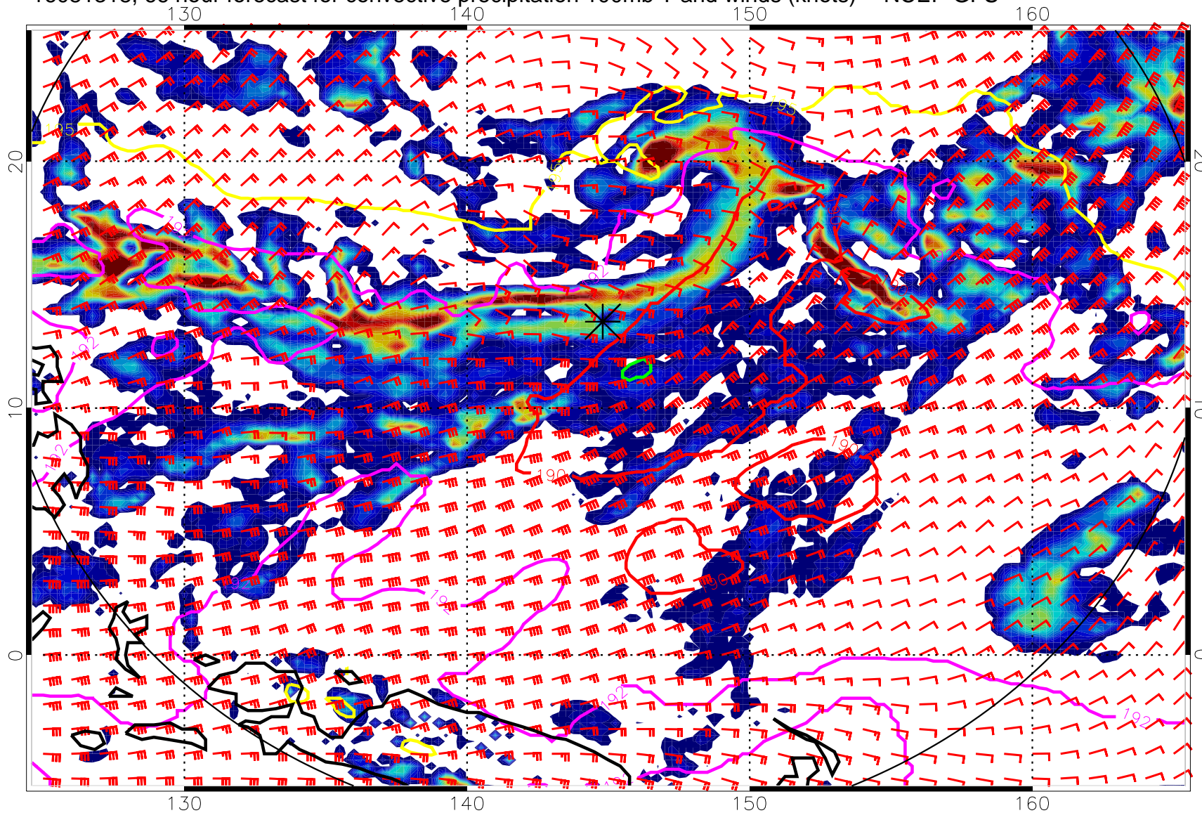
16081318, 66 hour forecast for convective precipitation 100mb T and winds (knots) -- NCEP GFS
