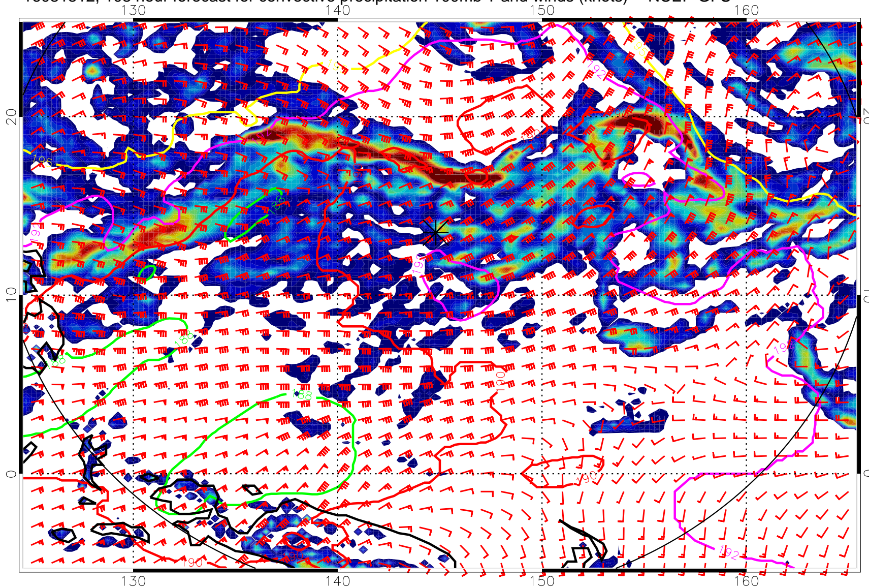
16081512, 108 hour forecast for convective precipitation 100mb T and winds (knots) -- NCEP GFS
