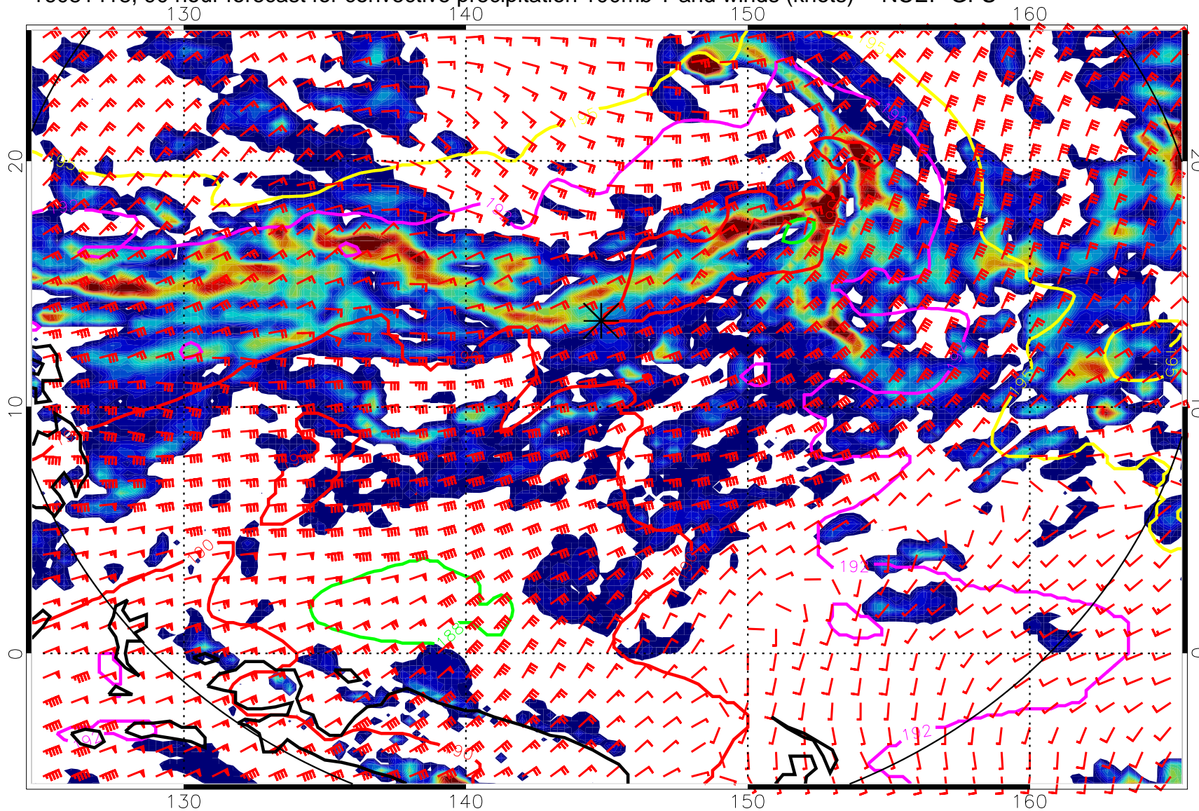
16081418, 90 hour forecast for convective precipitation 100mb T and winds (knots) -- NCEP GFS
