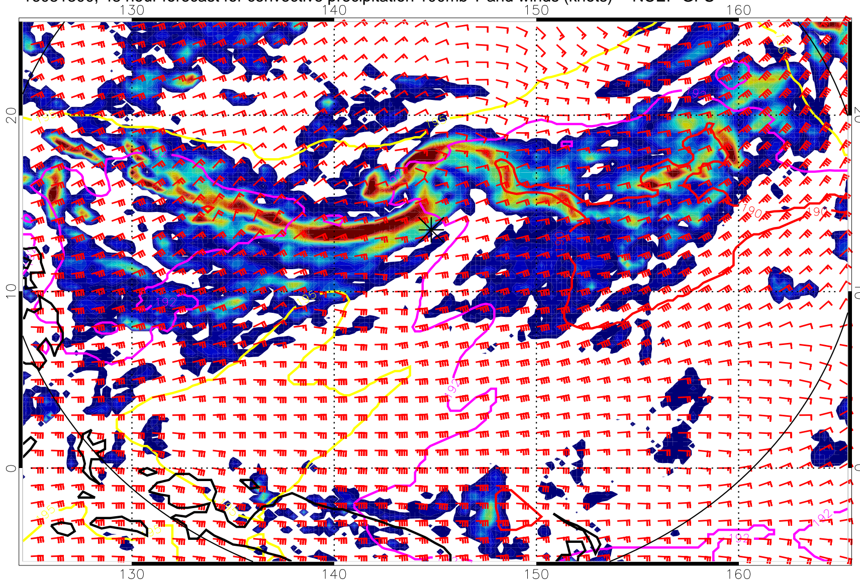
16081300, 48 hour forecast for convective precipitation 100mb T and winds (knots) -- NCEP GFS
