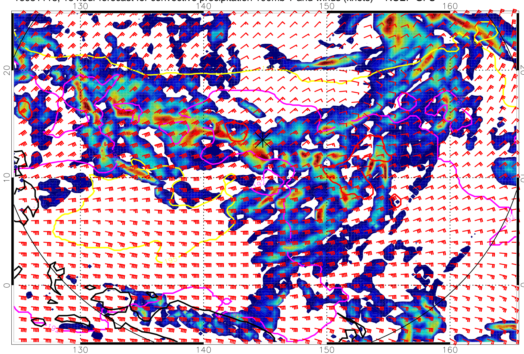
16081118, 18 hour forecast for convective precipitation 100mb T and winds (knots) -- NCEP GFS
