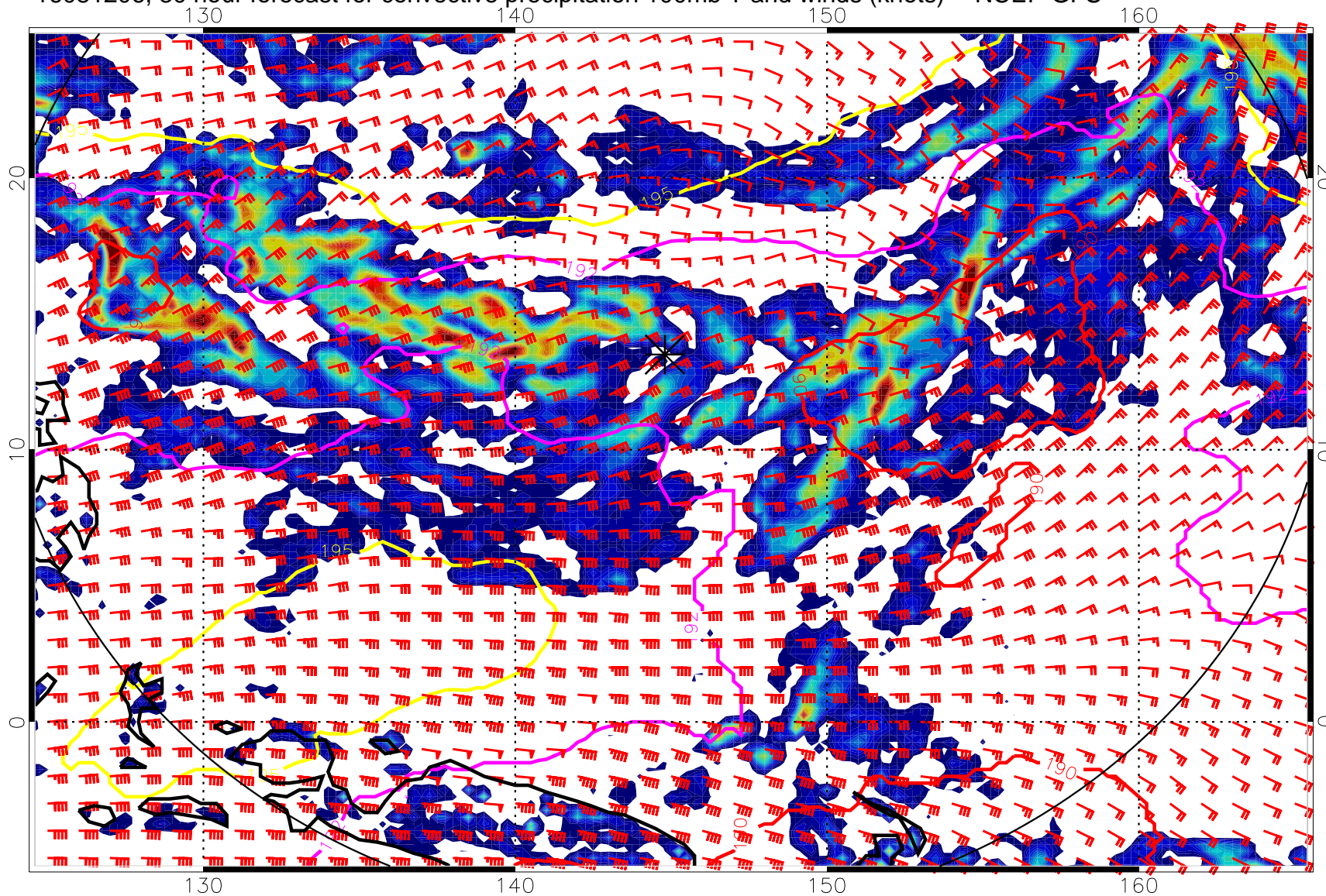
16081206, 30 hour forecast for convective precipitation 100mb T and winds (knots) -- NCEP GFS
