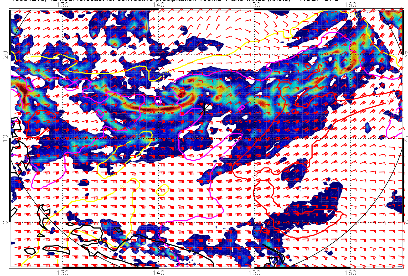
16081218, 42 hour forecast for convective precipitation 100mb T and winds (knots) -- NCEP GFS
