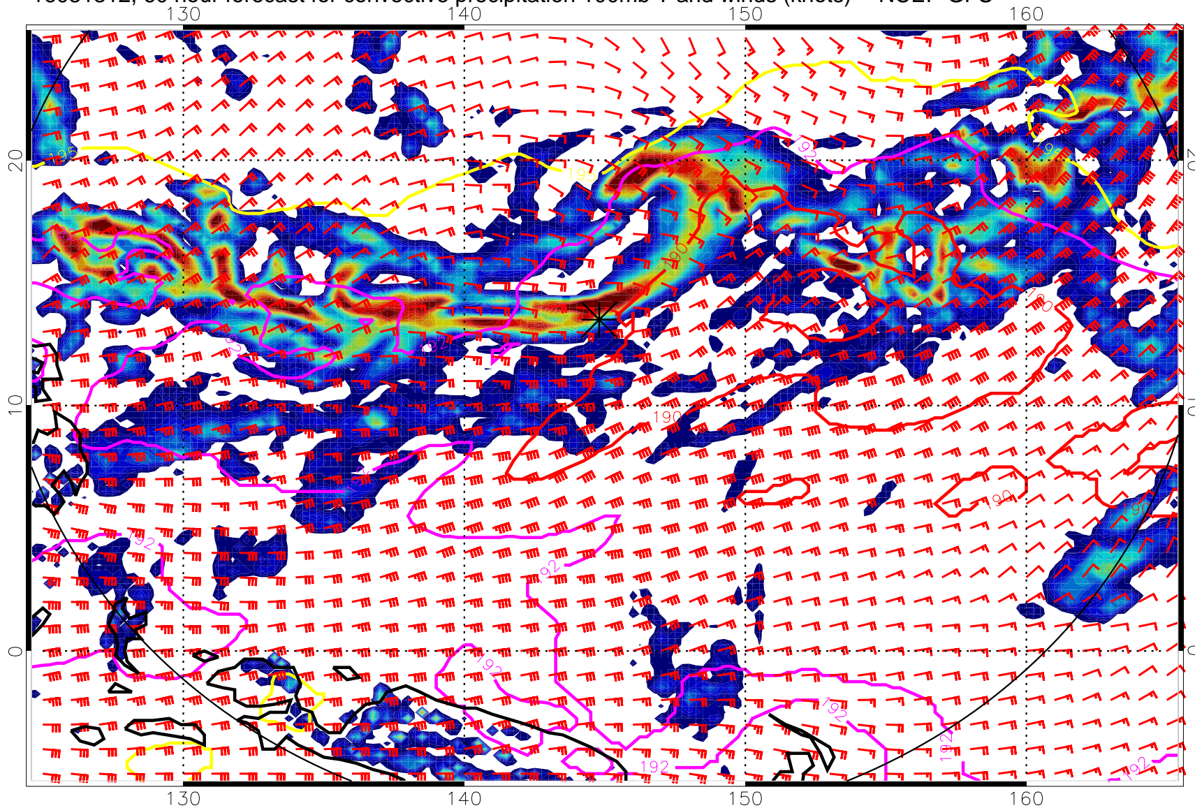
16081312, 60 hour forecast for convective precipitation 100mb T and winds (knots) -- NCEP GFS
