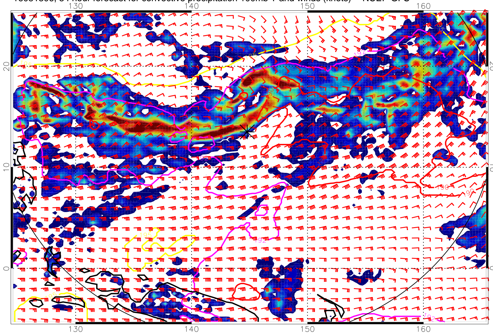
16081306, 54 hour forecast for convective precipitation 100mb T and winds (knots) -- NCEP GFS
