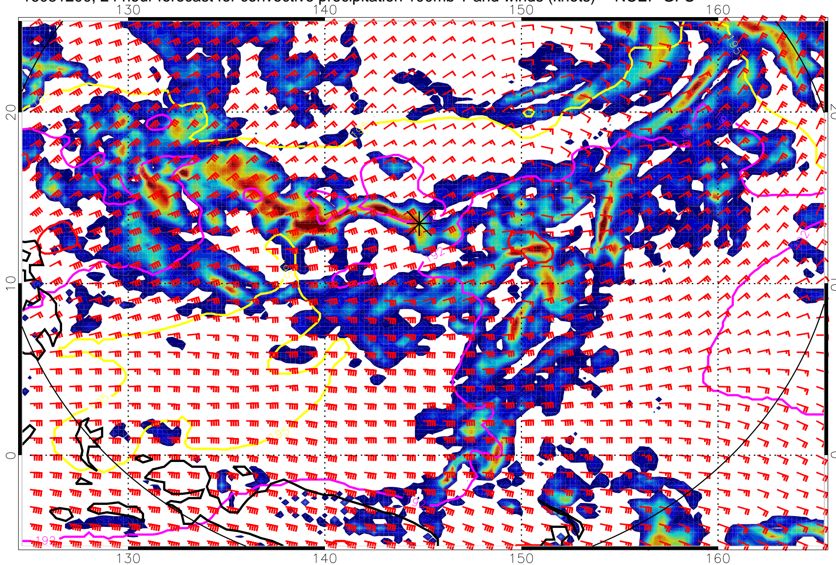
16081200, 24 hour forecast for convective precipitation 100mb T and winds (knots) -- NCEP GFS
