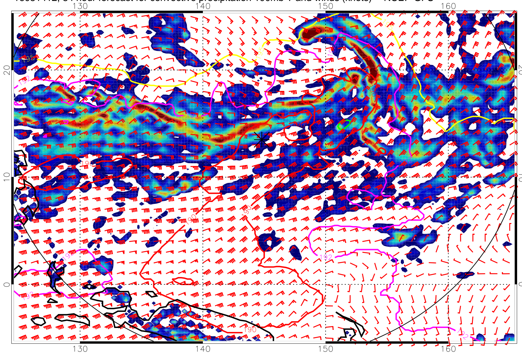
16081412, 84 hour forecast for convective precipitation 100mb T and winds (knots) -- NCEP GFS
