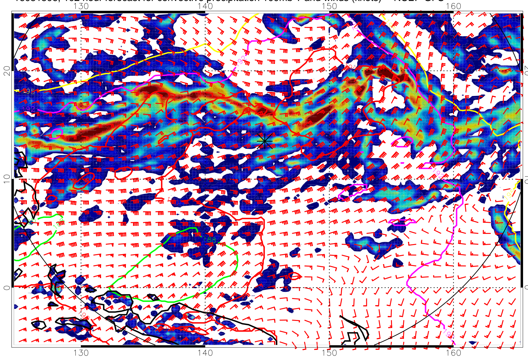
16081506, 102 hour forecast for convective precipitation 100mb T and winds (knots) -- NCEP GFS
