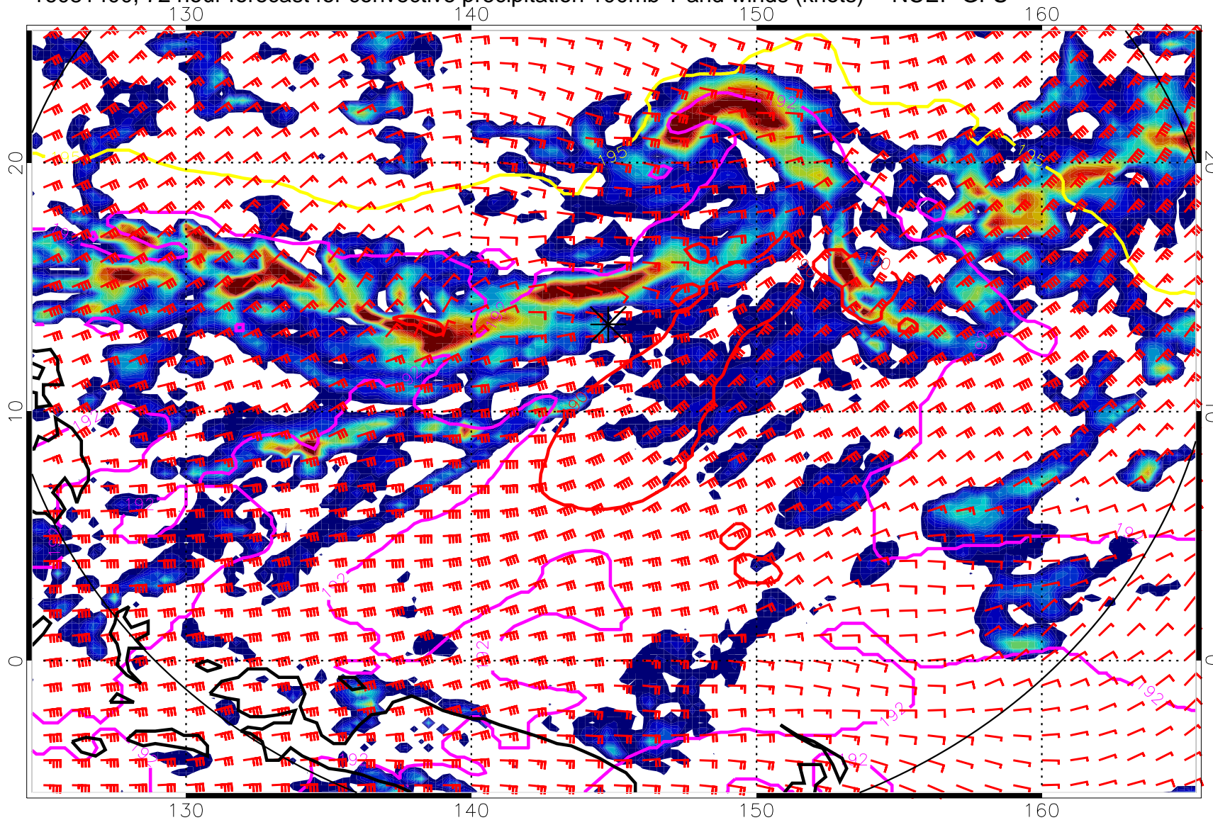
16081400, 72 hour forecast for convective precipitation 100mb T and winds (knots) -- NCEP GFS
