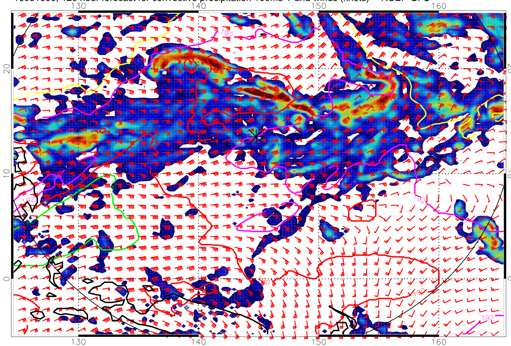
16081600, 120 hour forecast for convective precipitation 100mb T and winds (knots) -- NCEP GFS
