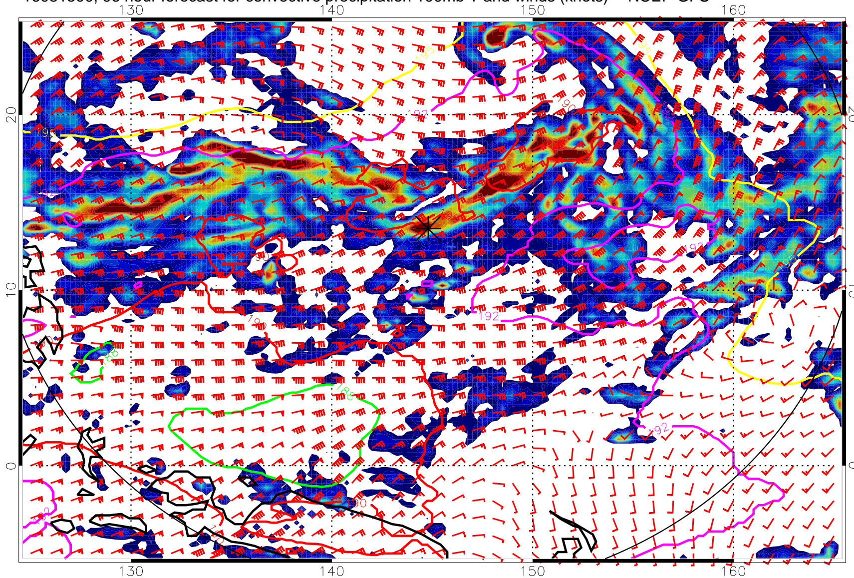
16081500, 96 hour forecast for convective precipitation 100mb T and winds (knots) -- NCEP GFS
