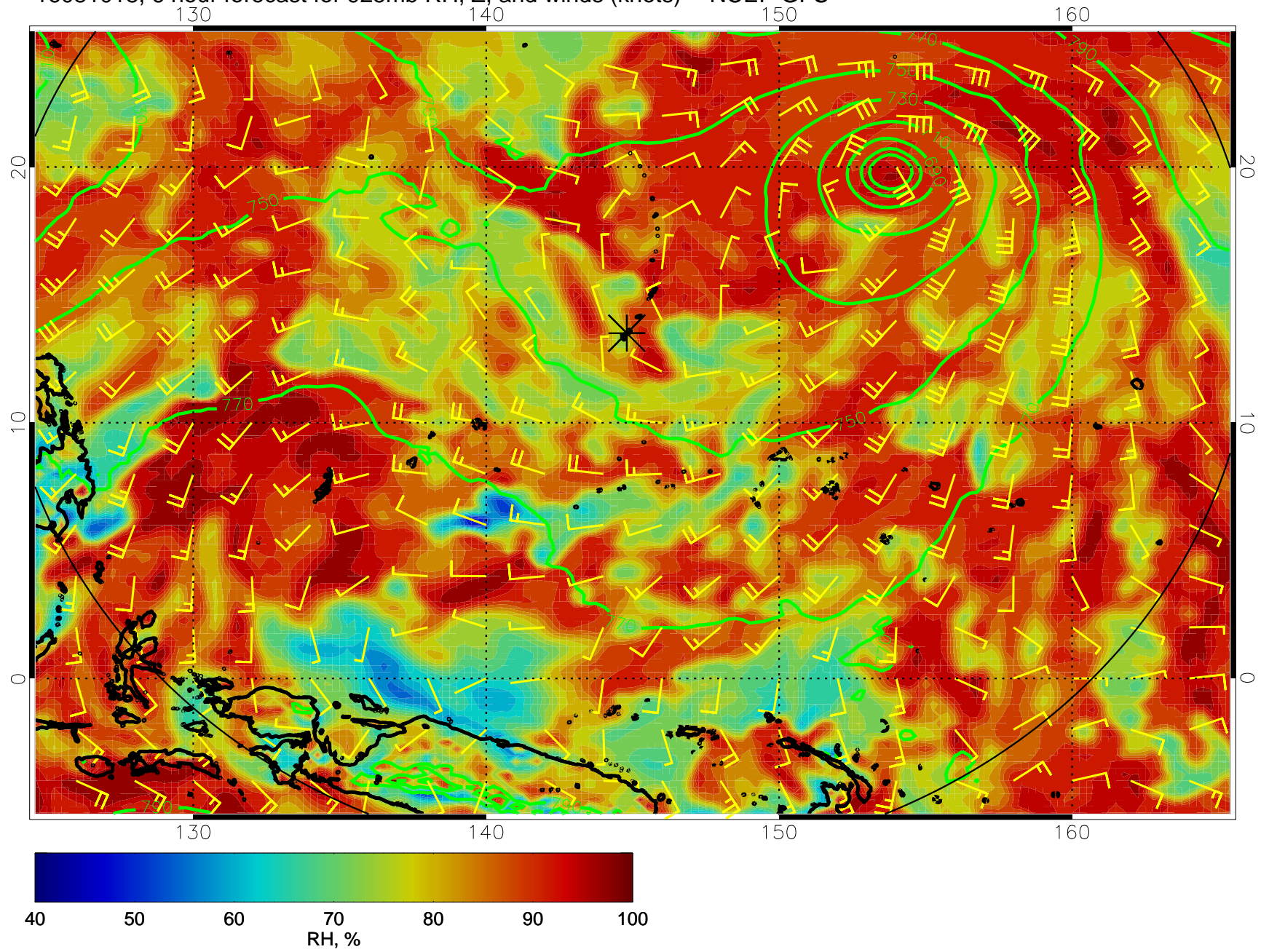
16081018, 6 hour forecast for 925mb RH, Z, and winds (knots) -- NCEP GFS
