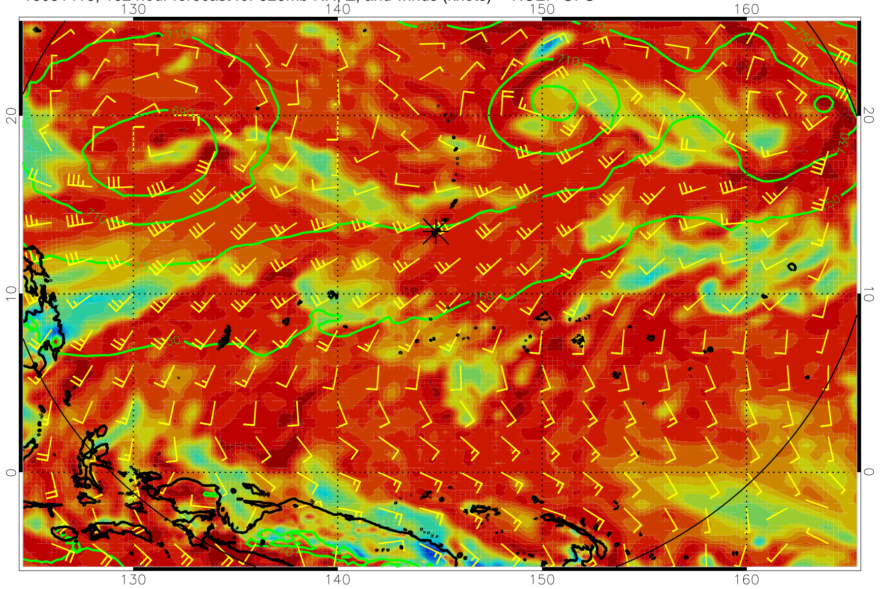
16081418, 102 hour forecast for 925mb RH, Z, and winds (knots) -- NCEP GFS
