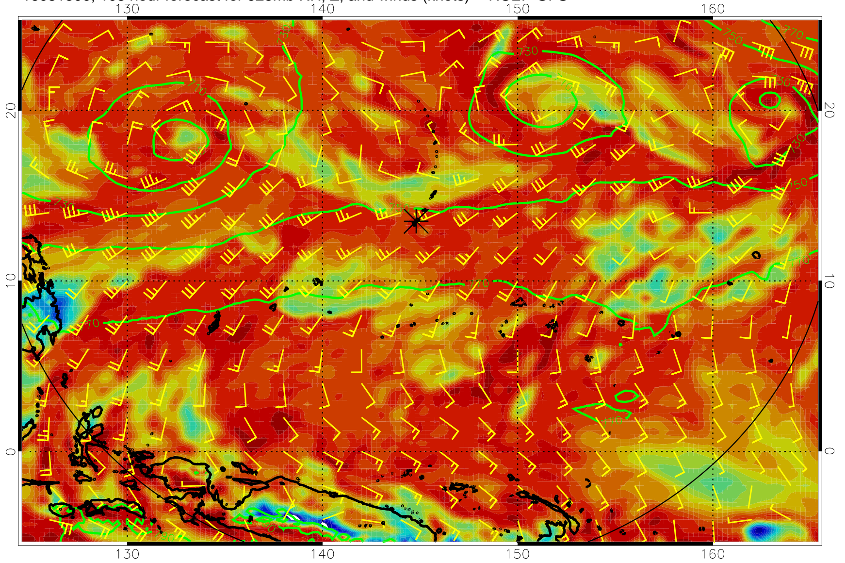
16081500, 108 hour forecast for 925mb RH, Z, and winds (knots) -- NCEP GFS
