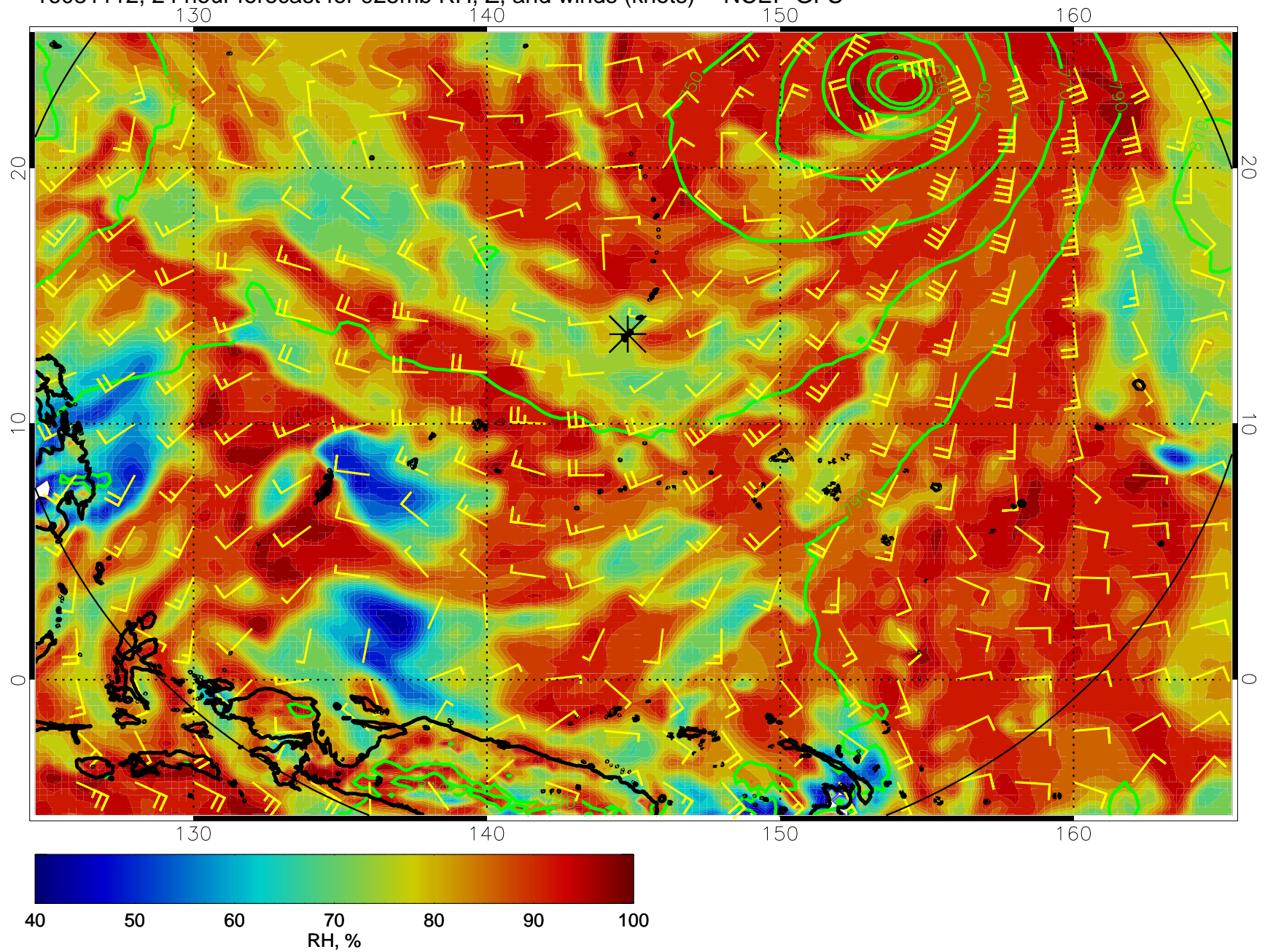
16081112, 24 hour forecast for 925mb RH, Z, and winds (knots) -- NCEP GFS
