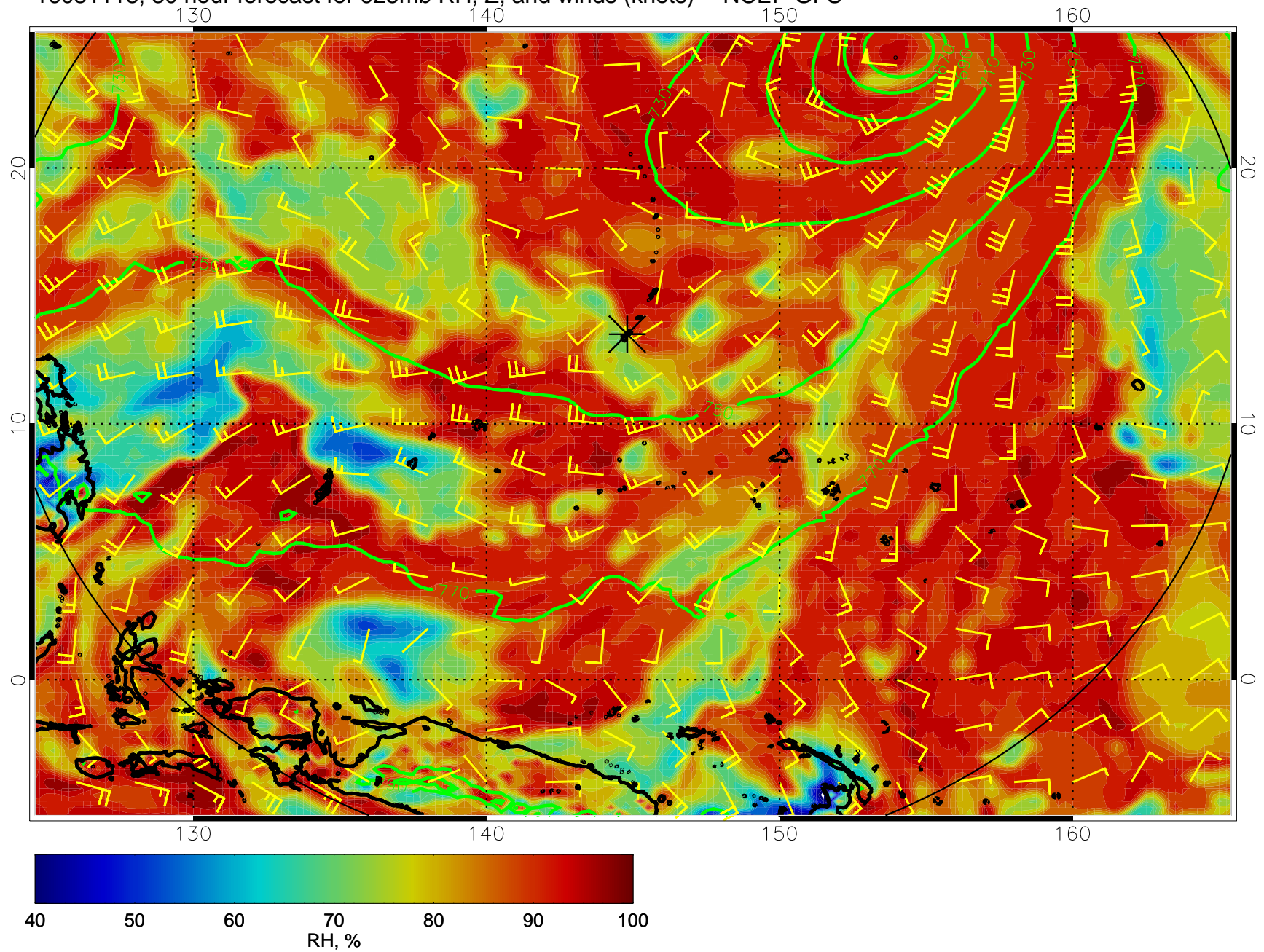
16081118, 30 hour forecast for 925mb RH, Z, and winds (knots) -- NCEP GFS
