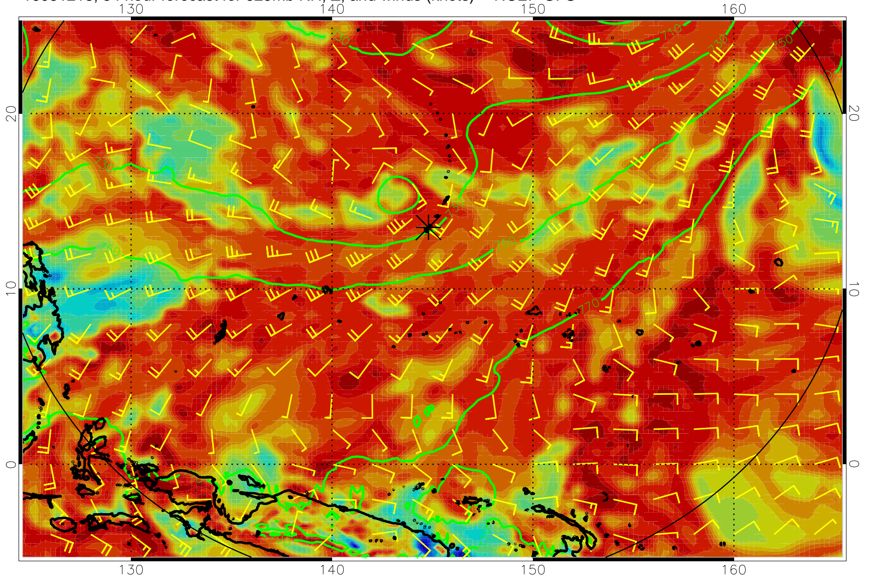
16081218, 54 hour forecast for 925mb RH, Z, and winds (knots) -- NCEP GFS
