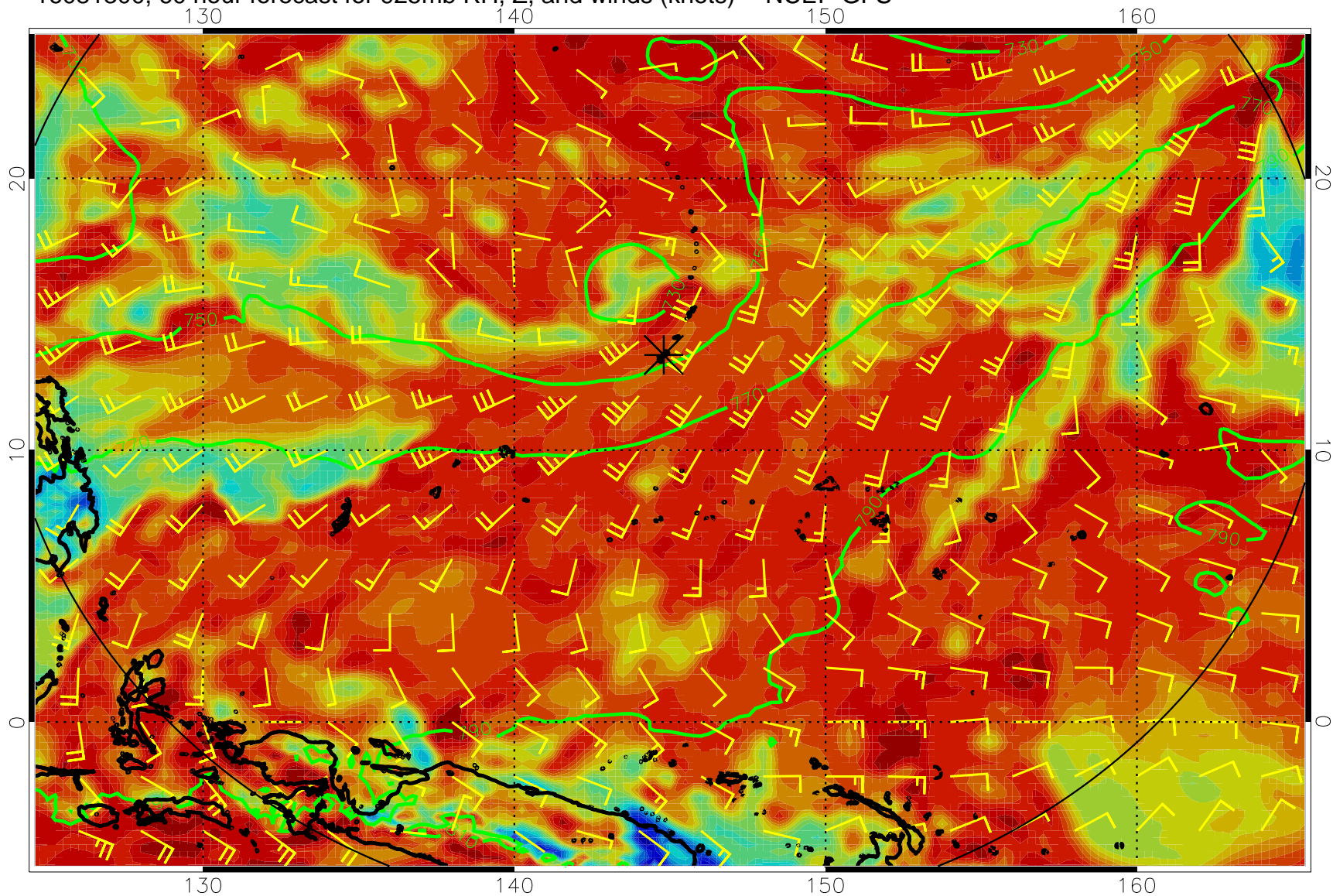
16081300, 60 hour forecast for 925mb RH, Z, and winds (knots) -- NCEP GFS
