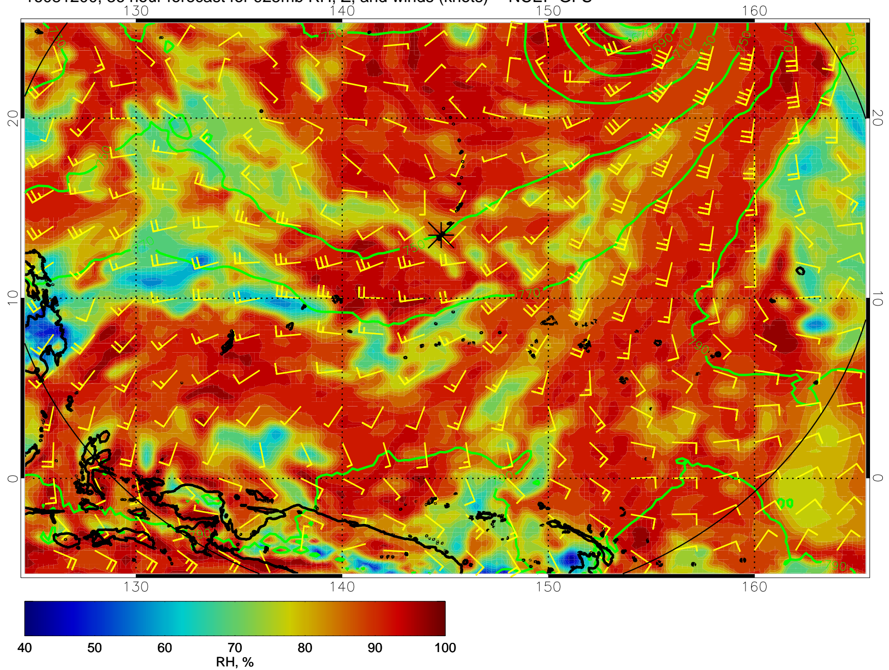
16081200, 36 hour forecast for 925mb RH, Z, and winds (knots) -- NCEP GFS
