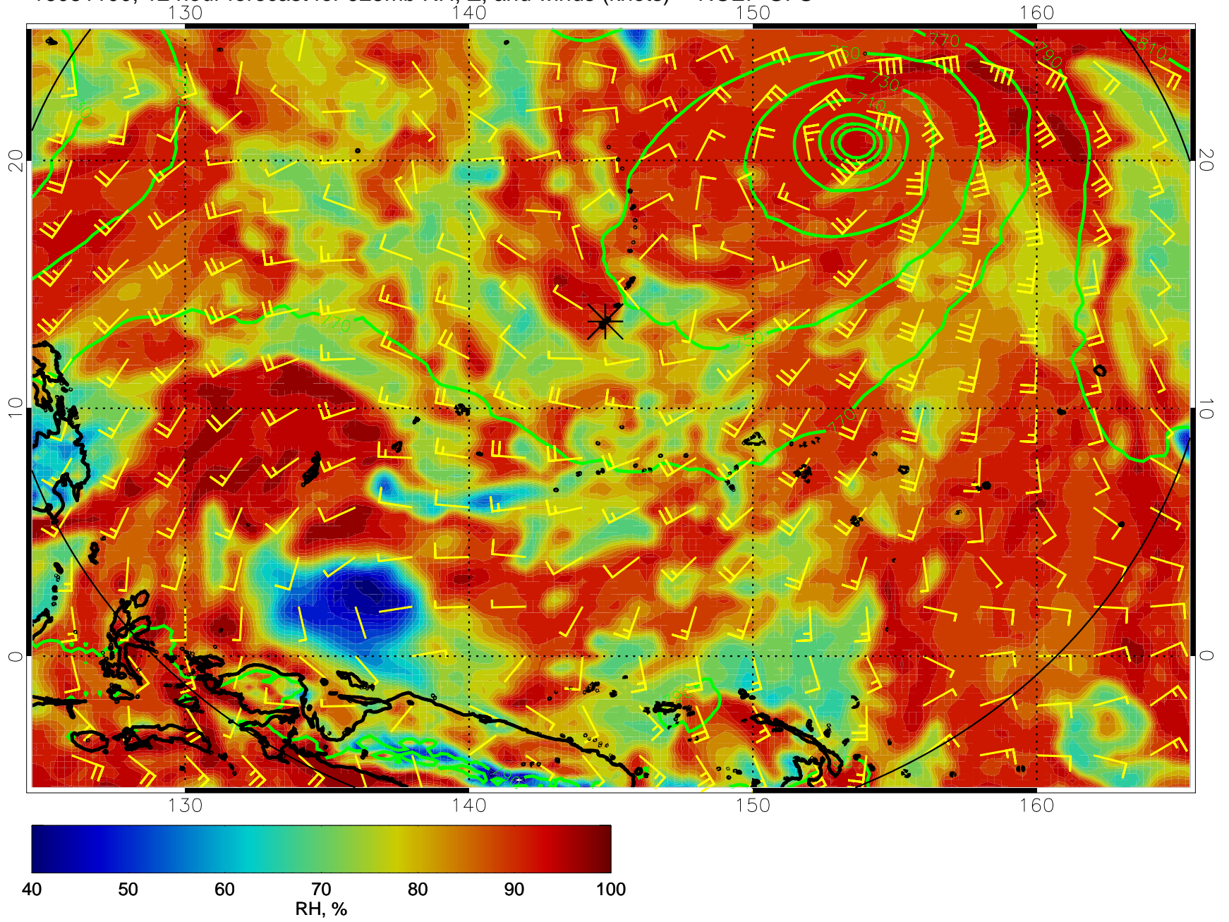
16081100, 12 hour forecast for 925mb RH, Z, and winds (knots) -- NCEP GFS
