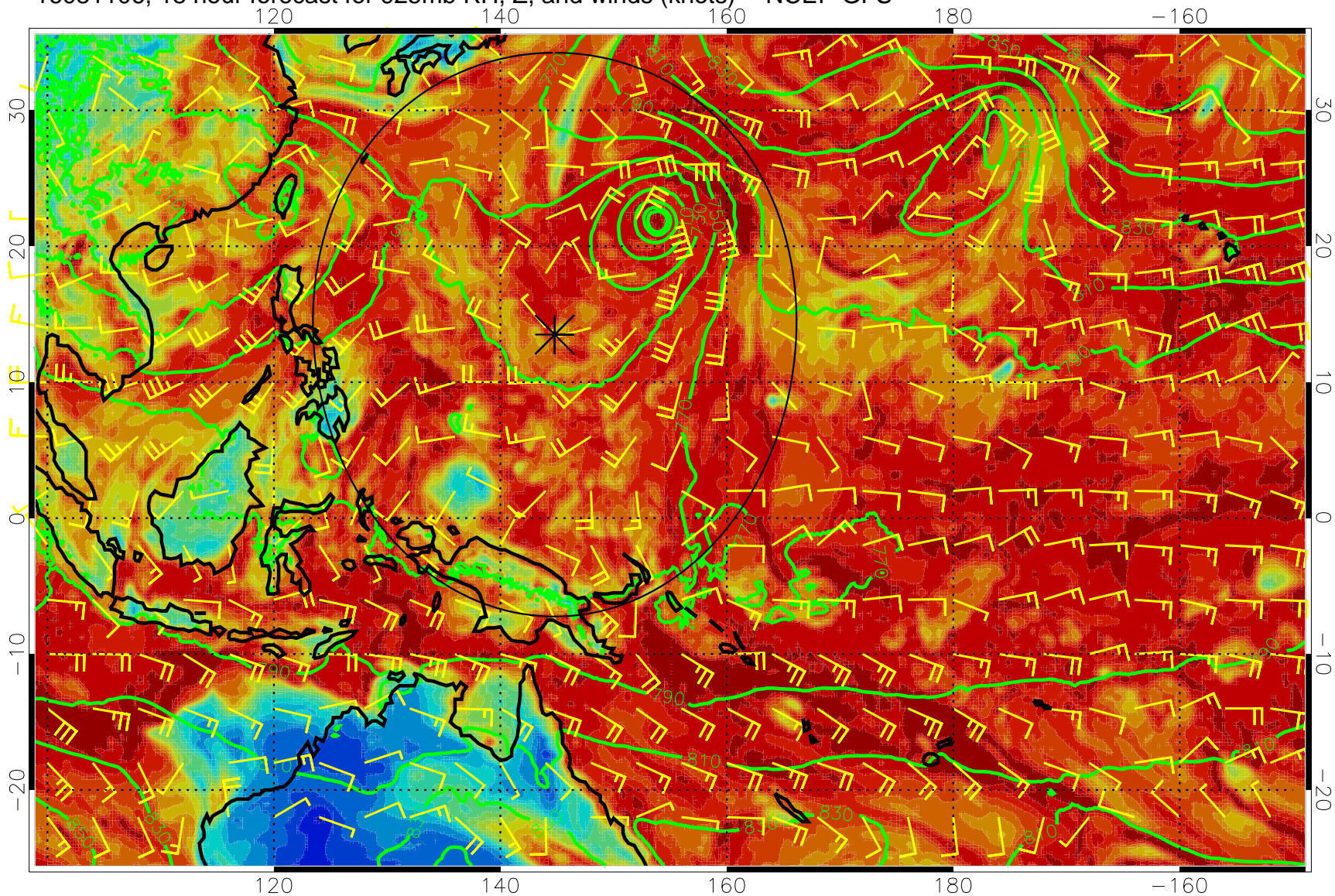
16081106, 18 hour forecast for 925mb RH, Z, and winds (knots) -- NCEP GFS
