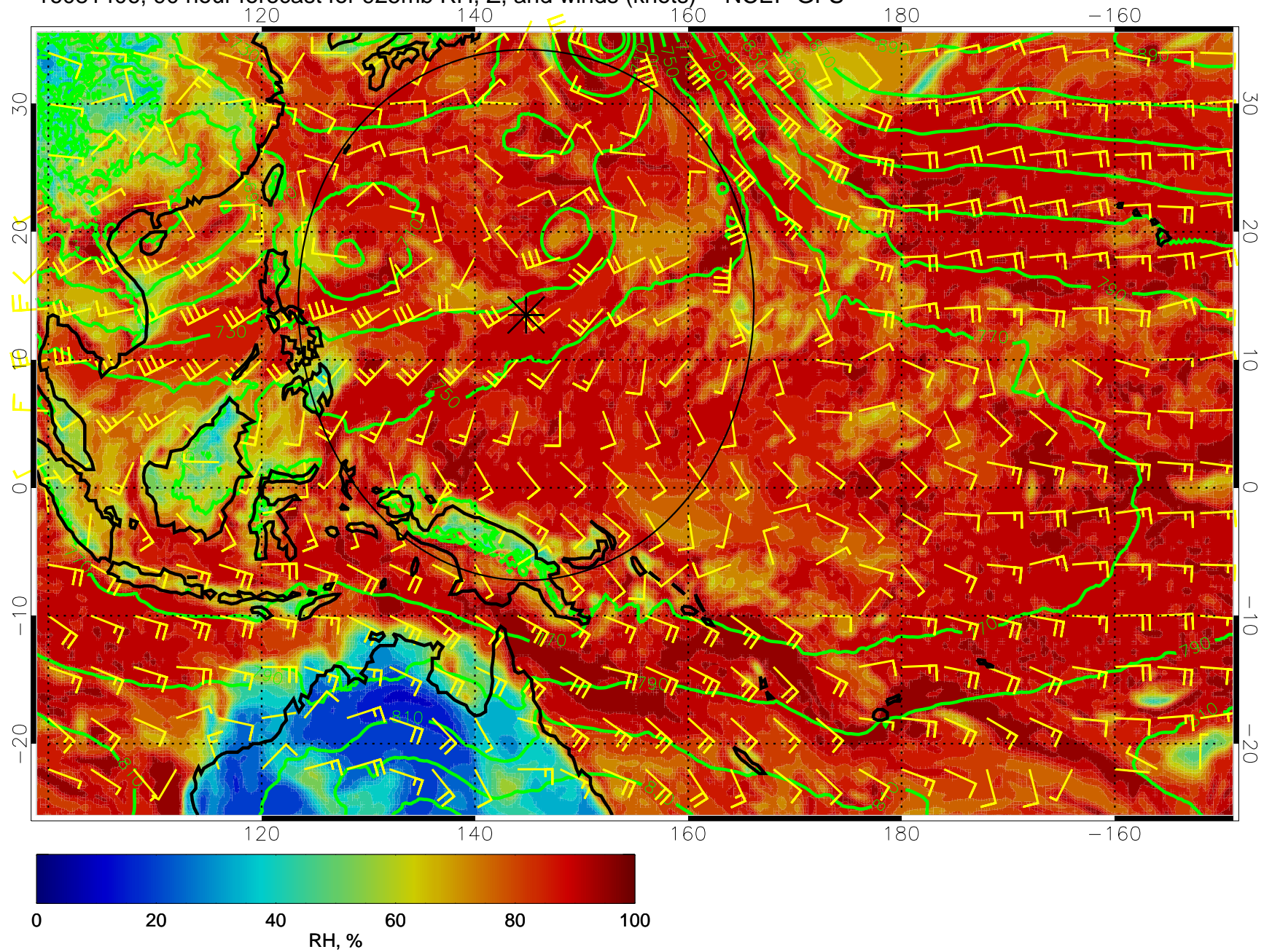
16081406, 90 hour forecast for 925mb RH, Z, and winds (knots) -- NCEP GFS
