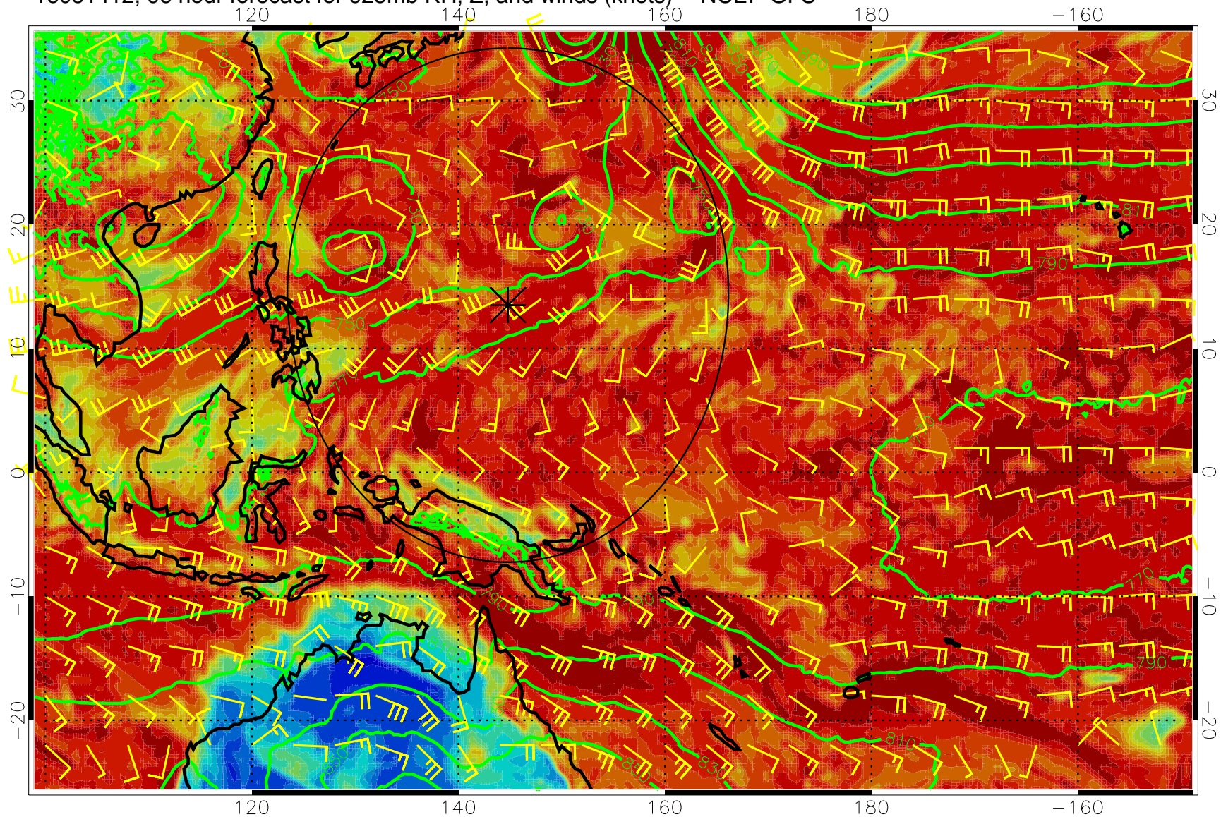
16081412, 96 hour forecast for 925mb RH, Z, and winds (knots) -- NCEP GFS
