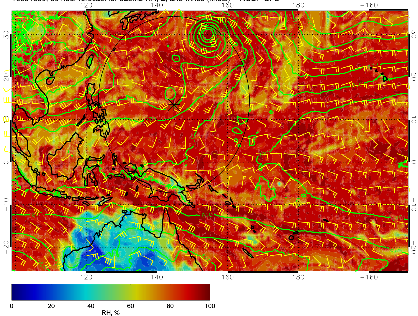
16081300, 60 hour forecast for 925mb RH, Z, and winds (knots) -- NCEP GFS
