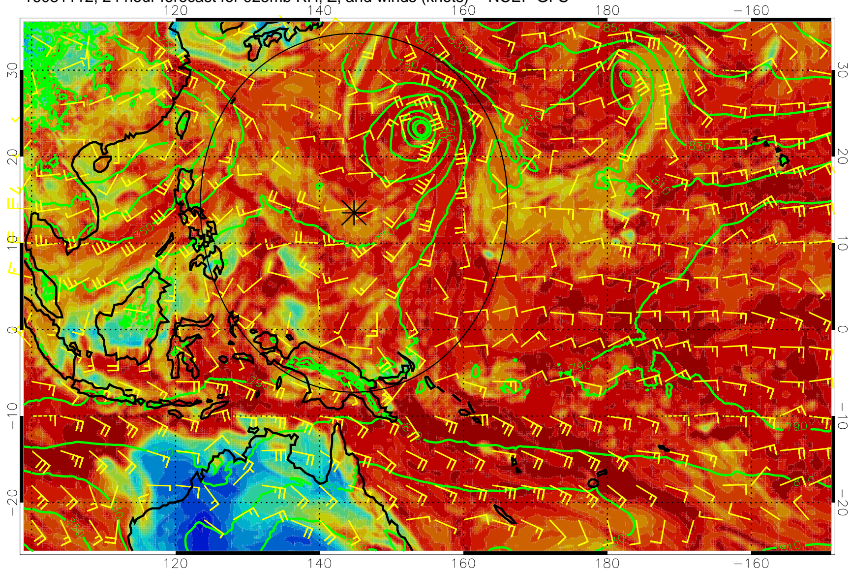
16081112, 24 hour forecast for 925mb RH, Z, and winds (knots) -- NCEP GFS
