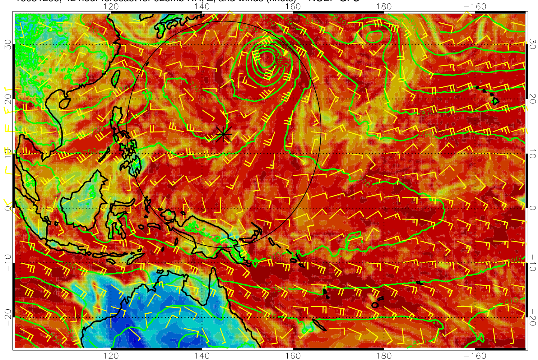
16081206, 42 hour forecast for 925mb RH, Z, and winds (knots) -- NCEP GFS
