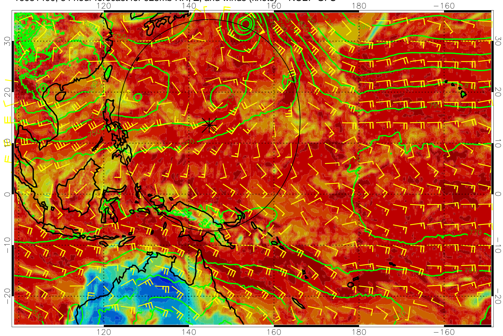
16081400, 84 hour forecast for 925mb RH, Z, and winds (knots) -- NCEP GFS
