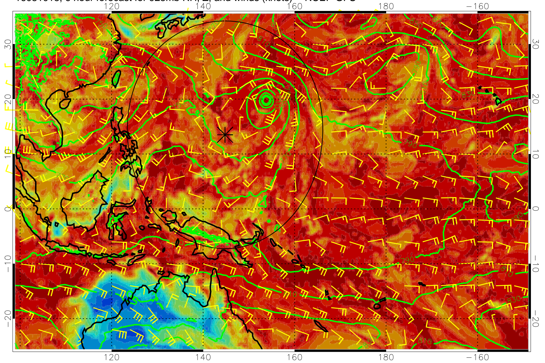
16081018, 6 hour forecast for 925mb RH, Z, and winds (knots) -- NCEP GFS
