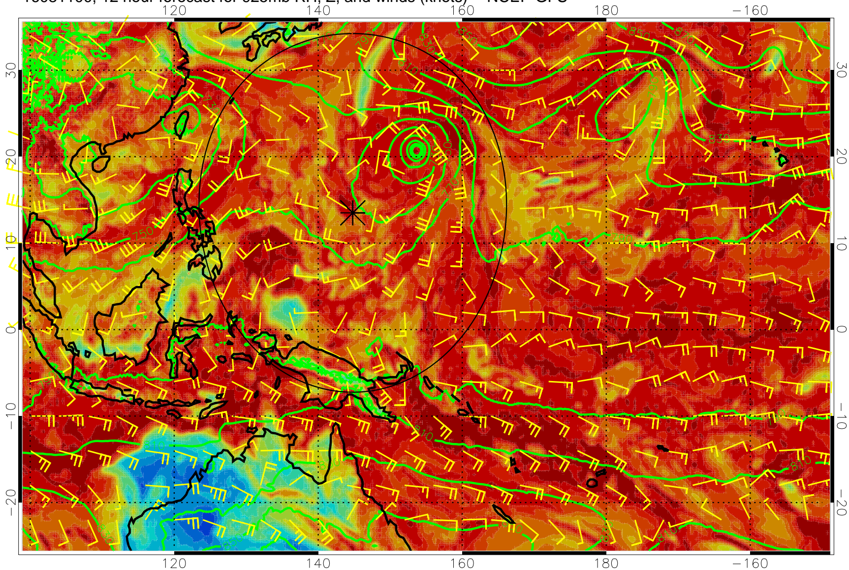
16081100, 12 hour forecast for 925mb RH, Z, and winds (knots) -- NCEP GFS
