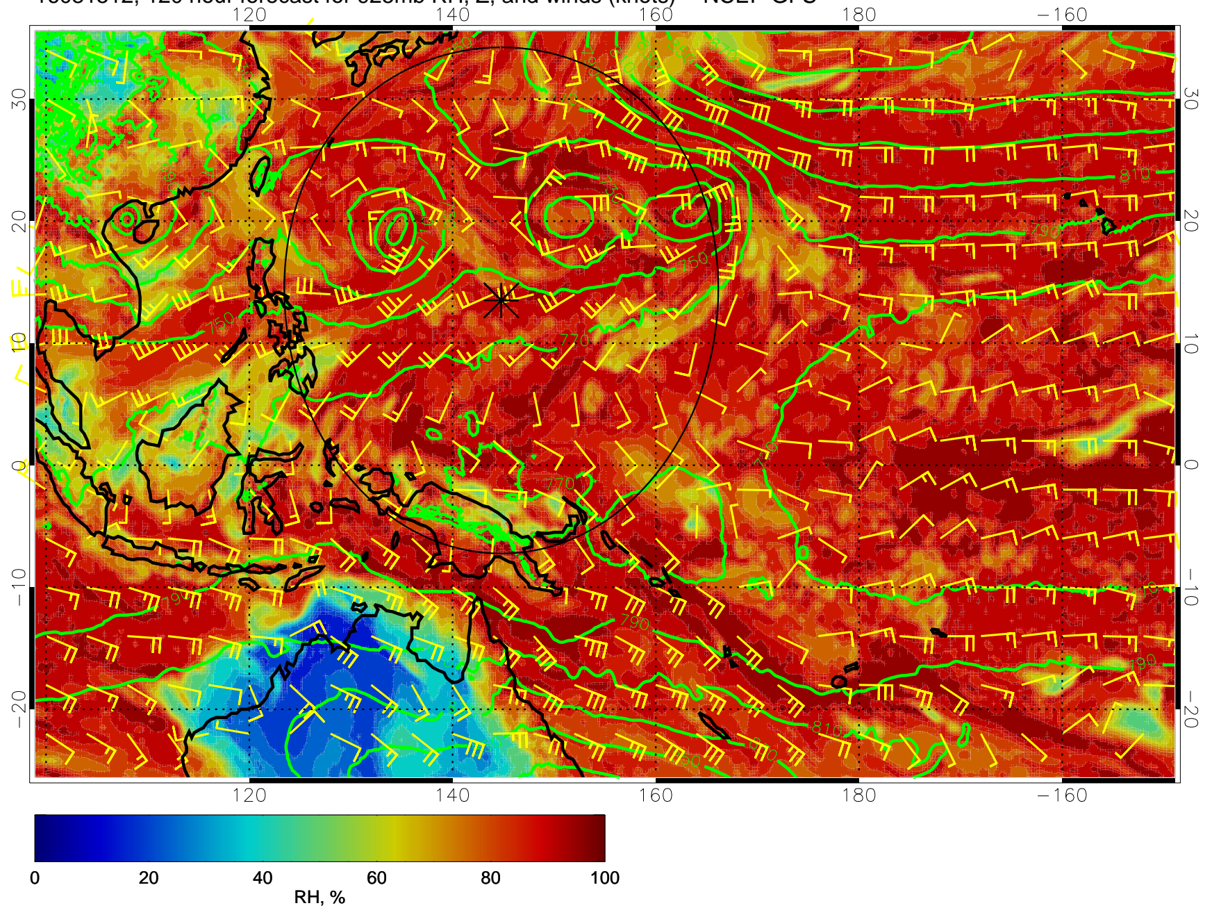
16081512, 120 hour forecast for 925mb RH, Z, and winds (knots) -- NCEP GFS
