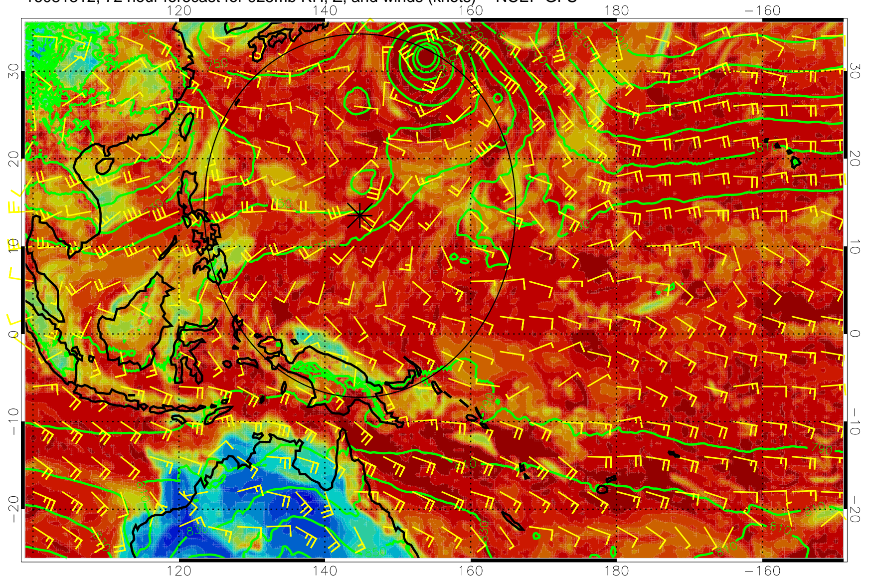
16081312, 72 hour forecast for 925mb RH, Z, and winds (knots) -- NCEP GFS
