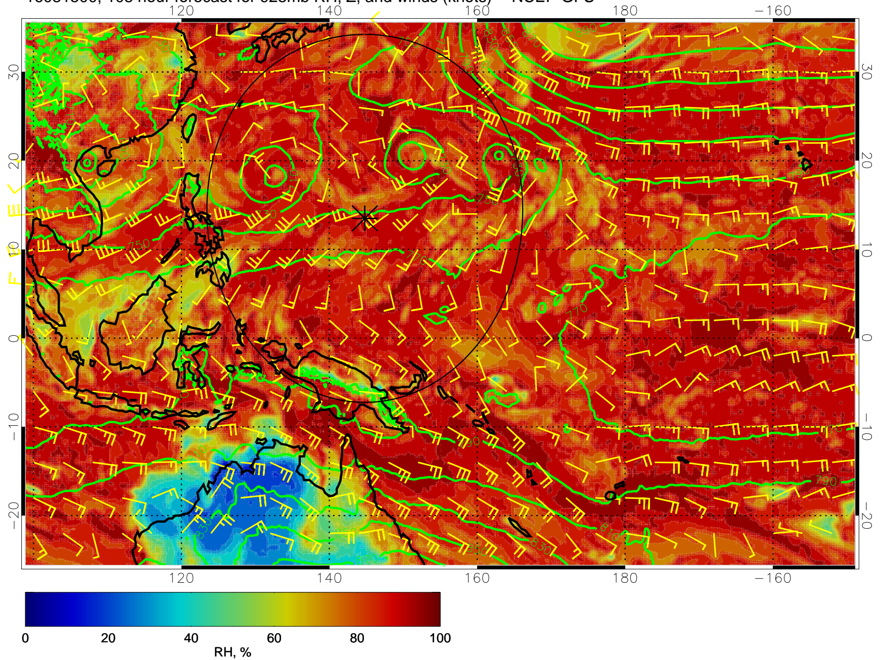
16081500, 108 hour forecast for 925mb RH, Z, and winds (knots) -- NCEP GFS
