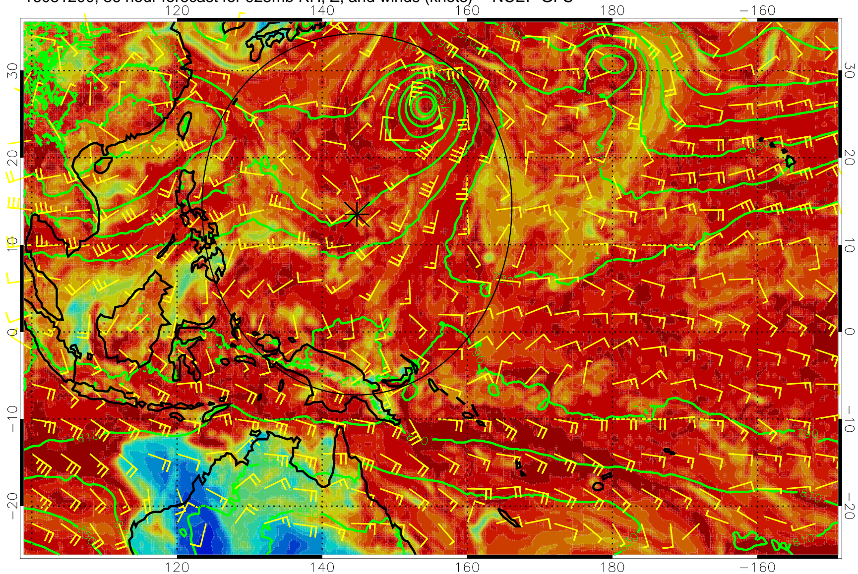
16081200, 36 hour forecast for 925mb RH, Z, and winds (knots) -- NCEP GFS
