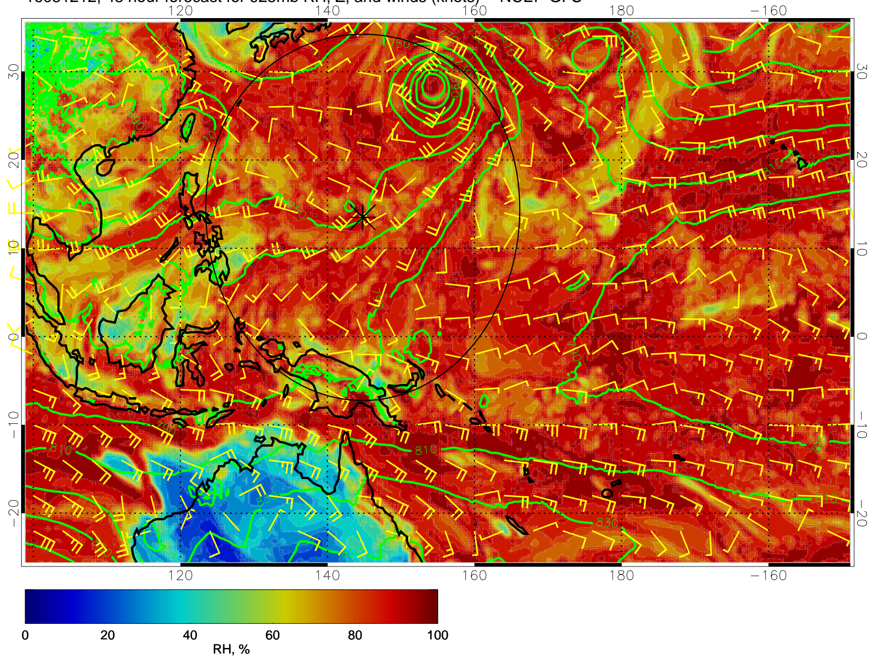
16081212, 48 hour forecast for 925mb RH, Z, and winds (knots) -- NCEP GFS
