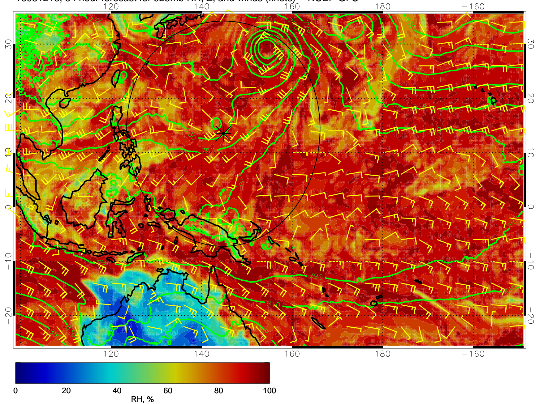
16081218, 54 hour forecast for 925mb RH, Z, and winds (knots) -- NCEP GFS
