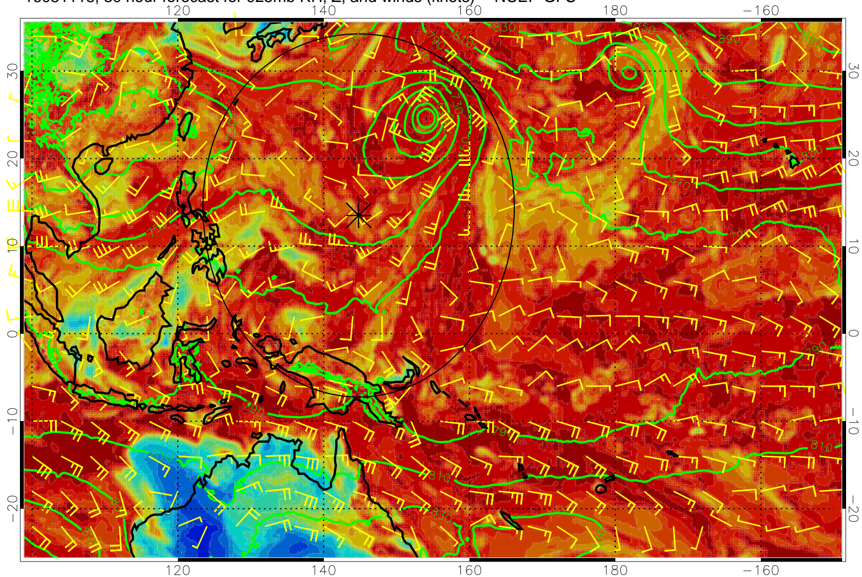
16081118, 30 hour forecast for 925mb RH, Z, and winds (knots) -- NCEP GFS
