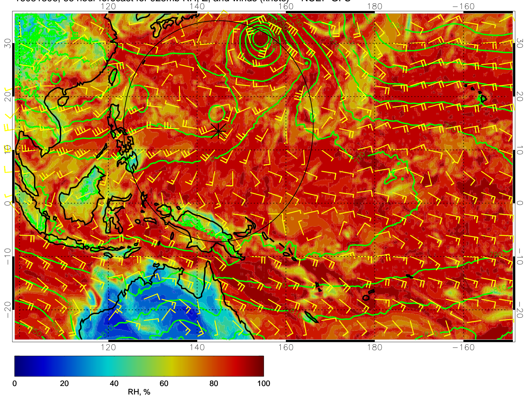
16081306, 66 hour forecast for 925mb RH, Z, and winds (knots) -- NCEP GFS
