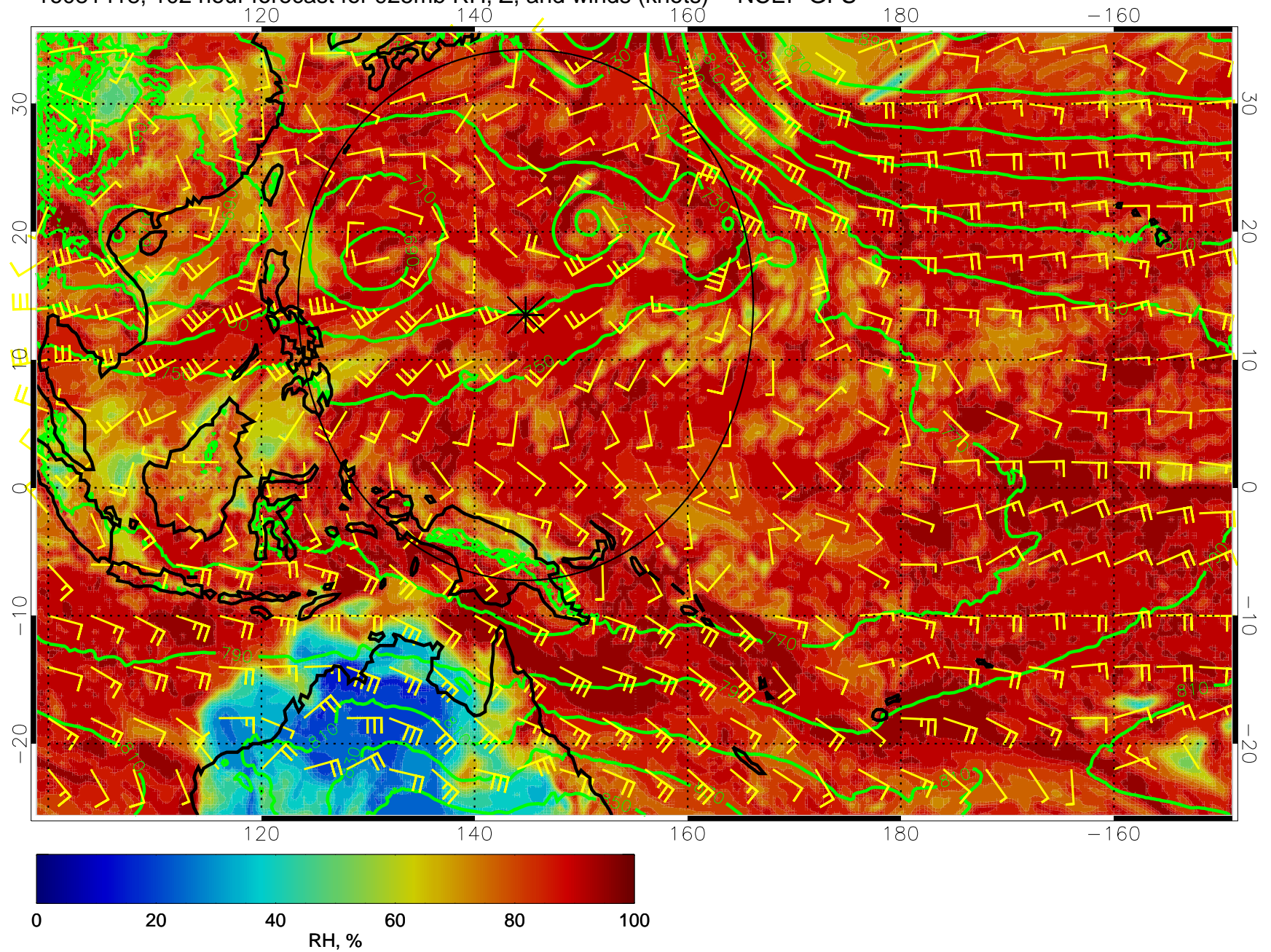
16081418, 102 hour forecast for 925mb RH, Z, and winds (knots) -- NCEP GFS
