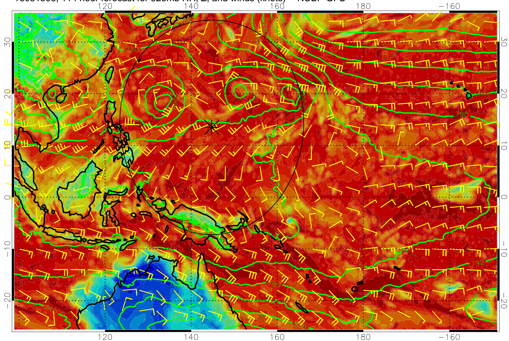
16081506, 114 hour forecast for 925mb RH, Z, and winds (knots) -- NCEP GFS
