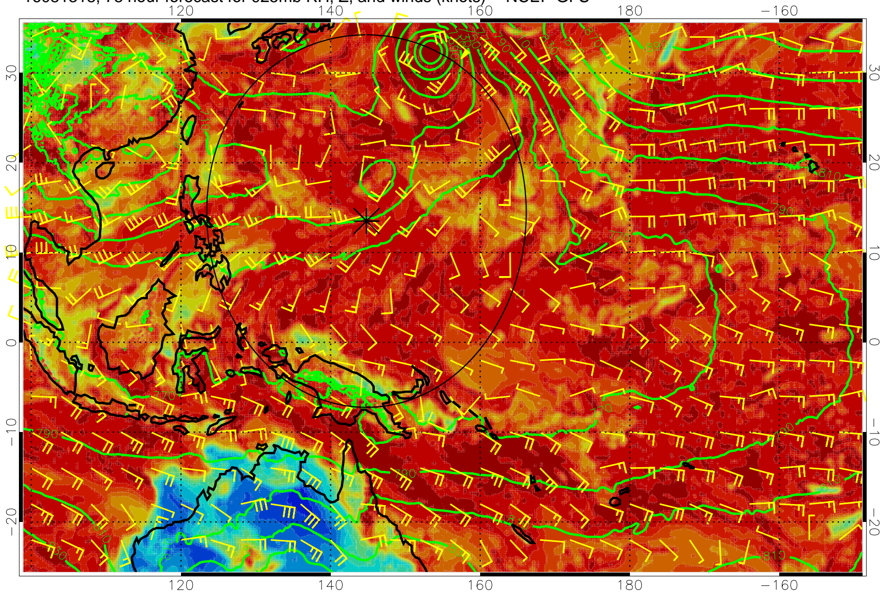
16081318, 78 hour forecast for 925mb RH, Z, and winds (knots) -- NCEP GFS
