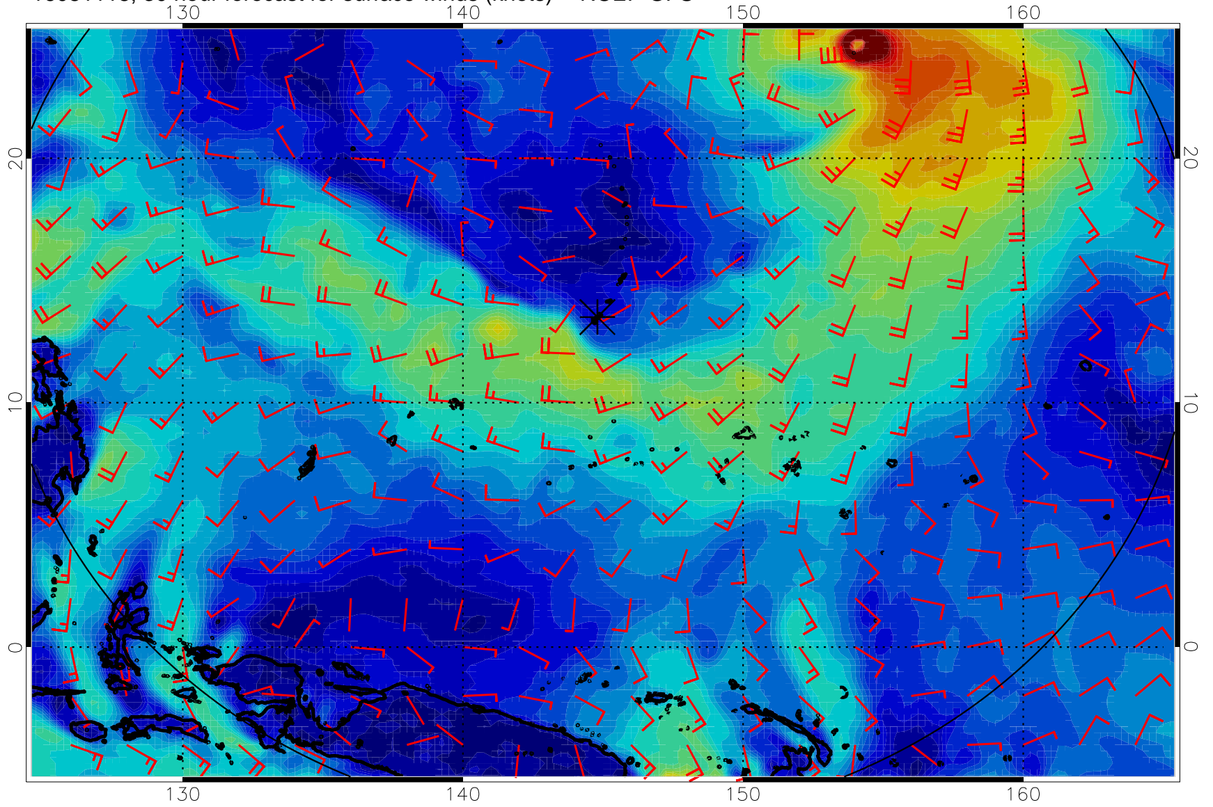
16081118, 30 hour forecast for surface winds (knots) -- NCEP GFS
