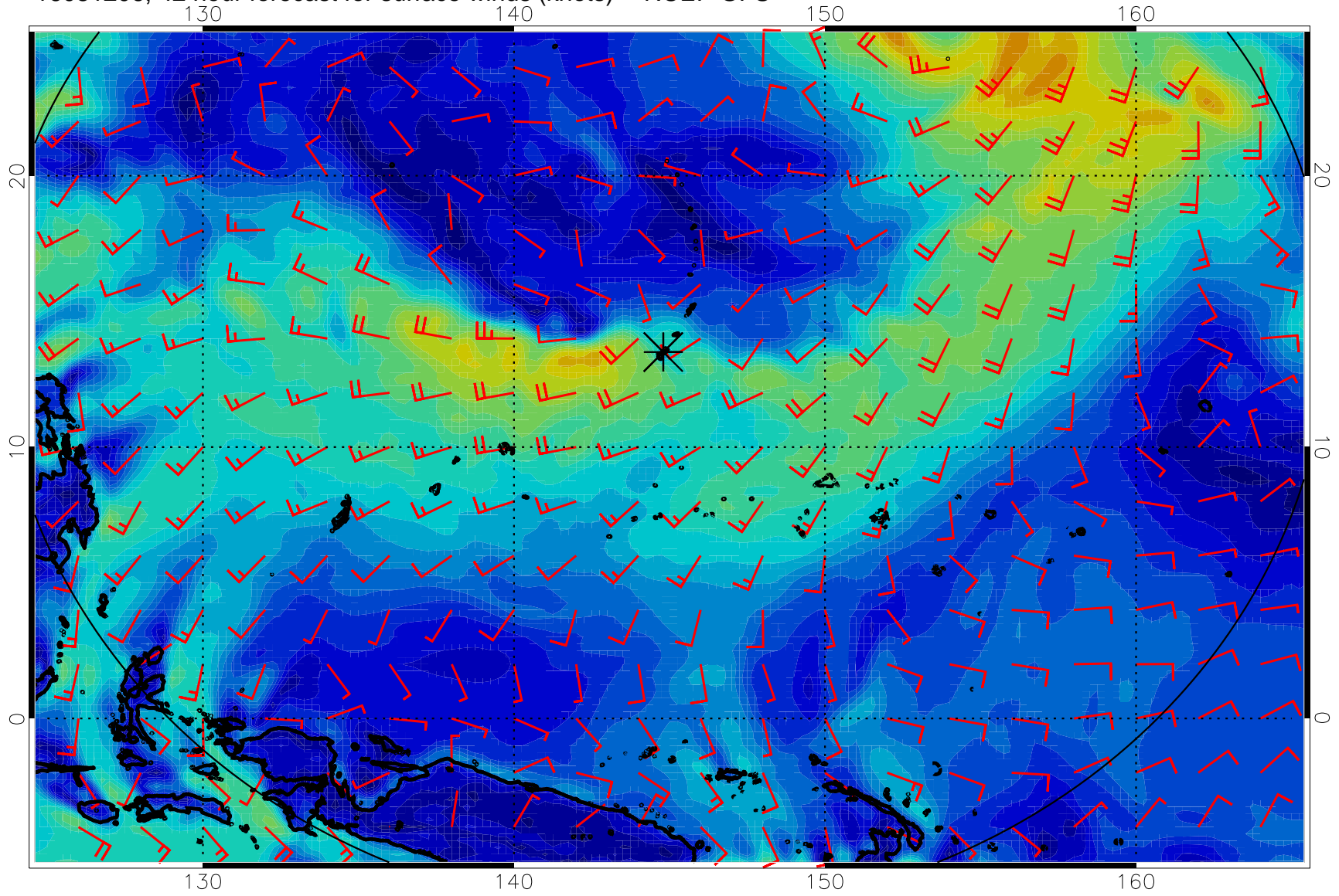
16081206, 42 hour forecast for surface winds (knots) -- NCEP GFS
