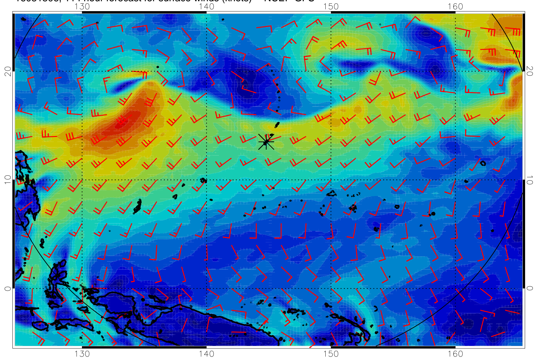
16081506, 114 hour forecast for surface winds (knots) -- NCEP GFS
