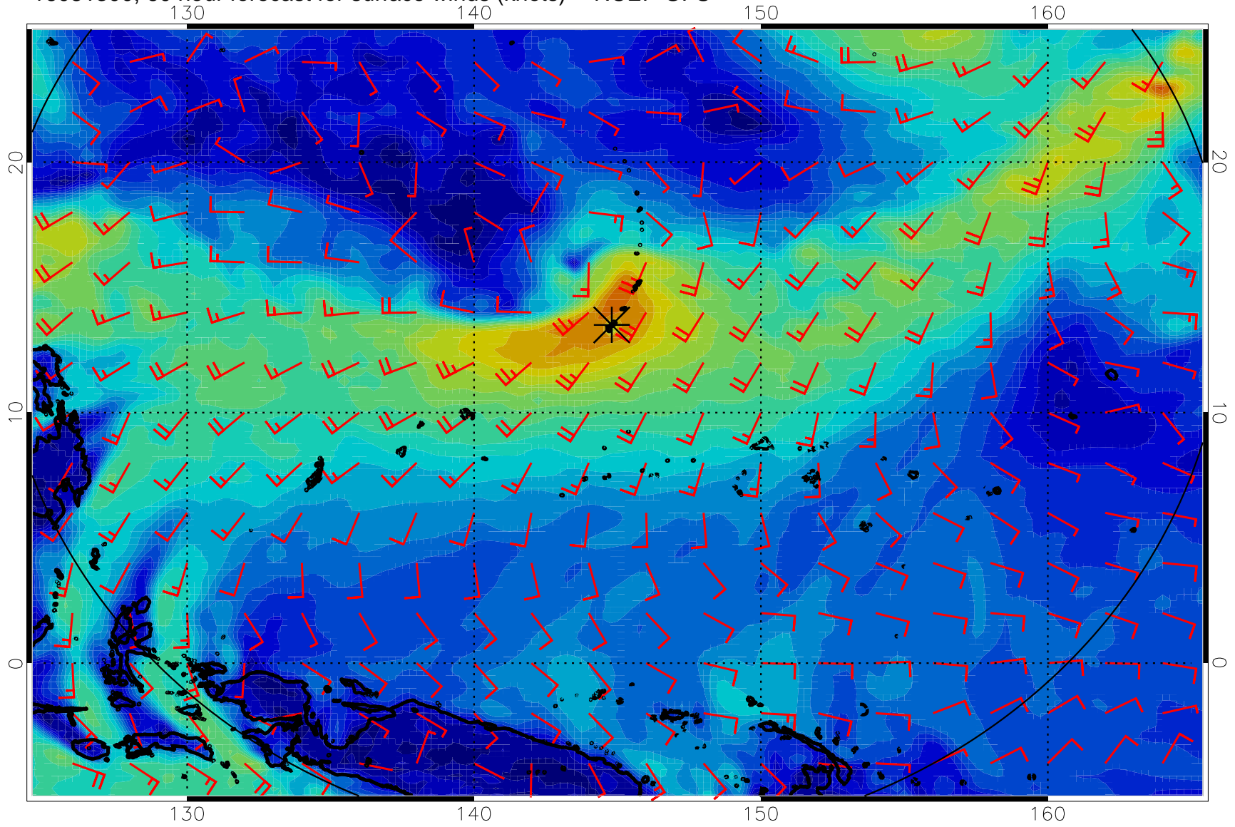
16081300, 60 hour forecast for surface winds (knots) -- NCEP GFS
