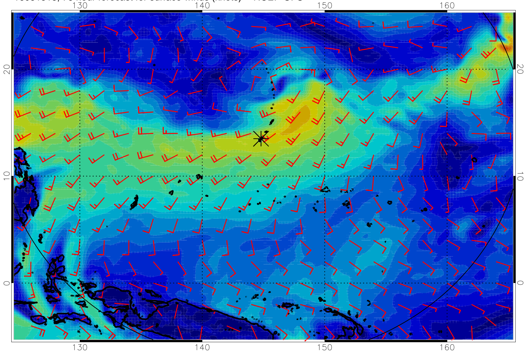
16081318, 78 hour forecast for surface winds (knots) -- NCEP GFS
