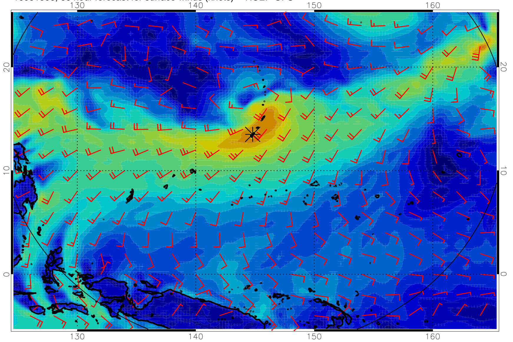
16081306, 66 hour forecast for surface winds (knots) -- NCEP GFS
