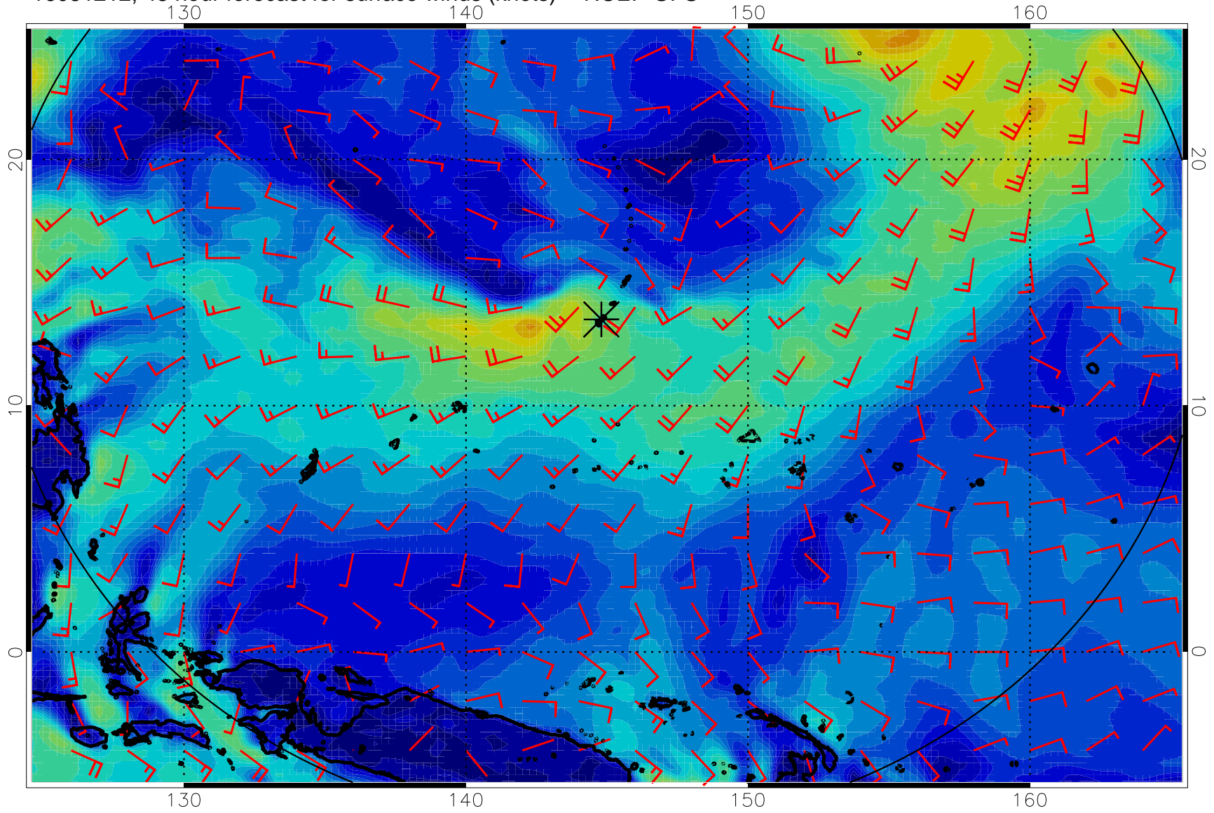
16081212, 48 hour forecast for surface winds (knots) -- NCEP GFS
