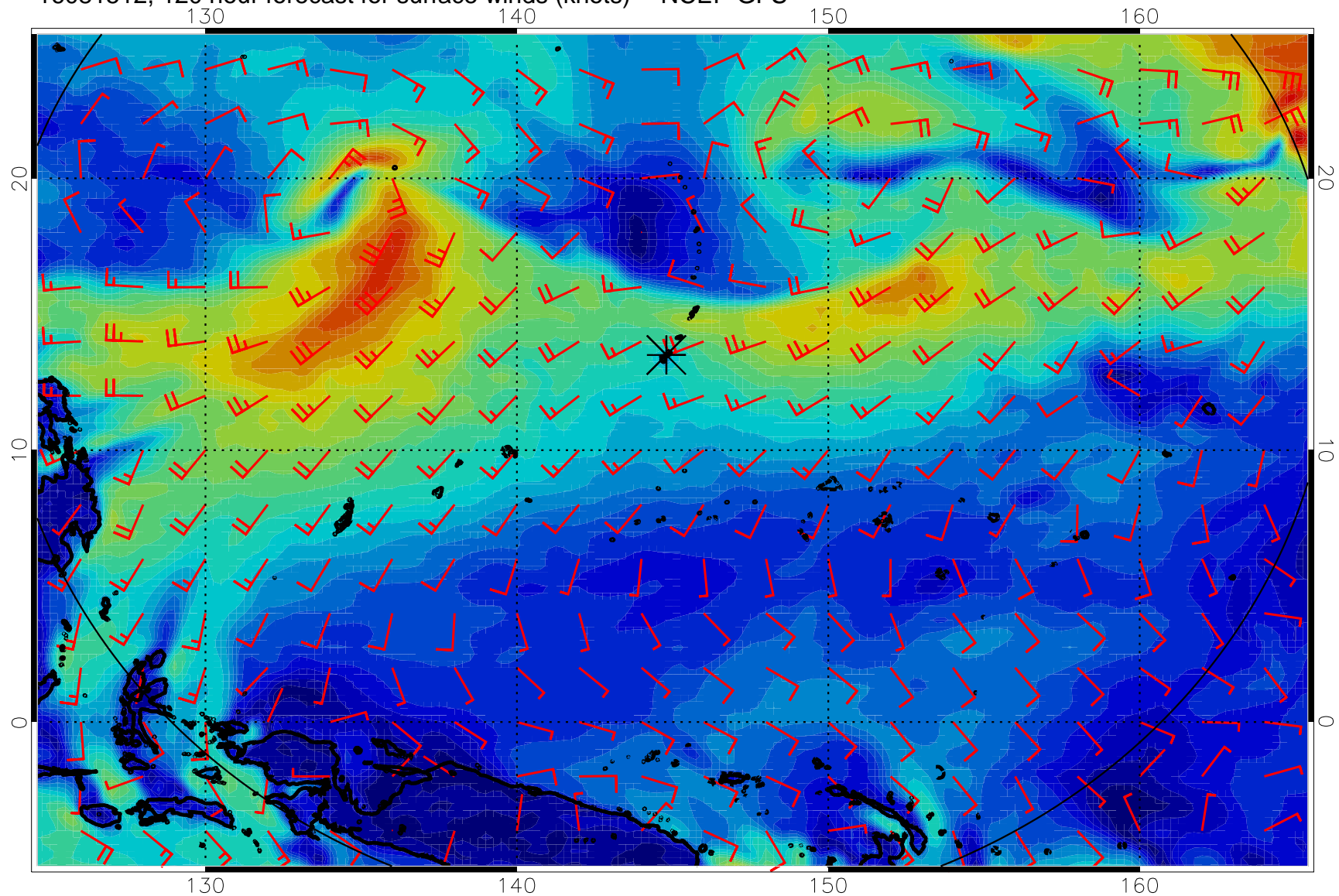
16081512, 120 hour forecast for surface winds (knots) -- NCEP GFS
