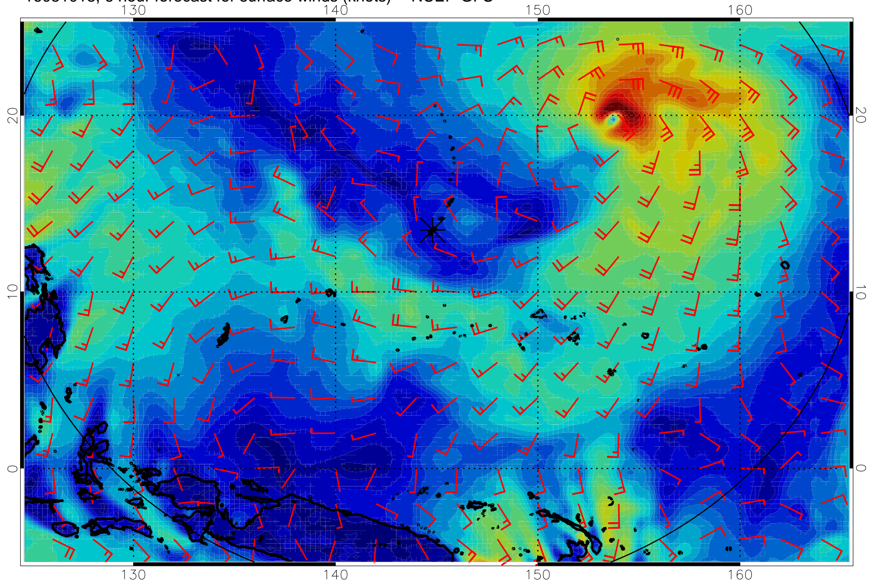
16081018, 6 hour forecast for surface winds (knots) -- NCEP GFS
