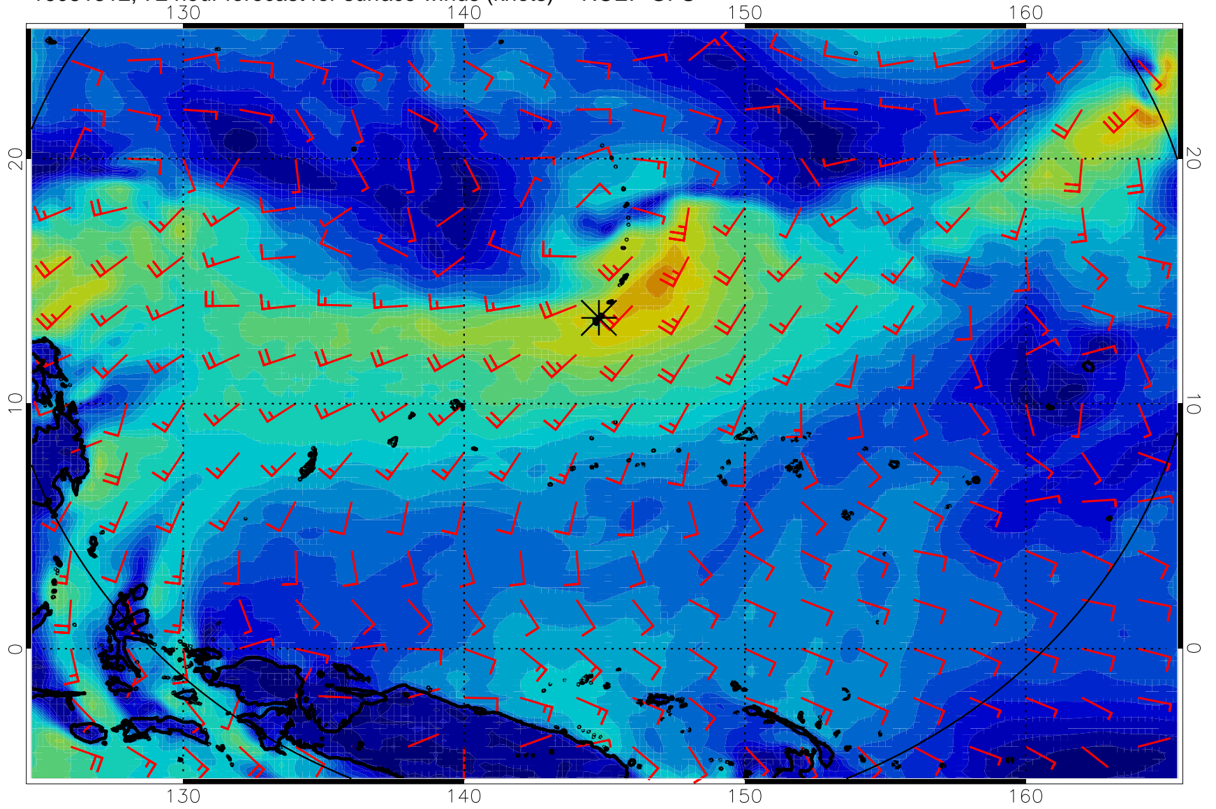
16081312, 72 hour forecast for surface winds (knots) -- NCEP GFS
