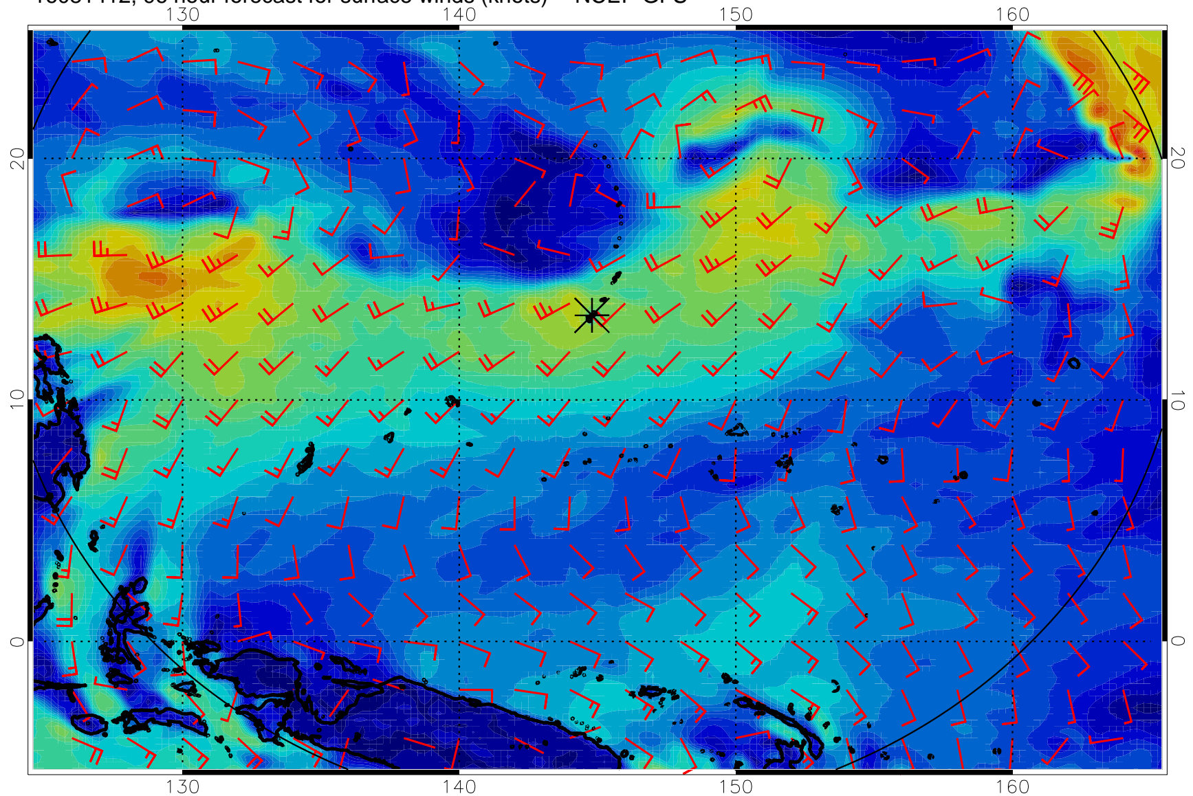
16081412, 96 hour forecast for surface winds (knots) -- NCEP GFS
