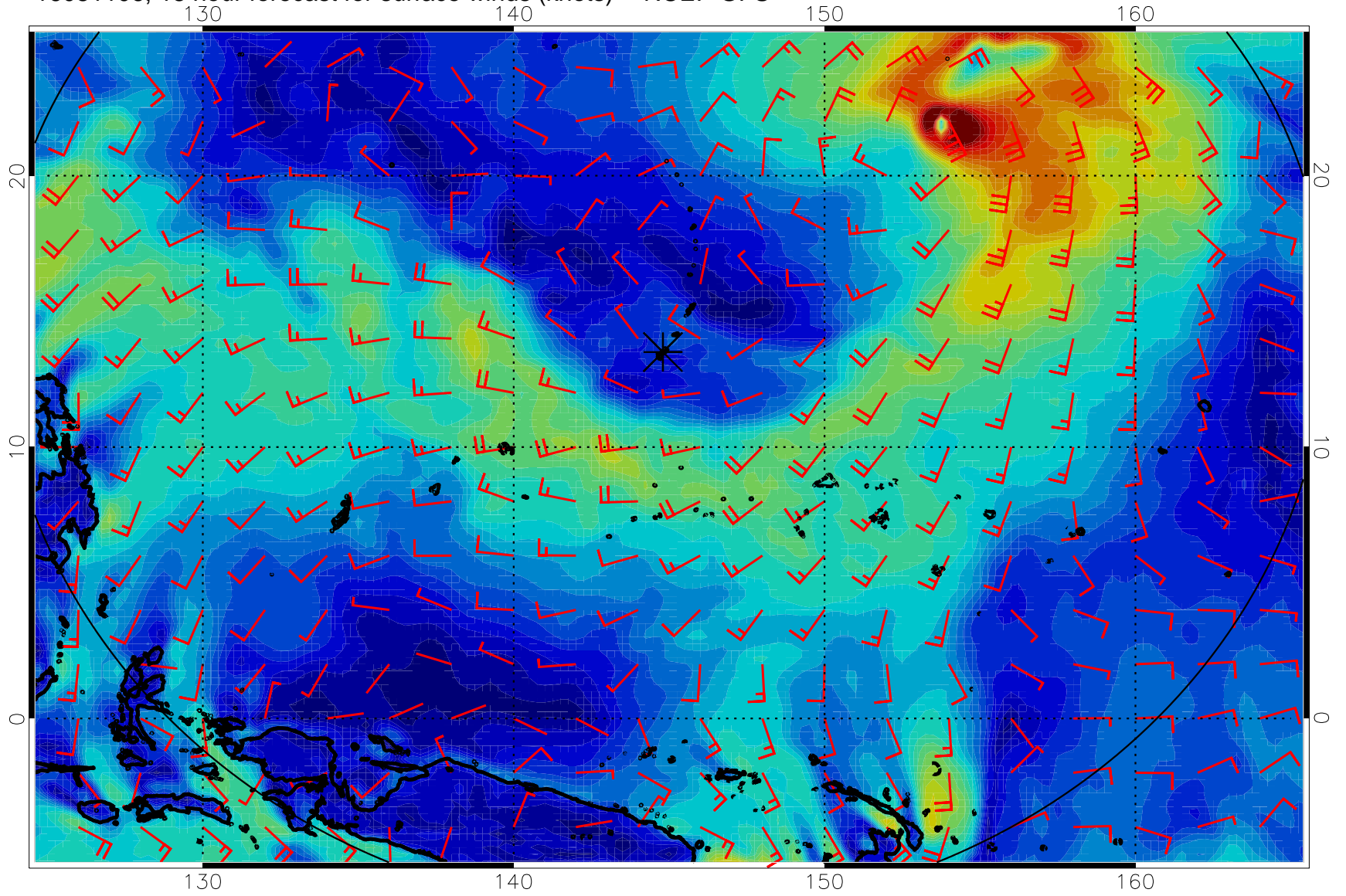
16081106, 18 hour forecast for surface winds (knots) -- NCEP GFS
