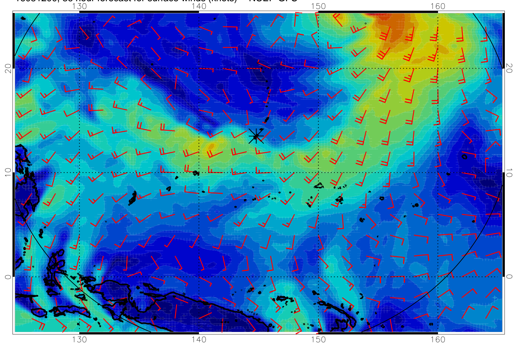
16081200, 36 hour forecast for surface winds (knots) -- NCEP GFS
