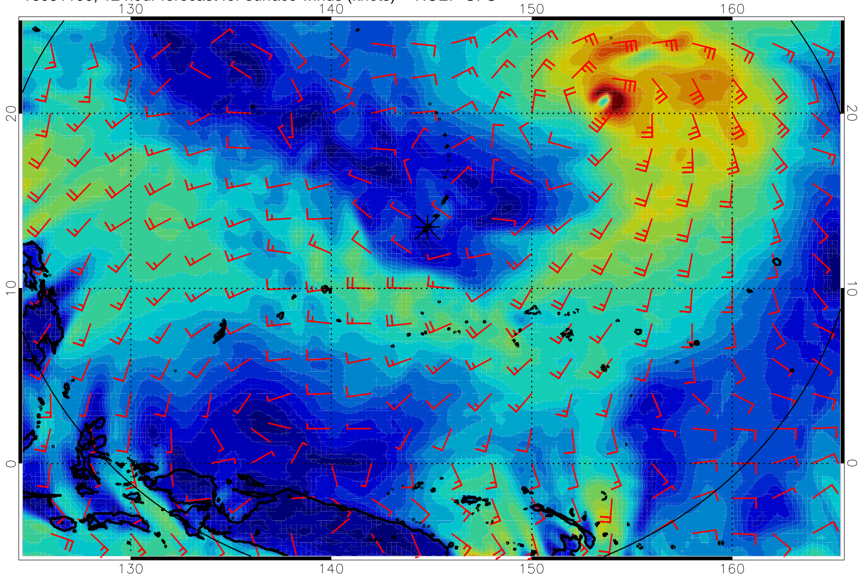
16081100, 12 hour forecast for surface winds (knots) -- NCEP GFS
