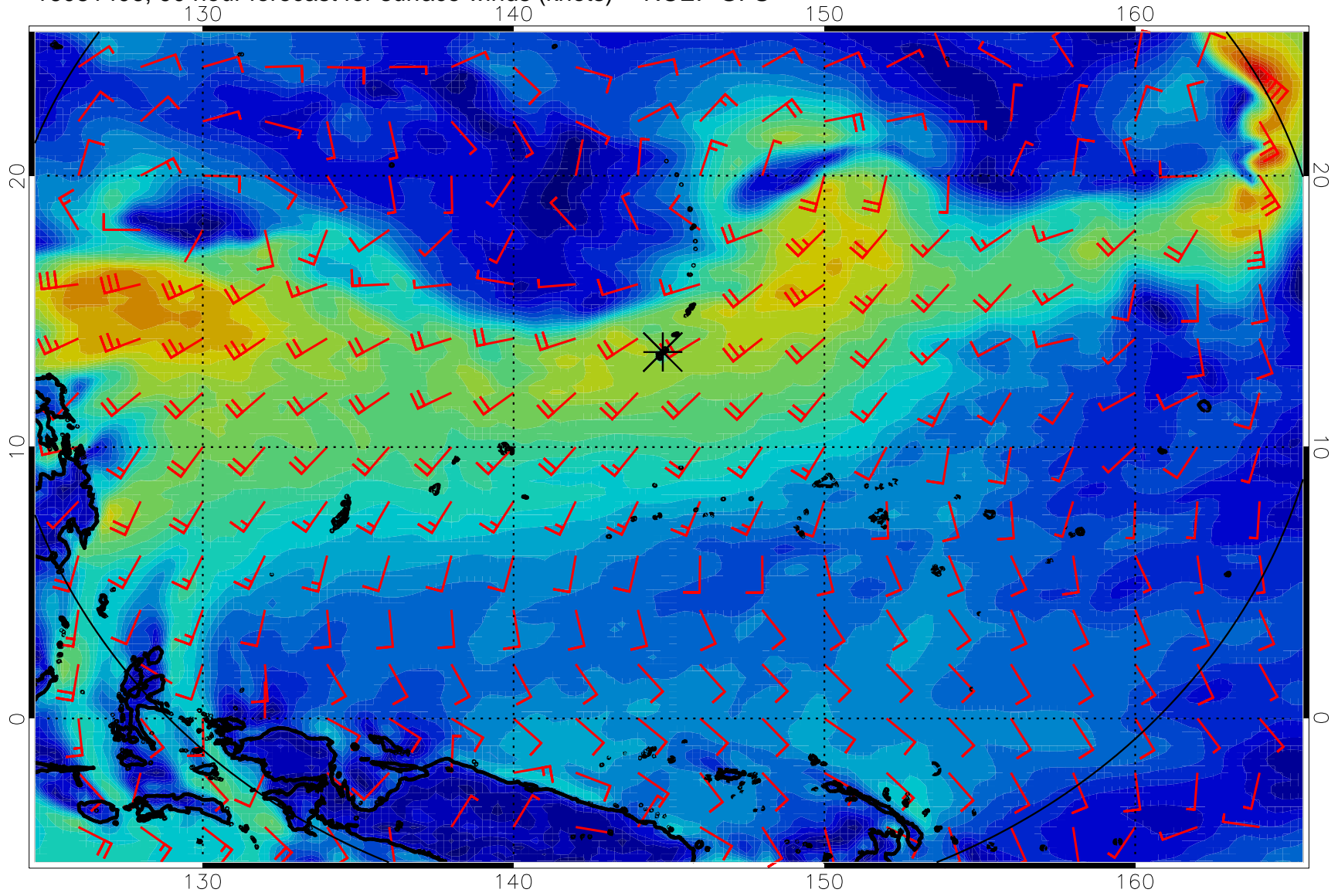
16081406, 90 hour forecast for surface winds (knots) -- NCEP GFS
