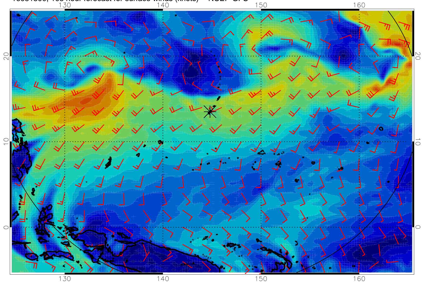
16081500, 108 hour forecast for surface winds (knots) -- NCEP GFS
