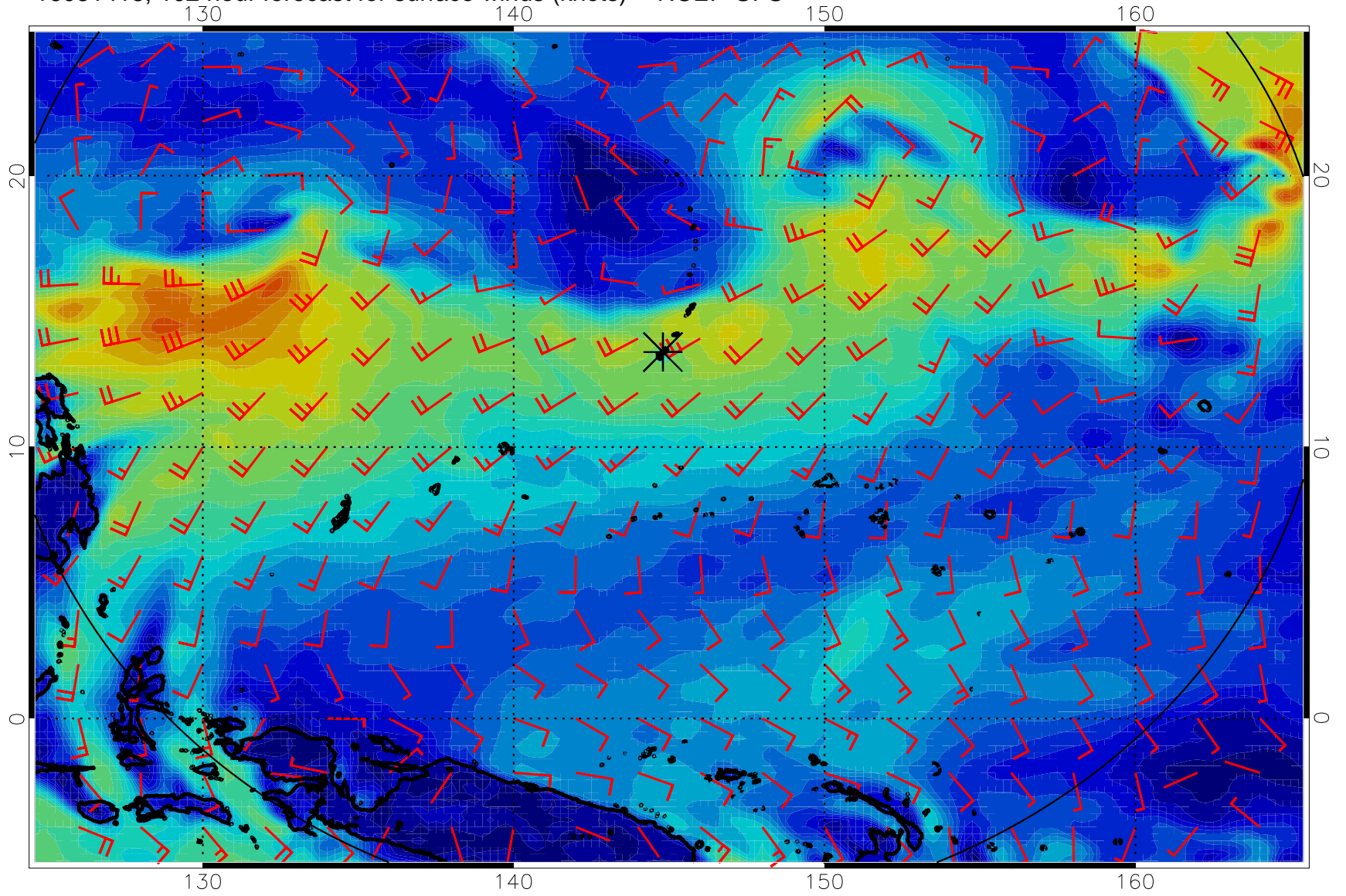
16081418, 102 hour forecast for surface winds (knots) -- NCEP GFS
