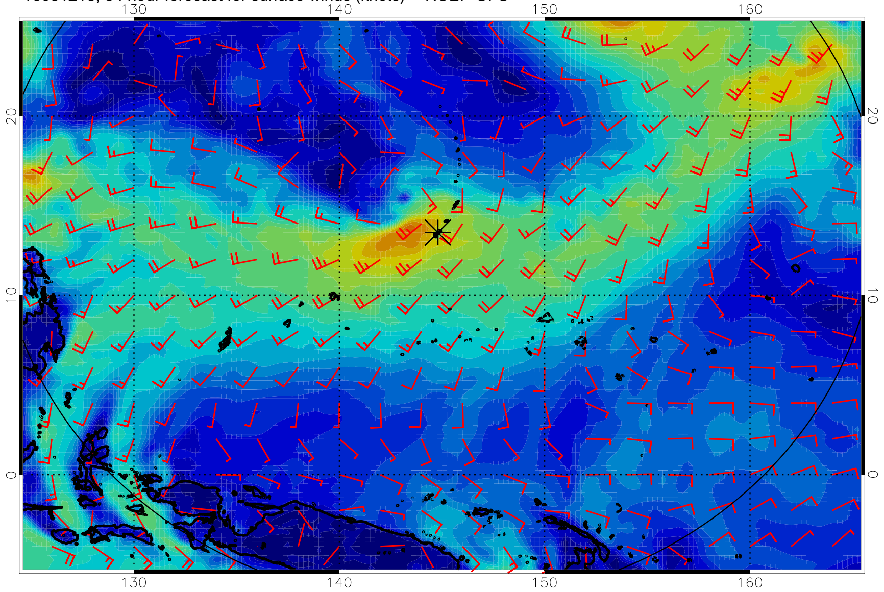
16081218, 54 hour forecast for surface winds (knots) -- NCEP GFS
