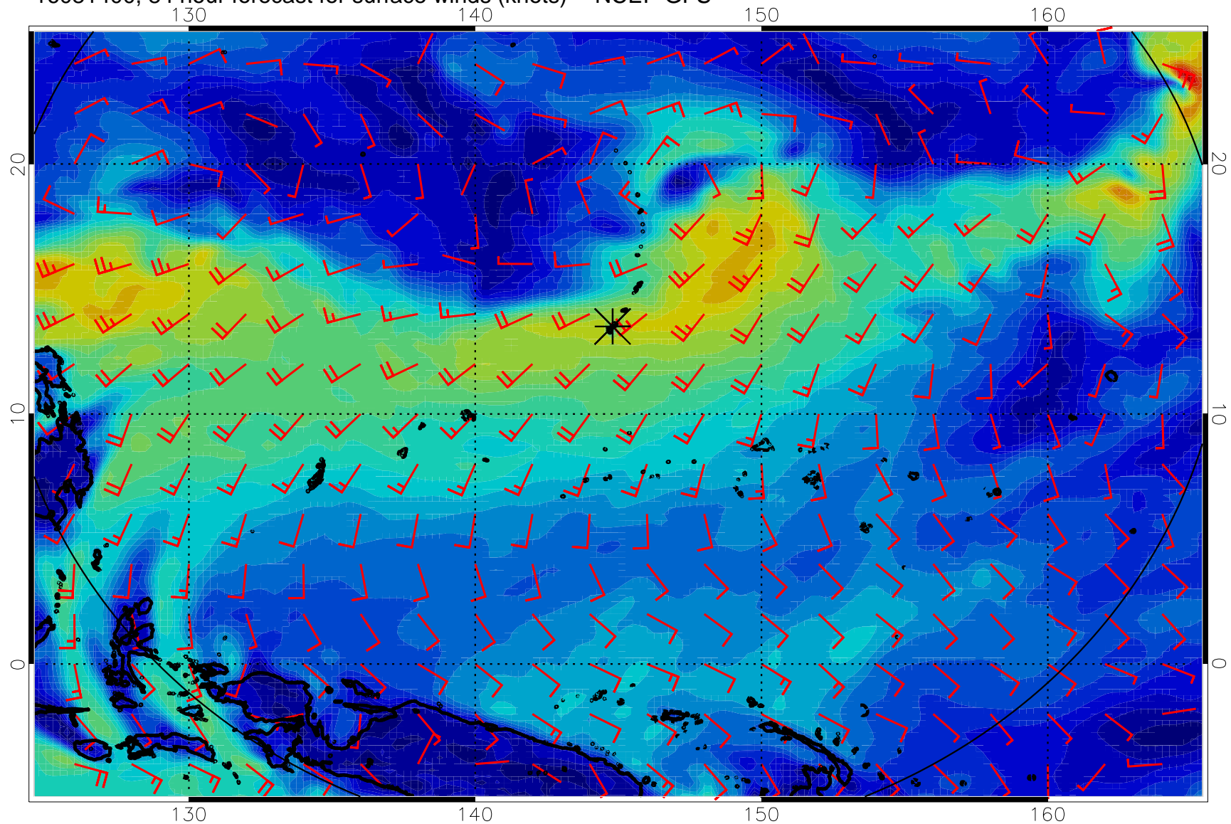
16081400, 84 hour forecast for surface winds (knots) -- NCEP GFS
