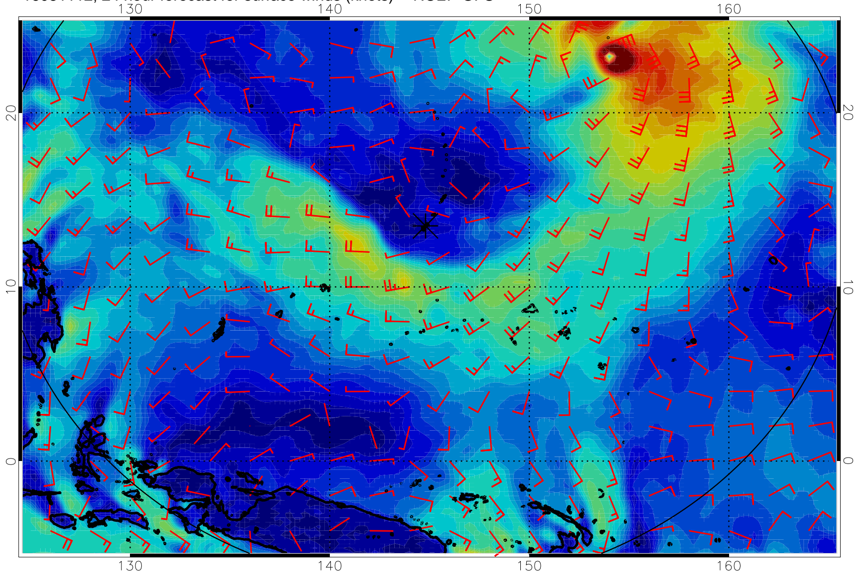
16081112, 24 hour forecast for surface winds (knots) -- NCEP GFS
