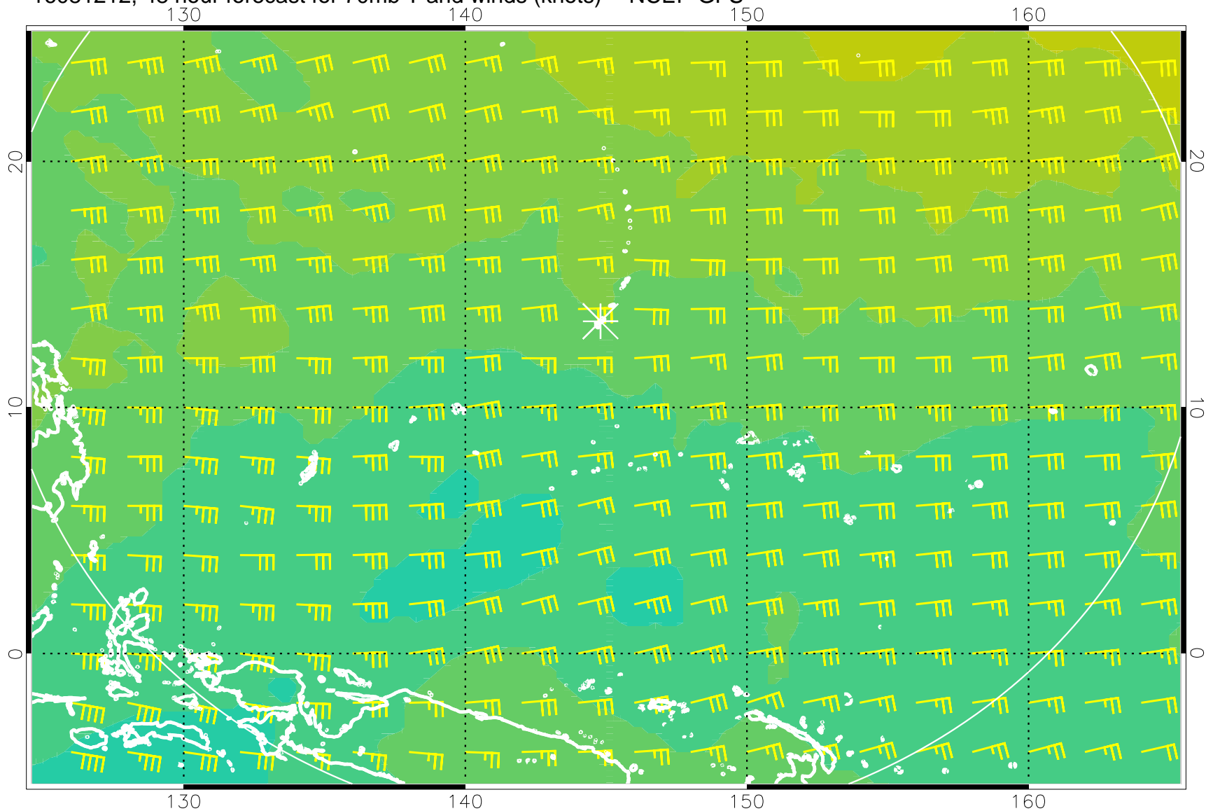
16081212, 48 hour forecast for 70mb T and winds (knots) -- NCEP GFS
