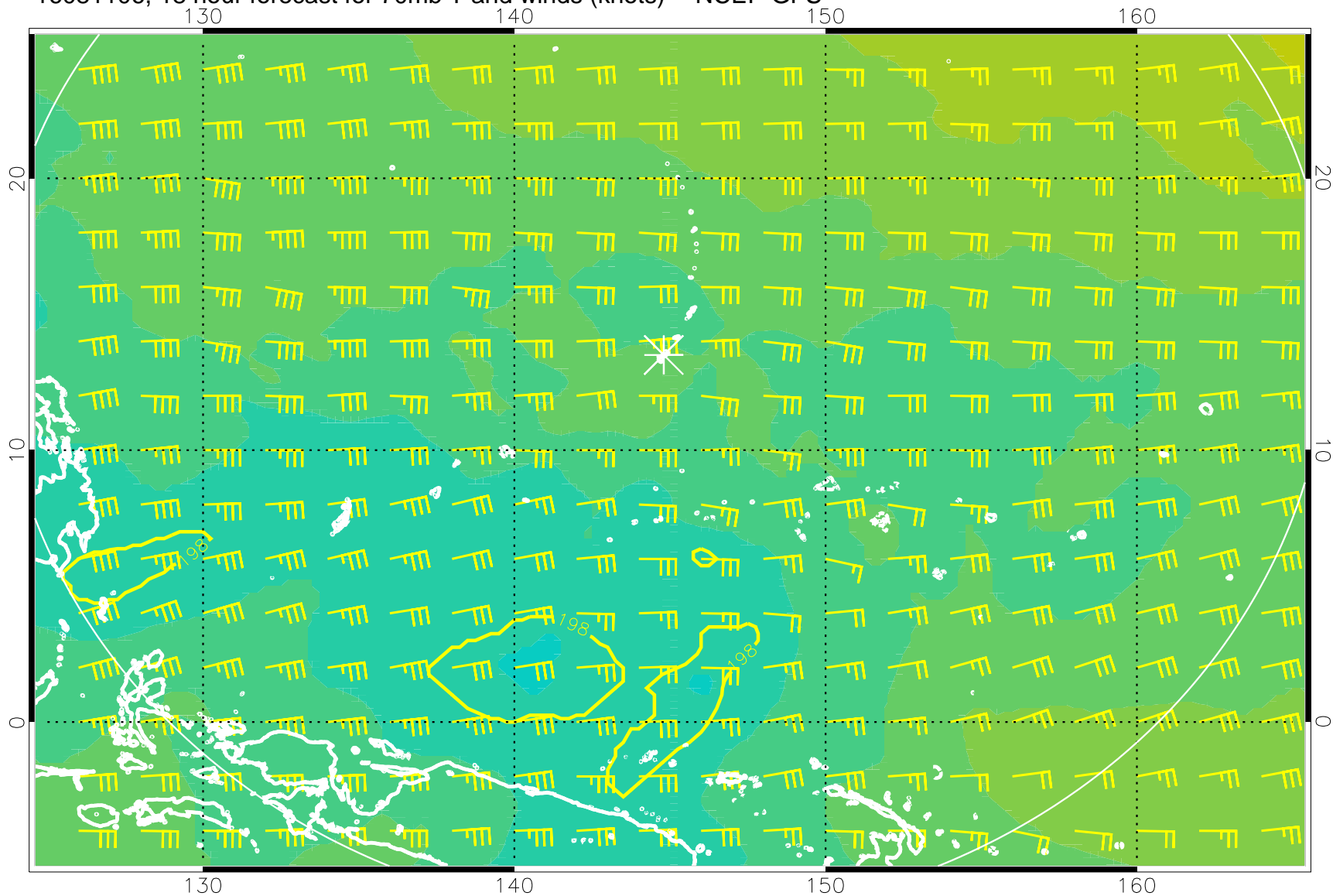
16081106, 18 hour forecast for 70mb T and winds (knots) -- NCEP GFS
