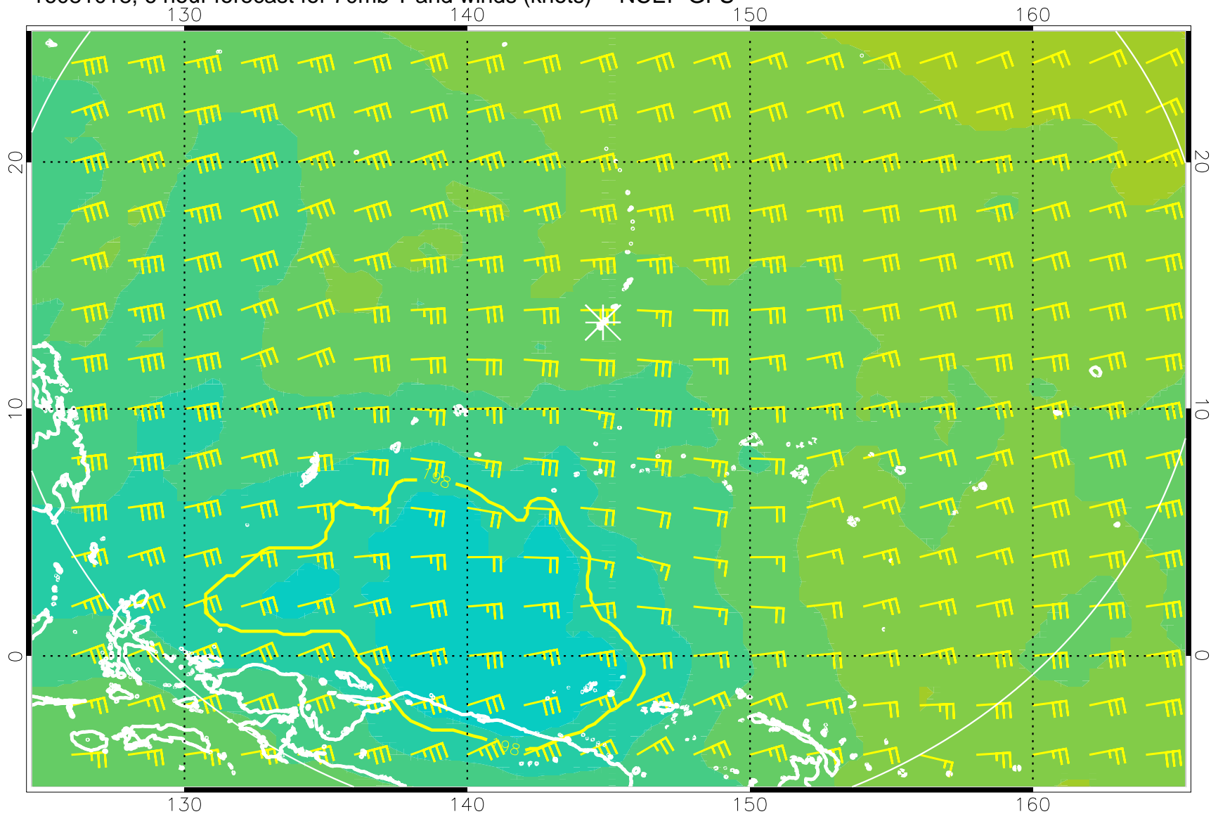
16081018, 6 hour forecast for 70mb T and winds (knots) -- NCEP GFS
