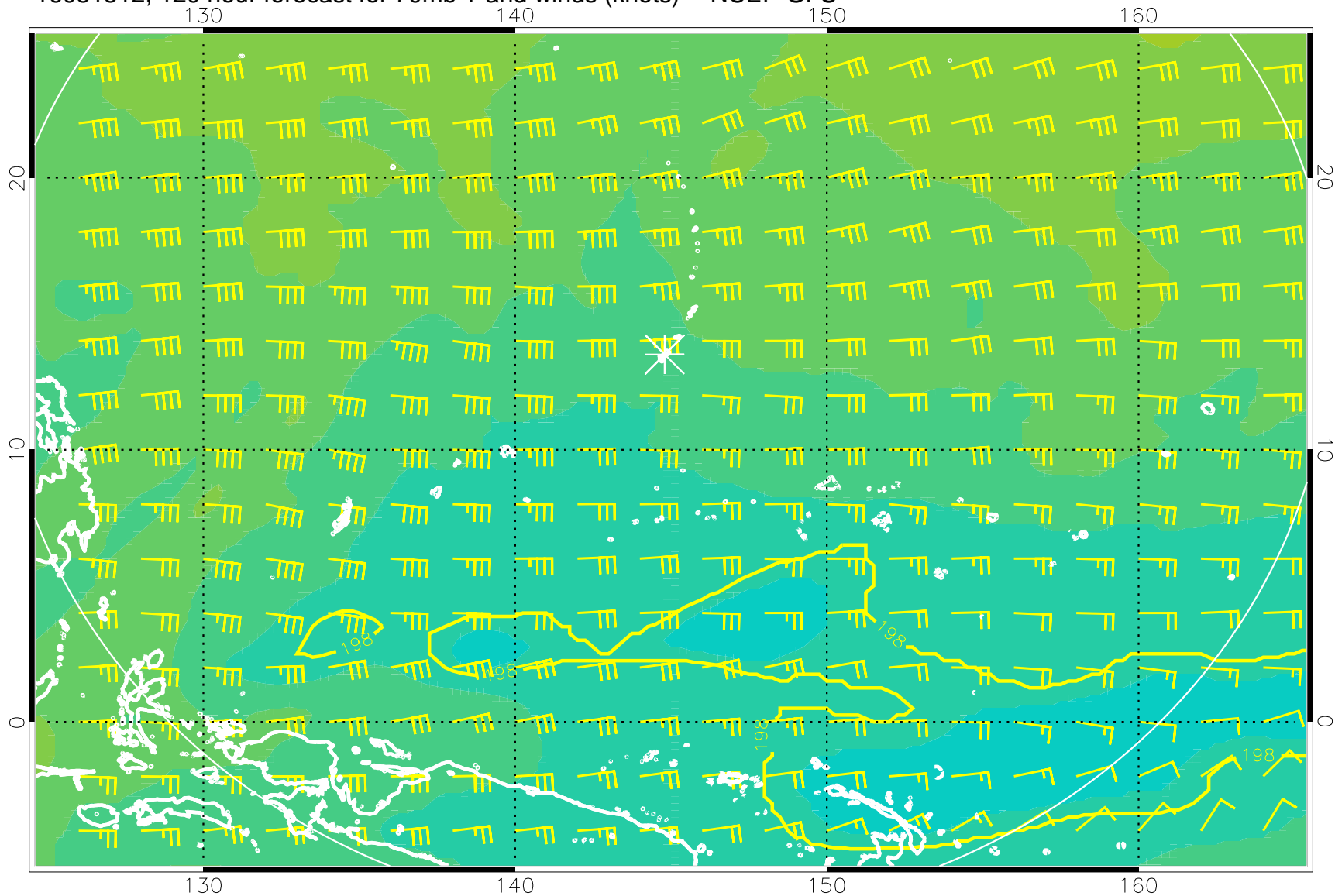
16081512, 120 hour forecast for 70mb T and winds (knots) -- NCEP GFS
