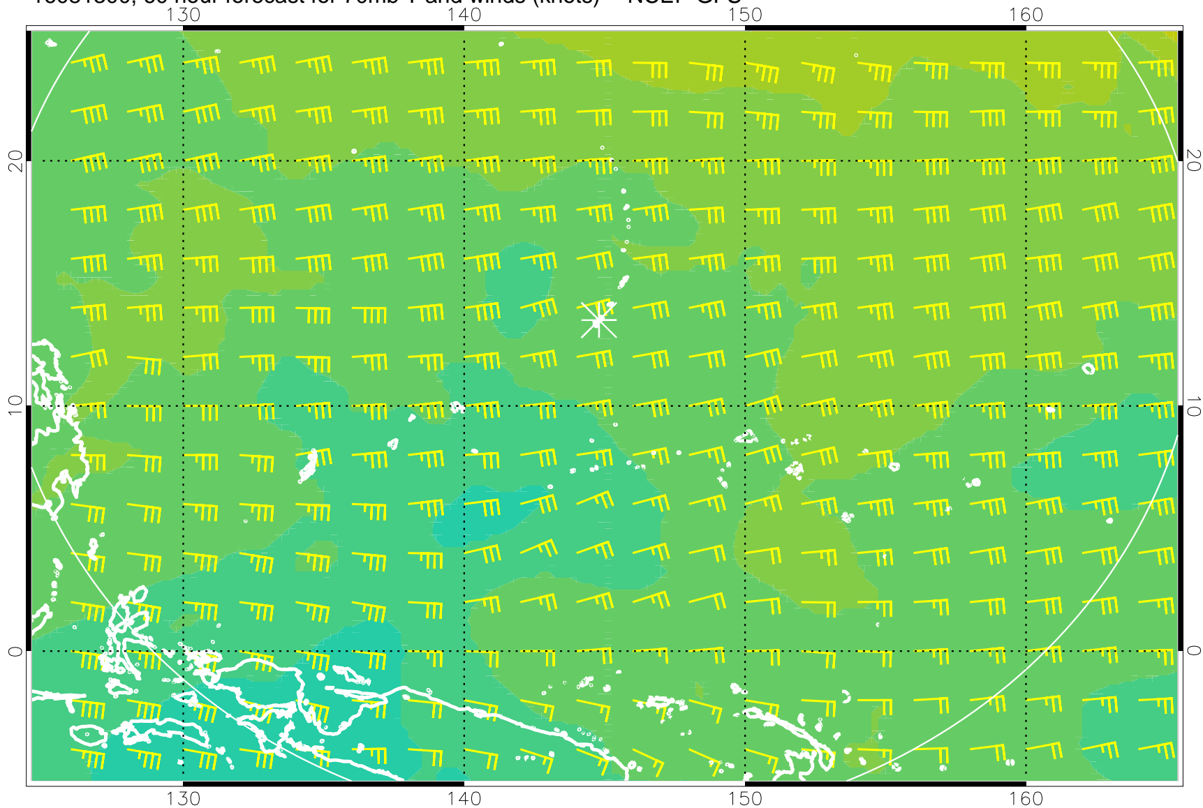
16081300, 60 hour forecast for 70mb T and winds (knots) -- NCEP GFS
