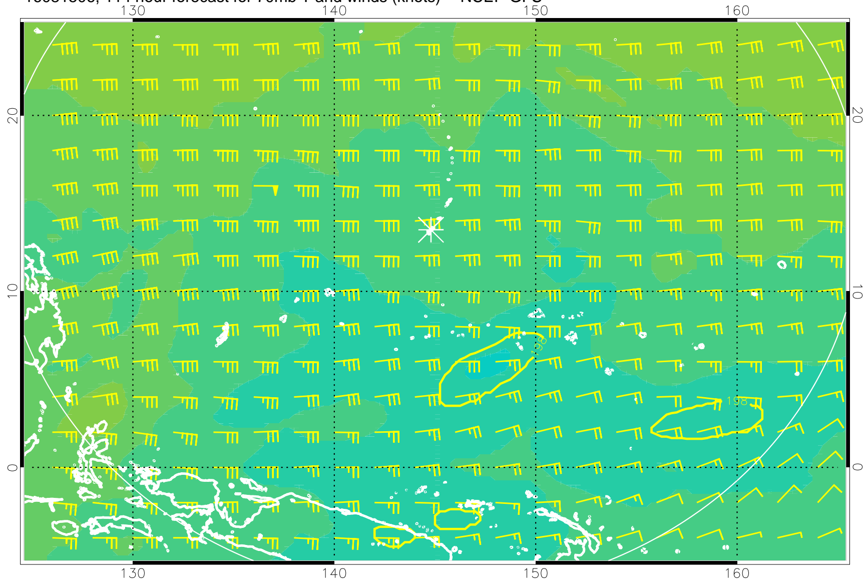
16081506, 114 hour forecast for 70mb T and winds (knots) -- NCEP GFS
