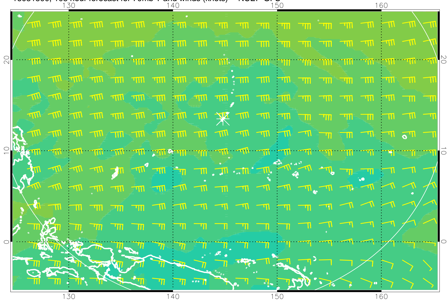
16081500, 108 hour forecast for 70mb T and winds (knots) -- NCEP GFS
