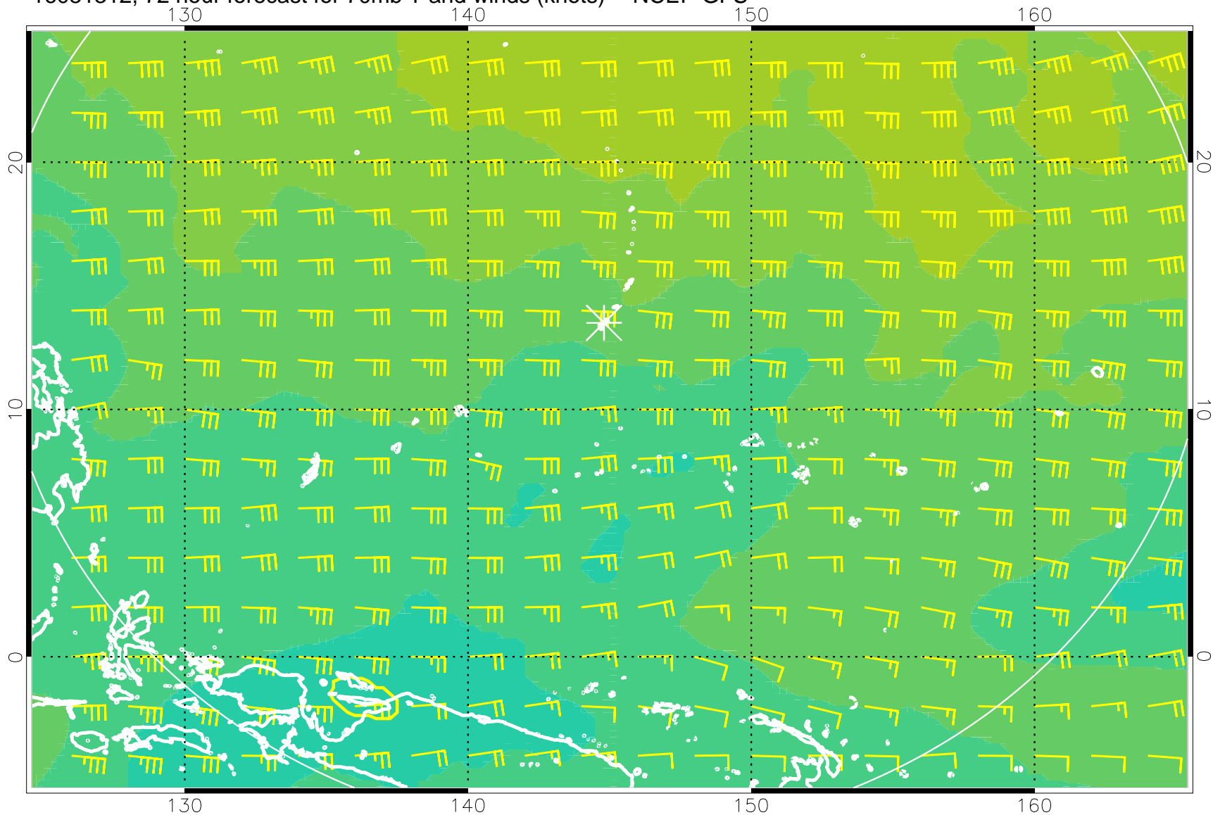
16081312, 72 hour forecast for 70mb T and winds (knots) -- NCEP GFS
