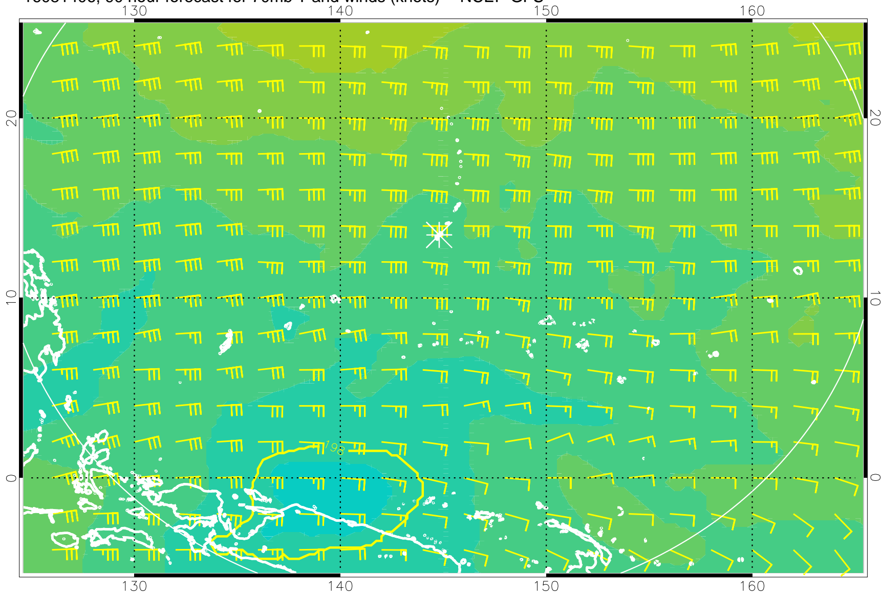
16081406, 90 hour forecast for 70mb T and winds (knots) -- NCEP GFS
