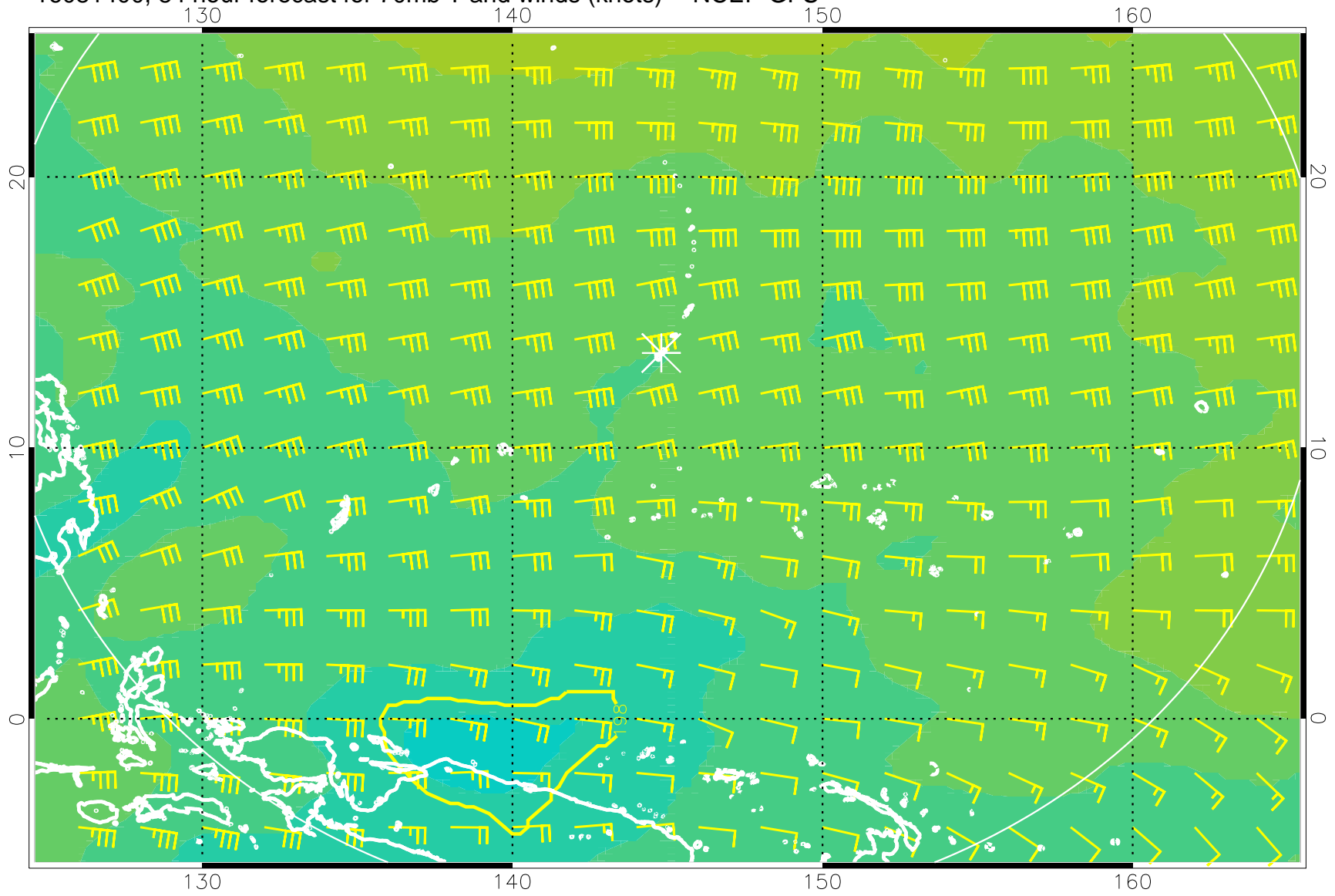
16081400, 84 hour forecast for 70mb T and winds (knots) -- NCEP GFS
