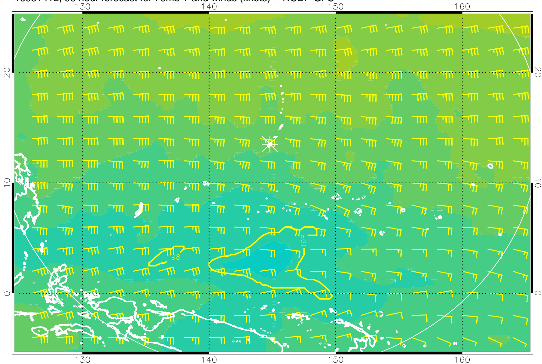
16081412, 96 hour forecast for 70mb T and winds (knots) -- NCEP GFS
