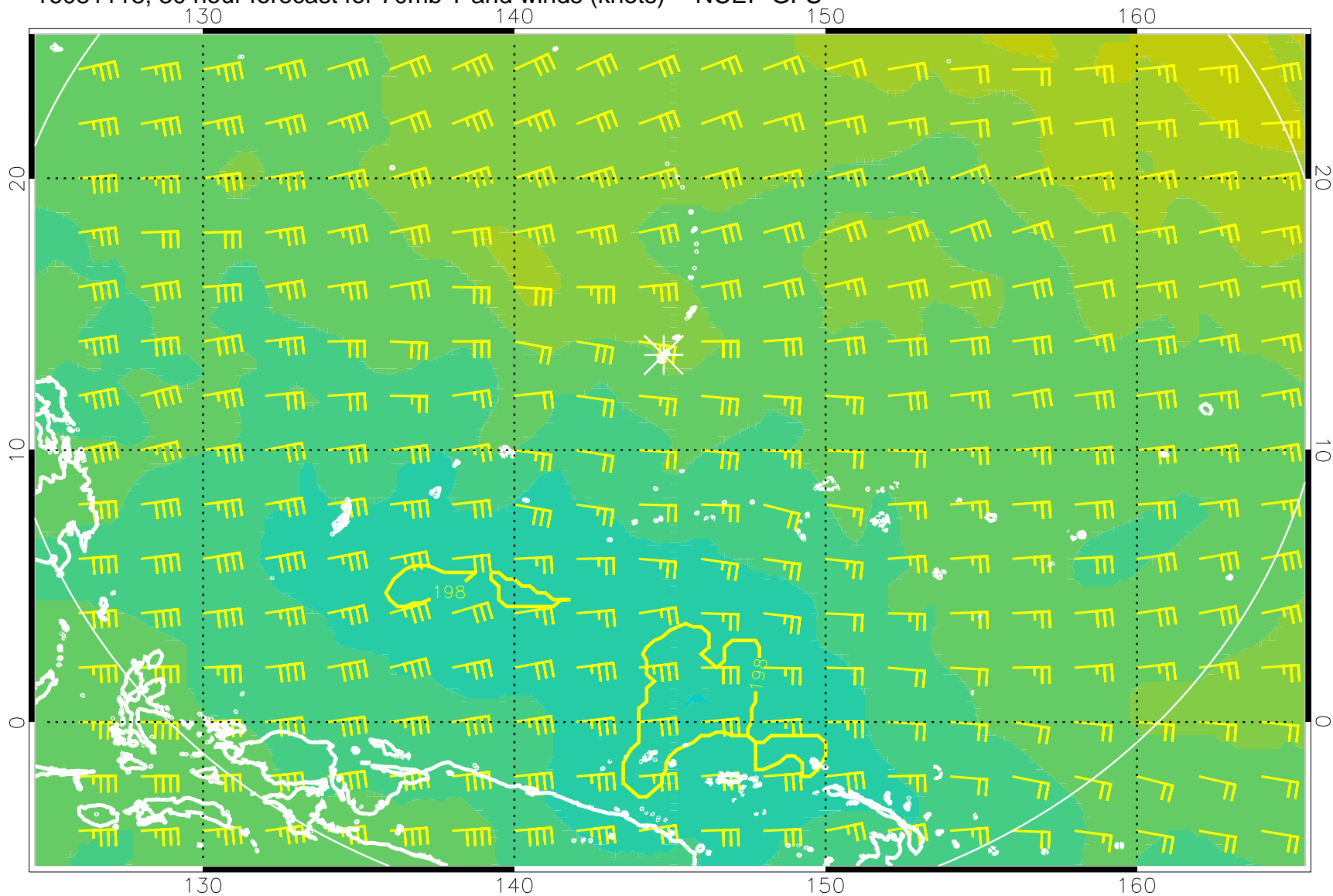
16081118, 30 hour forecast for 70mb T and winds (knots) -- NCEP GFS
