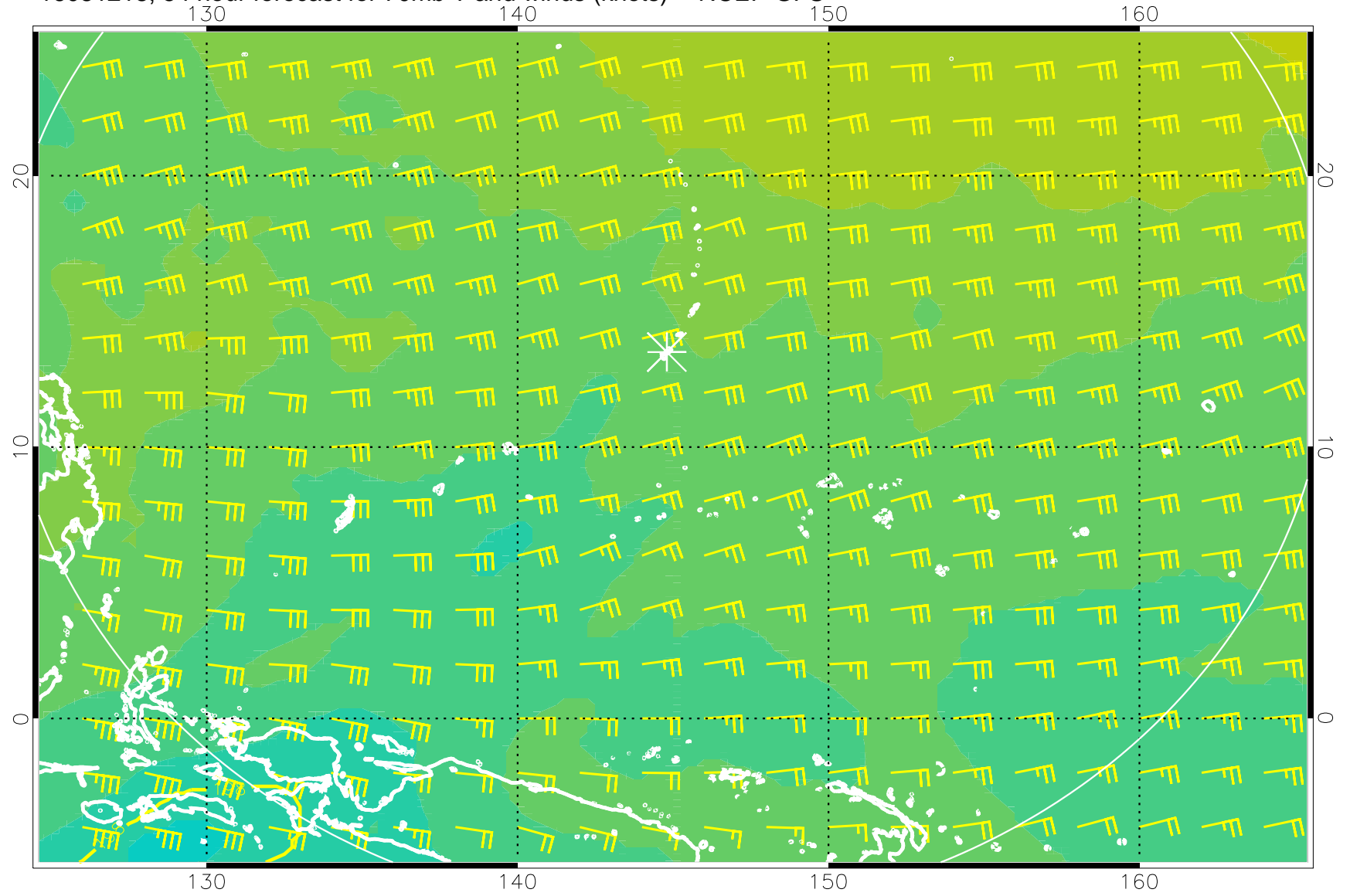
16081218, 54 hour forecast for 70mb T and winds (knots) -- NCEP GFS
