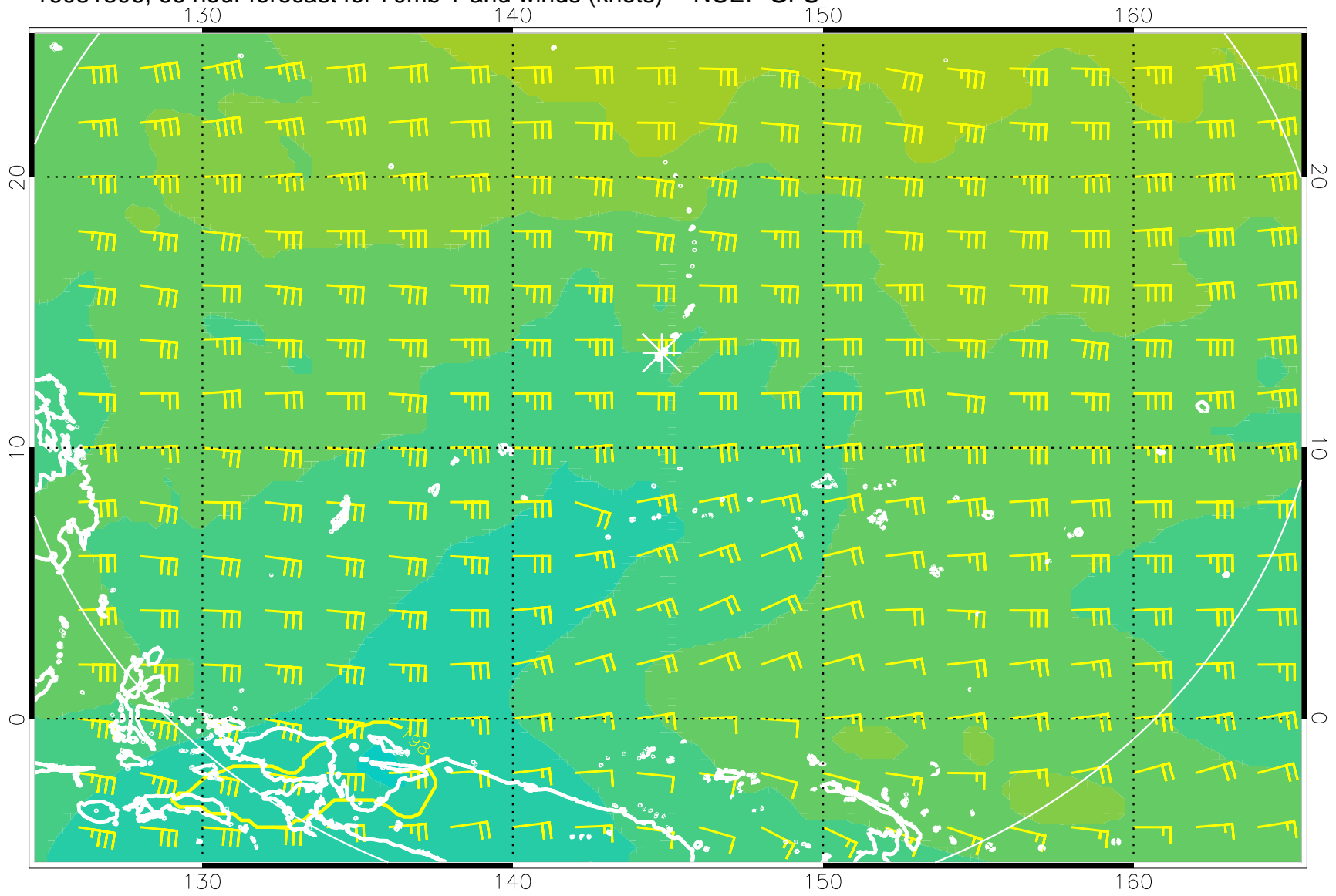
16081306, 66 hour forecast for 70mb T and winds (knots) -- NCEP GFS
