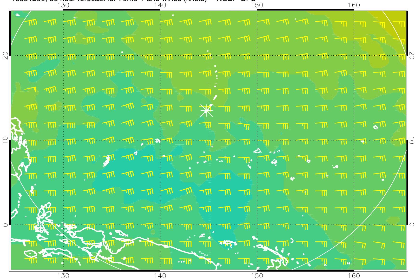
16081200, 36 hour forecast for 70mb T and winds (knots) -- NCEP GFS
