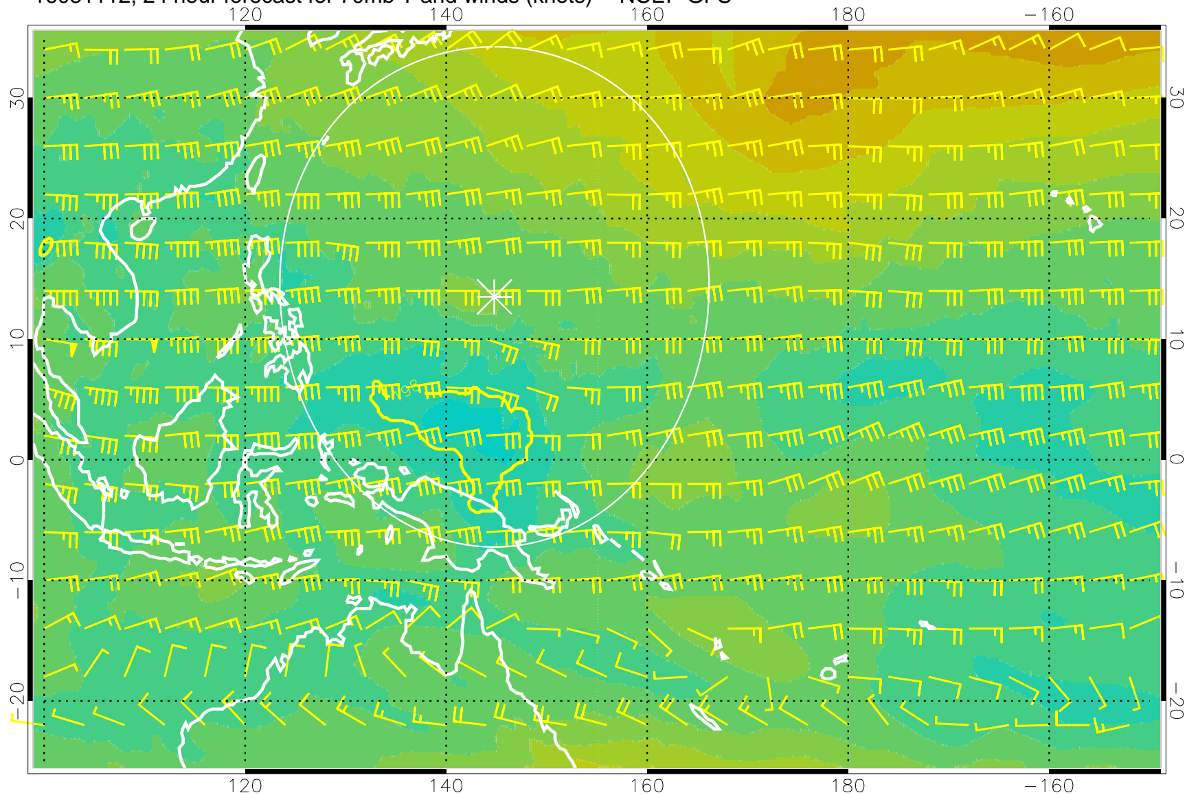
16081112, 24 hour forecast for 70mb T and winds (knots) -- NCEP GFS
