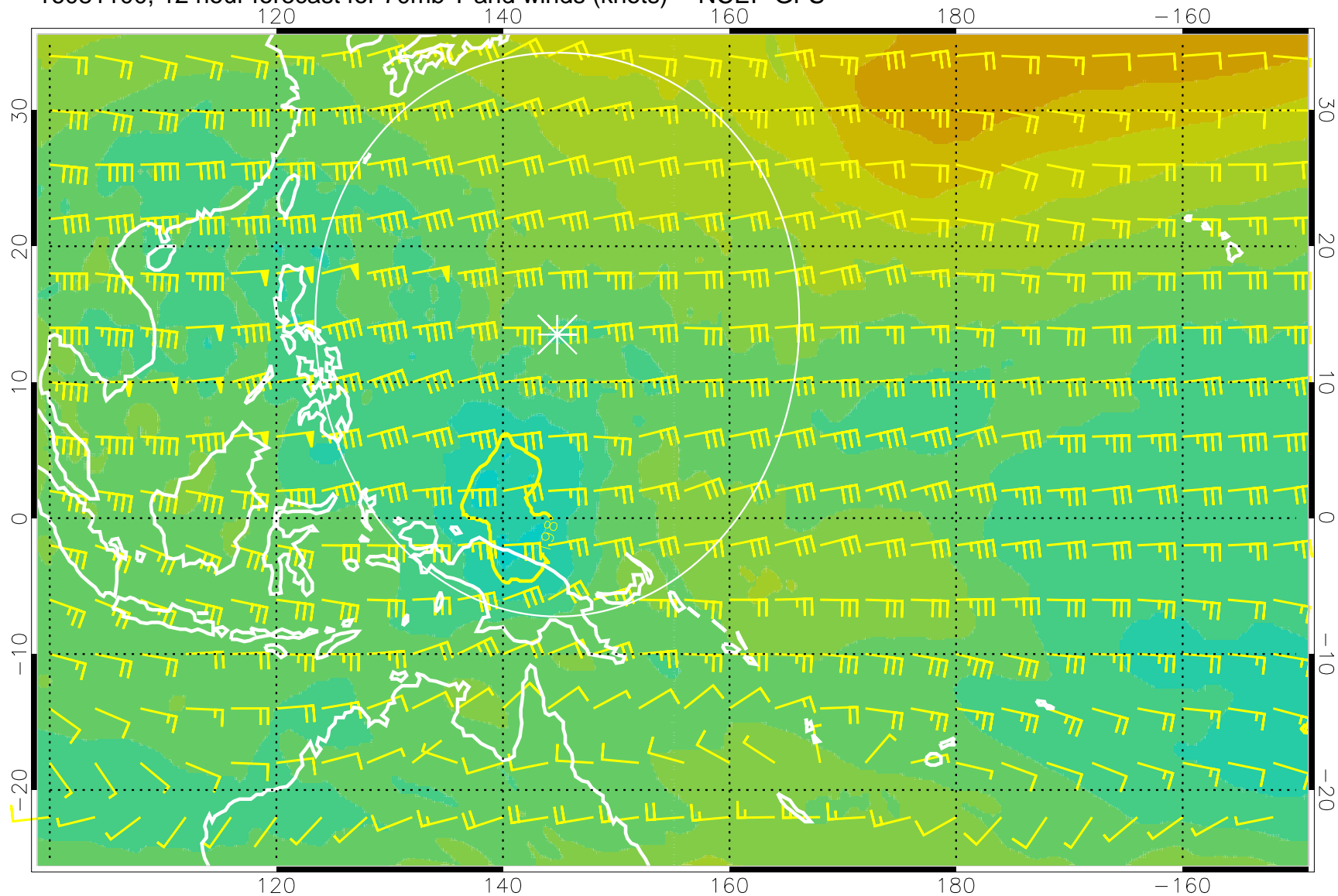
16081100, 12 hour forecast for 70mb T and winds (knots) -- NCEP GFS
