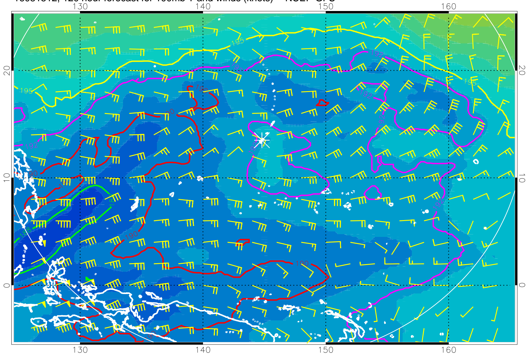
16081512, 120 hour forecast for 100mb T and winds (knots) -- NCEP GFS
