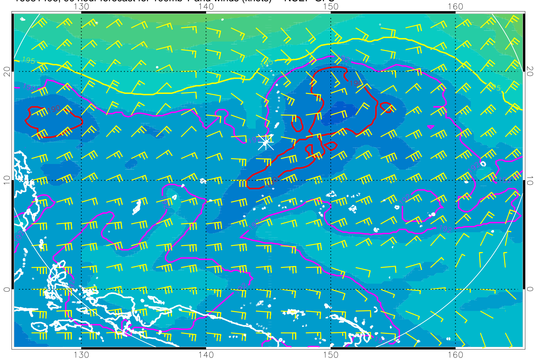
16081406, 90 hour forecast for 100mb T and winds (knots) -- NCEP GFS
