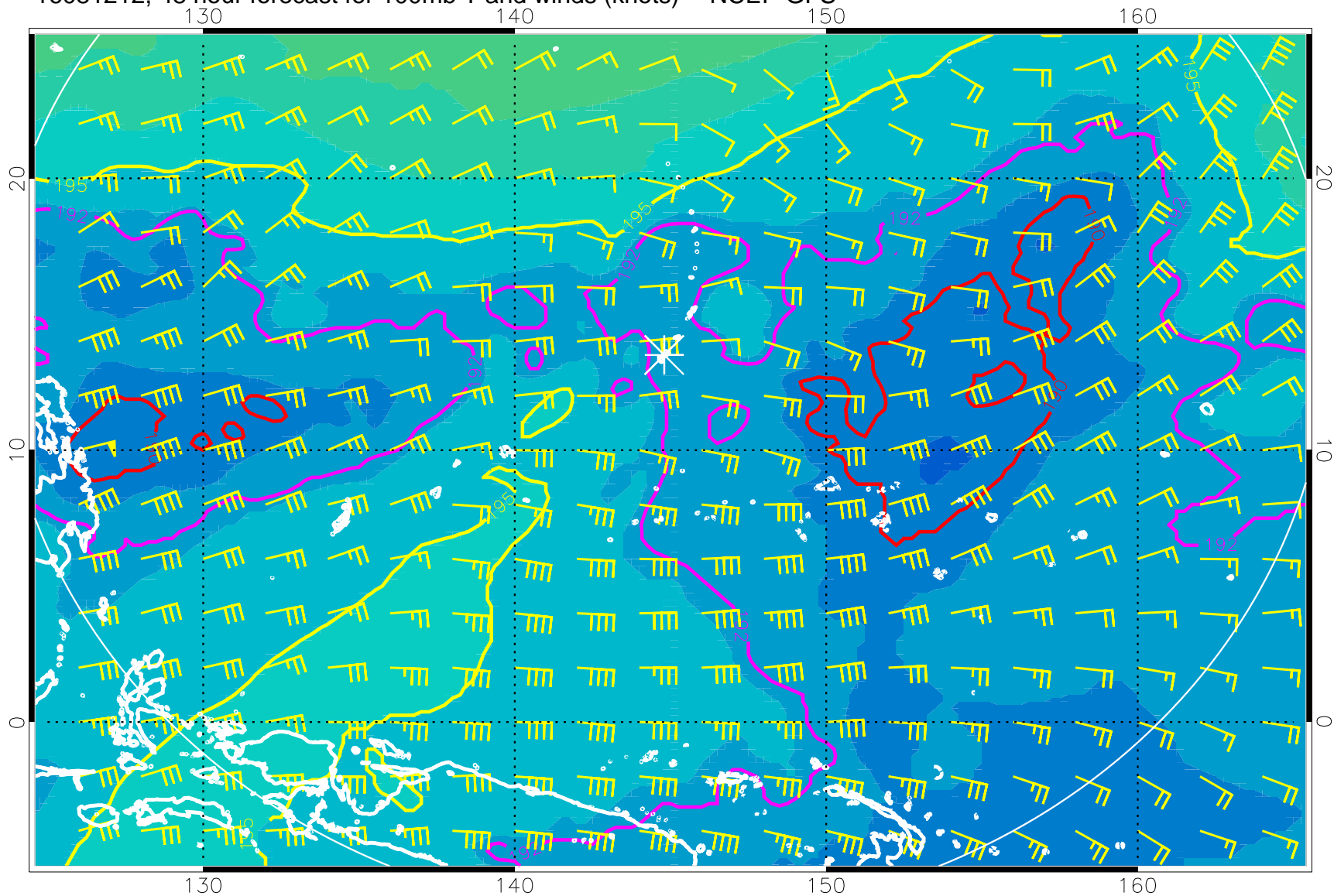
16081212, 48 hour forecast for 100mb T and winds (knots) -- NCEP GFS
