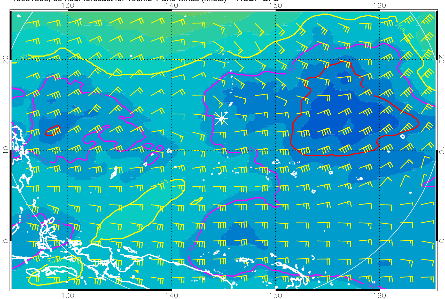
16081306, 66 hour forecast for 100mb T and winds (knots) -- NCEP GFS
