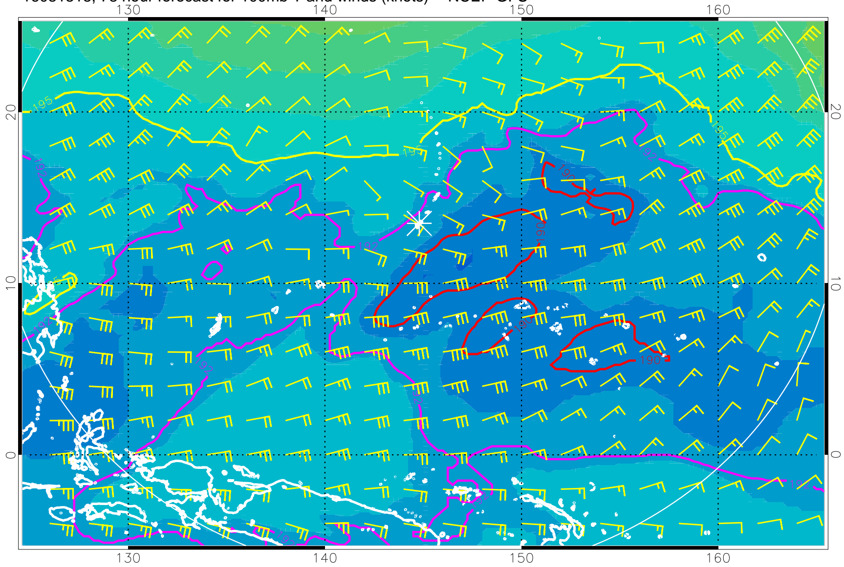
16081318, 78 hour forecast for 100mb T and winds (knots) -- NCEP GFS
