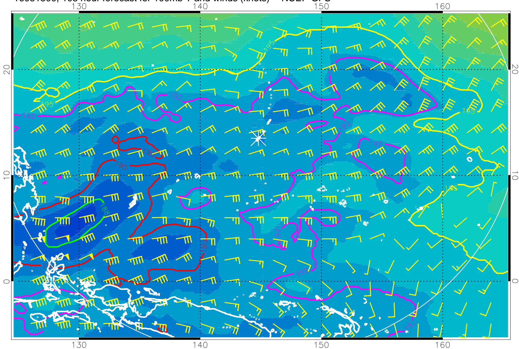
16081500, 108 hour forecast for 100mb T and winds (knots) -- NCEP GFS
