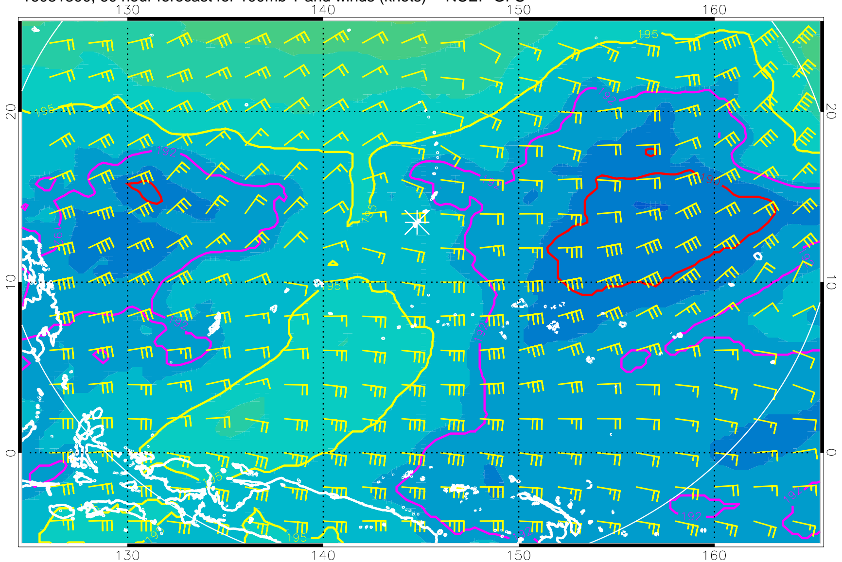
16081300, 60 hour forecast for 100mb T and winds (knots) -- NCEP GFS
