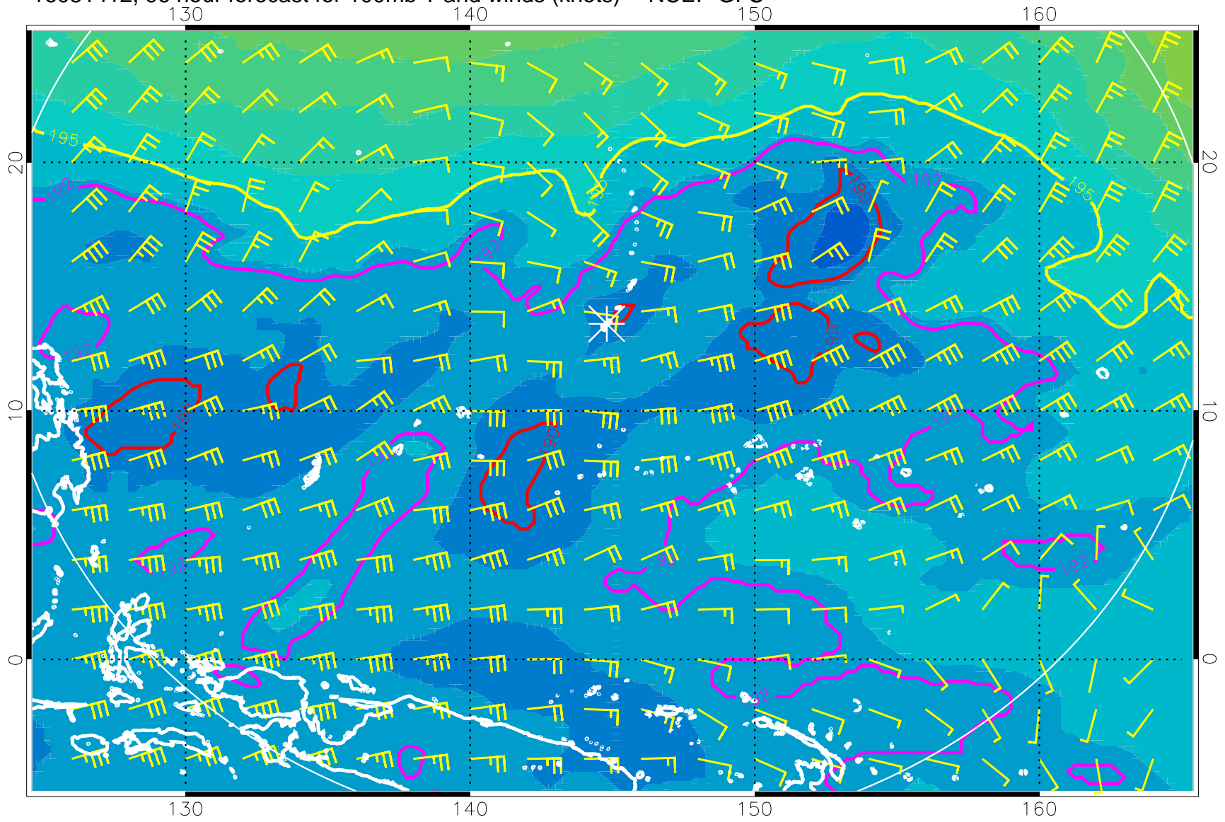
16081412, 96 hour forecast for 100mb T and winds (knots) -- NCEP GFS
