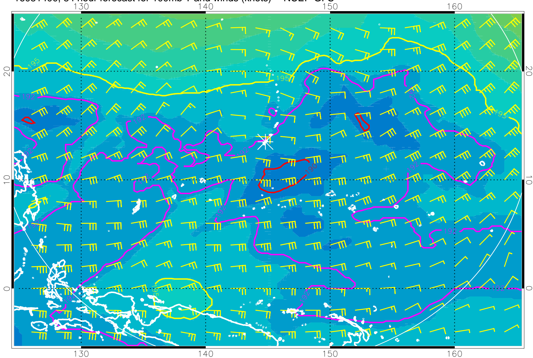
16081400, 84 hour forecast for 100mb T and winds (knots) -- NCEP GFS
