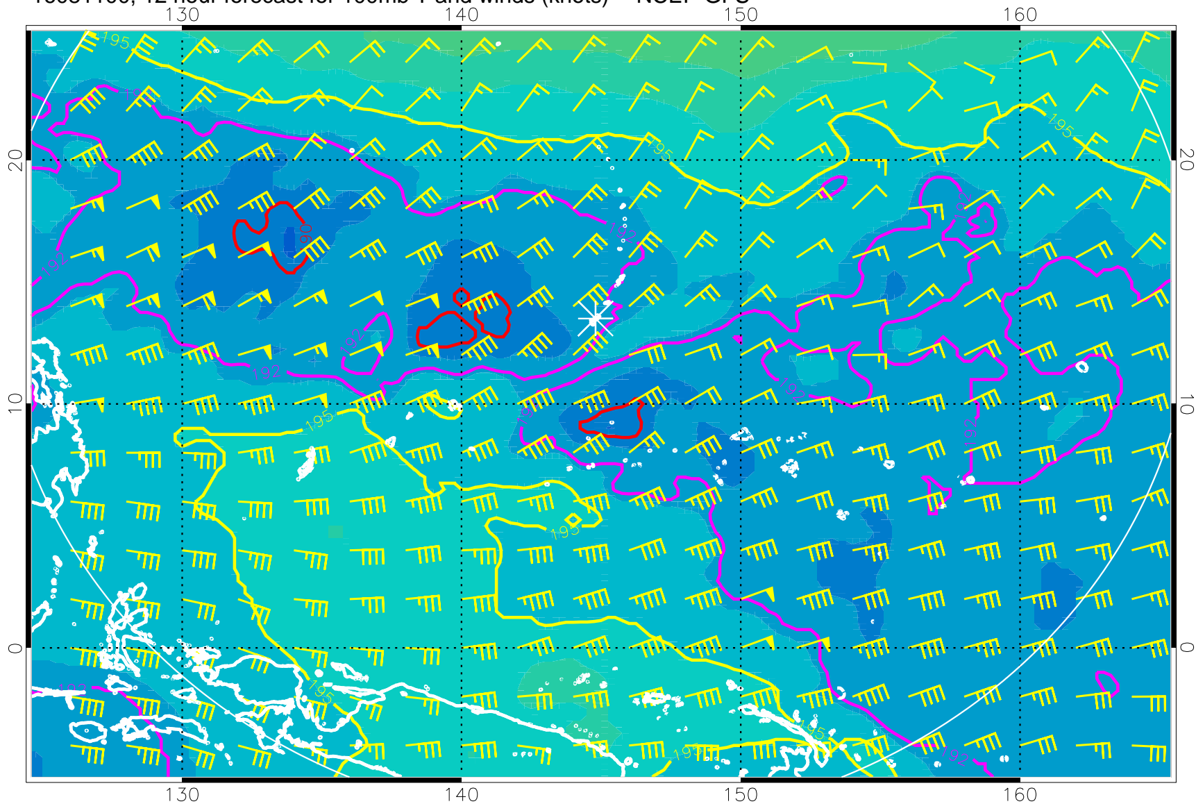
16081100, 12 hour forecast for 100mb T and winds (knots) -- NCEP GFS
