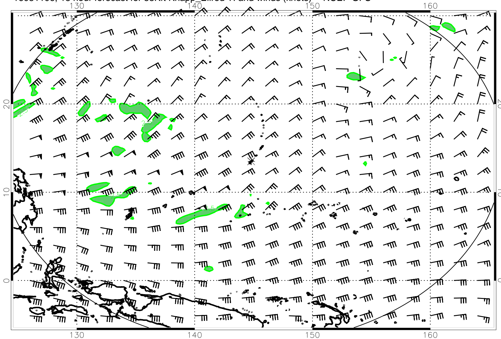
16081106, 18 hour forecast for 53Kft Knapp_Ellrod TI and winds (knots) -- NCEP GFS
