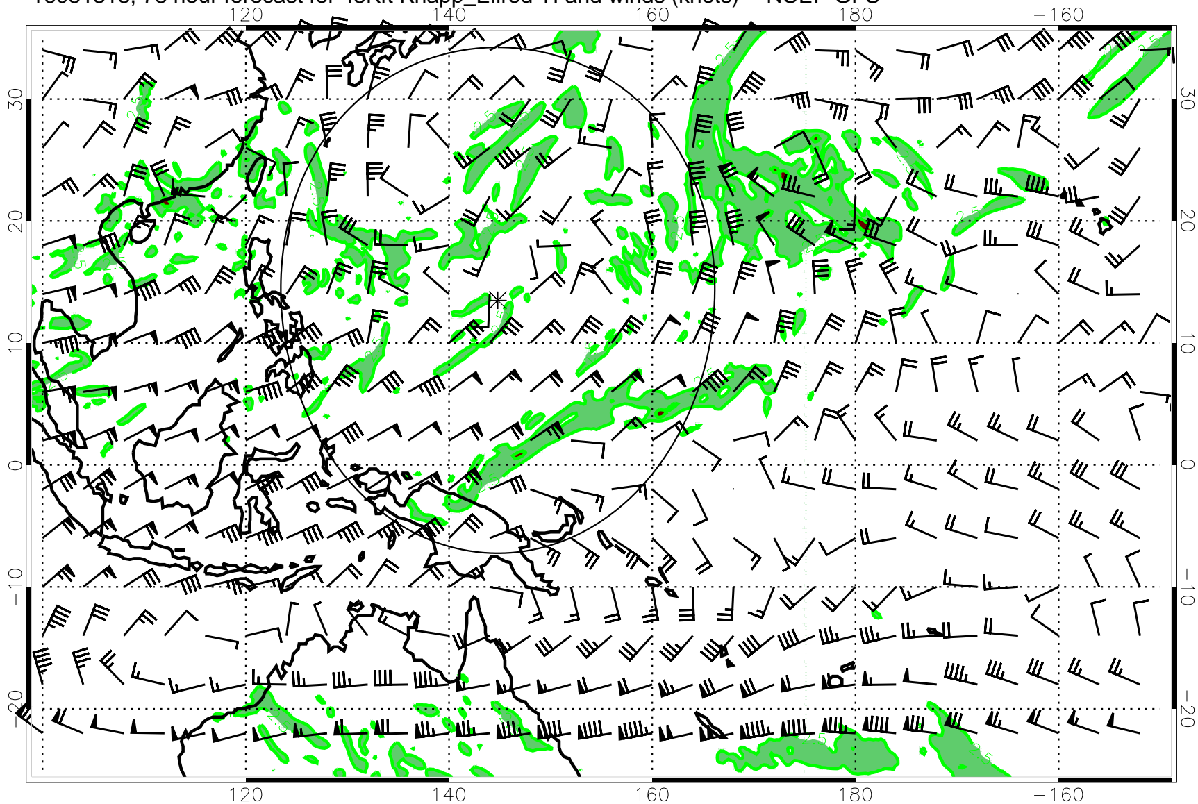
16081318, 78 hour forecast for 45Kft Knapp_Ellrod TI and winds (knots) -- NCEP GFS
