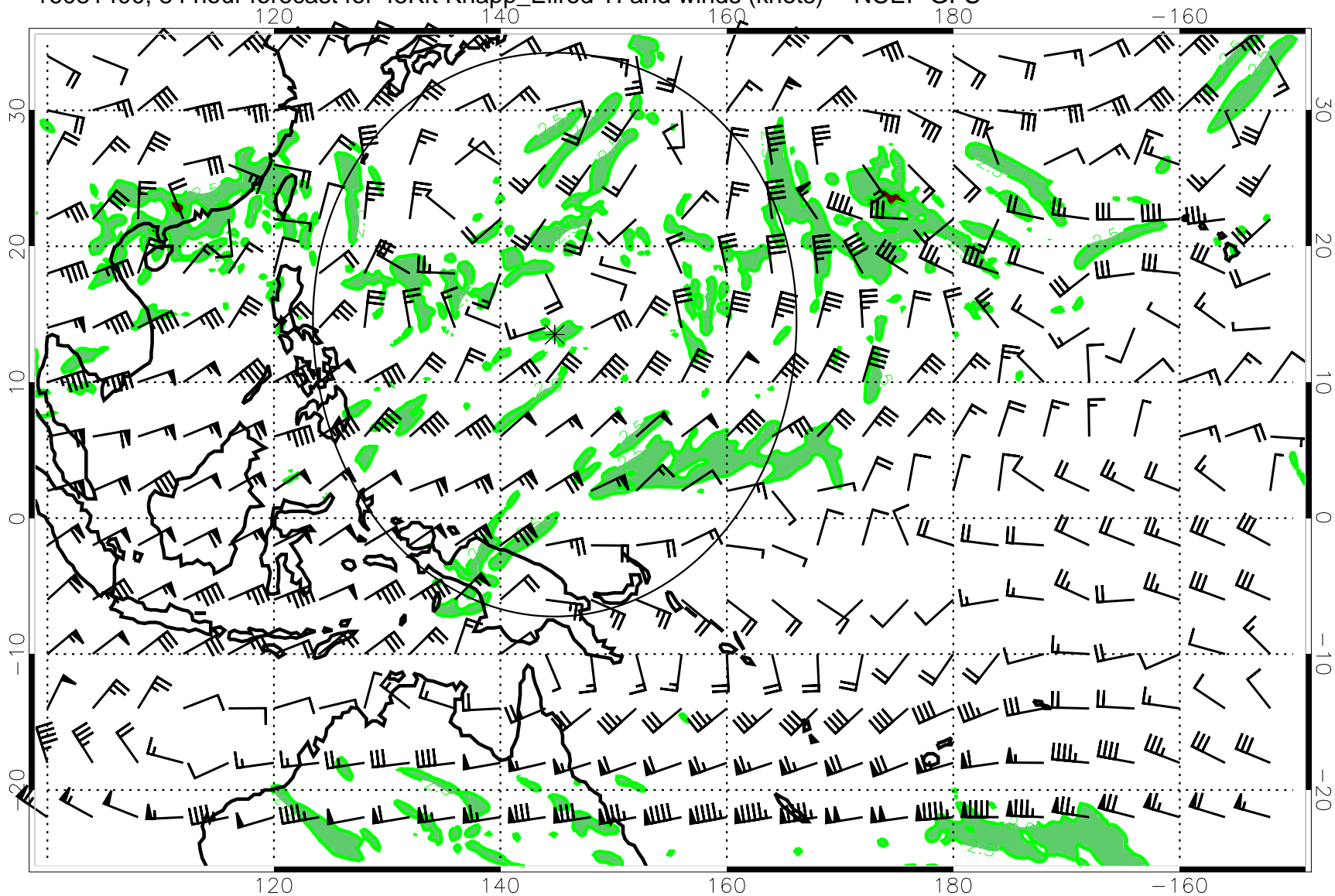
16081400, 84 hour forecast for 45Kft Knapp_Ellrod TI and winds (knots) -- NCEP GFS
