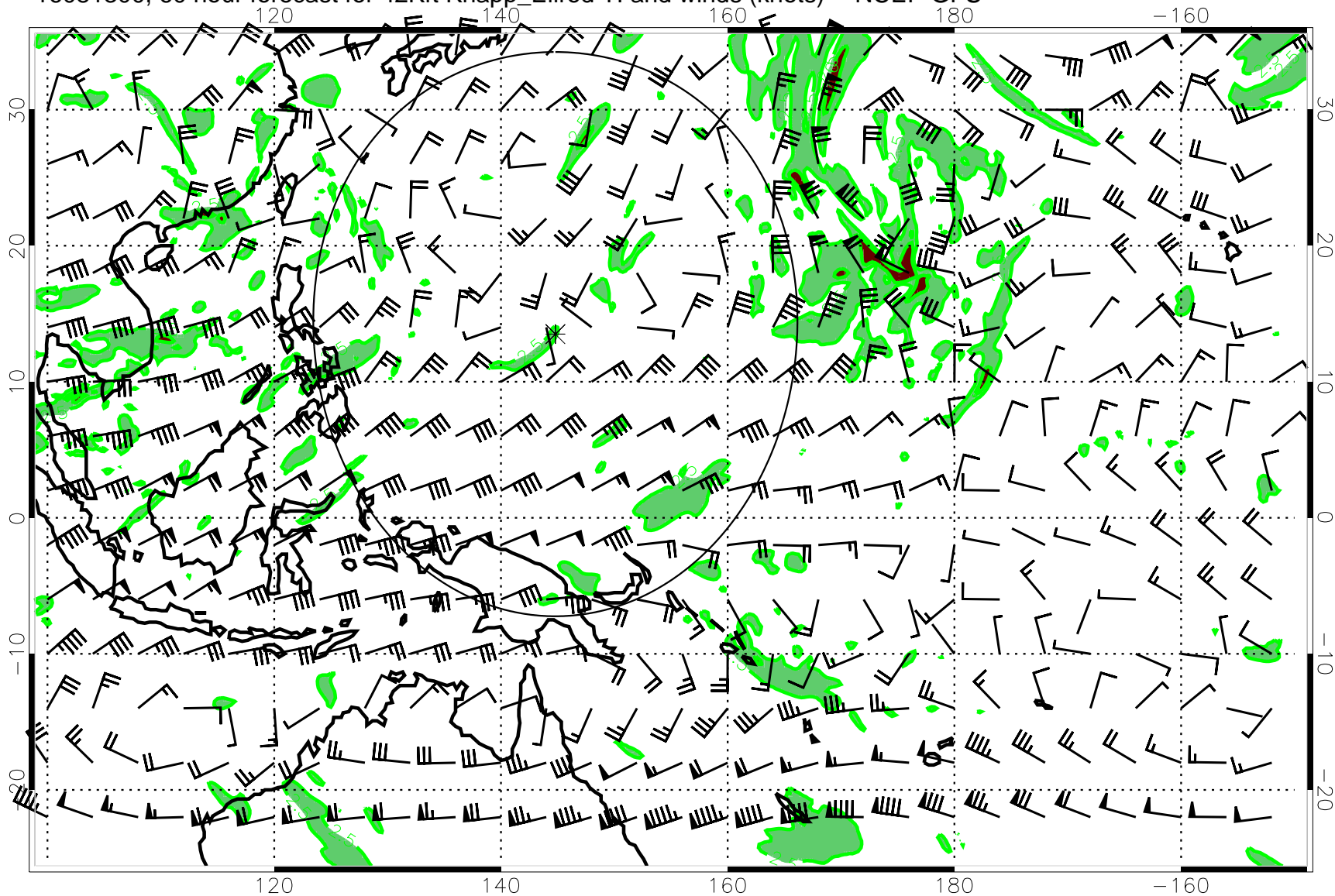
16081300, 60 hour forecast for 42Kft Knapp_Ellrod TI and winds (knots) -- NCEP GFS
