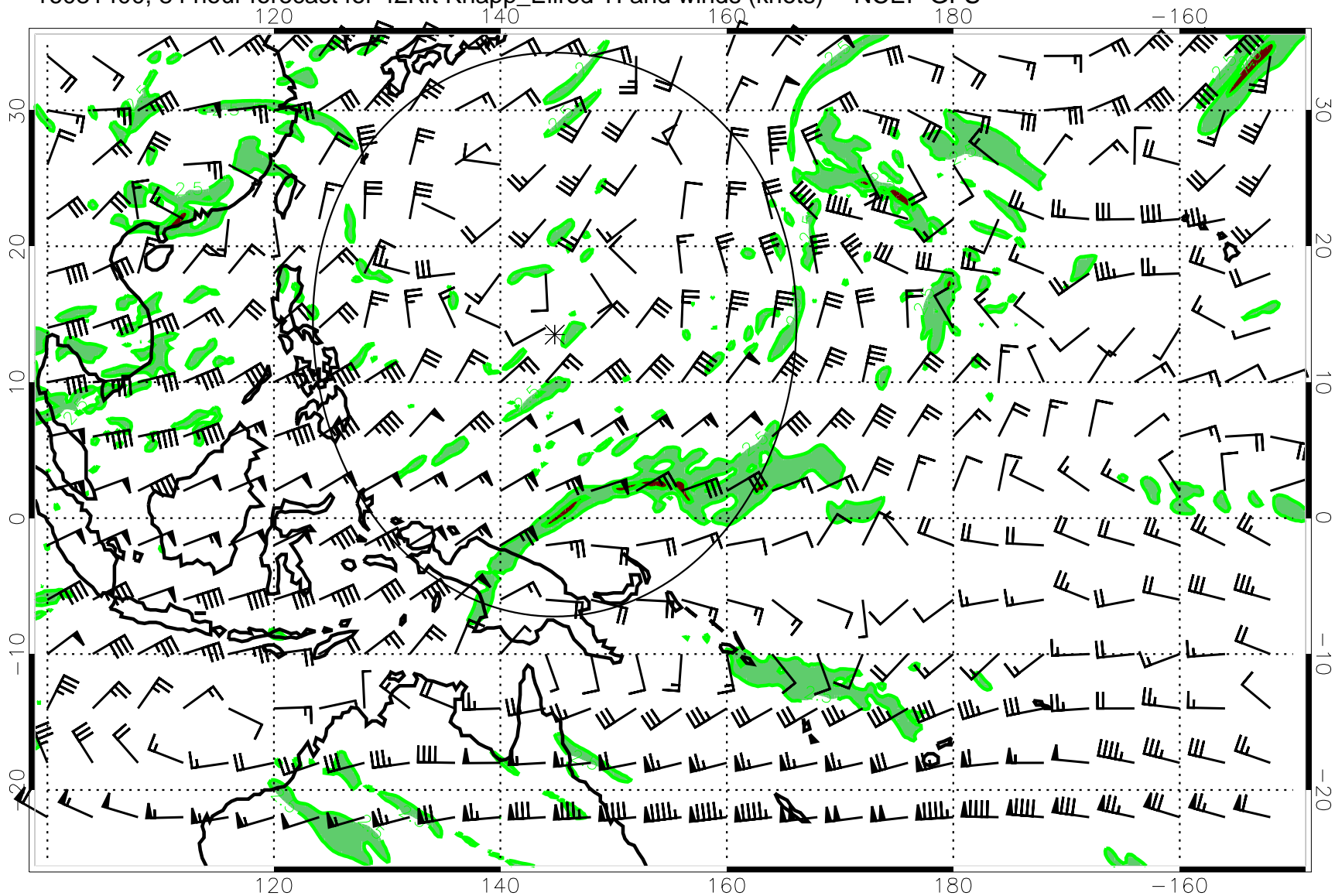
16081400, 84 hour forecast for 42Kft Knapp_Ellrod TI and winds (knots) -- NCEP GFS
