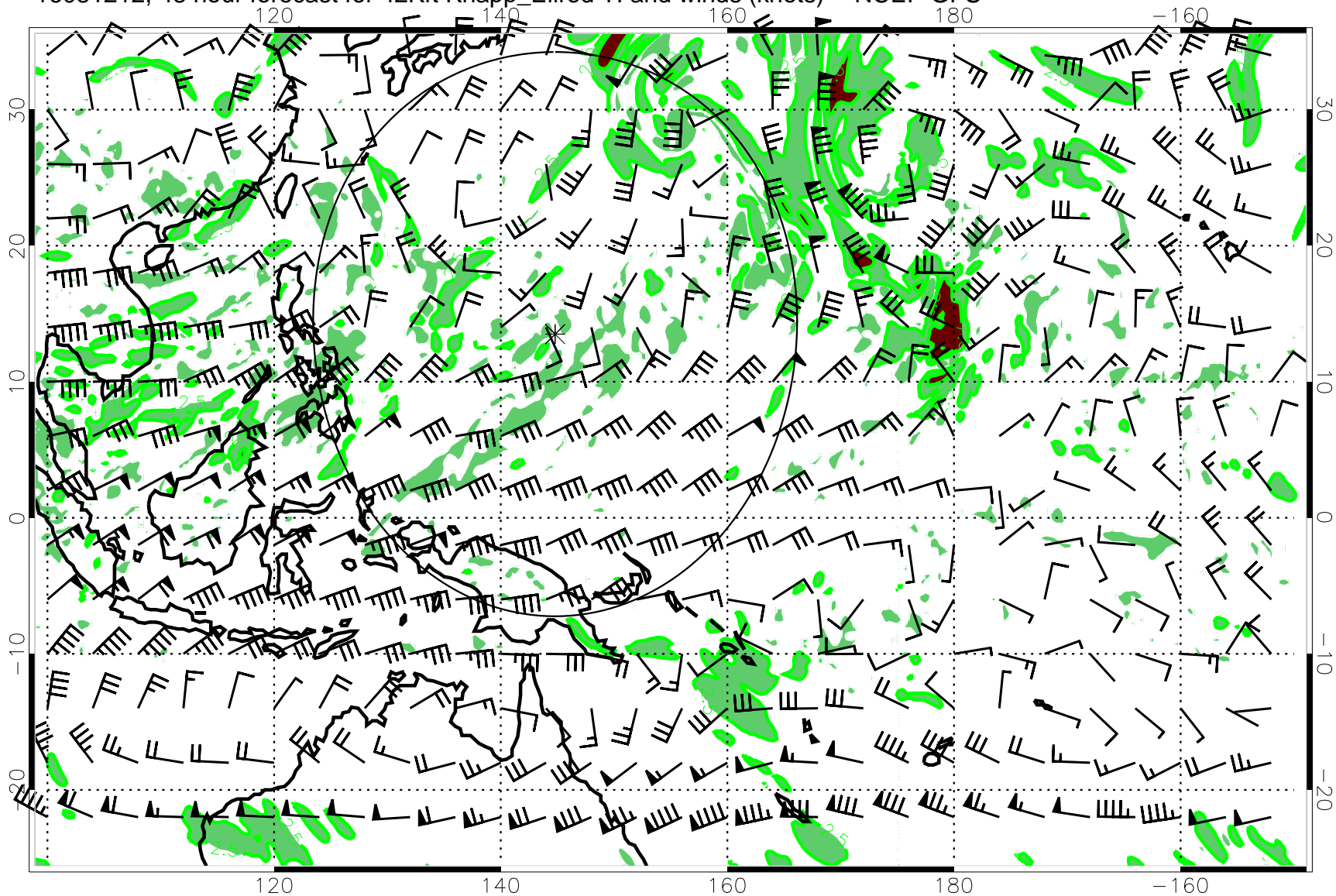
16081212, 48 hour forecast for 42Kft Knapp_Ellrod TI and winds (knots) -- NCEP GFS
