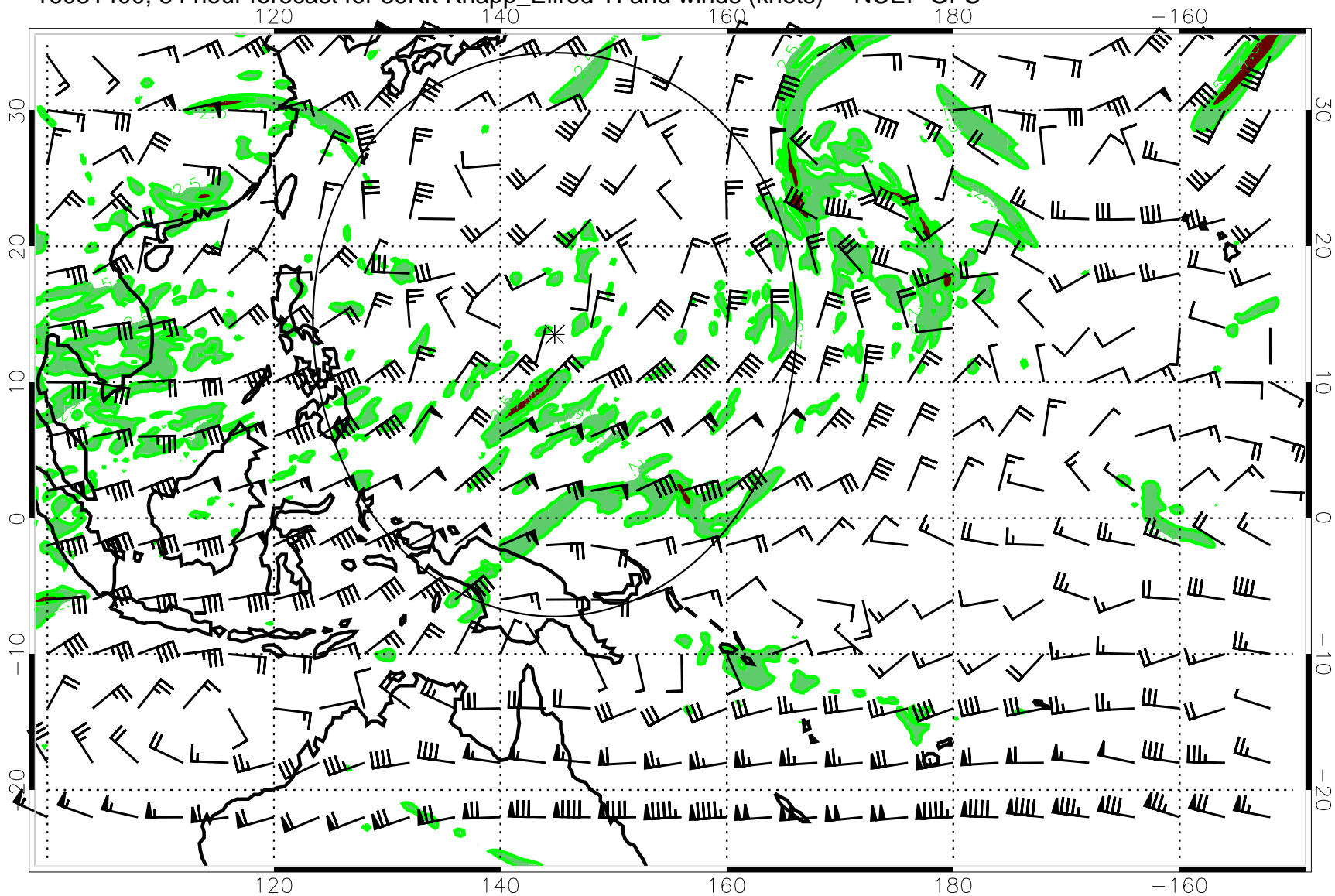
16081400, 84 hour forecast for 39Kft Knapp_Ellrod TI and winds (knots) -- NCEP GFS
