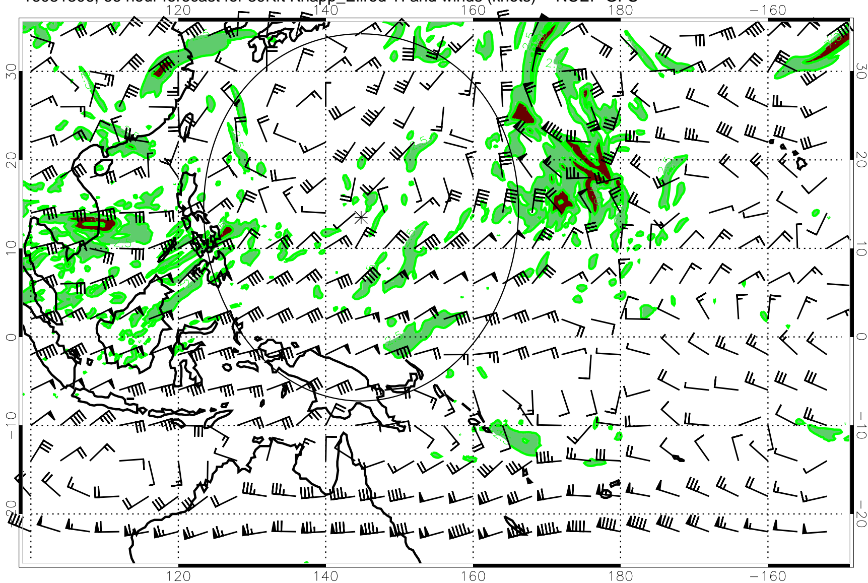
16081306, 66 hour forecast for 39Kft Knapp_Ellrod TI and winds (knots) -- NCEP GFS
