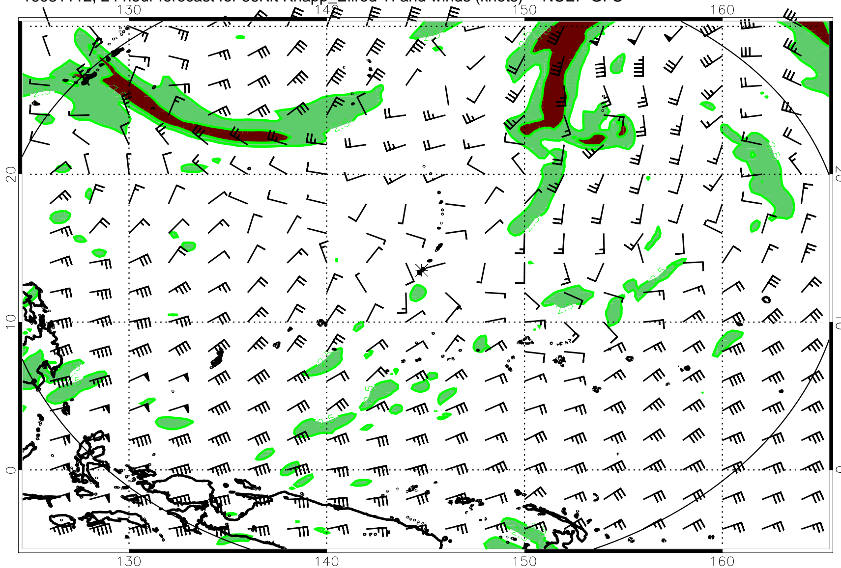
16081112, 24 hour forecast for 36Kft Knapp_Ellrod TI and winds (knots) -- NCEP GFS
