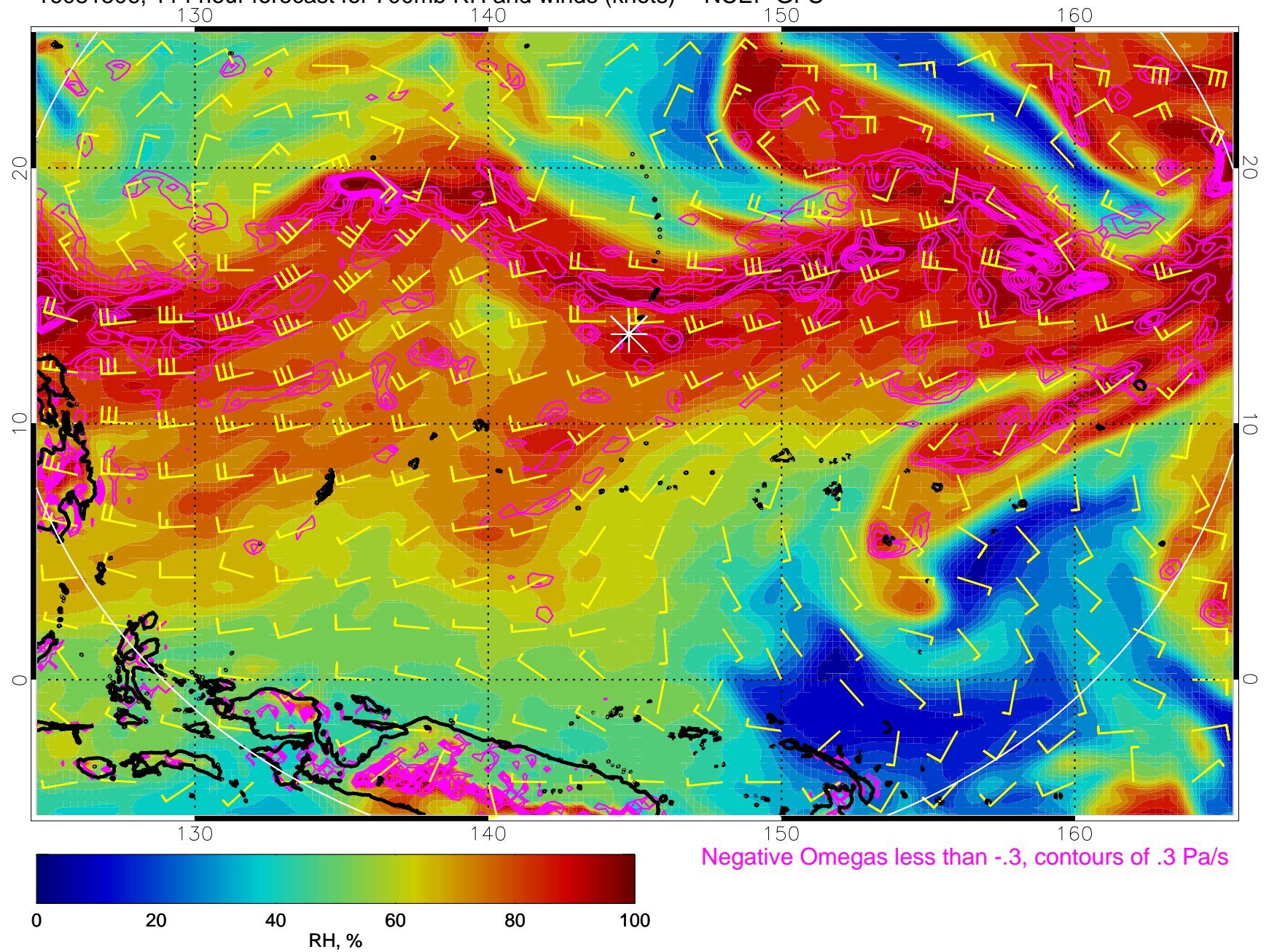
16081506, 114 hour forecast for 700mb RH and winds (knots) -- NCEP GFS
