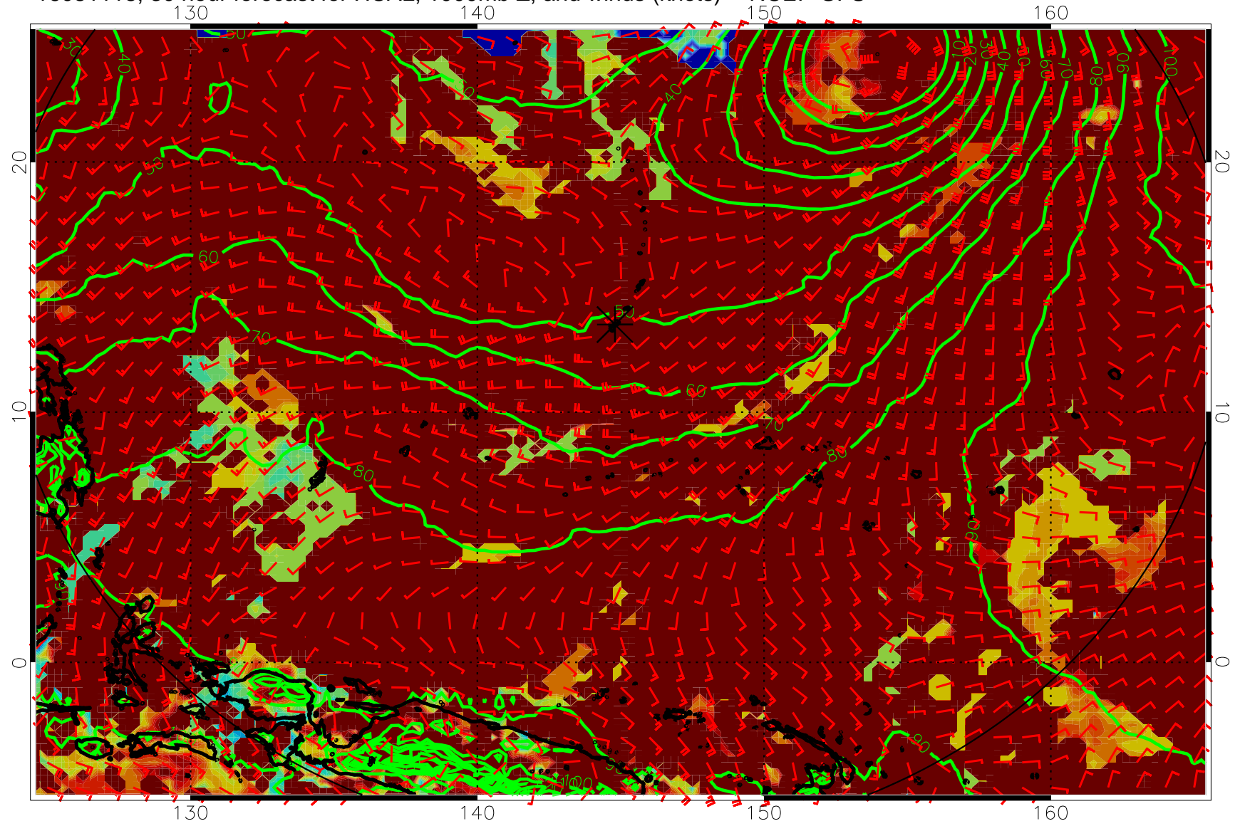
16081118, 30 hour forecast for HCAL, 1000mb Z, and winds (knots) -- NCEP GFS
