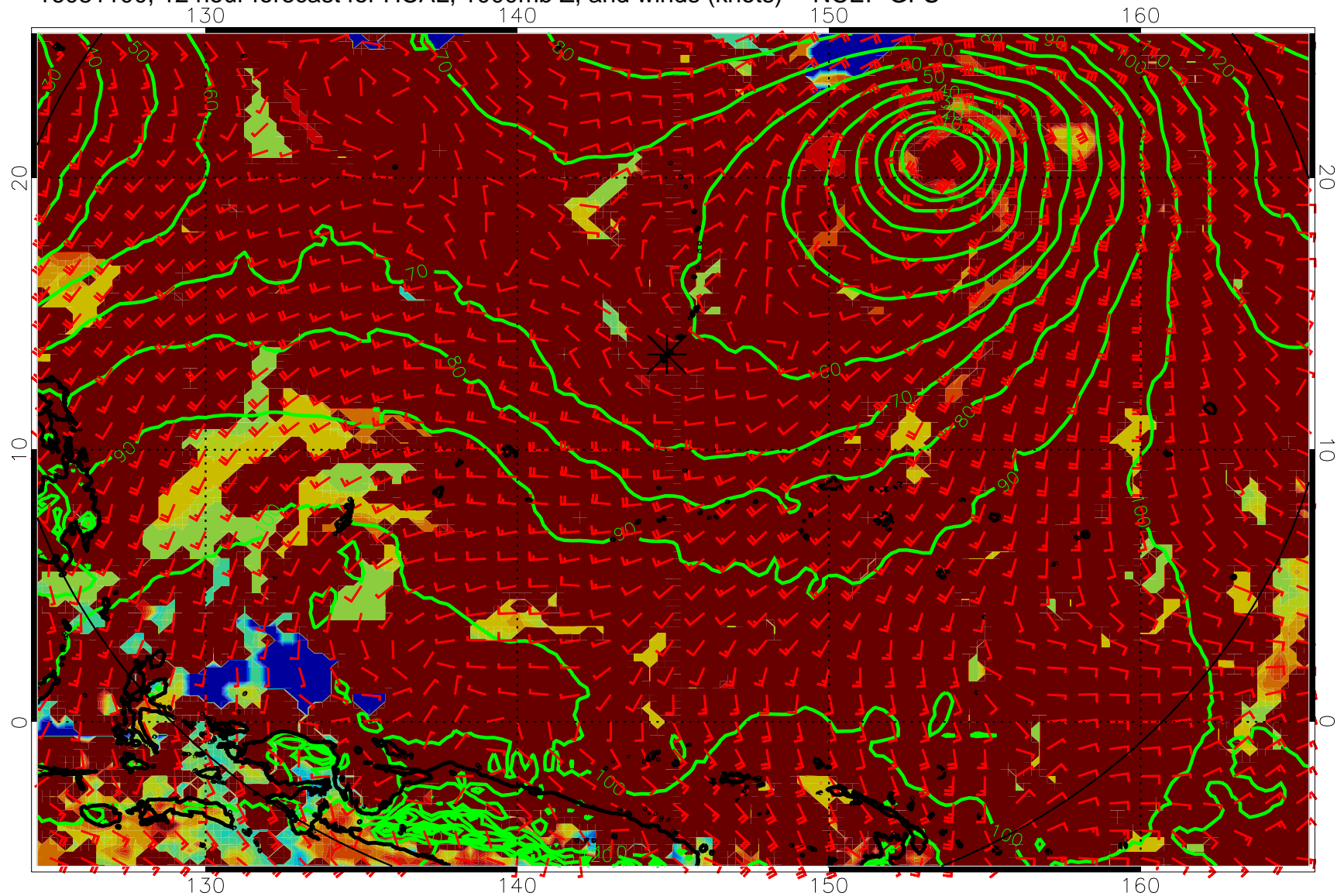
16081100, 12 hour forecast for HCAL, 1000mb Z, and winds (knots) -- NCEP GFS
