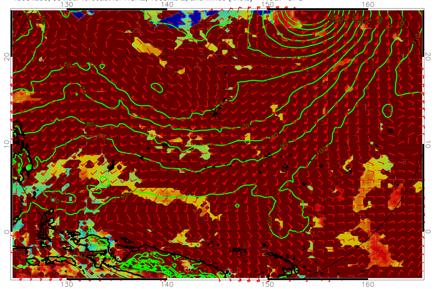
16081200, 36 hour forecast for HCAL, 1000mb Z, and winds (knots) -- NCEP GFS
