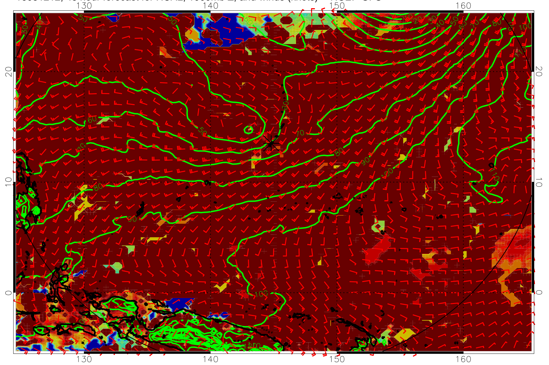
16081212, 48 hour forecast for HCAL, 1000mb Z, and winds (knots) -- NCEP GFS
