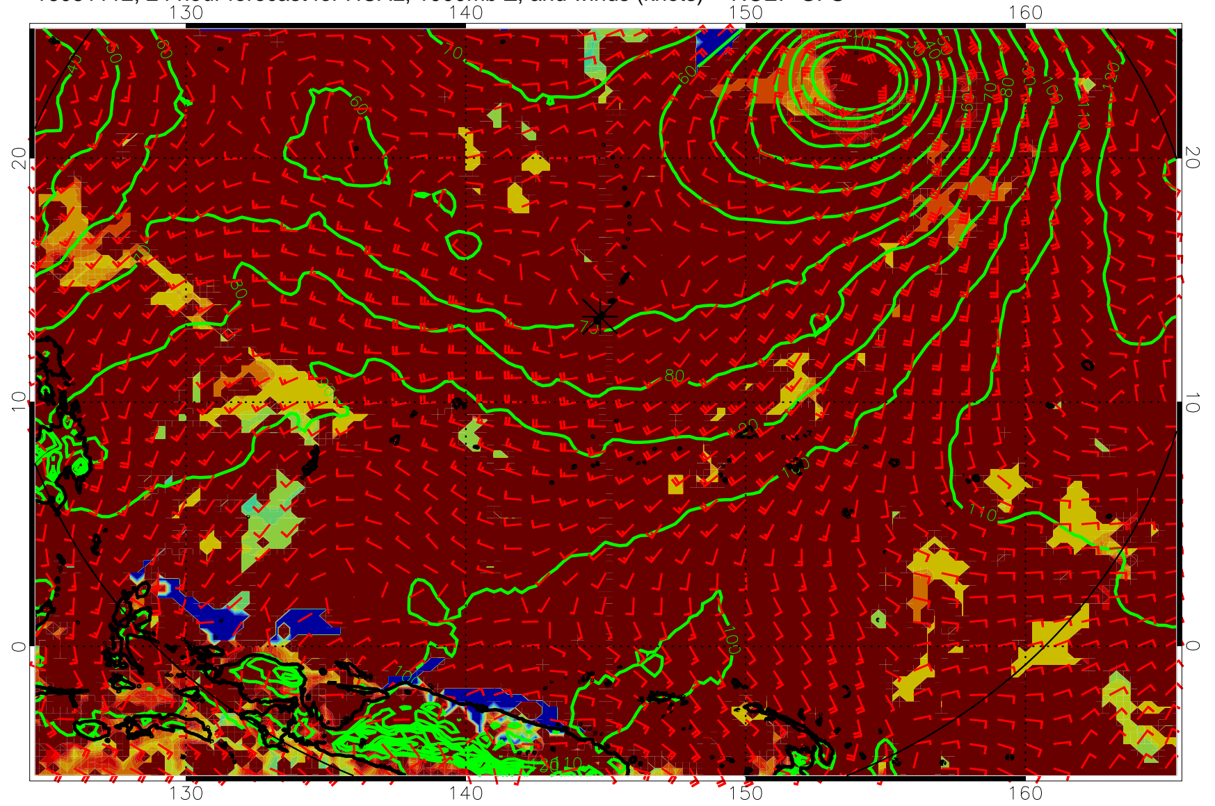
16081112, 24 hour forecast for HCAL, 1000mb Z, and winds (knots) -- NCEP GFS
