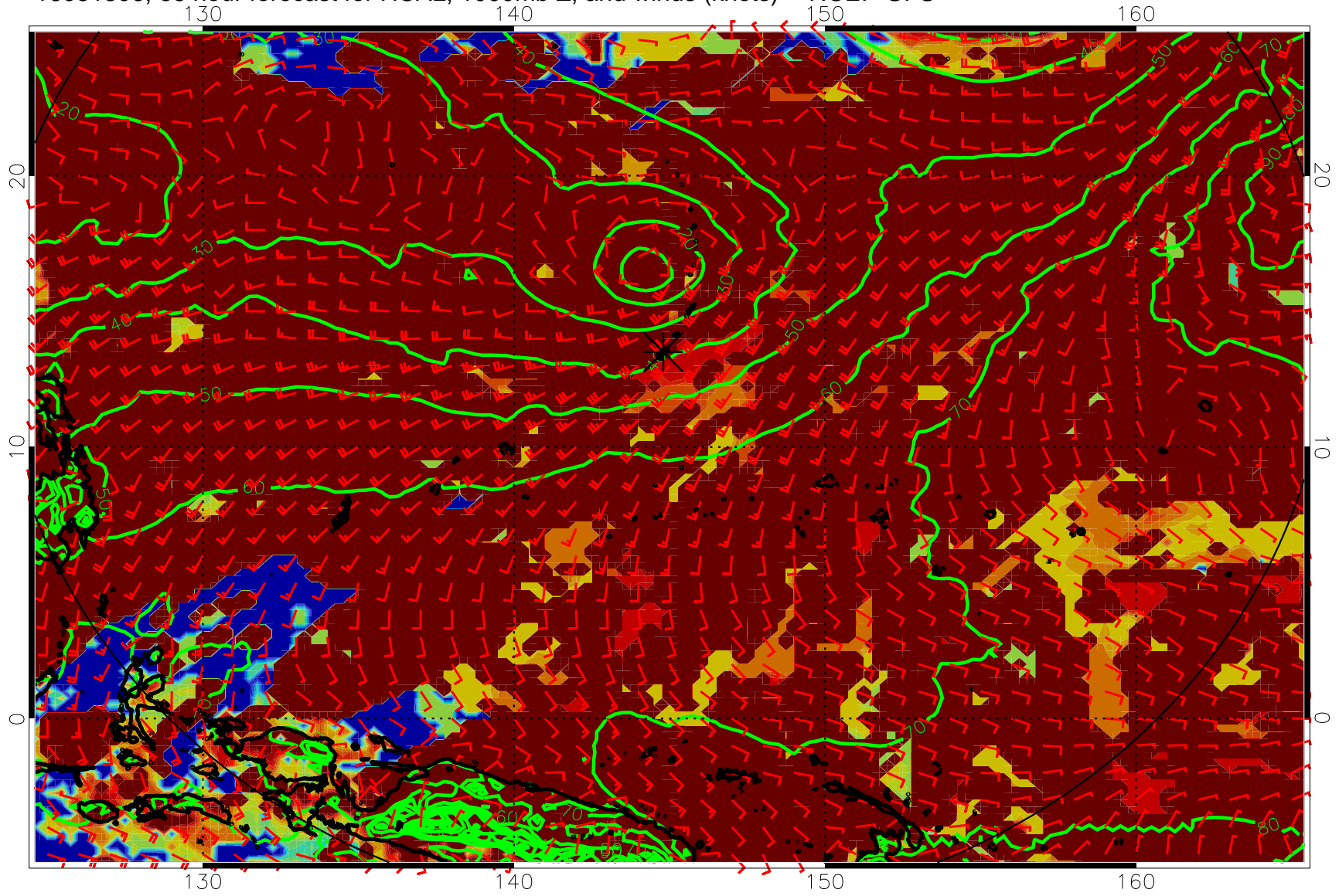
16081306, 66 hour forecast for HCAL, 1000mb Z, and winds (knots) -- NCEP GFS
