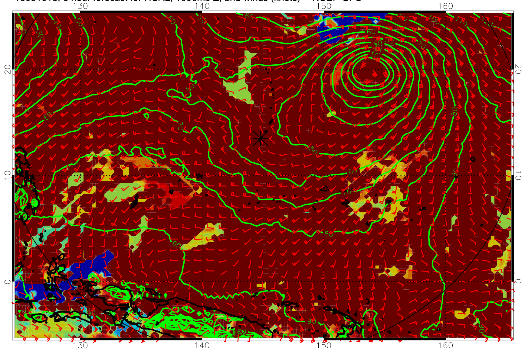
16081018, 6 hour forecast for HCAL, 1000mb Z, and winds (knots) -- NCEP GFS
