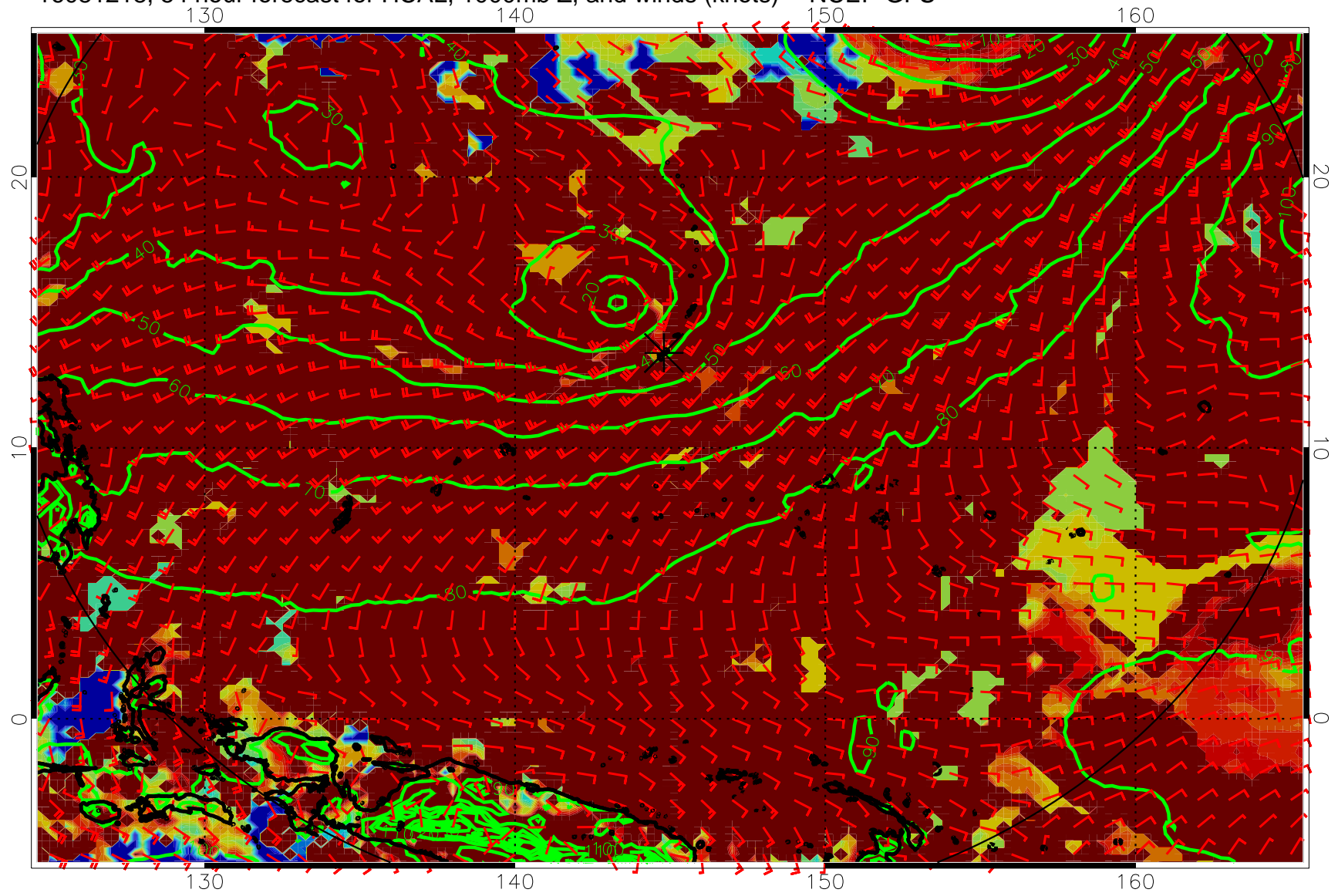
16081218, 54 hour forecast for HCAL, 1000mb Z, and winds (knots) -- NCEP GFS
