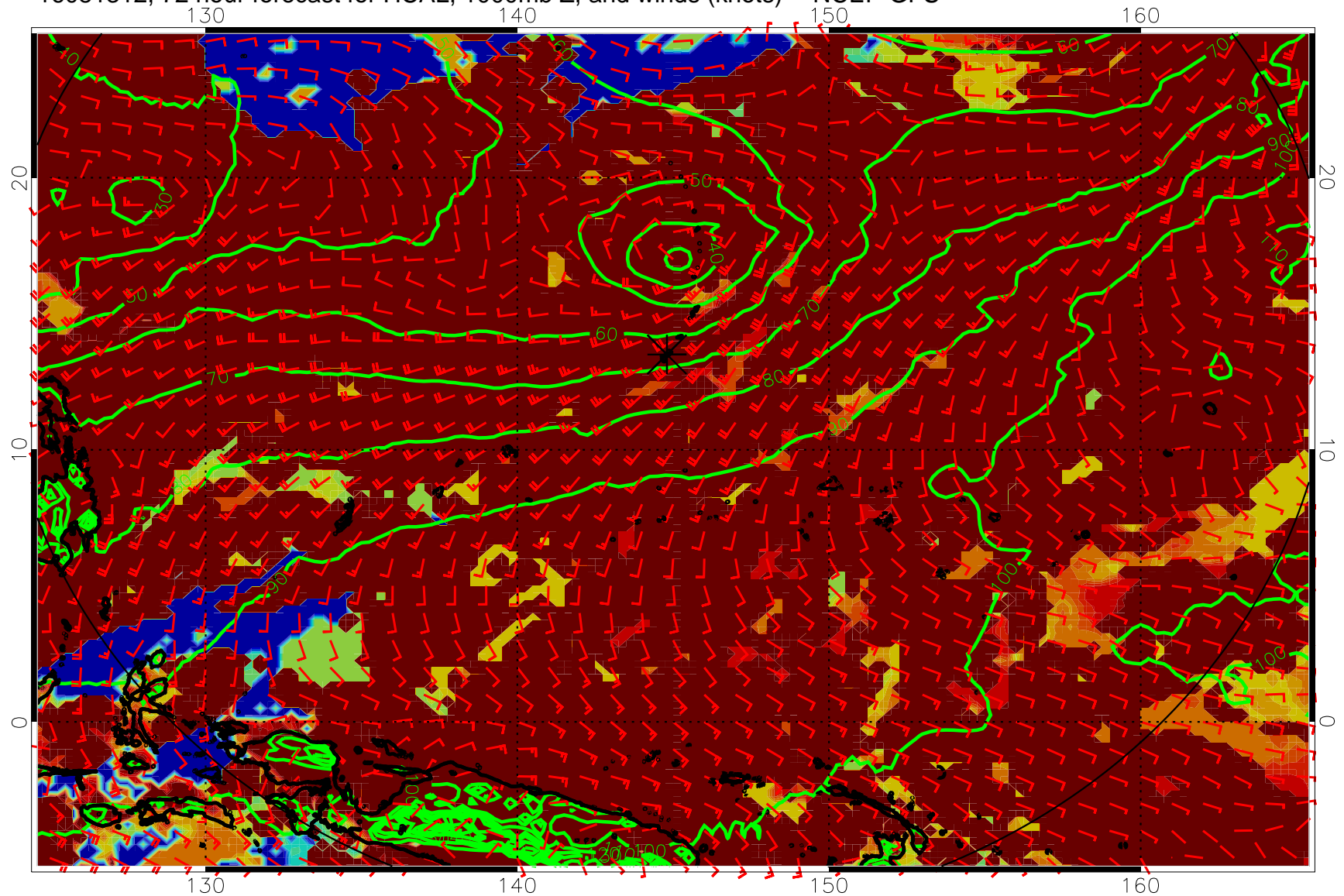
16081312, 72 hour forecast for HCAL, 1000mb Z, and winds (knots) -- NCEP GFS
