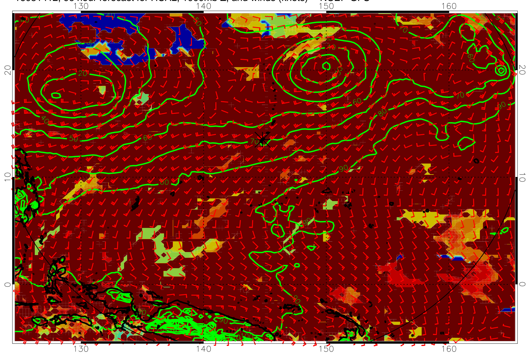
16081412, 96 hour forecast for HCAL, 1000mb Z, and winds (knots) -- NCEP GFS
