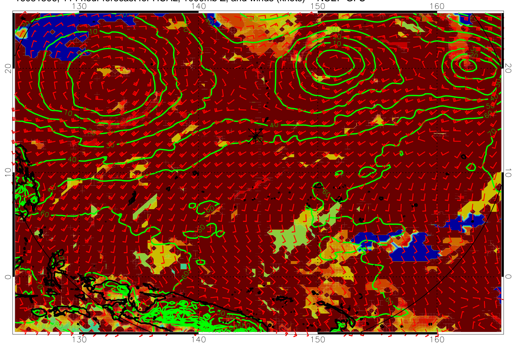
16081506, 114 hour forecast for HCAL, 1000mb Z, and winds (knots) -- NCEP GFS
