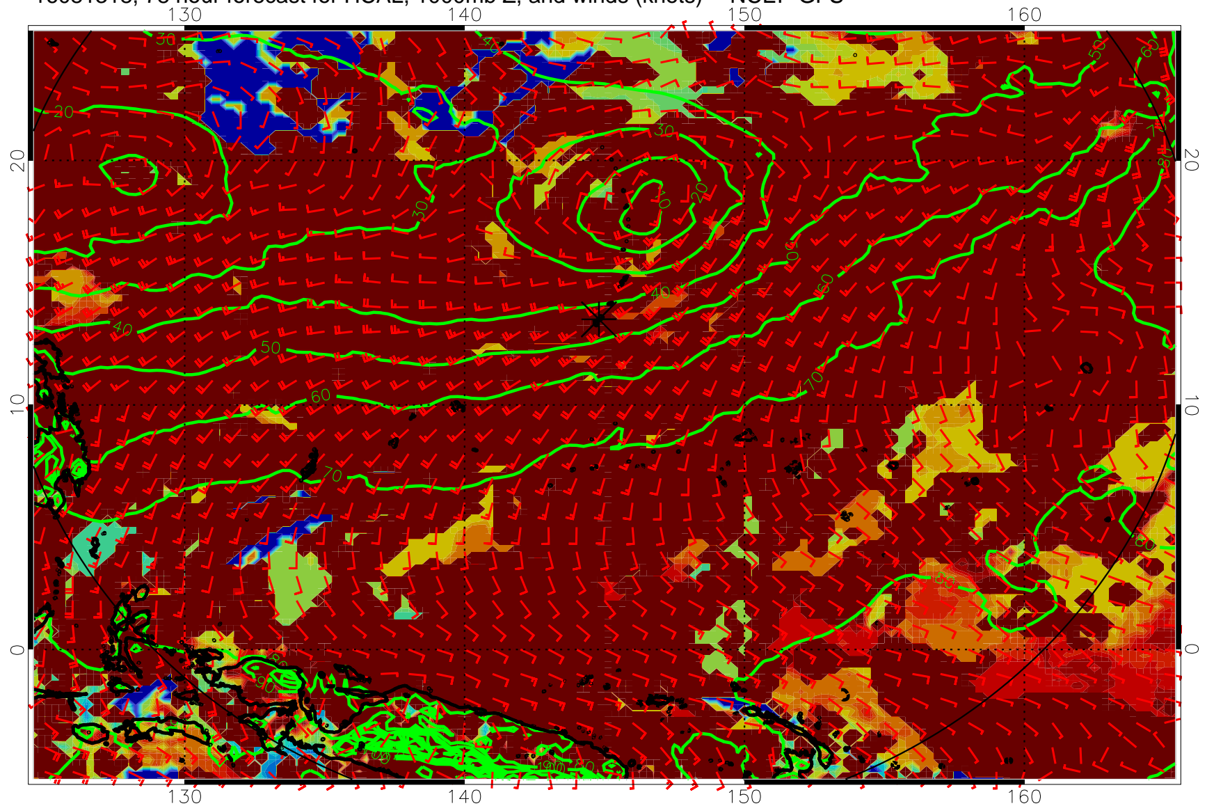
16081318, 78 hour forecast for HCAL, 1000mb Z, and winds (knots) -- NCEP GFS
