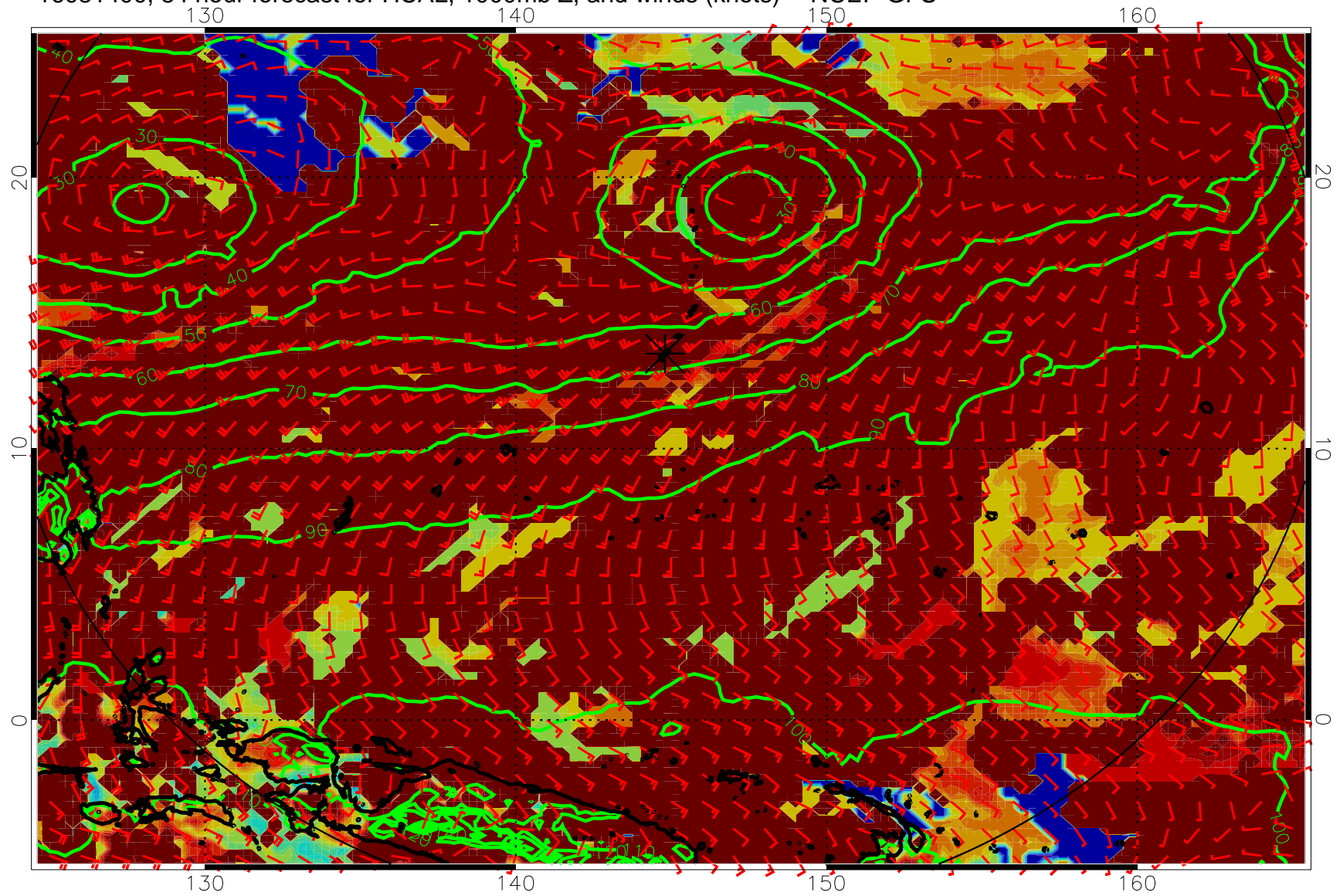
16081400, 84 hour forecast for HCAL, 1000mb Z, and winds (knots) -- NCEP GFS
