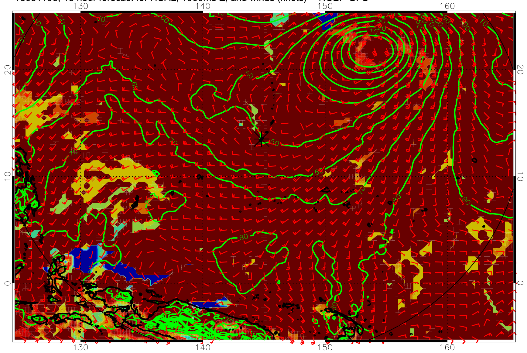
16081106, 18 hour forecast for HCAL, 1000mb Z, and winds (knots) -- NCEP GFS
