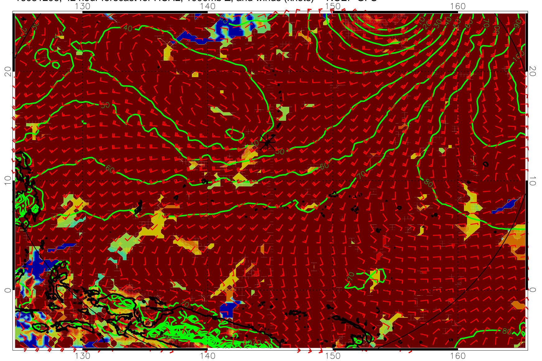
16081206, 42 hour forecast for HCAL, 1000mb Z, and winds (knots) -- NCEP GFS
