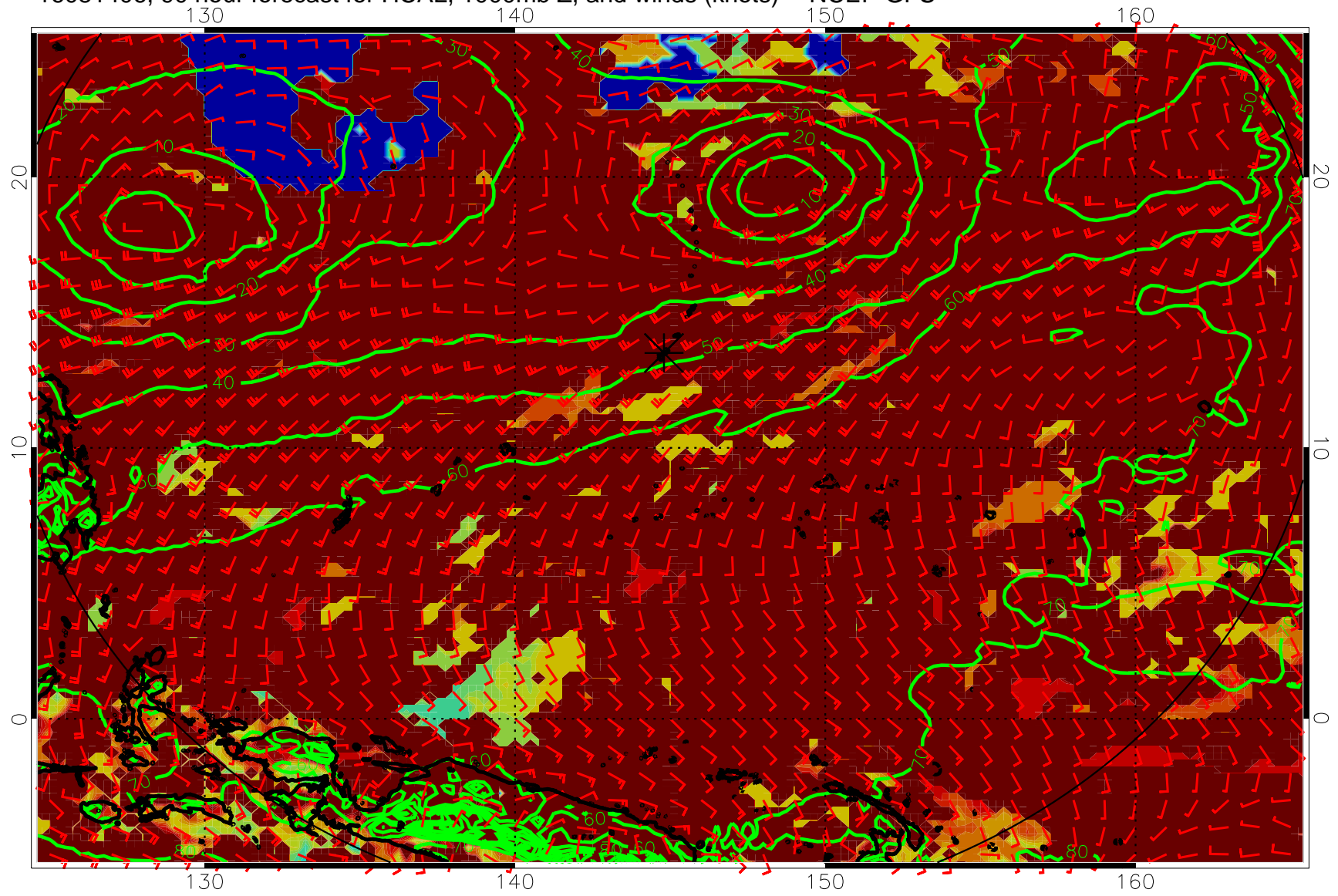
16081406, 90 hour forecast for HCAL, 1000mb Z, and winds (knots) -- NCEP GFS
