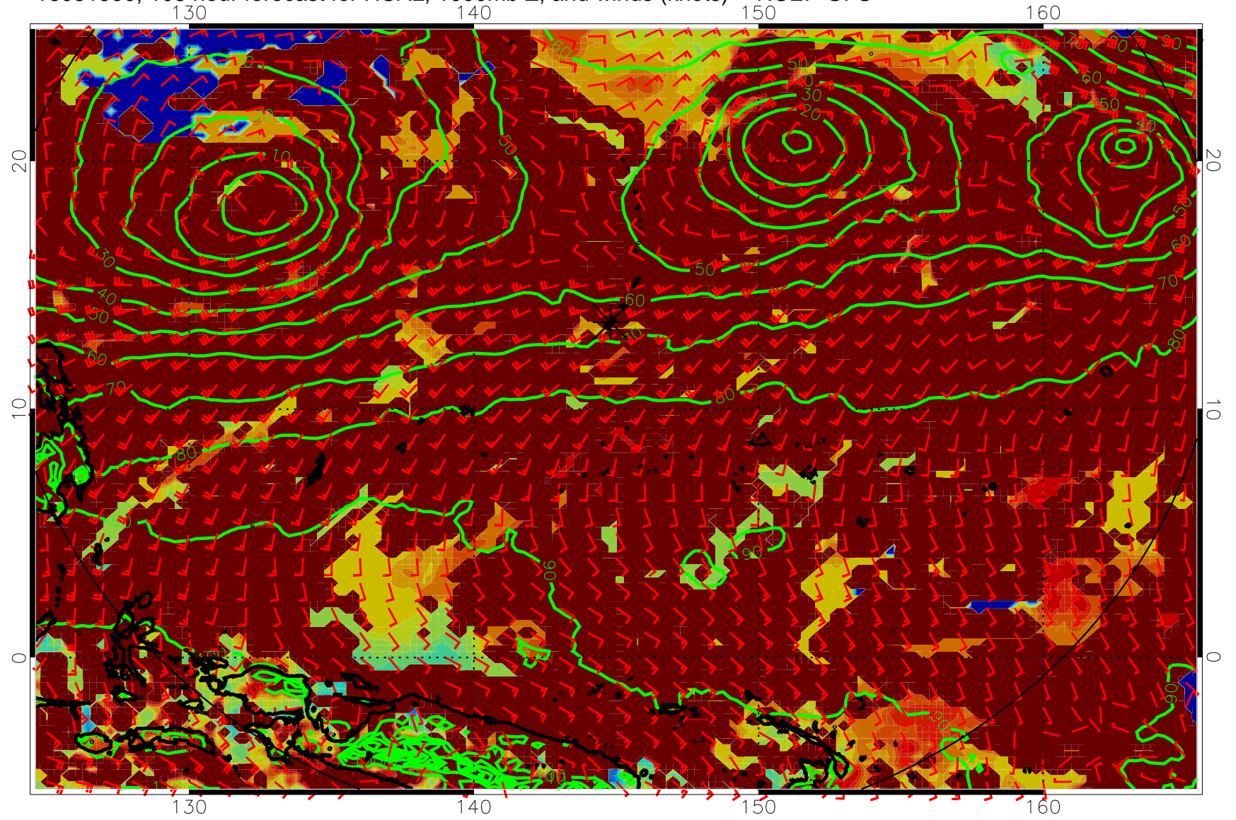
16081500, 108 hour forecast for HCAL, 1000mb Z, and winds (knots) -- NCEP GFS
