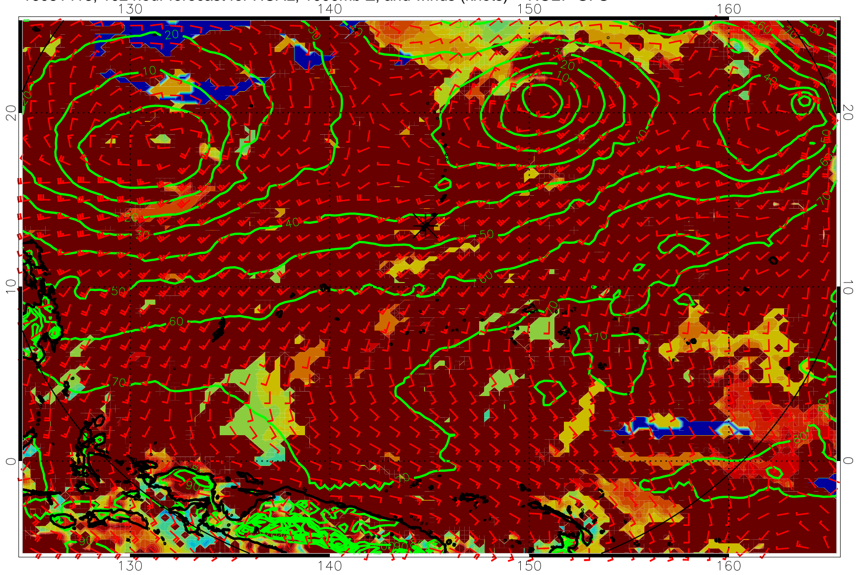
16081418, 102 hour forecast for HCAL, 1000mb Z, and winds (knots) -- NCEP GFS
