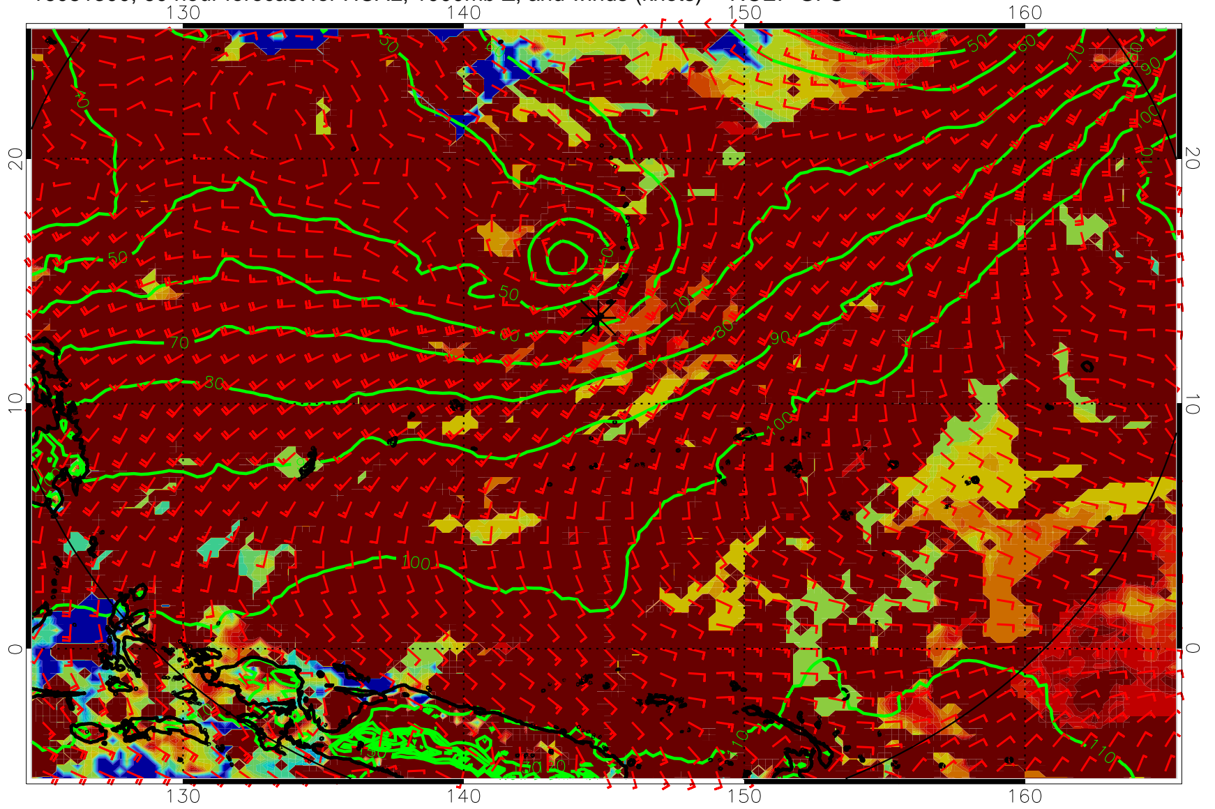
16081300, 60 hour forecast for HCAL, 1000mb Z, and winds (knots) -- NCEP GFS
