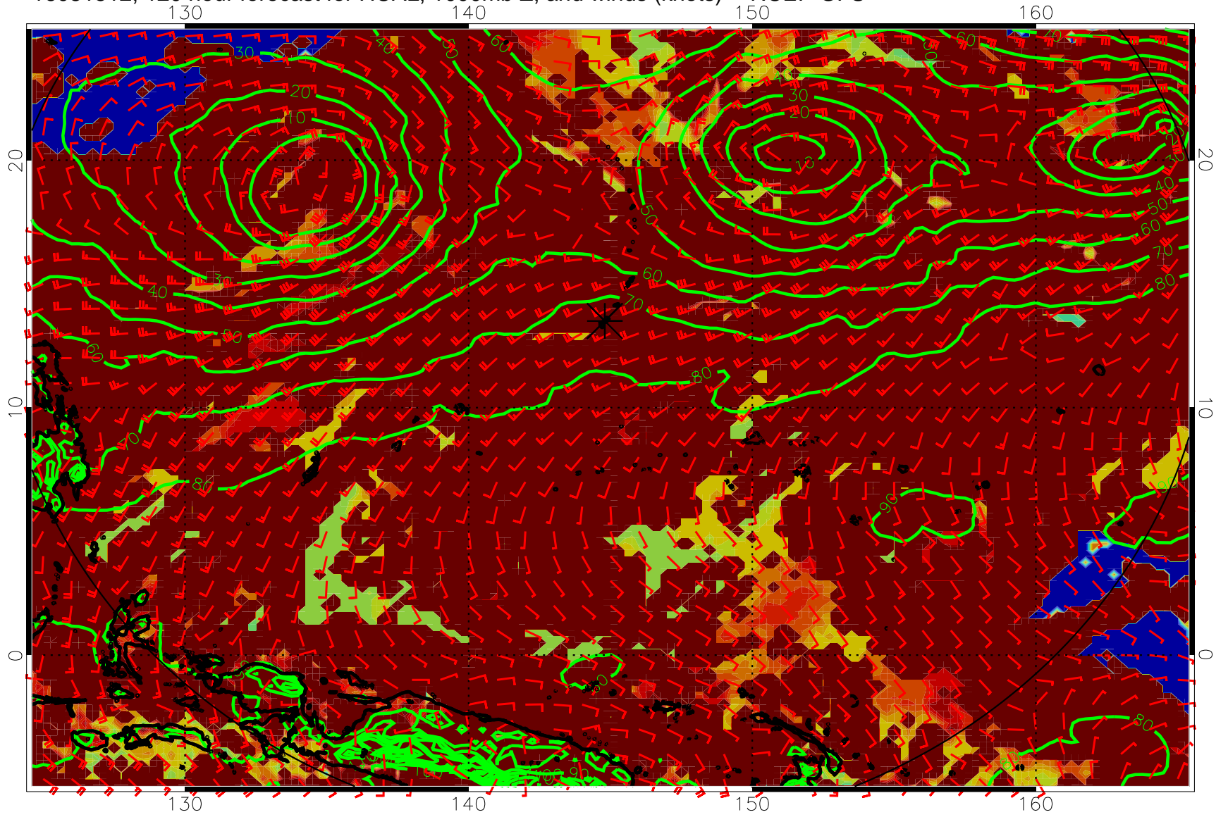
16081512, 120 hour forecast for HCAL, 1000mb Z, and winds (knots) -- NCEP GFS
