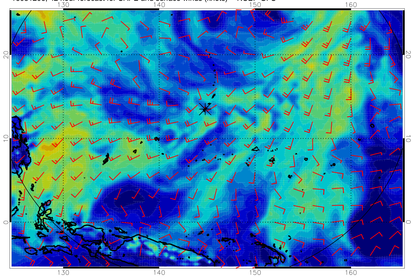
16081206, 42 hour forecast for CAPE and surface winds (knots) -- NCEP GFS
