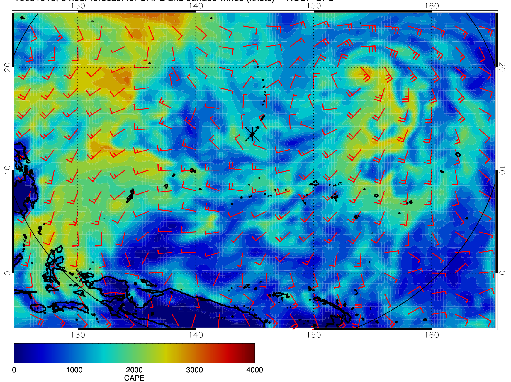
16081018, 6 hour forecast for CAPE and surface winds (knots) -- NCEP GFS
