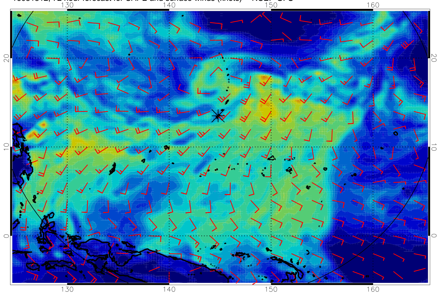
16081312, 72 hour forecast for CAPE and surface winds (knots) -- NCEP GFS
