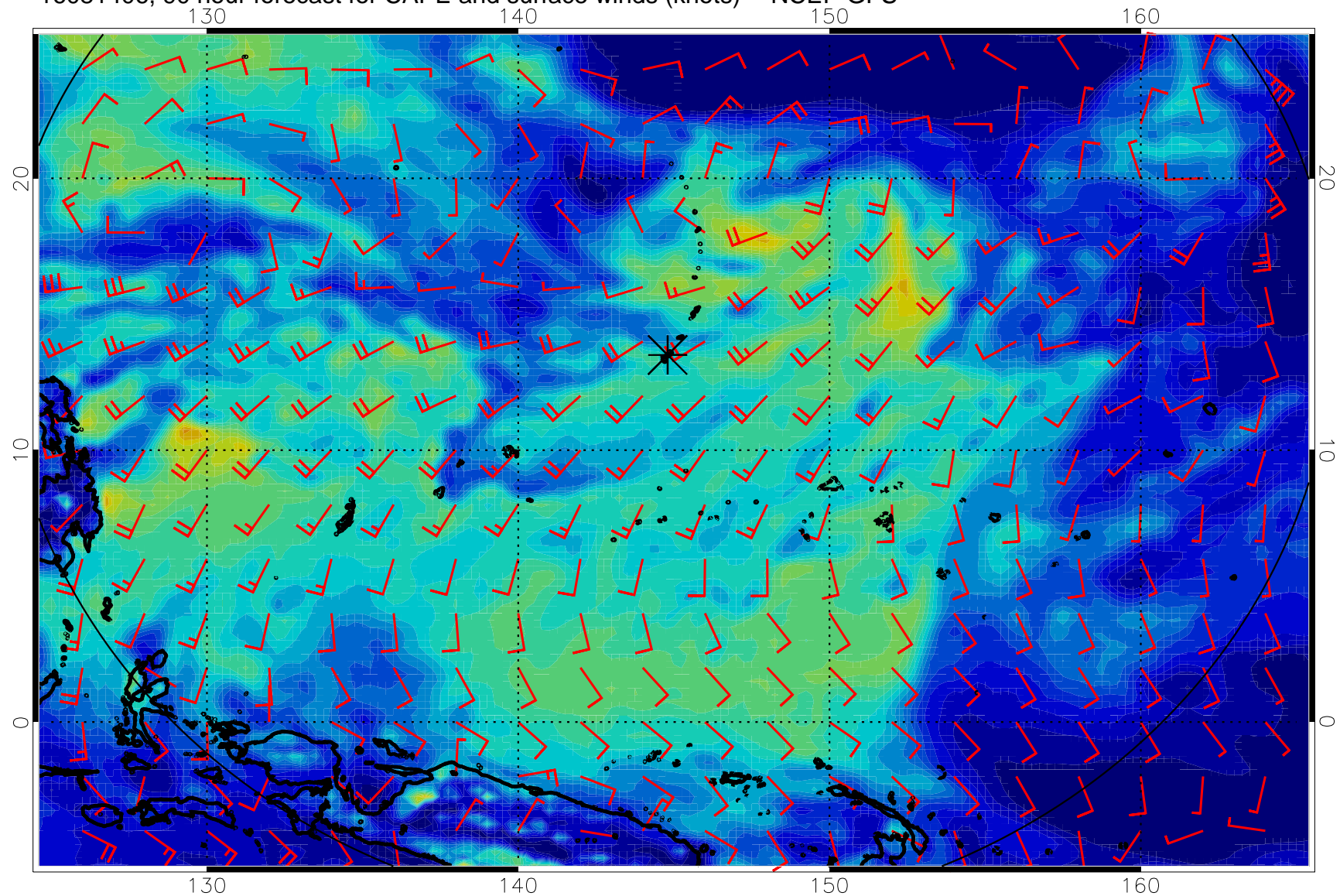
16081406, 90 hour forecast for CAPE and surface winds (knots) -- NCEP GFS
