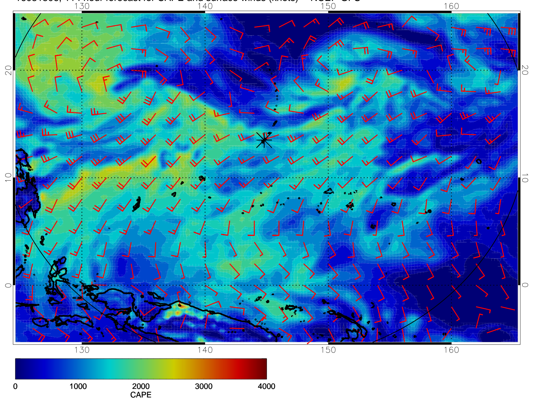
16081506, 114 hour forecast for CAPE and surface winds (knots) -- NCEP GFS
