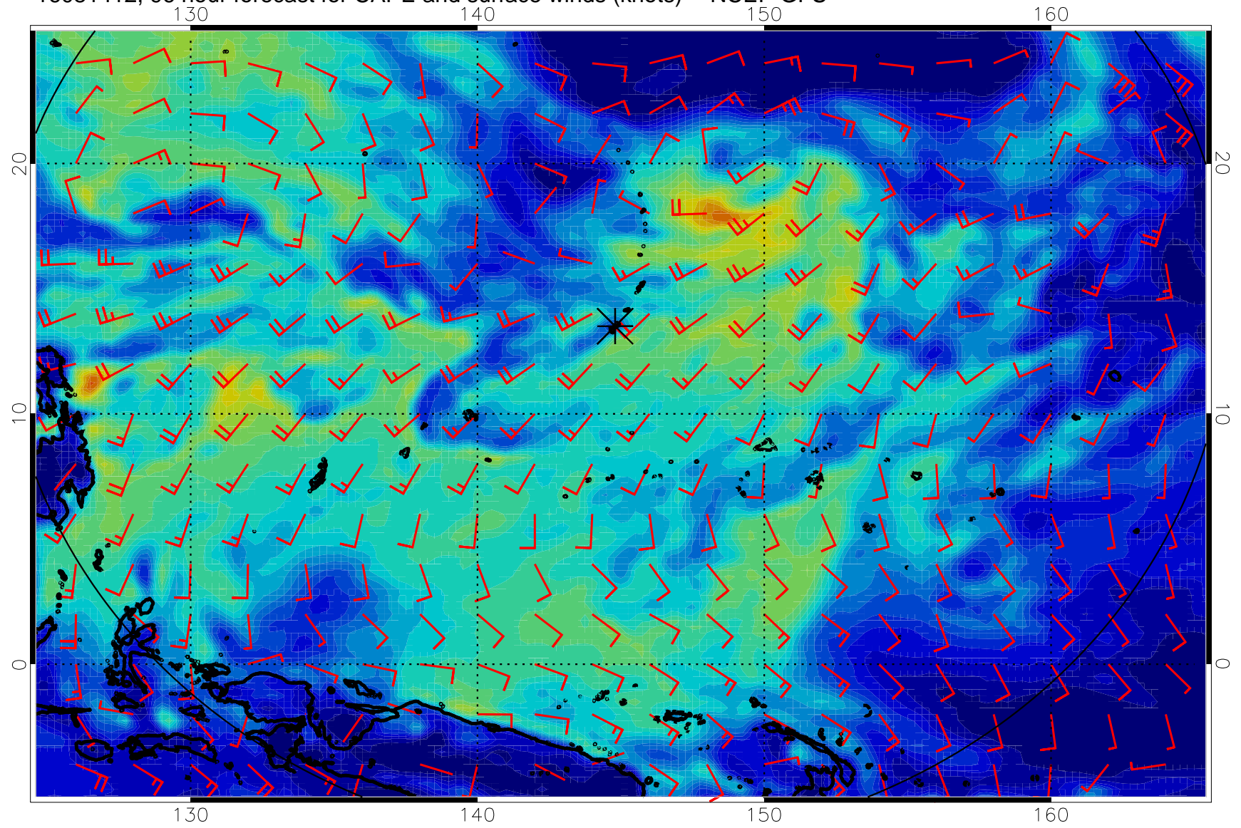
16081412, 96 hour forecast for CAPE and surface winds (knots) -- NCEP GFS
