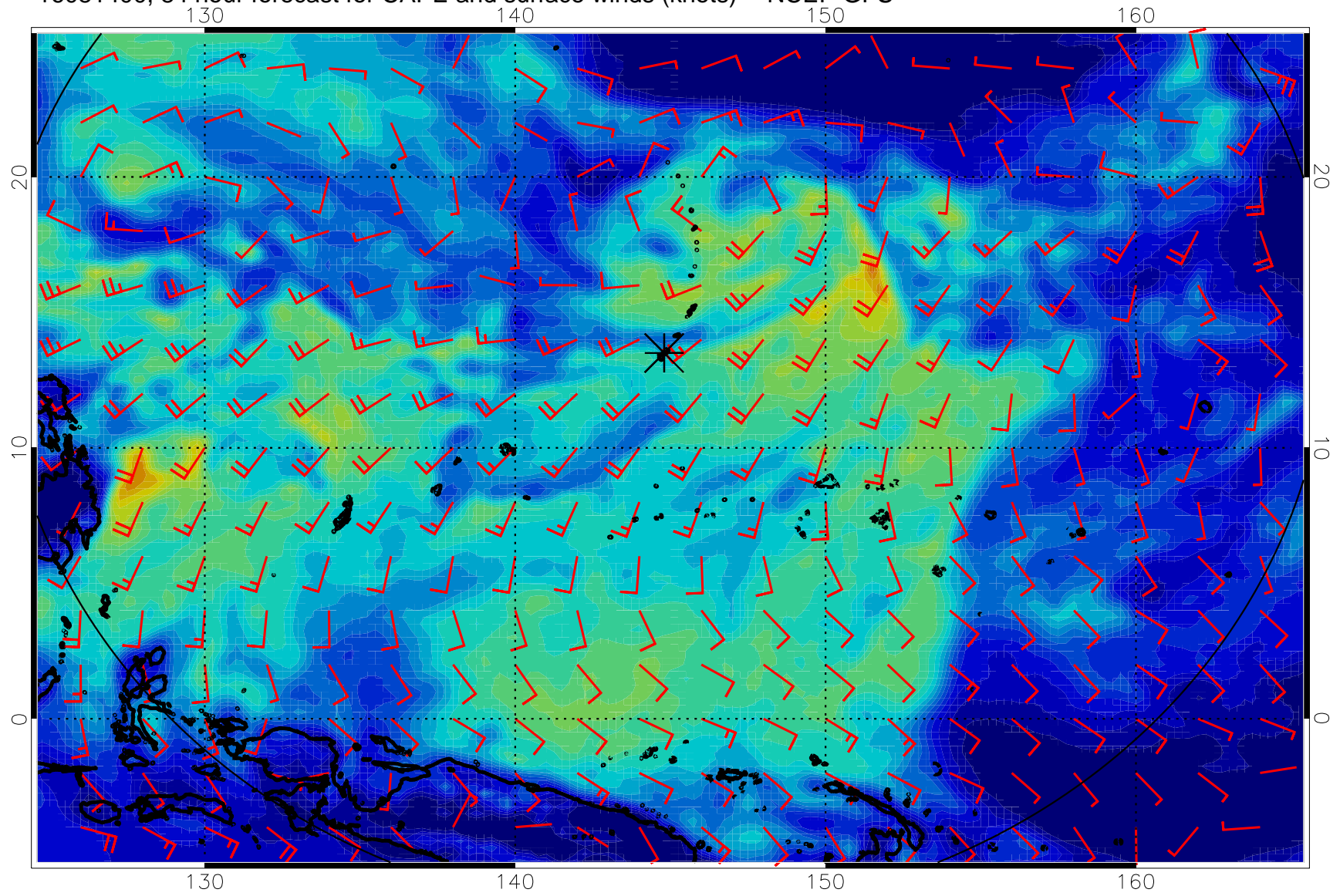
16081400, 84 hour forecast for CAPE and surface winds (knots) -- NCEP GFS
