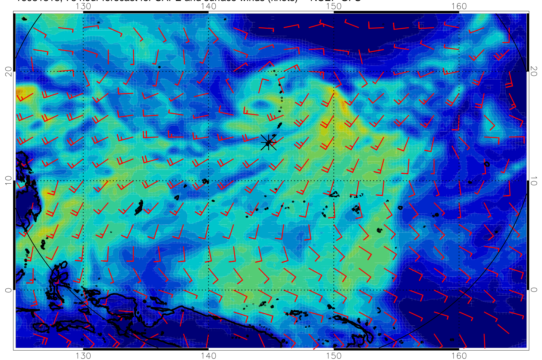
16081318, 78 hour forecast for CAPE and surface winds (knots) -- NCEP GFS
