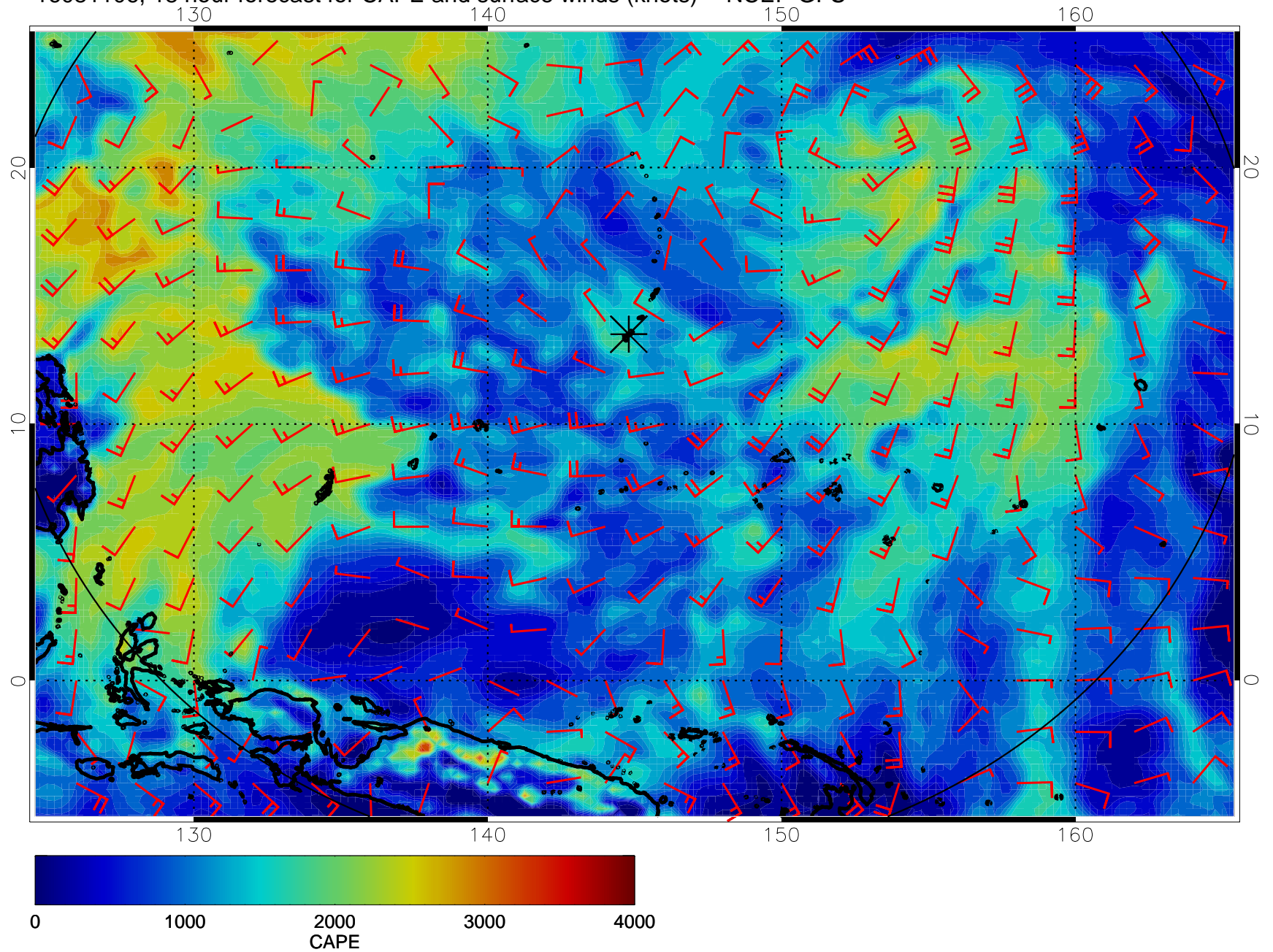
16081106, 18 hour forecast for CAPE and surface winds (knots) -- NCEP GFS
