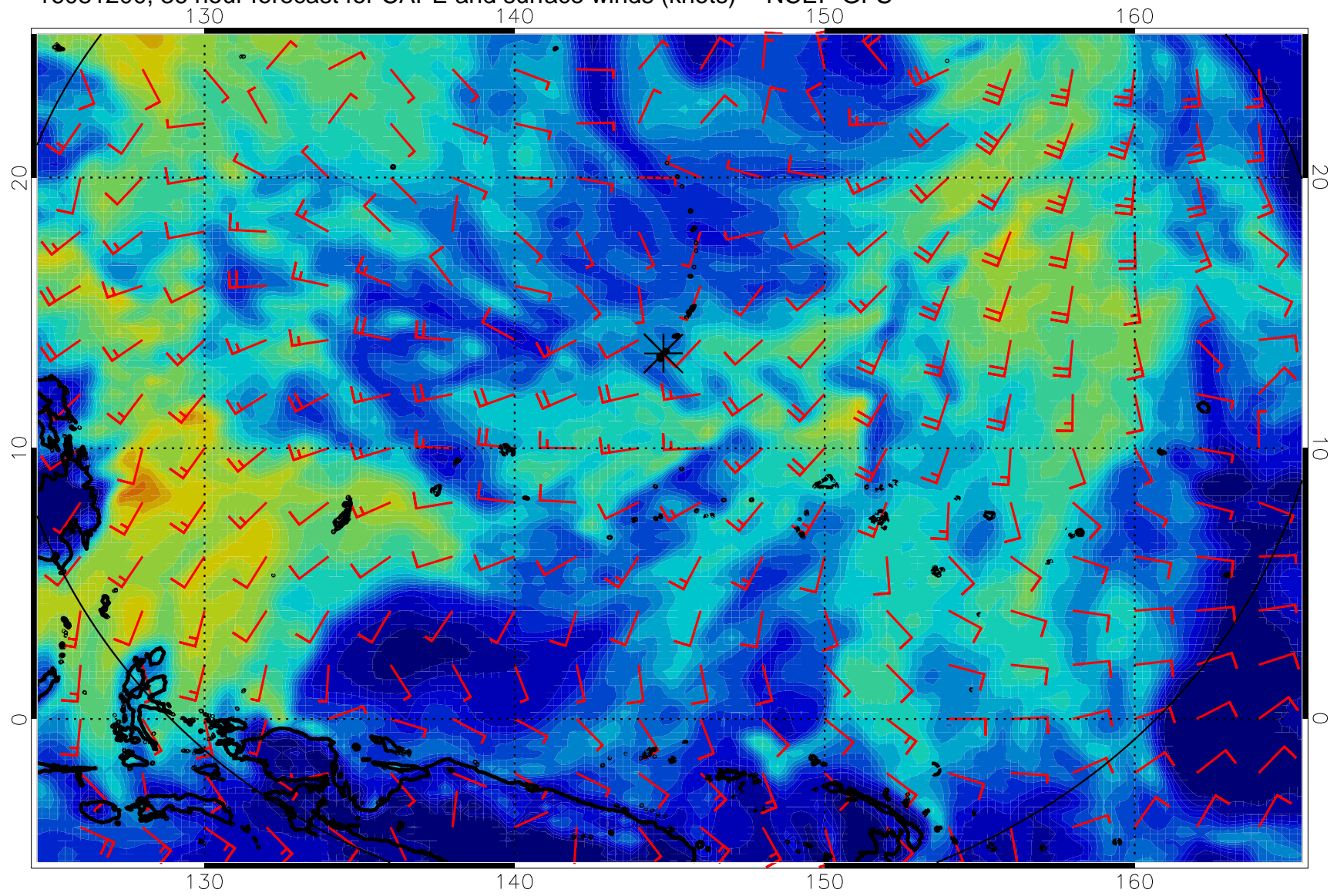
16081200, 36 hour forecast for CAPE and surface winds (knots) -- NCEP GFS
