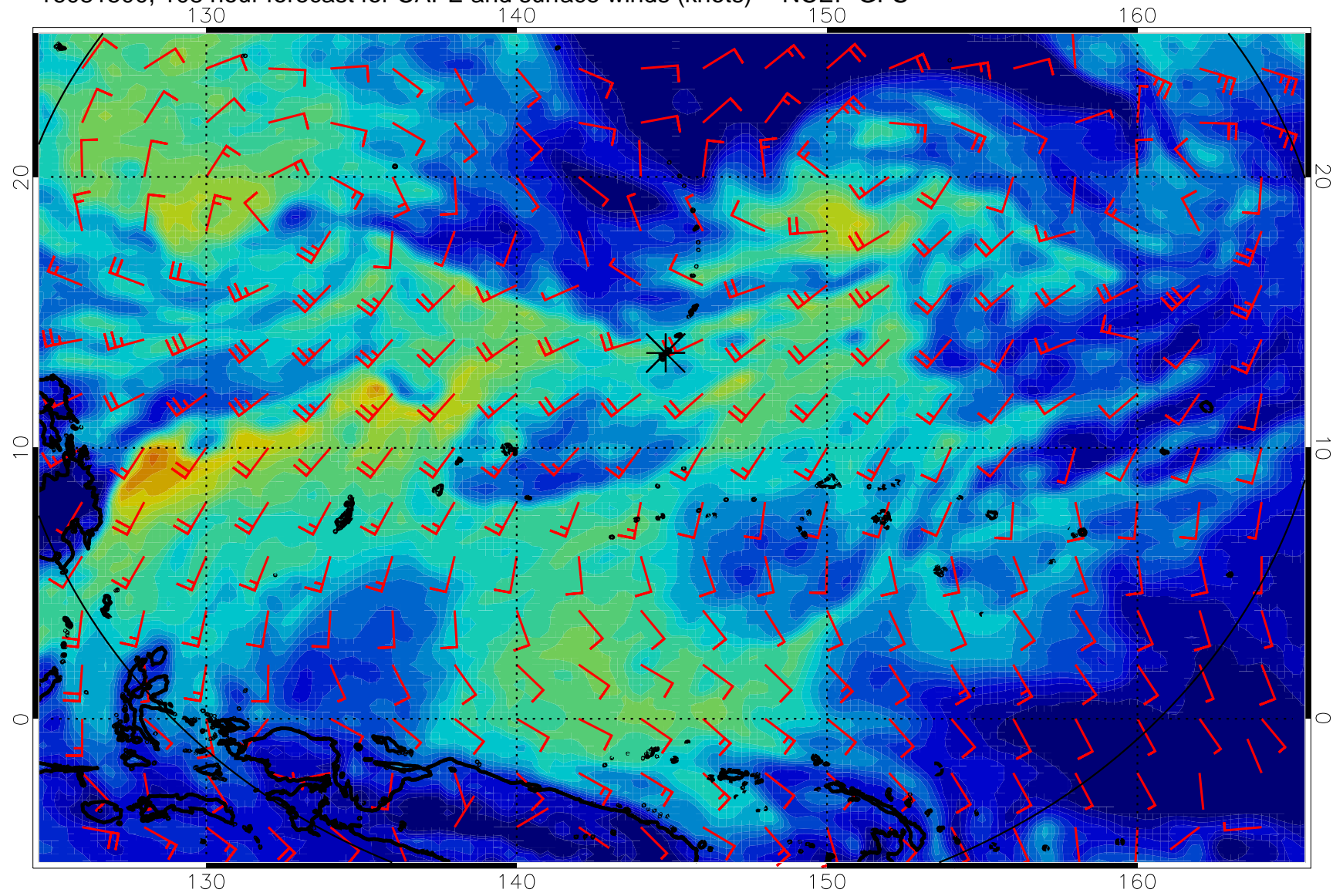
16081500, 108 hour forecast for CAPE and surface winds (knots) -- NCEP GFS
