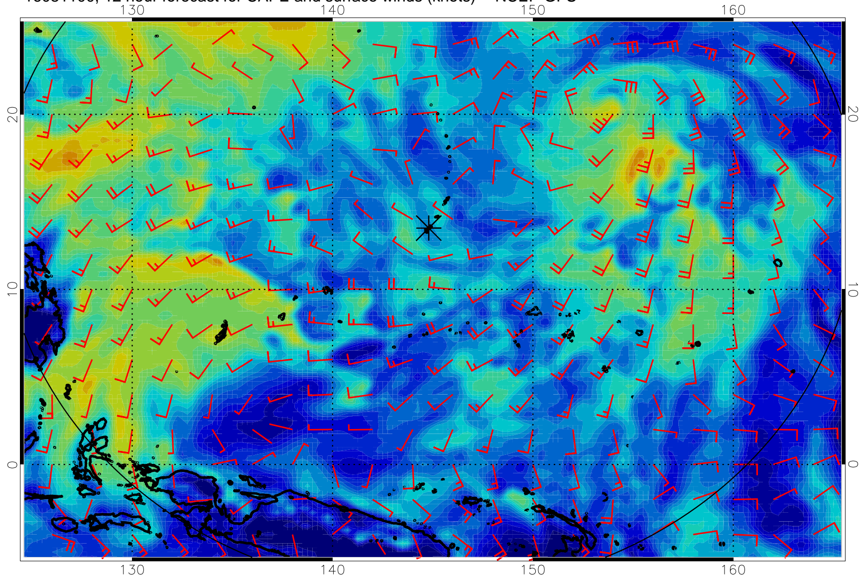
16081100, 12 hour forecast for CAPE and surface winds (knots) -- NCEP GFS
