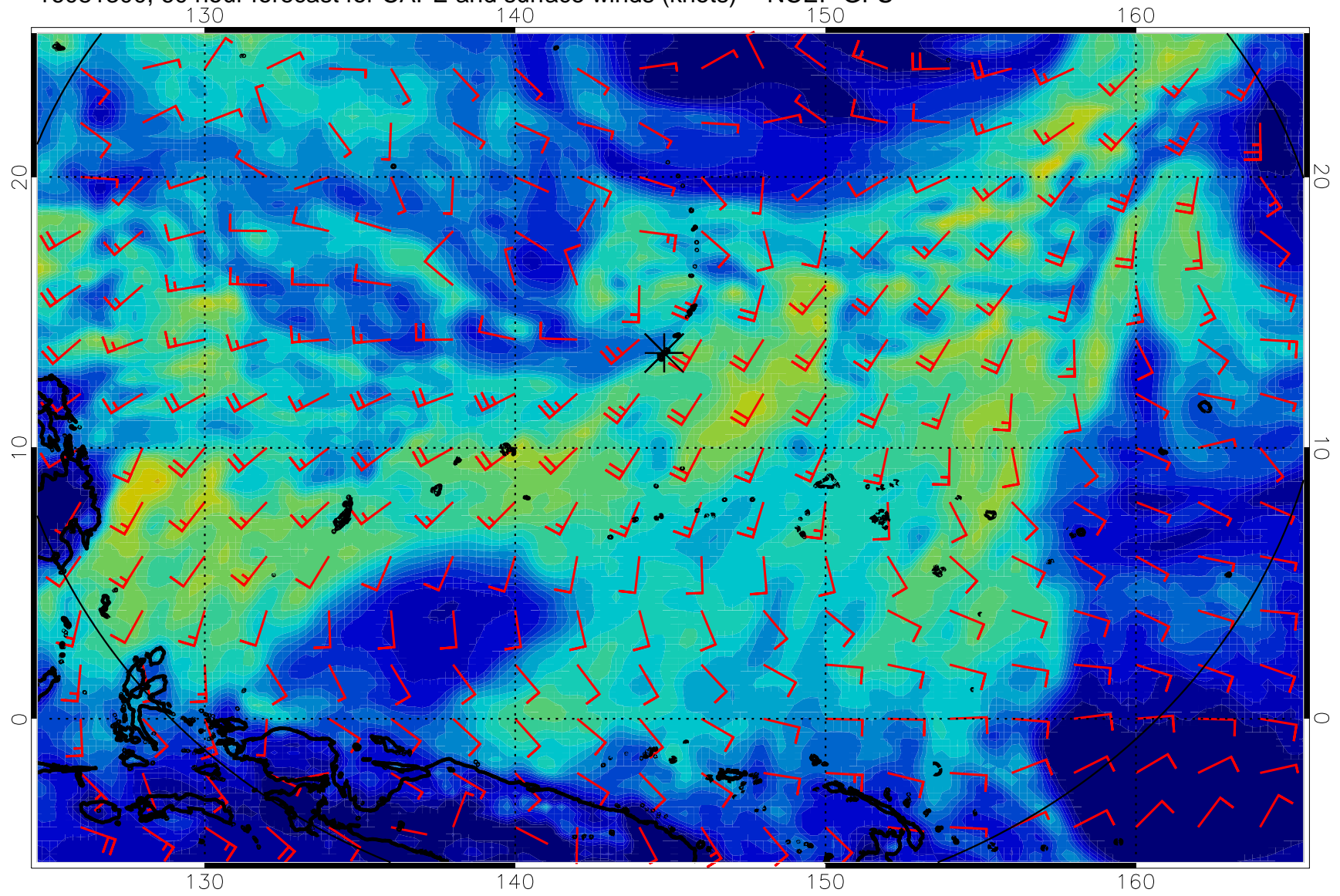
16081300, 60 hour forecast for CAPE and surface winds (knots) -- NCEP GFS
