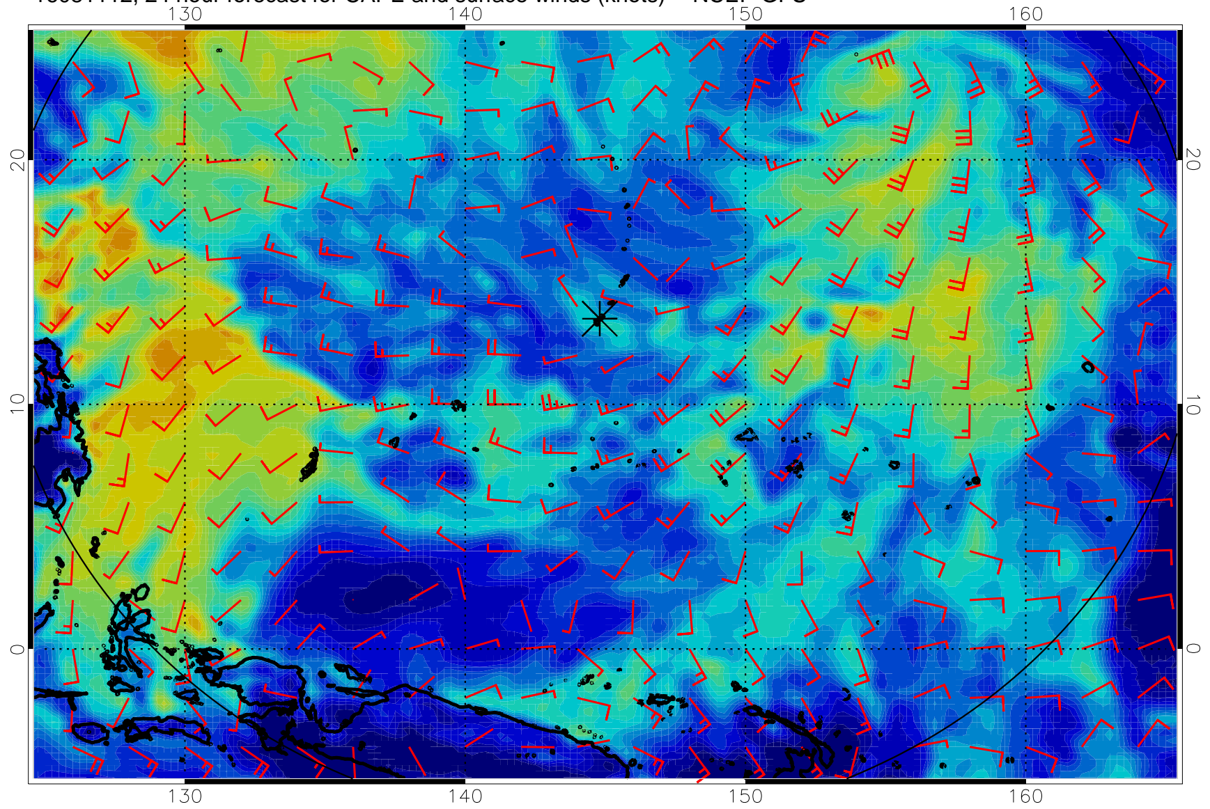
16081112, 24 hour forecast for CAPE and surface winds (knots) -- NCEP GFS
