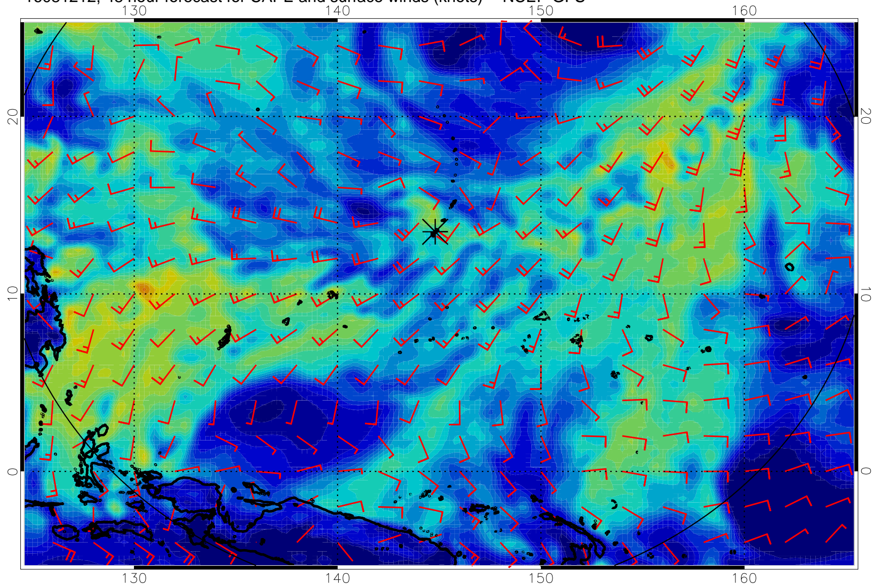
16081212, 48 hour forecast for CAPE and surface winds (knots) -- NCEP GFS
