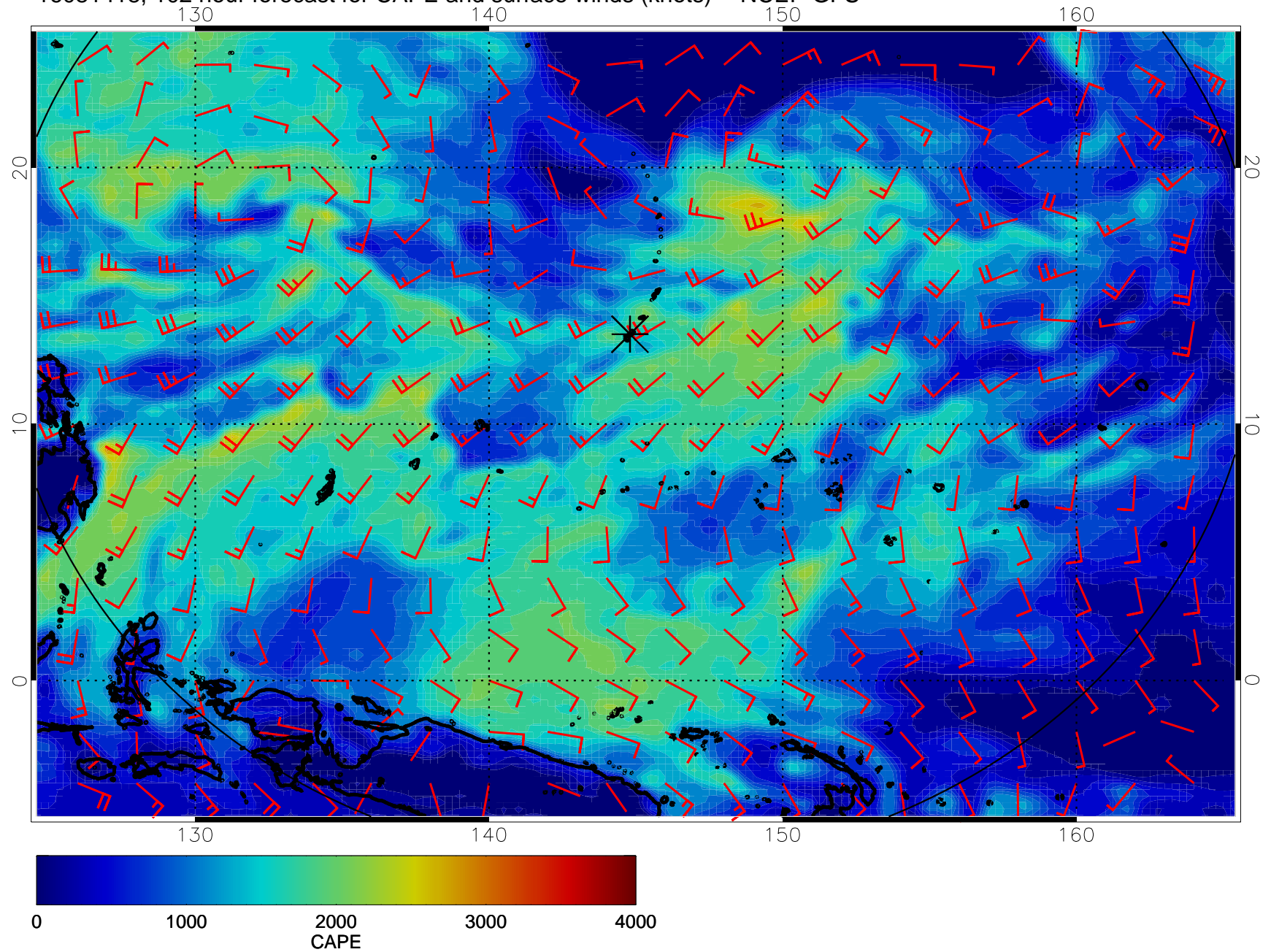
16081418, 102 hour forecast for CAPE and surface winds (knots) -- NCEP GFS
