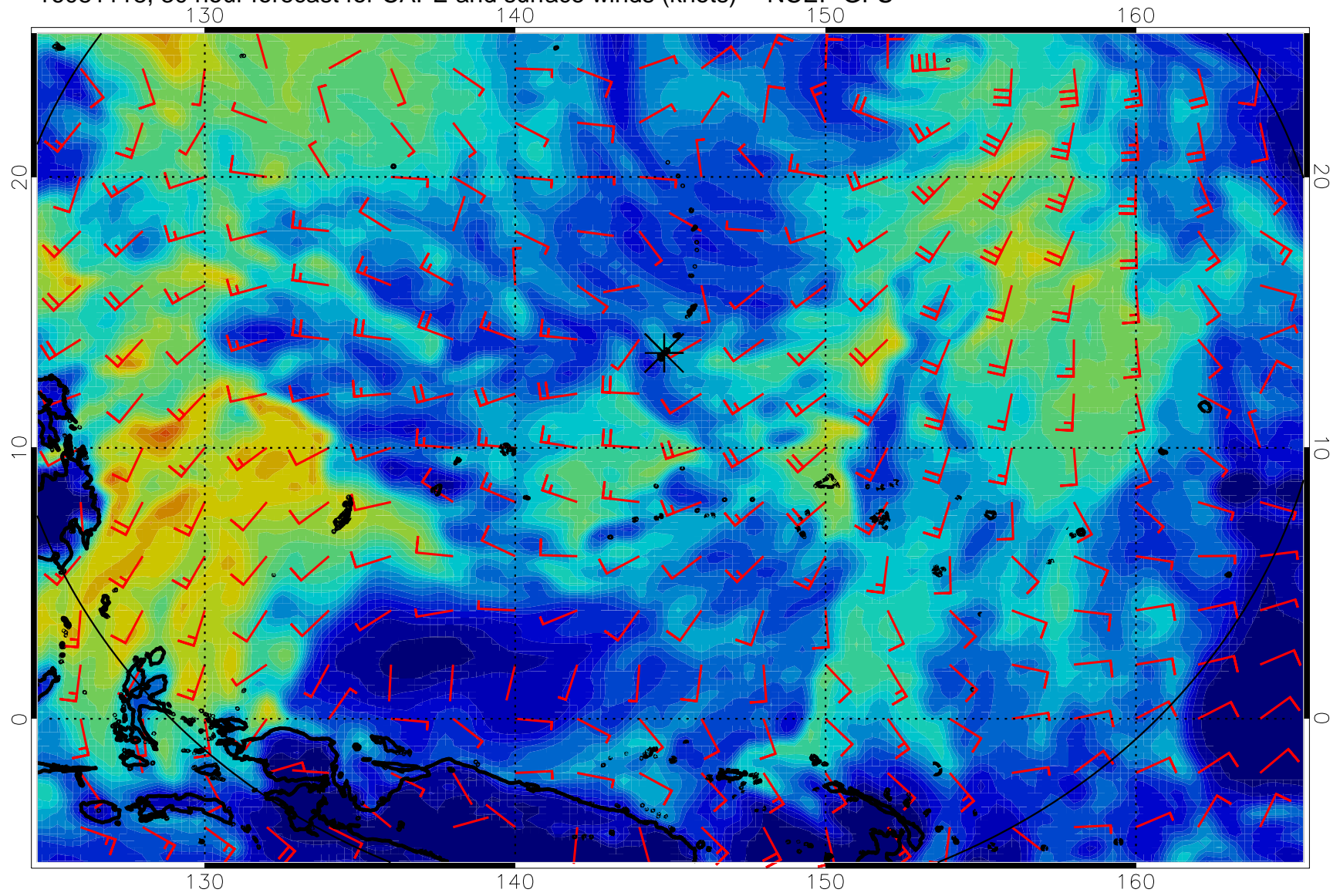
16081118, 30 hour forecast for CAPE and surface winds (knots) -- NCEP GFS
