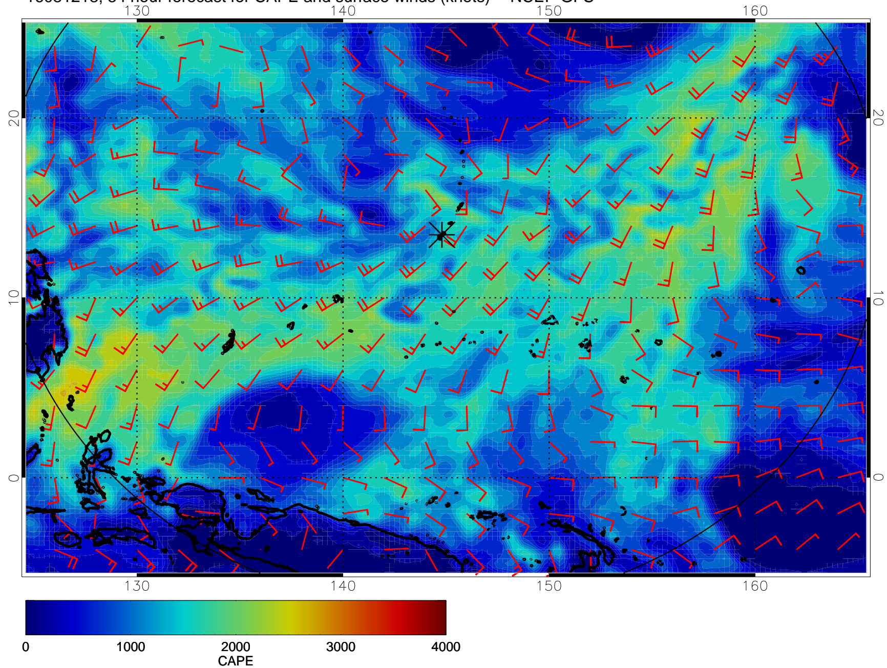
16081218, 54 hour forecast for CAPE and surface winds (knots) -- NCEP GFS
