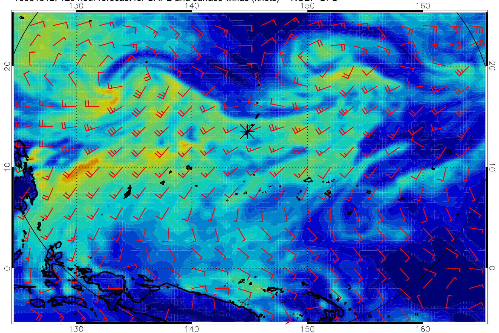
16081512, 120 hour forecast for CAPE and surface winds (knots) -- NCEP GFS
