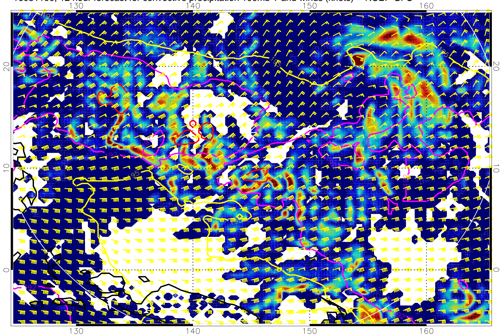
16081100, 12 hour forecast for convective precipitation 100mb T and winds (knots) -- NCEP GFS
