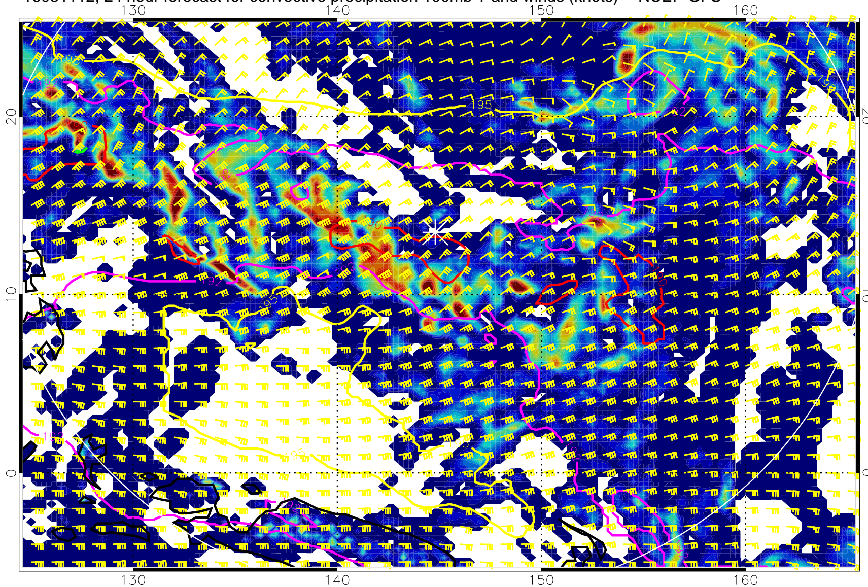
16081112, 24 hour forecast for convective precipitation 100mb T and winds (knots) -- NCEP GFS
