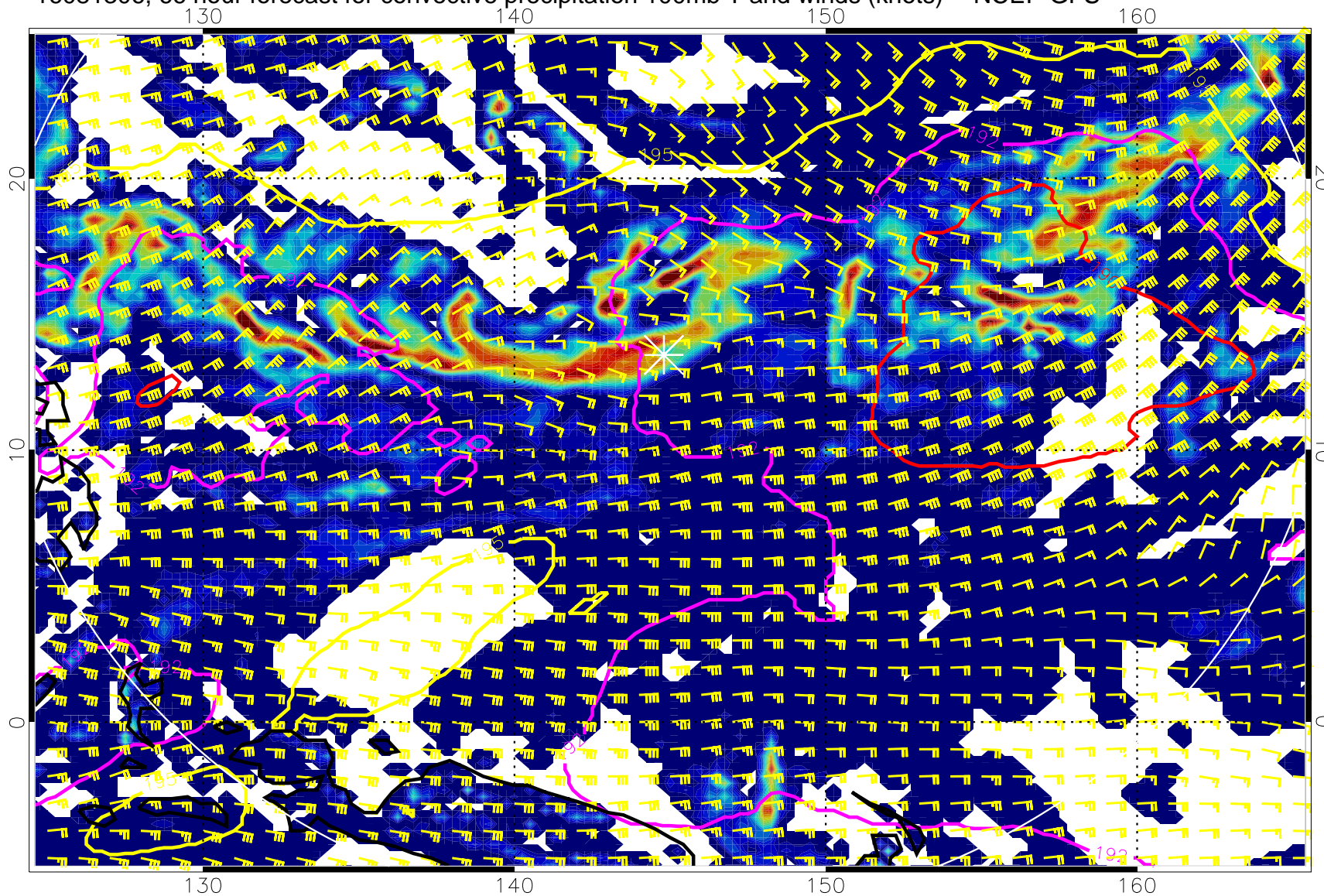
16081306, 66 hour forecast for convective precipitation 100mb T and winds (knots) -- NCEP GFS
