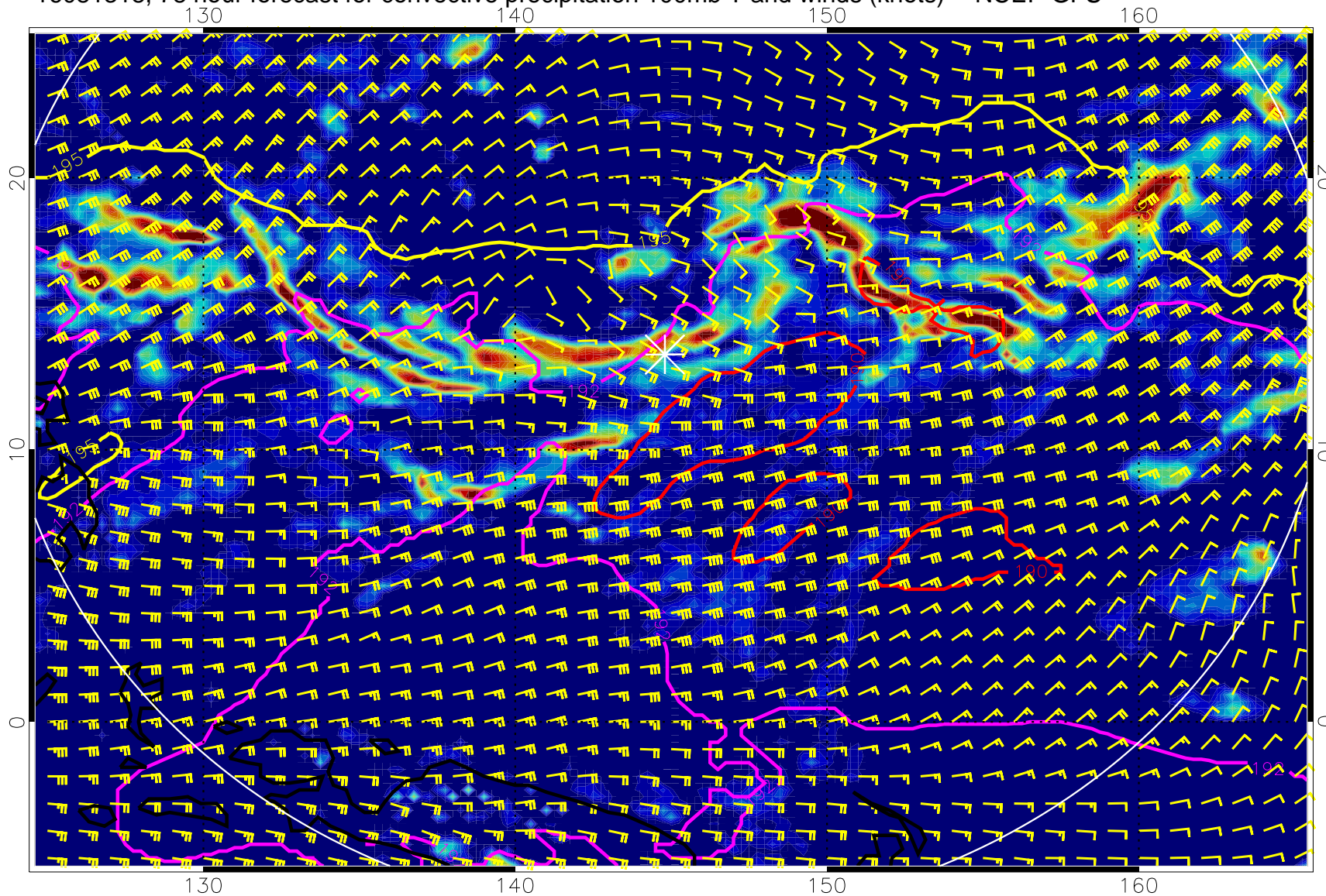
16081318, 78 hour forecast for convective precipitation 100mb T and winds (knots) -- NCEP GFS
