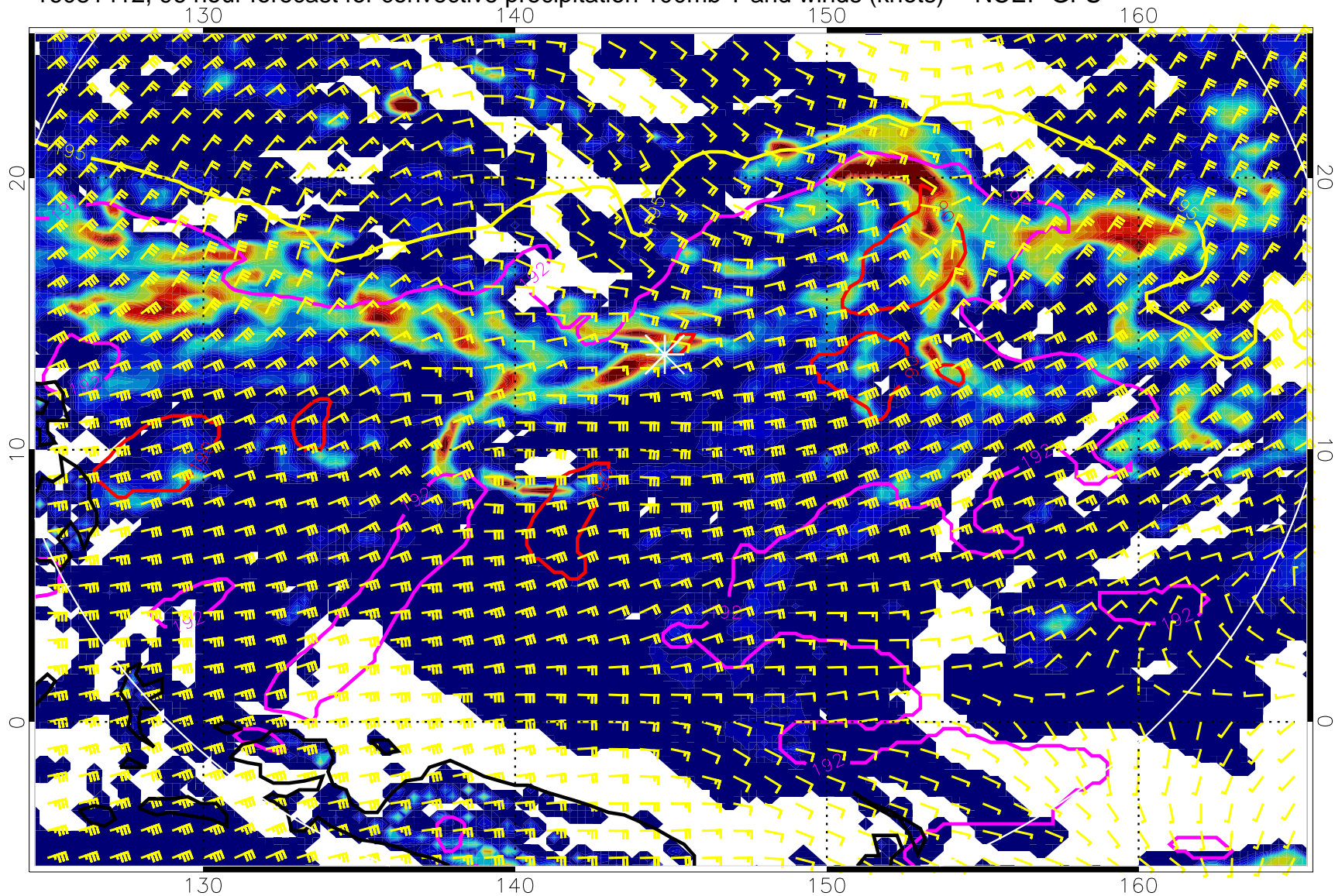
16081412, 96 hour forecast for convective precipitation 100mb T and winds (knots) -- NCEP GFS
