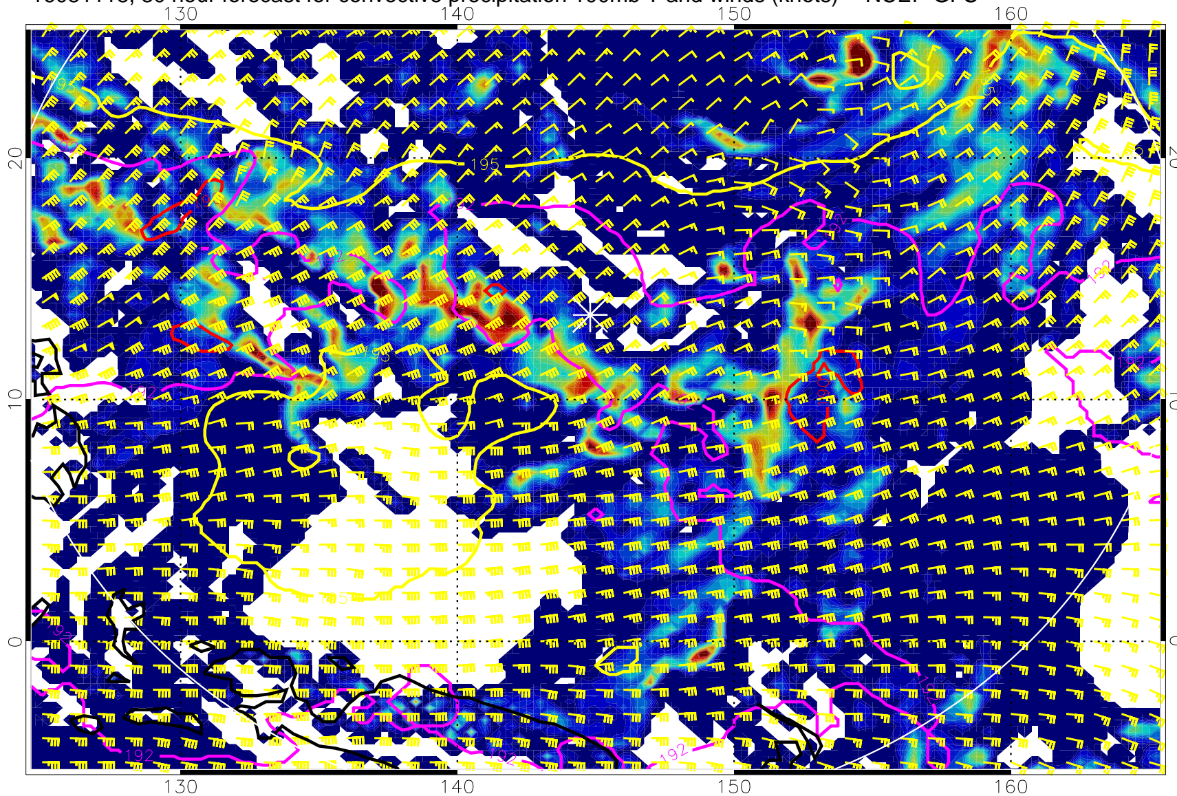
16081118, 30 hour forecast for convective precipitation 100mb T and winds (knots) -- NCEP GFS
