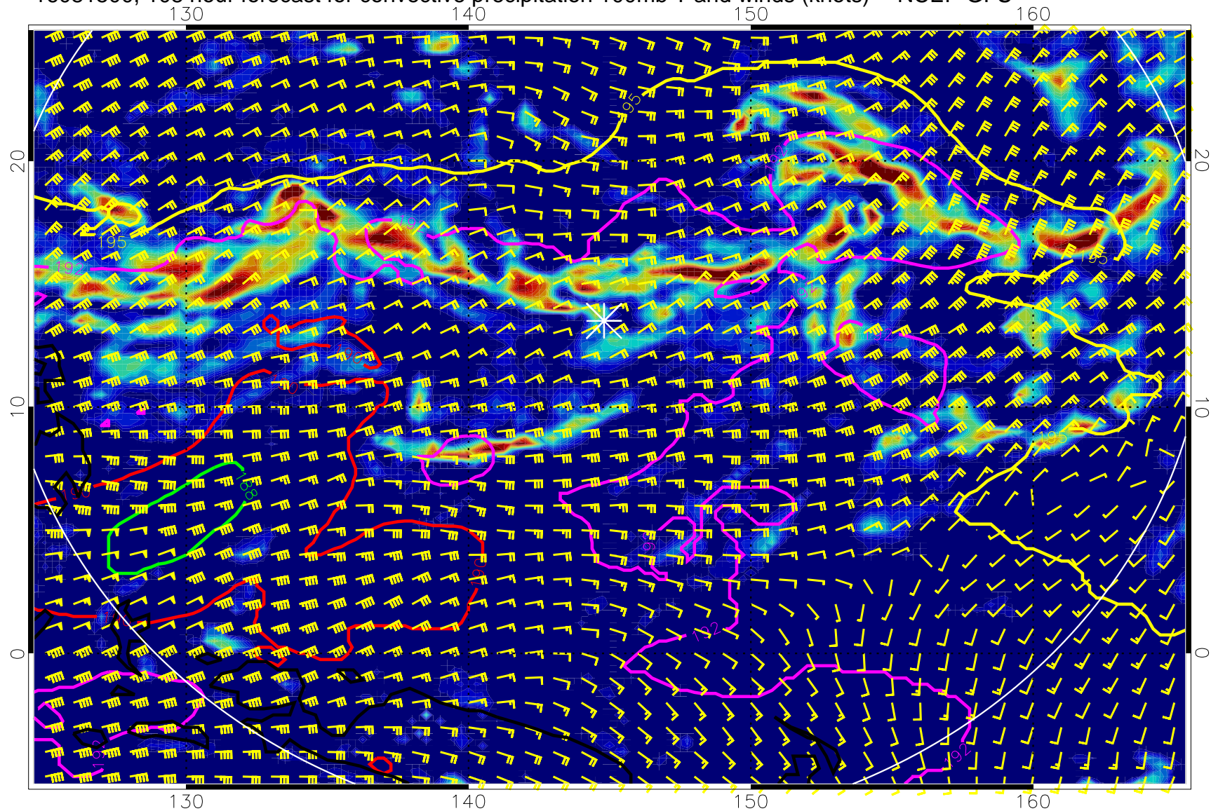
16081500, 108 hour forecast for convective precipitation 100mb T and winds (knots) -- NCEP GFS
