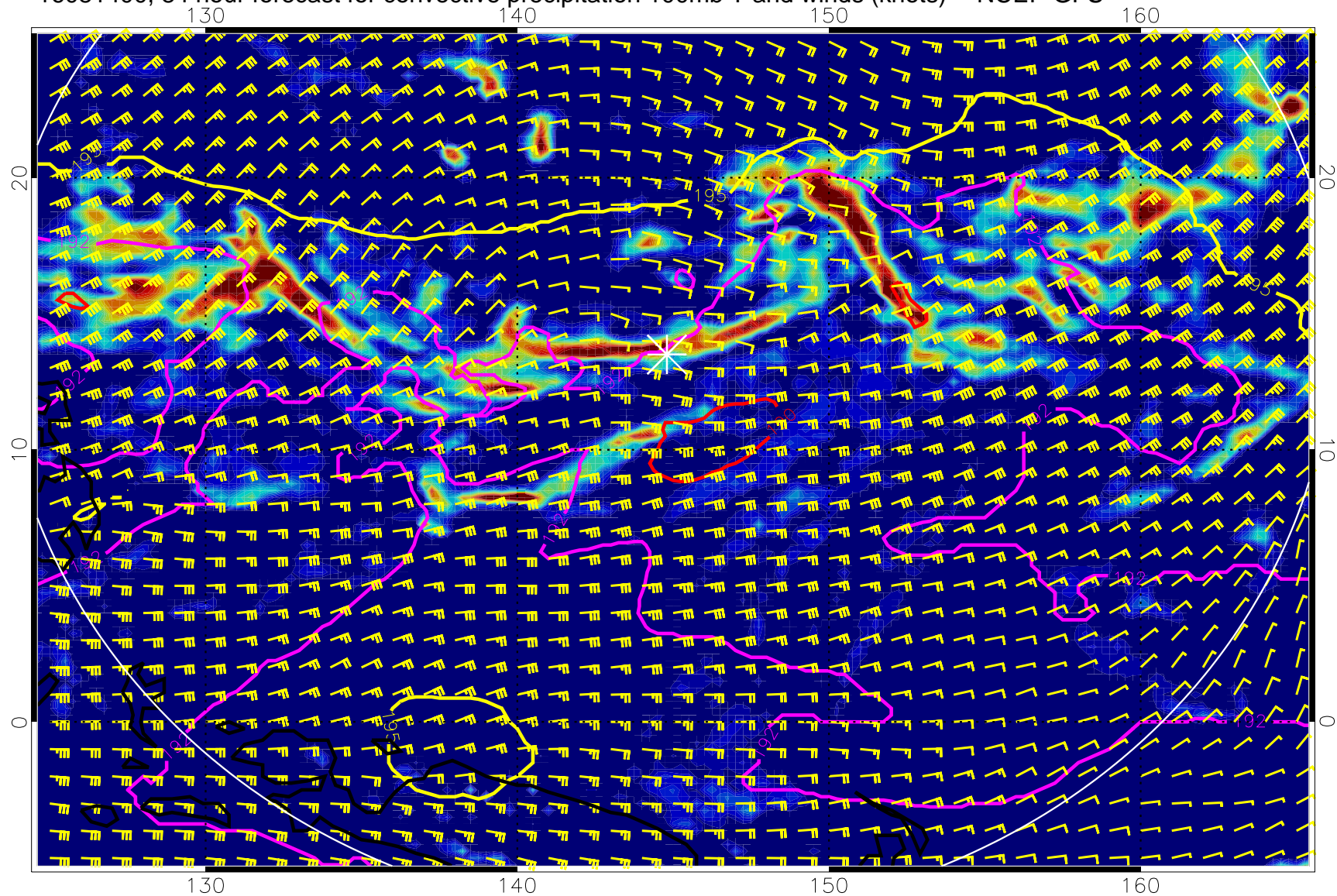
16081400, 84 hour forecast for convective precipitation 100mb T and winds (knots) -- NCEP GFS
