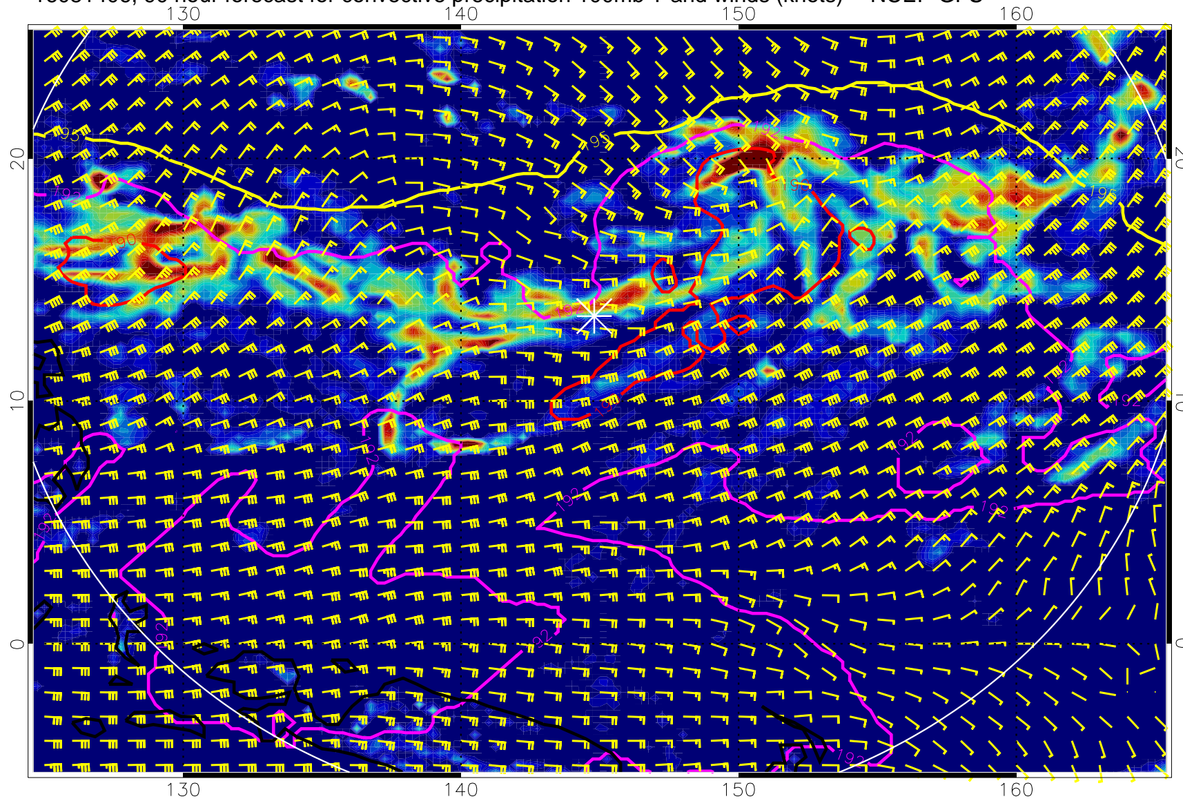
16081406, 90 hour forecast for convective precipitation 100mb T and winds (knots) -- NCEP GFS
