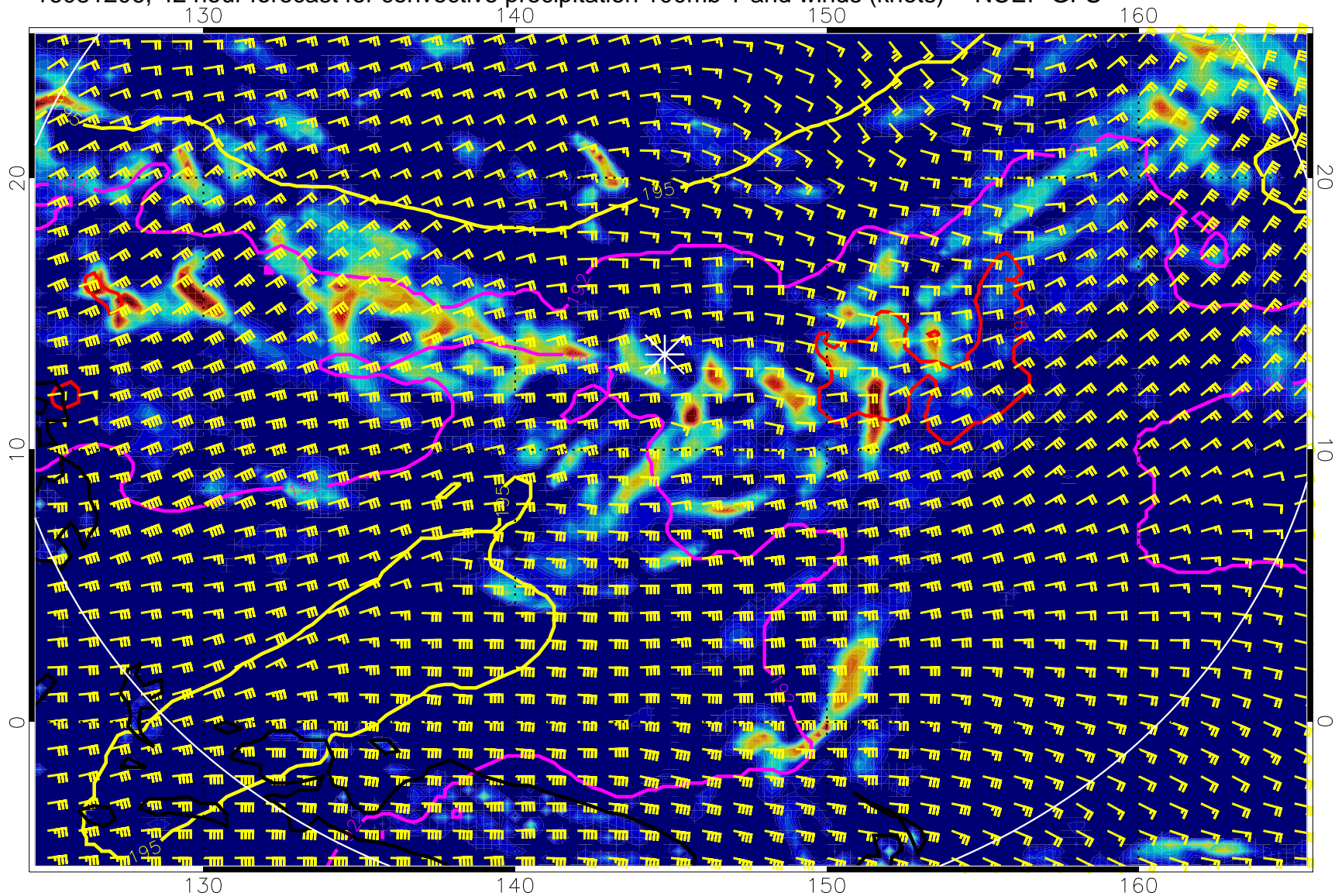
16081206, 42 hour forecast for convective precipitation 100mb T and winds (knots) -- NCEP GFS
