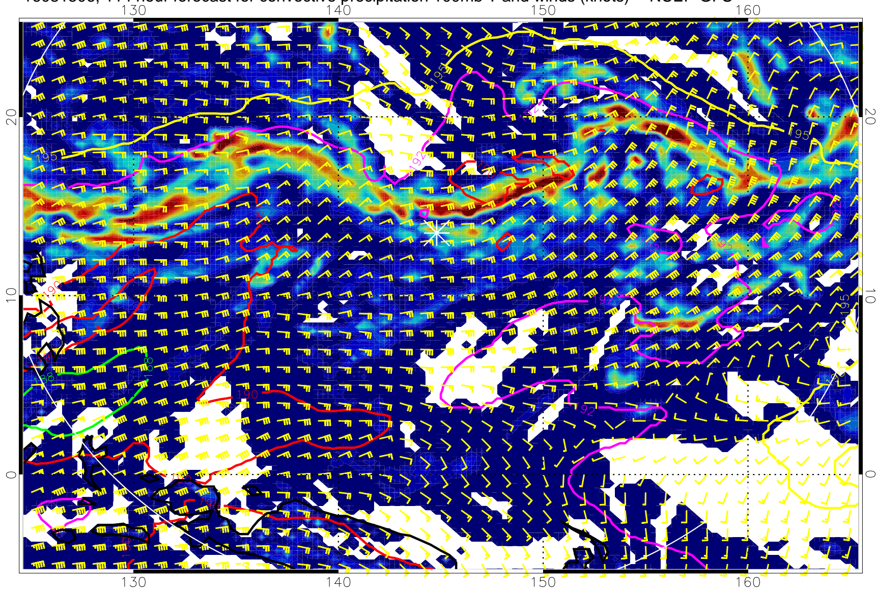
16081506, 114 hour forecast for convective precipitation 100mb T and winds (knots) -- NCEP GFS
