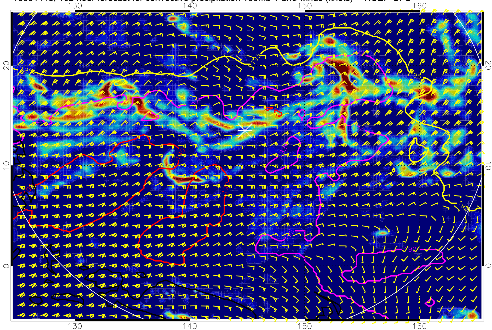
16081418, 102 hour forecast for convective precipitation 100mb T and winds (knots) -- NCEP GFS
