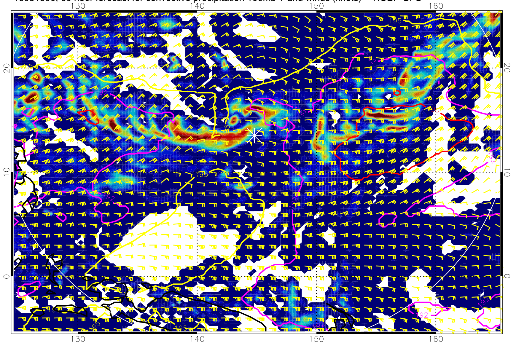
16081300, 60 hour forecast for convective precipitation 100mb T and winds (knots) -- NCEP GFS
