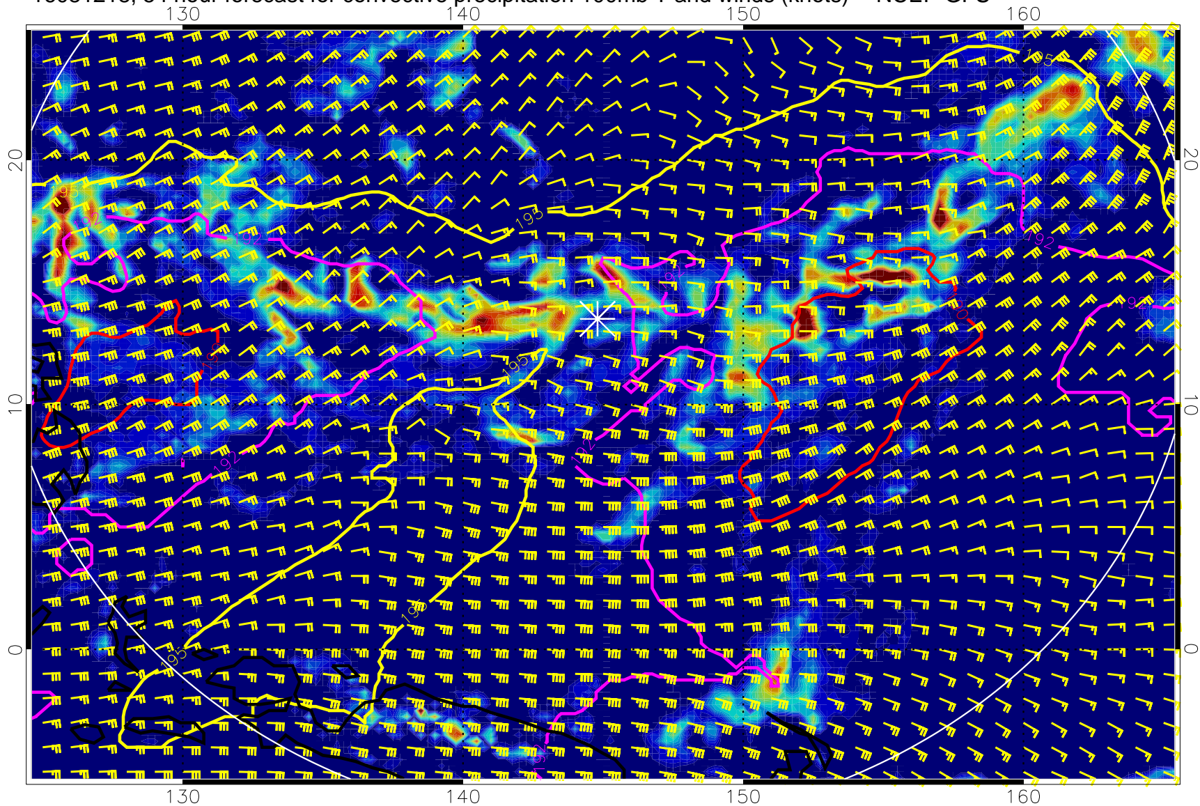
16081218, 54 hour forecast for convective precipitation 100mb T and winds (knots) -- NCEP GFS
