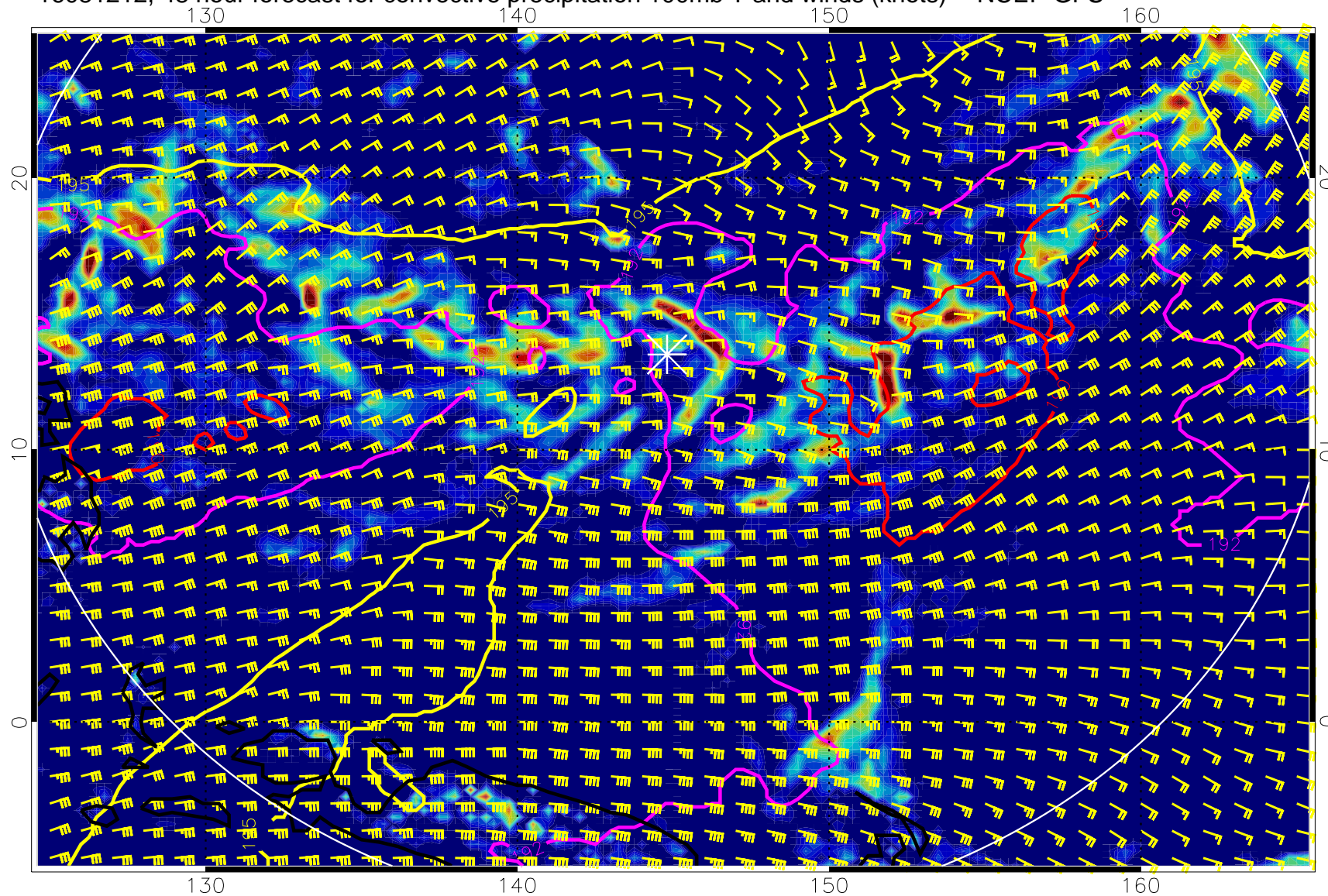
16081212, 48 hour forecast for convective precipitation 100mb T and winds (knots) -- NCEP GFS
