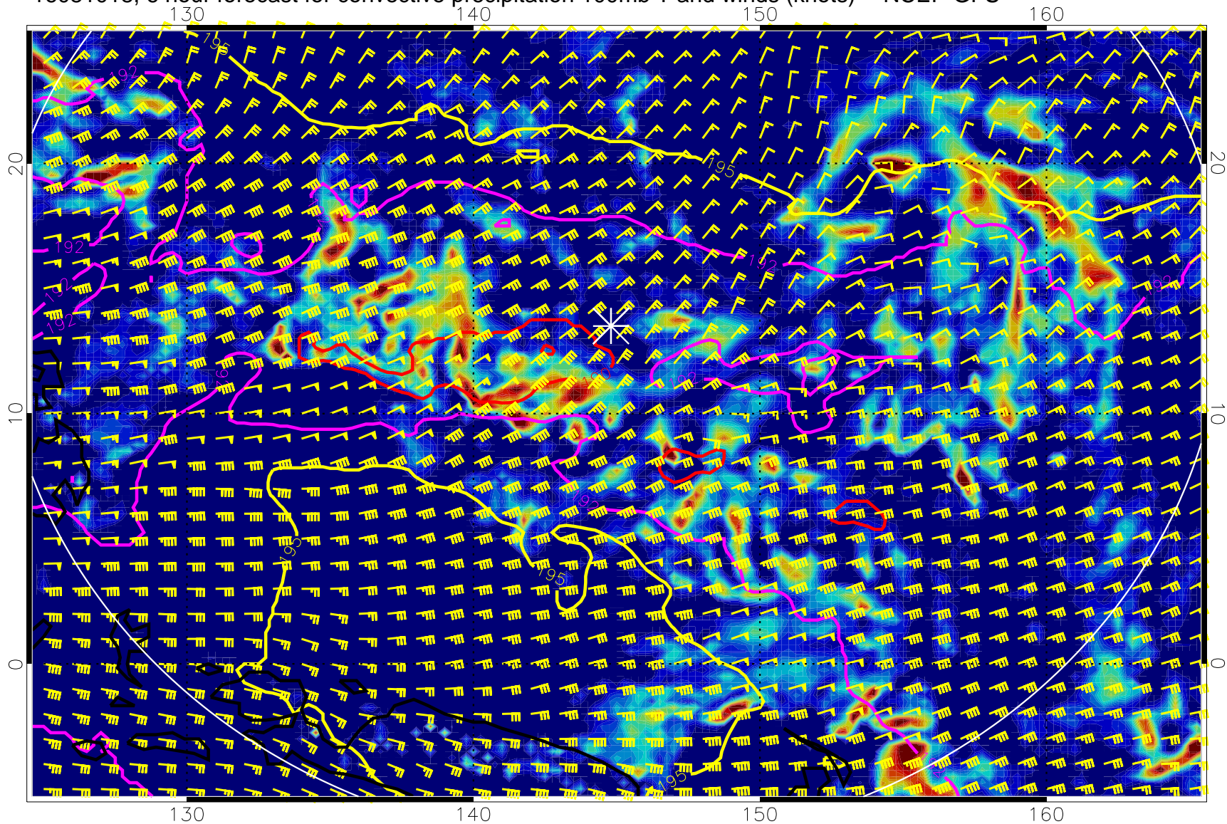
16081018, 6 hour forecast for convective precipitation 100mb T and winds (knots) -- NCEP GFS
