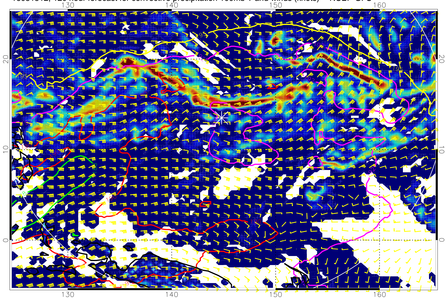
16081512, 120 hour forecast for convective precipitation 100mb T and winds (knots) -- NCEP GFS
