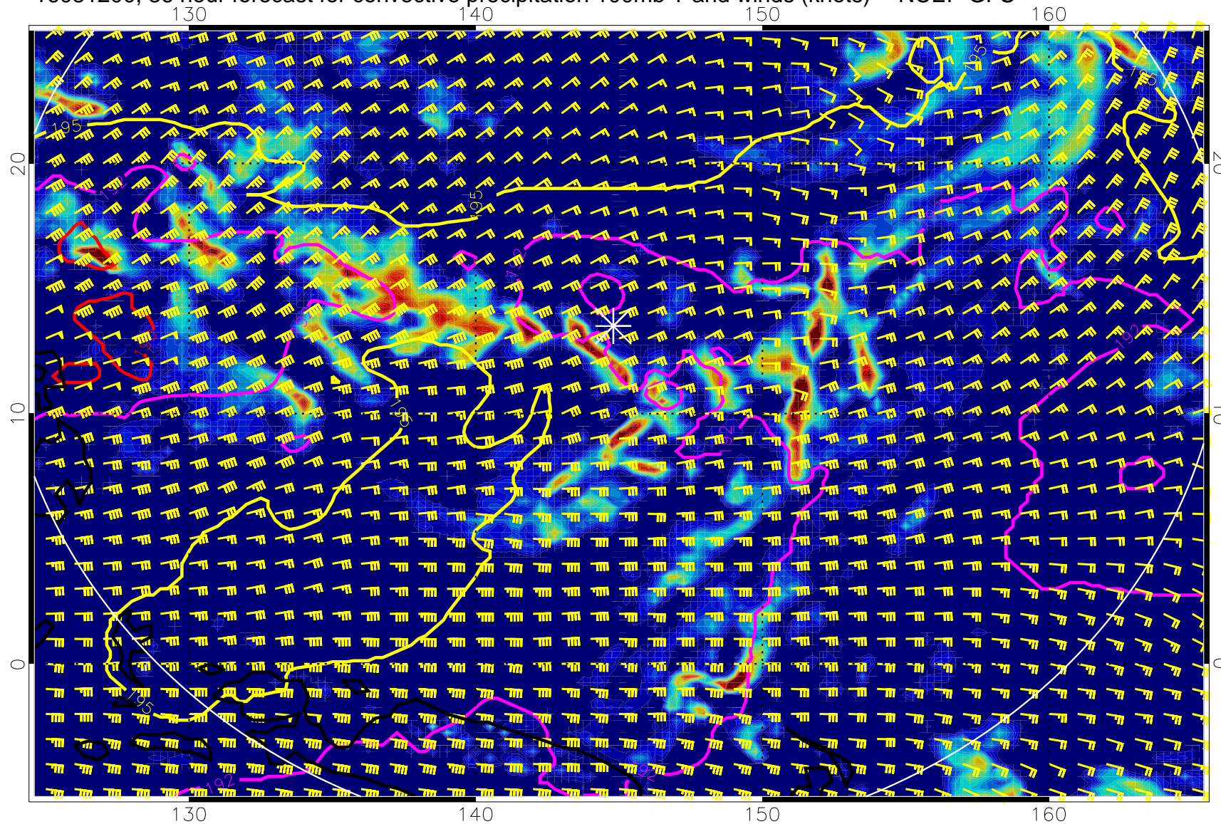
16081200, 36 hour forecast for convective precipitation 100mb T and winds (knots) -- NCEP GFS
