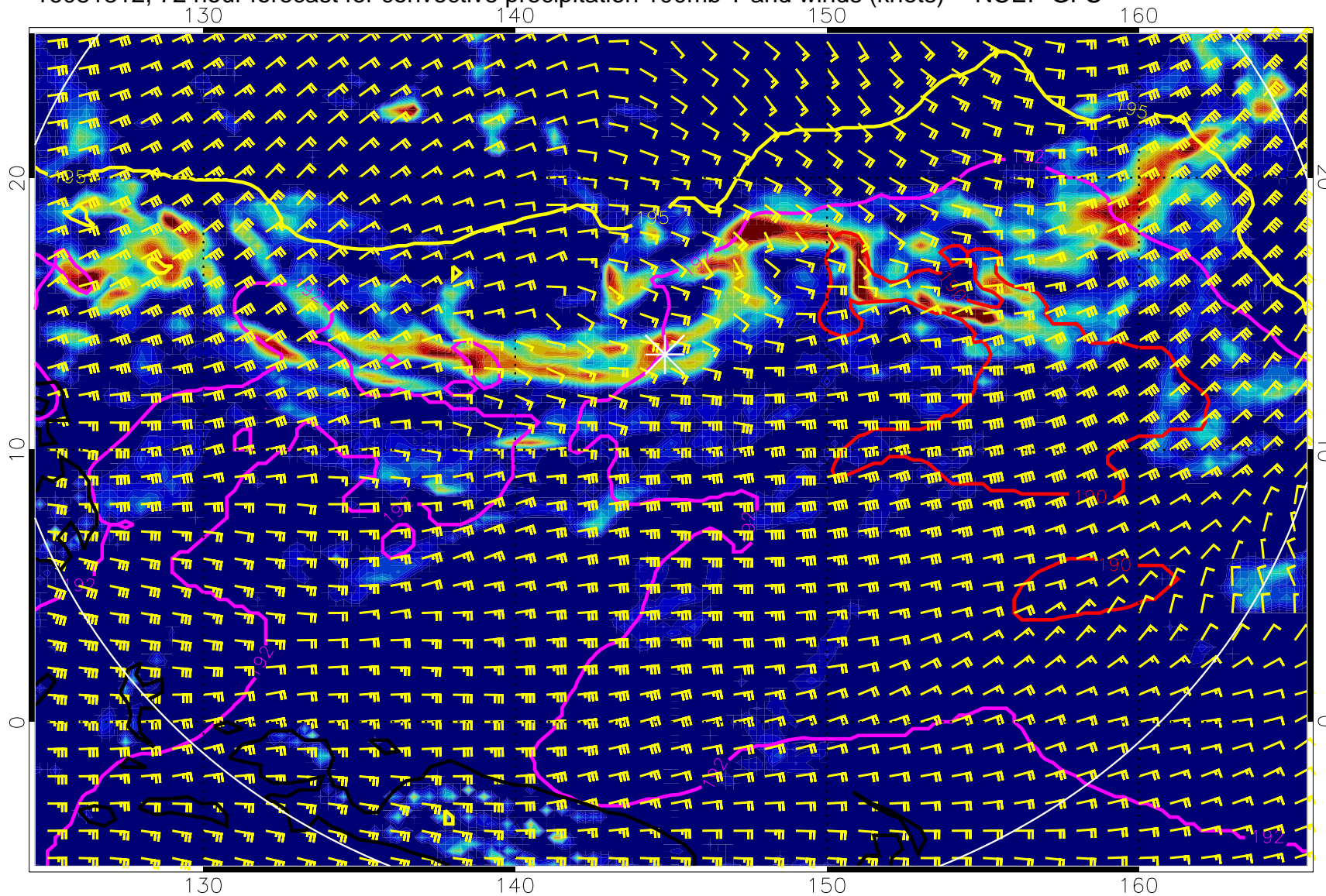
16081312, 72 hour forecast for convective precipitation 100mb T and winds (knots) -- NCEP GFS
