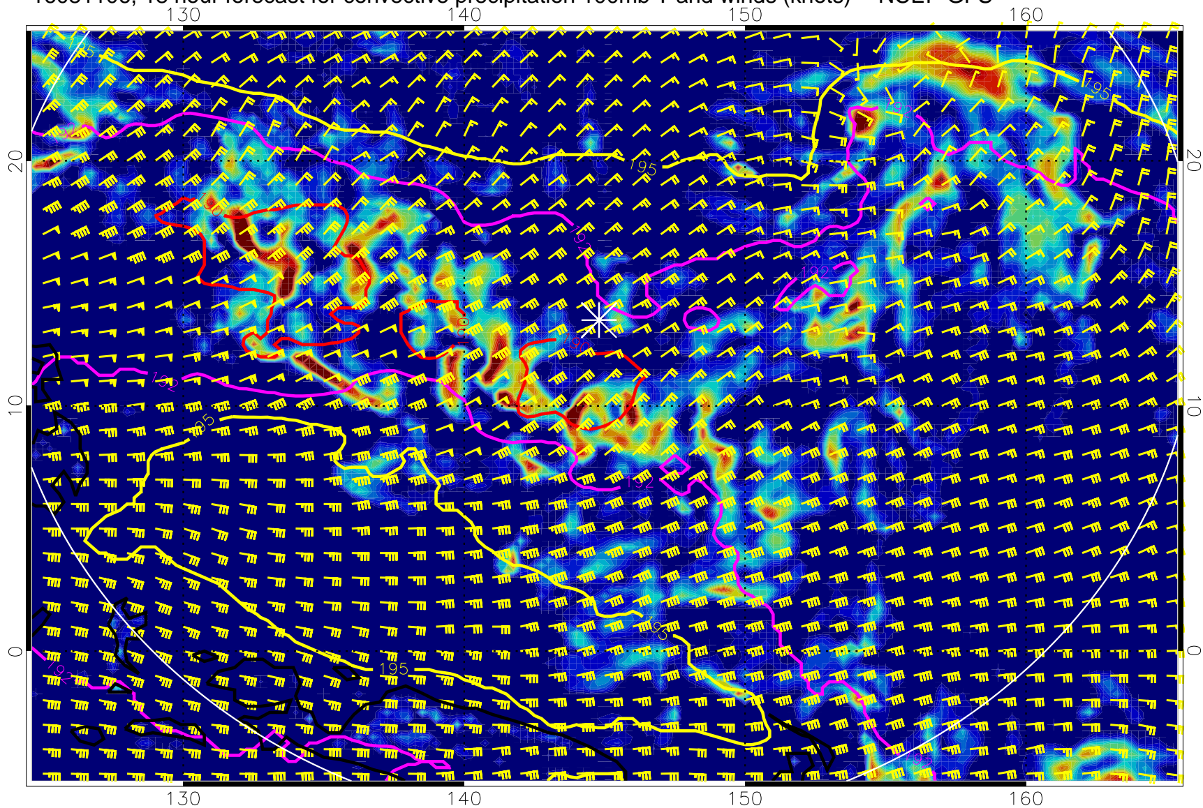
16081106, 18 hour forecast for convective precipitation 100mb T and winds (knots) -- NCEP GFS
