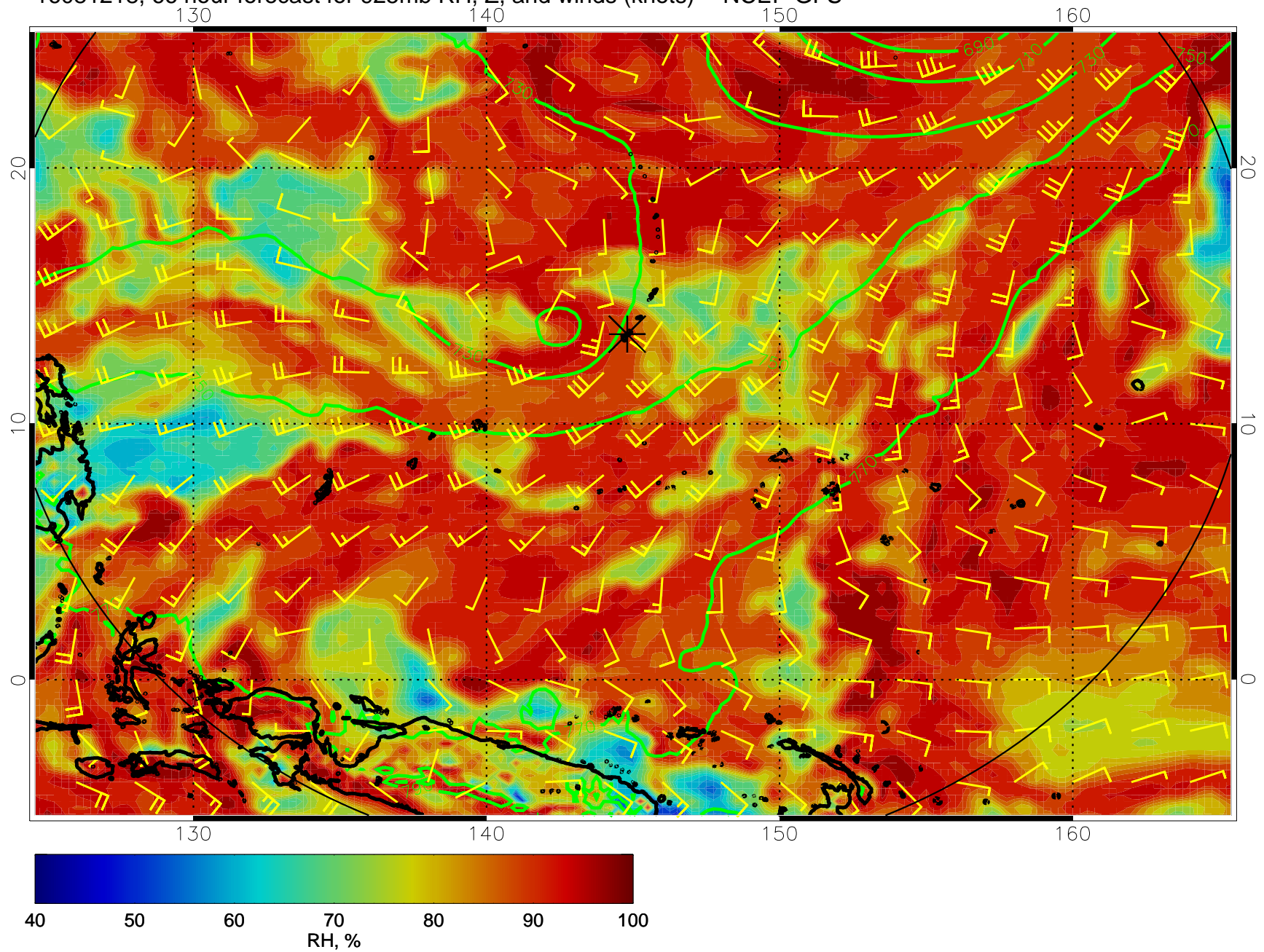
16081218, 66 hour forecast for 925mb RH, Z, and winds (knots) -- NCEP GFS
