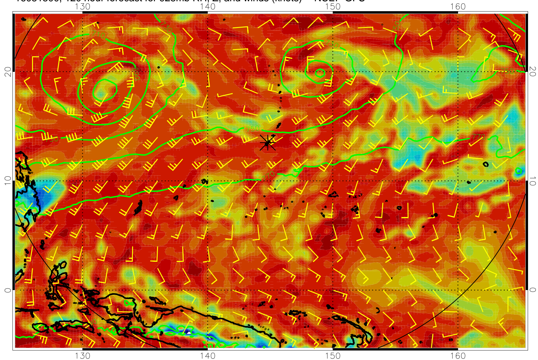
16081500, 120 hour forecast for 925mb RH, Z, and winds (knots) -- NCEP GFS
