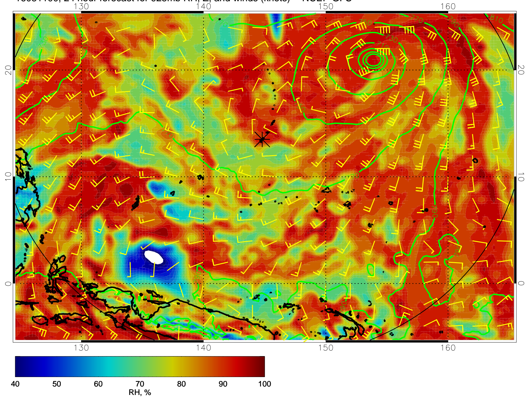
16081100, 24 hour forecast for 925mb RH, Z, and winds (knots) -- NCEP GFS
