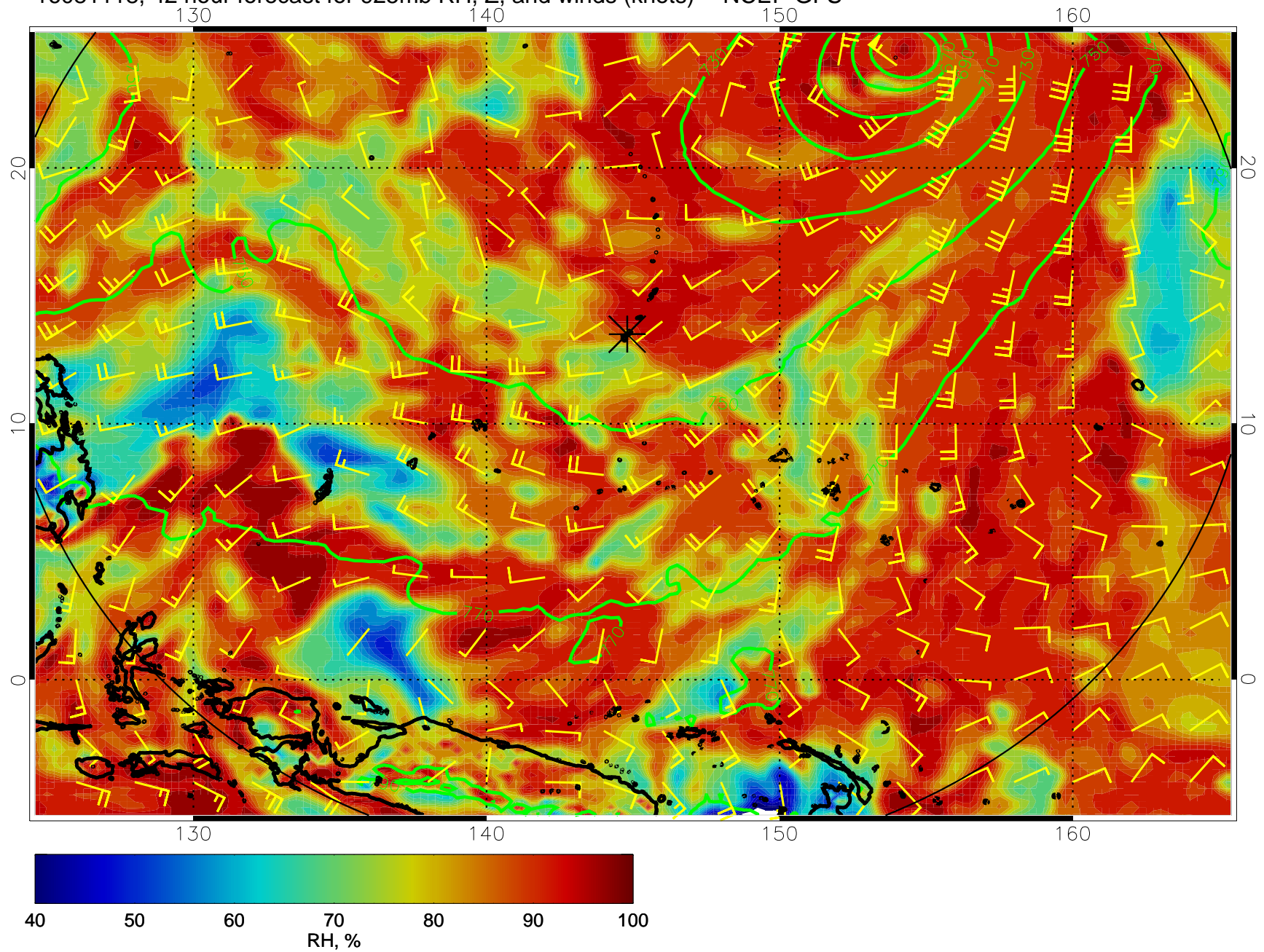
16081118, 42 hour forecast for 925mb RH, Z, and winds (knots) -- NCEP GFS
