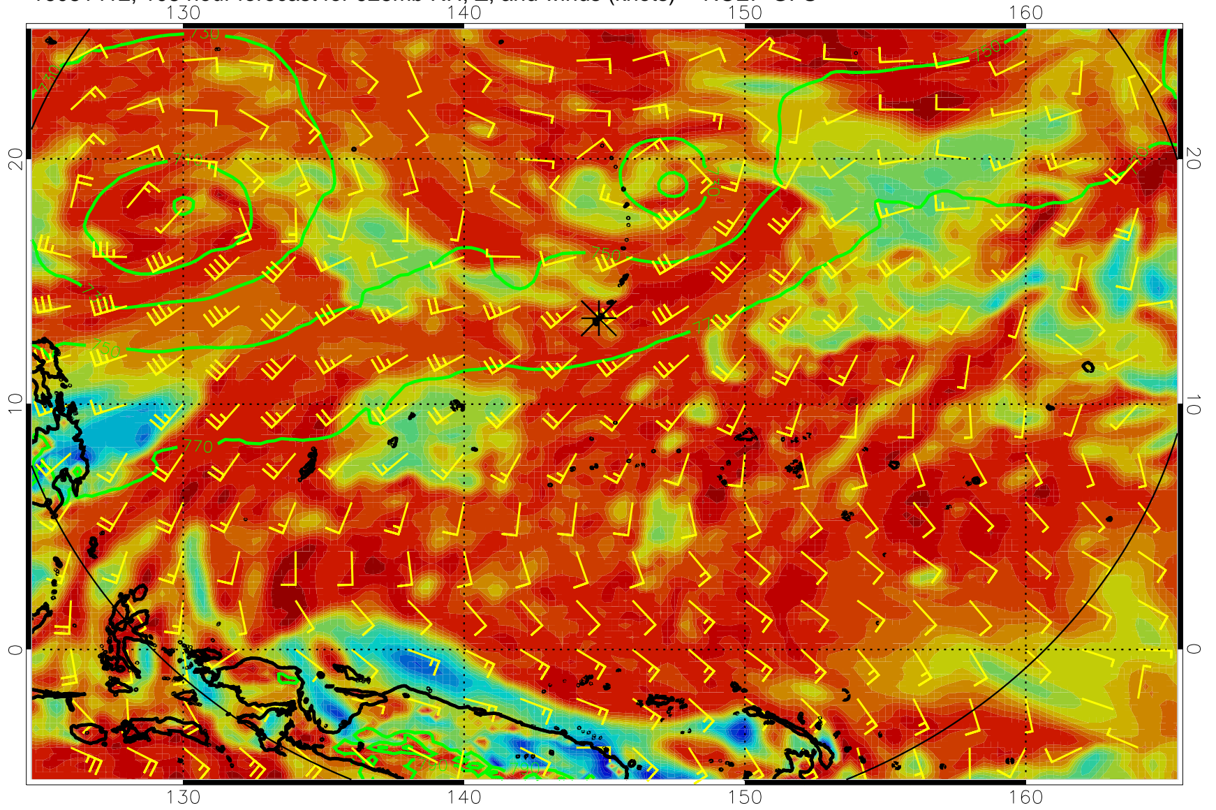
16081412, 108 hour forecast for 925mb RH, Z, and winds (knots) -- NCEP GFS
