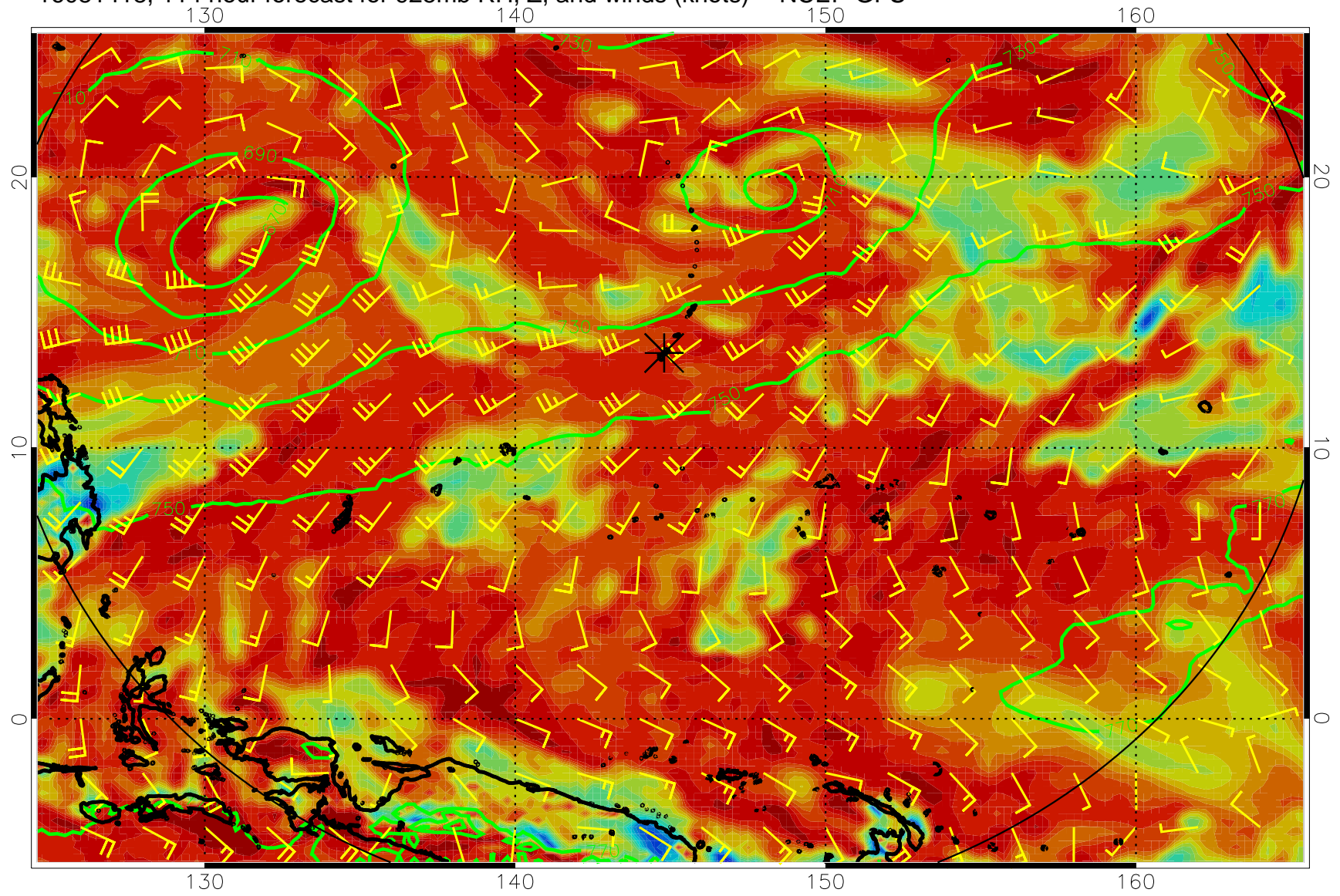
16081418, 114 hour forecast for 925mb RH, Z, and winds (knots) -- NCEP GFS
