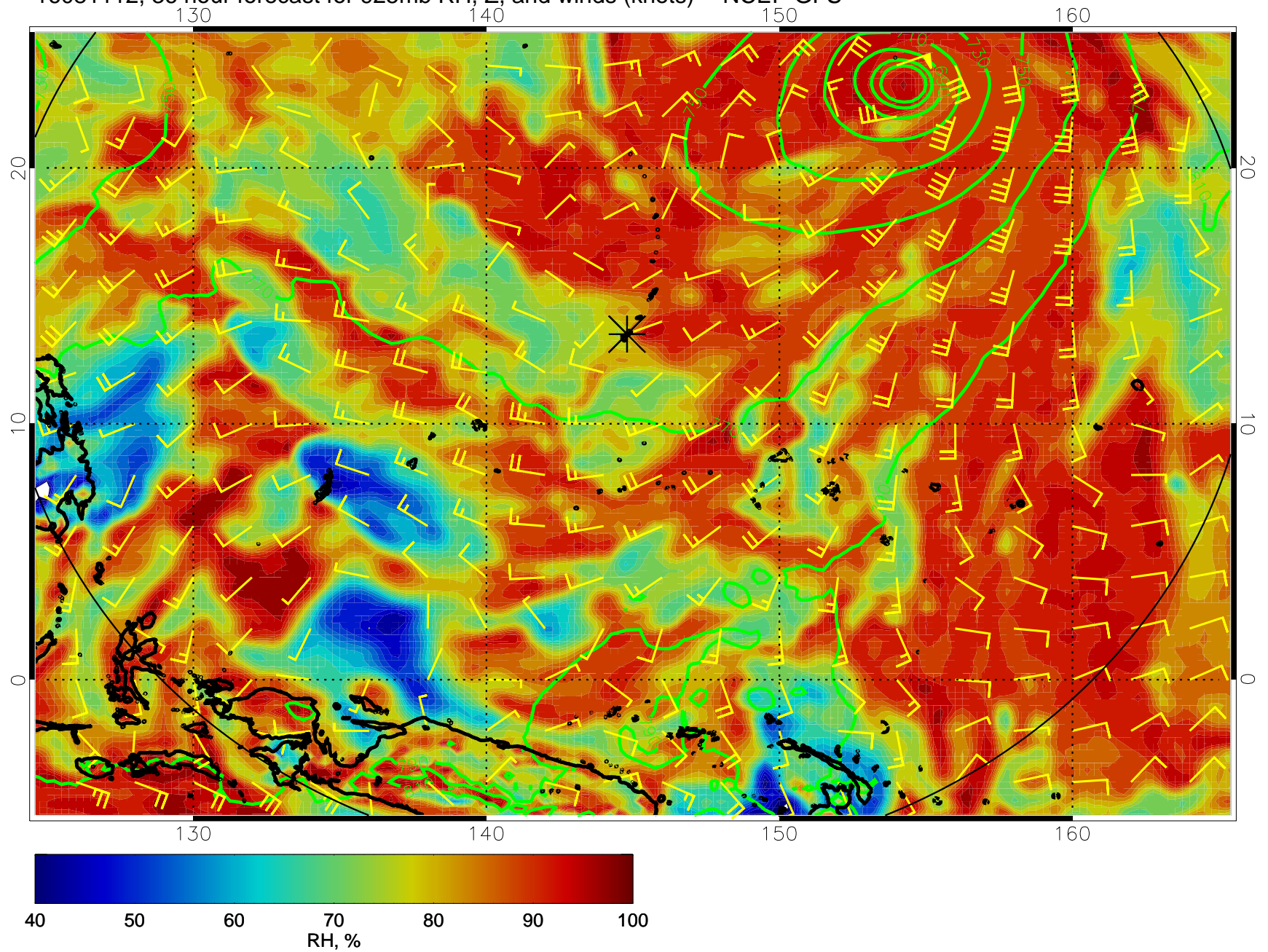
16081112, 36 hour forecast for 925mb RH, Z, and winds (knots) -- NCEP GFS
