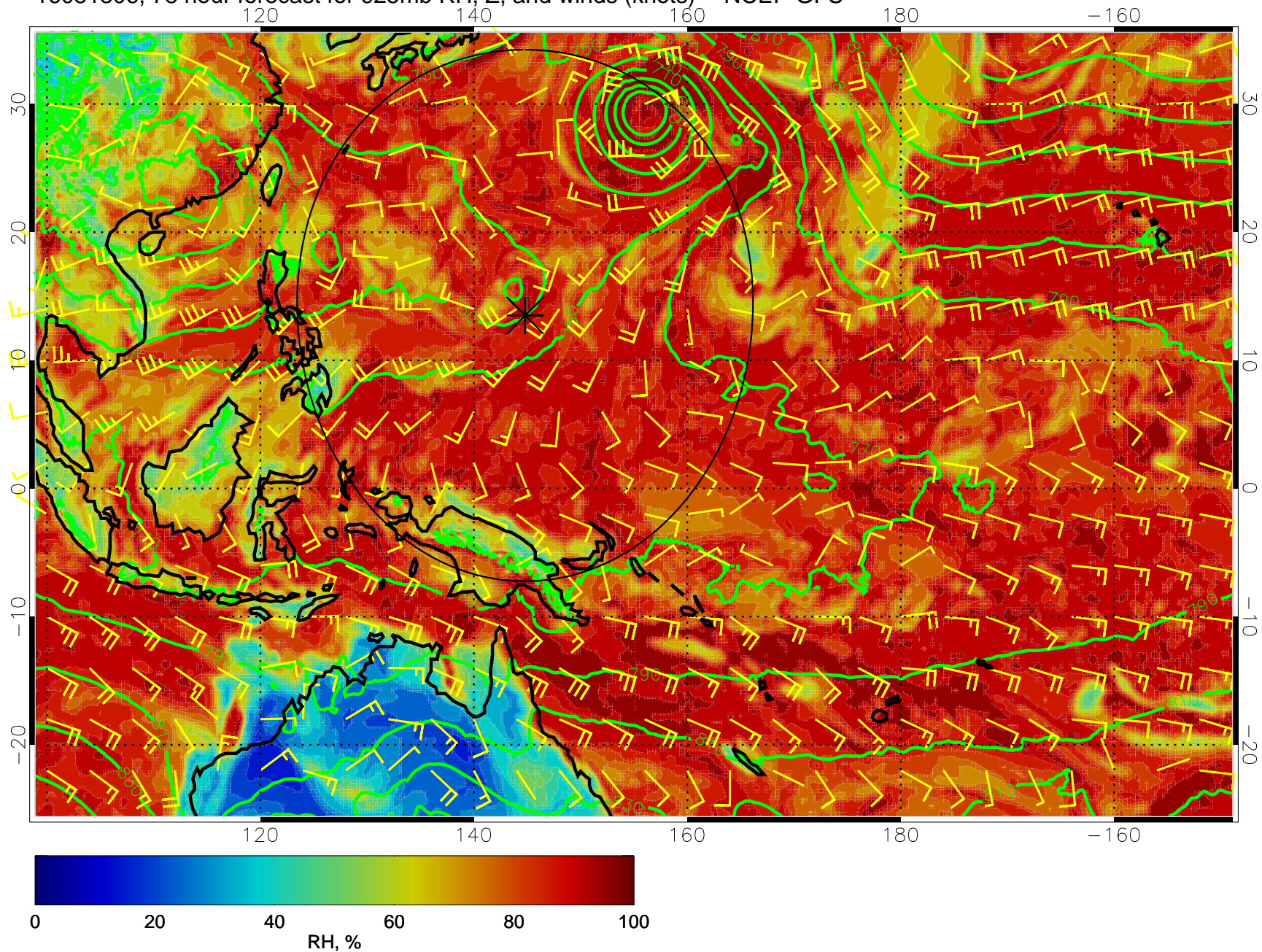
16081306, 78 hour forecast for 925mb RH, Z, and winds (knots) -- NCEP GFS
