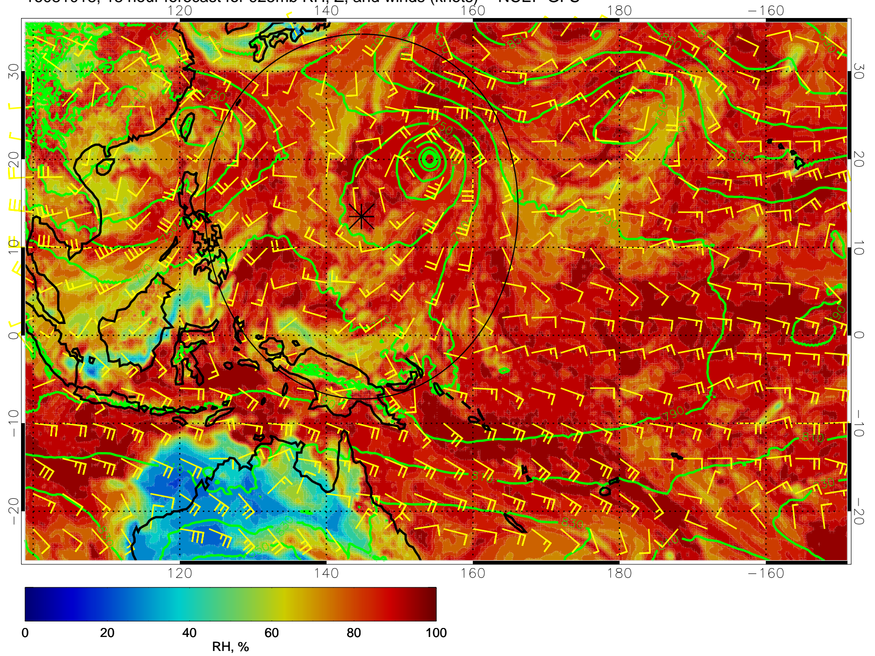
16081018, 18 hour forecast for 925mb RH, Z, and winds (knots) -- NCEP GFS
