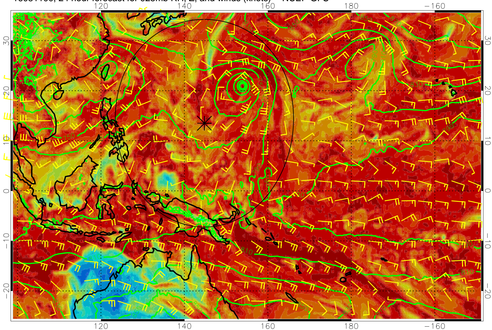
16081100, 24 hour forecast for 925mb RH, Z, and winds (knots) -- NCEP GFS
