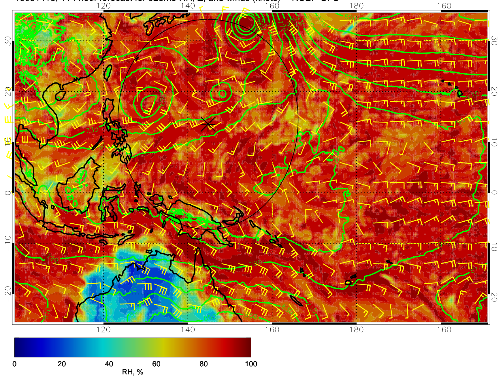
16081418, 114 hour forecast for 925mb RH, Z, and winds (knots) -- NCEP GFS
