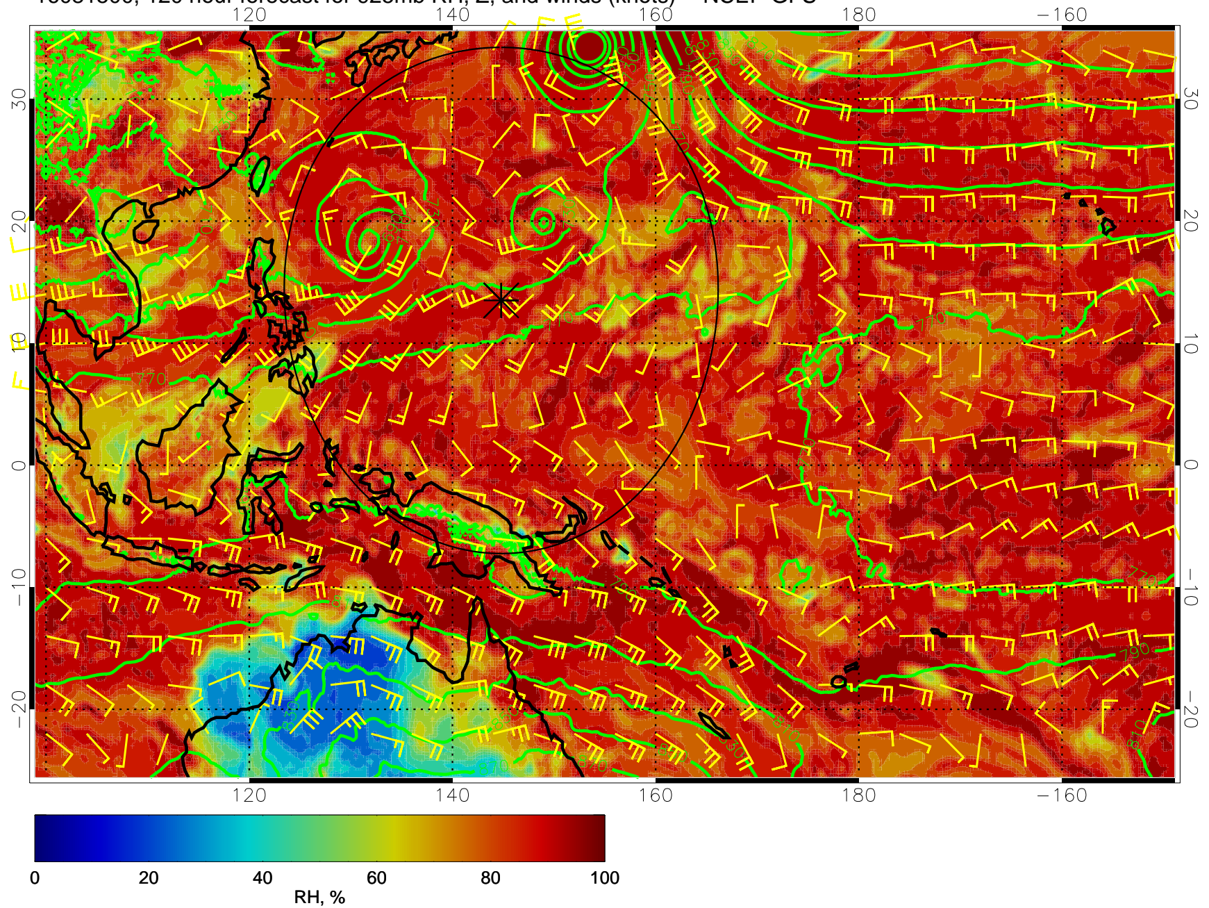
16081500, 120 hour forecast for 925mb RH, Z, and winds (knots) -- NCEP GFS
