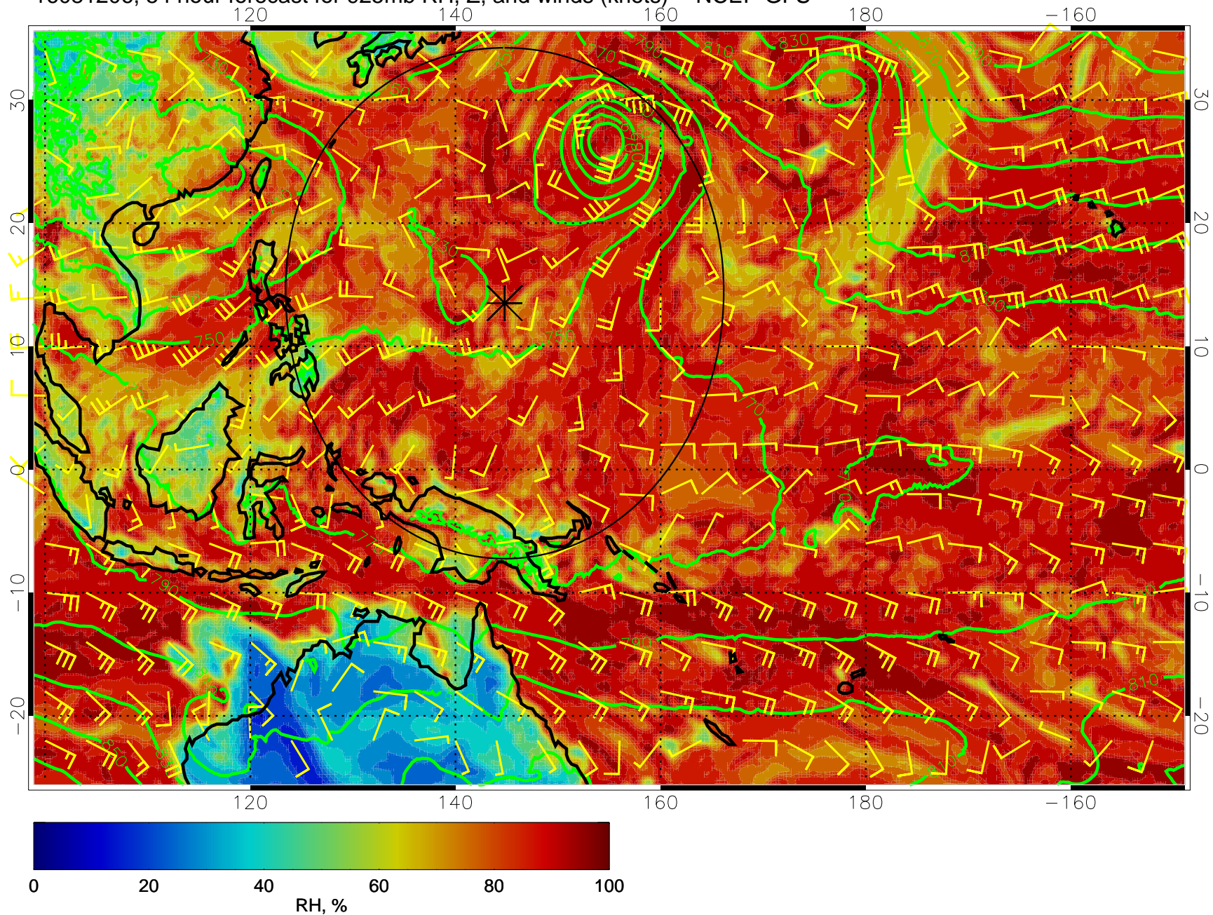
16081206, 54 hour forecast for 925mb RH, Z, and winds (knots) -- NCEP GFS
