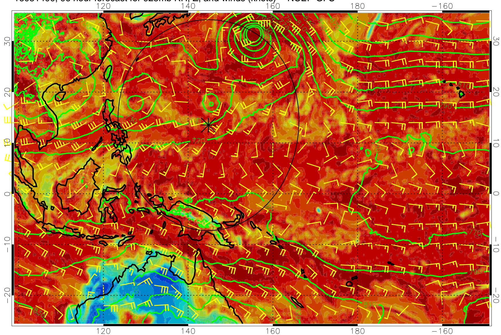
16081400, 96 hour forecast for 925mb RH, Z, and winds (knots) -- NCEP GFS
