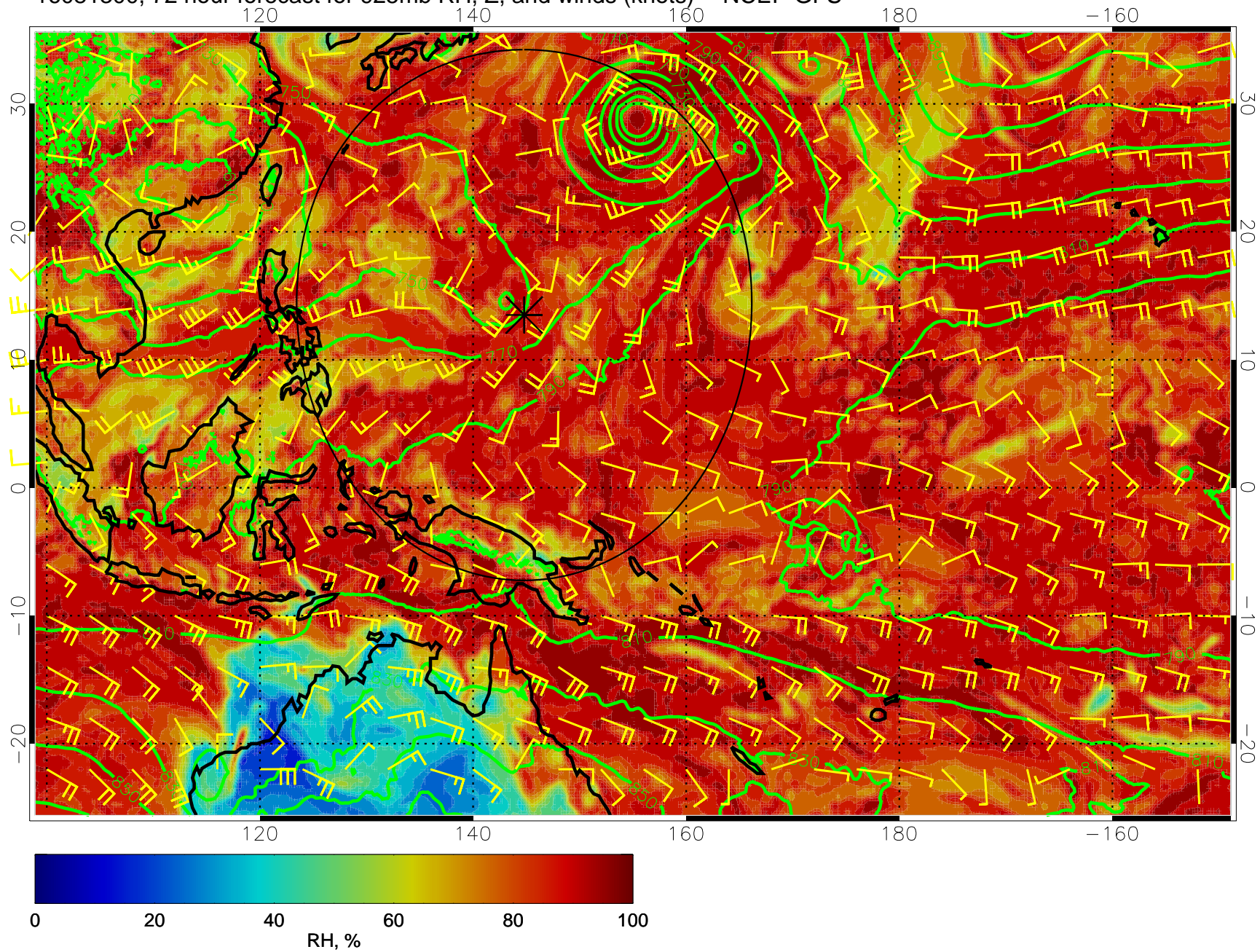
16081300, 72 hour forecast for 925mb RH, Z, and winds (knots) -- NCEP GFS
