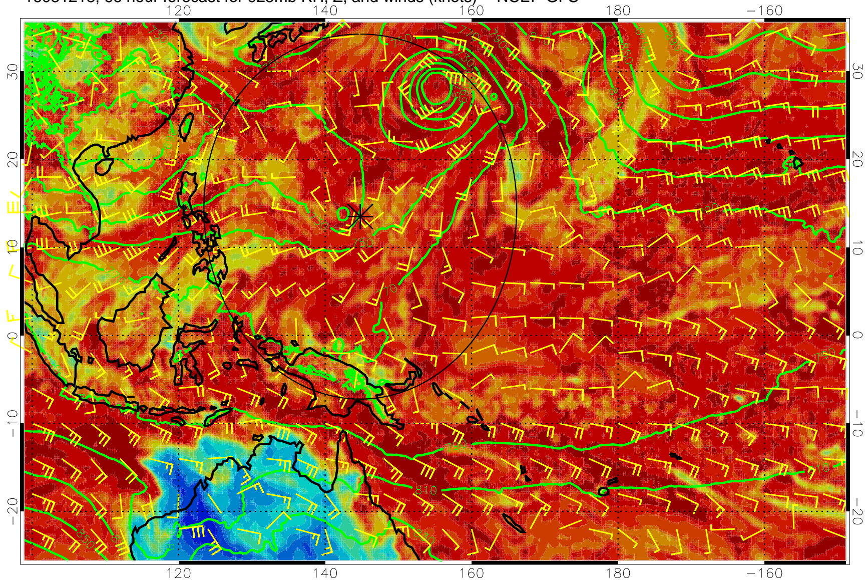
16081218, 66 hour forecast for 925mb RH, Z, and winds (knots) -- NCEP GFS
