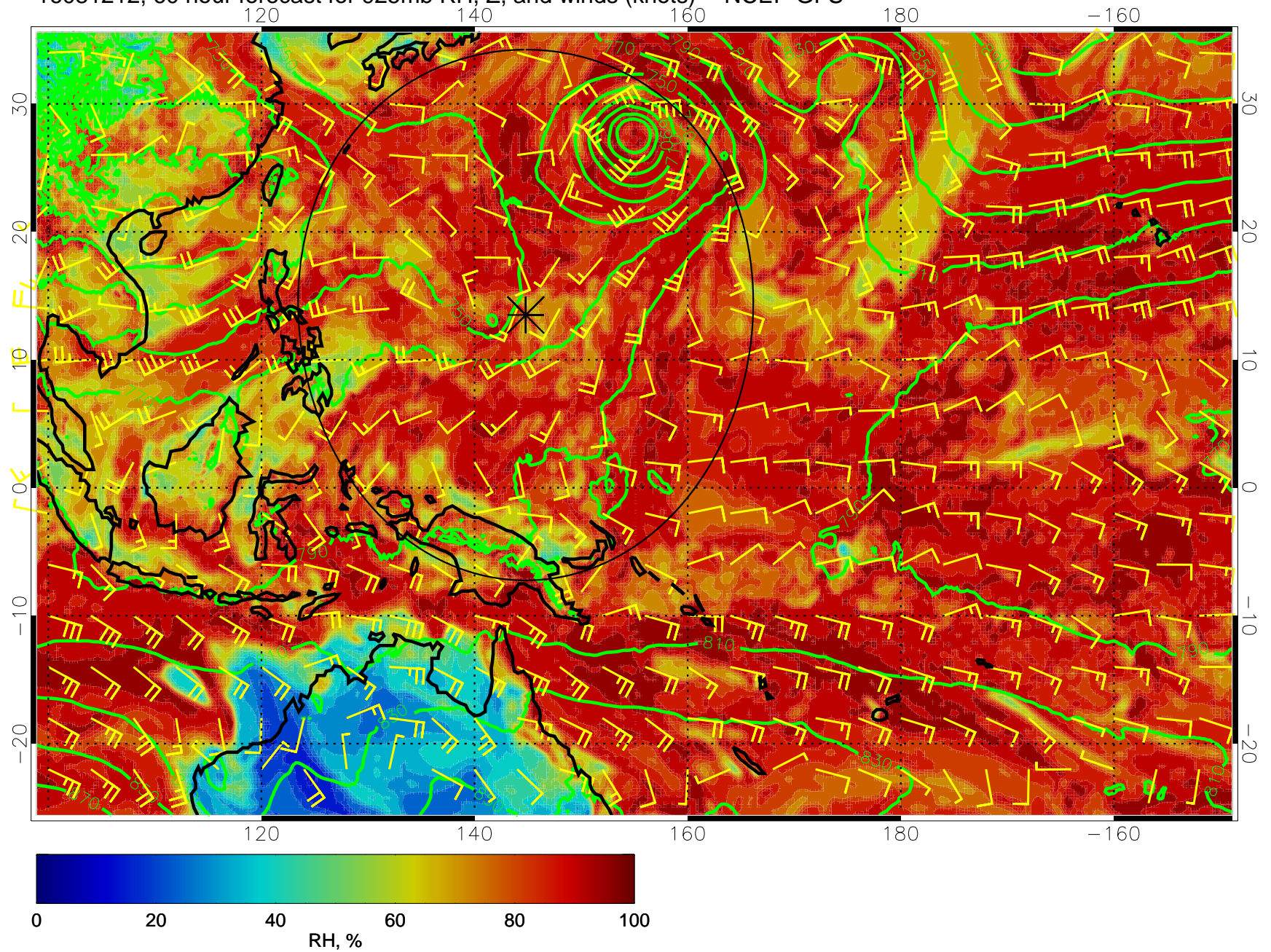
16081212, 60 hour forecast for 925mb RH, Z, and winds (knots) -- NCEP GFS
