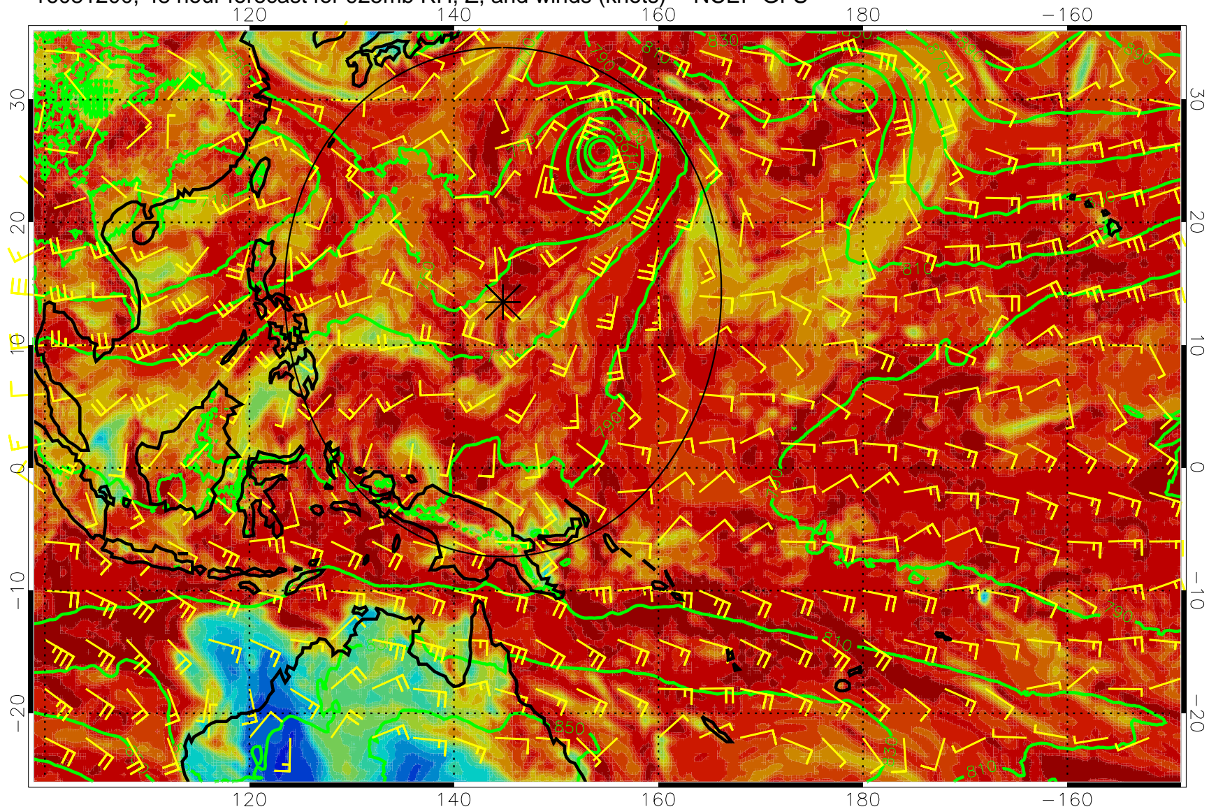
16081200, 48 hour forecast for 925mb RH, Z, and winds (knots) -- NCEP GFS
