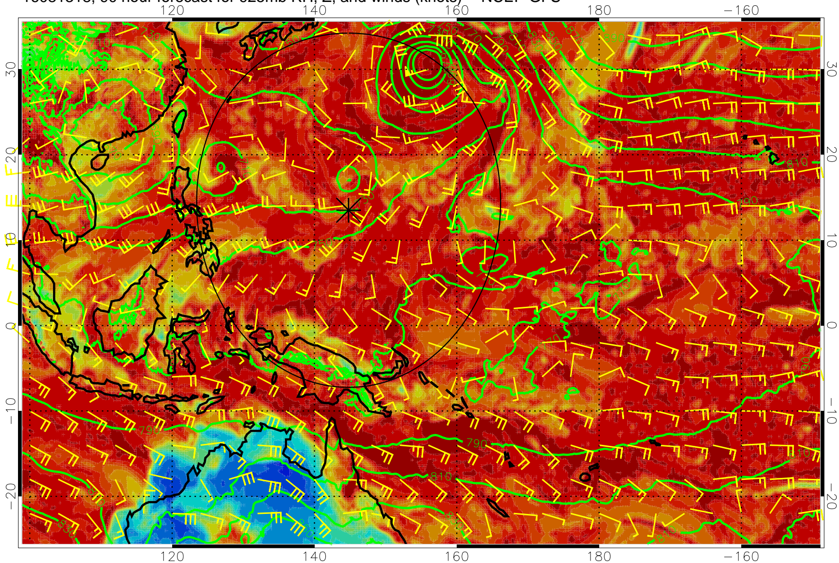
16081318, 90 hour forecast for 925mb RH, Z, and winds (knots) -- NCEP GFS
