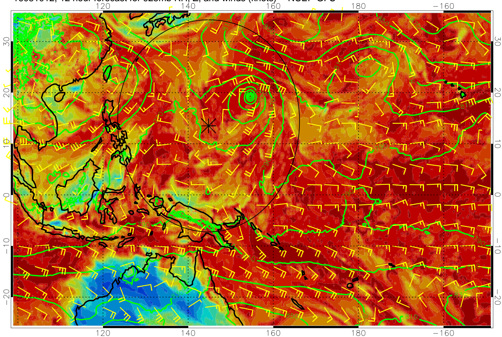
16081012, 12 hour forecast for 925mb RH, Z, and winds (knots) -- NCEP GFS
