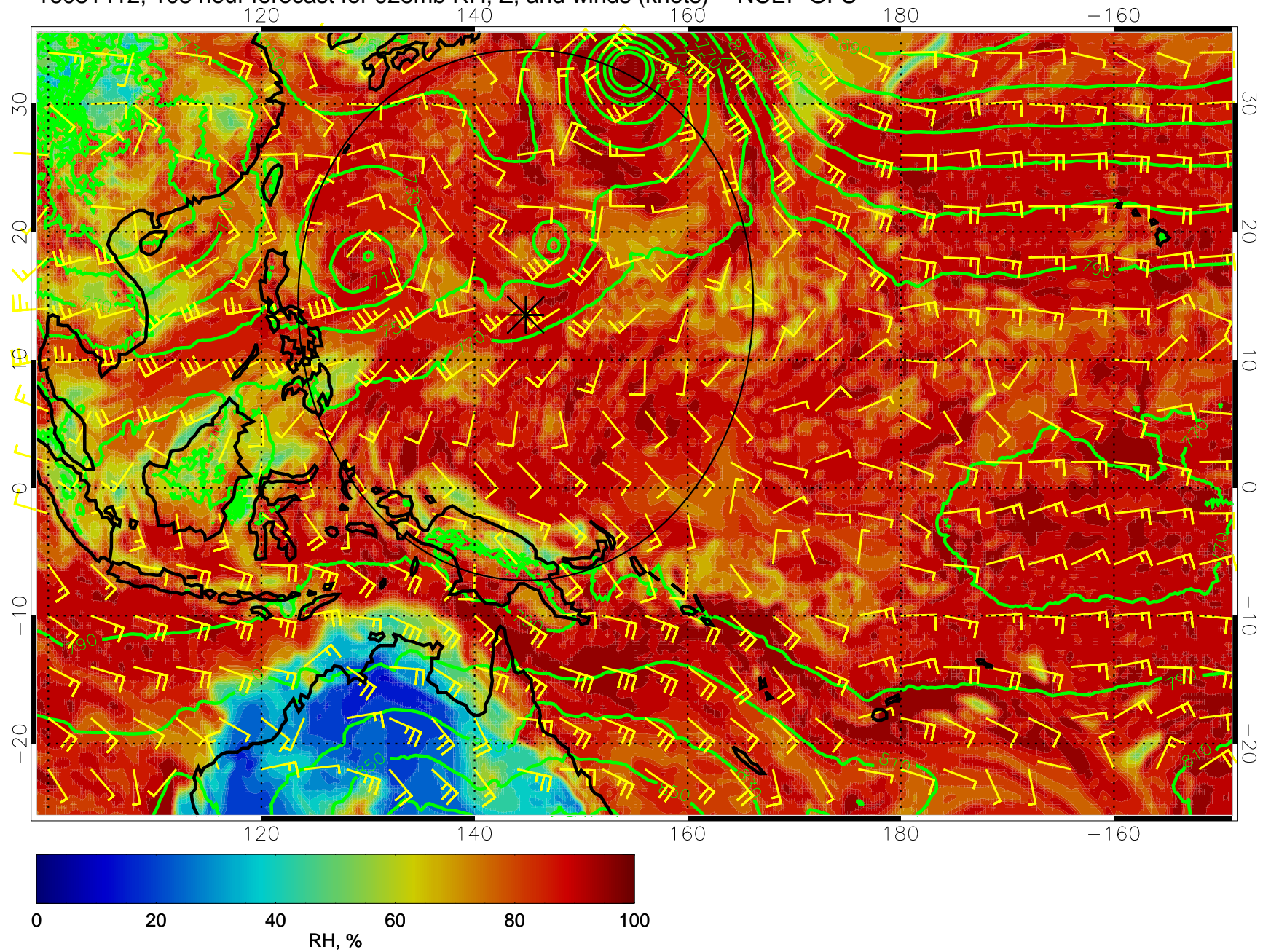
16081412, 108 hour forecast for 925mb RH, Z, and winds (knots) -- NCEP GFS
