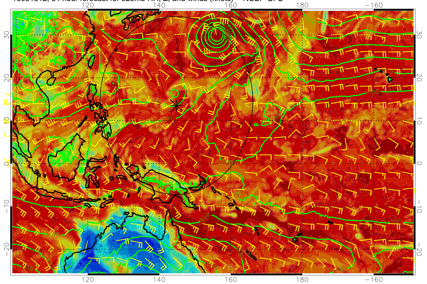
16081312, 84 hour forecast for 925mb RH, Z, and winds (knots) -- NCEP GFS
