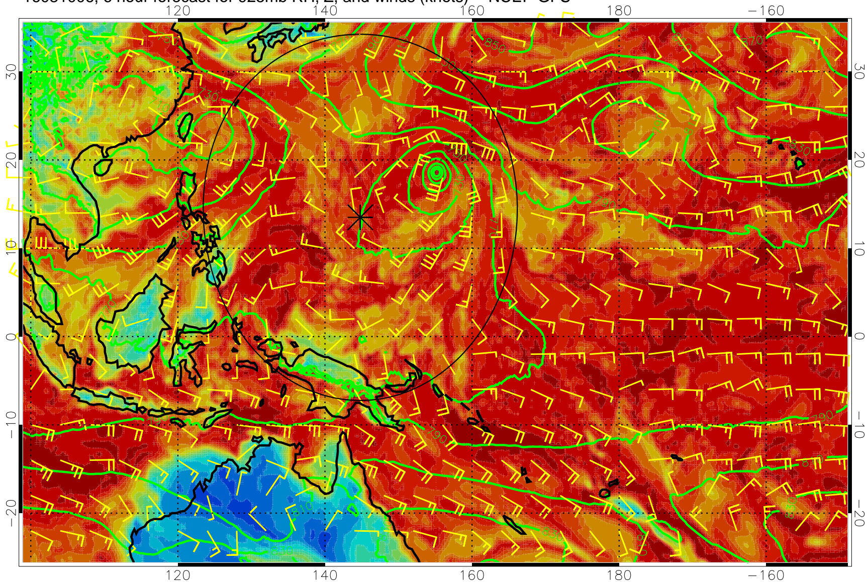
16081006, 6 hour forecast for 925mb RH, Z, and winds (knots) -- NCEP GFS
