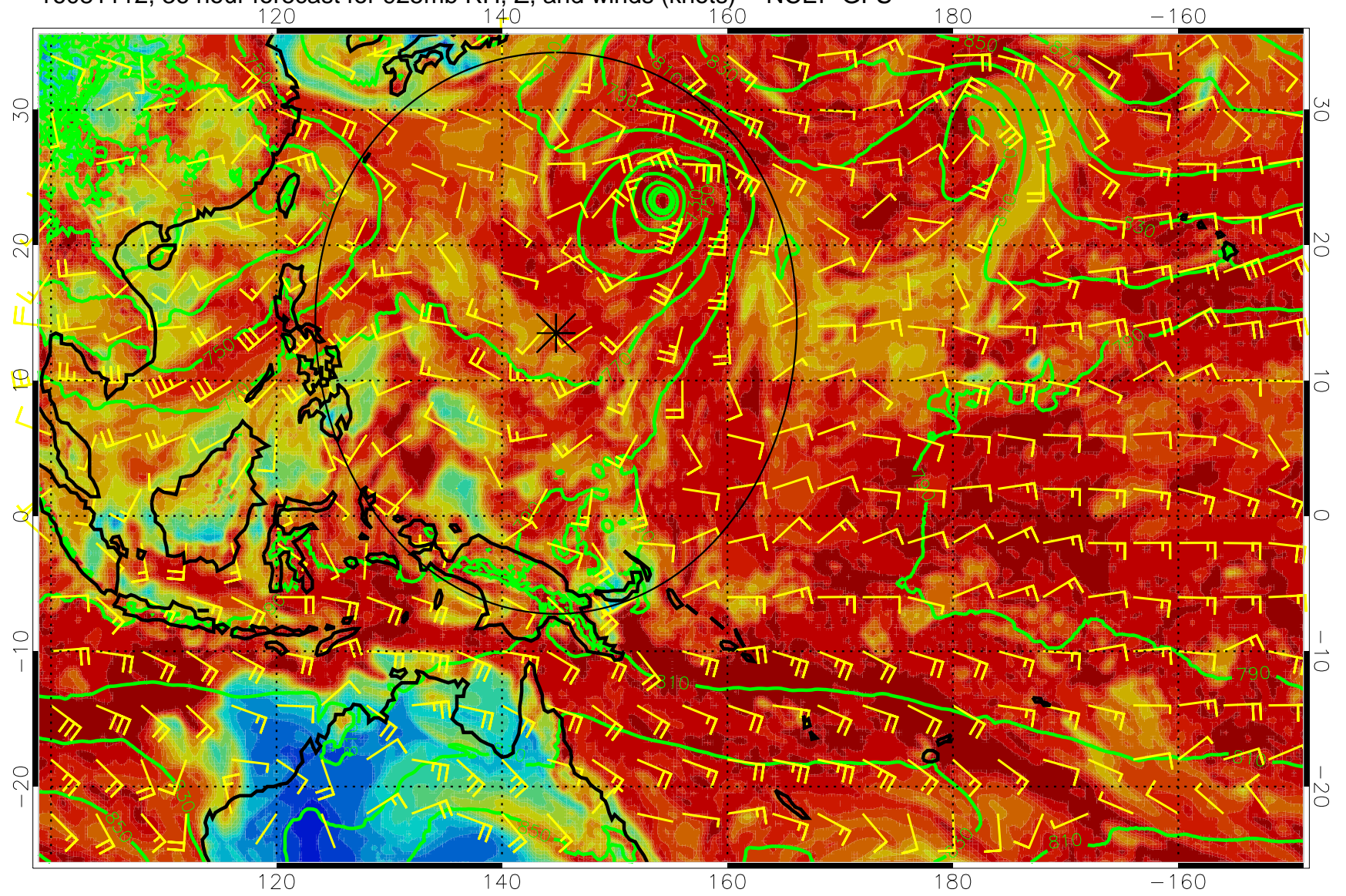
16081112, 36 hour forecast for 925mb RH, Z, and winds (knots) -- NCEP GFS
