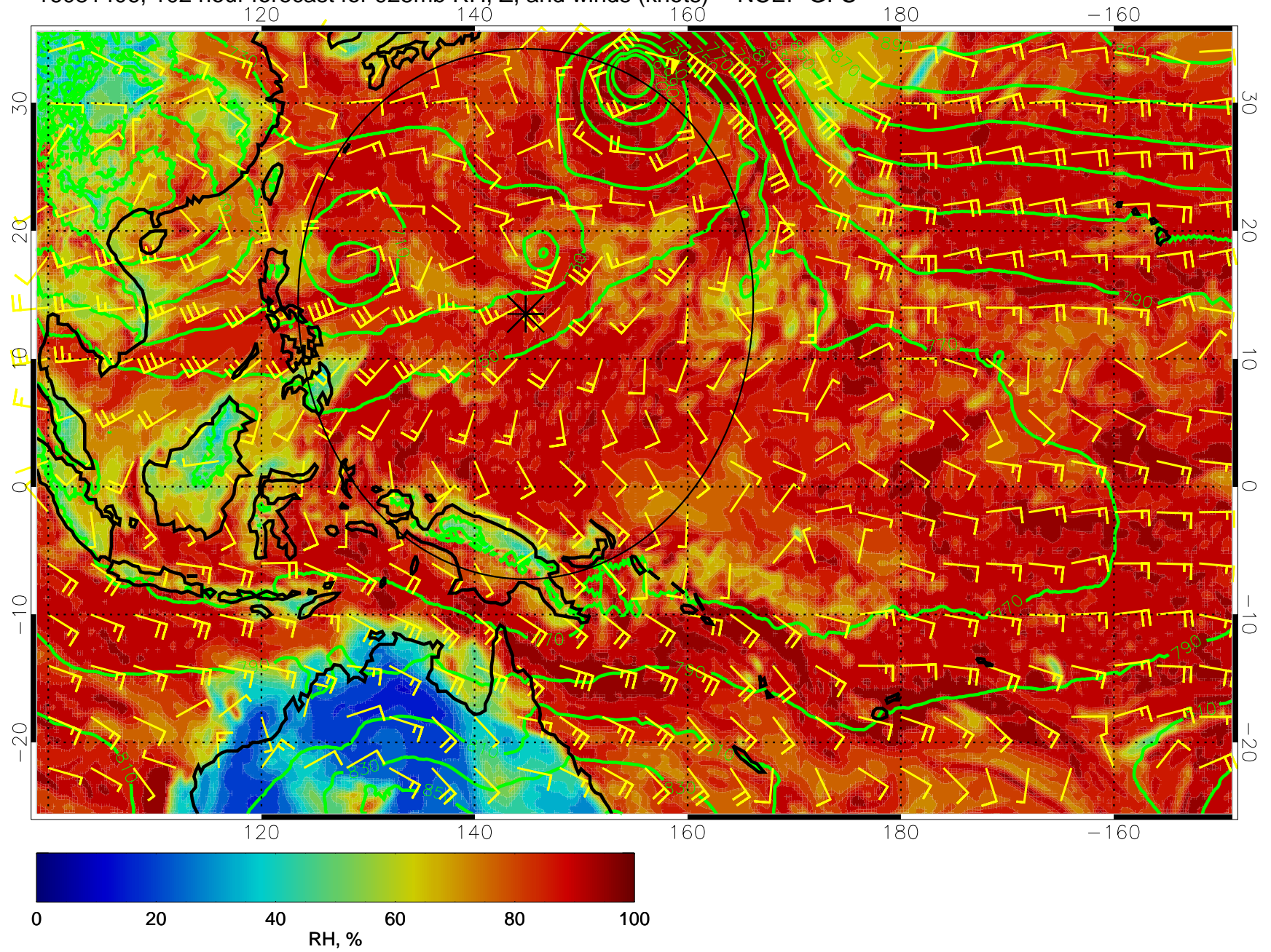
16081406, 102 hour forecast for 925mb RH, Z, and winds (knots) -- NCEP GFS
