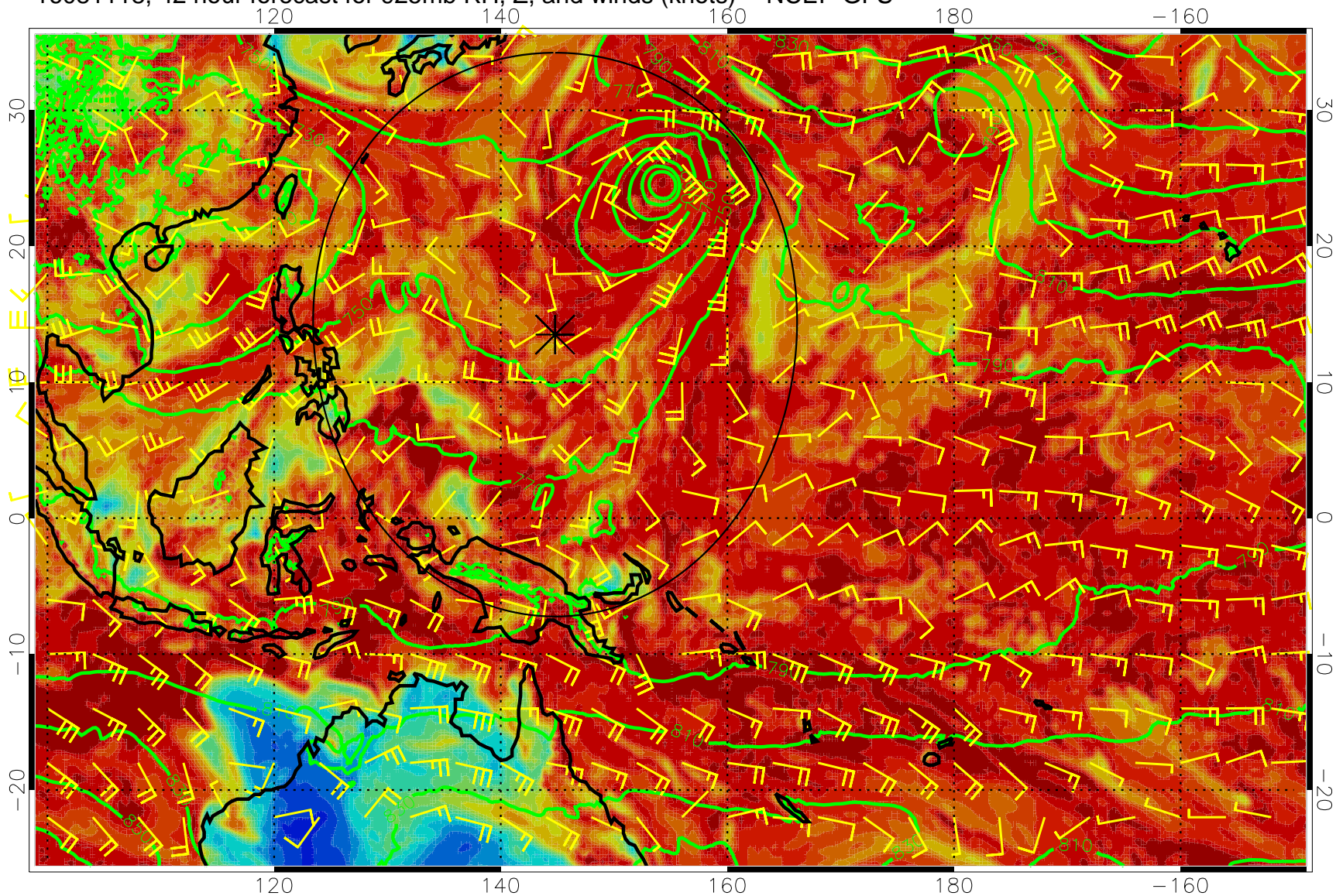
16081118, 42 hour forecast for 925mb RH, Z, and winds (knots) -- NCEP GFS
