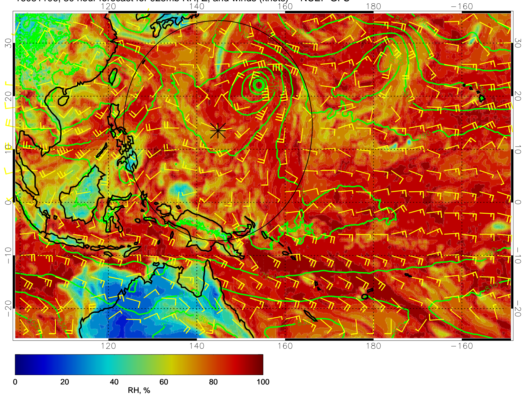
16081106, 30 hour forecast for 925mb RH, Z, and winds (knots) -- NCEP GFS
