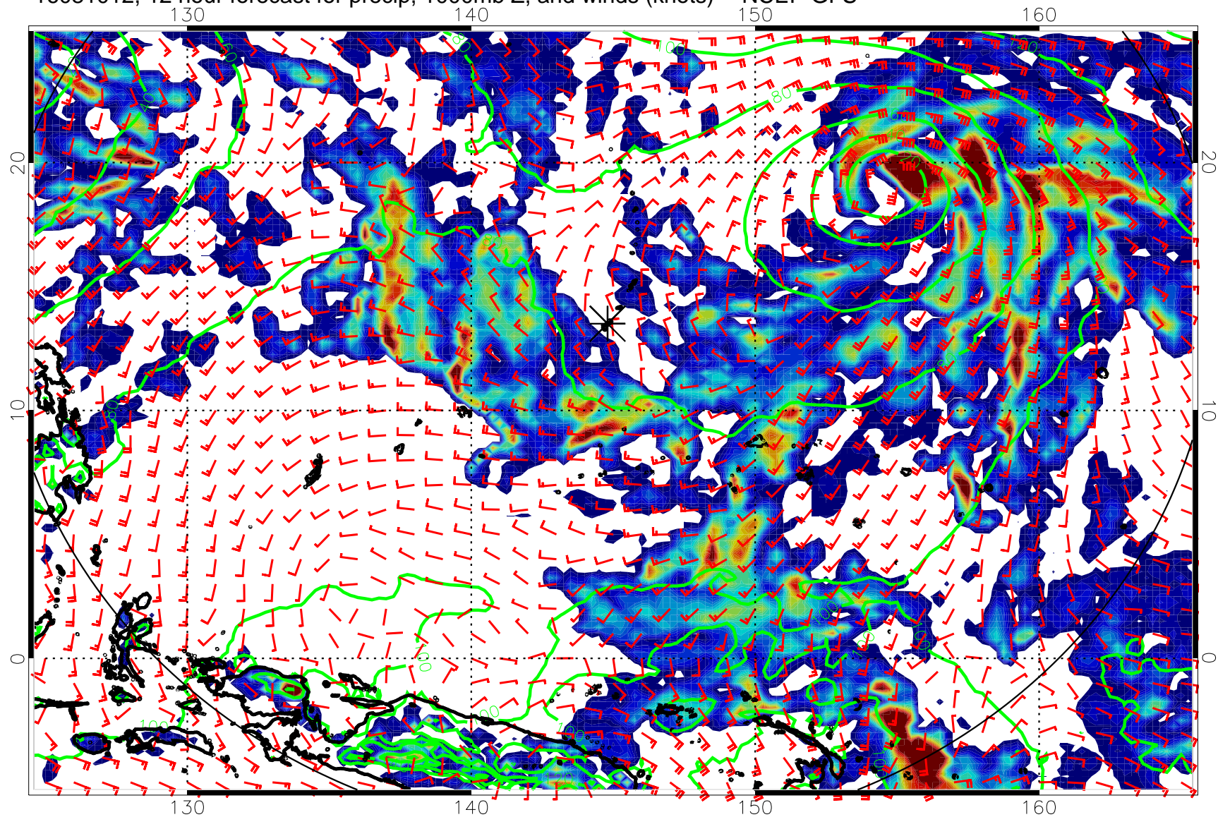
16081012, 12 hour forecast for precip, 1000mb Z, and winds (knots) -- NCEP GFS
