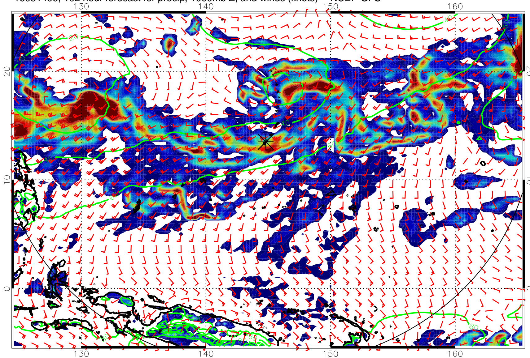
16081406, 102 hour forecast for precip, 1000mb Z, and winds (knots) -- NCEP GFS
