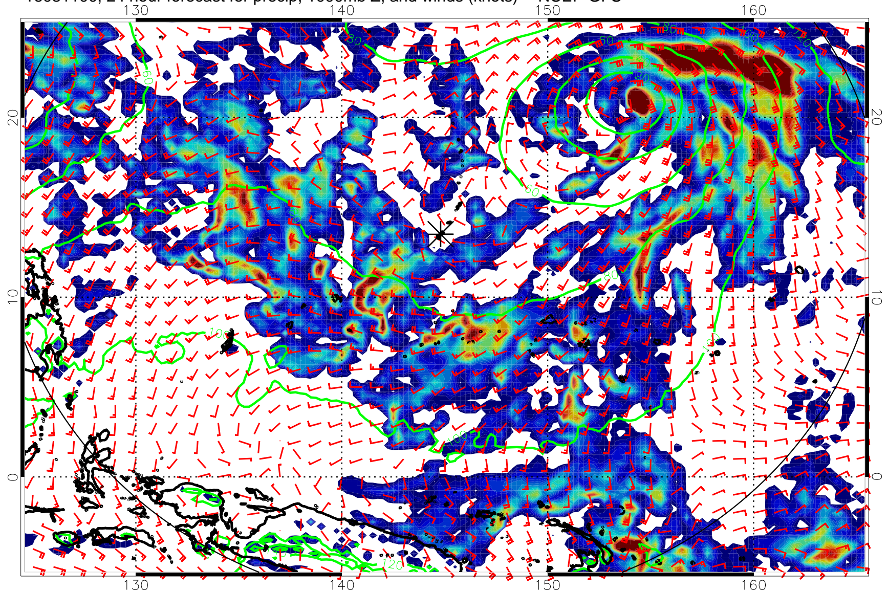
16081100, 24 hour forecast for precip, 1000mb Z, and winds (knots) -- NCEP GFS
