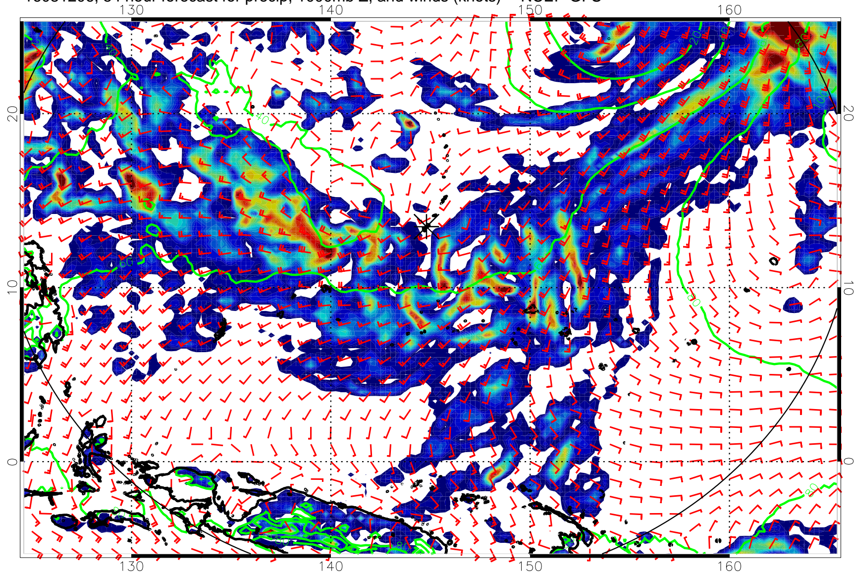
16081206, 54 hour forecast for precip, 1000mb Z, and winds (knots) -- NCEP GFS
