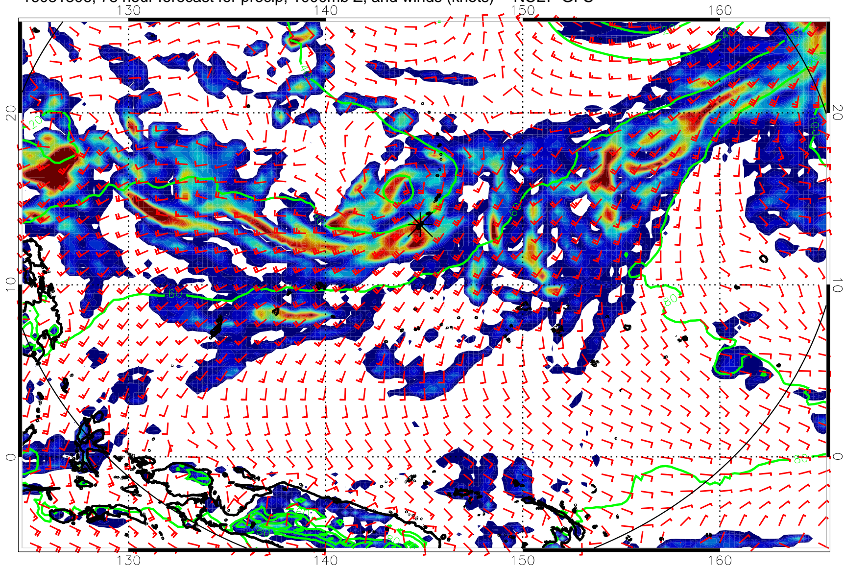
16081306, 78 hour forecast for precip, 1000mb Z, and winds (knots) -- NCEP GFS
