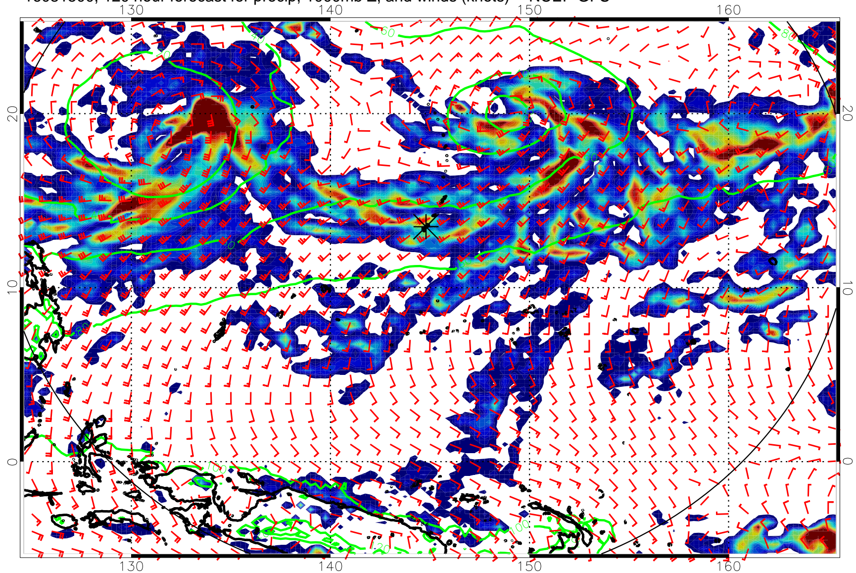
16081500, 120 hour forecast for precip, 1000mb Z, and winds (knots) -- NCEP GFS
