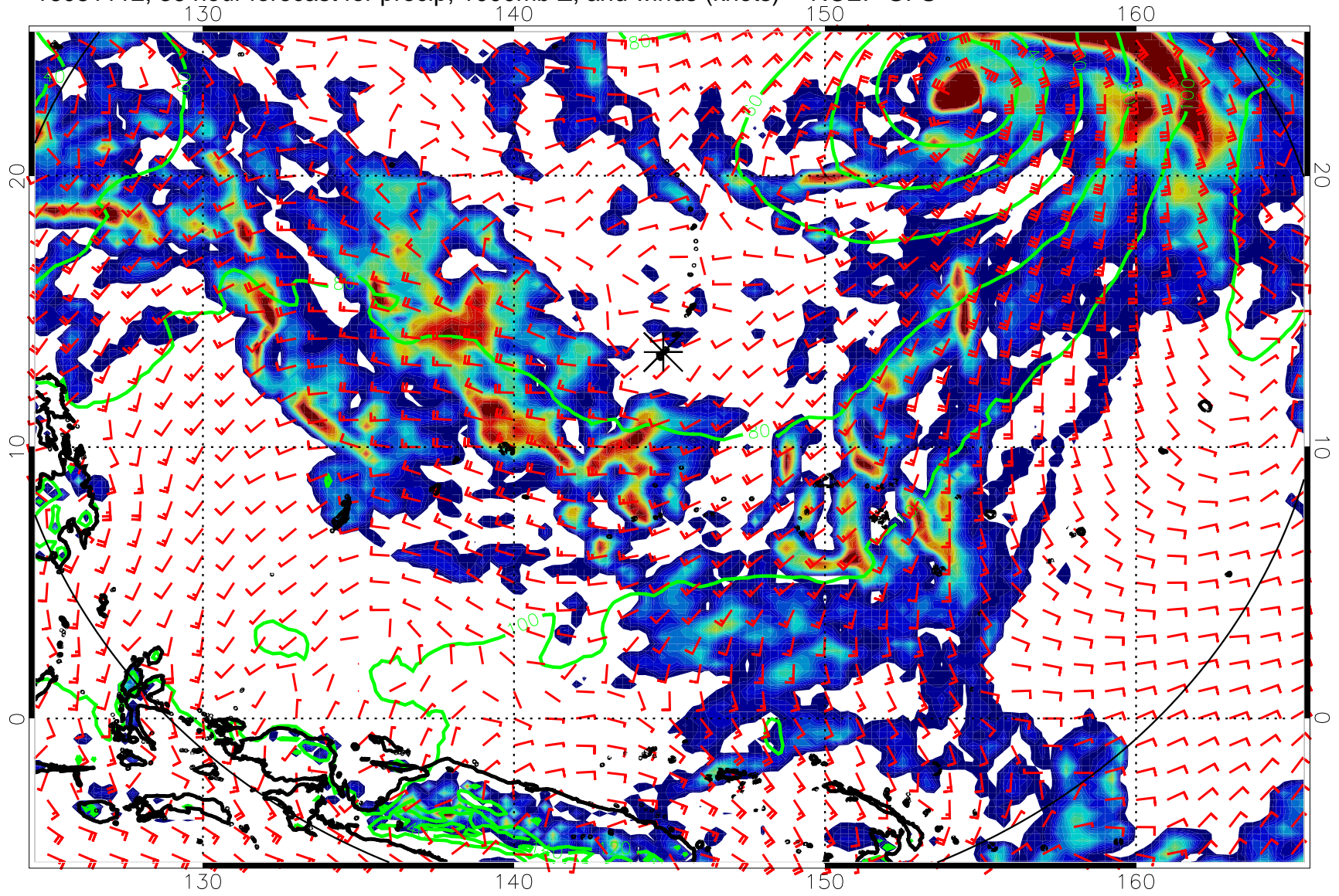
16081112, 36 hour forecast for precip, 1000mb Z, and winds (knots) -- NCEP GFS
