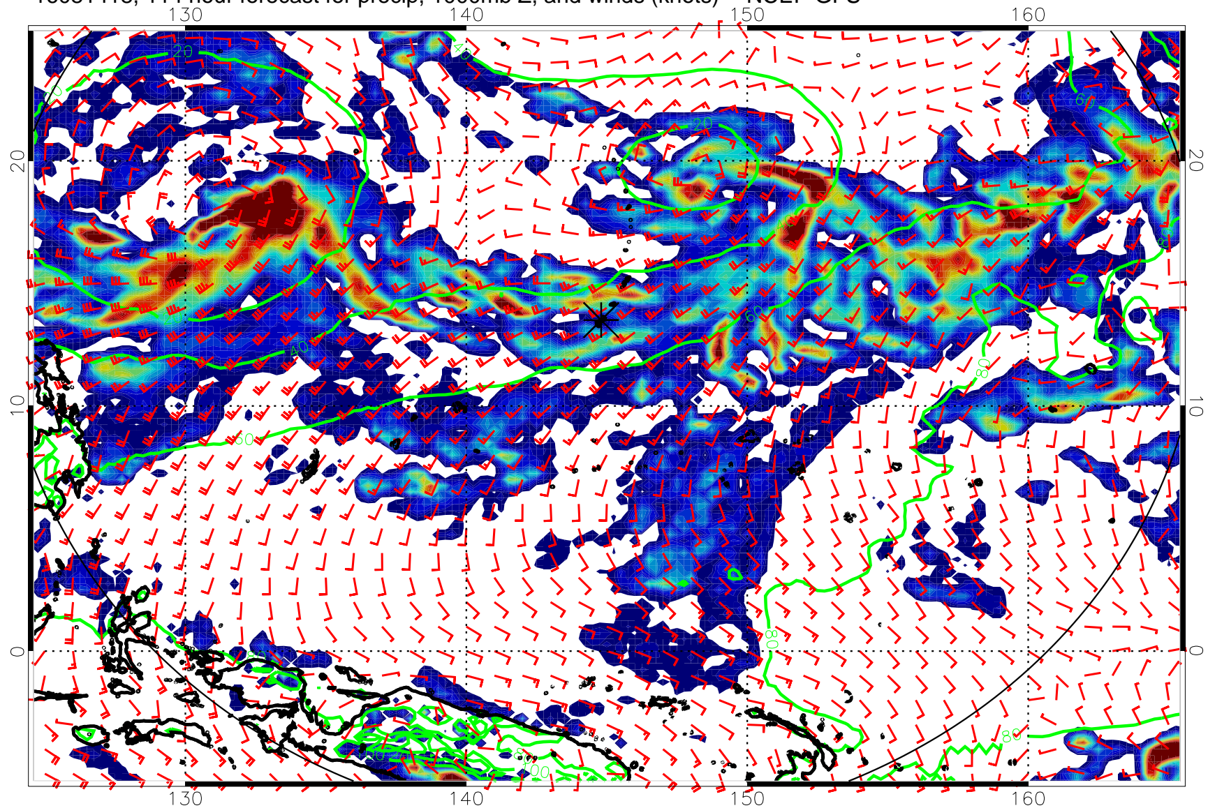
16081418, 114 hour forecast for precip, 1000mb Z, and winds (knots) -- NCEP GFS
