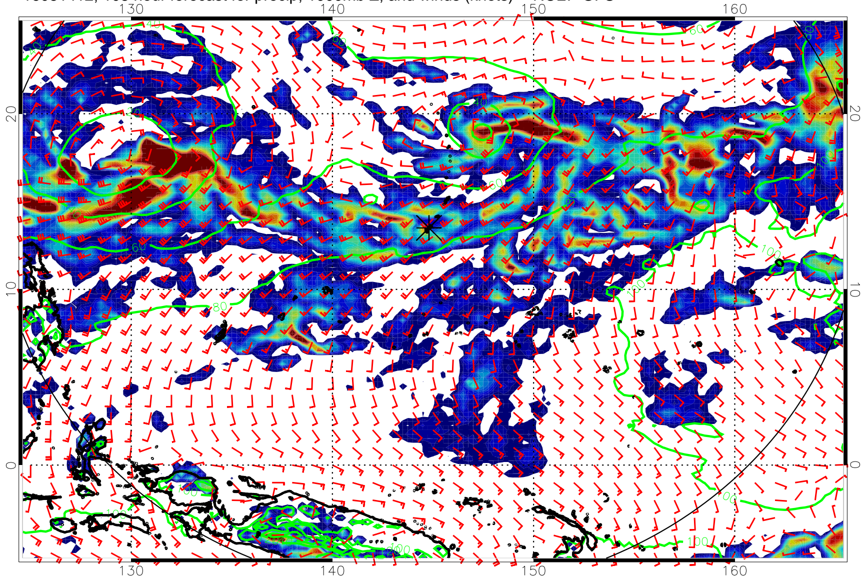
16081412, 108 hour forecast for precip, 1000mb Z, and winds (knots) -- NCEP GFS
