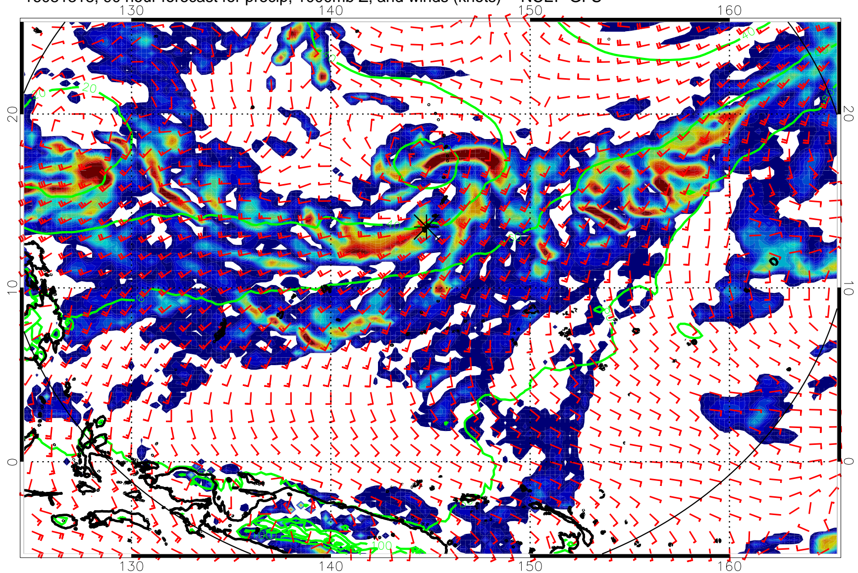
16081318, 90 hour forecast for precip, 1000mb Z, and winds (knots) -- NCEP GFS
