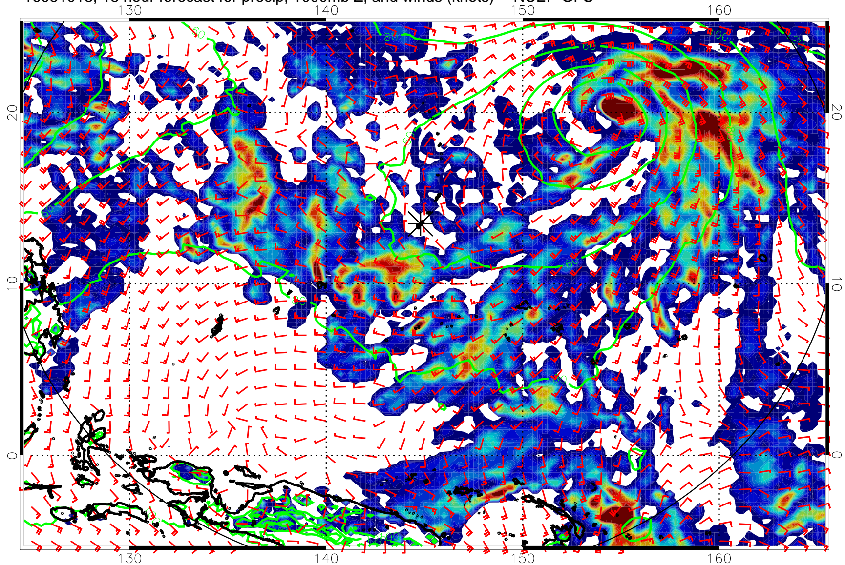
16081018, 18 hour forecast for precip, 1000mb Z, and winds (knots) -- NCEP GFS
