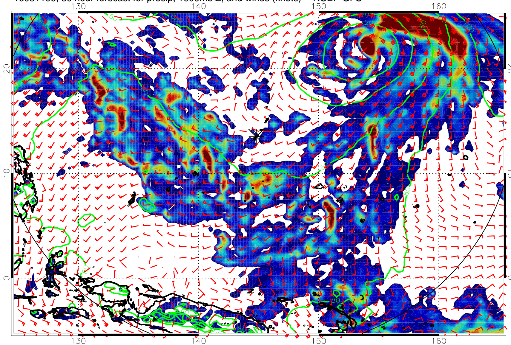
16081106, 30 hour forecast for precip, 1000mb Z, and winds (knots) -- NCEP GFS
