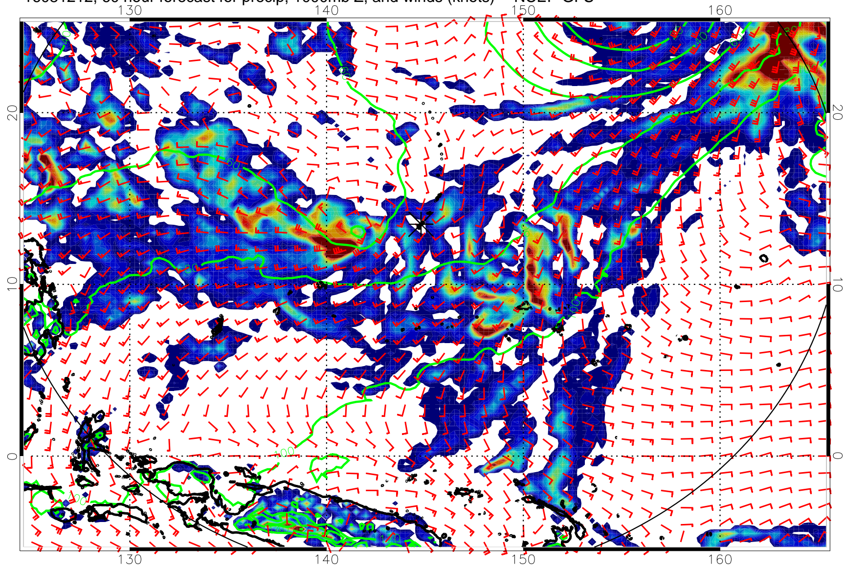
16081212, 60 hour forecast for precip, 1000mb Z, and winds (knots) -- NCEP GFS
