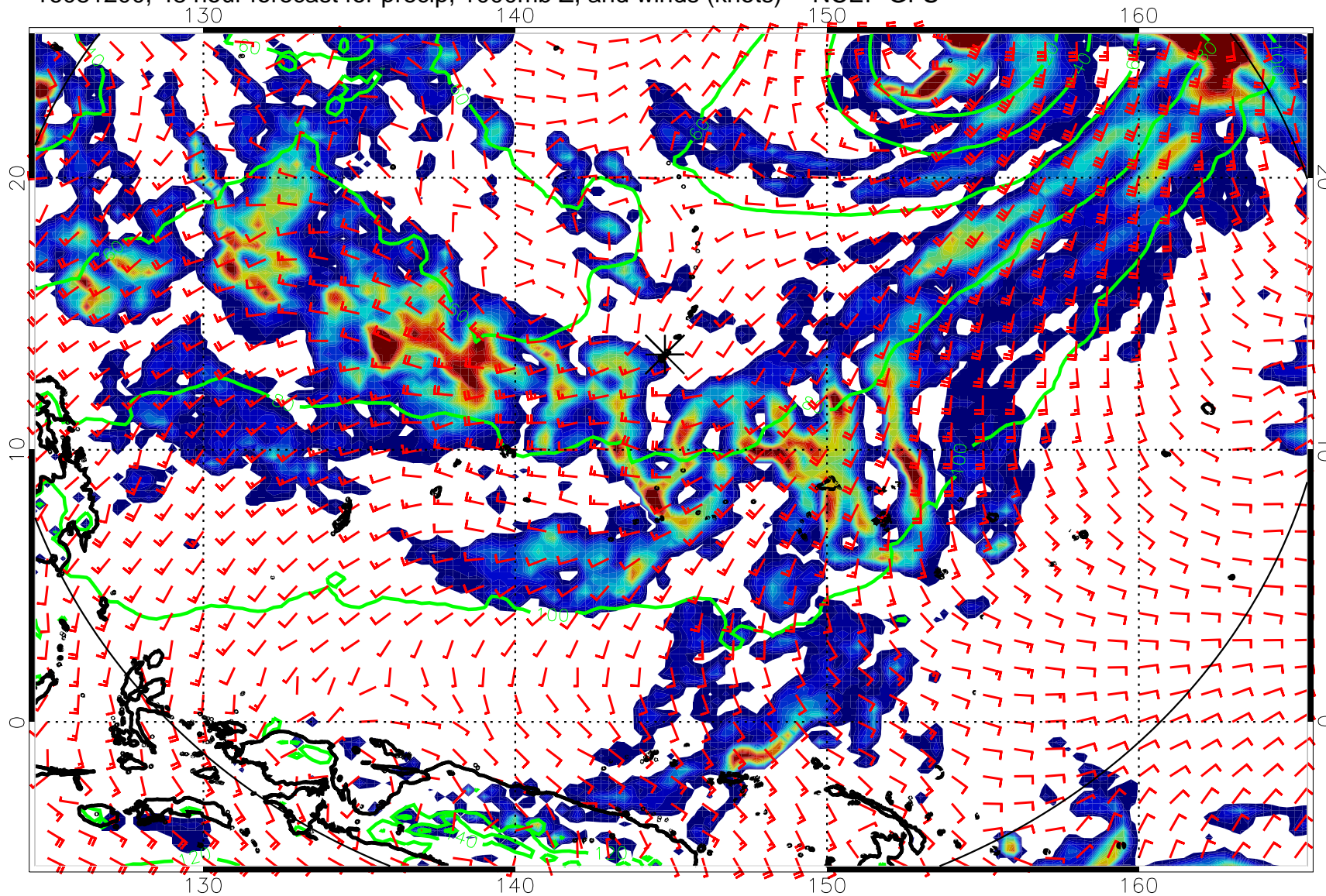
16081200, 48 hour forecast for precip, 1000mb Z, and winds (knots) -- NCEP GFS
