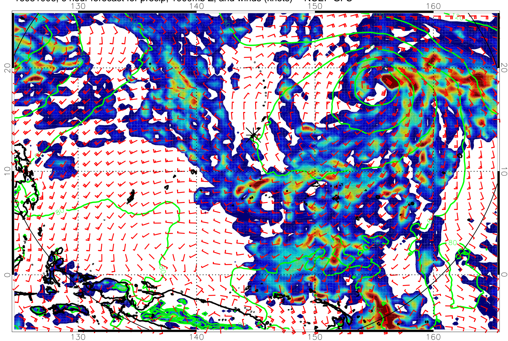
16081006, 6 hour forecast for precip, 1000mb Z, and winds (knots) -- NCEP GFS
