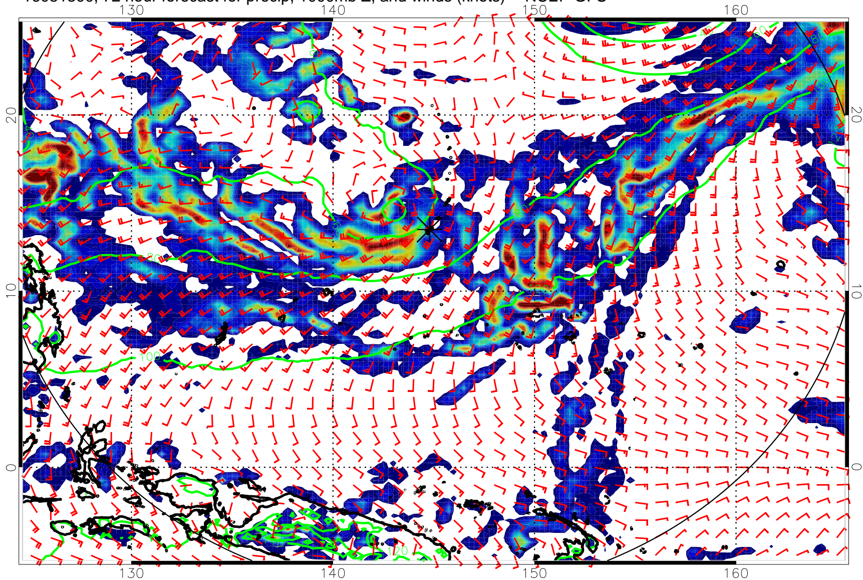
16081300, 72 hour forecast for precip, 1000mb Z, and winds (knots) -- NCEP GFS
