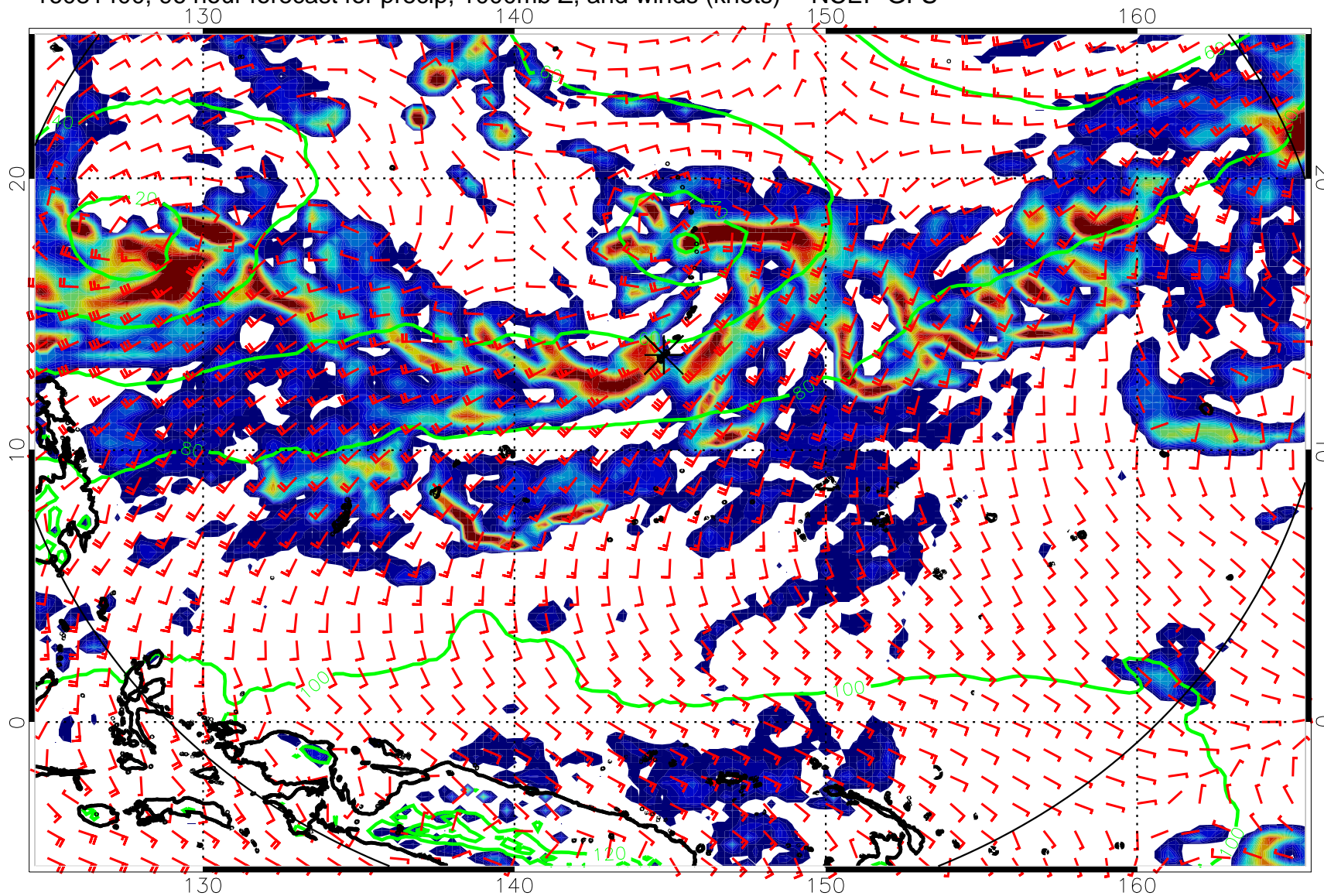
16081400, 96 hour forecast for precip, 1000mb Z, and winds (knots) -- NCEP GFS
