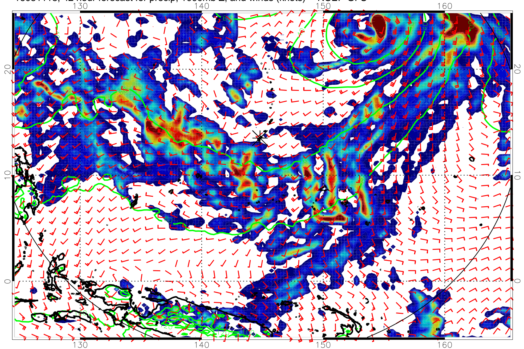
16081118, 42 hour forecast for precip, 1000mb Z, and winds (knots) -- NCEP GFS
