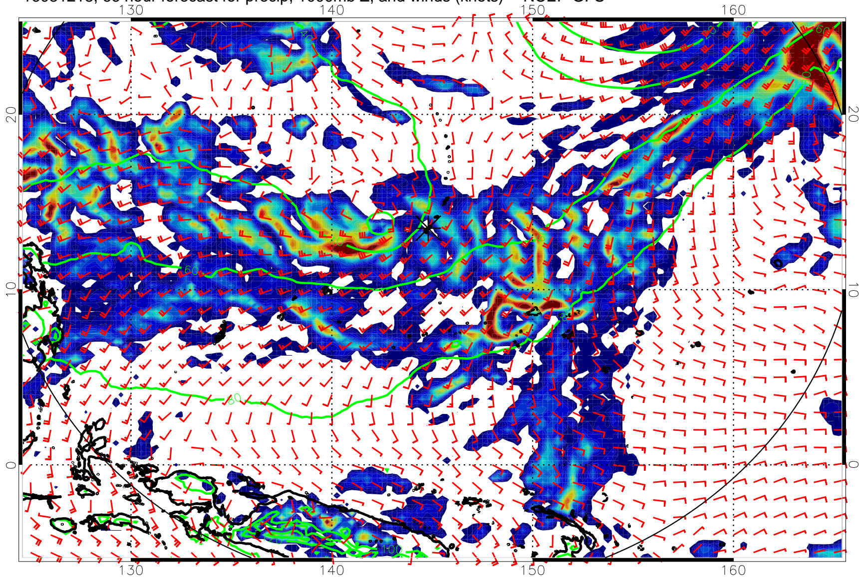
16081218, 66 hour forecast for precip, 1000mb Z, and winds (knots) -- NCEP GFS
