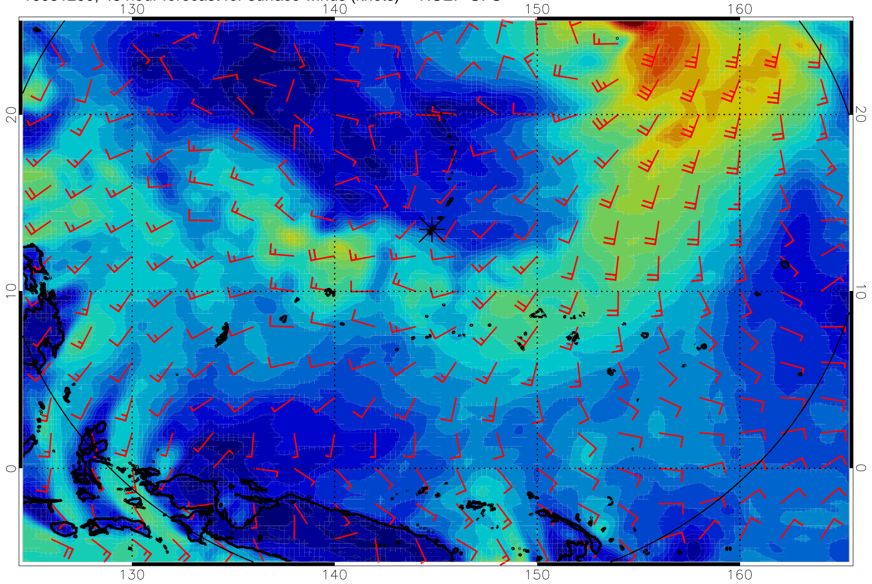
16081200, 48 hour forecast for surface winds (knots) -- NCEP GFS
