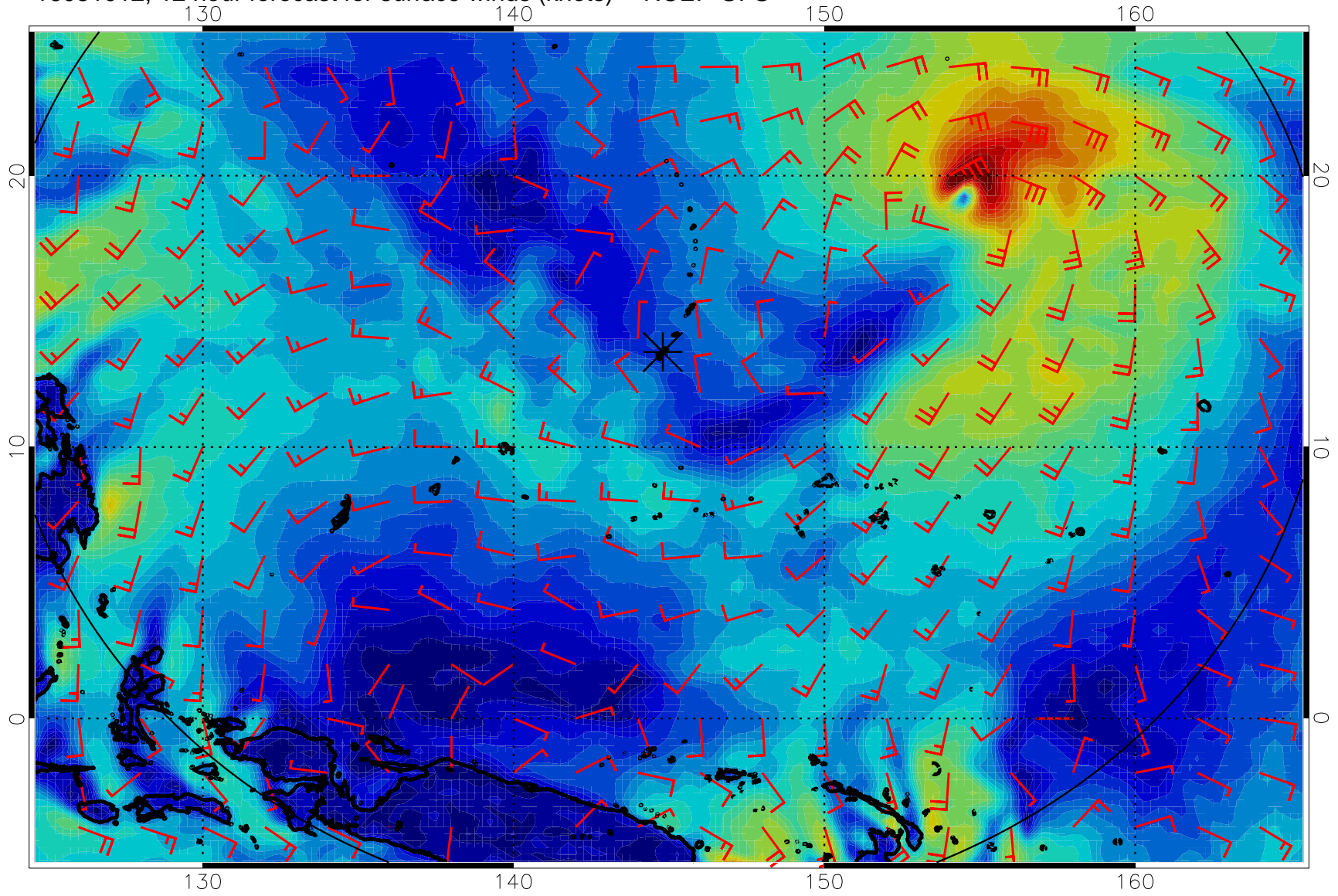
16081012, 12 hour forecast for surface winds (knots) -- NCEP GFS
