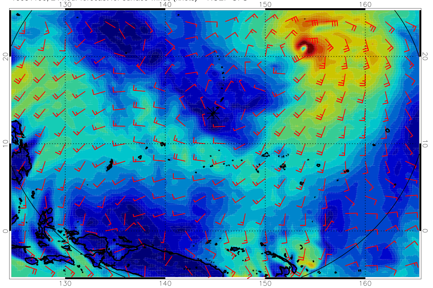
16081100, 24 hour forecast for surface winds (knots) -- NCEP GFS
