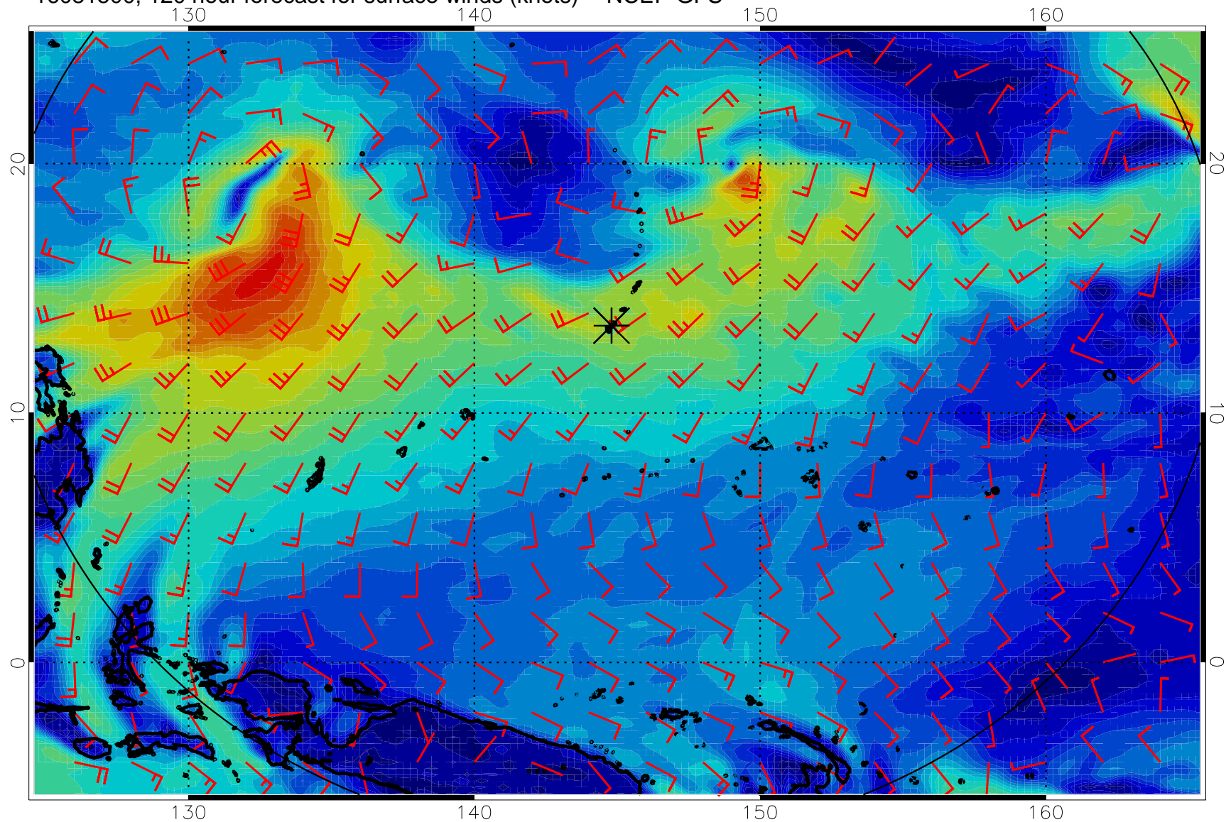
16081500, 120 hour forecast for surface winds (knots) -- NCEP GFS
