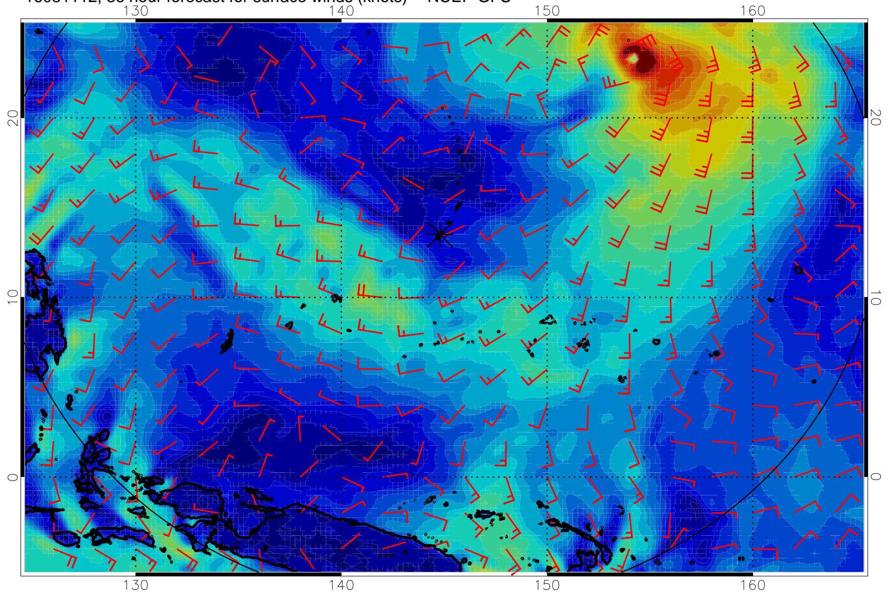
16081112, 36 hour forecast for surface winds (knots) -- NCEP GFS
