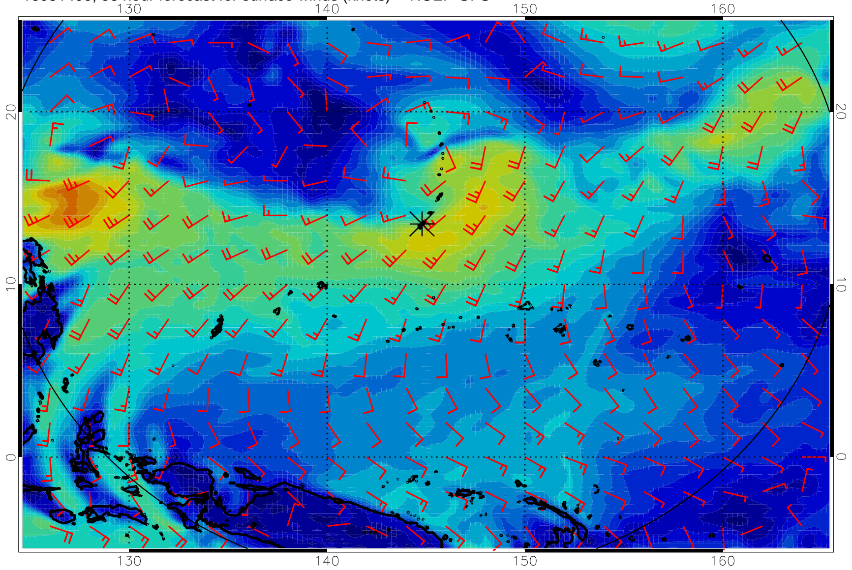
16081400, 96 hour forecast for surface winds (knots) -- NCEP GFS
