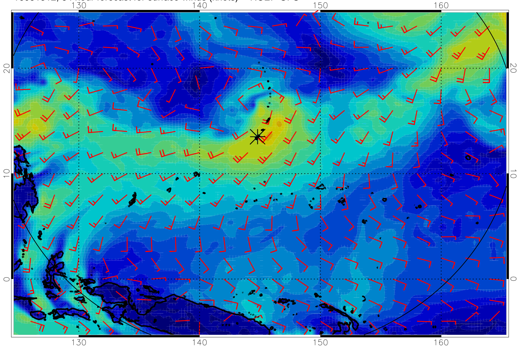
16081312, 84 hour forecast for surface winds (knots) -- NCEP GFS
