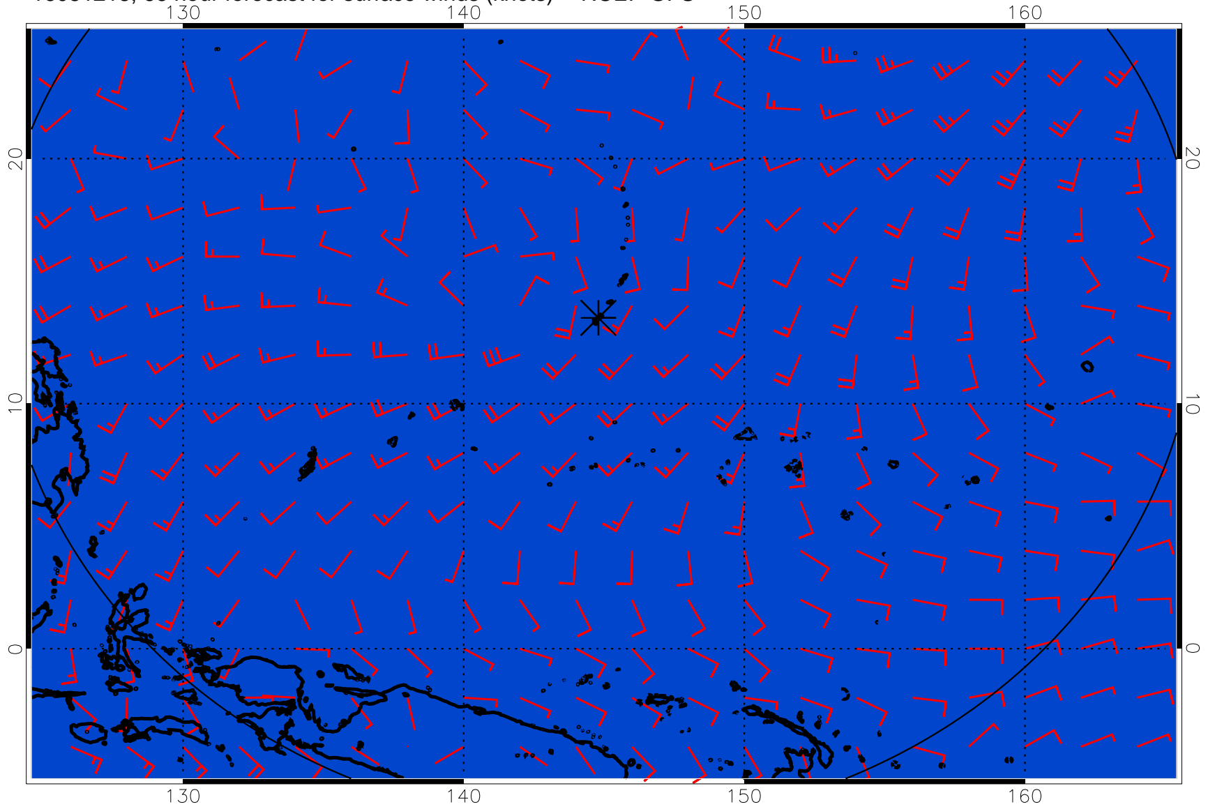
16081218, 66 hour forecast for surface winds (knots) -- NCEP GFS
