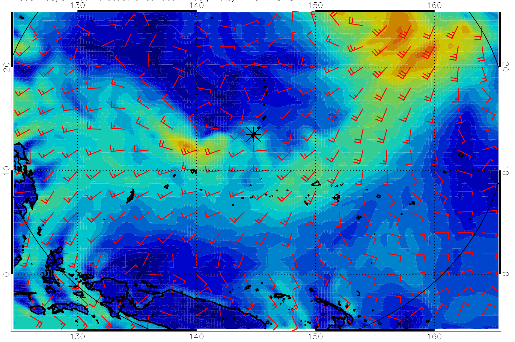
16081206, 54 hour forecast for surface winds (knots) -- NCEP GFS
