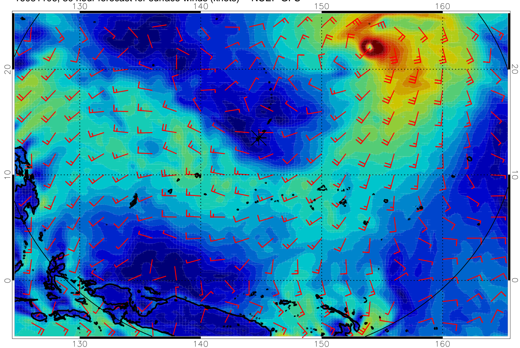
16081106, 30 hour forecast for surface winds (knots) -- NCEP GFS
