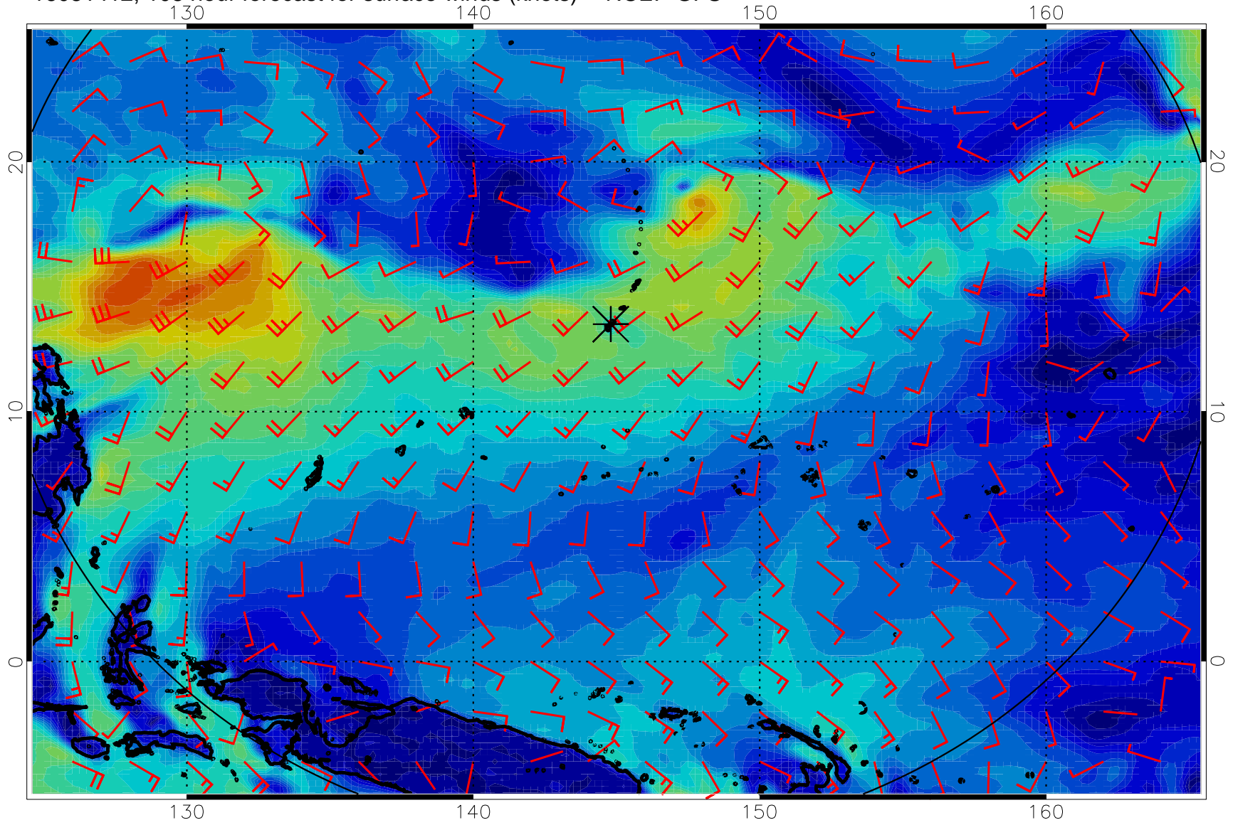
16081412, 108 hour forecast for surface winds (knots) -- NCEP GFS
