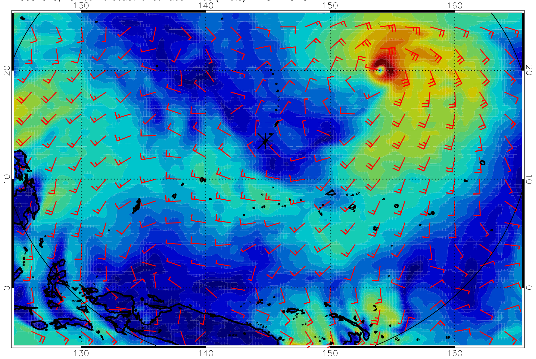
16081018, 18 hour forecast for surface winds (knots) -- NCEP GFS
