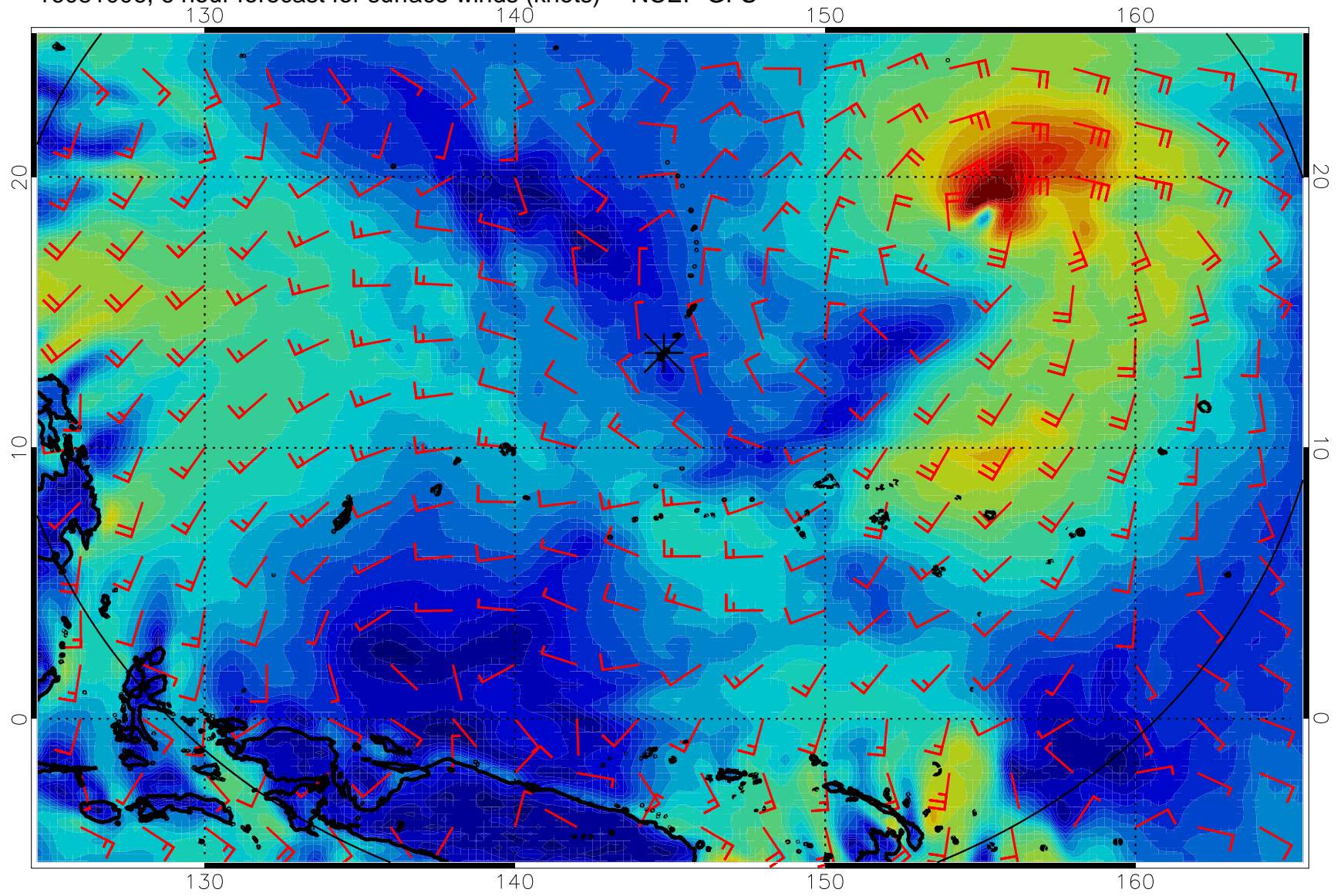
16081006, 6 hour forecast for surface winds (knots) -- NCEP GFS
