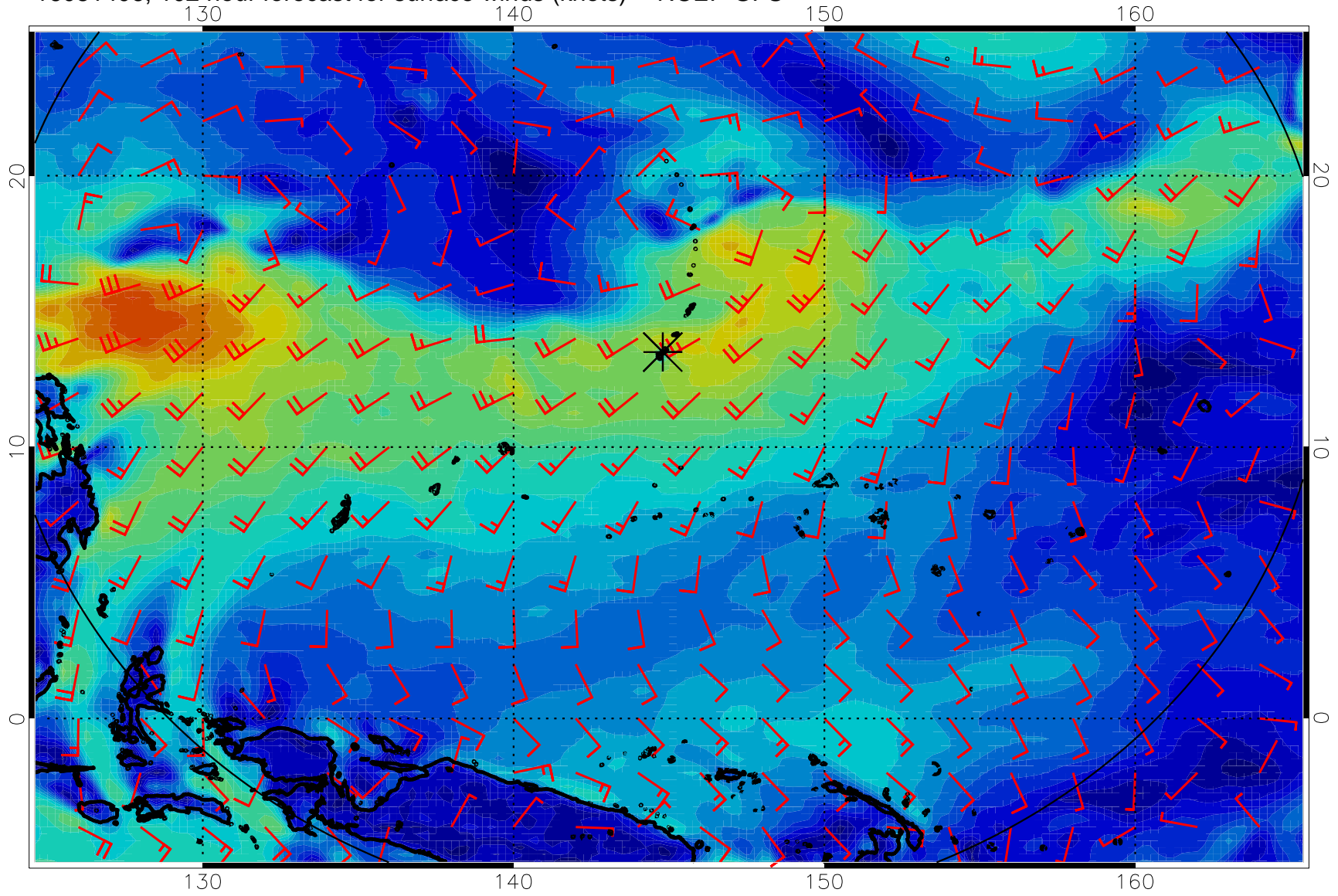
16081406, 102 hour forecast for surface winds (knots) -- NCEP GFS
