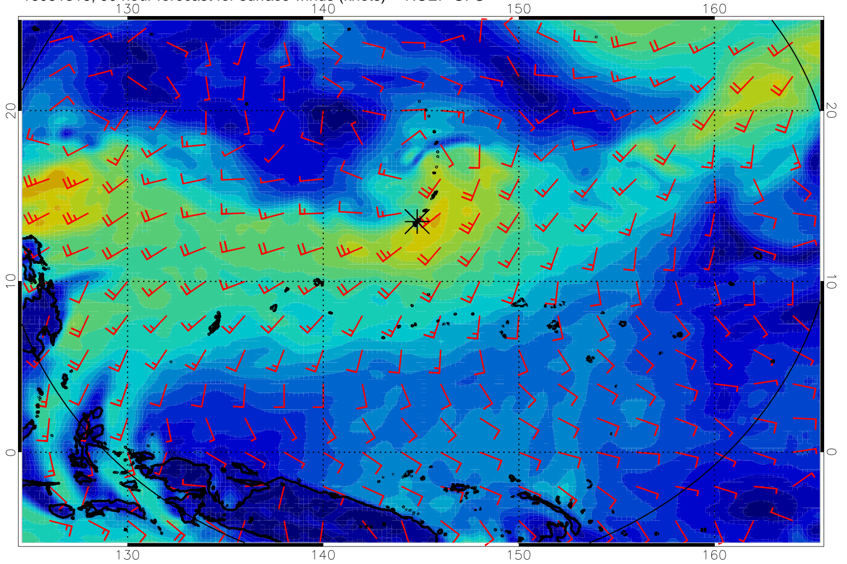
16081318, 90 hour forecast for surface winds (knots) -- NCEP GFS
