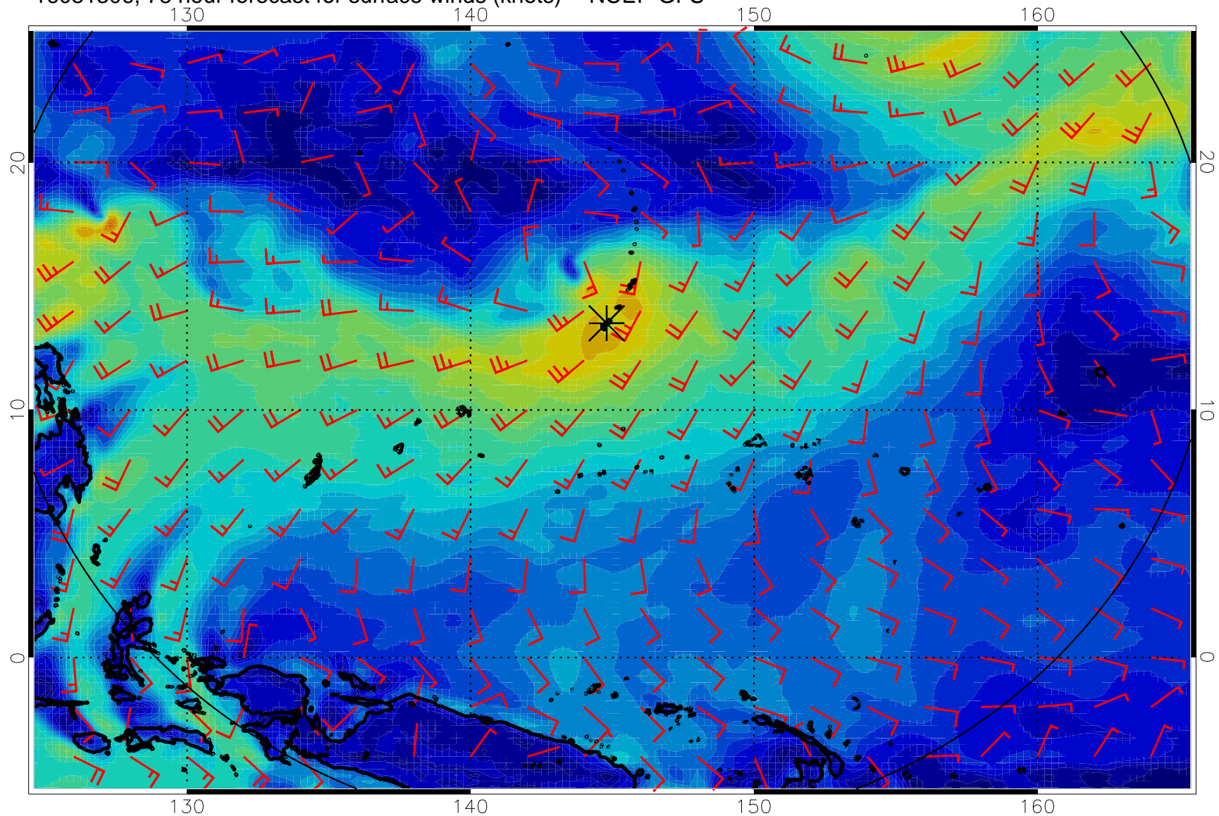
16081306, 78 hour forecast for surface winds (knots) -- NCEP GFS
