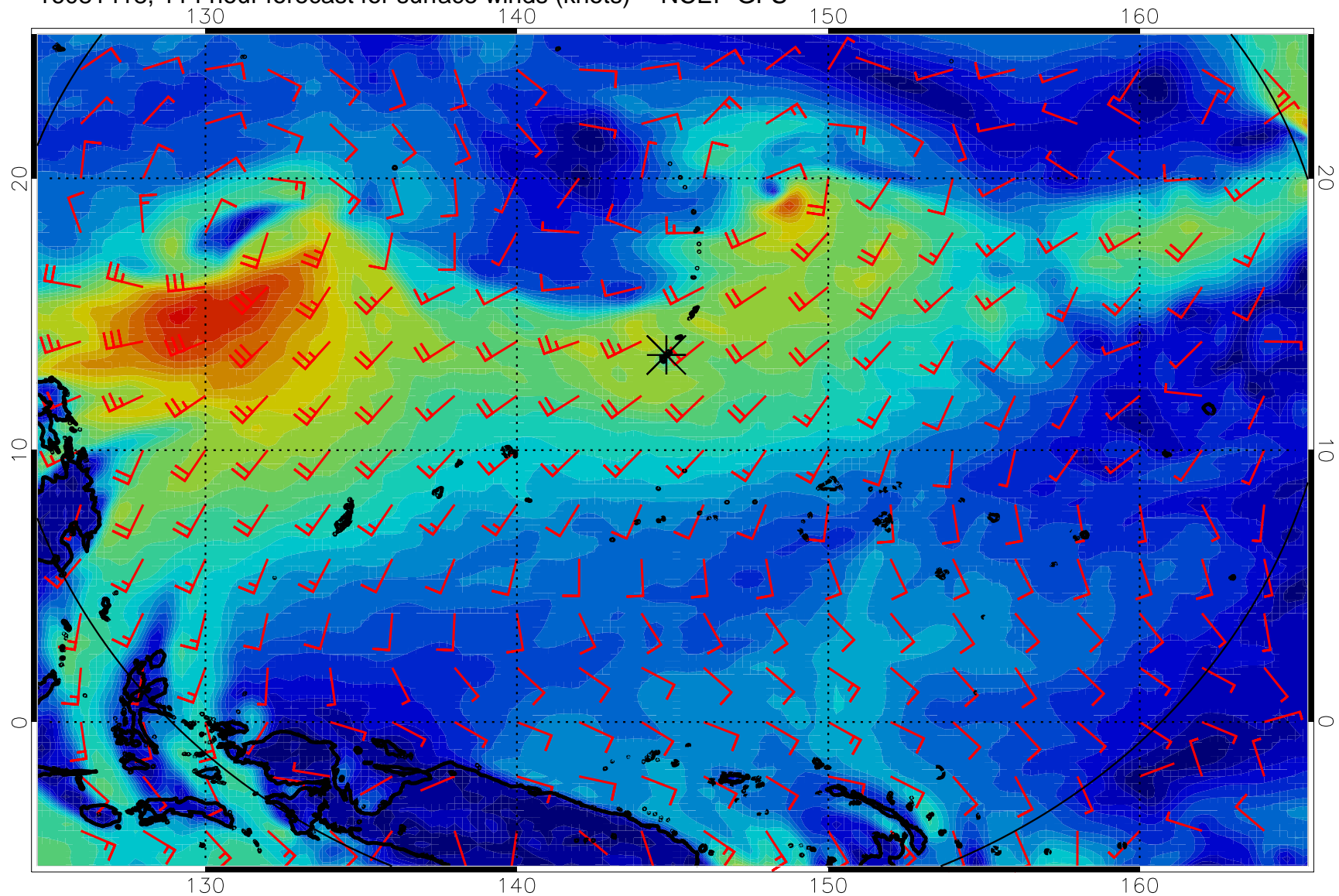
16081418, 114 hour forecast for surface winds (knots) -- NCEP GFS
