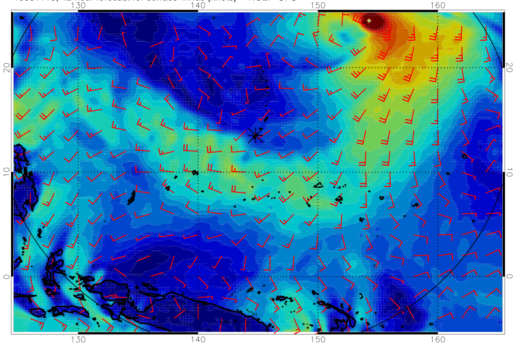
16081118, 42 hour forecast for surface winds (knots) -- NCEP GFS
