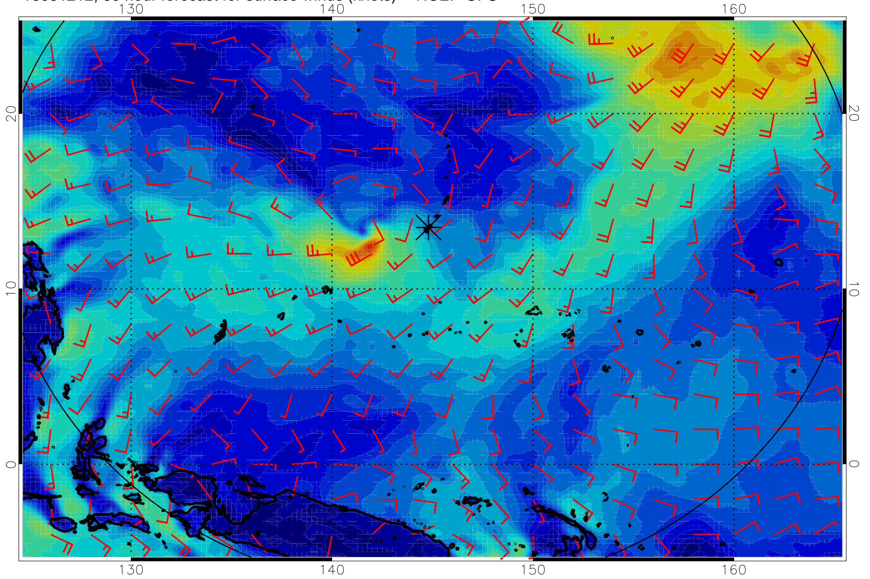
16081212, 60 hour forecast for surface winds (knots) -- NCEP GFS
