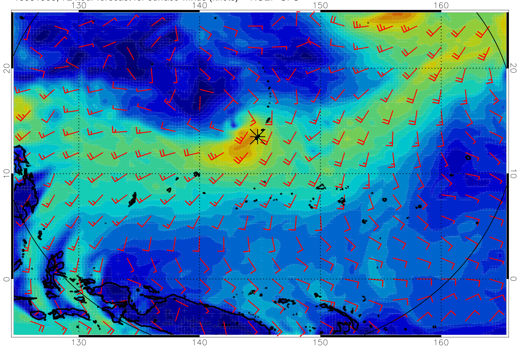
16081300, 72 hour forecast for surface winds (knots) -- NCEP GFS
