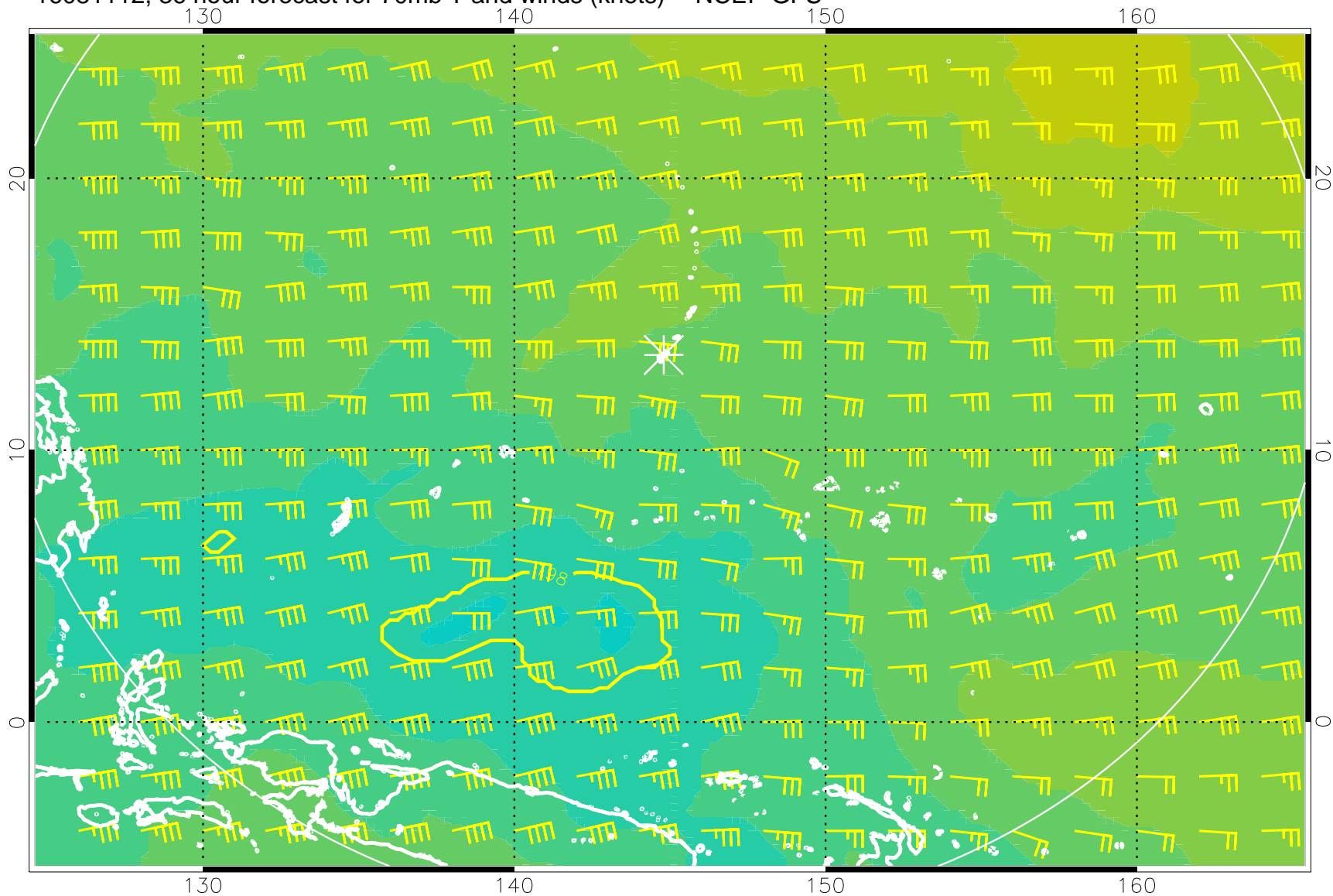
16081112, 36 hour forecast for 70mb T and winds (knots) -- NCEP GFS
