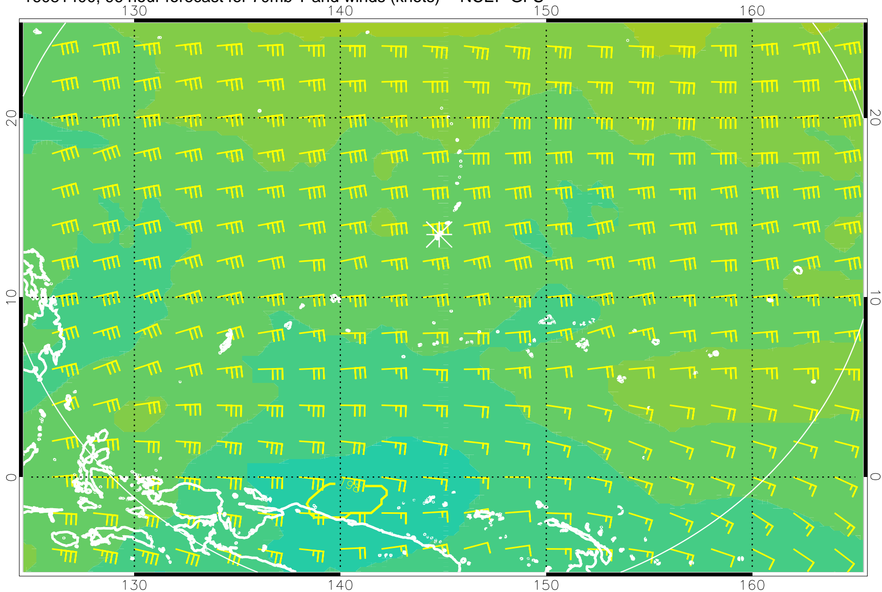
16081400, 96 hour forecast for 70mb T and winds (knots) -- NCEP GFS
