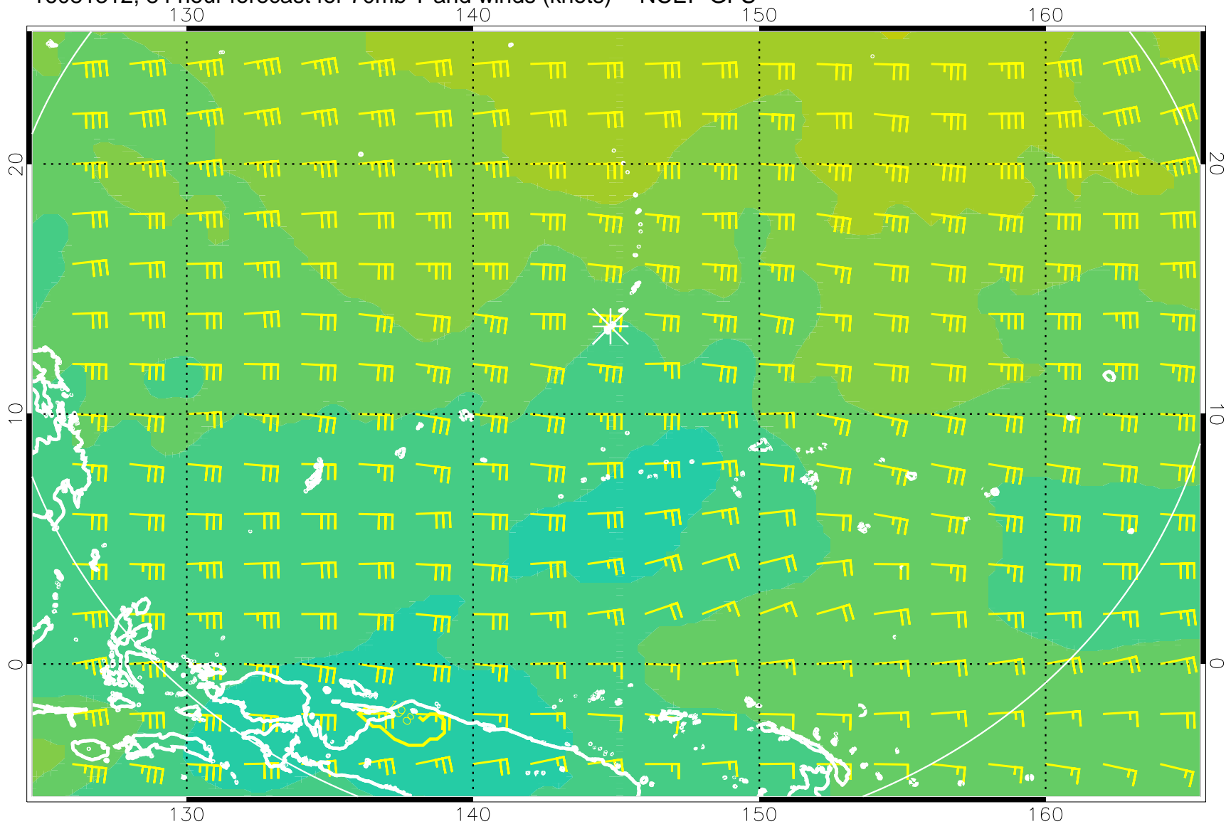
16081312, 84 hour forecast for 70mb T and winds (knots) -- NCEP GFS
