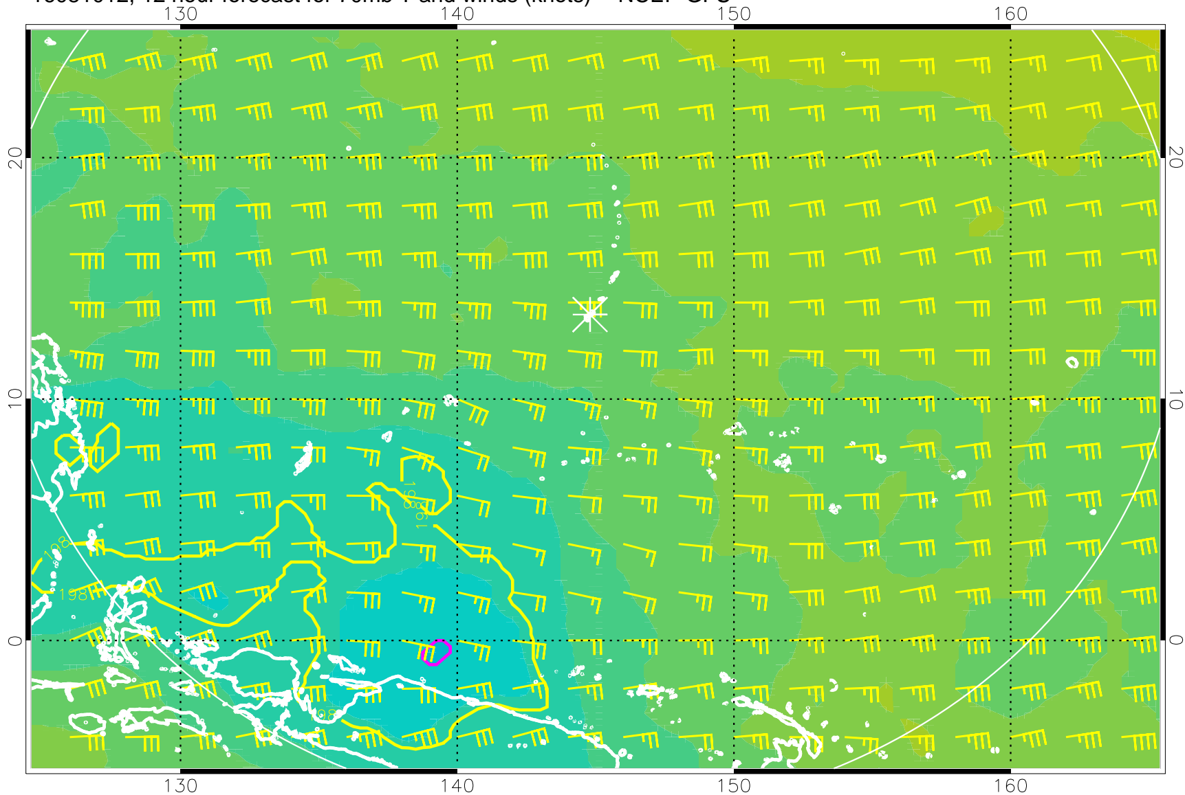
16081012, 12 hour forecast for 70mb T and winds (knots) -- NCEP GFS
