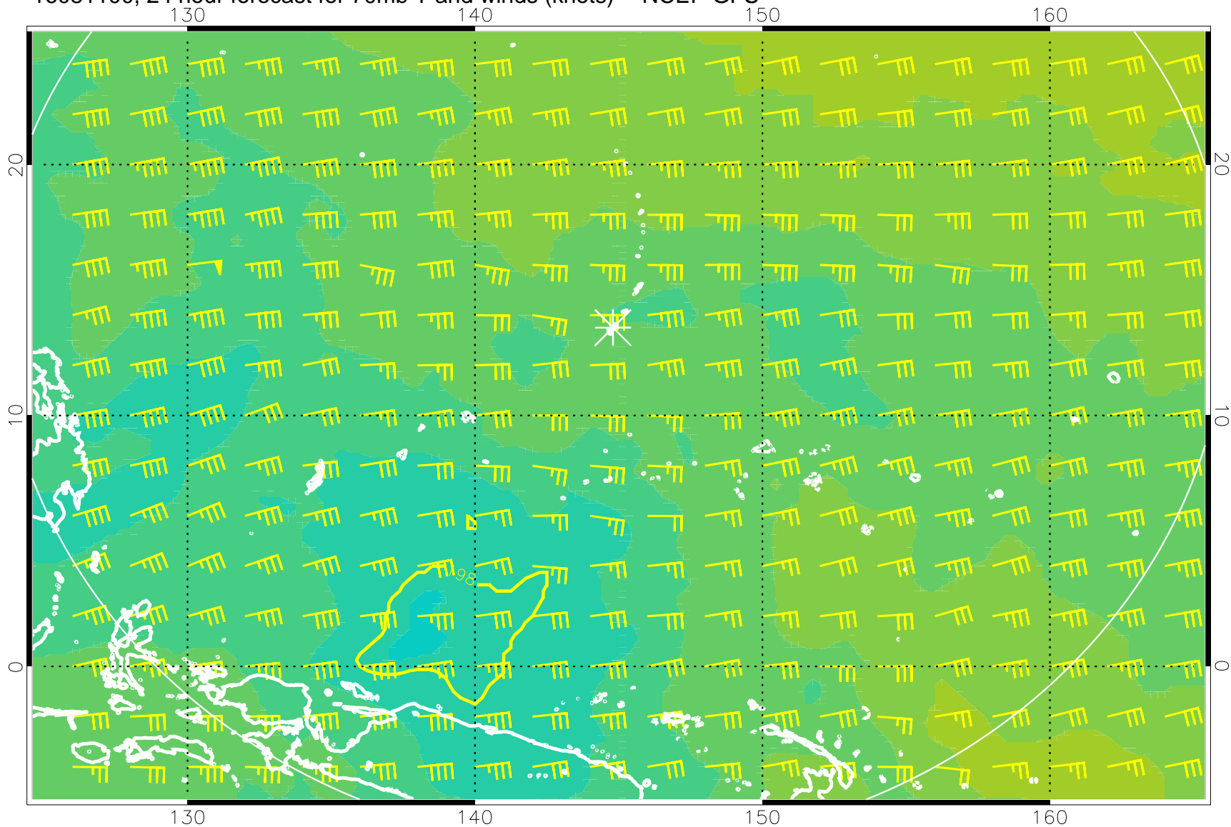
16081100, 24 hour forecast for 70mb T and winds (knots) -- NCEP GFS
