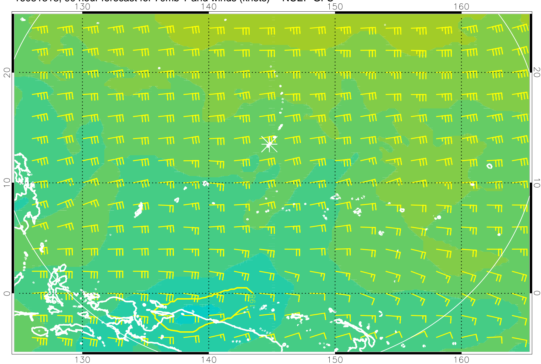
16081318, 90 hour forecast for 70mb T and winds (knots) -- NCEP GFS
