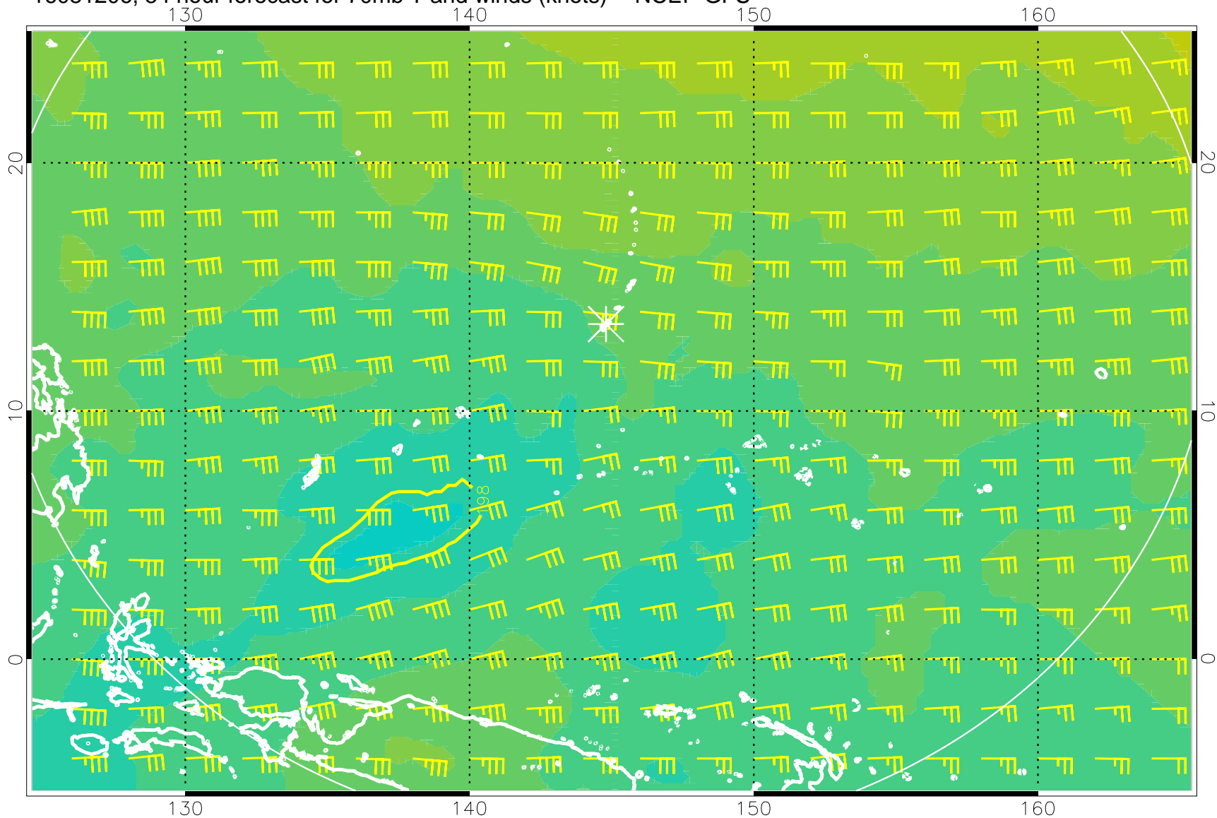
16081206, 54 hour forecast for 70mb T and winds (knots) -- NCEP GFS
