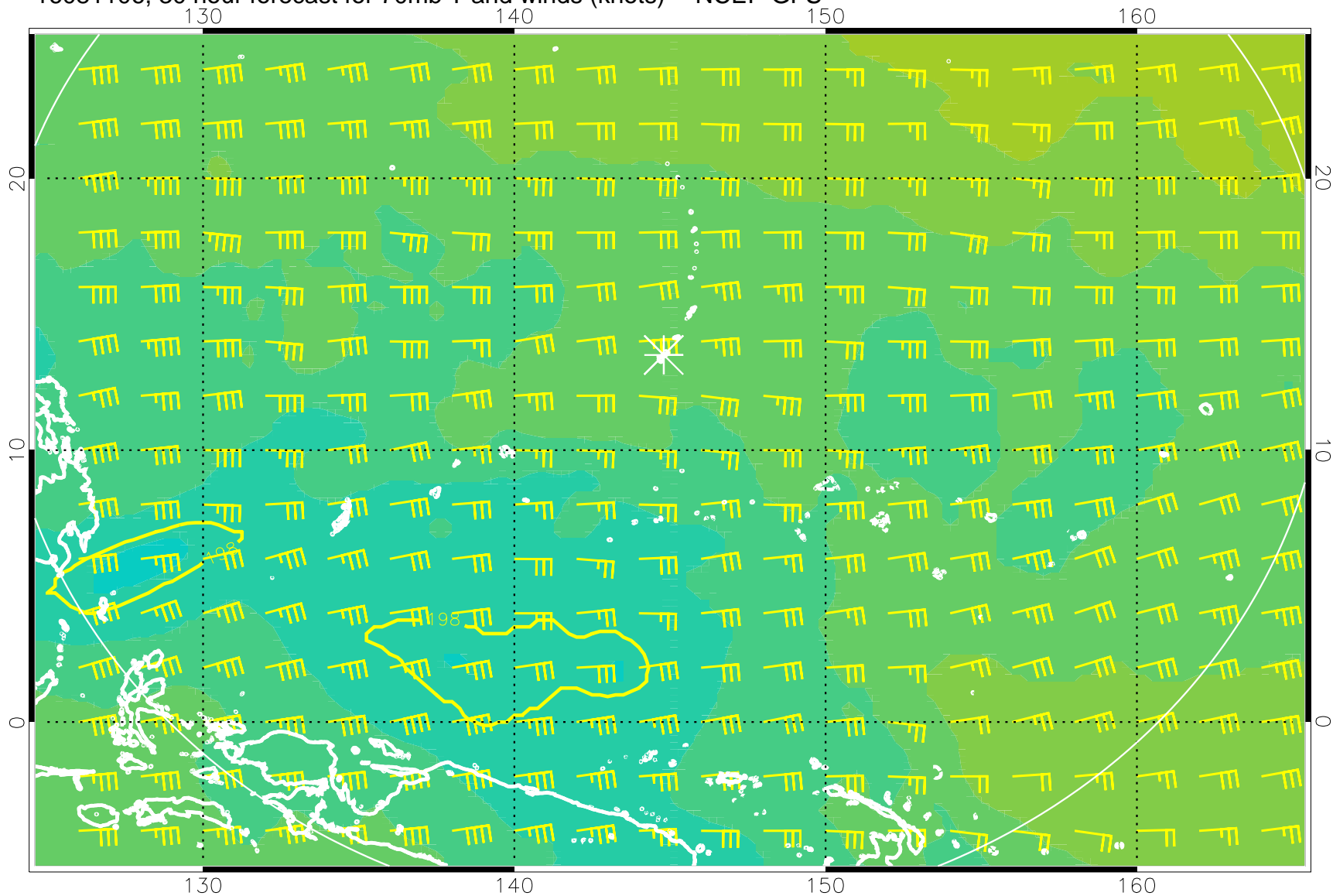
16081106, 30 hour forecast for 70mb T and winds (knots) -- NCEP GFS
