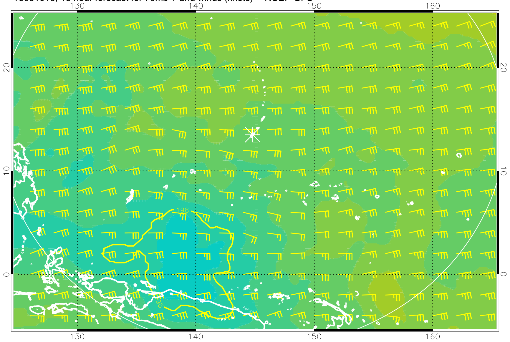
16081018, 18 hour forecast for 70mb T and winds (knots) -- NCEP GFS
