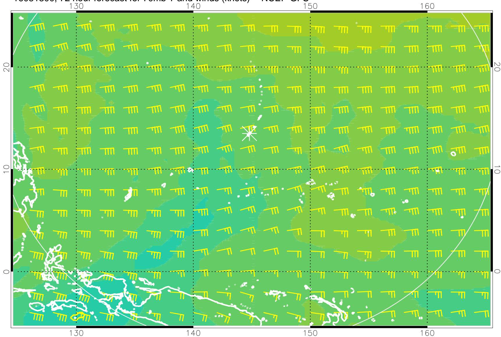
16081300, 72 hour forecast for 70mb T and winds (knots) -- NCEP GFS
