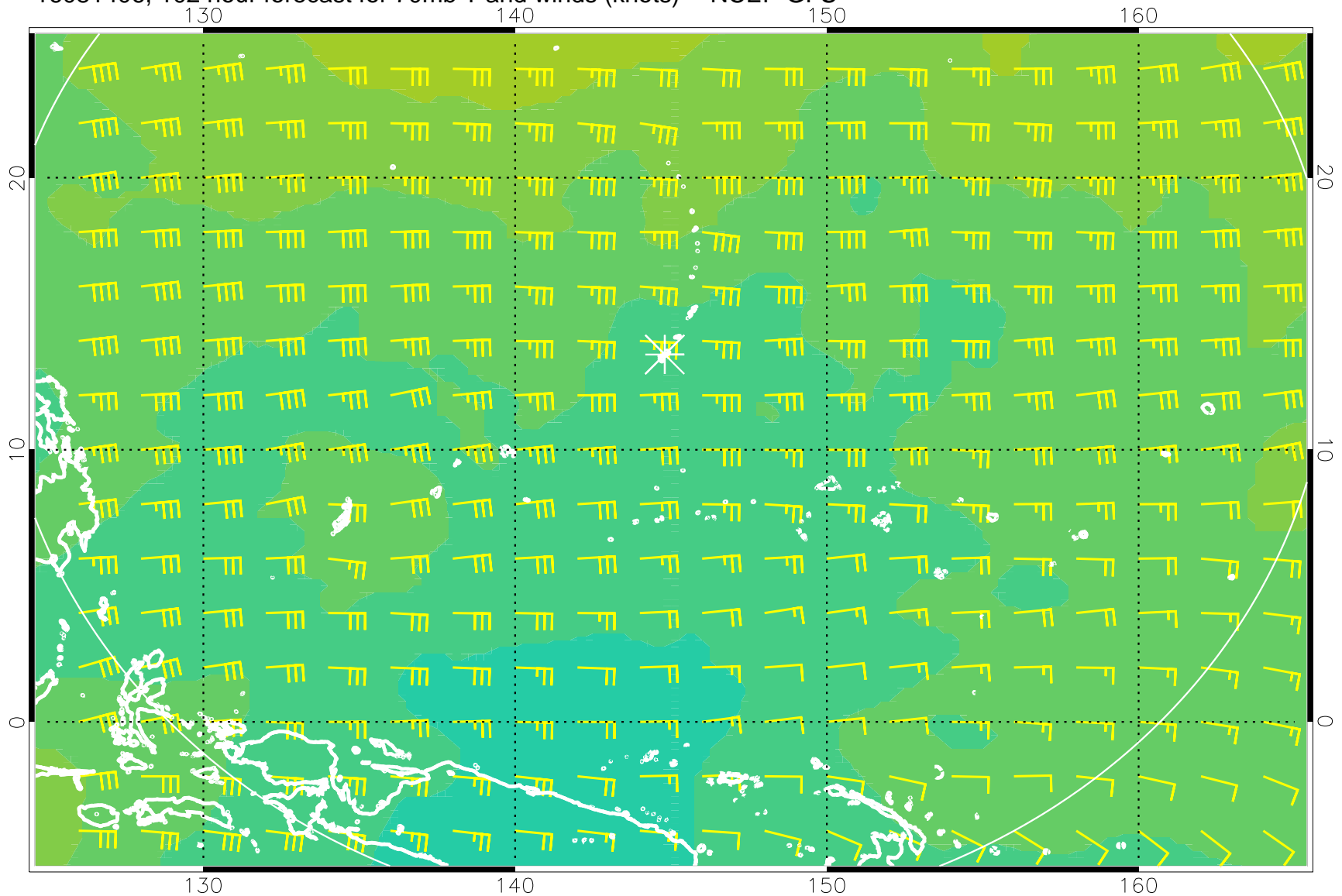
16081406, 102 hour forecast for 70mb T and winds (knots) -- NCEP GFS
