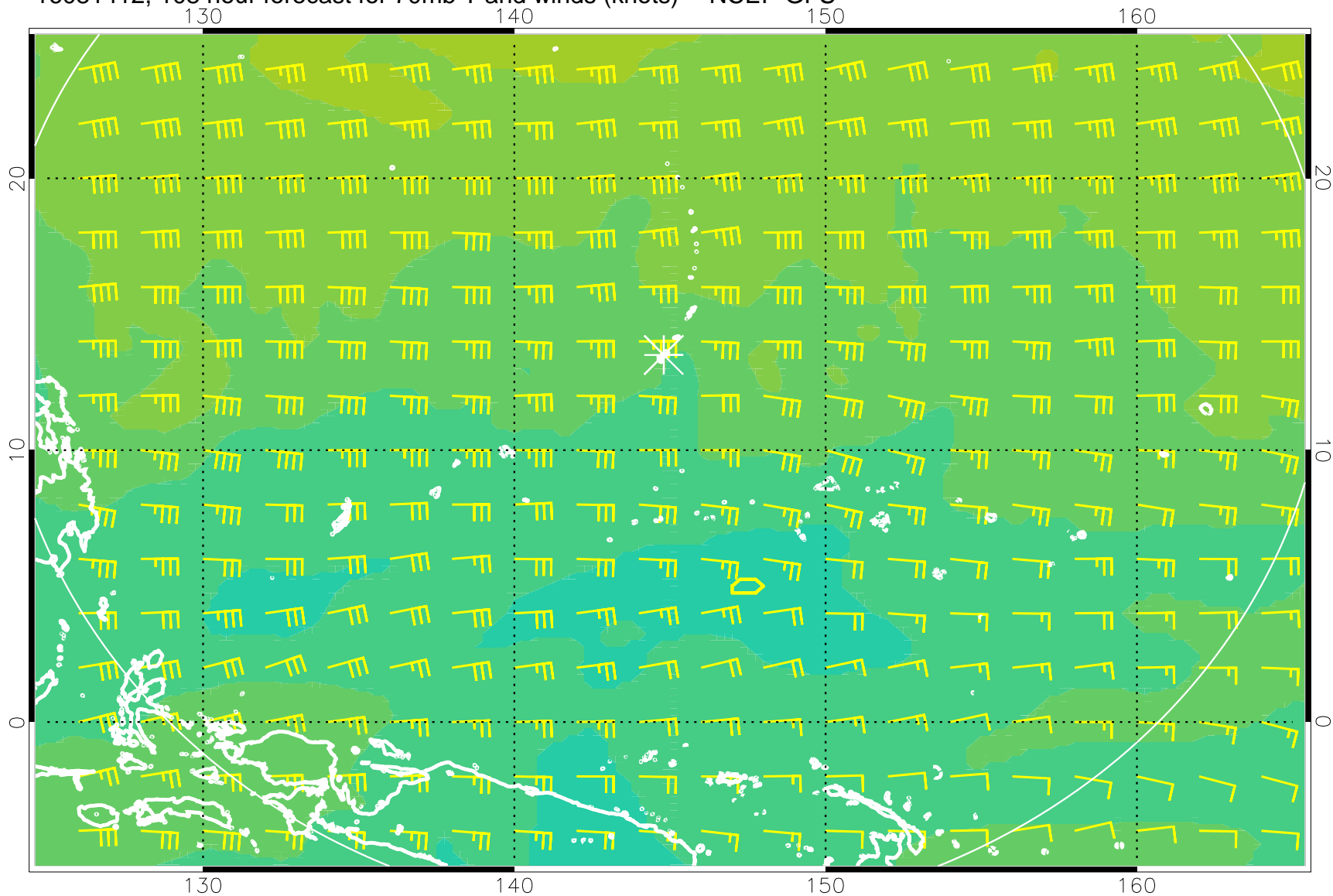
16081412, 108 hour forecast for 70mb T and winds (knots) -- NCEP GFS
