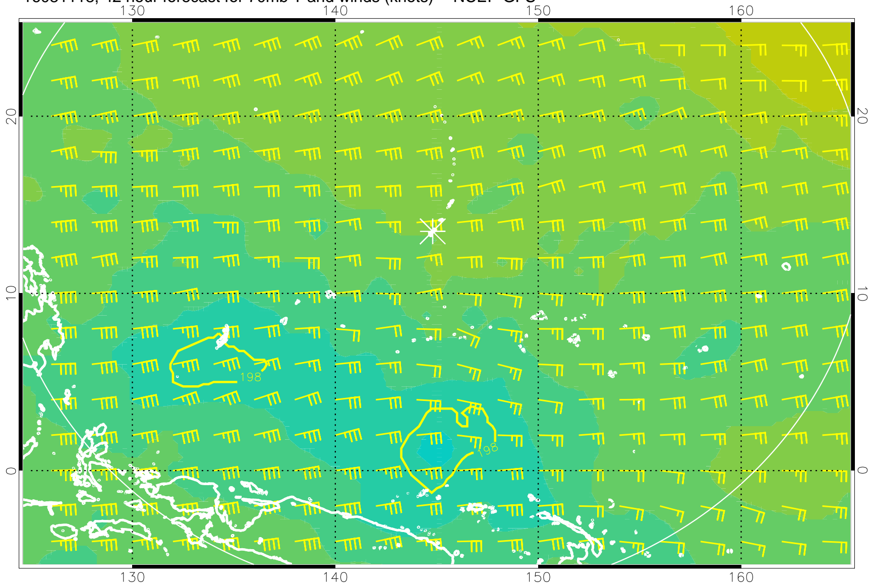
16081118, 42 hour forecast for 70mb T and winds (knots) -- NCEP GFS
