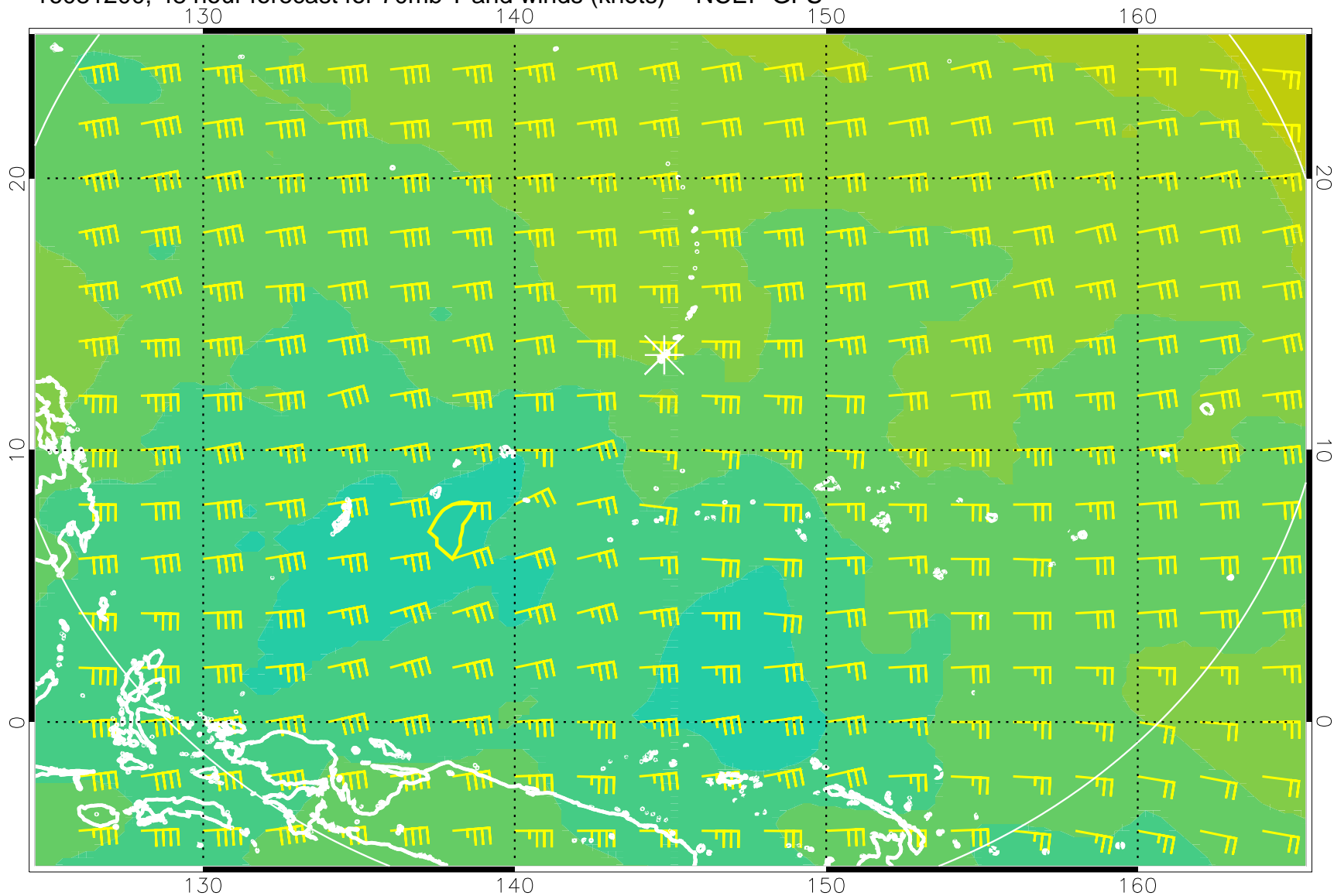
16081200, 48 hour forecast for 70mb T and winds (knots) -- NCEP GFS
