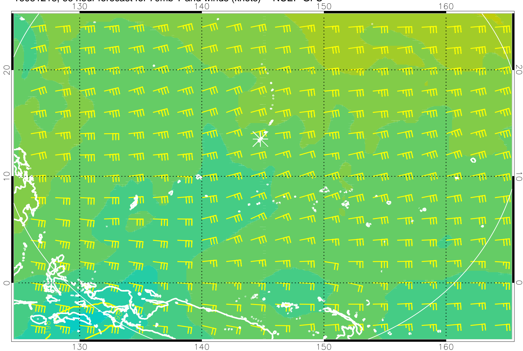
16081218, 66 hour forecast for 70mb T and winds (knots) -- NCEP GFS
