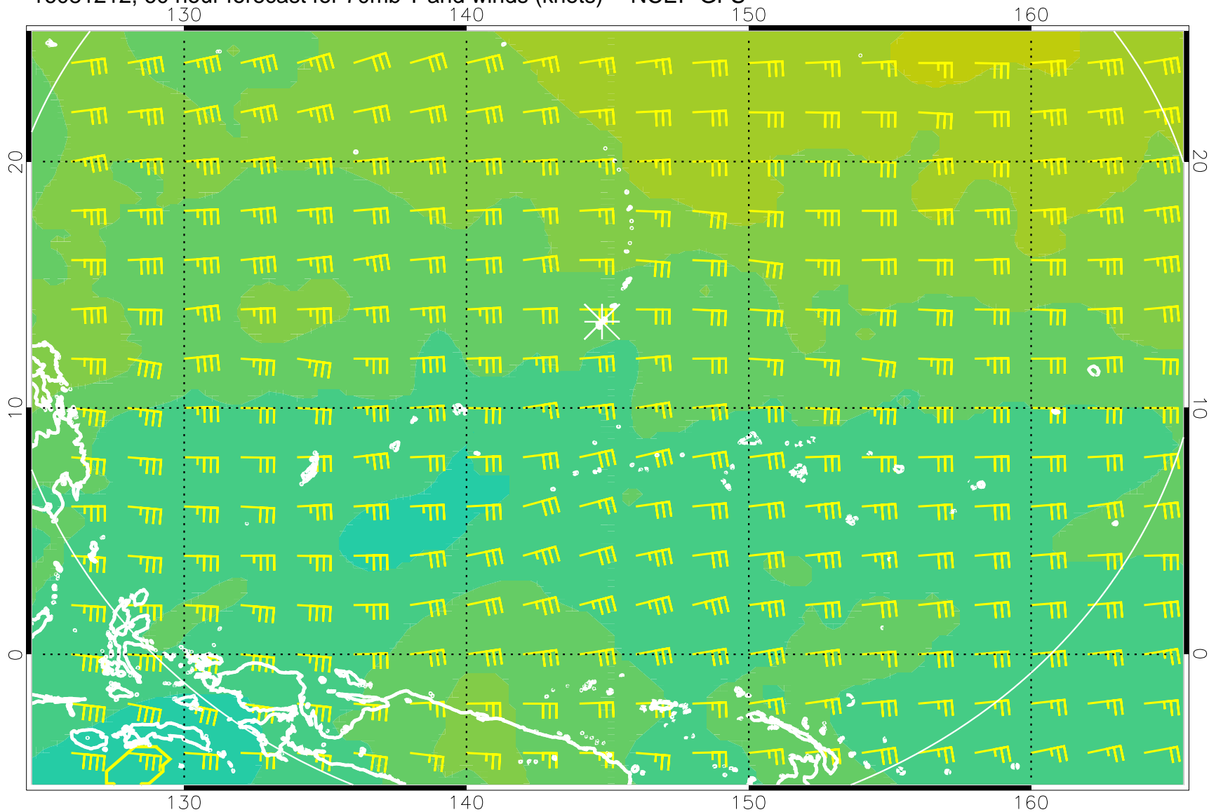
16081212, 60 hour forecast for 70mb T and winds (knots) -- NCEP GFS
