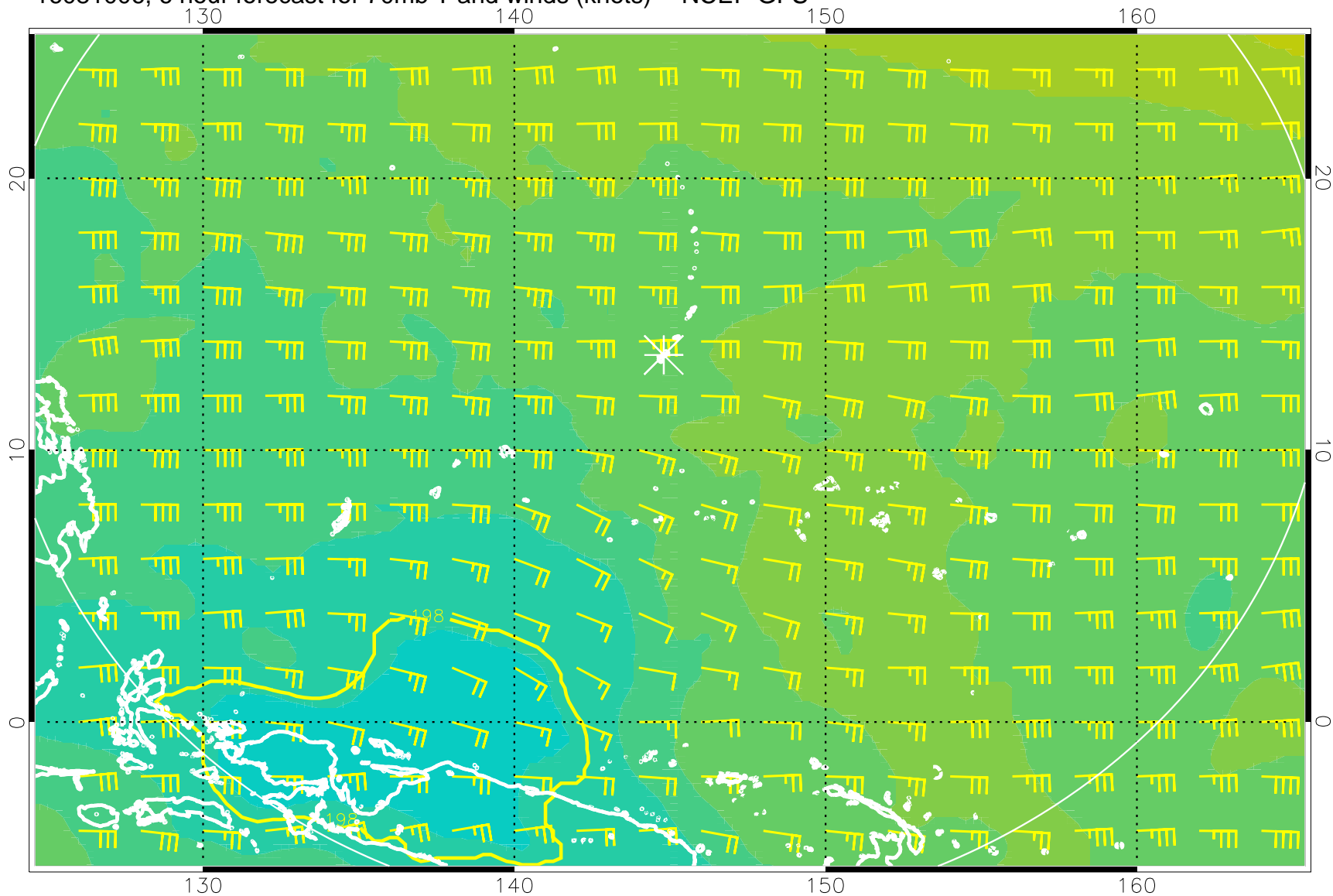
16081006, 6 hour forecast for 70mb T and winds (knots) -- NCEP GFS
