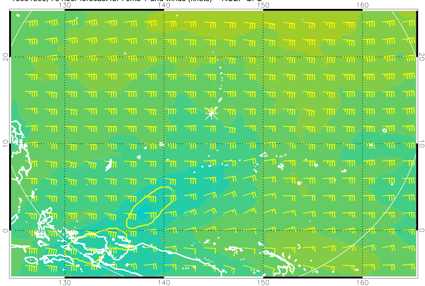
16081306, 78 hour forecast for 70mb T and winds (knots) -- NCEP GFS
