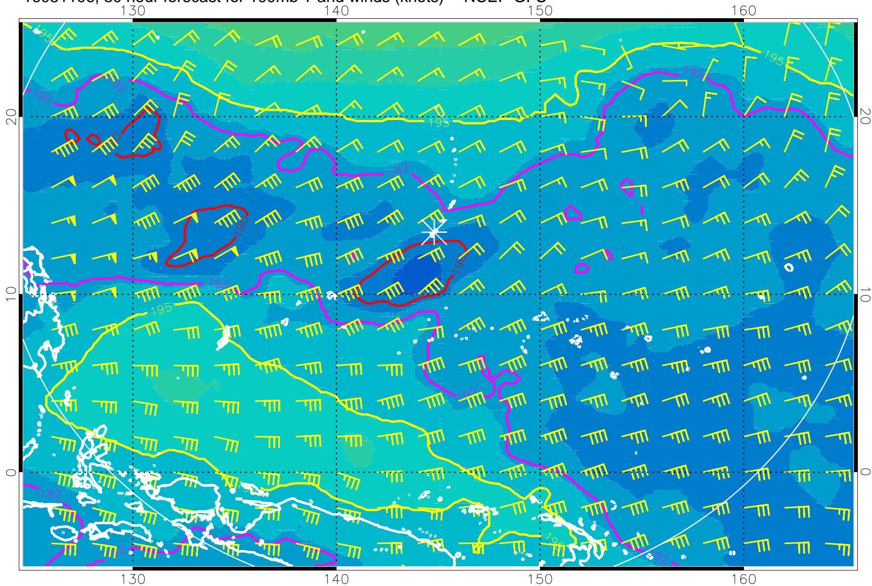
16081106, 30 hour forecast for 100mb T and winds (knots) -- NCEP GFS
