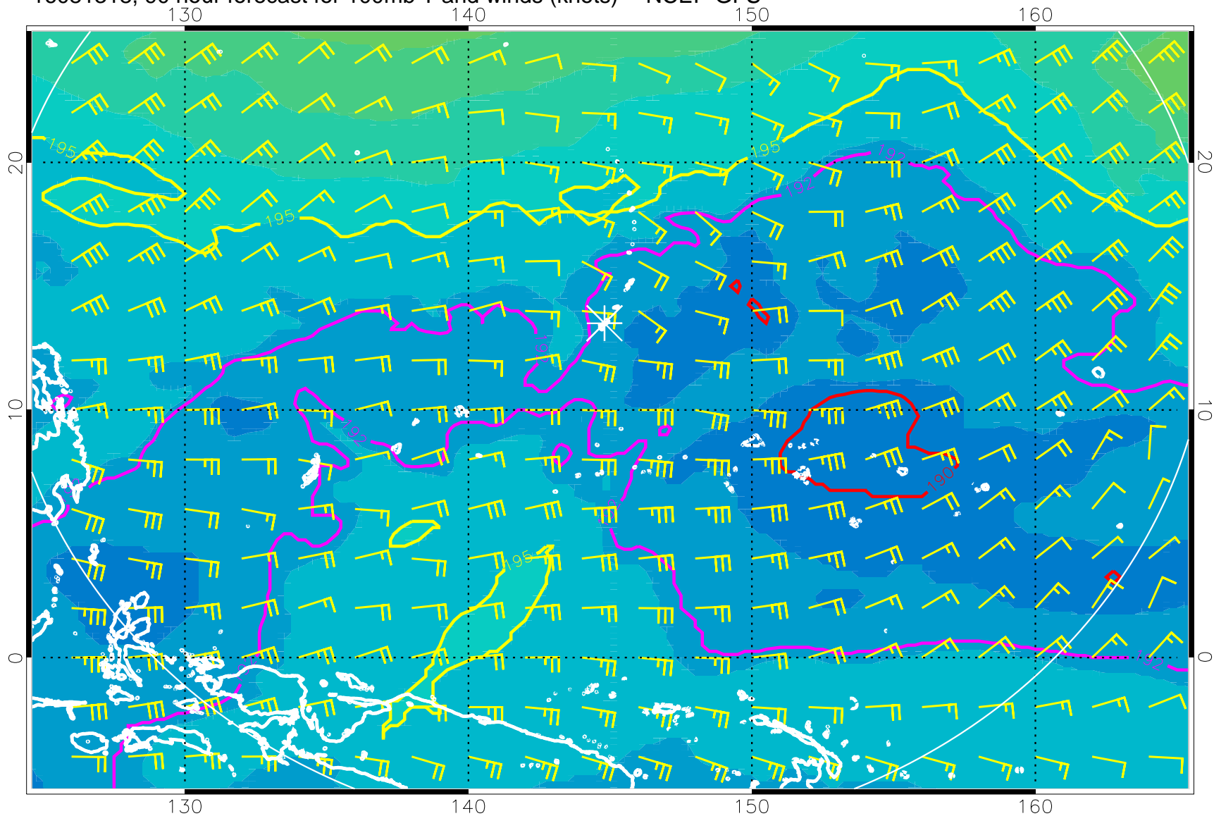
16081318, 90 hour forecast for 100mb T and winds (knots) -- NCEP GFS
