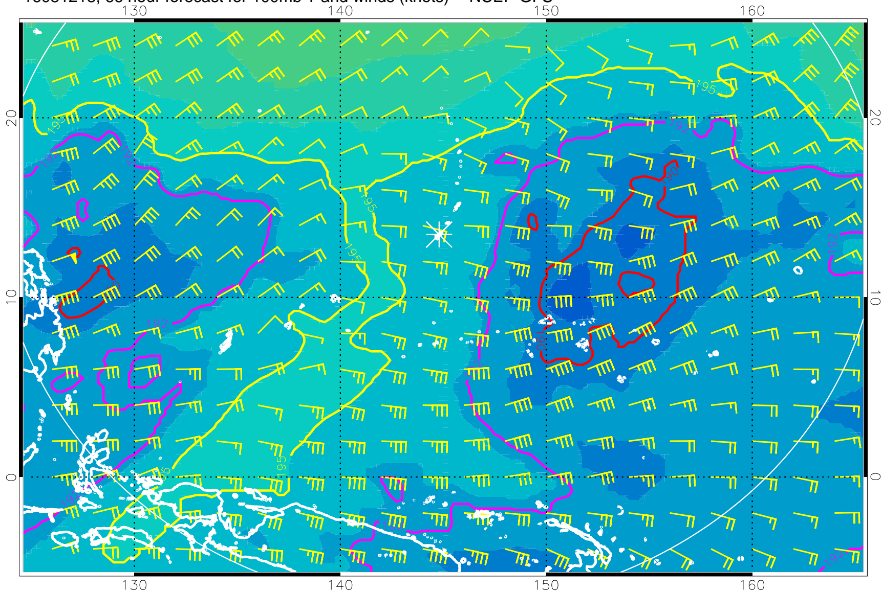
16081218, 66 hour forecast for 100mb T and winds (knots) -- NCEP GFS
