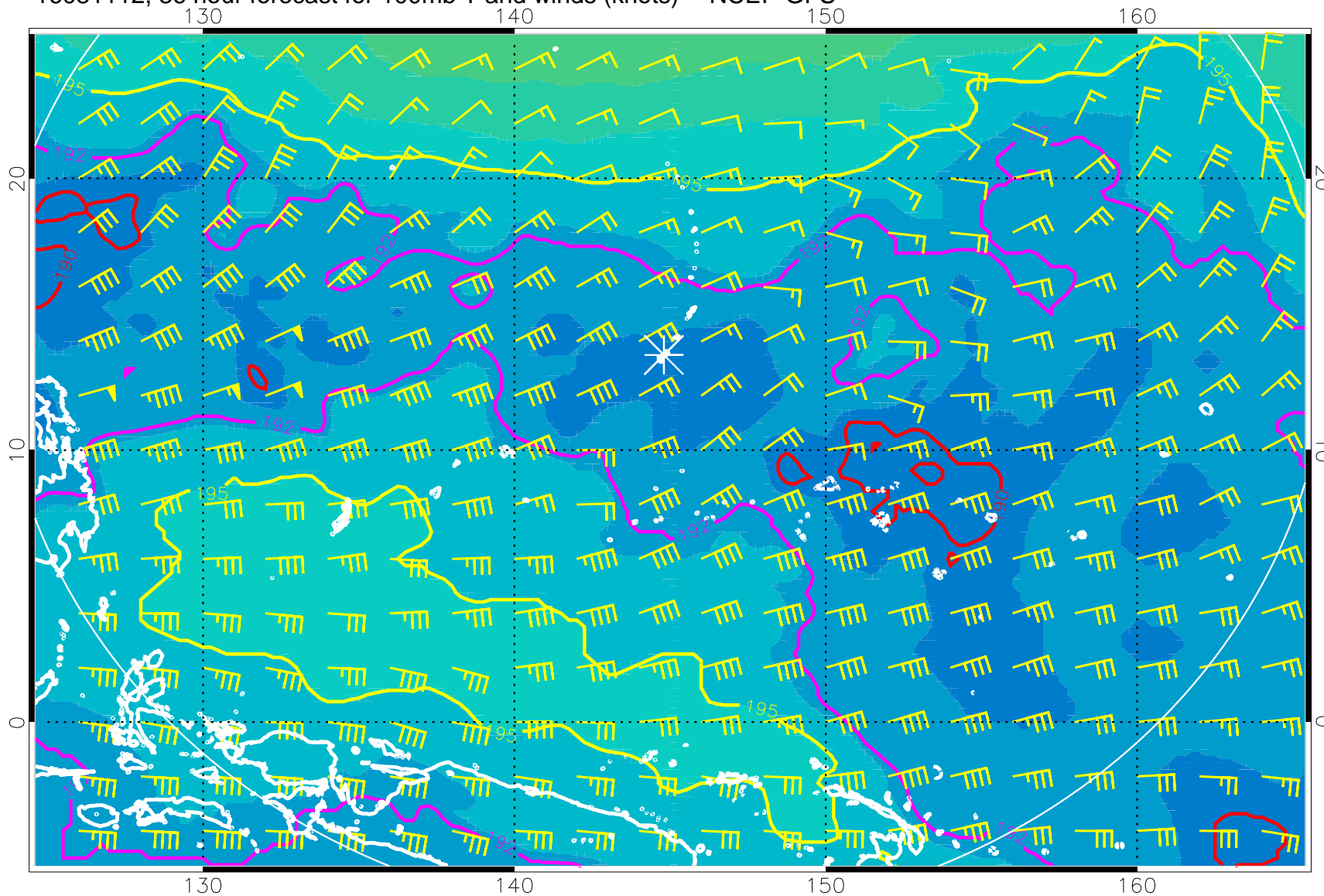
16081112, 36 hour forecast for 100mb T and winds (knots) -- NCEP GFS
