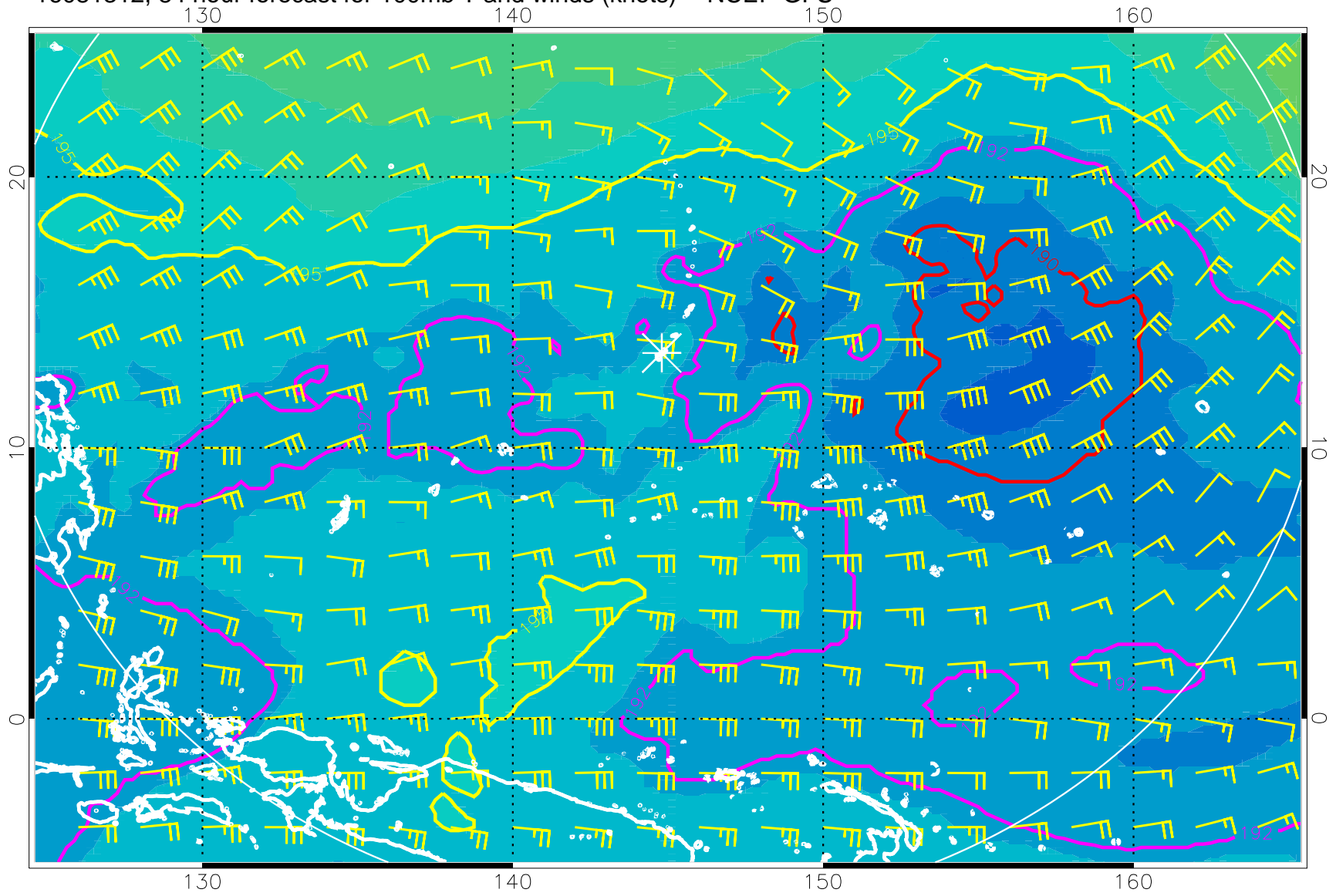
16081312, 84 hour forecast for 100mb T and winds (knots) -- NCEP GFS
