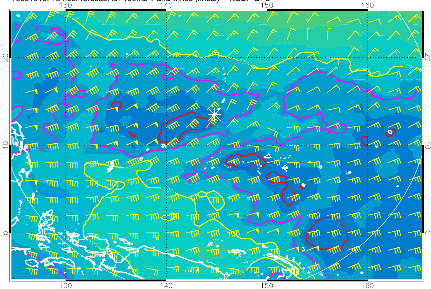
16081018, 18 hour forecast for 100mb T and winds (knots) -- NCEP GFS
