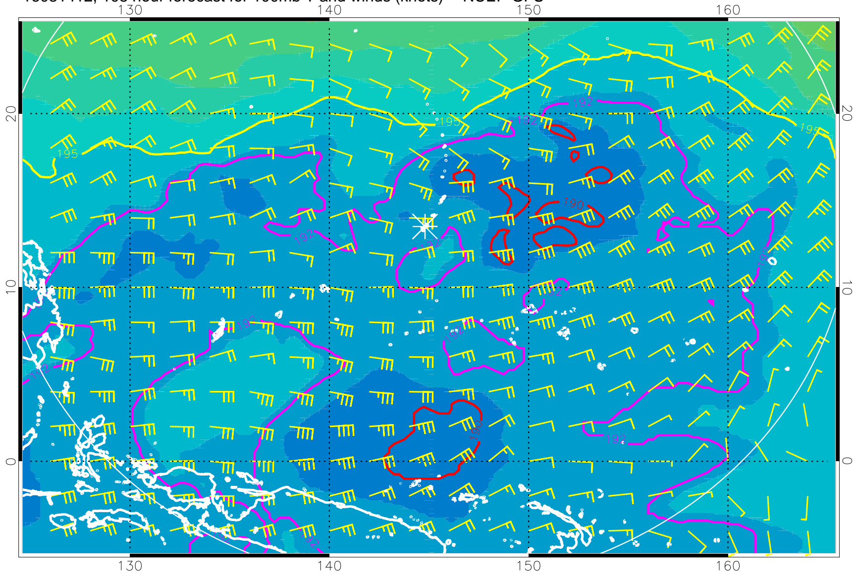
16081412, 108 hour forecast for 100mb T and winds (knots) -- NCEP GFS
