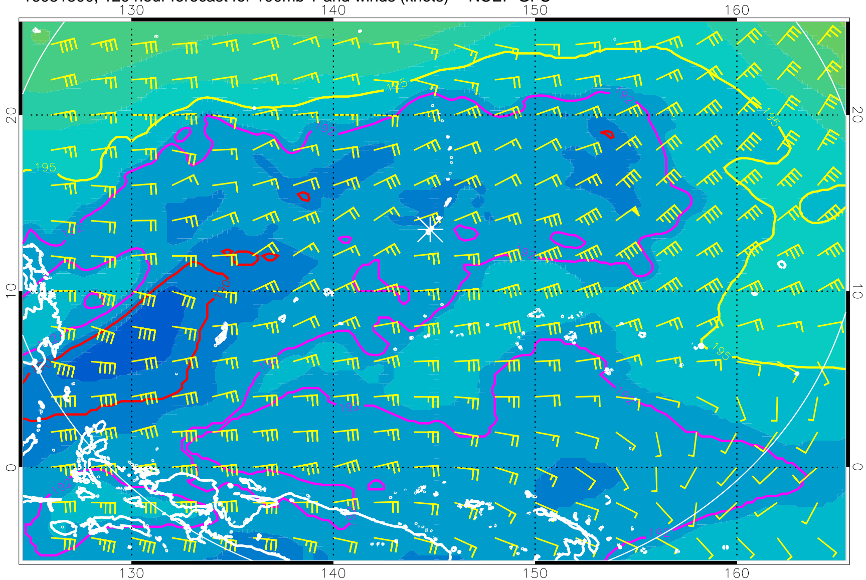
16081500, 120 hour forecast for 100mb T and winds (knots) -- NCEP GFS
