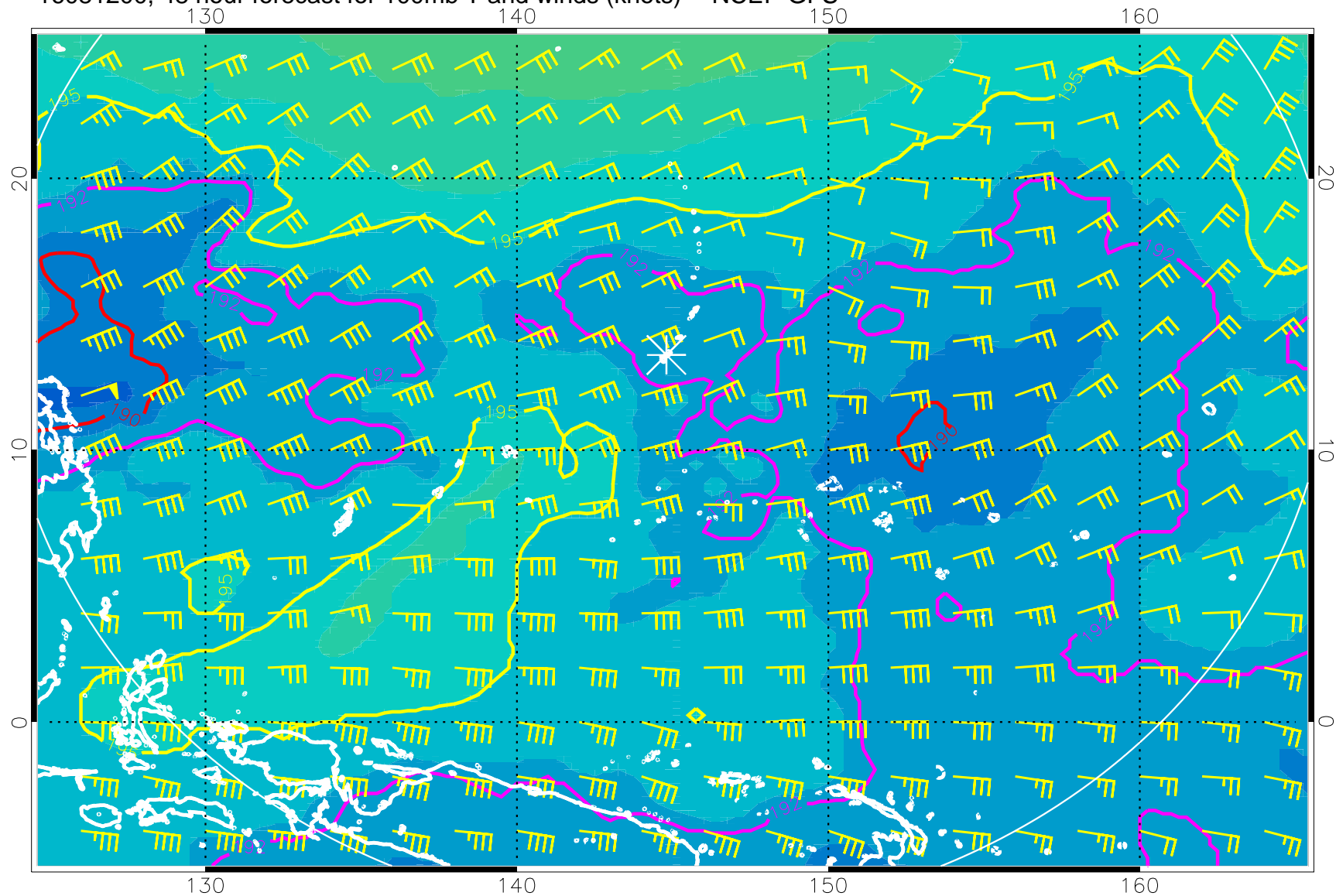
16081200, 48 hour forecast for 100mb T and winds (knots) -- NCEP GFS
