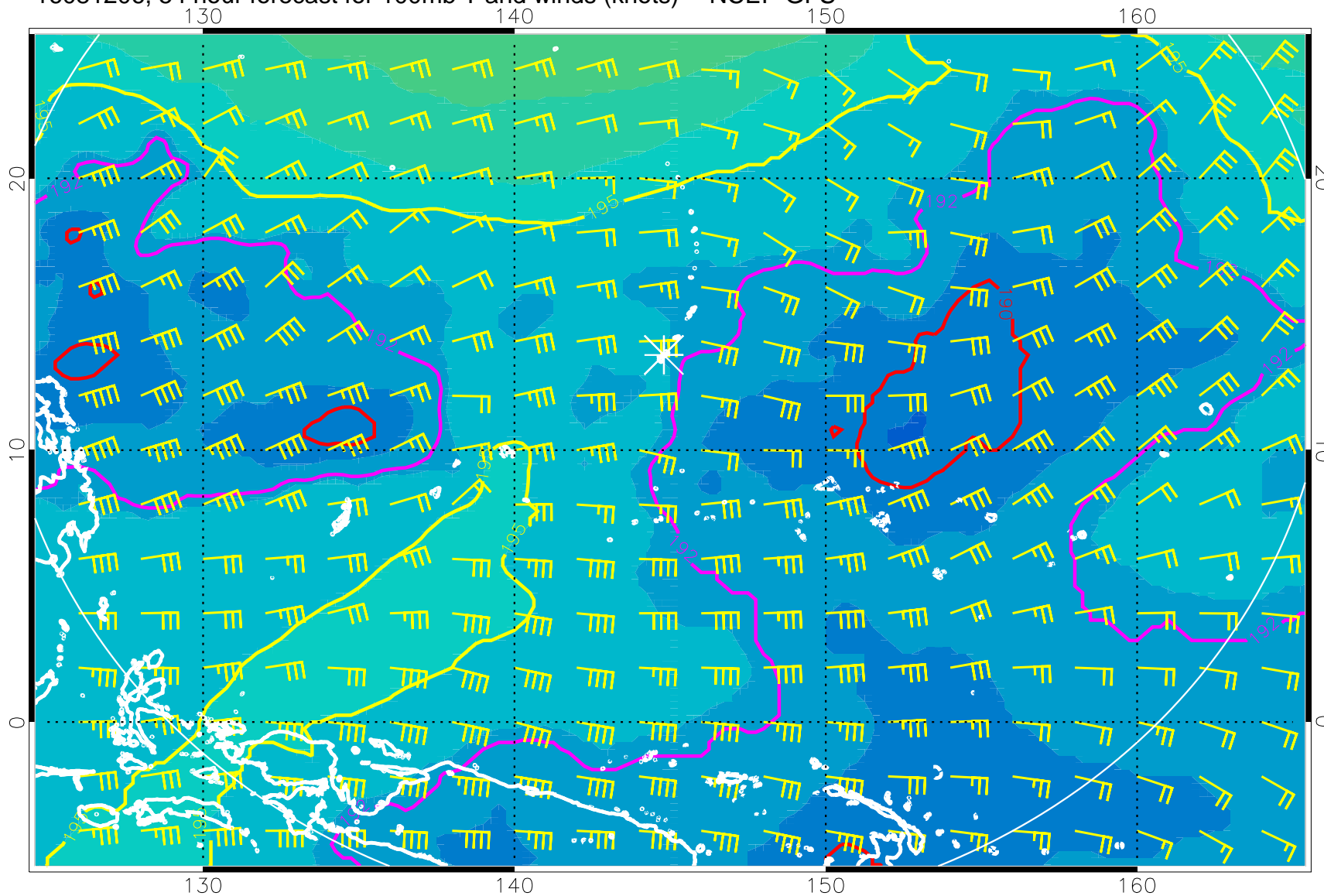
16081206, 54 hour forecast for 100mb T and winds (knots) -- NCEP GFS
