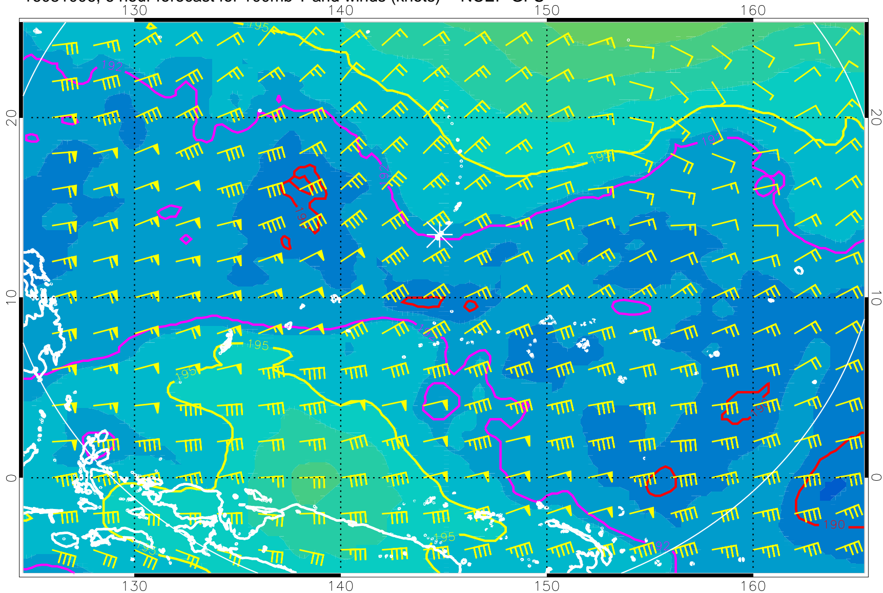
16081006, 6 hour forecast for 100mb T and winds (knots) -- NCEP GFS
