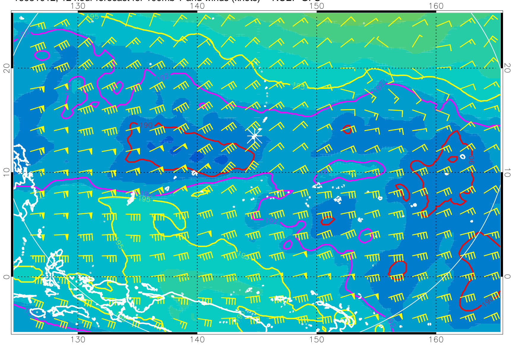
16081012, 12 hour forecast for 100mb T and winds (knots) -- NCEP GFS
