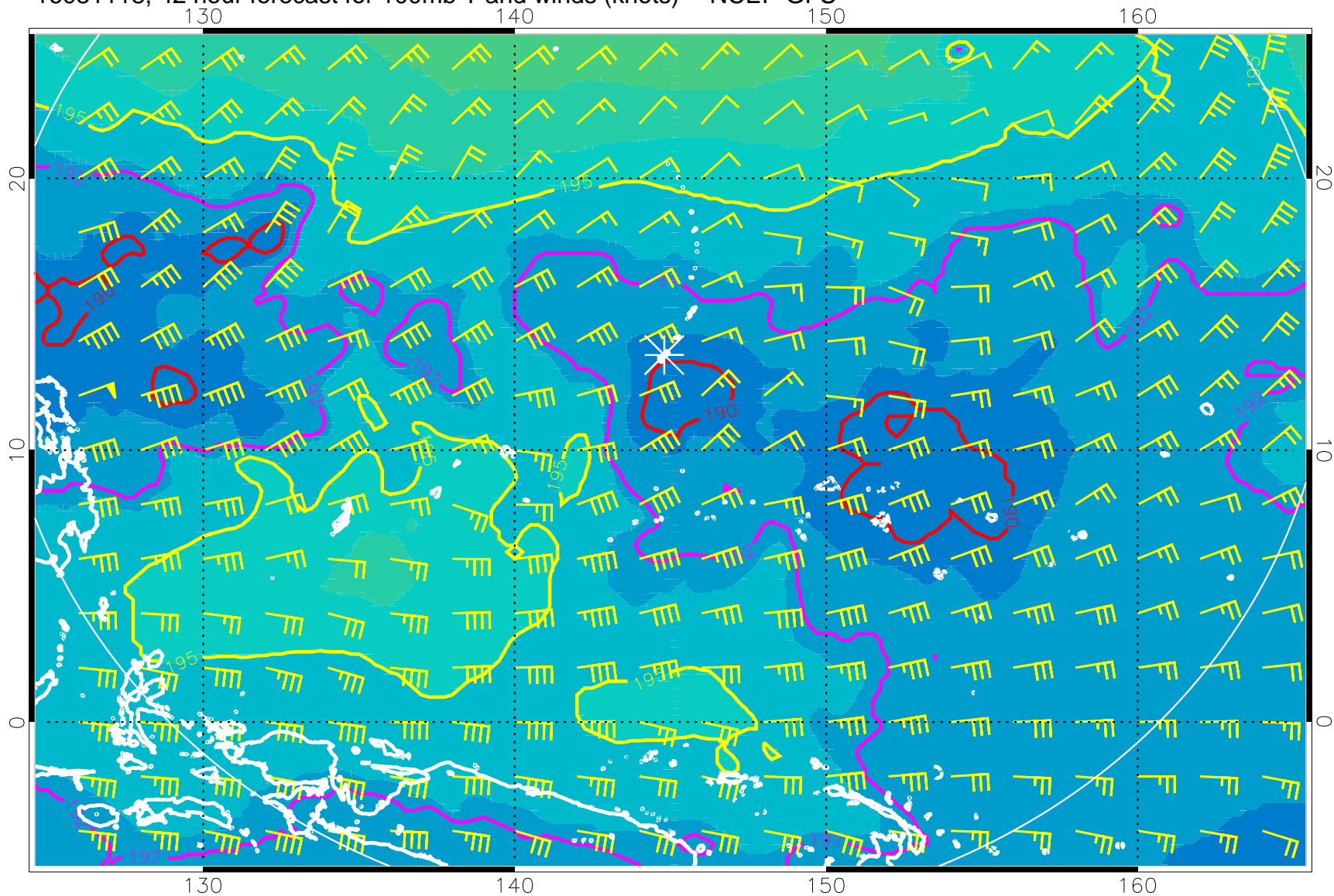
16081118, 42 hour forecast for 100mb T and winds (knots) -- NCEP GFS
