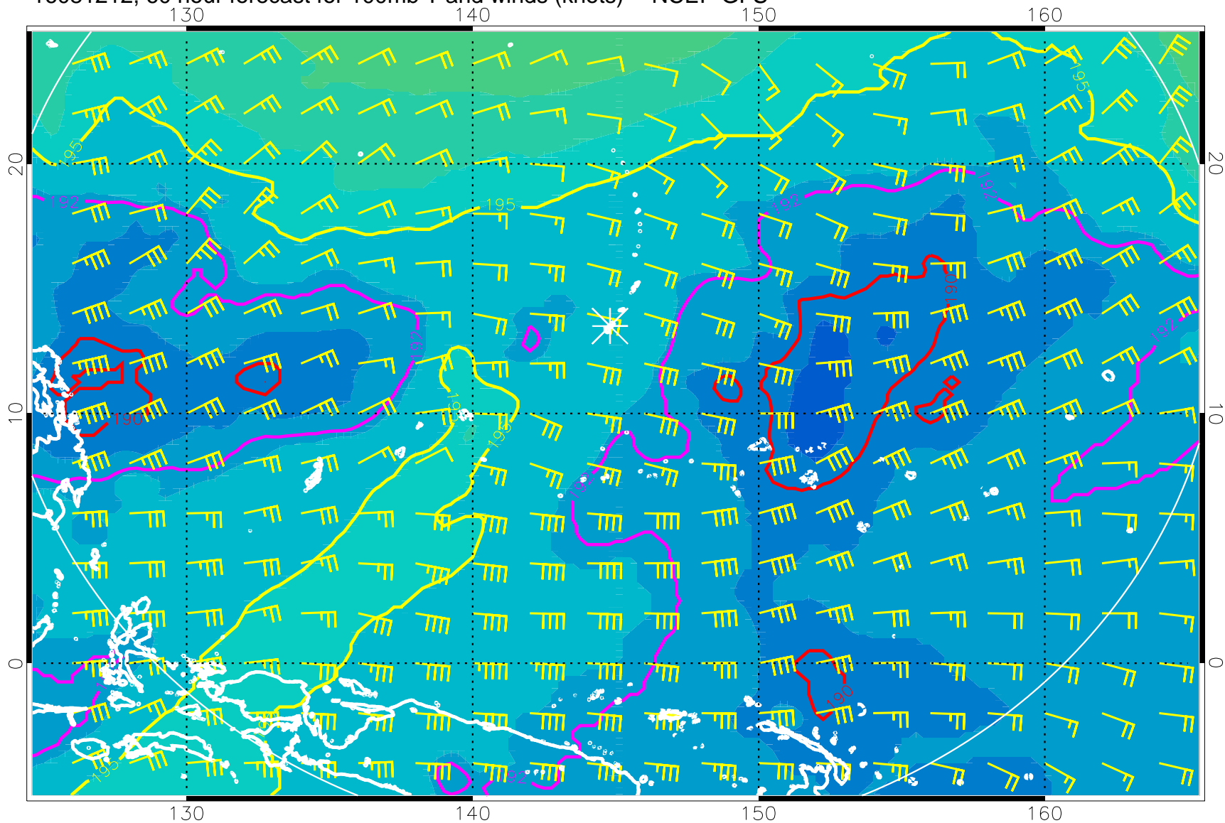
16081212, 60 hour forecast for 100mb T and winds (knots) -- NCEP GFS
