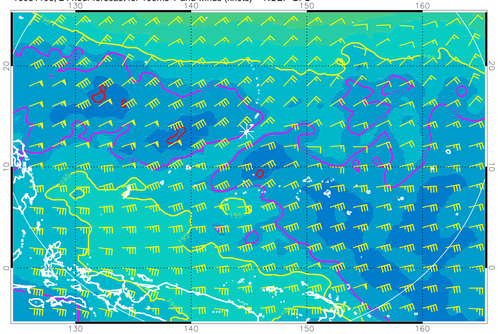
16081100, 24 hour forecast for 100mb T and winds (knots) -- NCEP GFS
