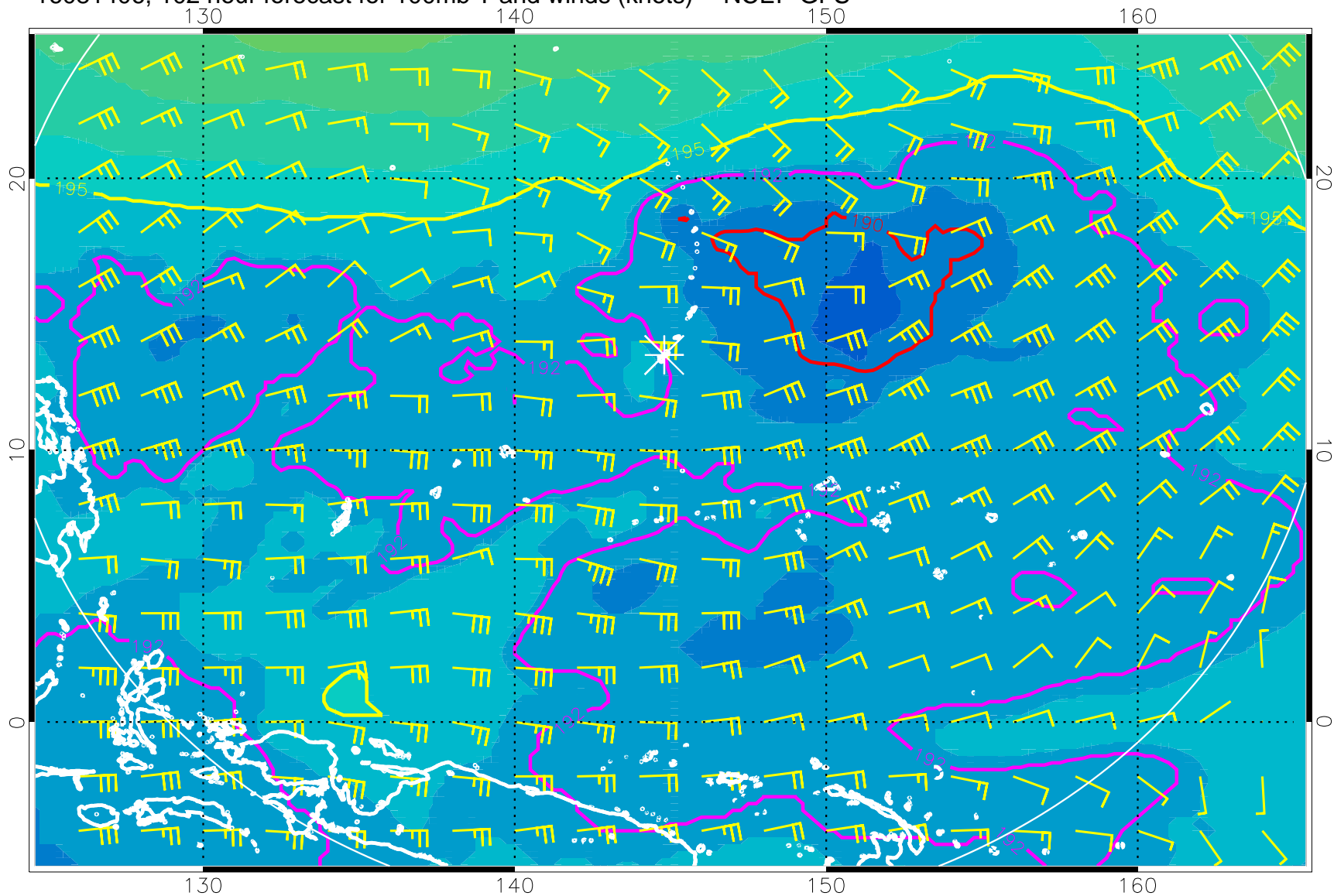
16081406, 102 hour forecast for 100mb T and winds (knots) -- NCEP GFS
