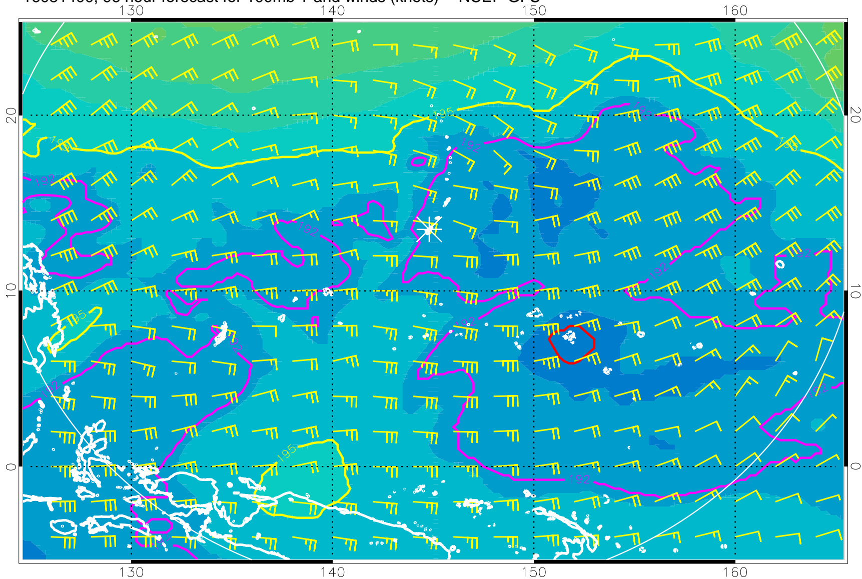
16081400, 96 hour forecast for 100mb T and winds (knots) -- NCEP GFS
