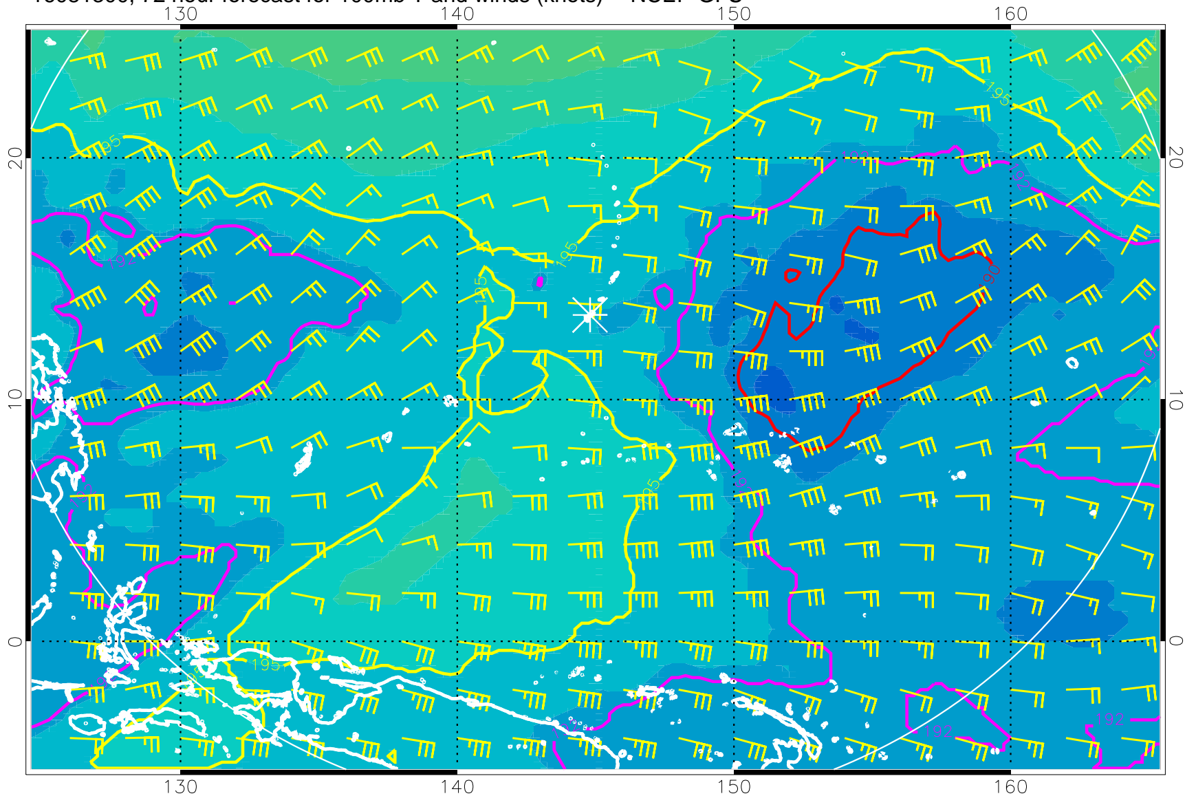
16081300, 72 hour forecast for 100mb T and winds (knots) -- NCEP GFS
