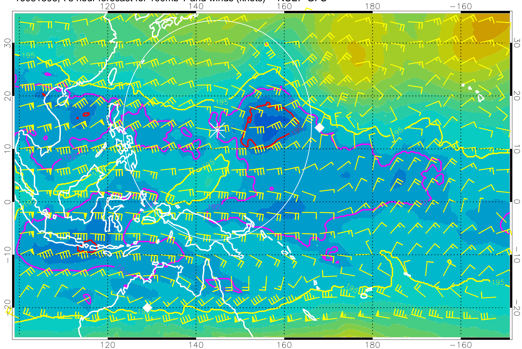
16081306, 78 hour forecast for 100mb T and winds (knots) -- NCEP GFS
