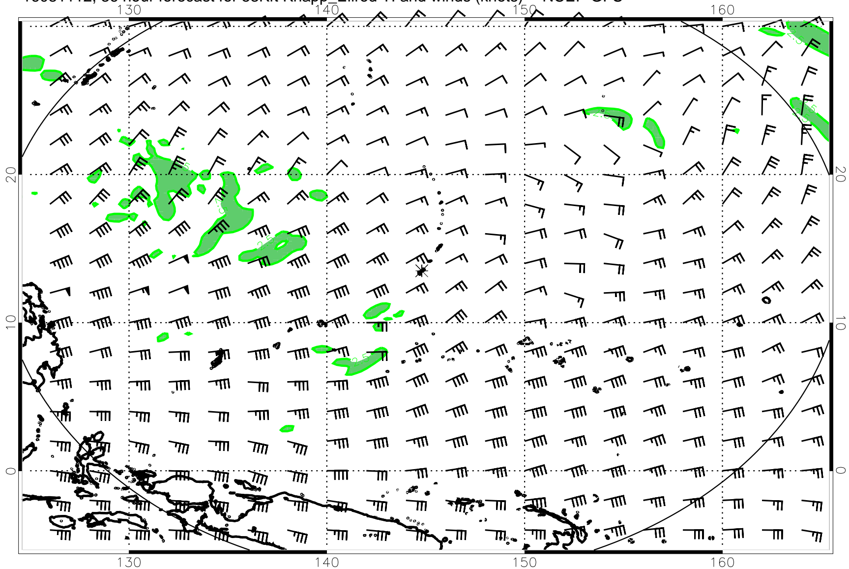
16081112, 36 hour forecast for 53Kft Knapp_Ellrod TI and winds (knots) -- NCEP GFS
