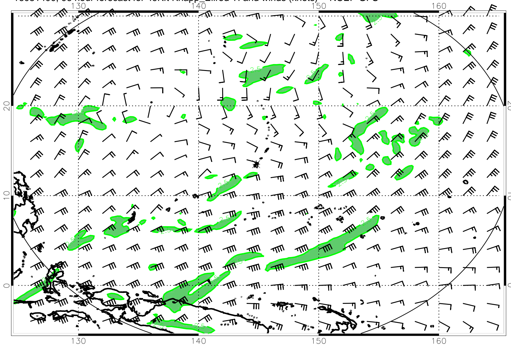
16081400, 96 hour forecast for 49Kft Knapp_Ellrod TI and winds (knots) -- NCEP GFS
