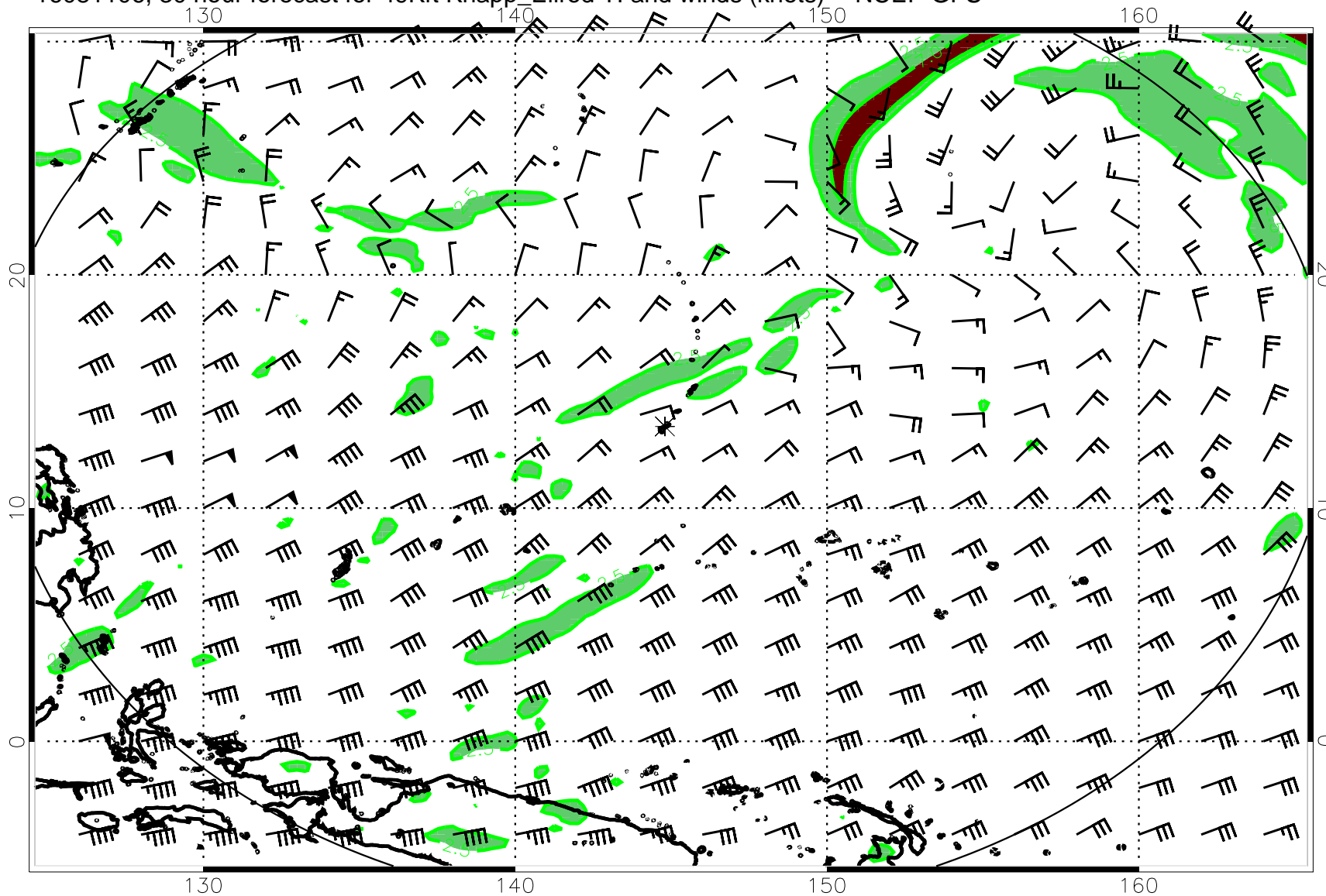
16081106, 30 hour forecast for 49Kft Knapp_Ellrod TI and winds (knots) -- NCEP GFS
