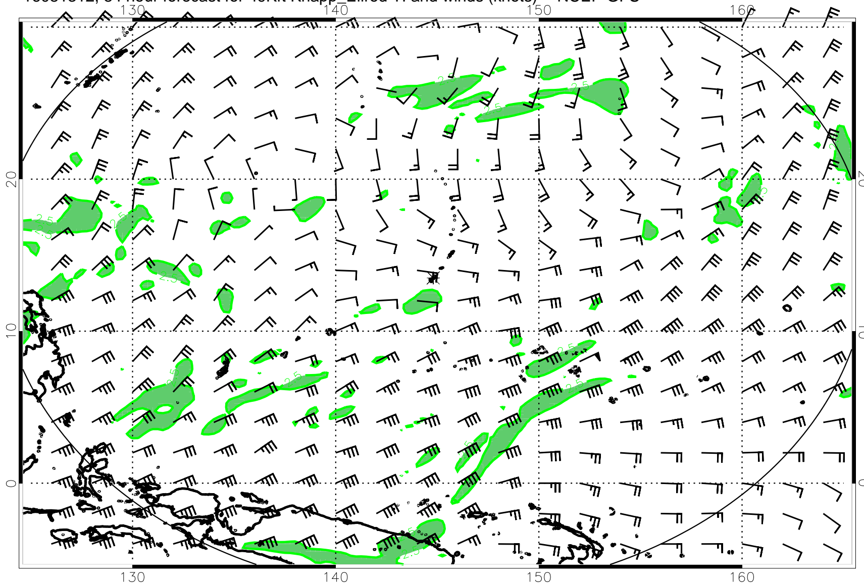
16081312, 84 hour forecast for 49Kft Knapp_Ellrod TI and winds (knots) -- NCEP GFS
