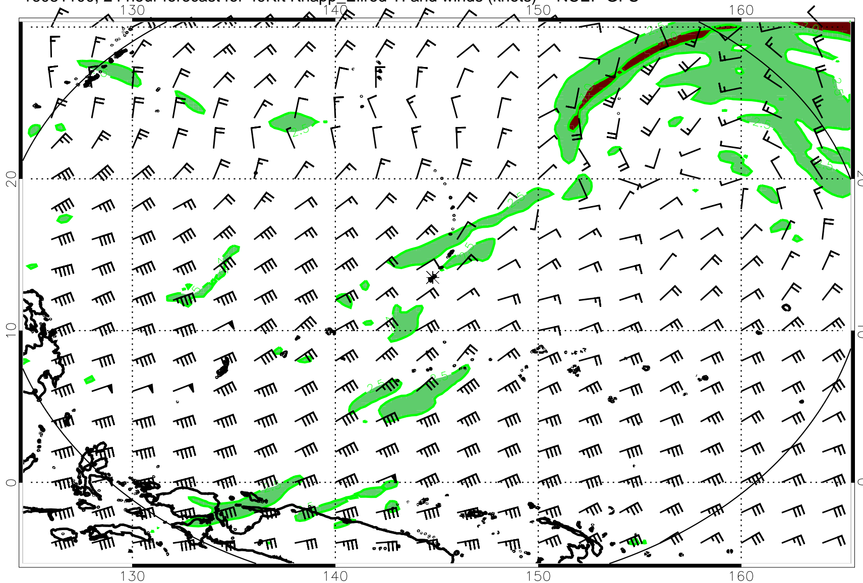
16081100, 24 hour forecast for 49Kft Knapp_Ellrod TI and winds (knots) -- NCEP GFS
