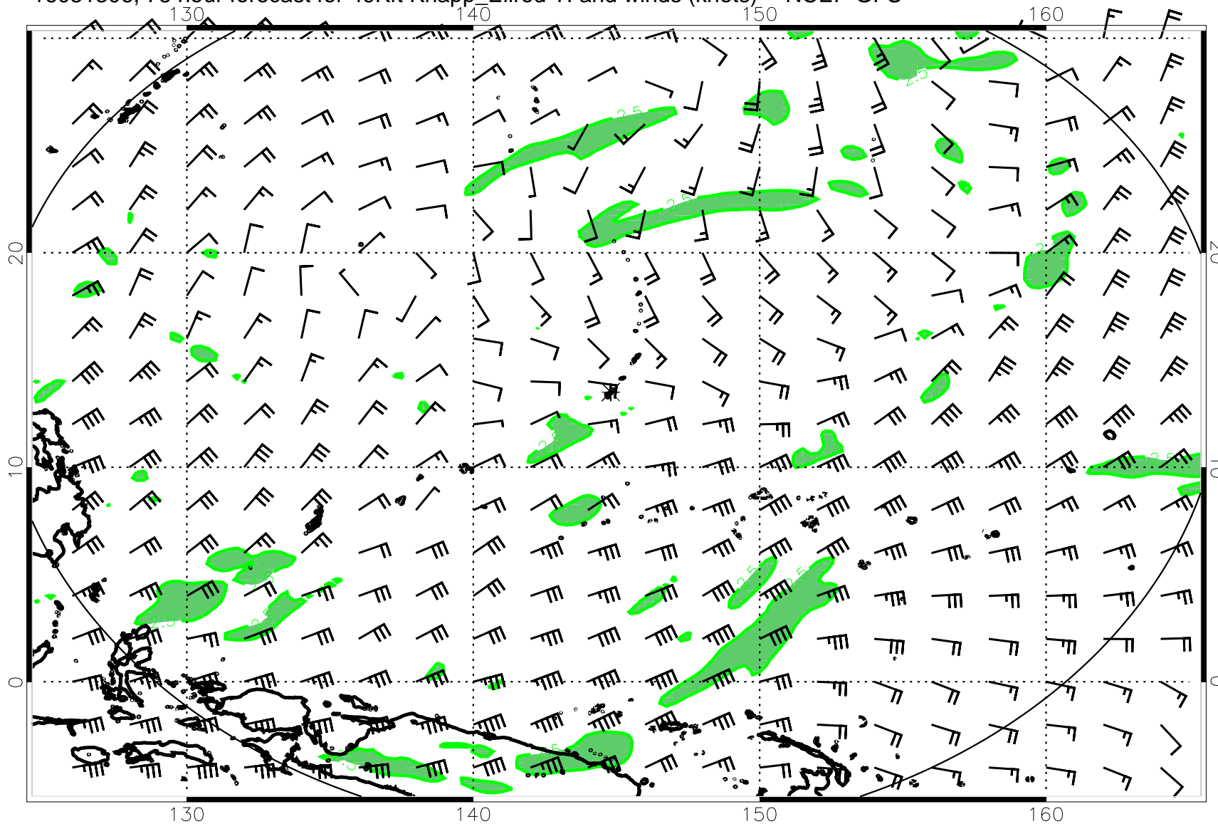
16081306, 78 hour forecast for 49Kft Knapp_Ellrod TI and winds (knots) -- NCEP GFS
