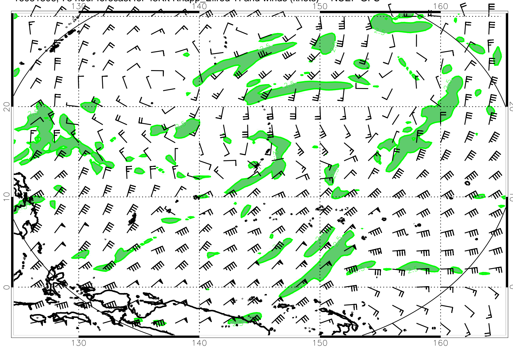
16081306, 78 hour forecast for 45Kft Knapp_Ellrod TI and winds (knots) -- NCEP GFS
