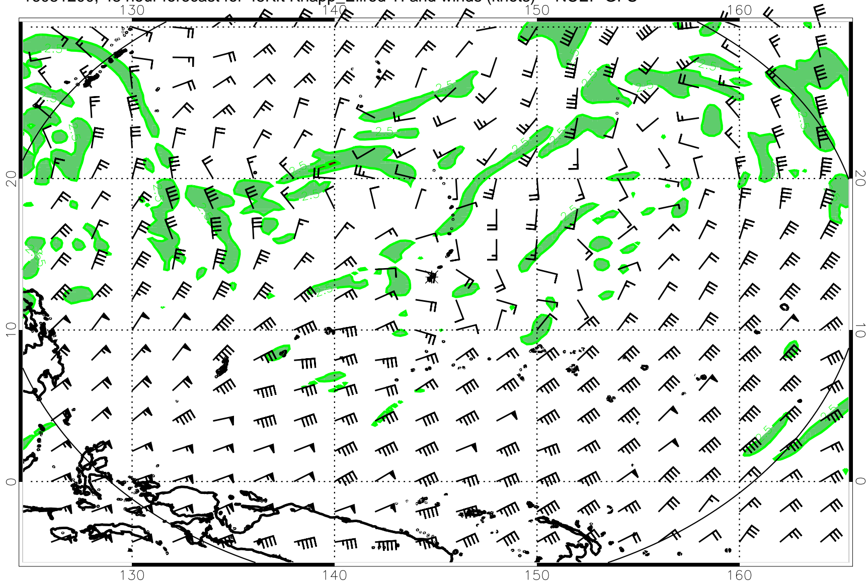
16081200, 48 hour forecast for 45Kft Knapp_Ellrod TI and winds (knots) -- NCEP GFS
