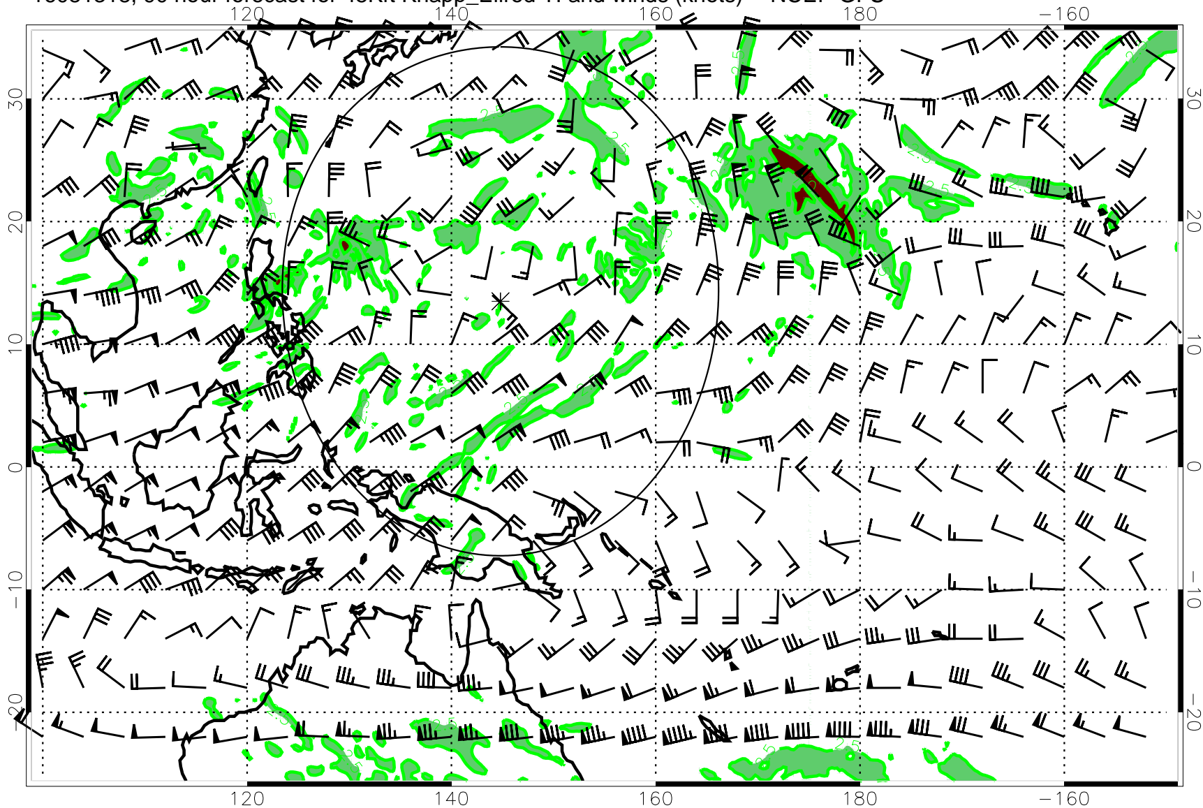
16081318, 90 hour forecast for 45Kft Knapp_Ellrod TI and winds (knots) -- NCEP GFS
