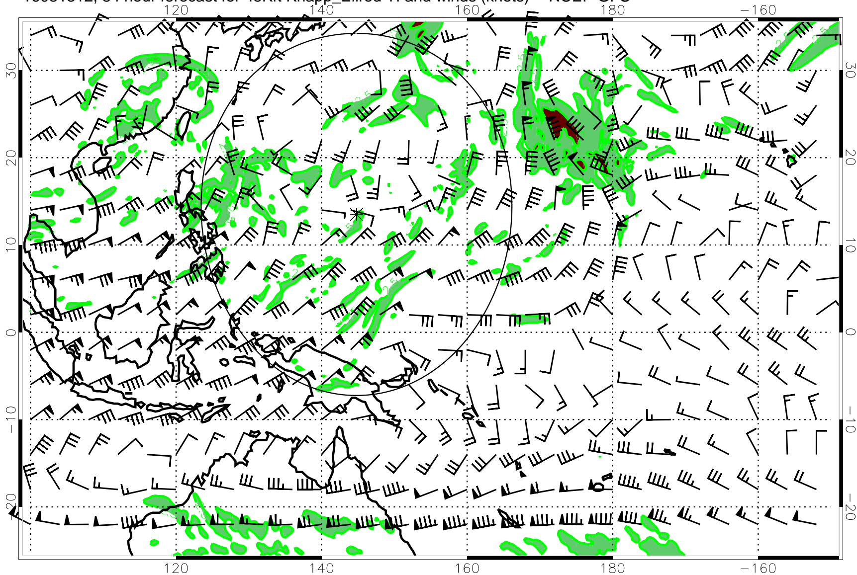
16081312, 84 hour forecast for 45Kft Knapp_Ellrod TI and winds (knots) -- NCEP GFS
