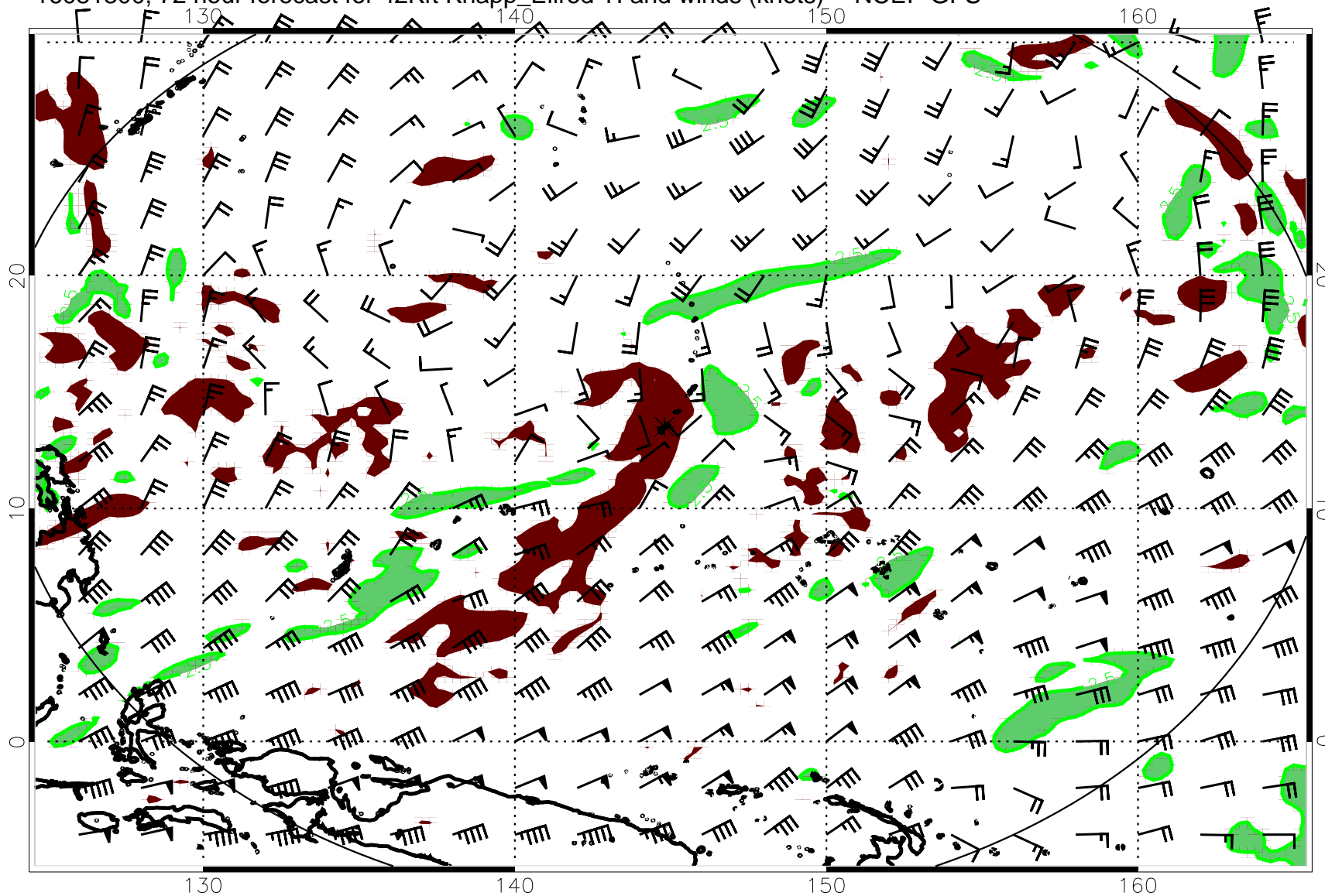
16081300, 72 hour forecast for 42Kft Knapp_Ellrod TI and winds (knots) -- NCEP GFS
