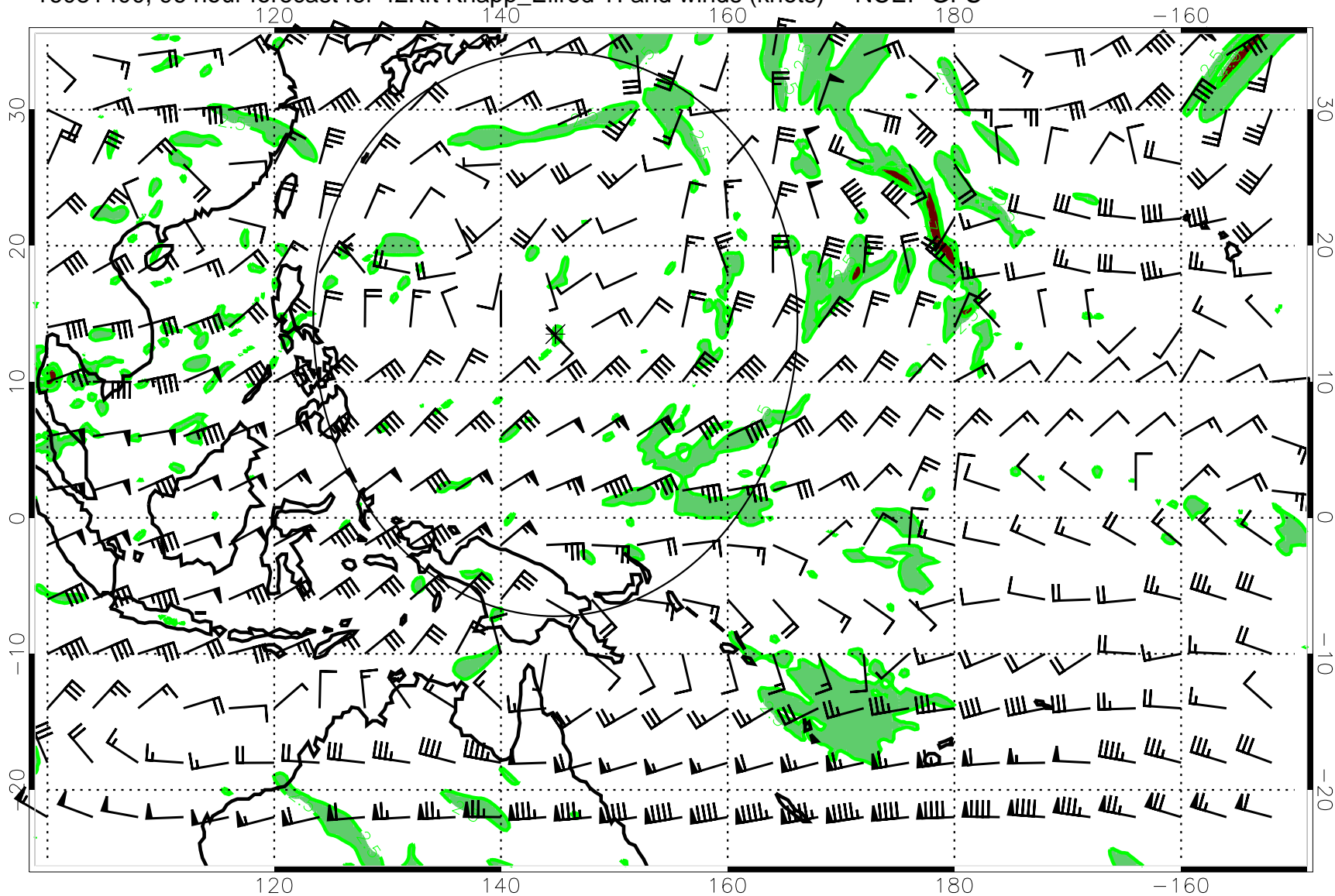
16081400, 96 hour forecast for 42Kft Knapp_Ellrod TI and winds (knots) -- NCEP GFS
