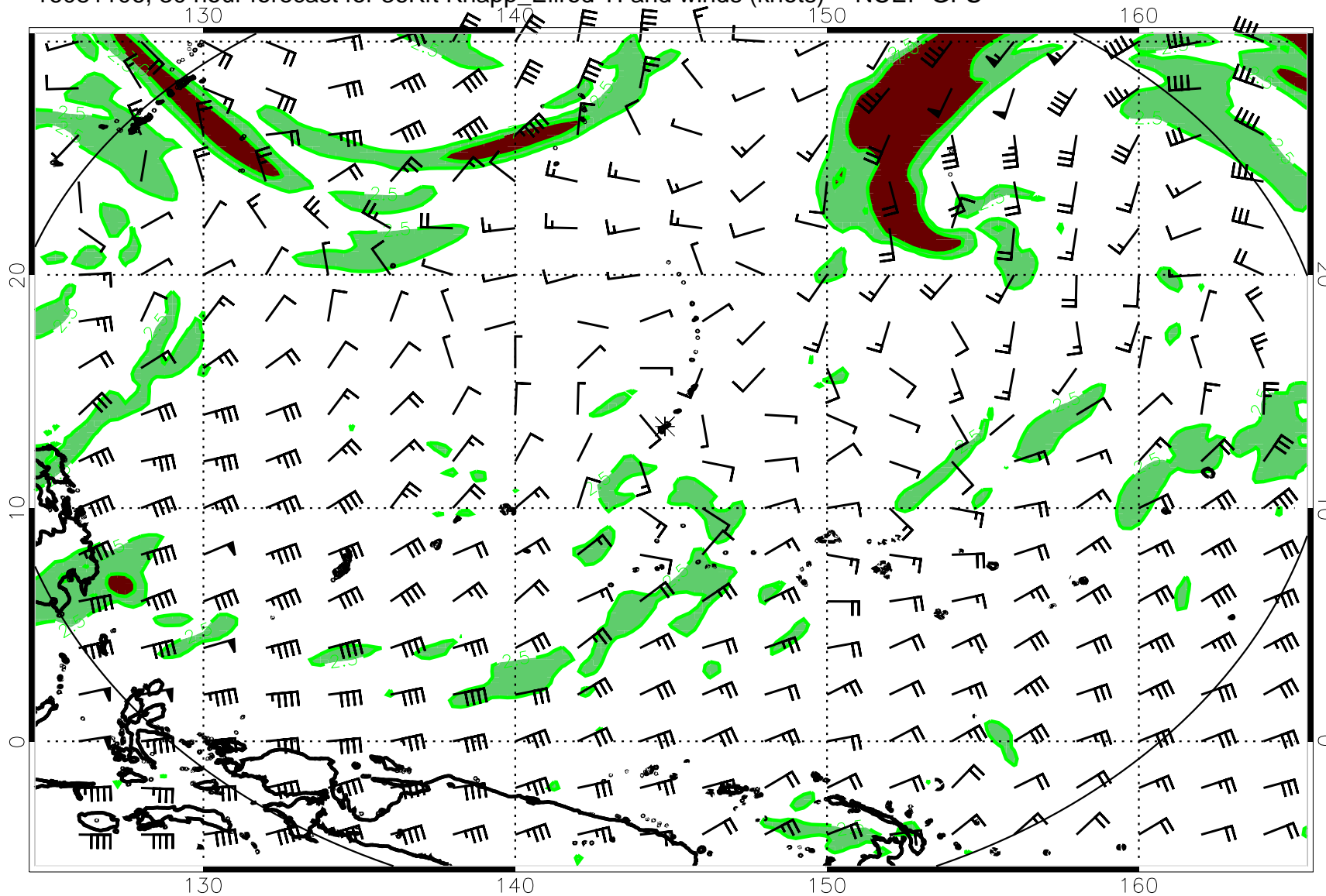
16081106, 30 hour forecast for 36Kft Knapp_Ellrod TI and winds (knots) -- NCEP GFS
