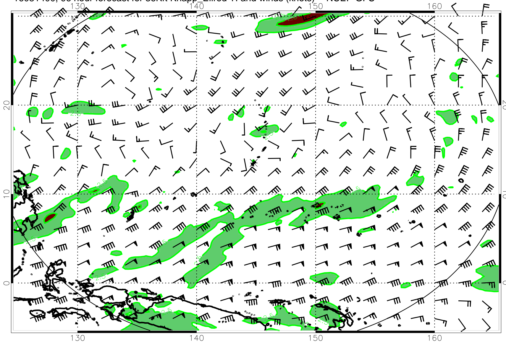
16081400, 96 hour forecast for 36Kft Knapp_Ellrod TI and winds (knots) -- NCEP GFS
