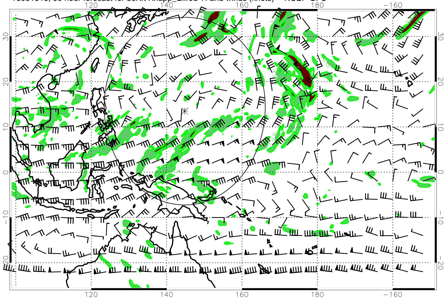
16081318, 90 hour forecast for 36Kft Knapp_Ellrod TI and winds (knots) -- NCEP GFS
