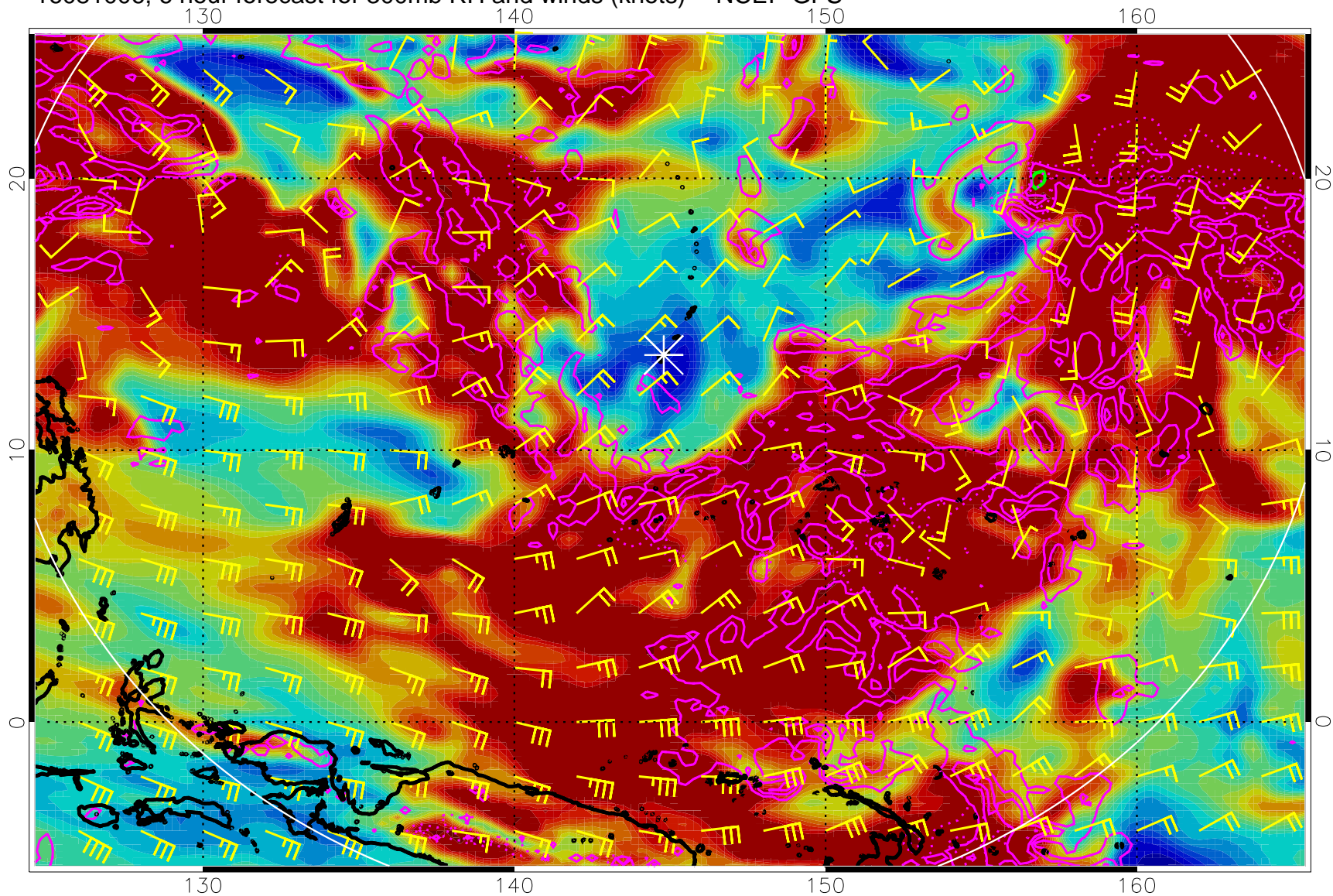
16081006, 6 hour forecast for 300mb RH and winds (knots) -- NCEP GFS
