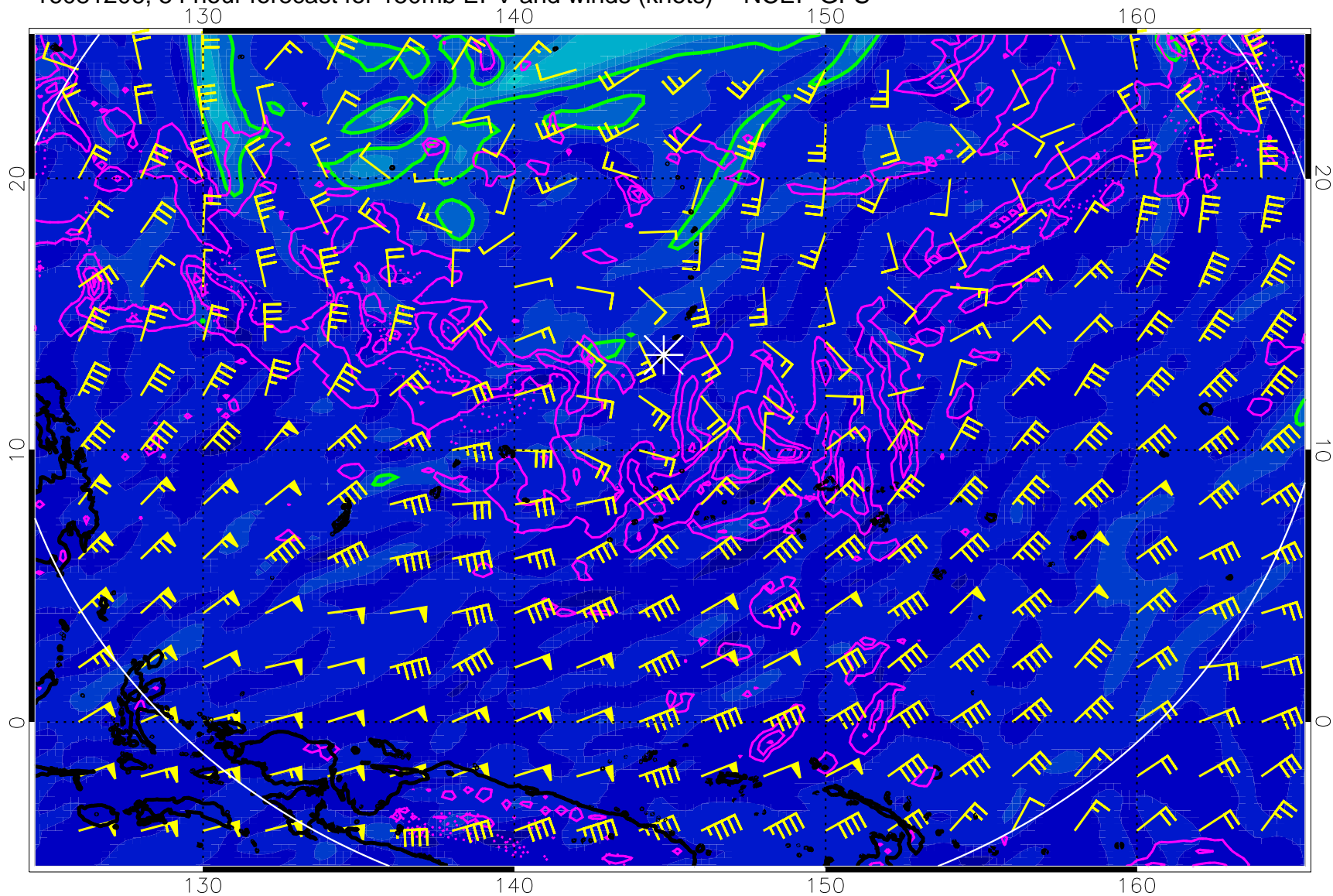
16081206, 54 hour forecast for 150mb EPV and winds (knots) -- NCEP GFS
