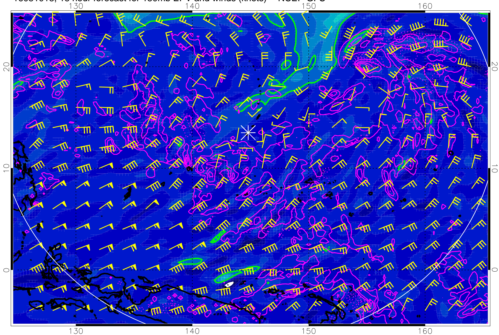
16081018, 18 hour forecast for 150mb EPV and winds (knots) -- NCEP GFS
