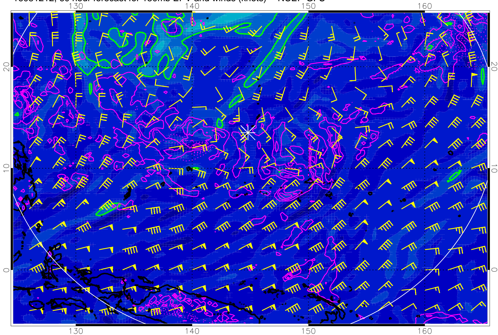
16081212, 60 hour forecast for 150mb EPV and winds (knots) -- NCEP GFS
