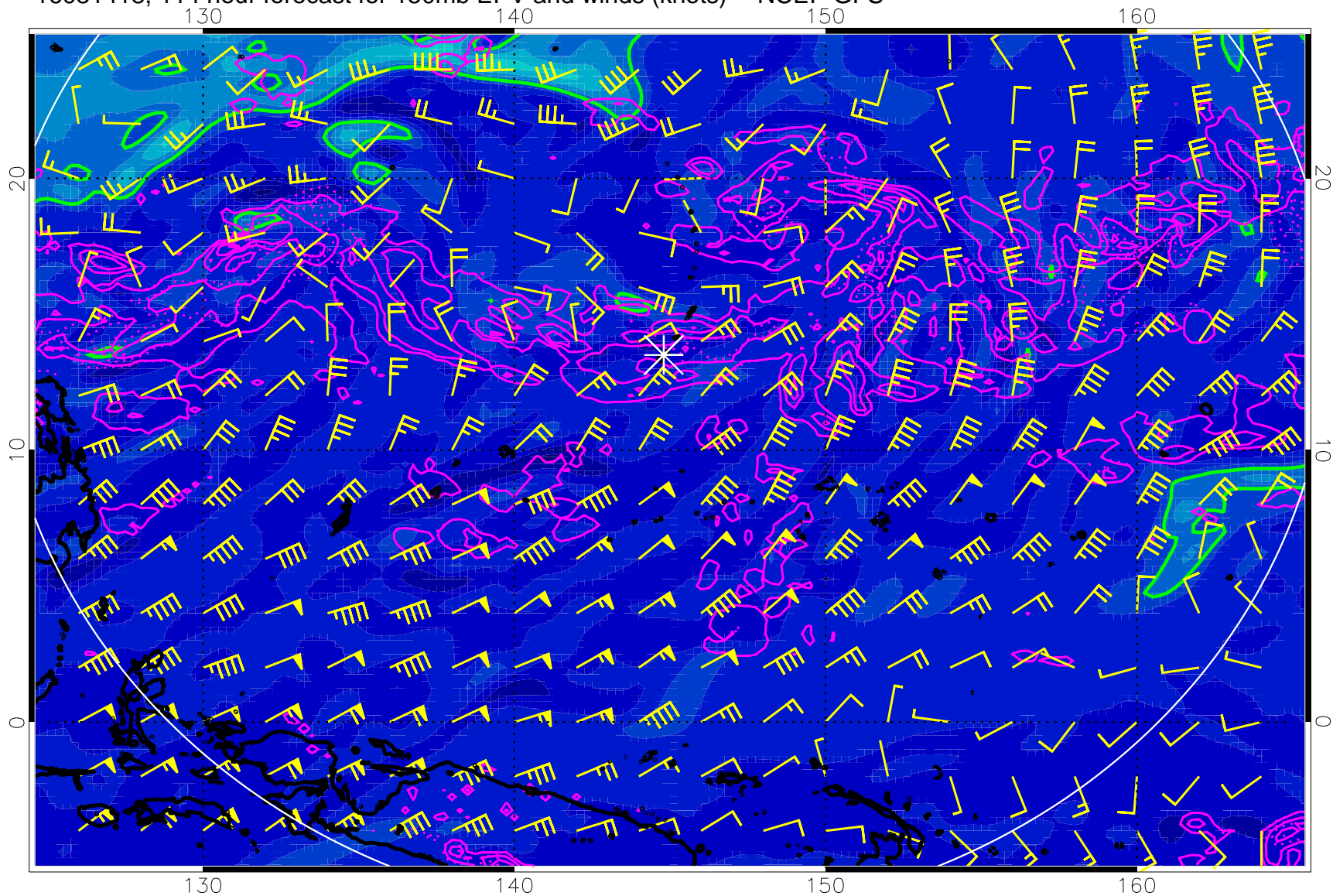
16081418, 114 hour forecast for 150mb EPV and winds (knots) -- NCEP GFS
