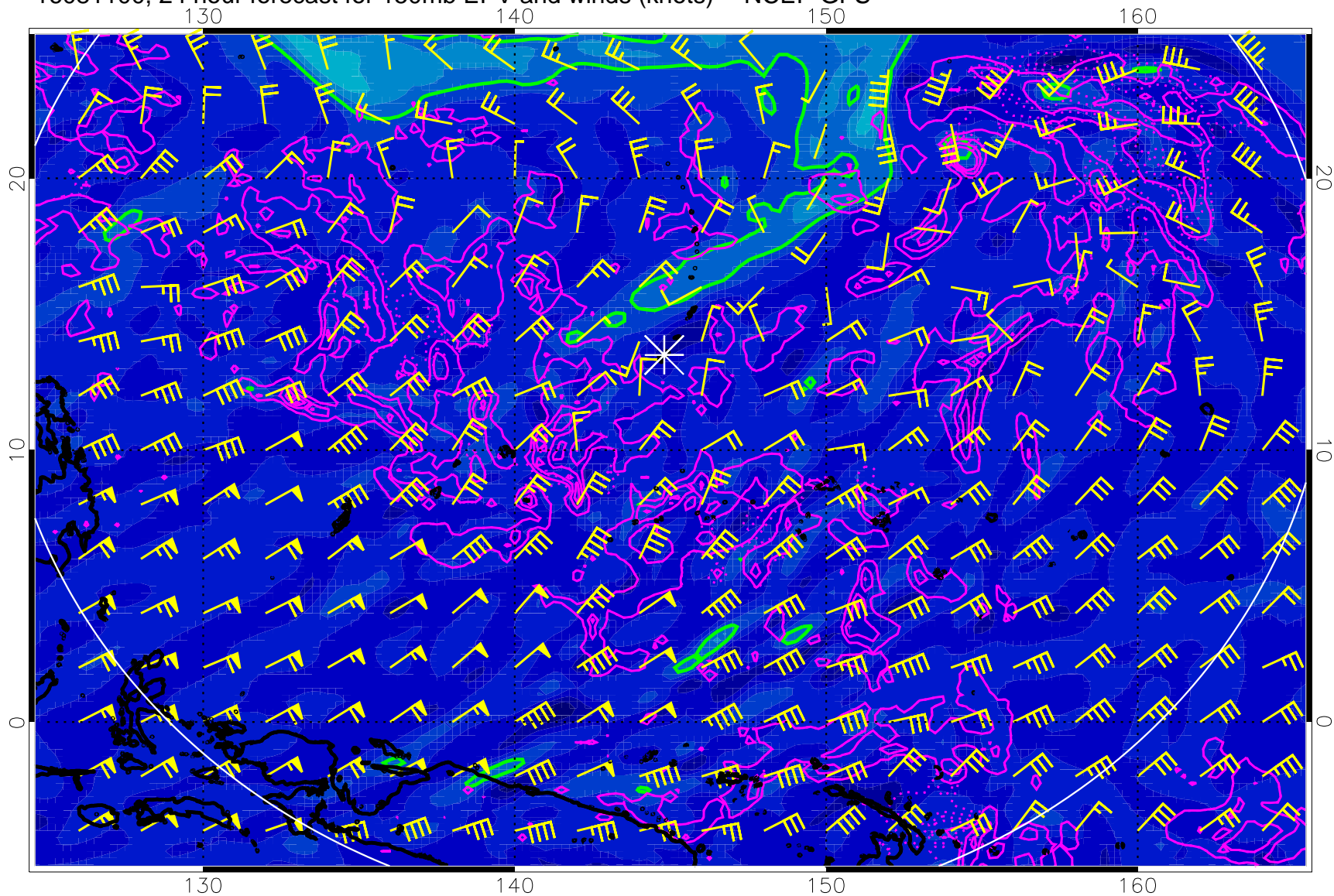
16081100, 24 hour forecast for 150mb EPV and winds (knots) -- NCEP GFS
