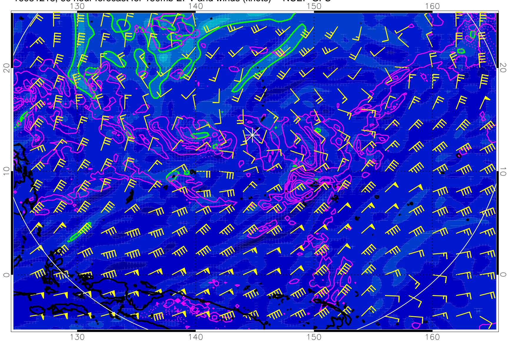
16081218, 66 hour forecast for 150mb EPV and winds (knots) -- NCEP GFS
