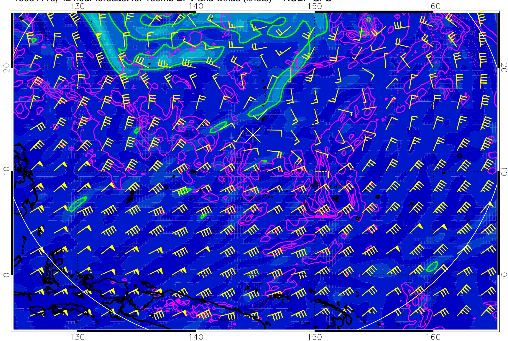
16081118, 42 hour forecast for 150mb EPV and winds (knots) -- NCEP GFS
