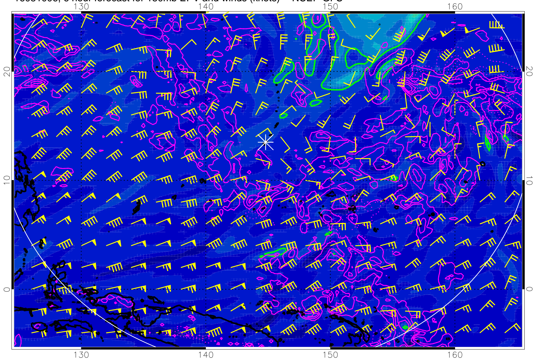
16081006, 6 hour forecast for 150mb EPV and winds (knots) -- NCEP GFS
