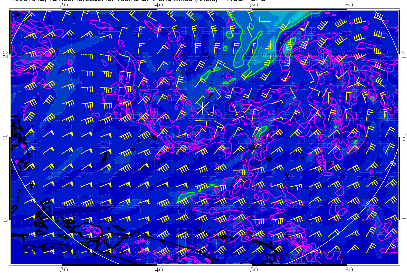
16081012, 12 hour forecast for 150mb EPV and winds (knots) -- NCEP GFS
