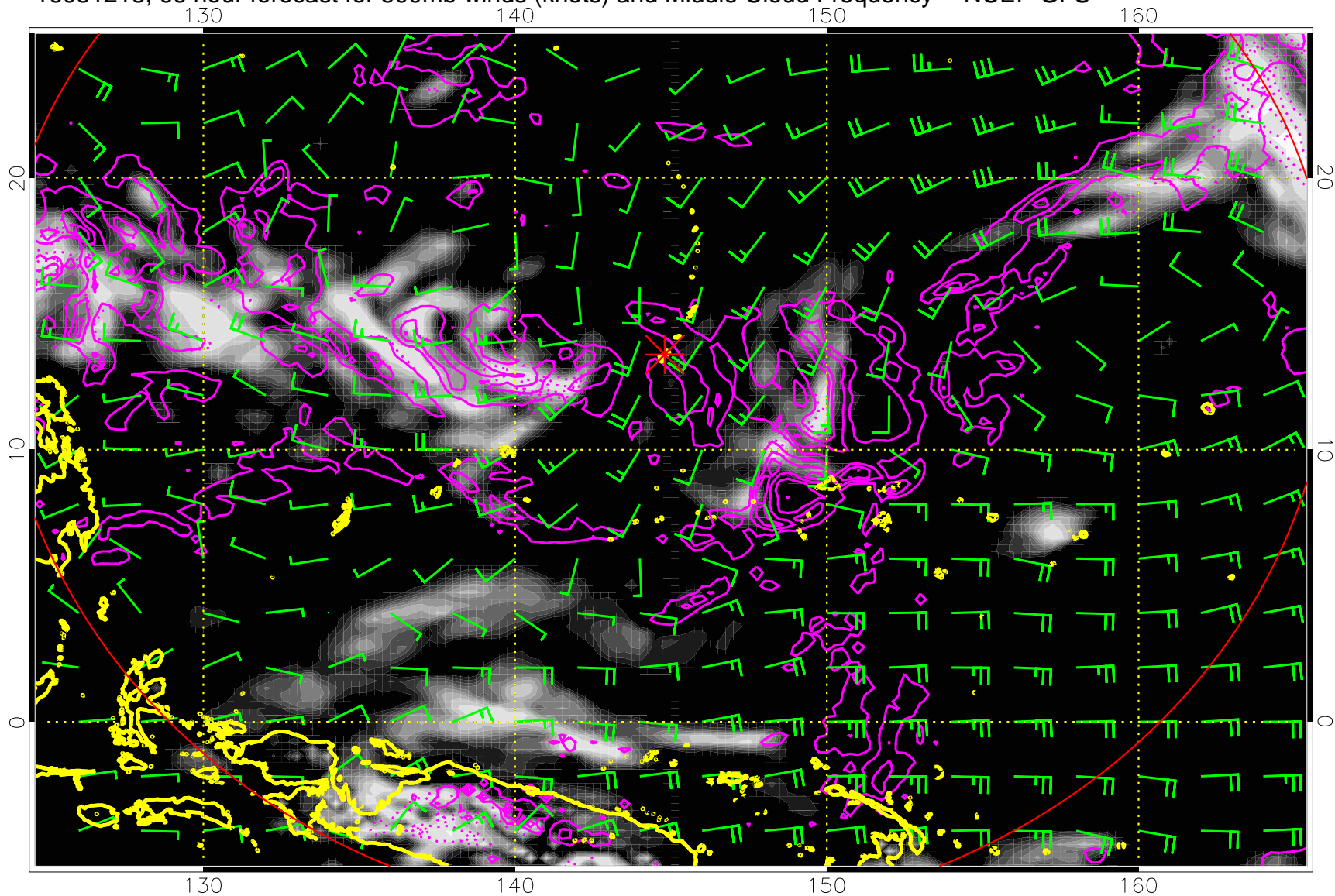
16081218, 66 hour forecast for 500mb winds (knots) and Middle Cloud Frequency -- NCEP GFS
