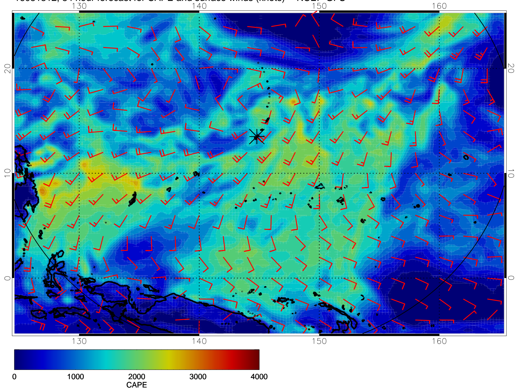
16081312, 84 hour forecast for CAPE and surface winds (knots) -- NCEP GFS
