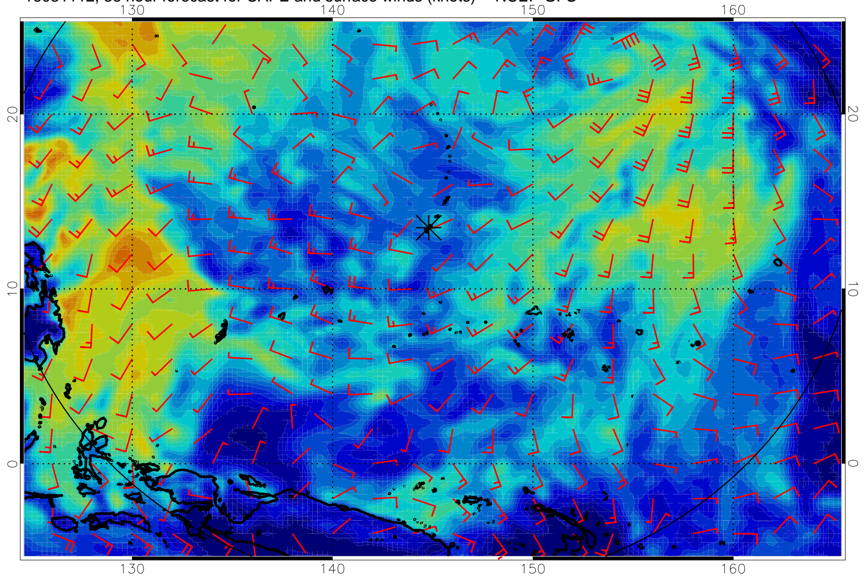
16081112, 36 hour forecast for CAPE and surface winds (knots) -- NCEP GFS
