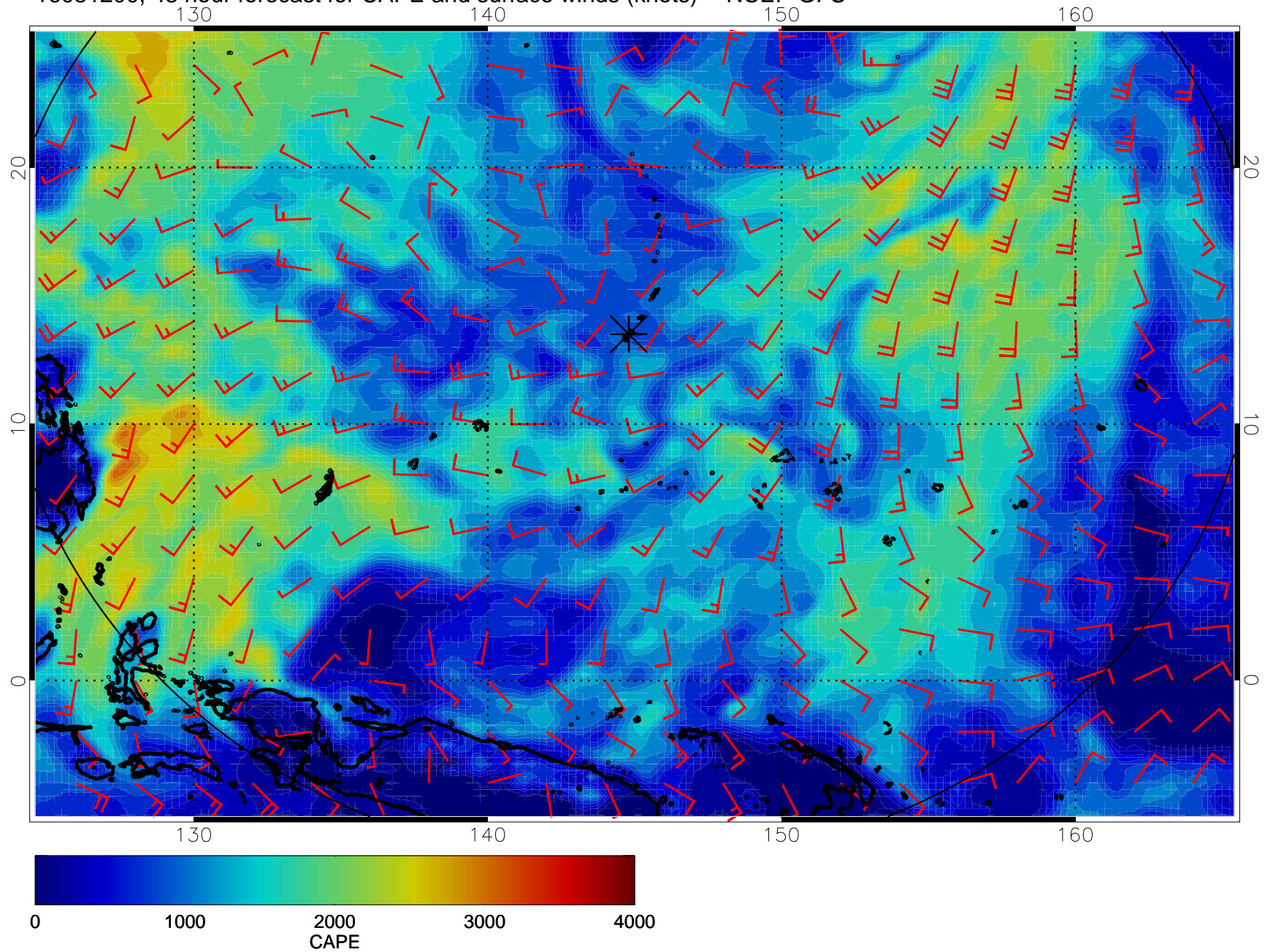
16081200, 48 hour forecast for CAPE and surface winds (knots) -- NCEP GFS
