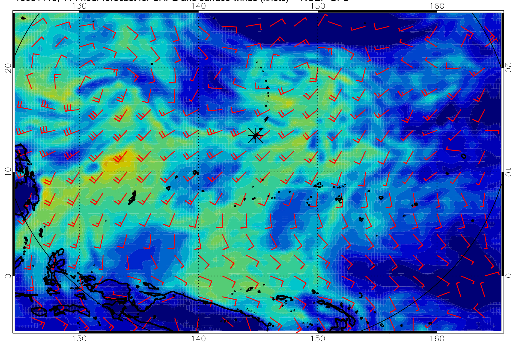
16081418, 114 hour forecast for CAPE and surface winds (knots) -- NCEP GFS
