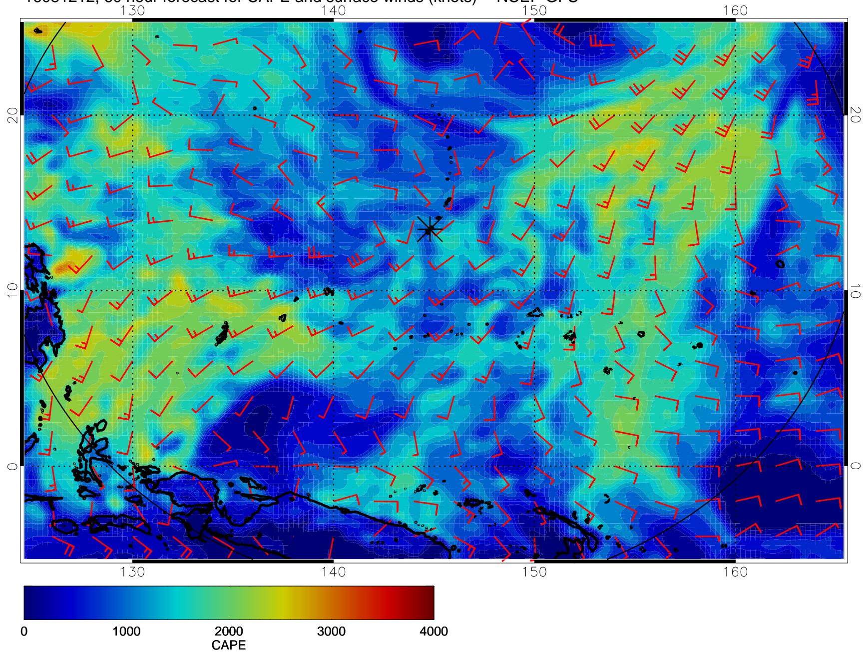
16081212, 60 hour forecast for CAPE and surface winds (knots) -- NCEP GFS
