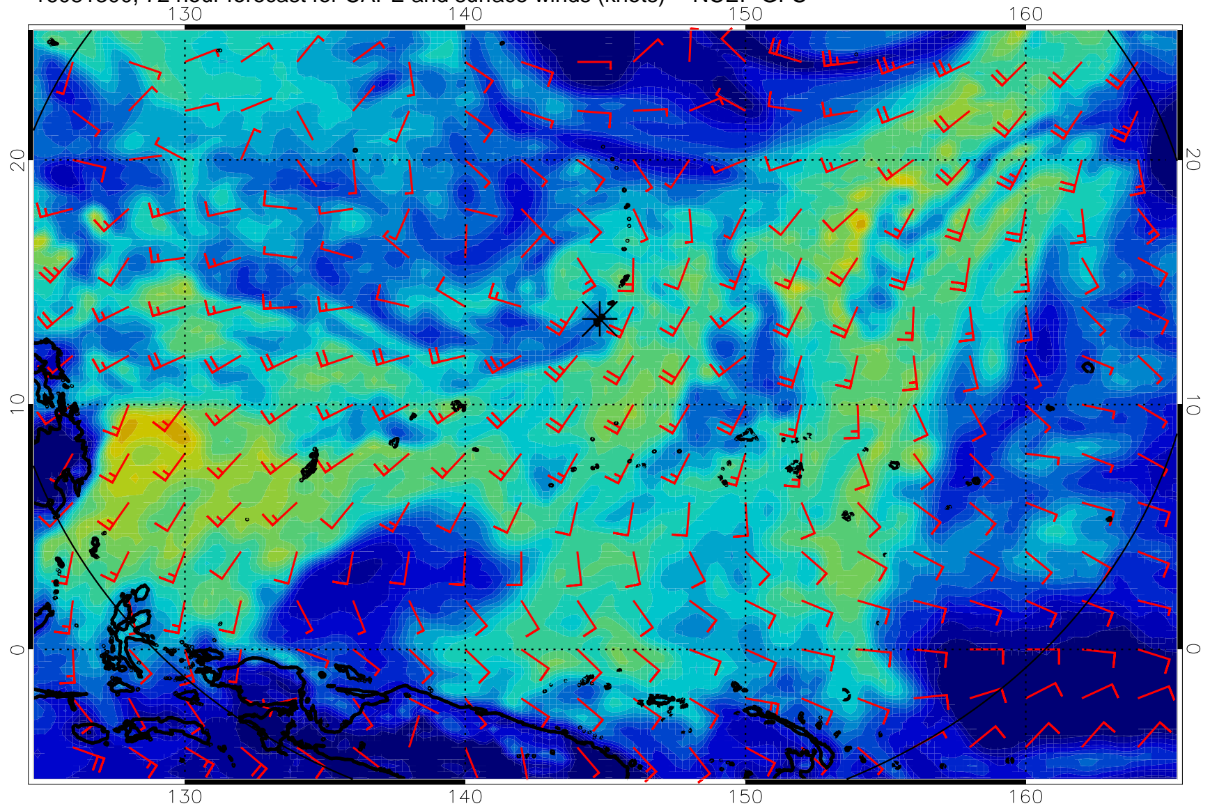
16081300, 72 hour forecast for CAPE and surface winds (knots) -- NCEP GFS
