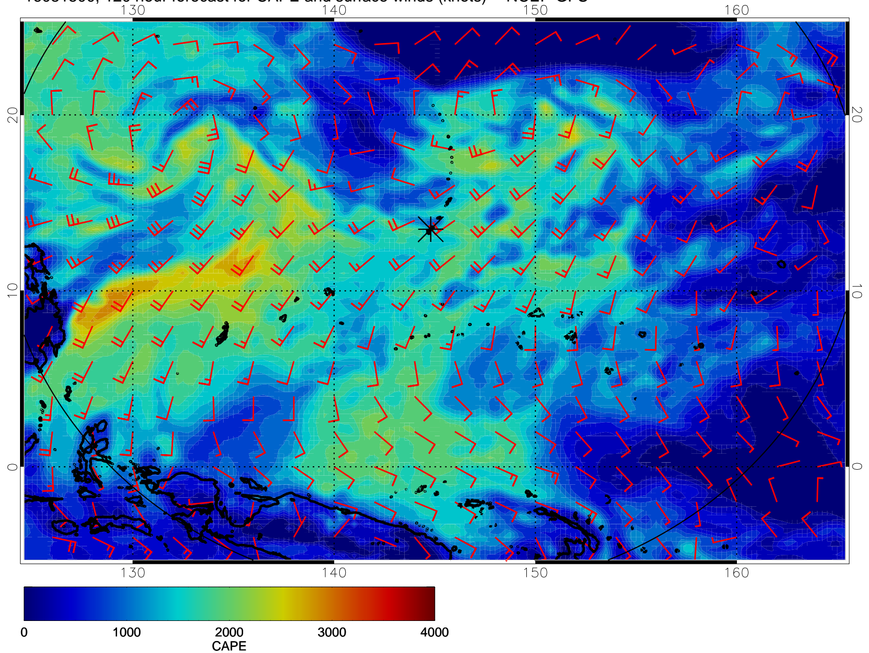
16081500, 120 hour forecast for CAPE and surface winds (knots) -- NCEP GFS
