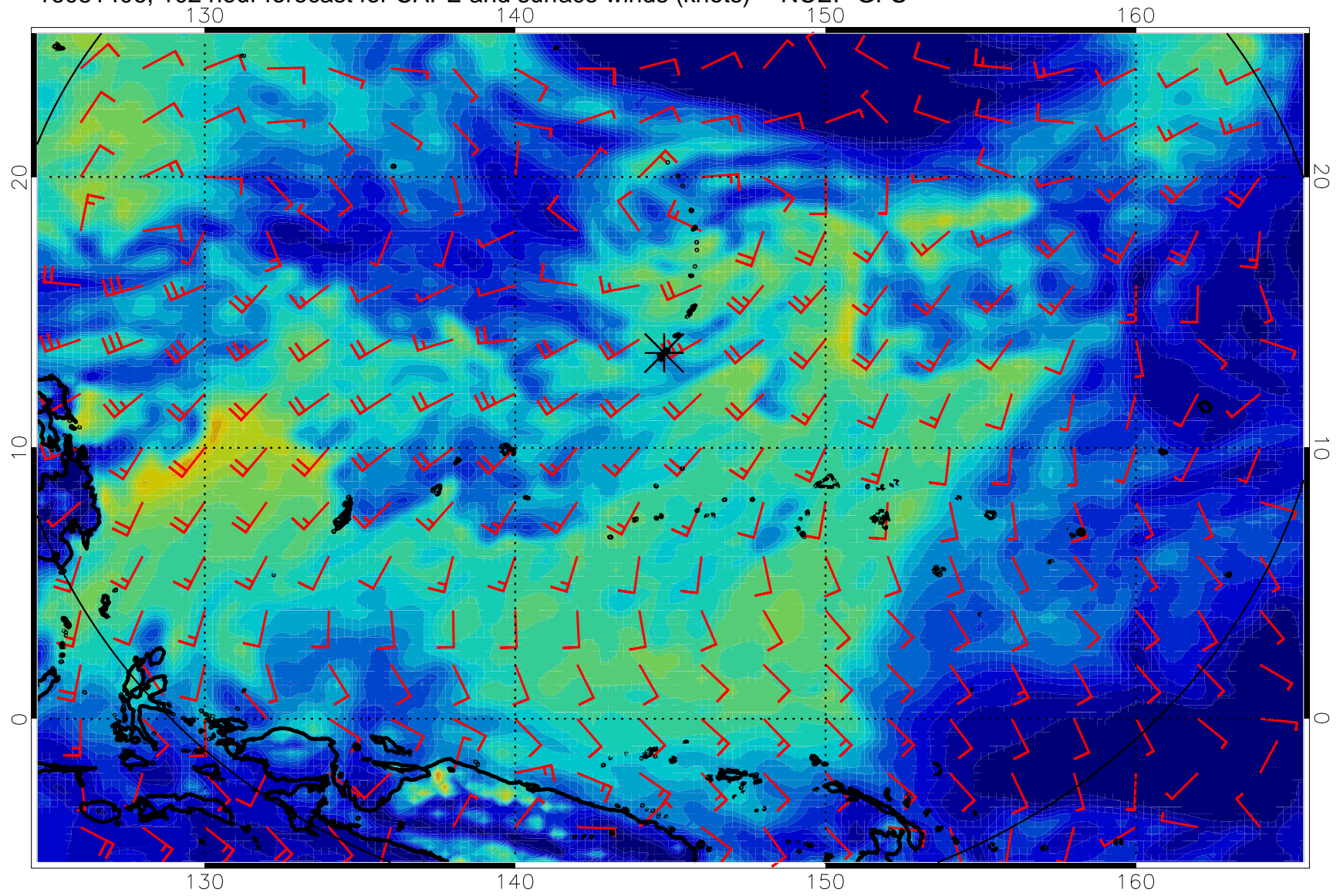
16081406, 102 hour forecast for CAPE and surface winds (knots) -- NCEP GFS
