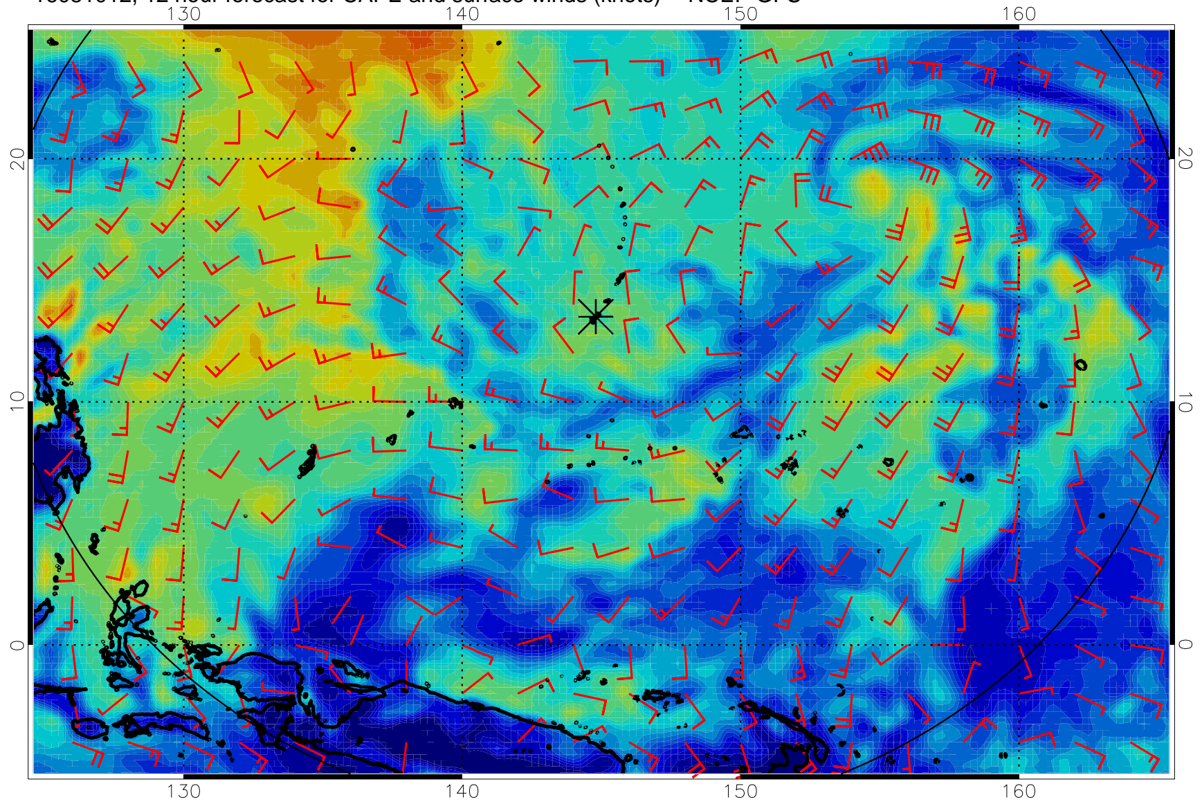
16081012, 12 hour forecast for CAPE and surface winds (knots) -- NCEP GFS
