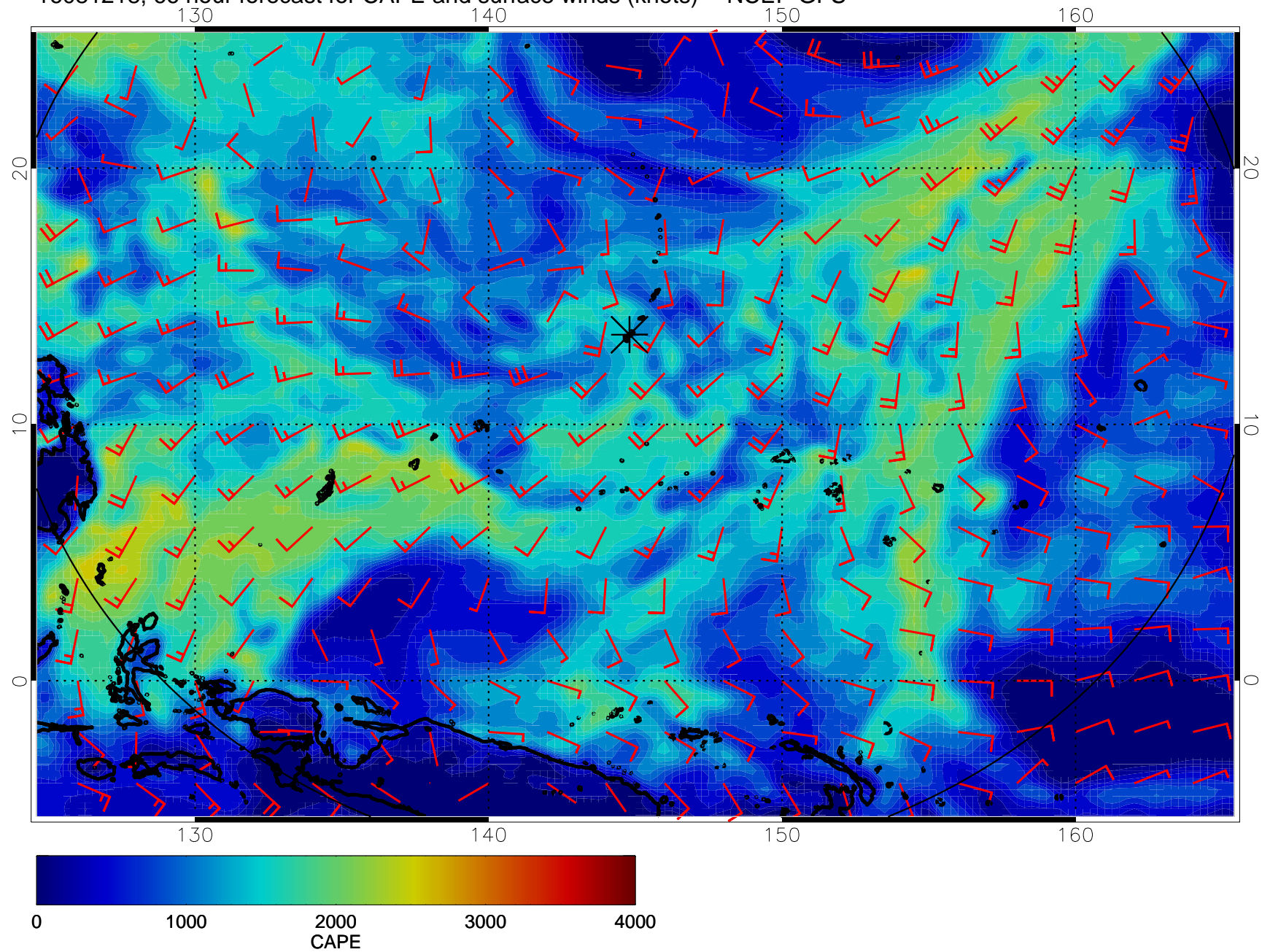
16081218, 66 hour forecast for CAPE and surface winds (knots) -- NCEP GFS
