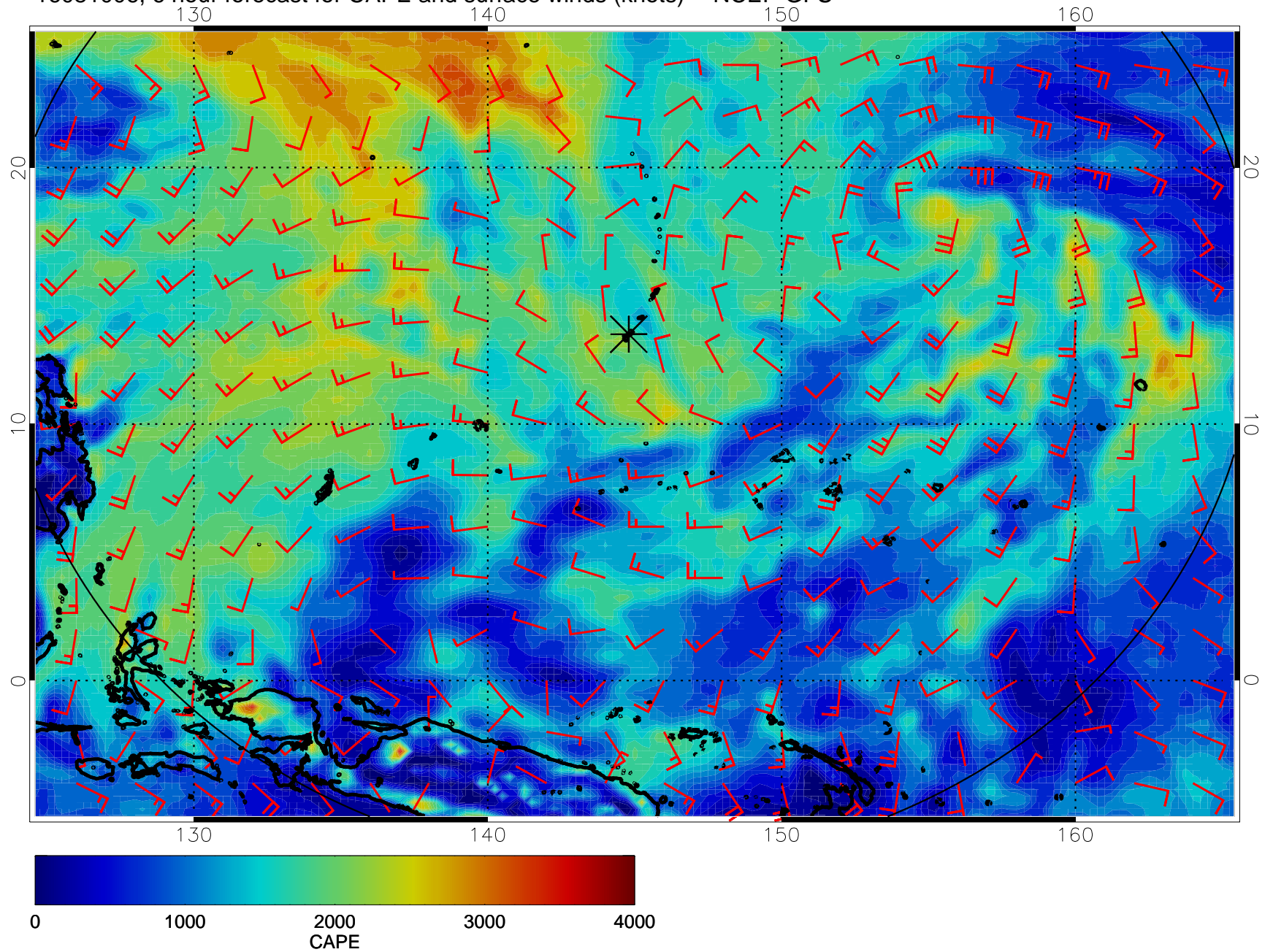
16081006, 6 hour forecast for CAPE and surface winds (knots) -- NCEP GFS
