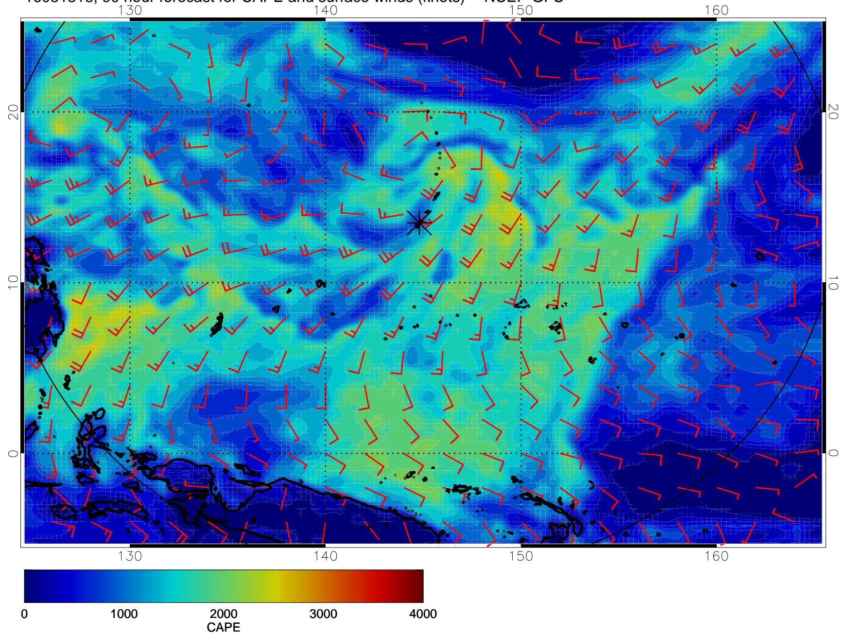
16081318, 90 hour forecast for CAPE and surface winds (knots) -- NCEP GFS
