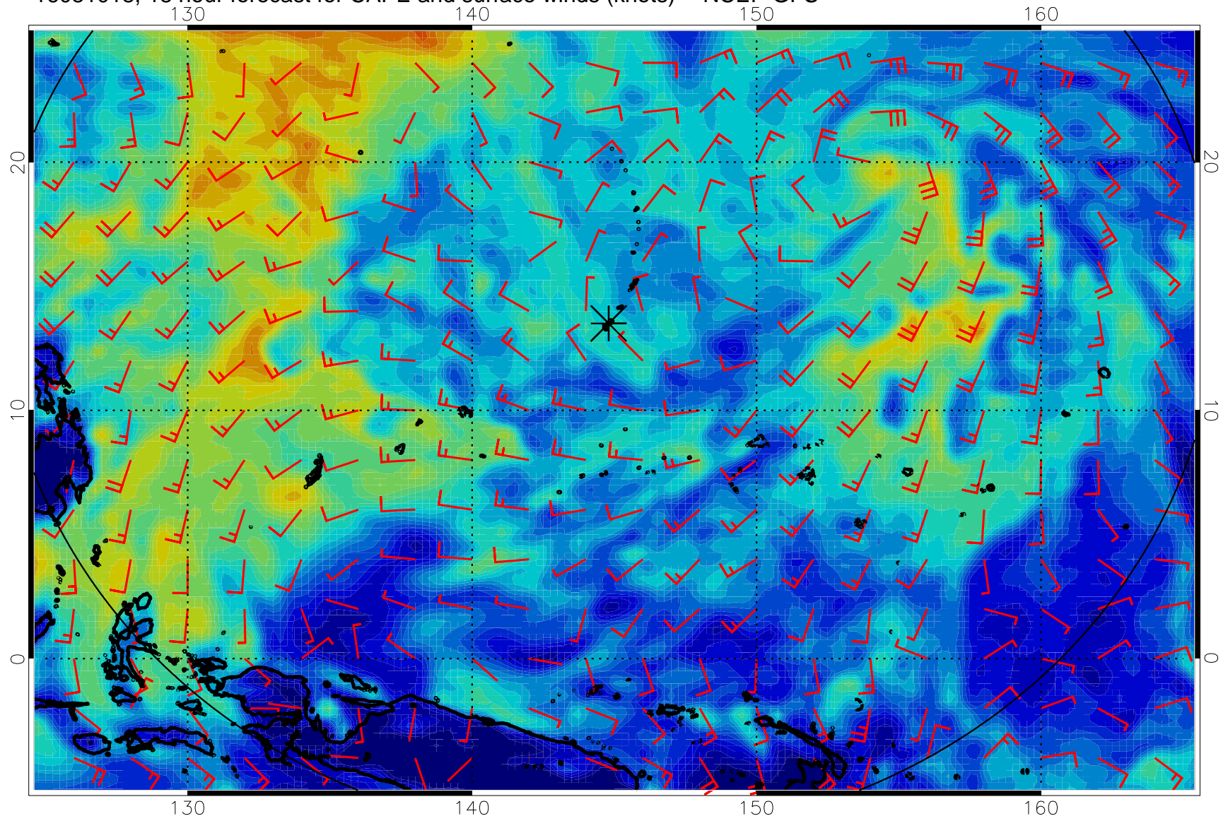
16081018, 18 hour forecast for CAPE and surface winds (knots) -- NCEP GFS
