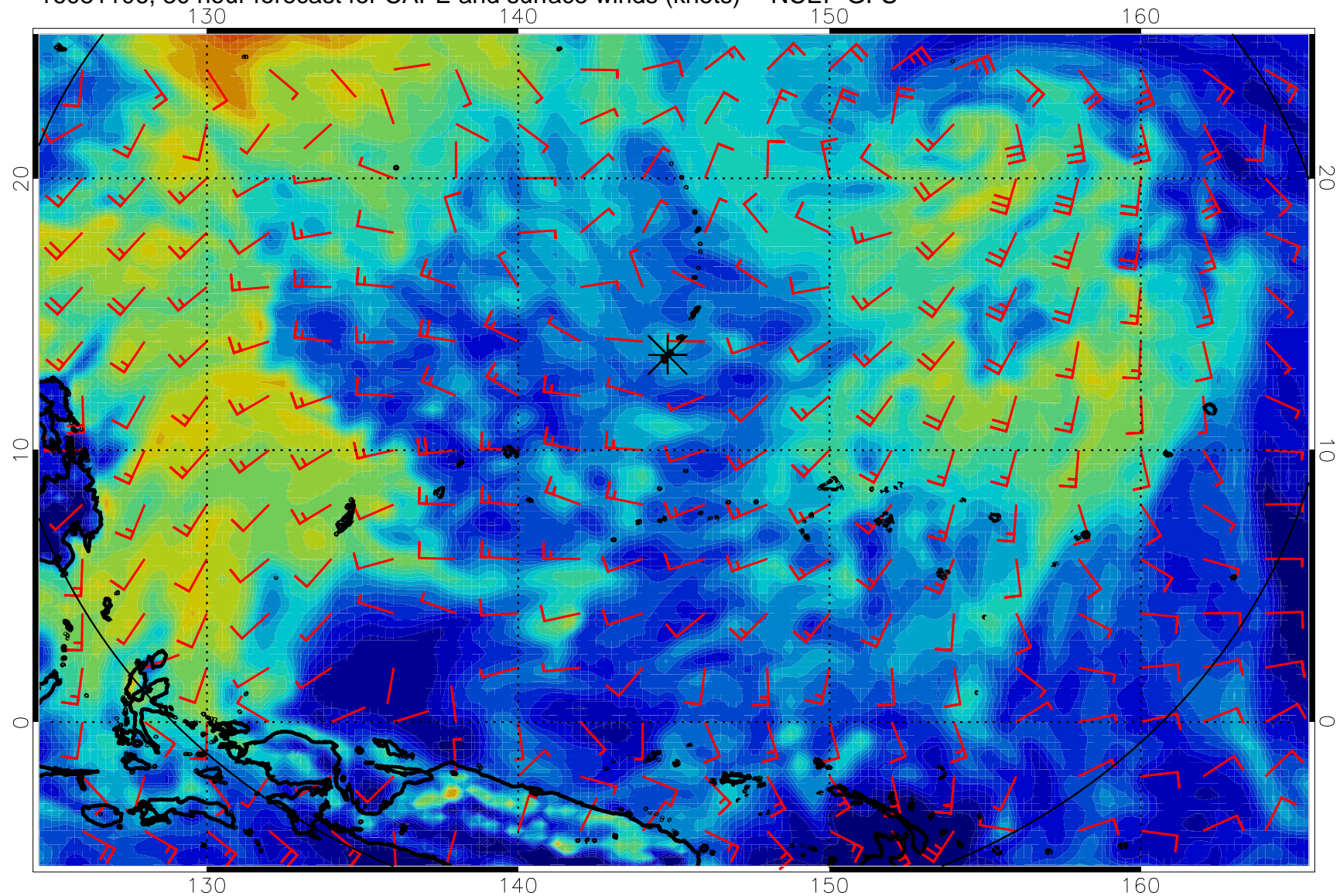
16081106, 30 hour forecast for CAPE and surface winds (knots) -- NCEP GFS
