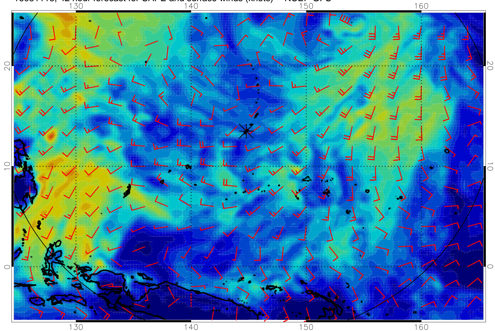
16081118, 42 hour forecast for CAPE and surface winds (knots) -- NCEP GFS
