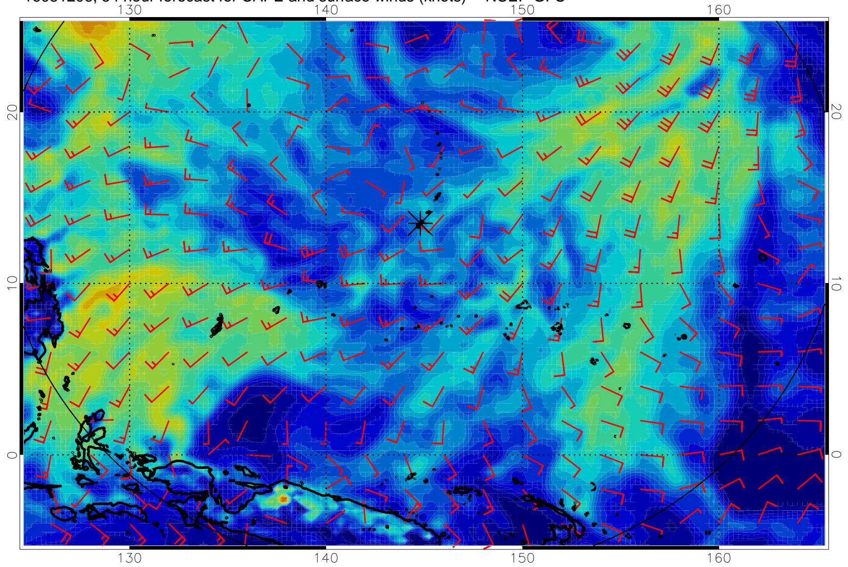
16081206, 54 hour forecast for CAPE and surface winds (knots) -- NCEP GFS
