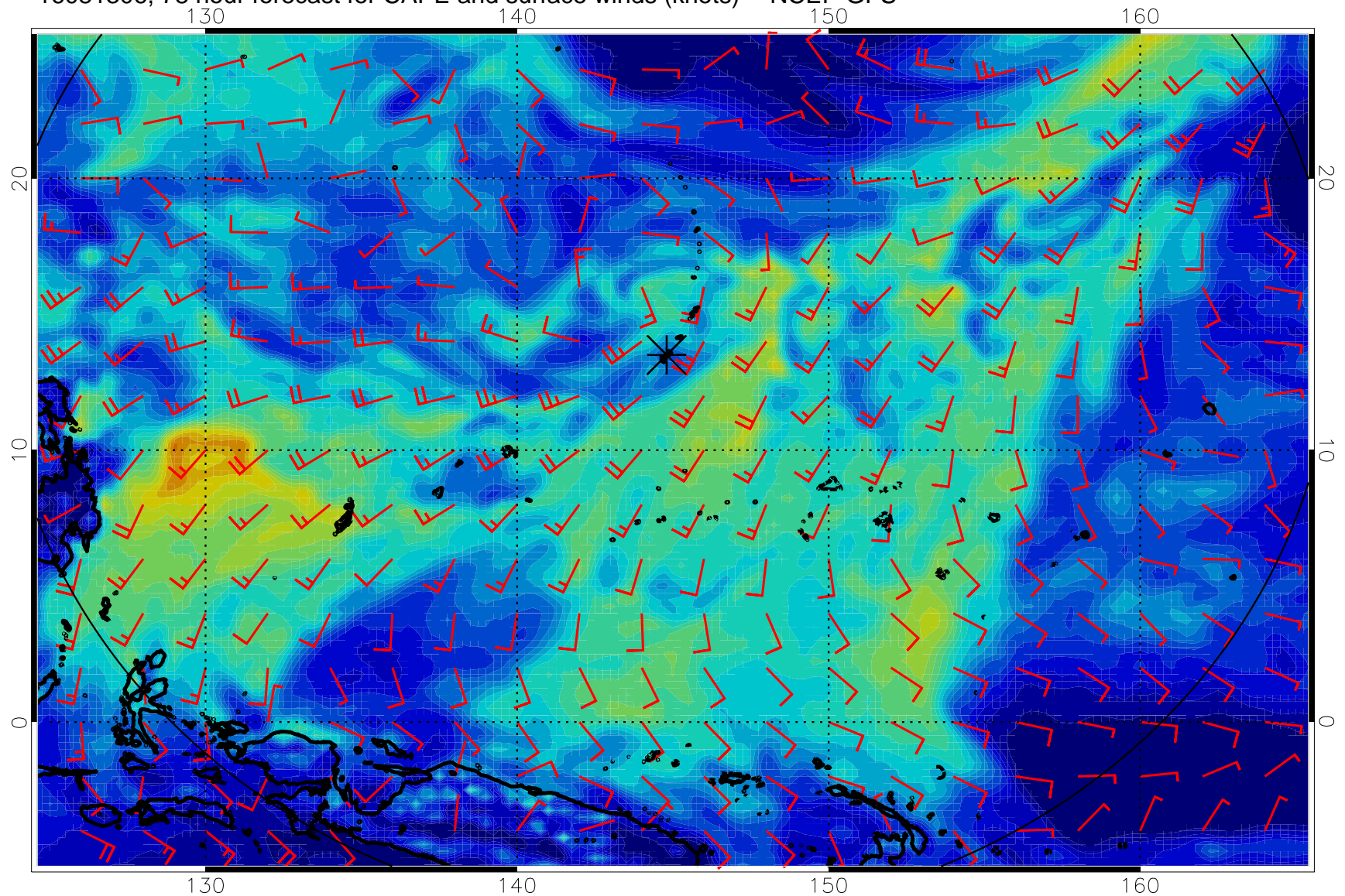
16081306, 78 hour forecast for CAPE and surface winds (knots) -- NCEP GFS
