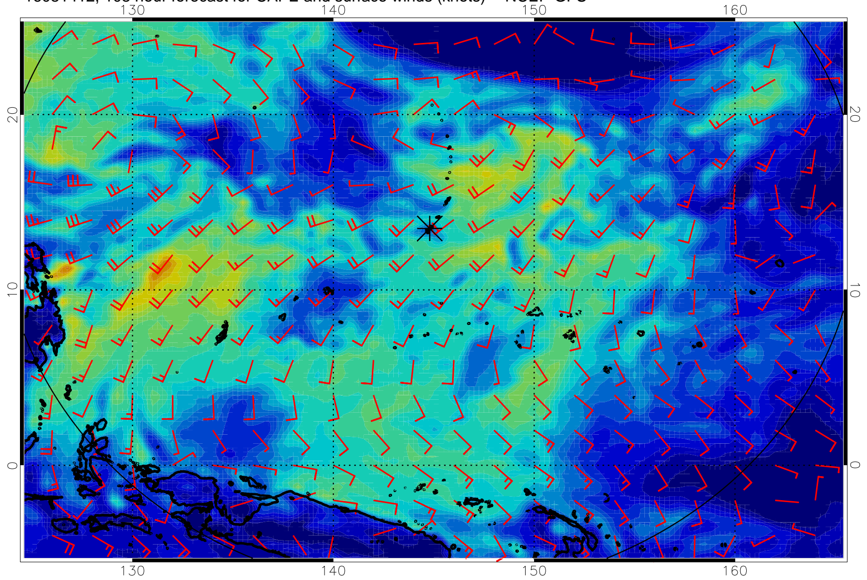
16081412, 108 hour forecast for CAPE and surface winds (knots) -- NCEP GFS
