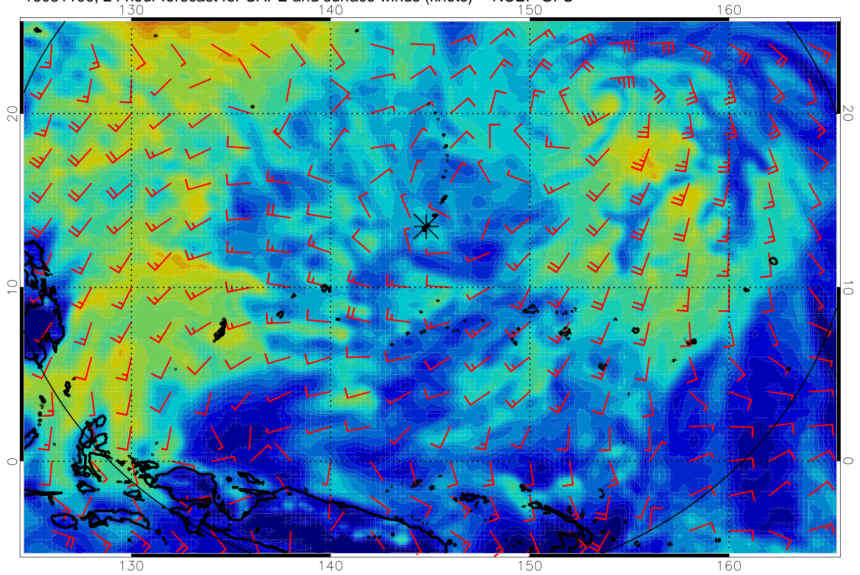
16081100, 24 hour forecast for CAPE and surface winds (knots) -- NCEP GFS
