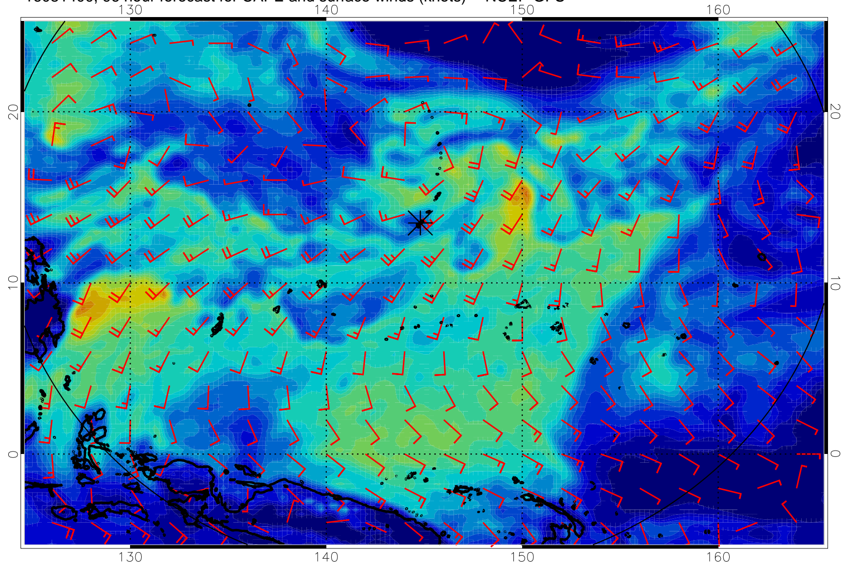
16081400, 96 hour forecast for CAPE and surface winds (knots) -- NCEP GFS
