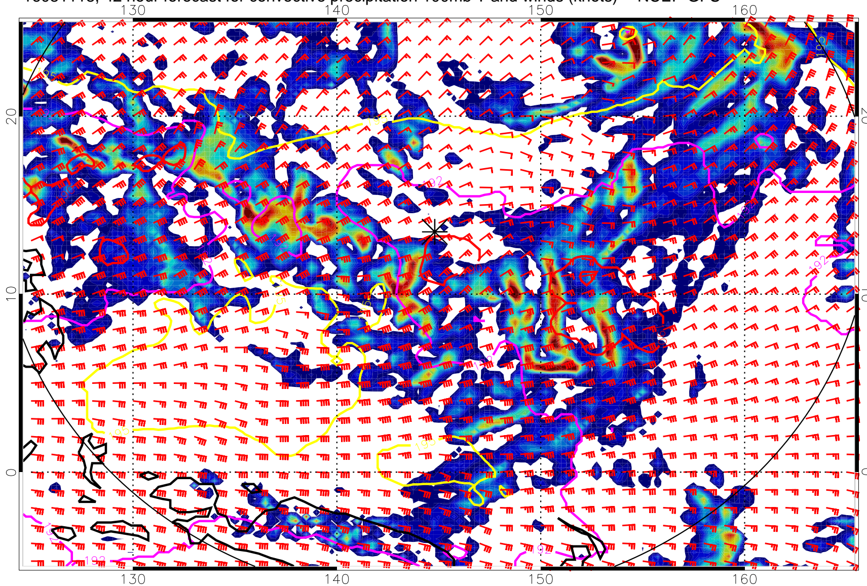
16081118, 42 hour forecast for convective precipitation 100mb T and winds (knots) -- NCEP GFS
