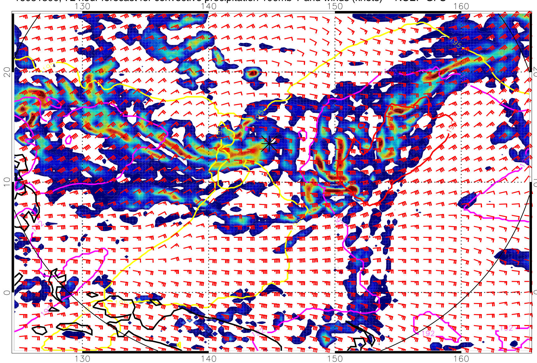
16081300, 72 hour forecast for convective precipitation 100mb T and winds (knots) -- NCEP GFS
