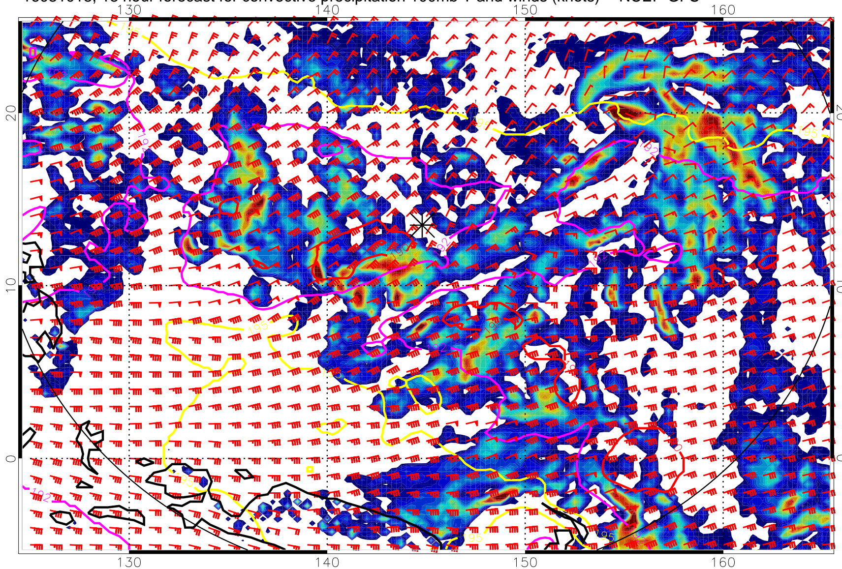
16081018, 18 hour forecast for convective precipitation 100mb T and winds (knots) -- NCEP GFS
