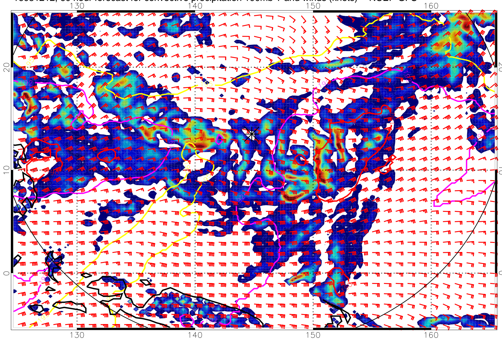
16081212, 60 hour forecast for convective precipitation 100mb T and winds (knots) -- NCEP GFS
