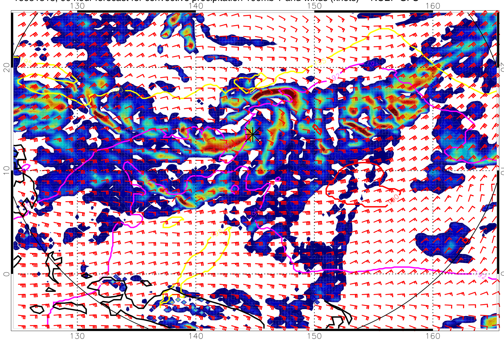
16081318, 90 hour forecast for convective precipitation 100mb T and winds (knots) -- NCEP GFS
