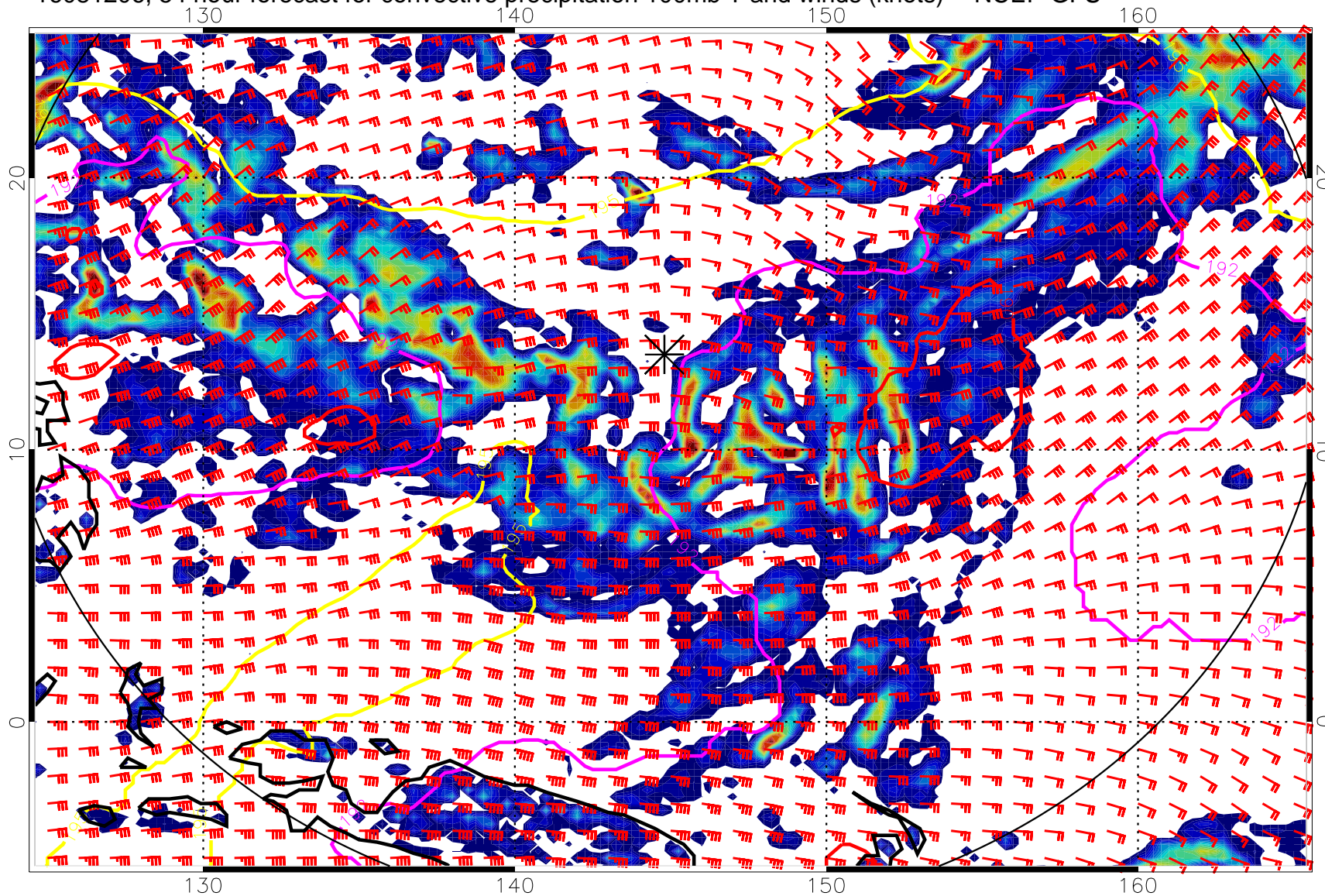
16081206, 54 hour forecast for convective precipitation 100mb T and winds (knots) -- NCEP GFS
