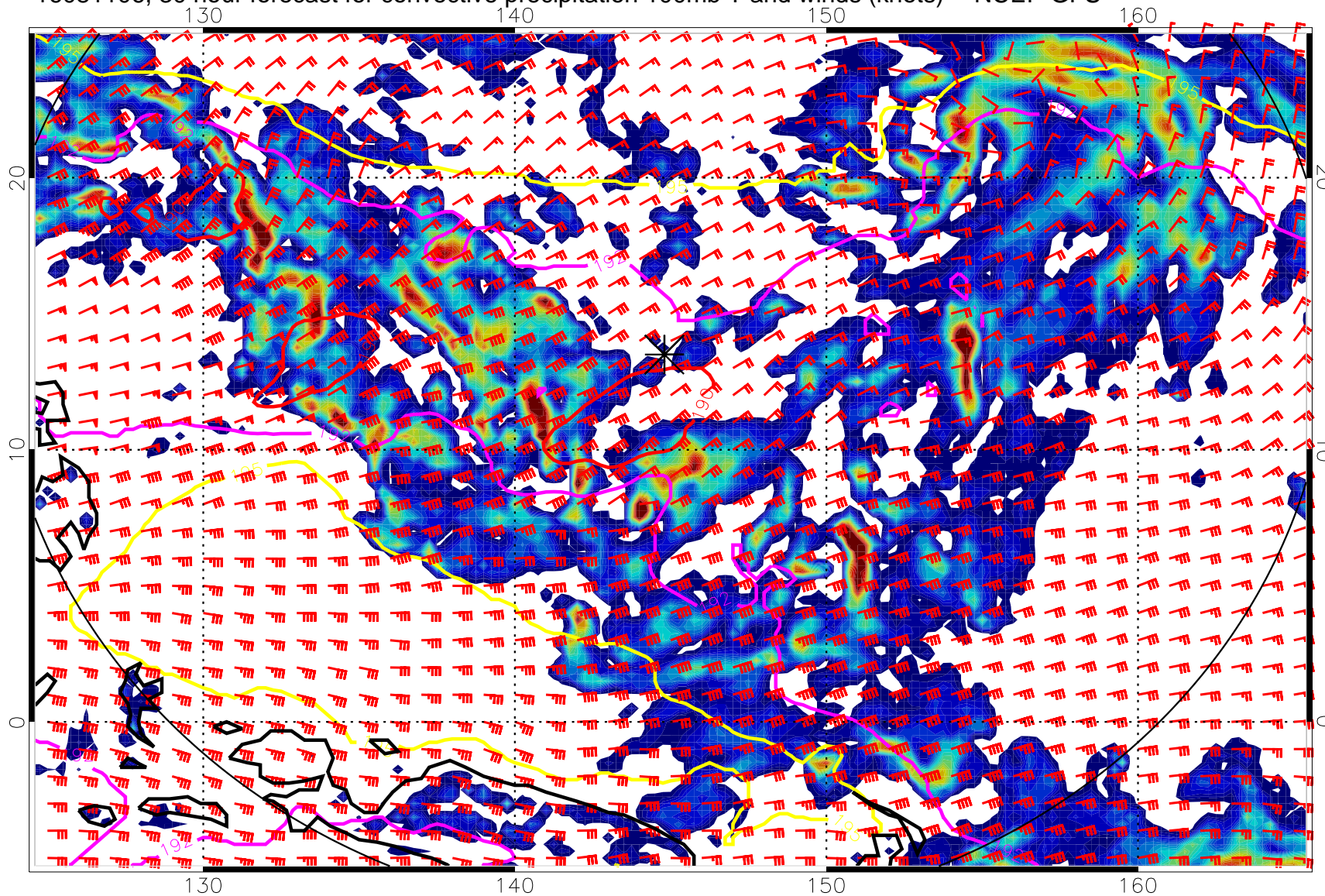
16081106, 30 hour forecast for convective precipitation 100mb T and winds (knots) -- NCEP GFS
