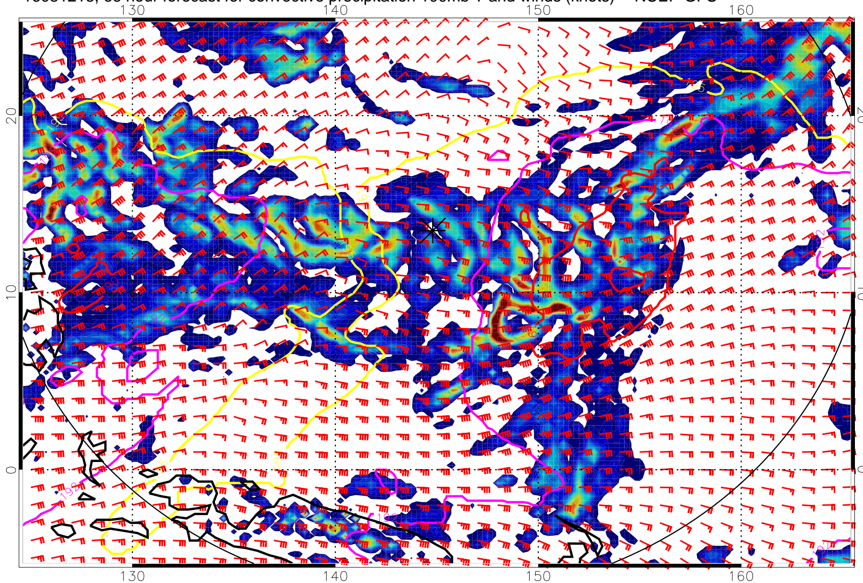
16081218, 66 hour forecast for convective precipitation 100mb T and winds (knots) -- NCEP GFS
