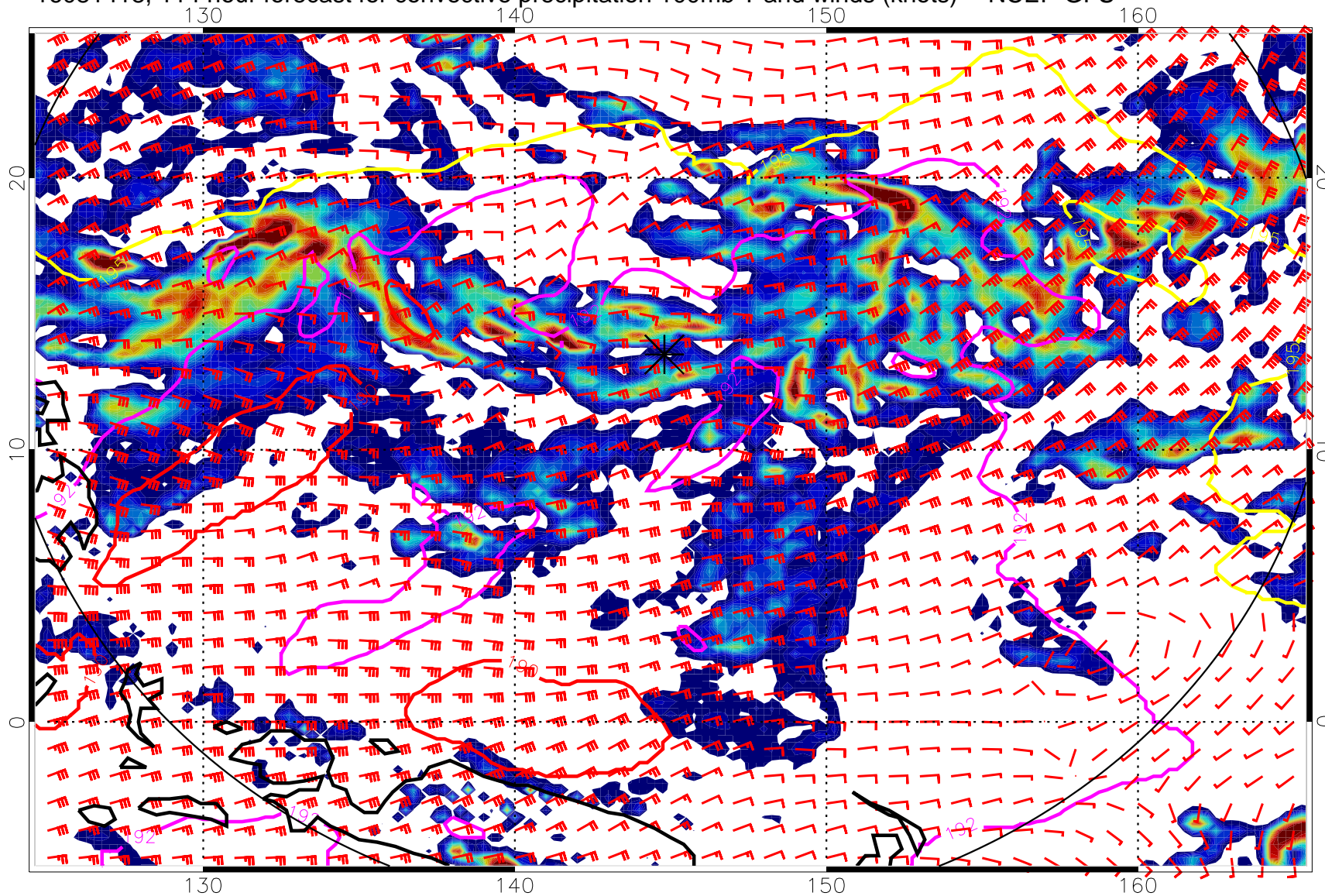
16081418, 114 hour forecast for convective precipitation 100mb T and winds (knots) -- NCEP GFS
