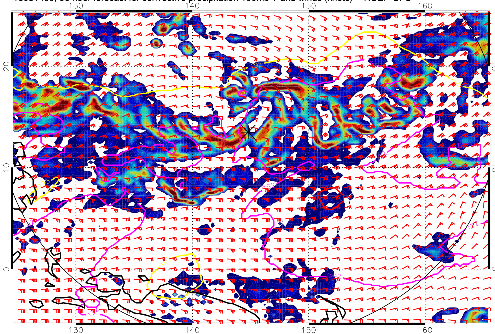
16081400, 96 hour forecast for convective precipitation 100mb T and winds (knots) -- NCEP GFS
