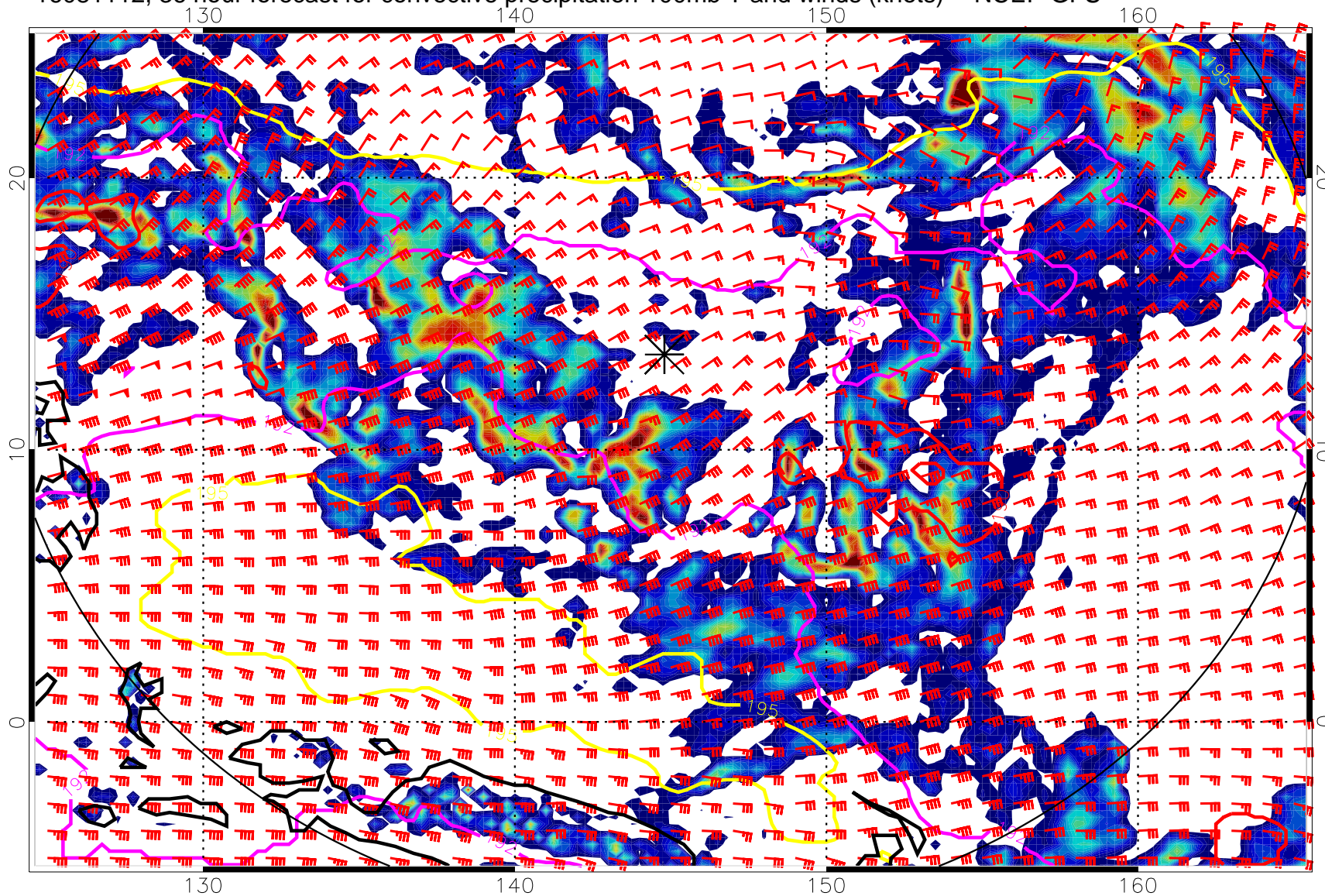
16081112, 36 hour forecast for convective precipitation 100mb T and winds (knots) -- NCEP GFS
