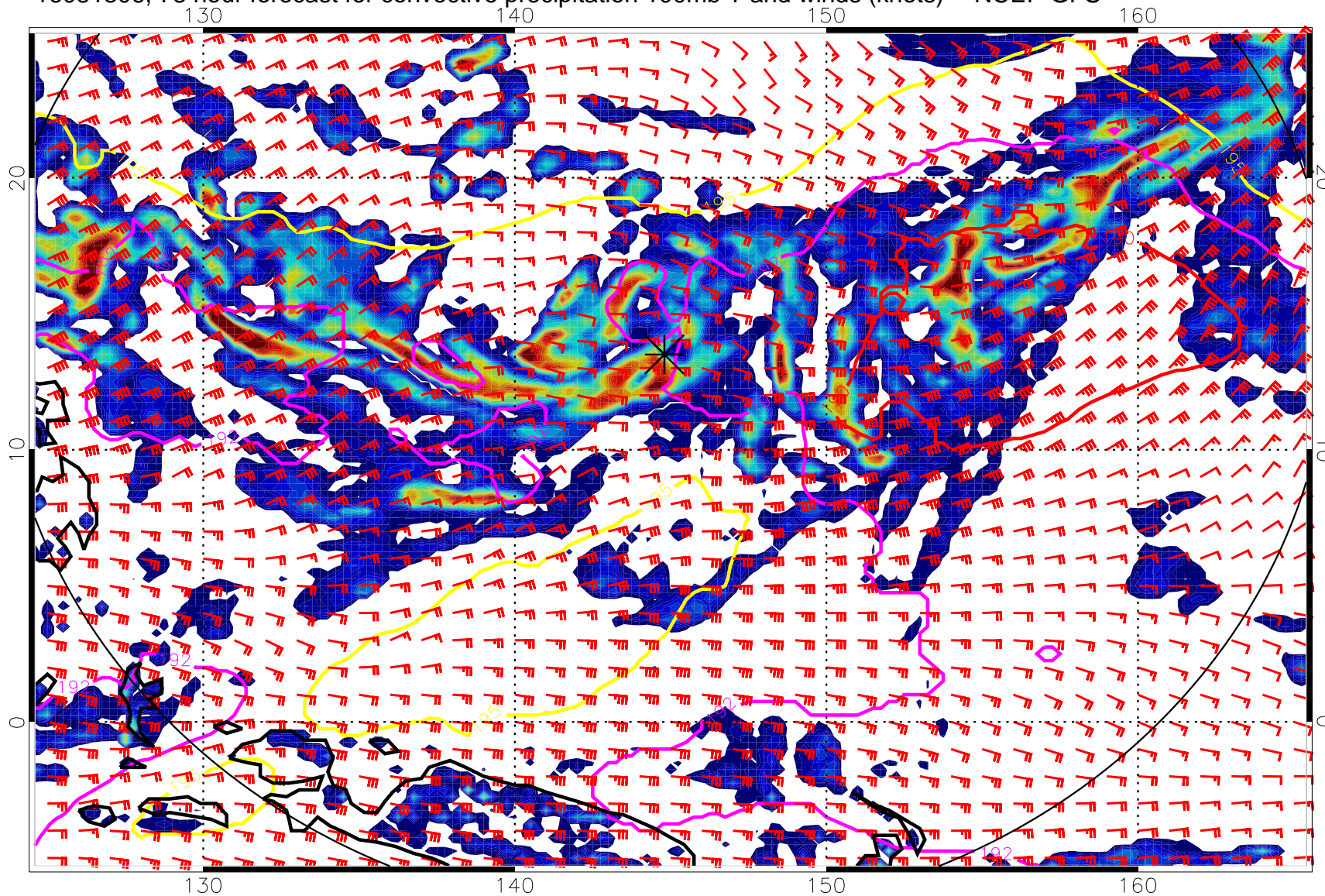
16081306, 78 hour forecast for convective precipitation 100mb T and winds (knots) -- NCEP GFS
