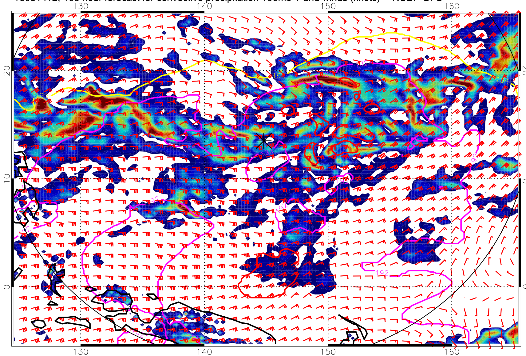
16081412, 108 hour forecast for convective precipitation 100mb T and winds (knots) -- NCEP GFS
