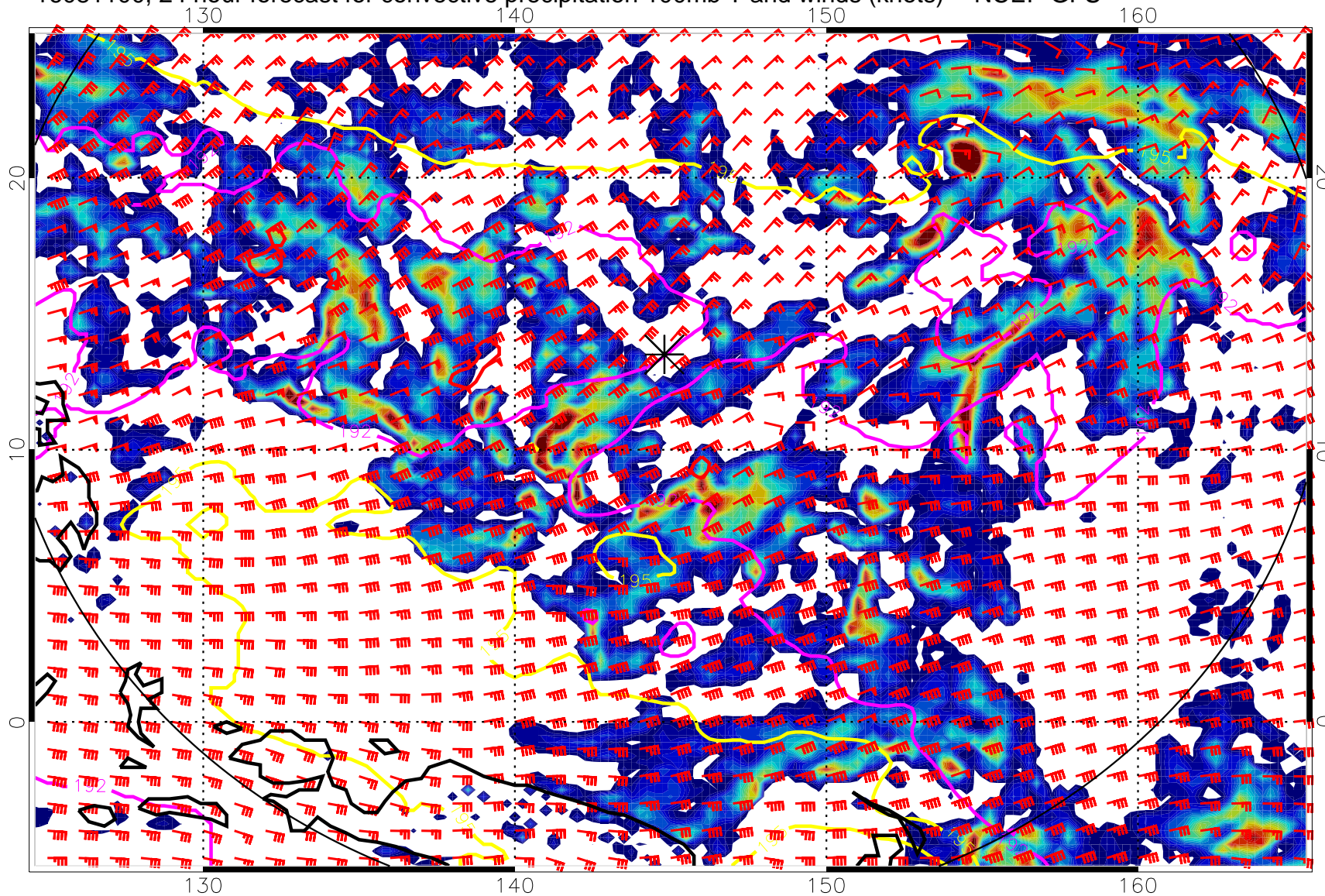
16081100, 24 hour forecast for convective precipitation 100mb T and winds (knots) -- NCEP GFS
