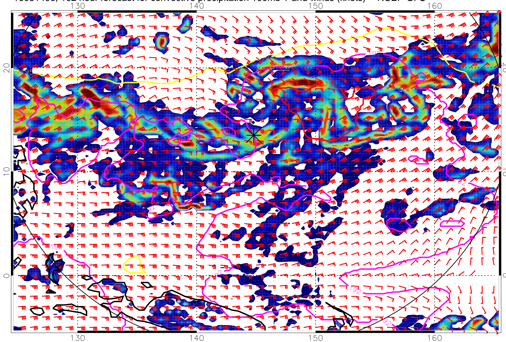
16081406, 102 hour forecast for convective precipitation 100mb T and winds (knots) -- NCEP GFS
