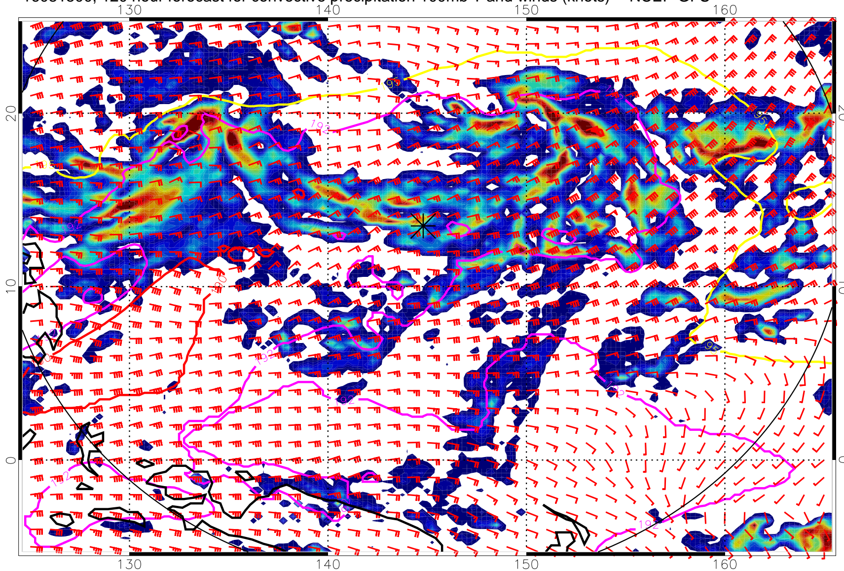
16081500, 120 hour forecast for convective precipitation 100mb T and winds (knots) -- NCEP GFS
