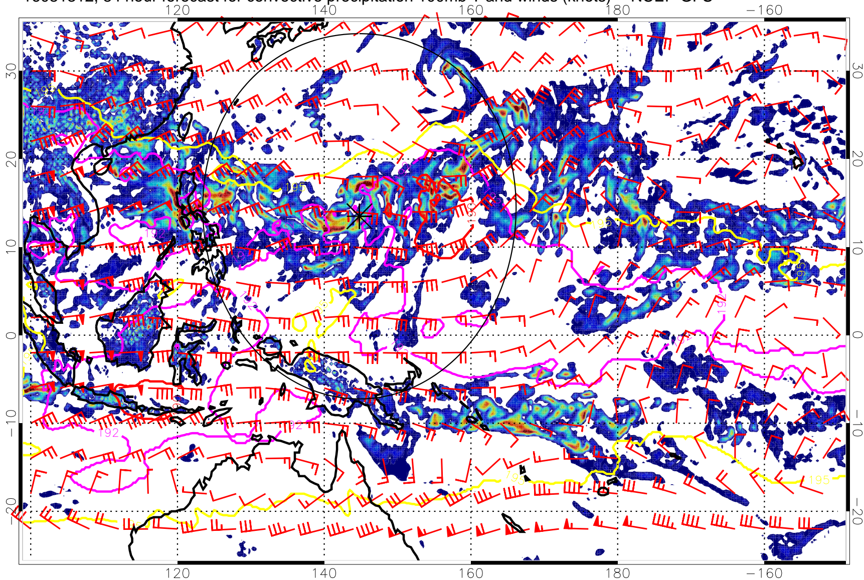
16081312, 84 hour forecast for convective precipitation 100mb T and winds (knots) -- NCEP GFS
