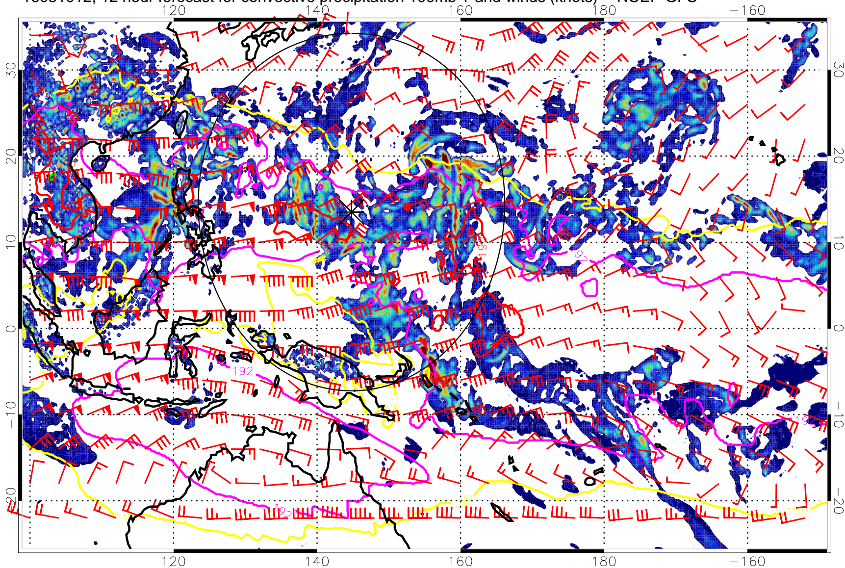
16081012, 12 hour forecast for convective precipitation 100mb T and winds (knots) -- NCEP GFS
