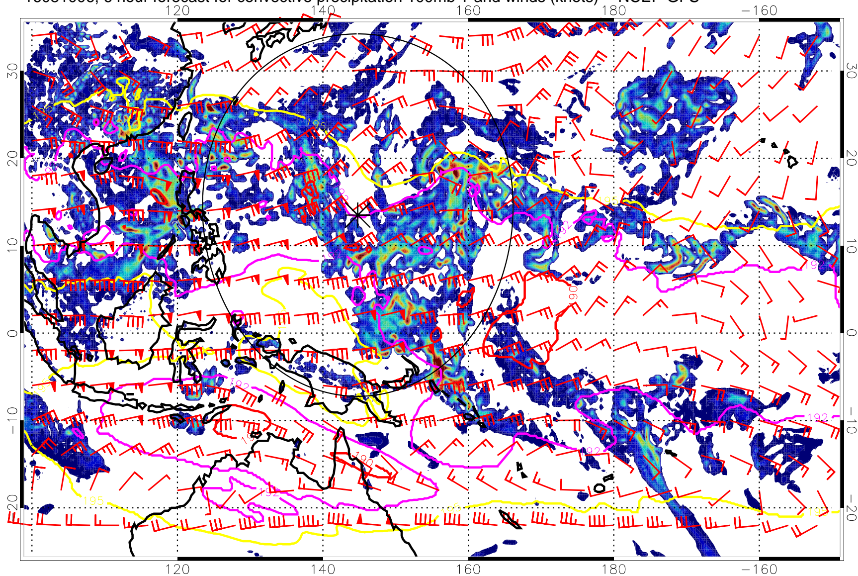
16081006, 6 hour forecast for convective precipitation 100mb T and winds (knots) -- NCEP GFS
